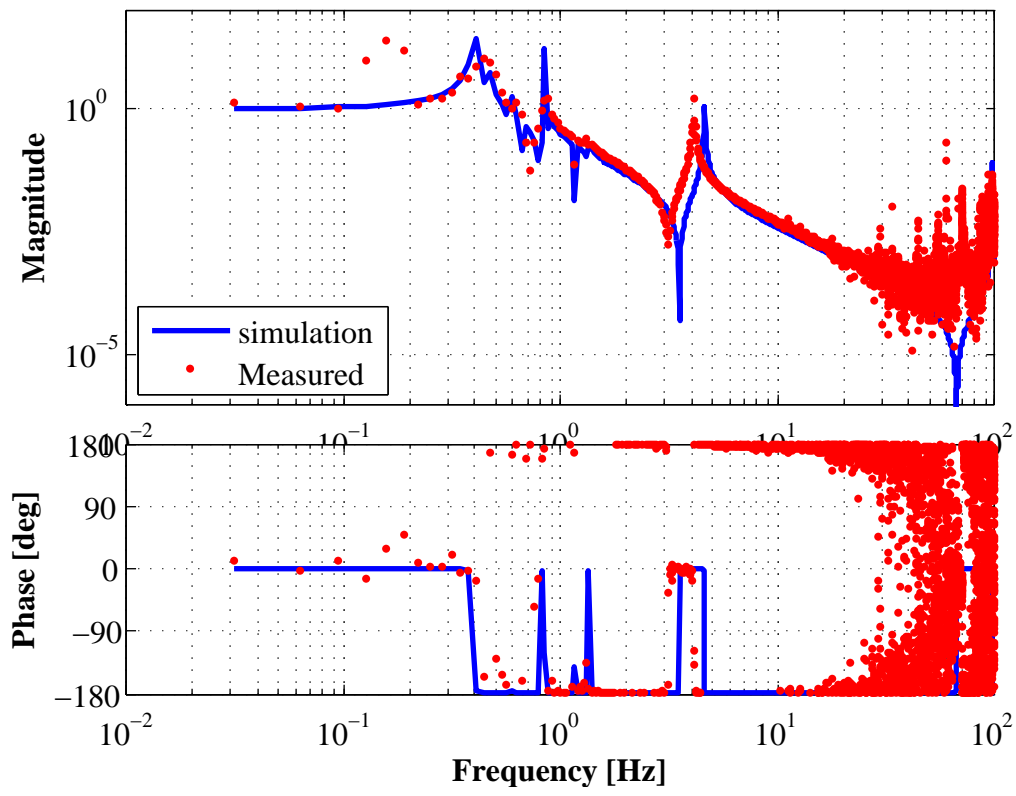
Transfer Function from actPIM to OSEM_PIM
