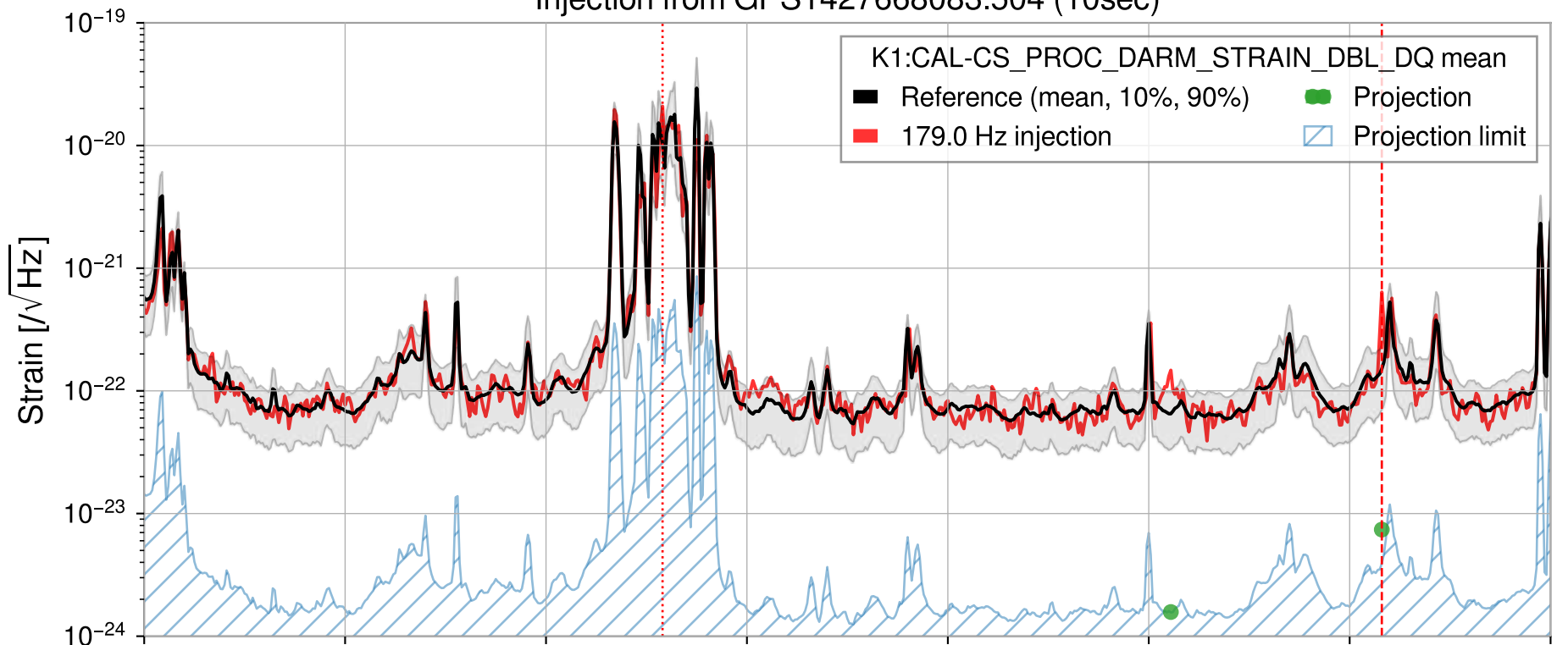
Injection from GPS1427668083.504 (10sec)
