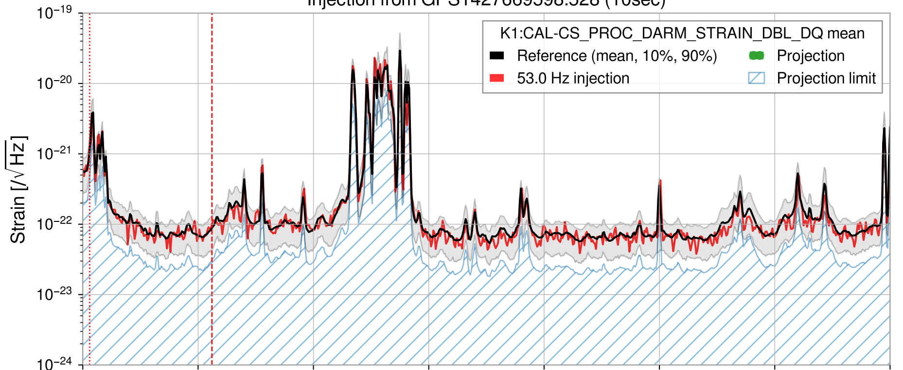
Injection from GPS1427669598.528 (10sec)
