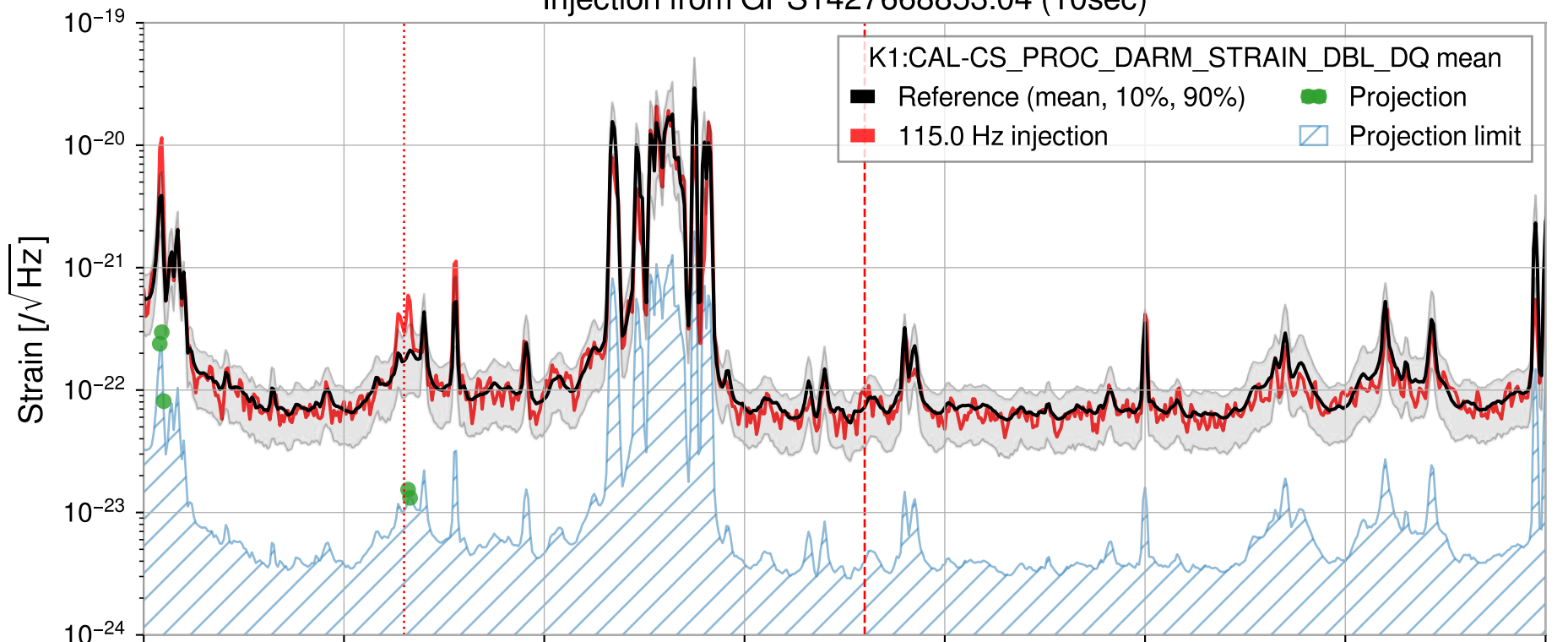
Injection from GPS1427668853.04 (10sec)
