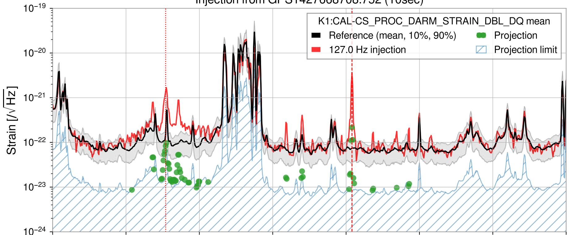
Injection from GPS1427668708.752 (10sec)
