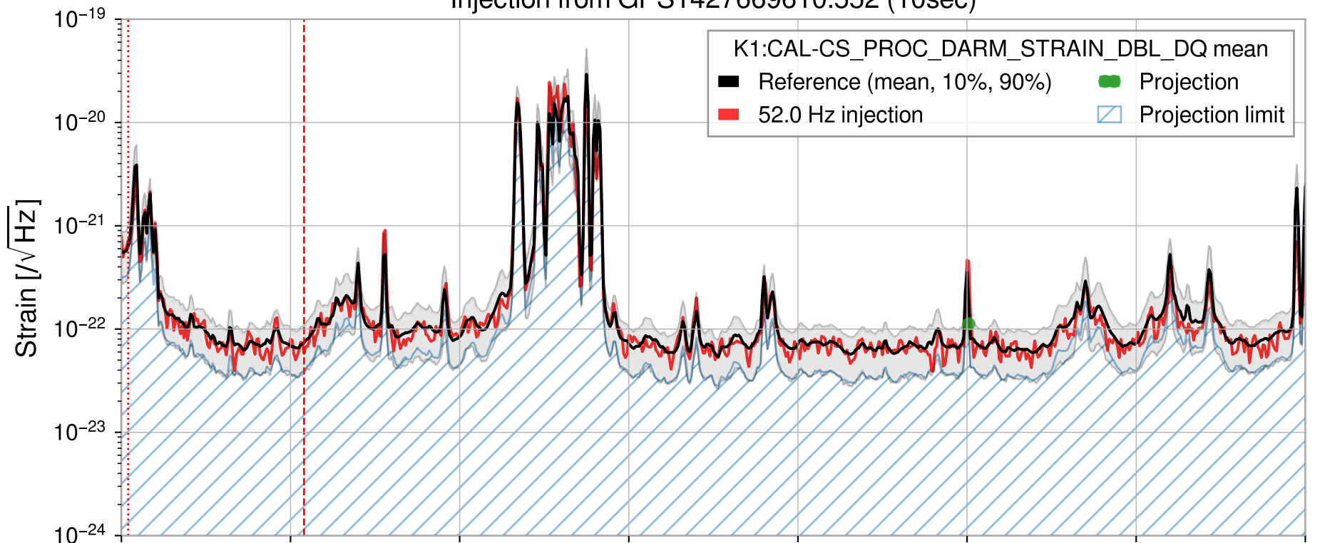
Injection from GPS1427669610.552 (10sec)
