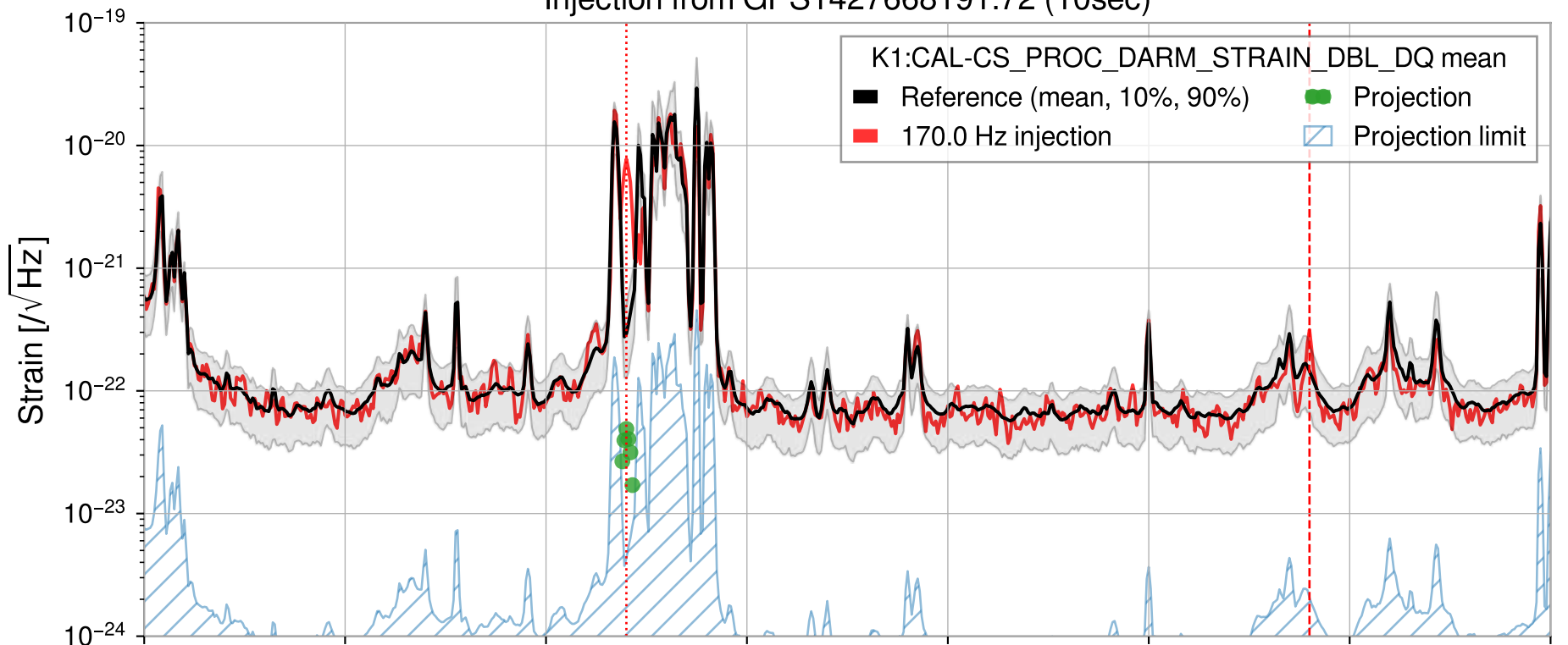
Injection from GPS1427668191.72 (10sec)
