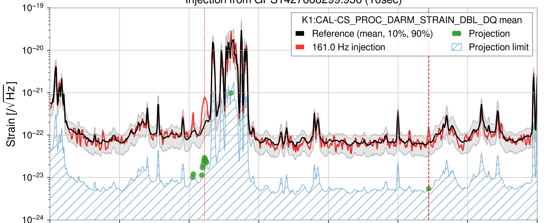
Injection from GPS1427668299.936 (10sec)
