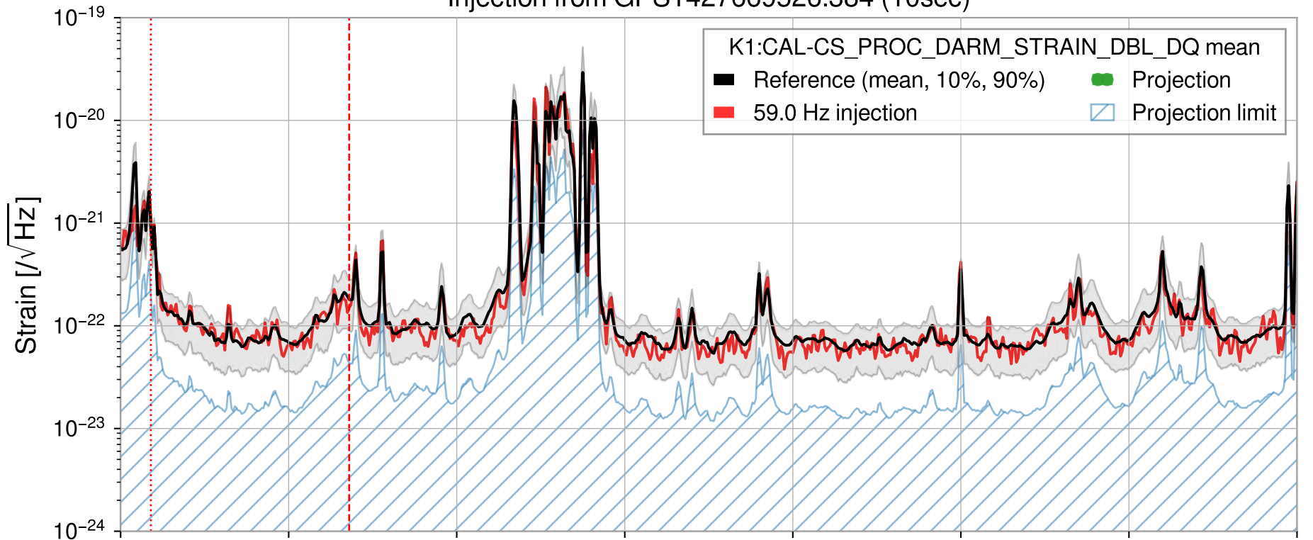
Injection from GPS1427669526.384 (10sec)
