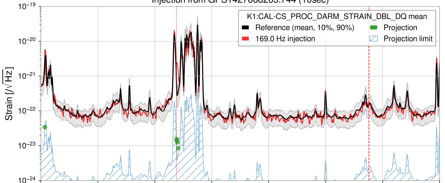
Injection from GPS1427668203.744 (10sec)
