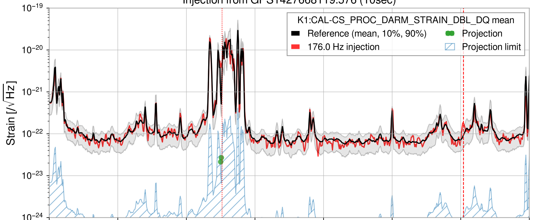
Injection from GPS1427668119.576 (10sec)
