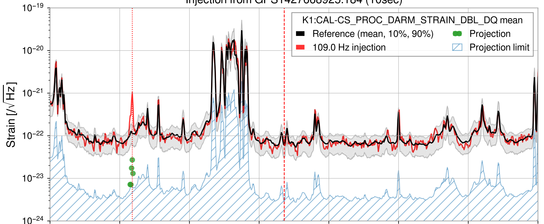
Injection from GPS1427668925.184 (10sec)
