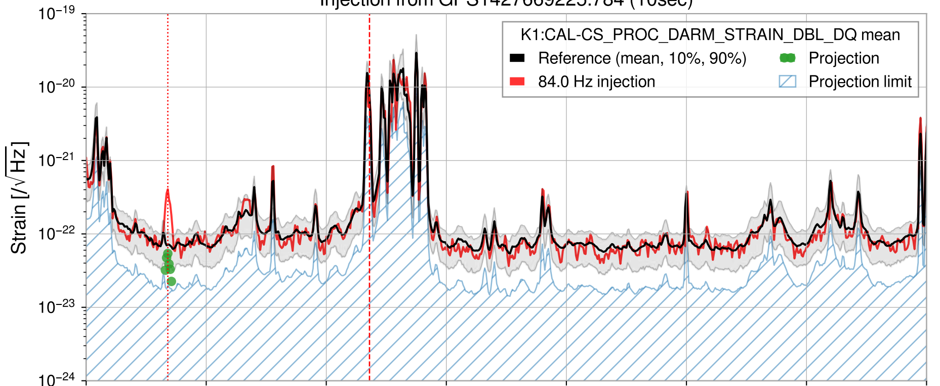
Injection from GPS1427669225.784 (10sec)
