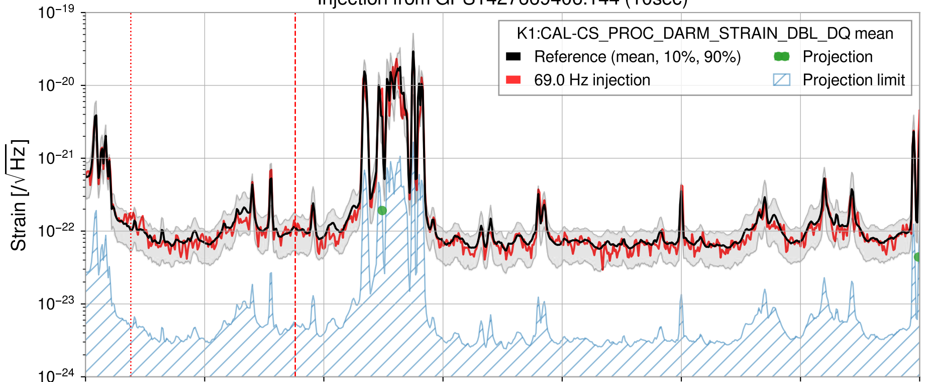
Injection from GPS1427669406.144 (10sec)
