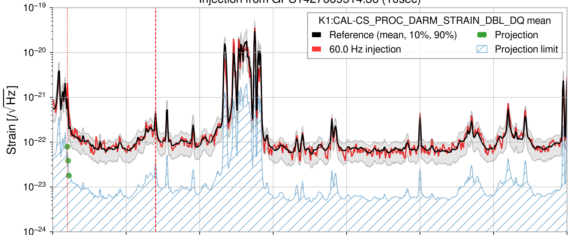
Injection from GPS1427669514.36 (10sec)
