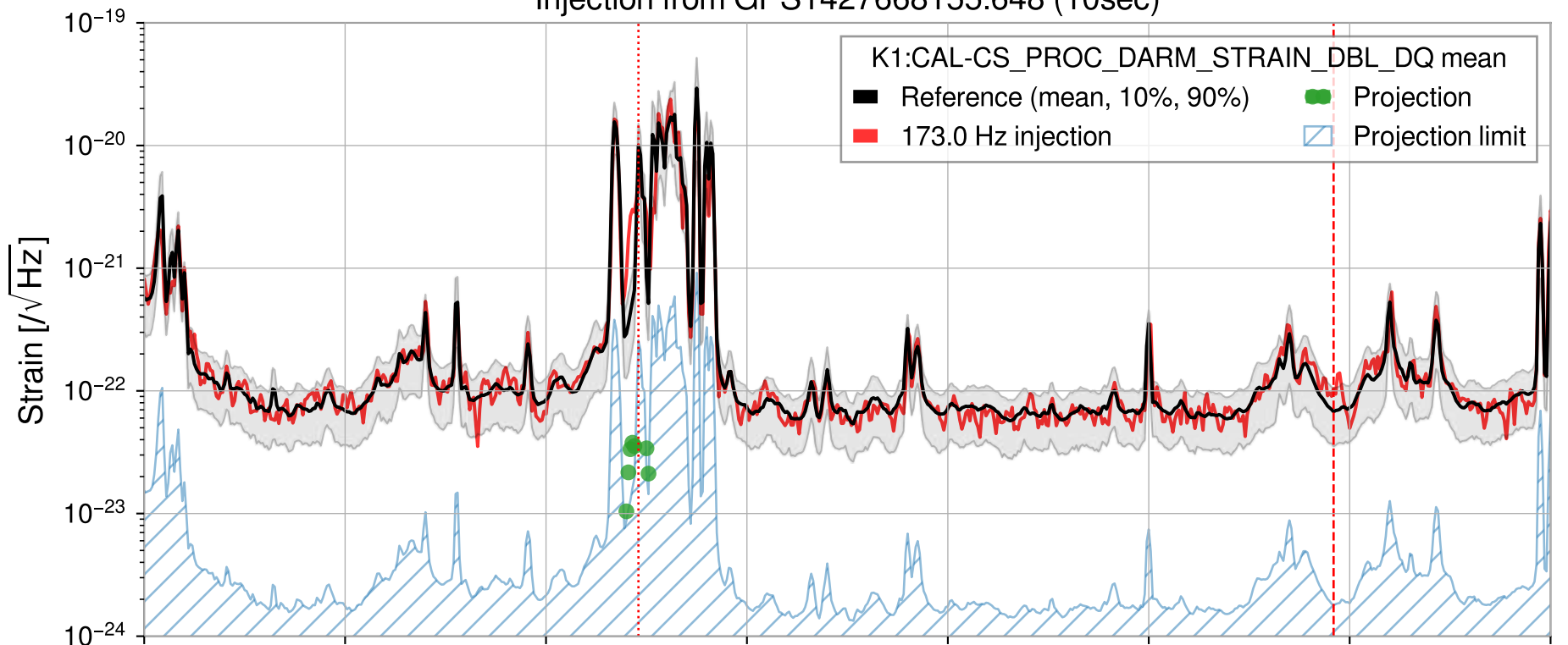
Injection from GPS1427668155.648 (10sec)
