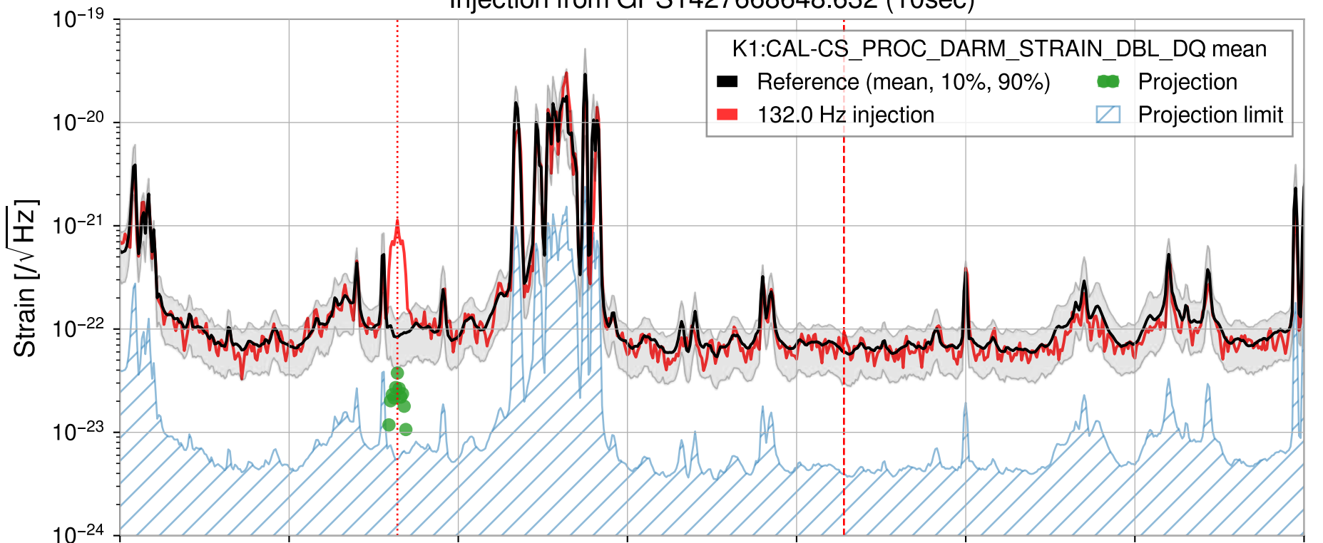
Injection from GPS1427668648.632 (10sec)
