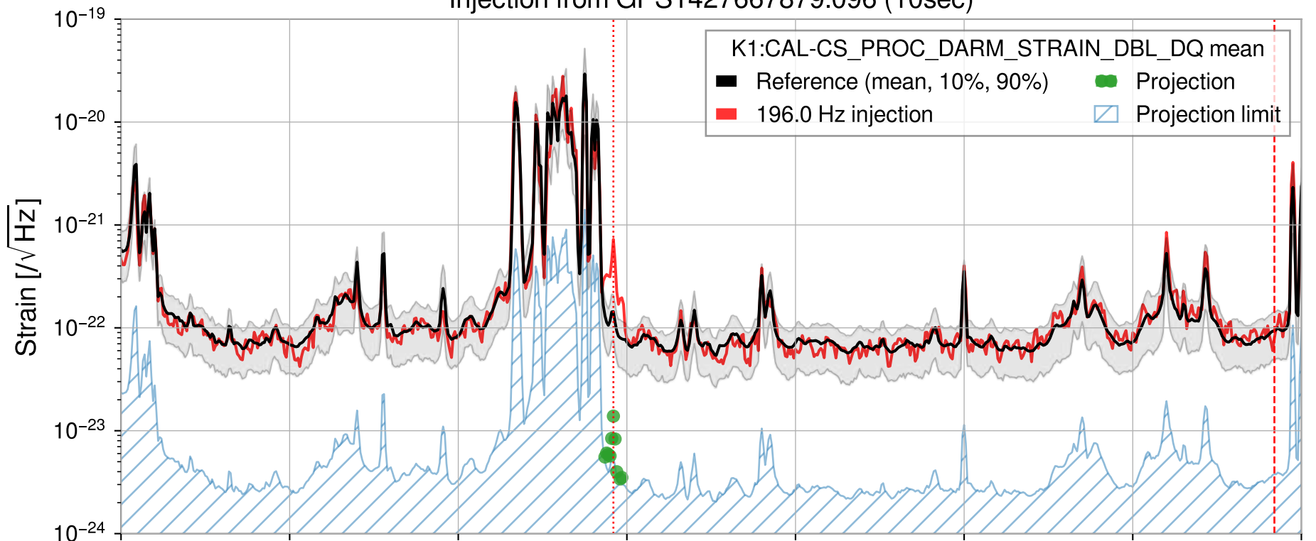
Injection from GPS1427667879.096 (10sec)
