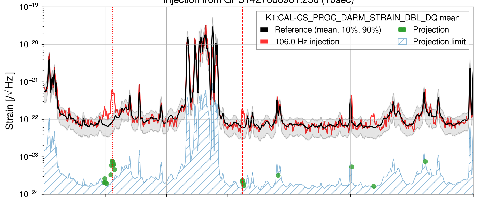
Injection from GPS1427668961.256 (10sec)
