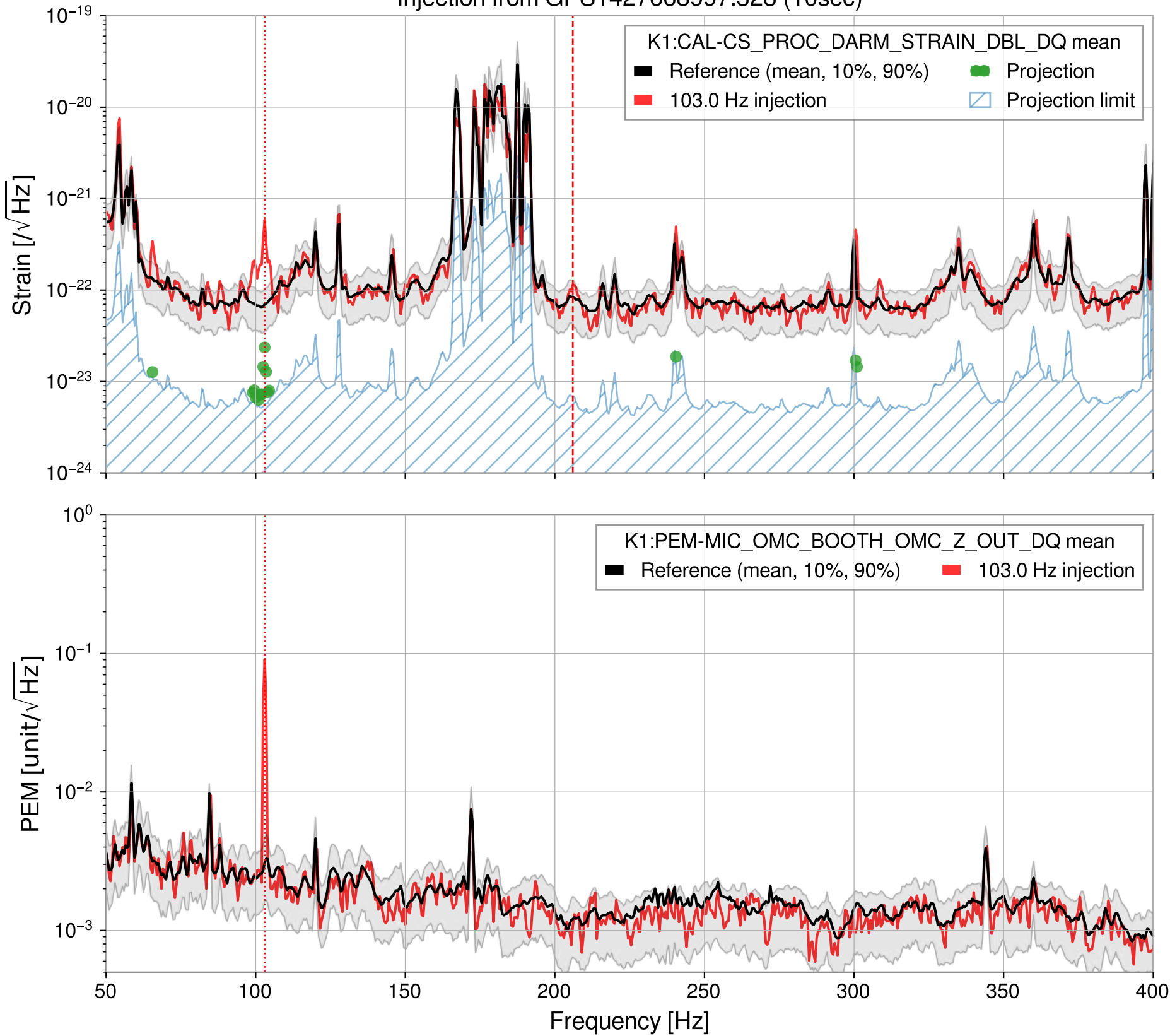
Injection from GPS1427668997.328 (10sec)
