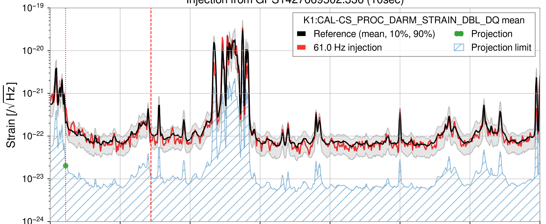
Injection from GPS1427669502.336 (10sec)
