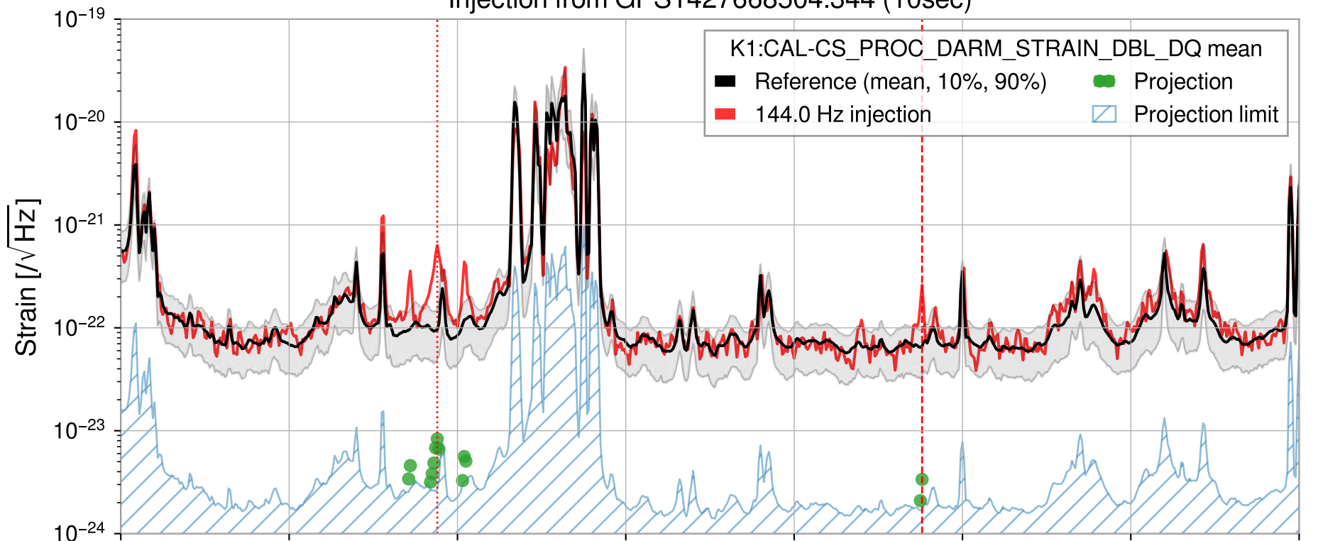
Injection from GPS1427668504.344 (10sec)
