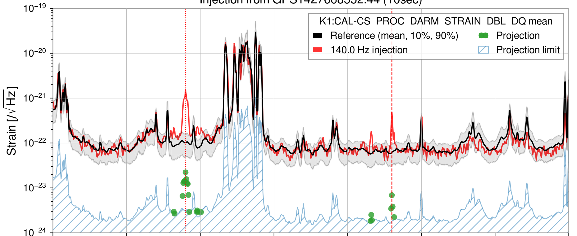
Injection from GPS1427668552.44 (10sec)
