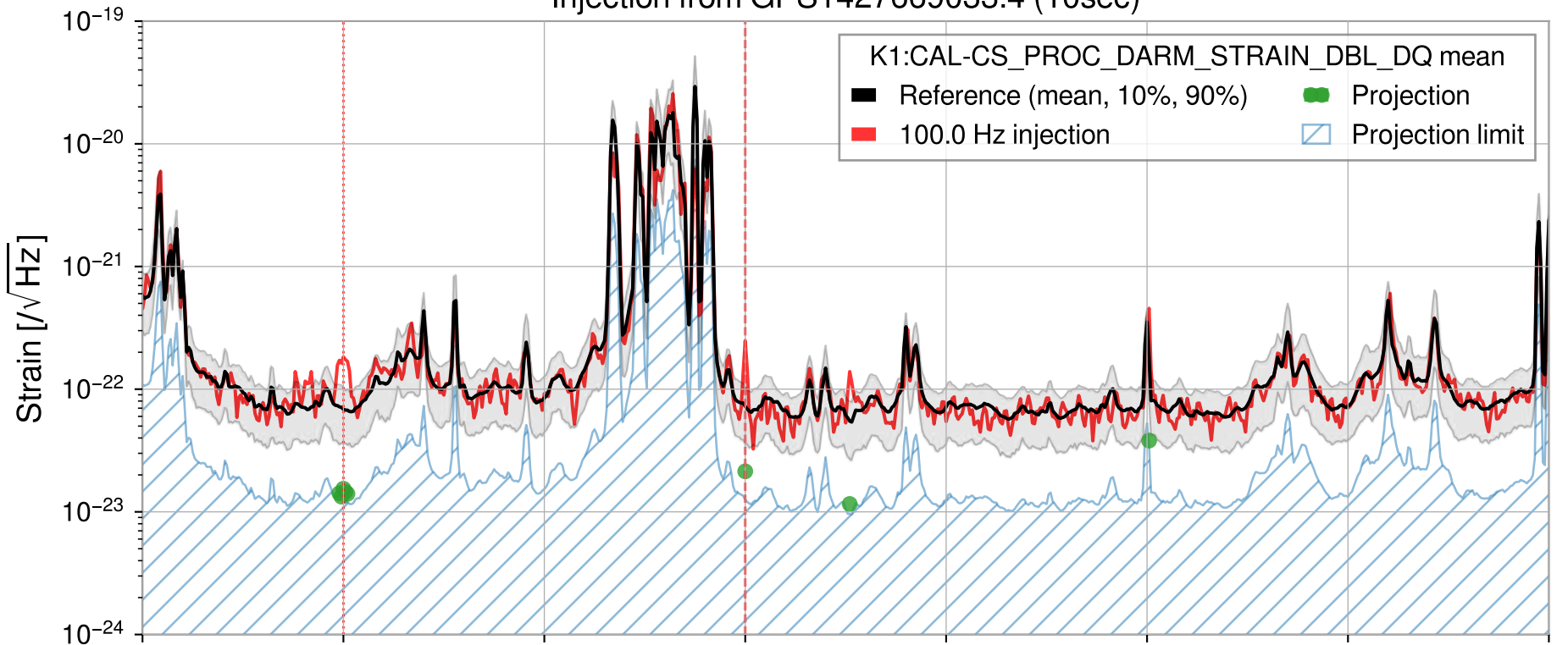
Injection from GPS1427669033.4 (10sec)
