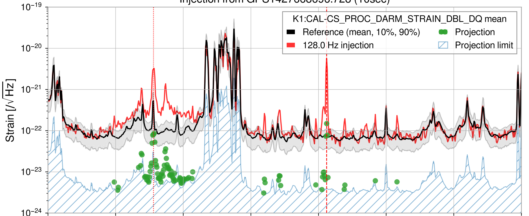
Injection from GPS1427668696.728 (10sec)
