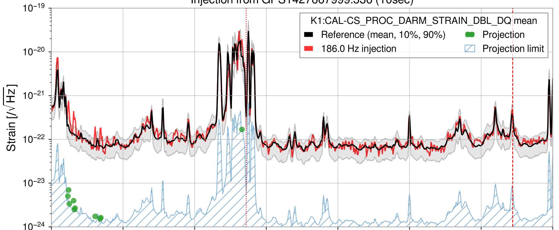
Injection from GPS1427667999.336 (10sec)
