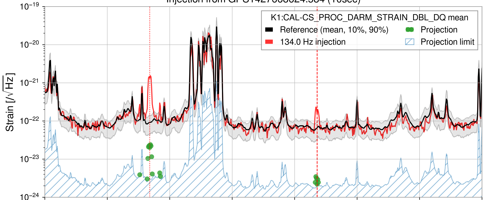
Injection from GPS1427668624.584 (10sec)
