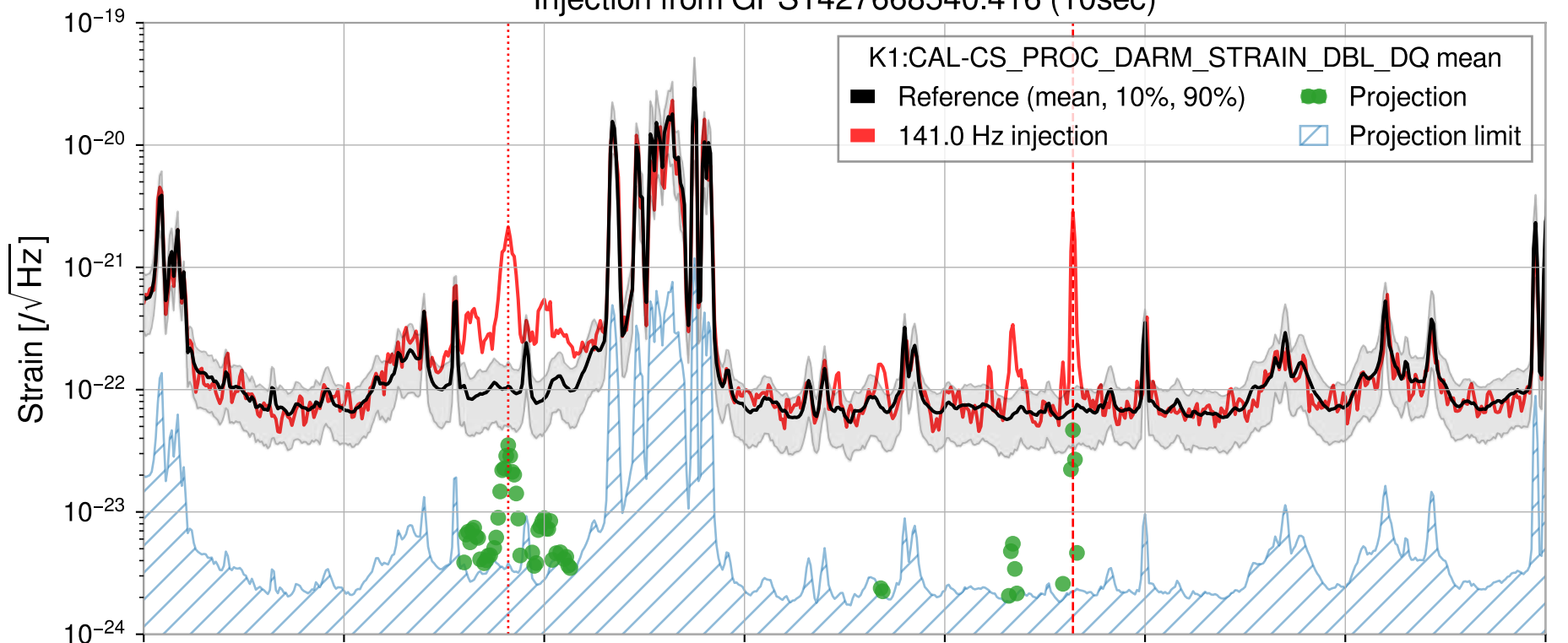
Injection from GPS1427668540.416 (10sec)
