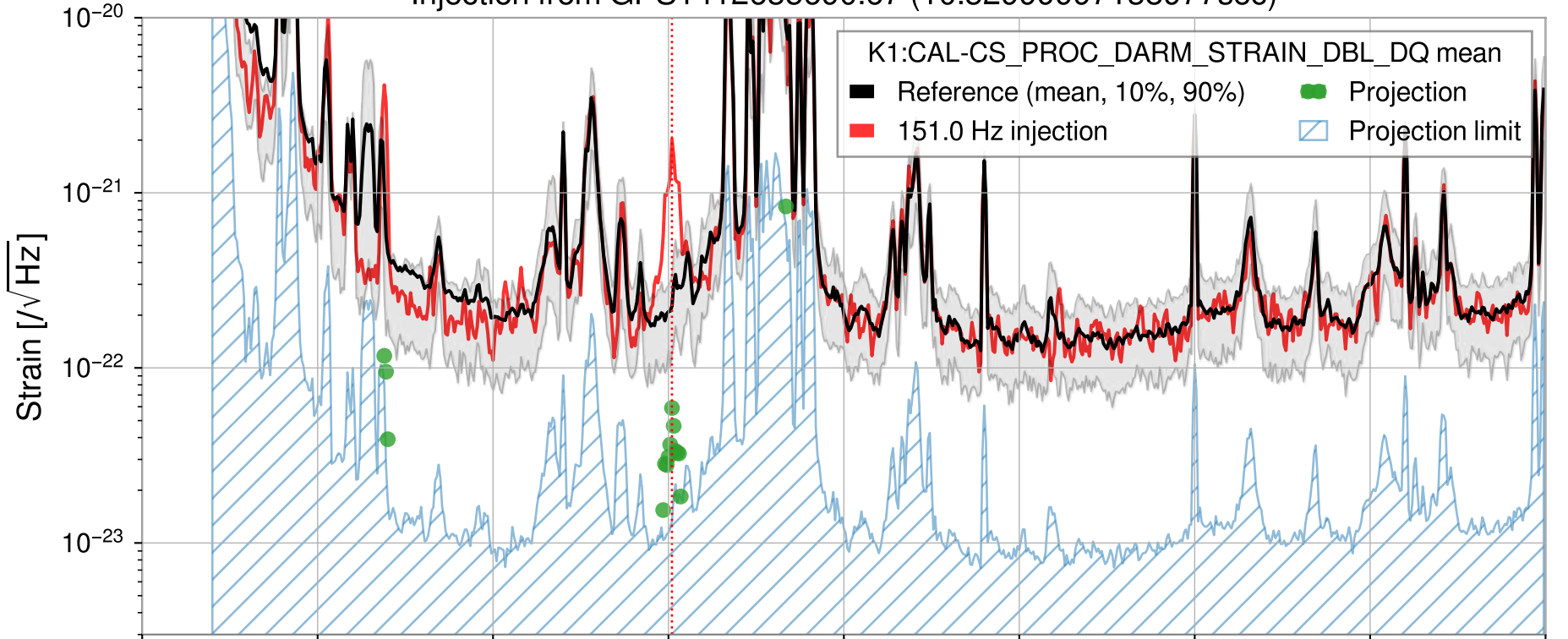
Injection from GPS1412635690.67 (10.52999997138977sec)
