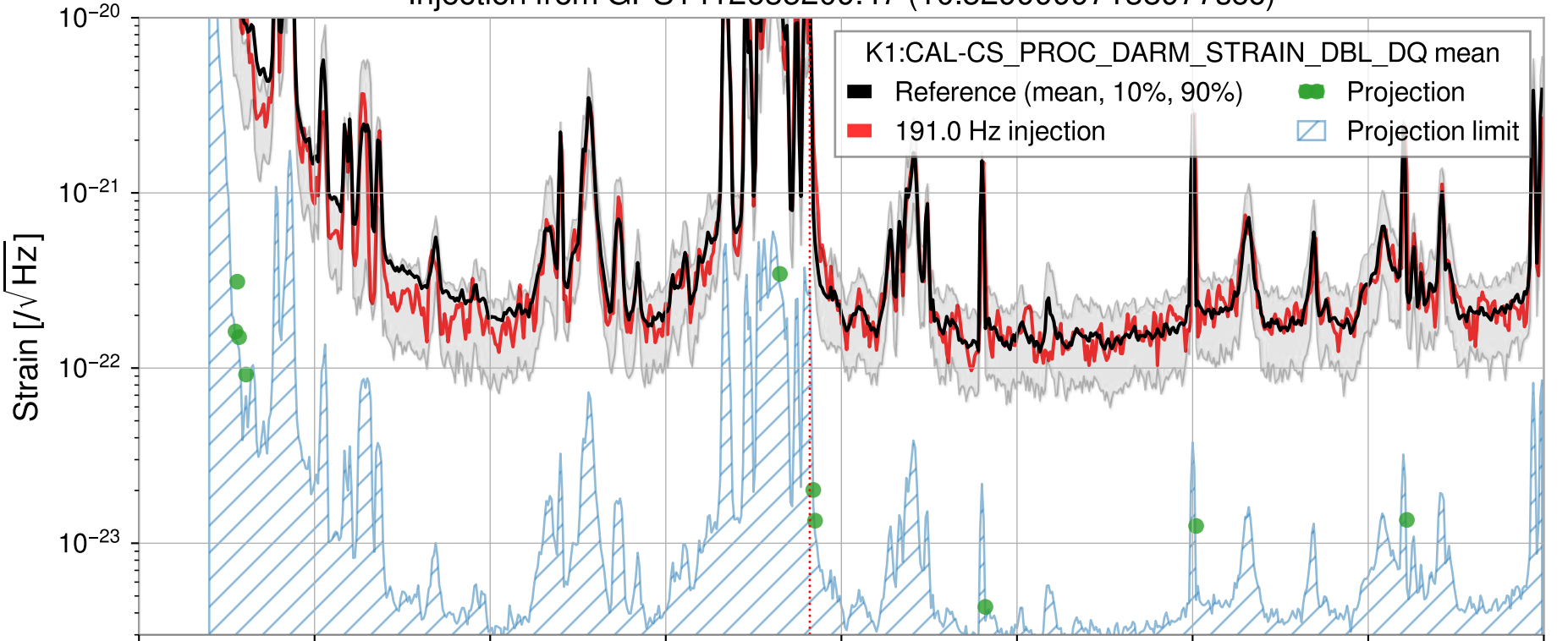
Injection from GPS1412635209.47 (10.52999997138977sec)
