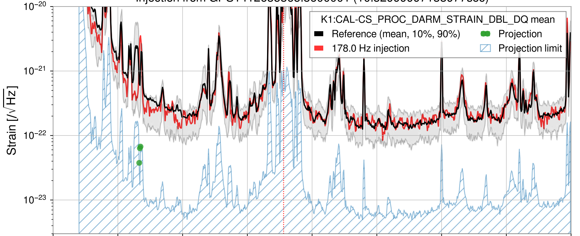
Injection from GPS1412635365.860001 (10.52999997138977sec)
