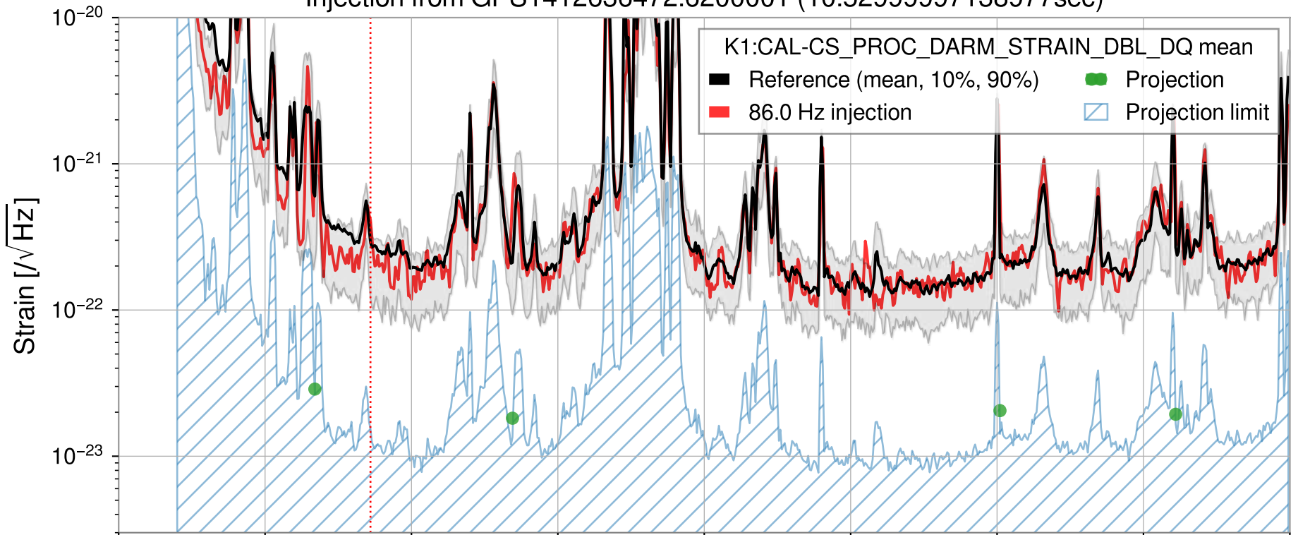
Injection from GPS1412636472.620001 (10.52999997138977sec)
