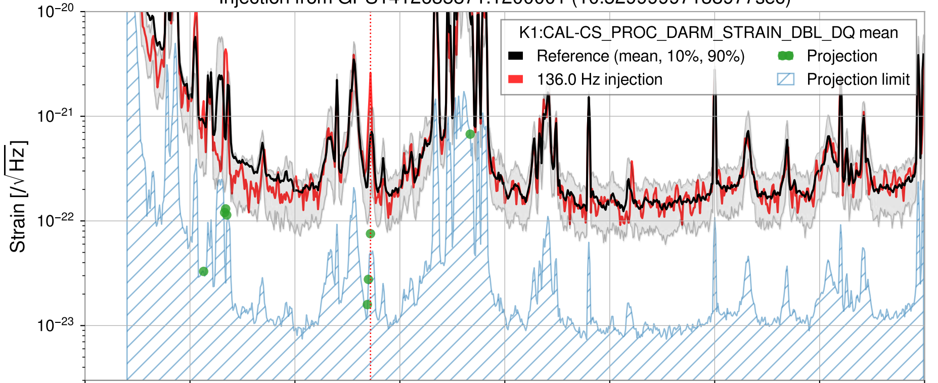
Injection from GPS1412635871.1200001 (10.52999997138977sec)
