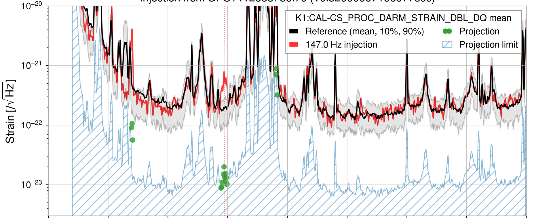
Injection from GPS1412635738.79 (10.52999997138977sec)
