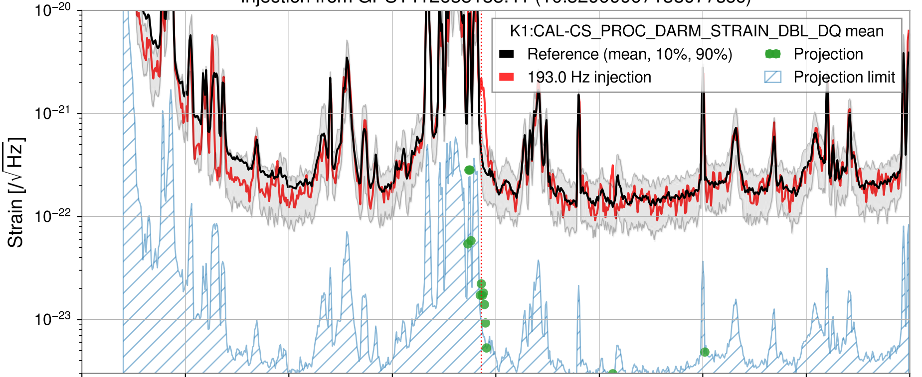
Injection from GPS1412635185.41 (10.52999997138977sec)
