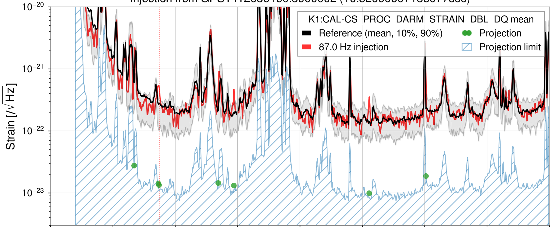
Injection from GPS1412636460.590002 (10.52999997138977sec)
