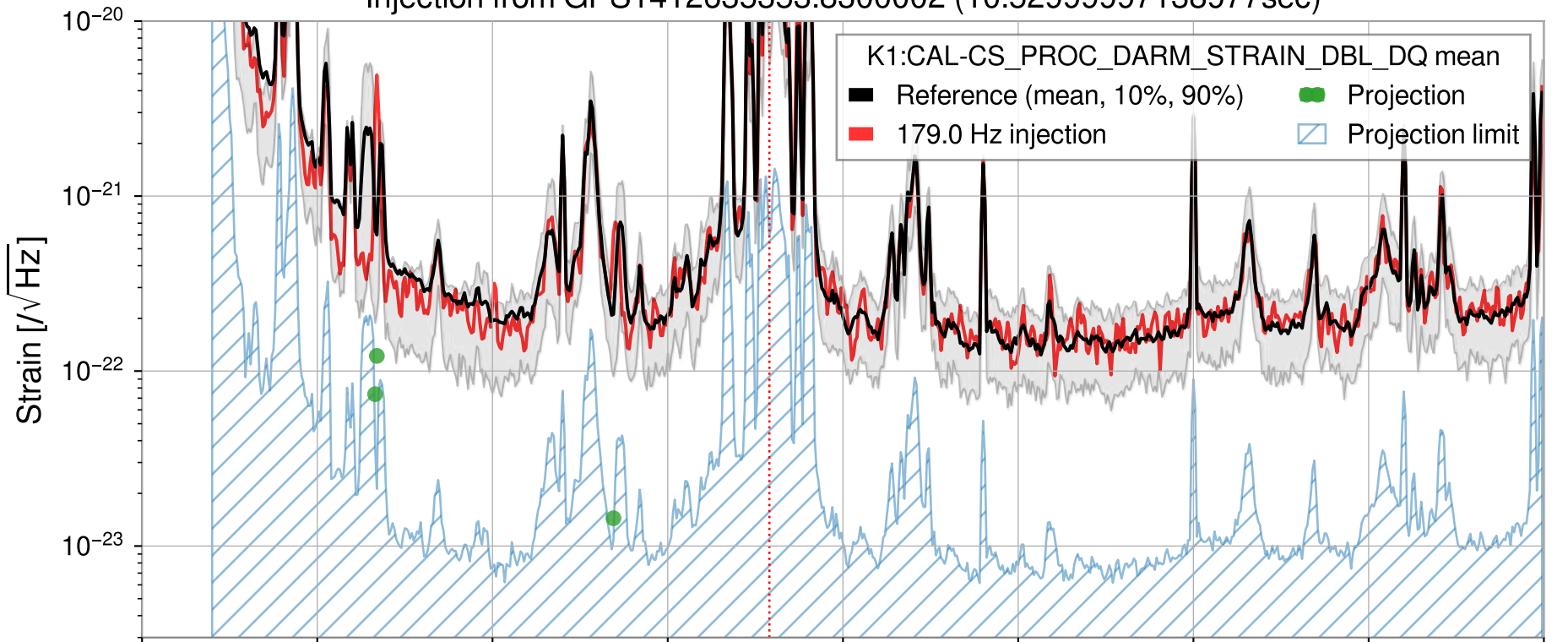
Injection from GPS1412635353.830002 (10.52999997138977sec)
