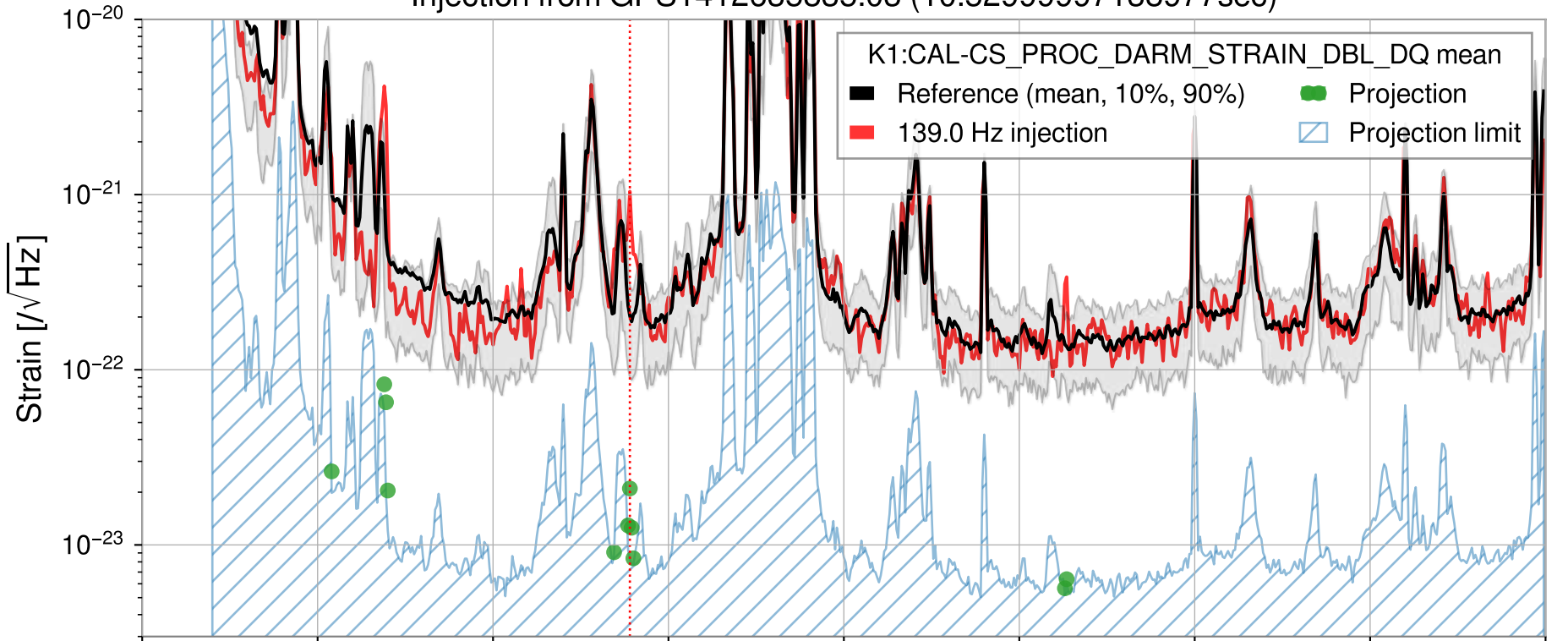
Injection from GPS1412635835.03 (10.52999997138977sec)
