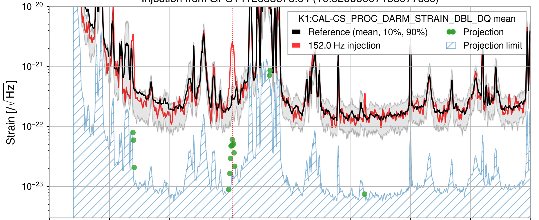
Injection from GPS1412635678.64 (10.52999997138977sec)
