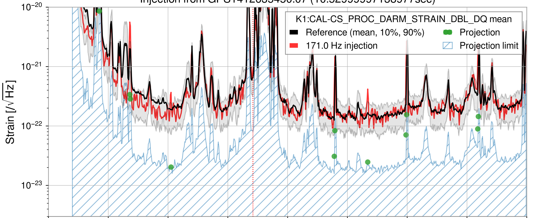
Injection from GPS1412635450.07 (10.52999997138977sec)
