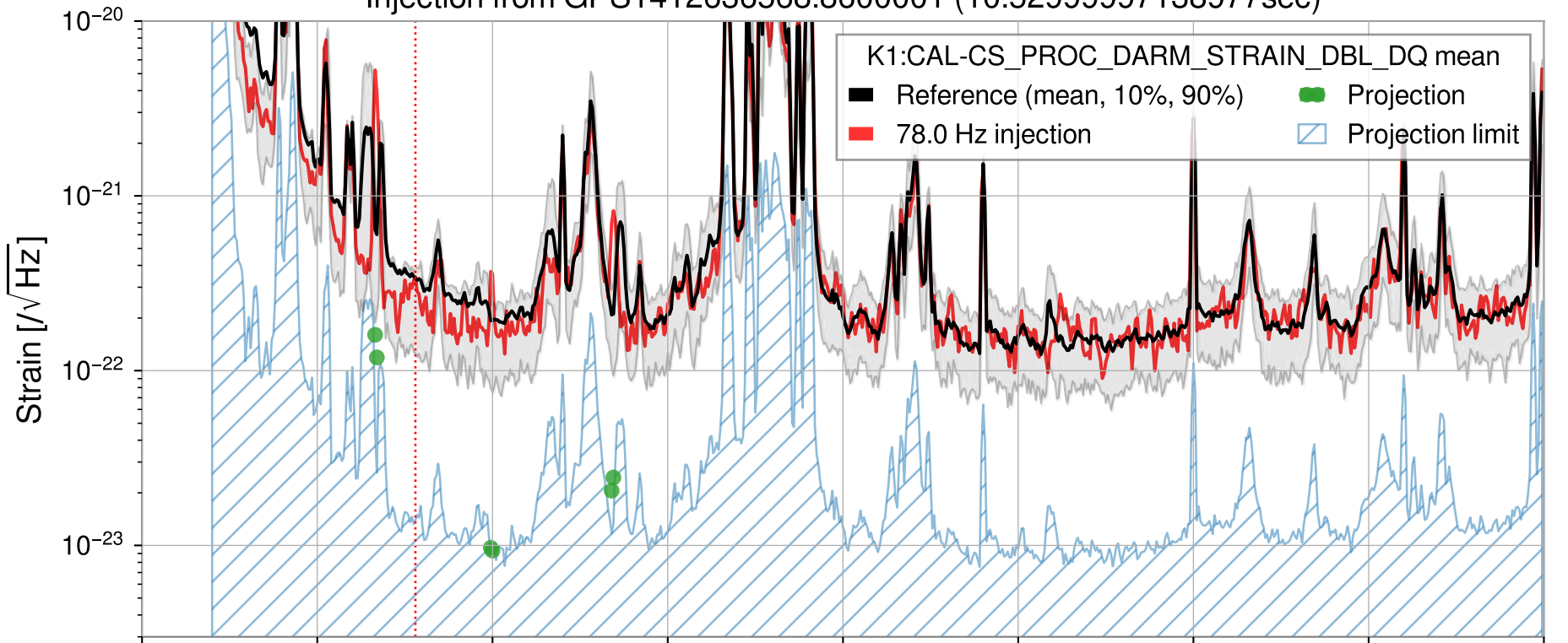
Injection from GPS1412636568.860001 (10.52999997138977sec)
