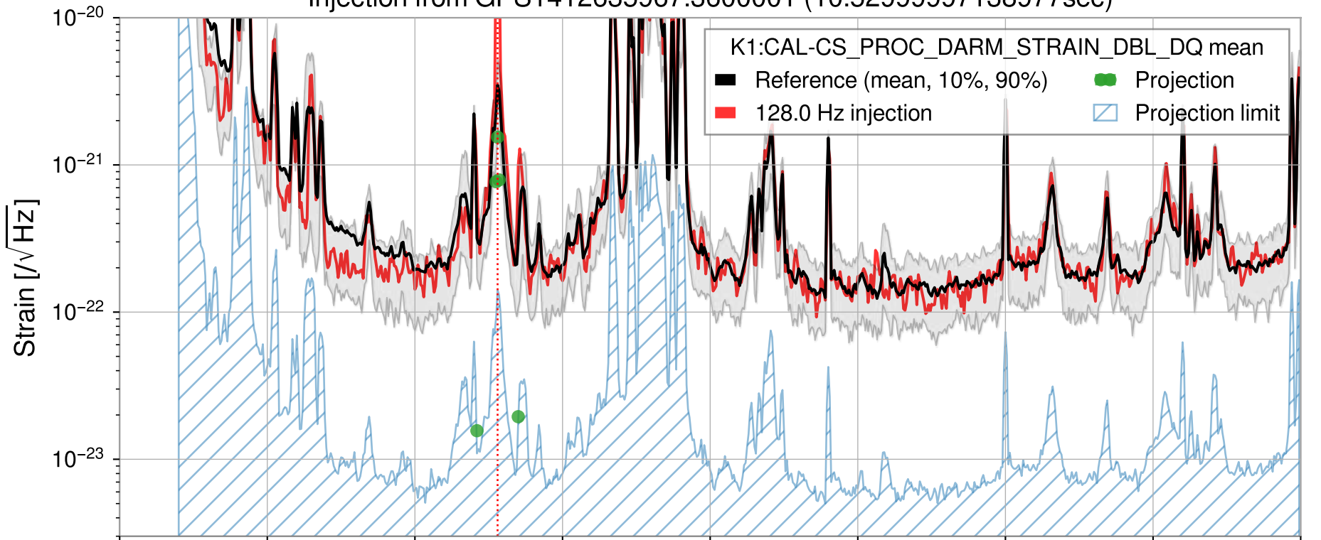
Injection from GPS1412635967.360001 (10.52999997138977sec)
