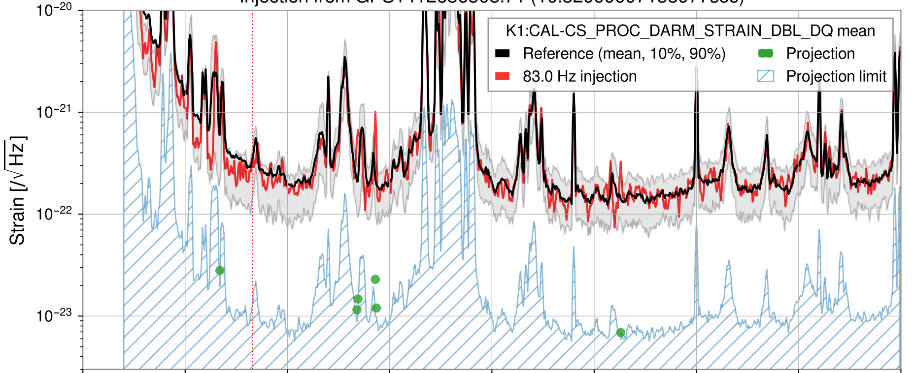
Injection from GPS1412636508.71 (10.52999997138977sec)
