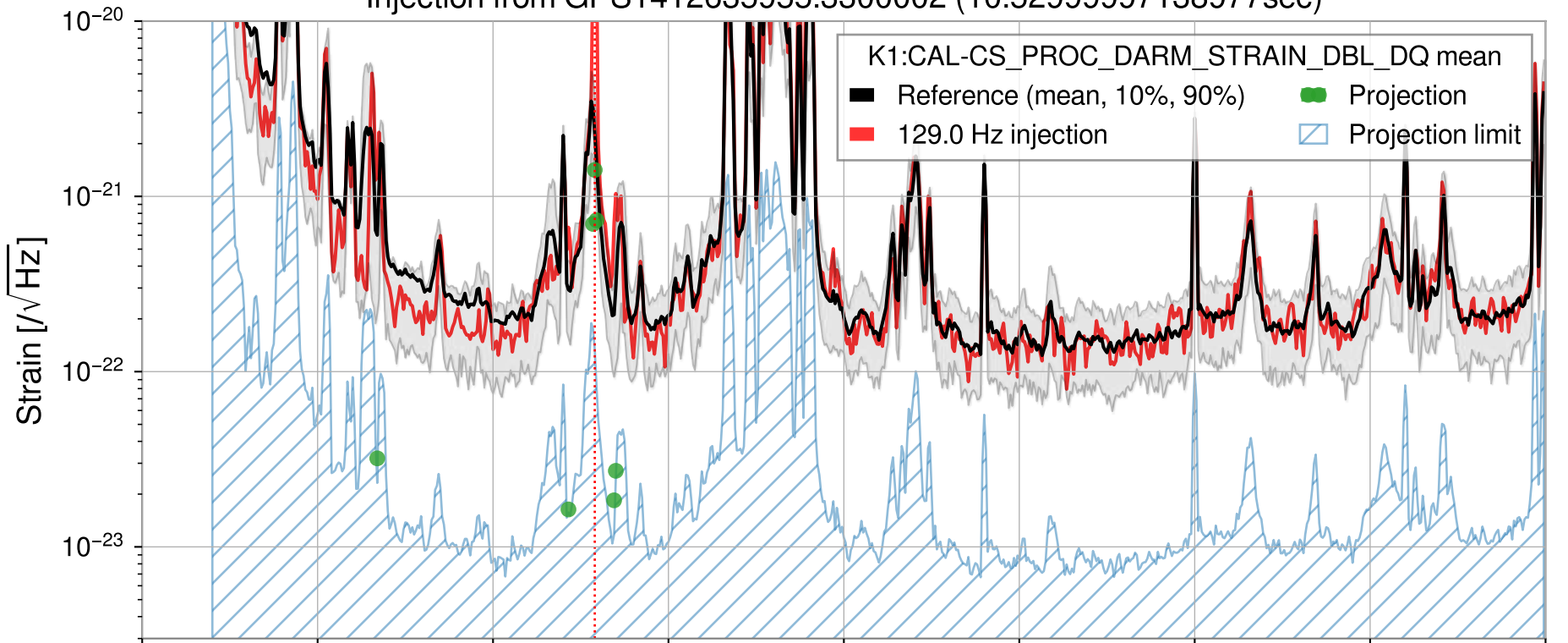
Injection from GPS141263595.330002 (10.52999997138977sec)
