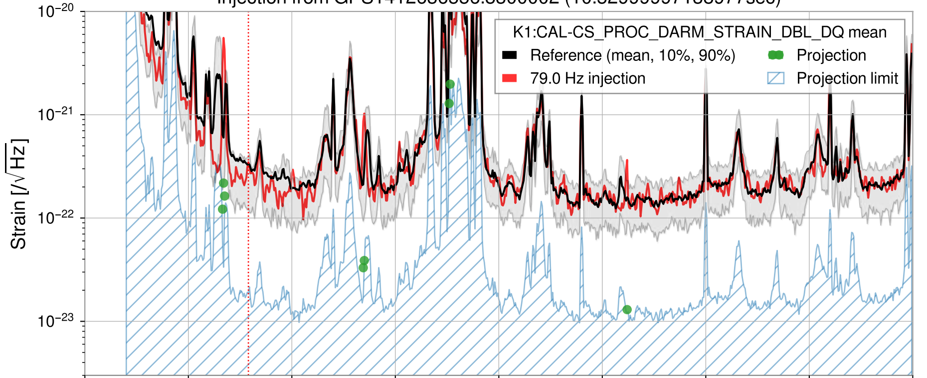
Injection from GPS1412636556.830002 (10.52999997138977sec)
