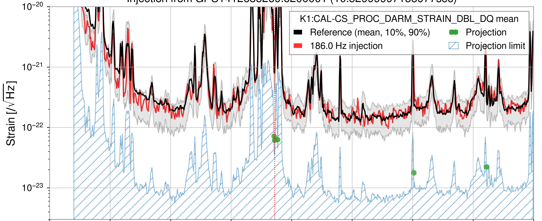
Injection from GPS1412635269.620001 (10.52999997138977sec)
