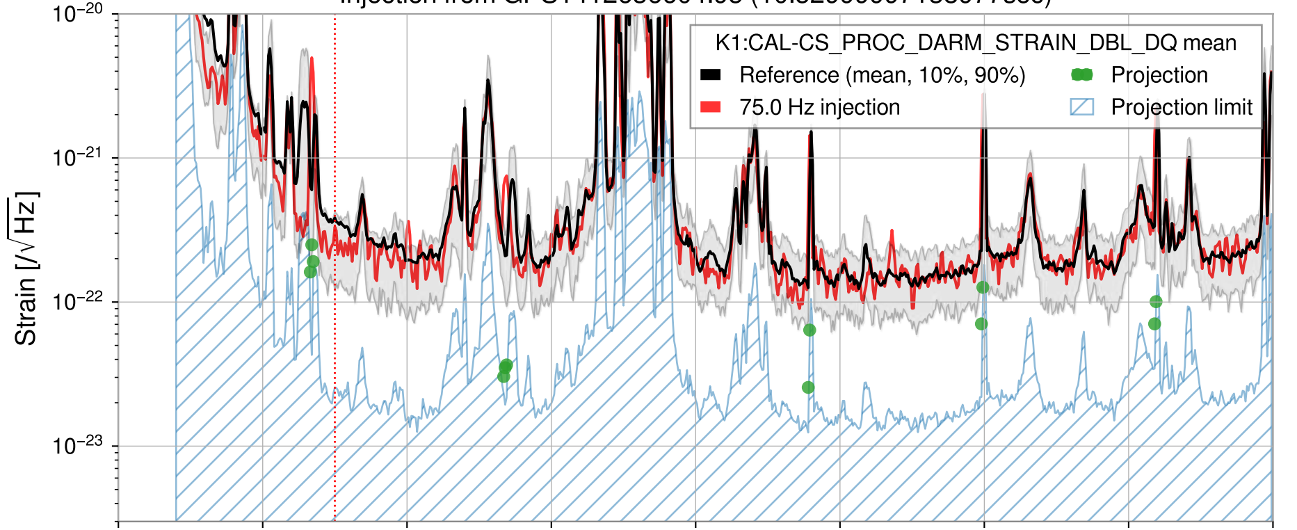
Injection from GPS1412636604.95 (10.52999997138977sec)
