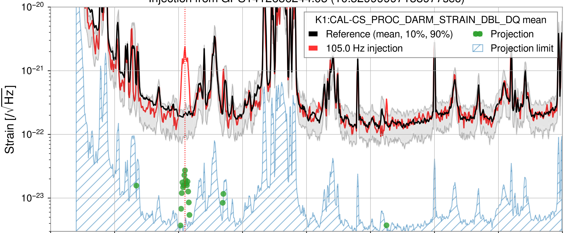
Injection from GPS1412636244.05 (10.52999997138977sec)
