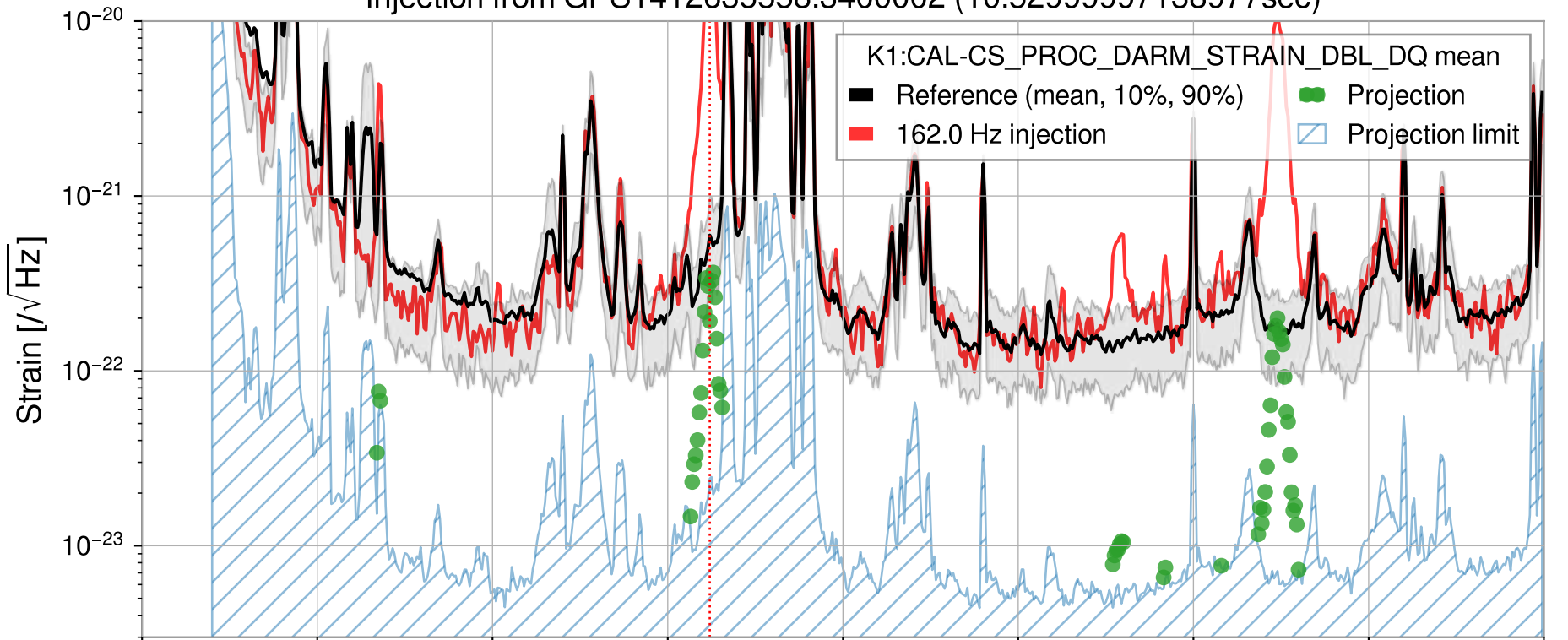
Injection from GPS1412635558.340002 (10.52999997138977sec)
