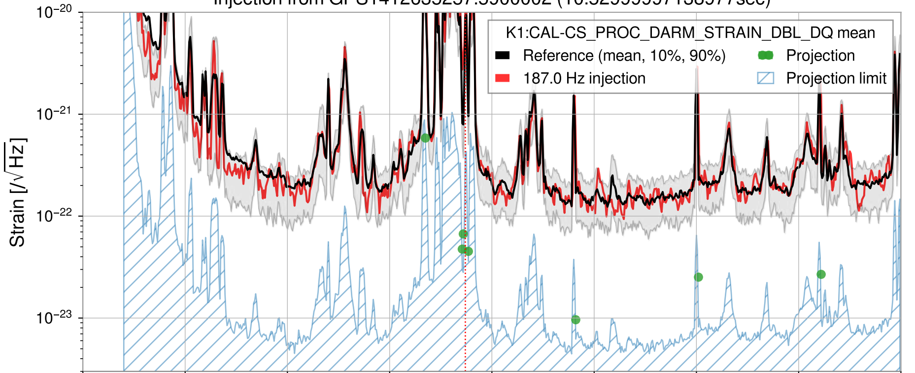
Injection from GPS1412635257.590002 (10.52999997138977sec)
