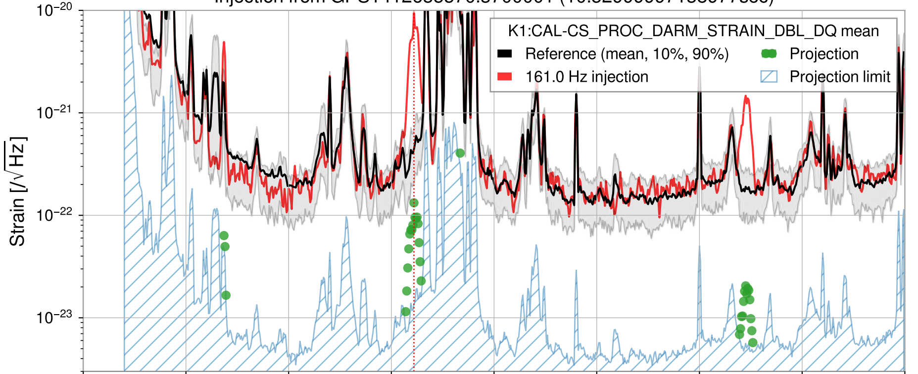
Injection from GPS1412635570.3700001 (10.52999997138977sec)
