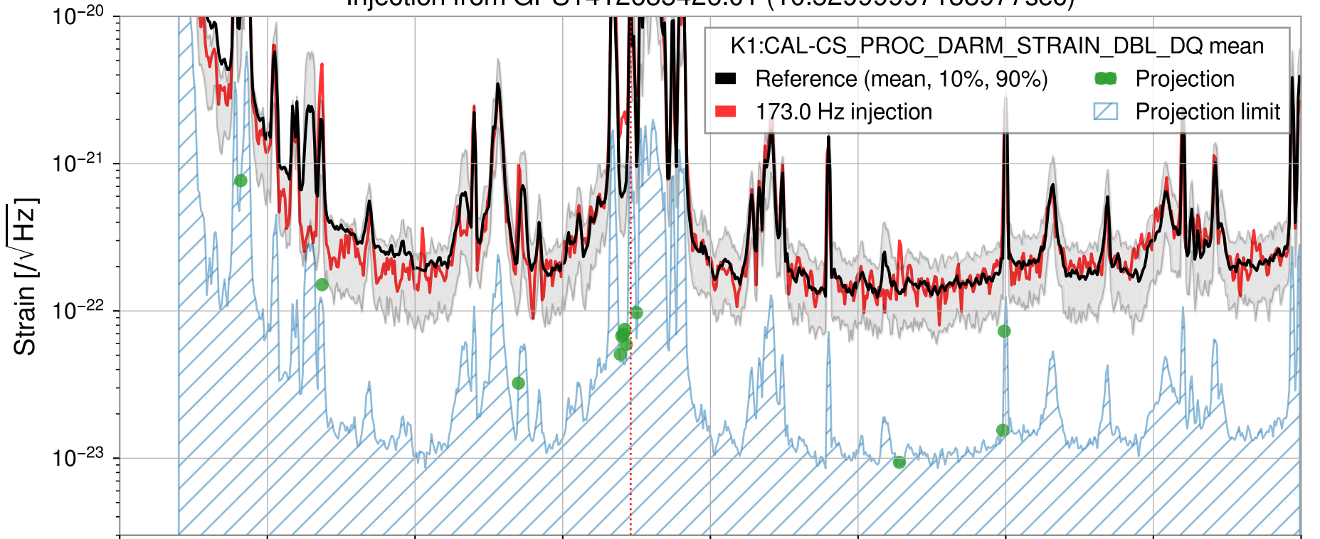
Injection from GPS1412635426.01 (10.52999997138977sec)
