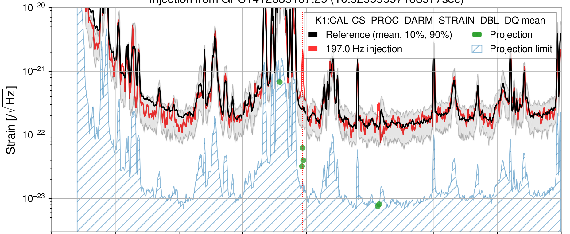
Injection from GPS1412635137.29 (10.52999997138977sec)
