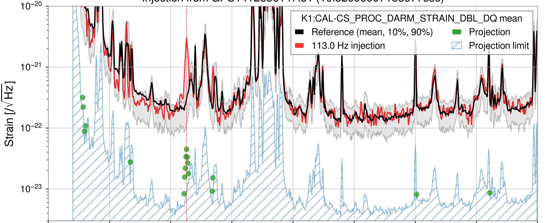
Injection from GPS1412636147.81 (10.52999997138977sec)
