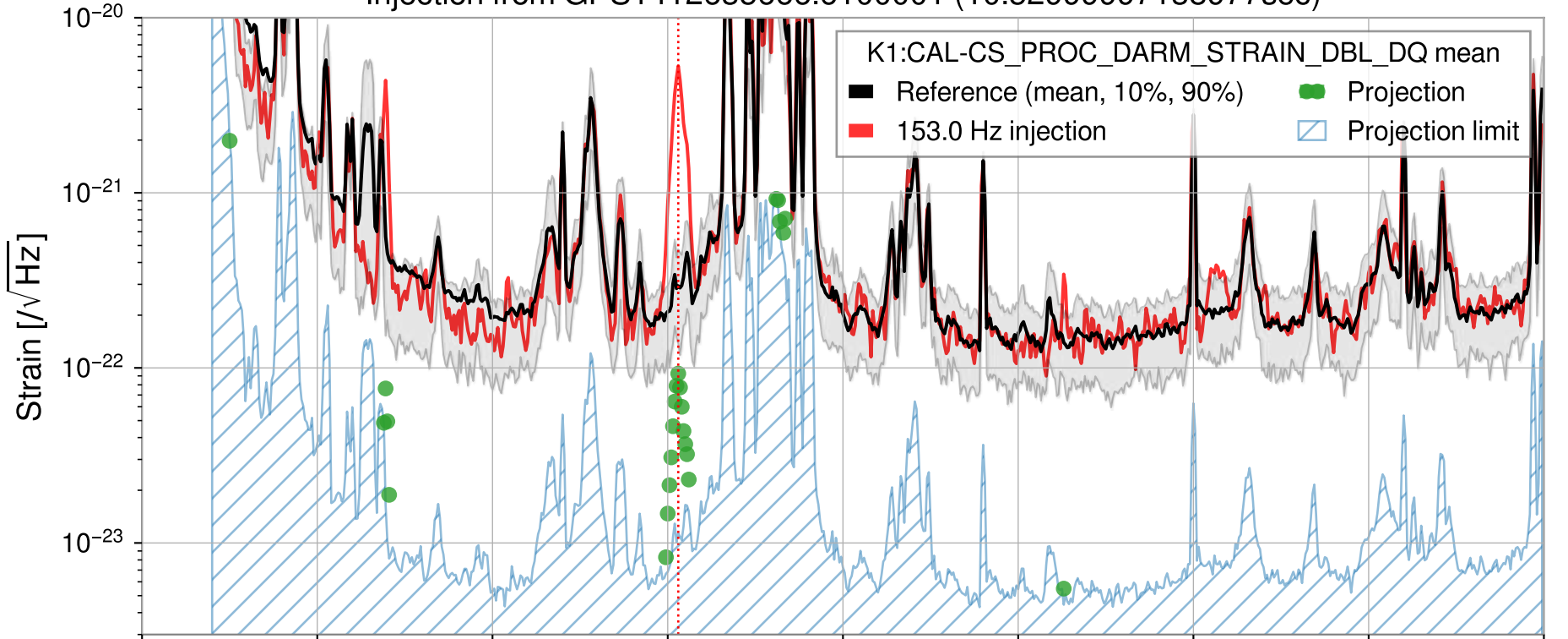
Injection from GPS1412635666.610001 (10.52999997138977sec)
