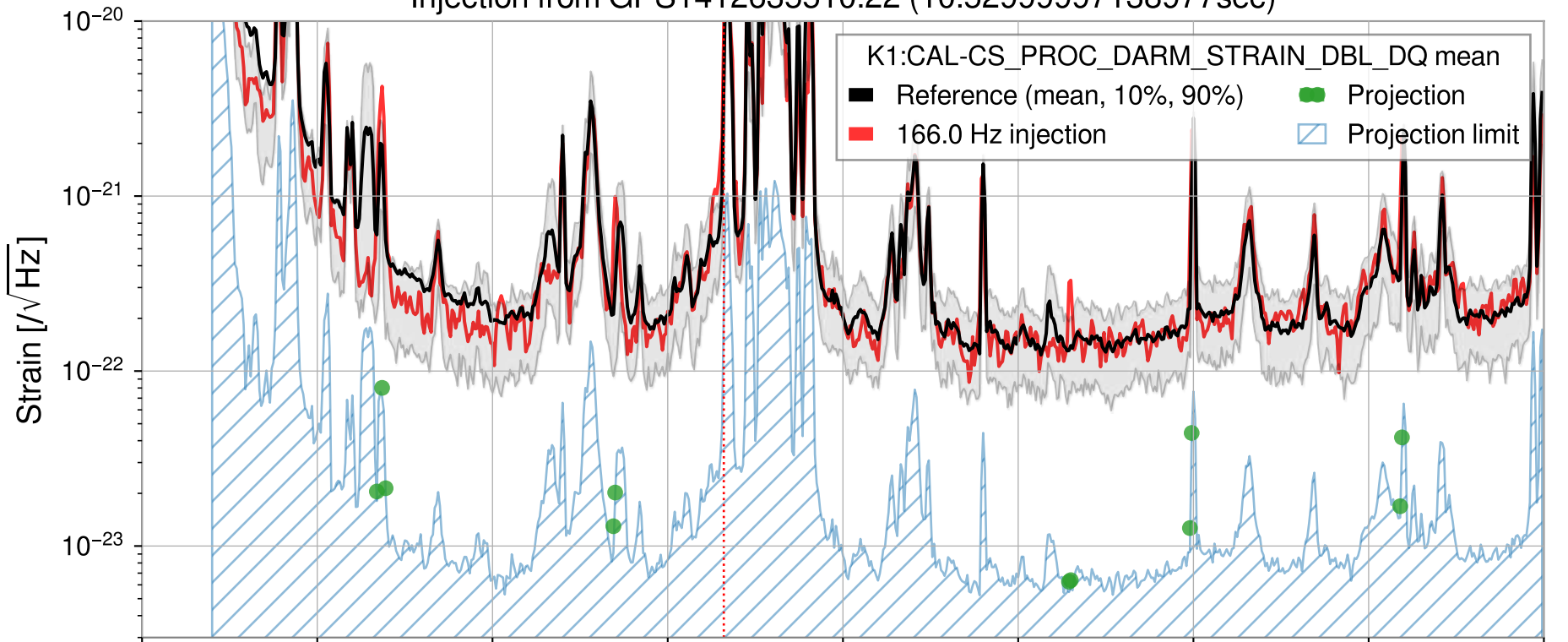
Injection from GPS1412635510.22 (10.52999997138977sec)
