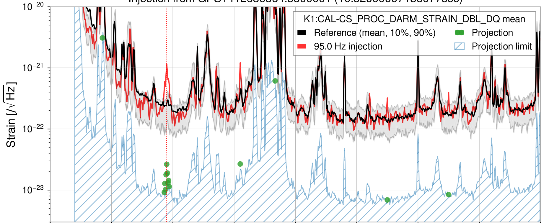
Injection from GPS1412636364.3500001 (10.52999997138977sec)
