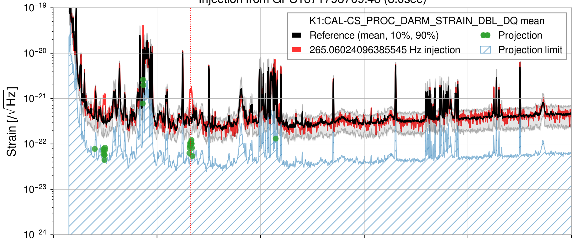
Injection from GPS1371793709.48 (8.0sec)
