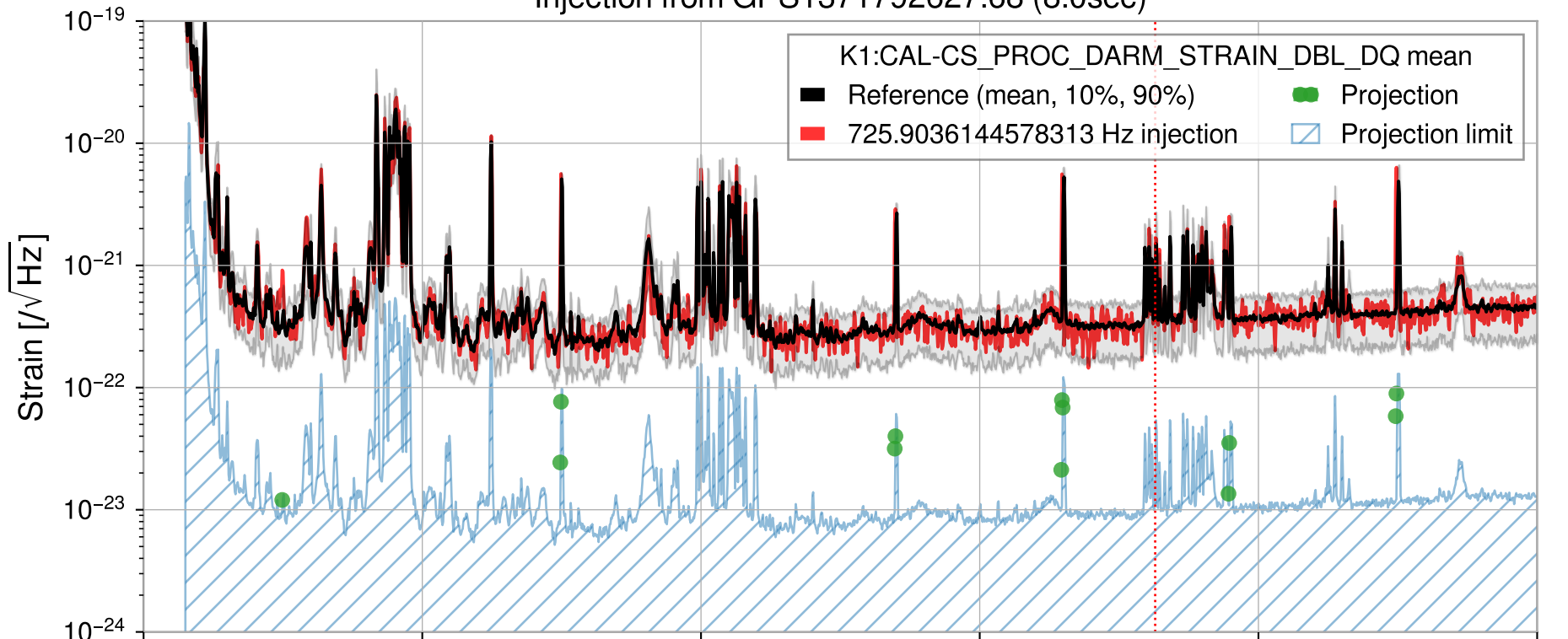
Injection from GPS1371792627.68 (8.0sec)
