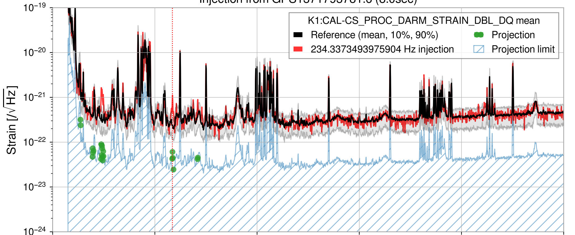
Injection from GPS1371793781.6 (8.0sec)
