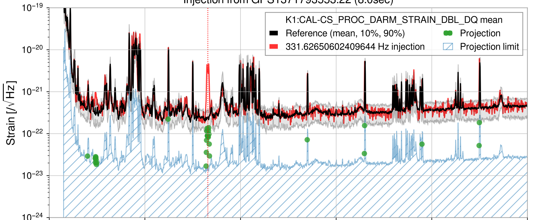
Injection from GPS1371793553.22 (8.0sec)
