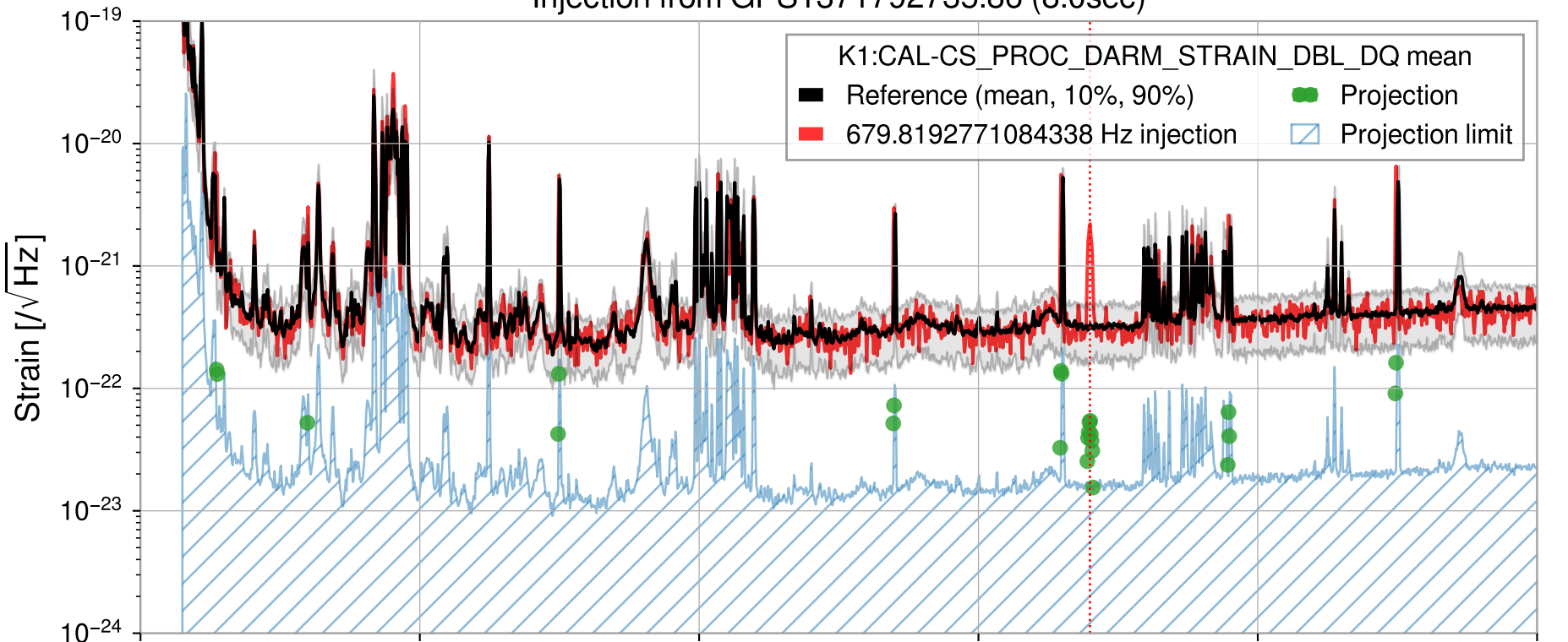
Injection from GPS1371792735.86 (8.0sec)
