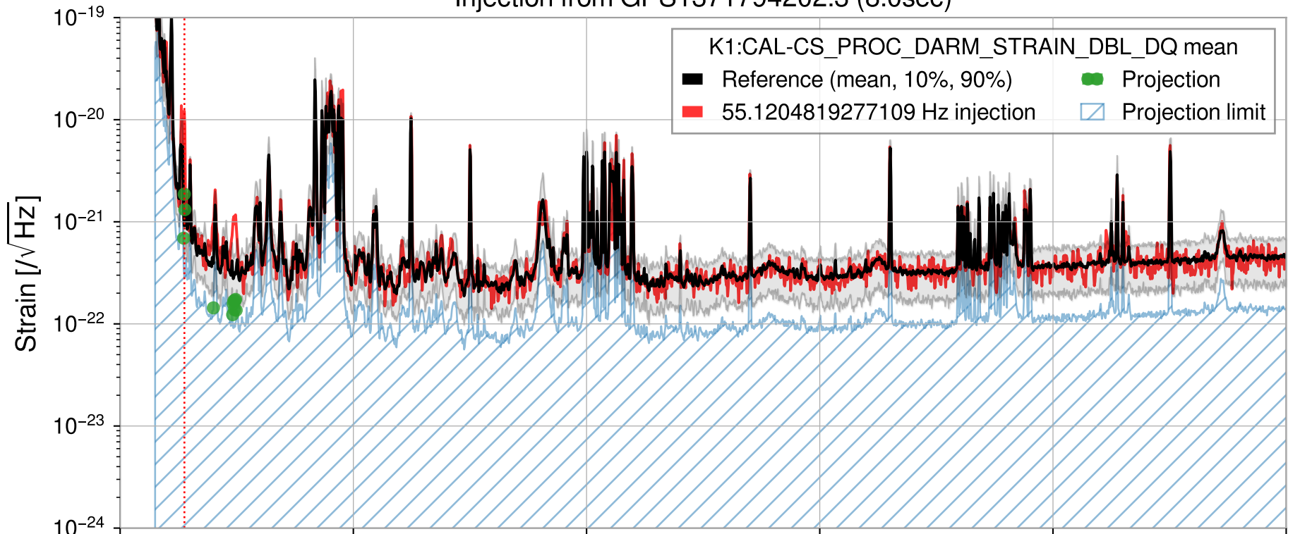
Injection from GPS1371794202.3 (8.0sec)
