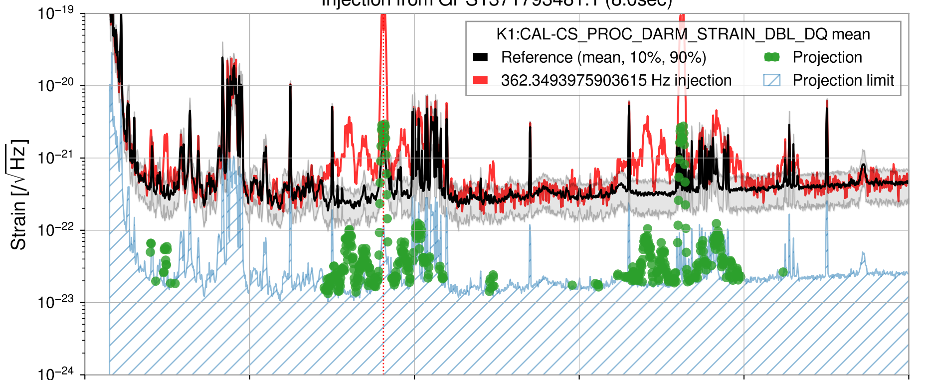
Injection from GPS1371793481.1 (8.0sec)
