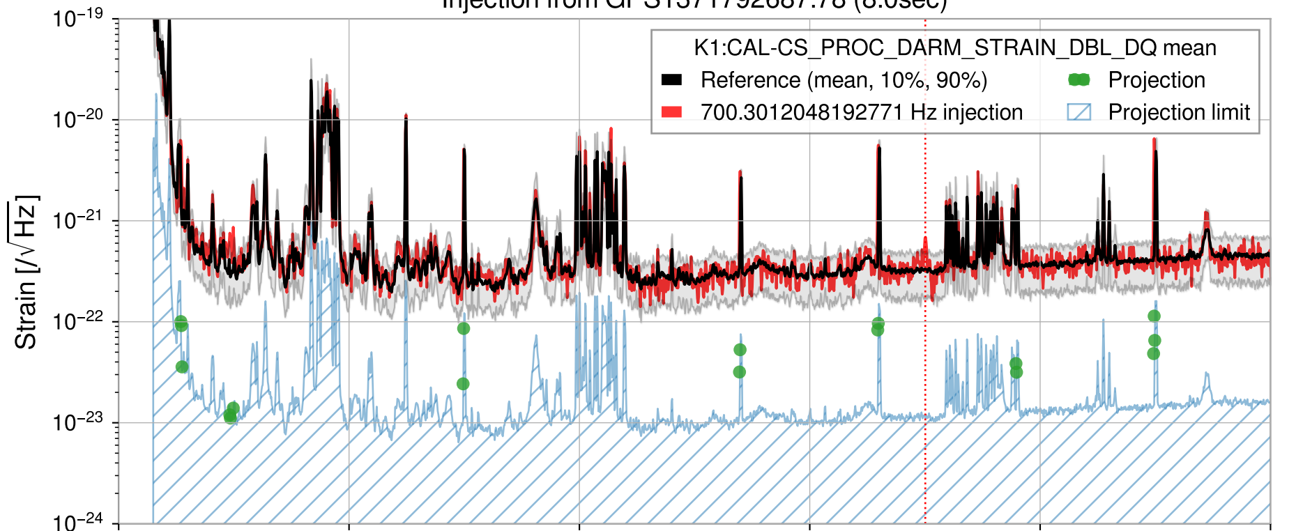
Injection from GPS1371792687.78 (8.0sec)
