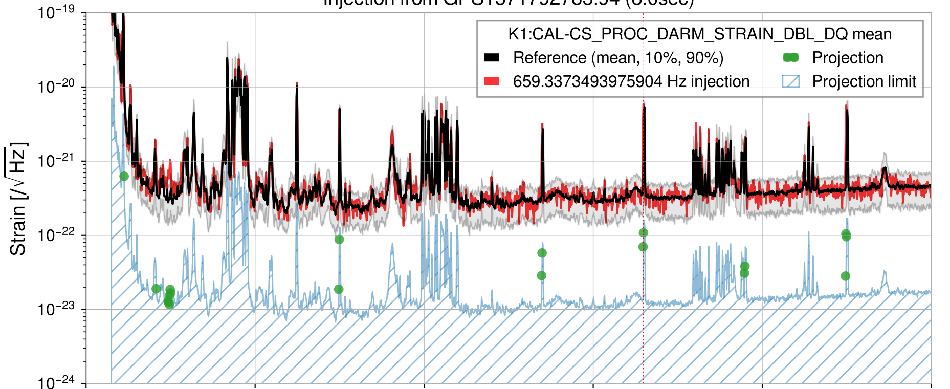
Injection from GPS1371792783.94 (8.0sec)
