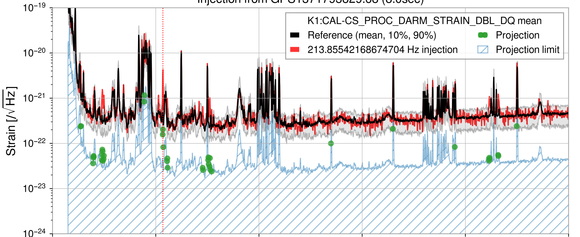
Injection from GPS1371793829.68 (8.0sec)
