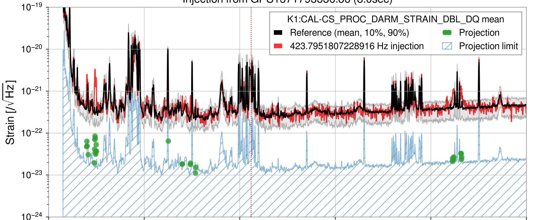
Injection from GPS1371793336.86 (8.0sec)
