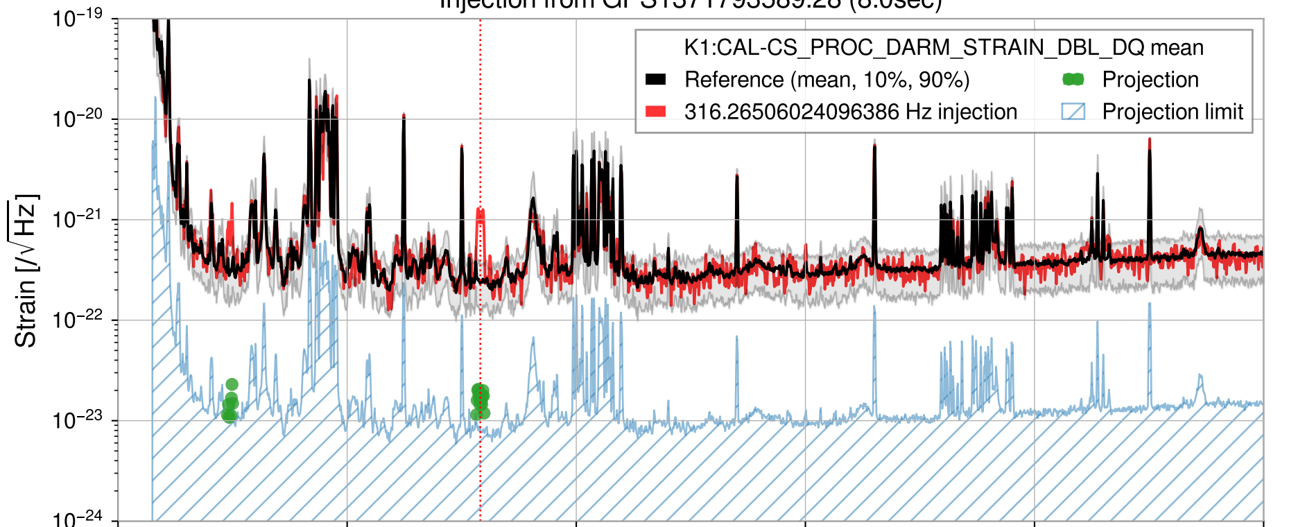
Injection from GPS1371793589.28 (8.0sec)
