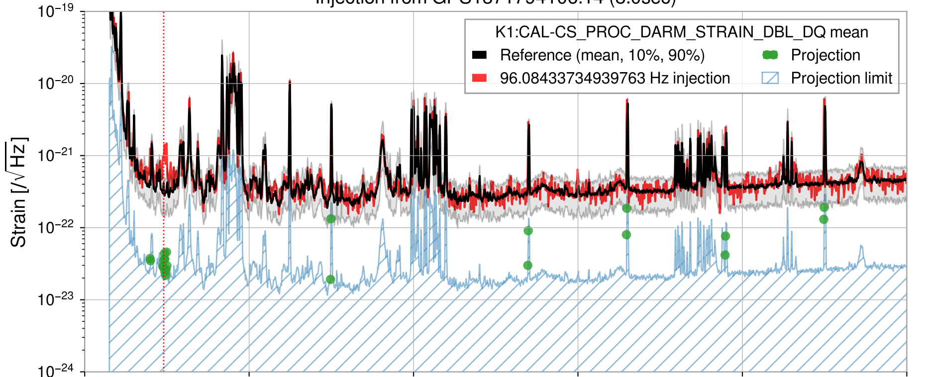
Injection from GPS1371794106.14 (8.0sec)
