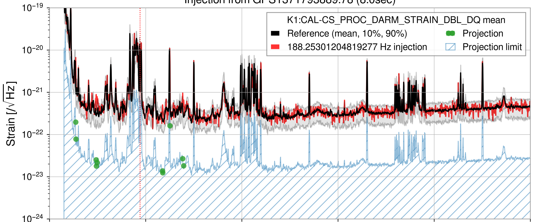
Injection from GPS1371793889.78 (8.0sec)
