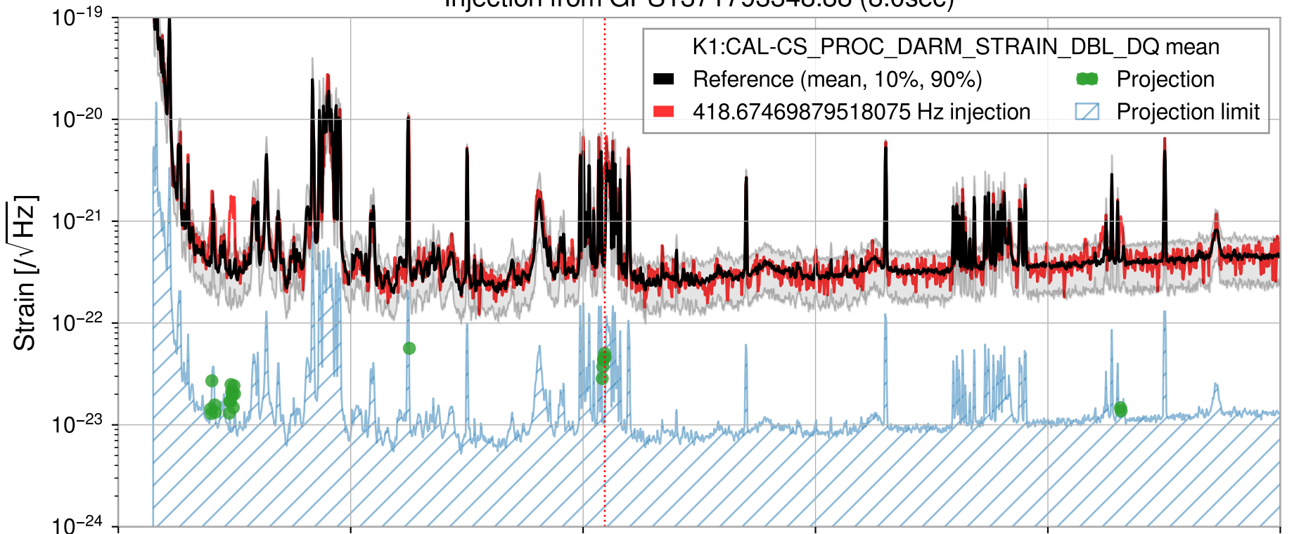
Injection from GPS1371793348.88 (8.0sec)
