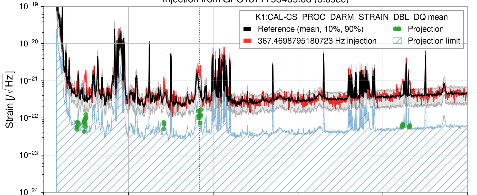
Injection from GPS1371793469.08 (8.0sec)
