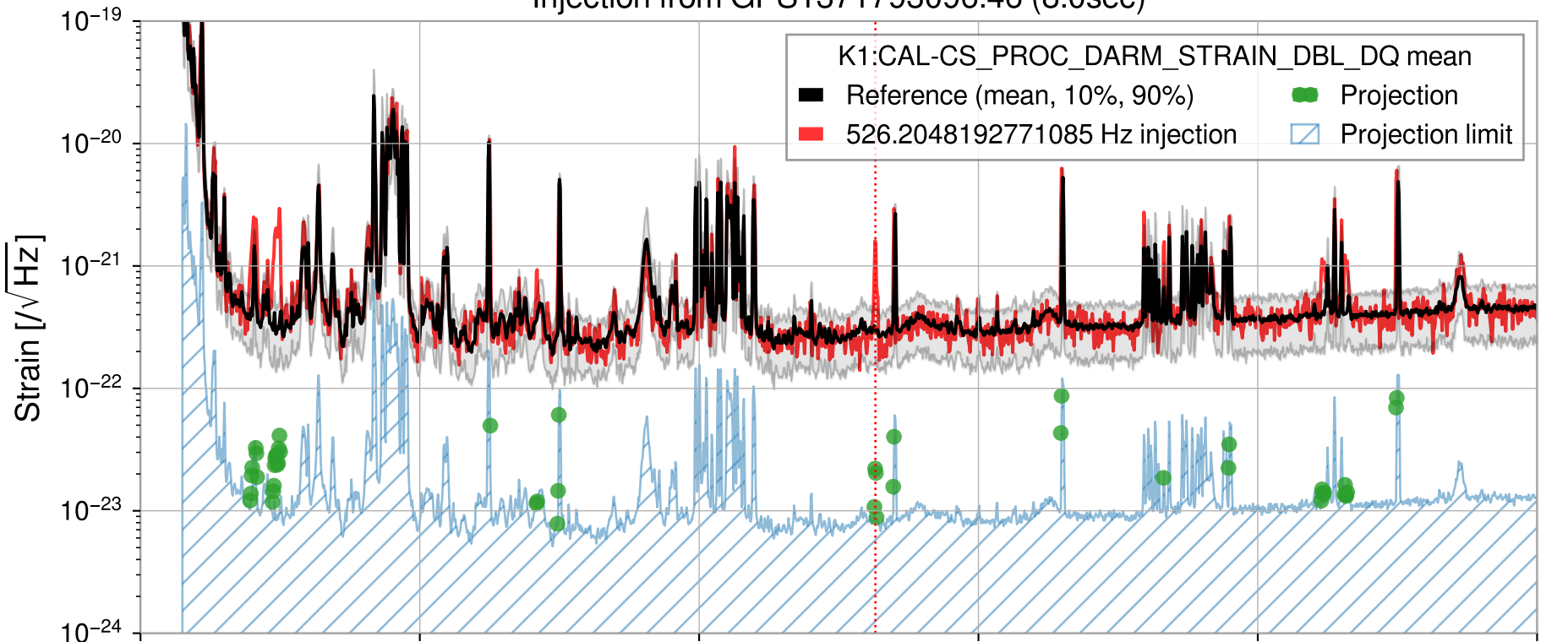
Injection from GPS1371793096.46 (8.0sec)
