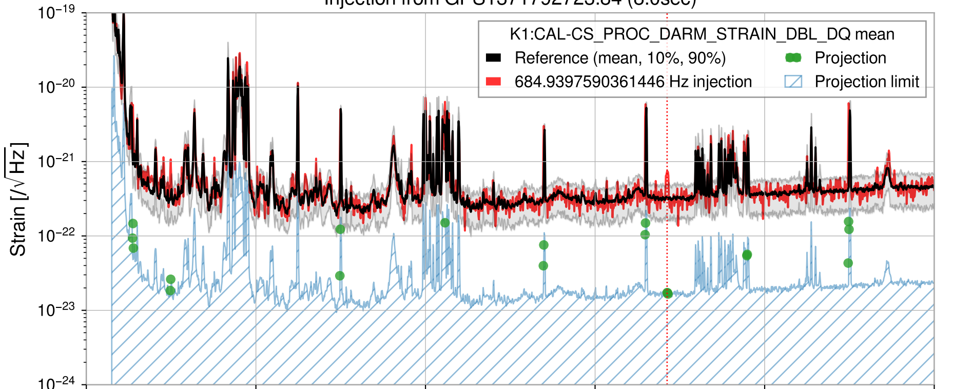
Injection from GPS1371792723.84 (8.0sec)
