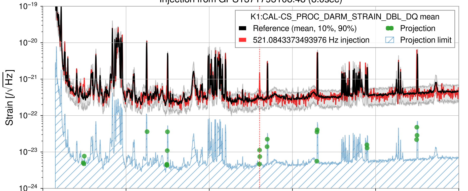
Injection from GPS1371793108.48 (8.0sec)
