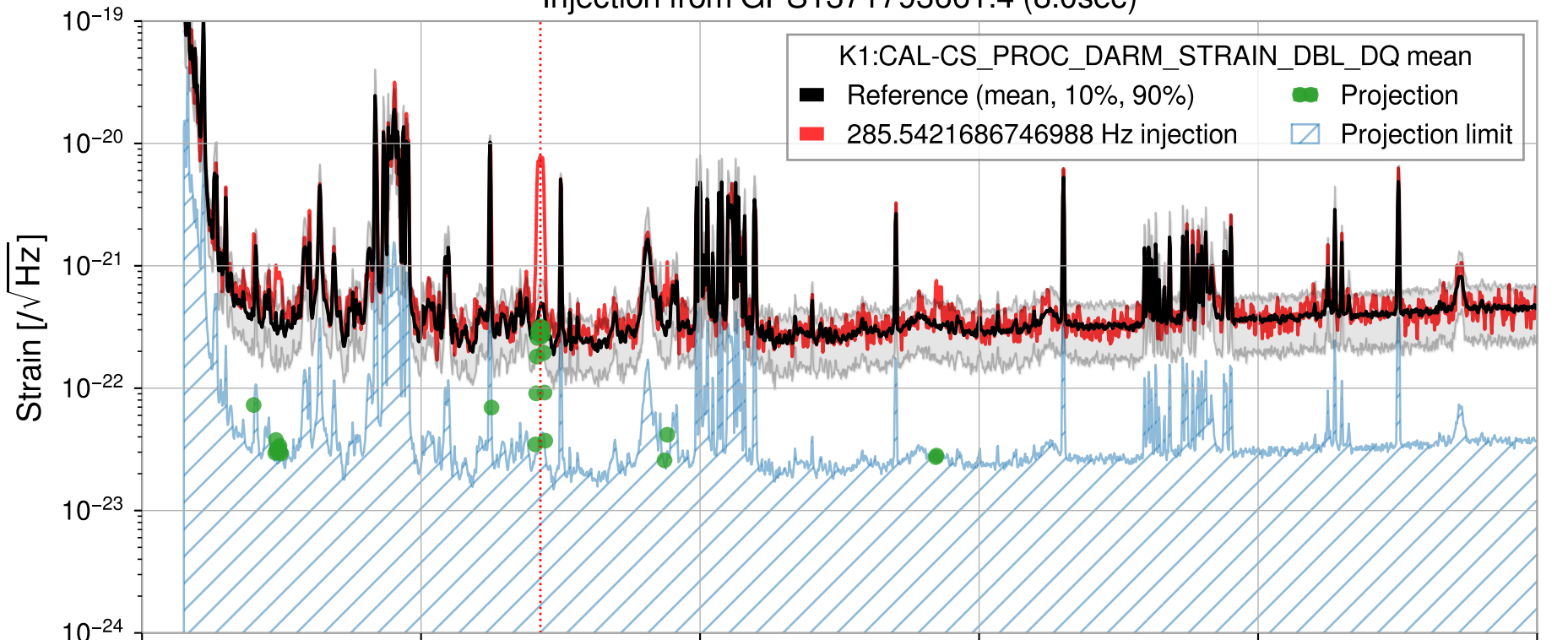
Injection from GPS1371793661.4 (8.0sec)
