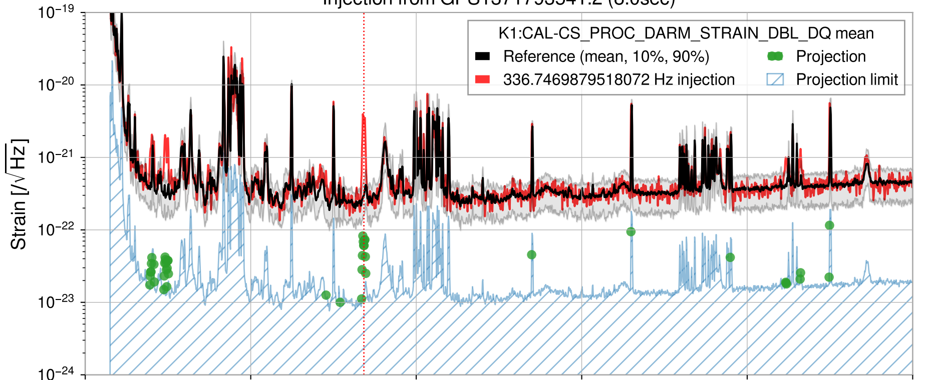
Injection from GPS1371793541.2 (8.0sec)
