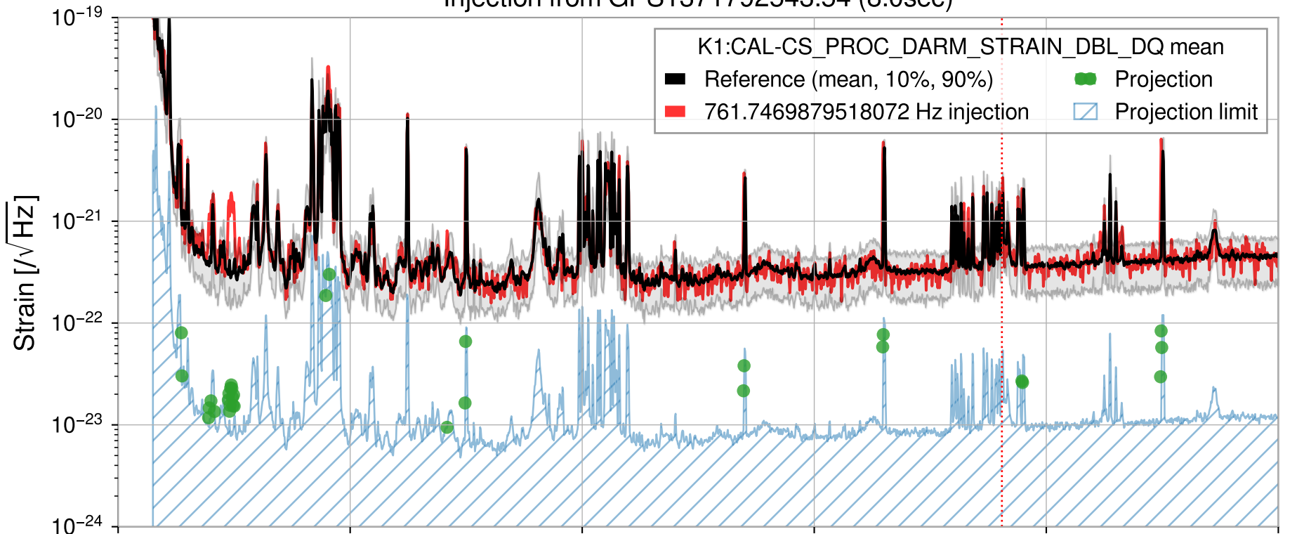
Injection from GPS1371792543.54 (8.0sec)
