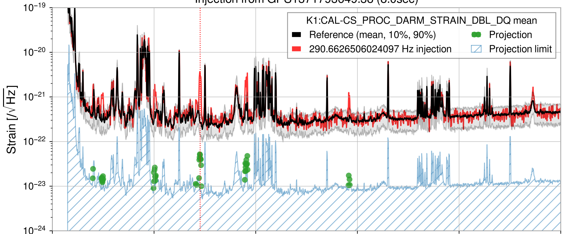
Injection from GPS1371793649.38 (8.0sec)
