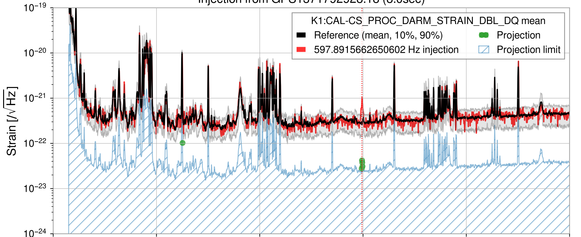
Injection from GPS1371792928.18 (8.0sec)
