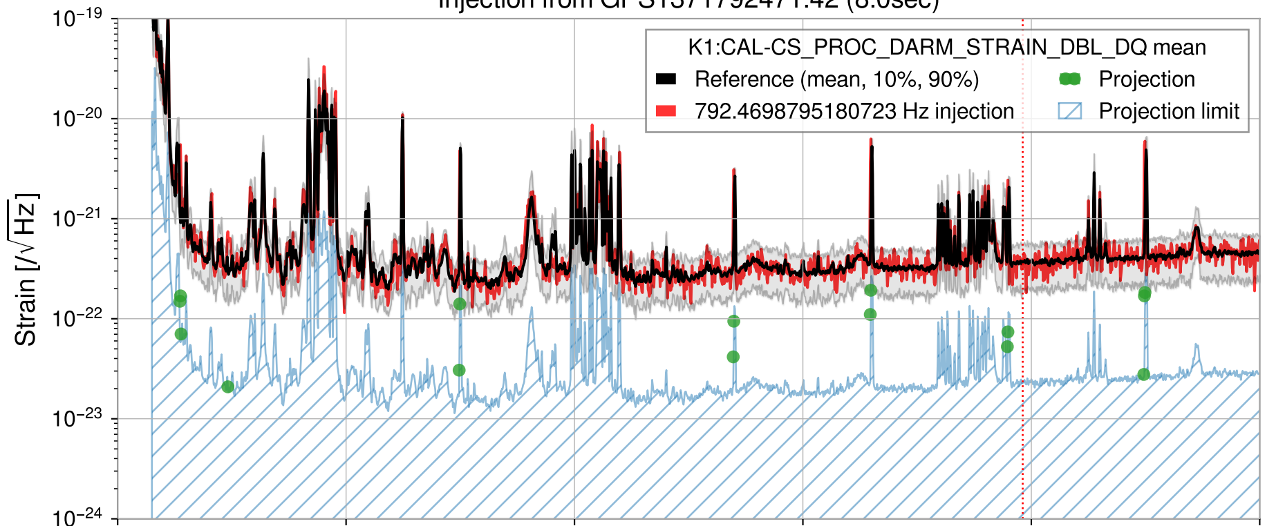
Injection from GPS1371792471.42 (8.0sec)
