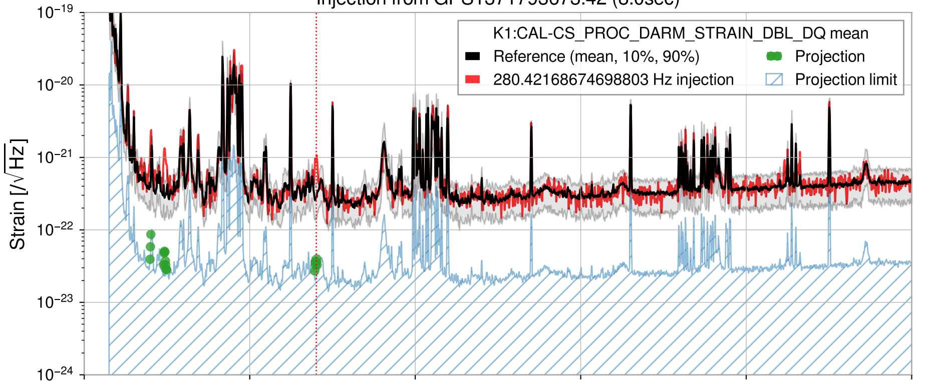
Injection from GPS1371793673.42 (8.0sec)
