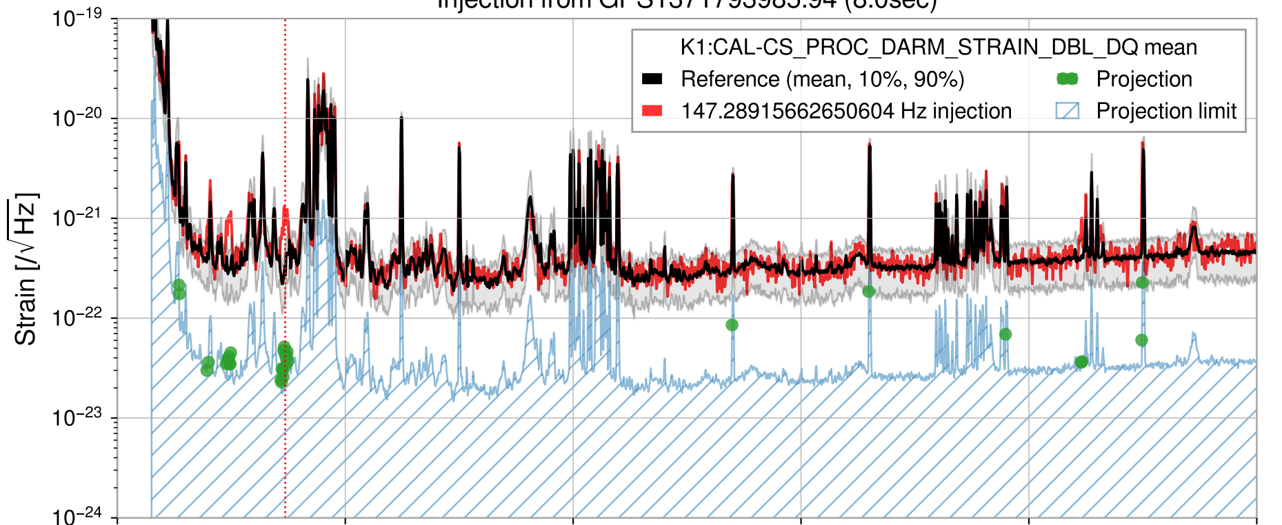
Injection from GPS1371793985.94 (8.0sec)
