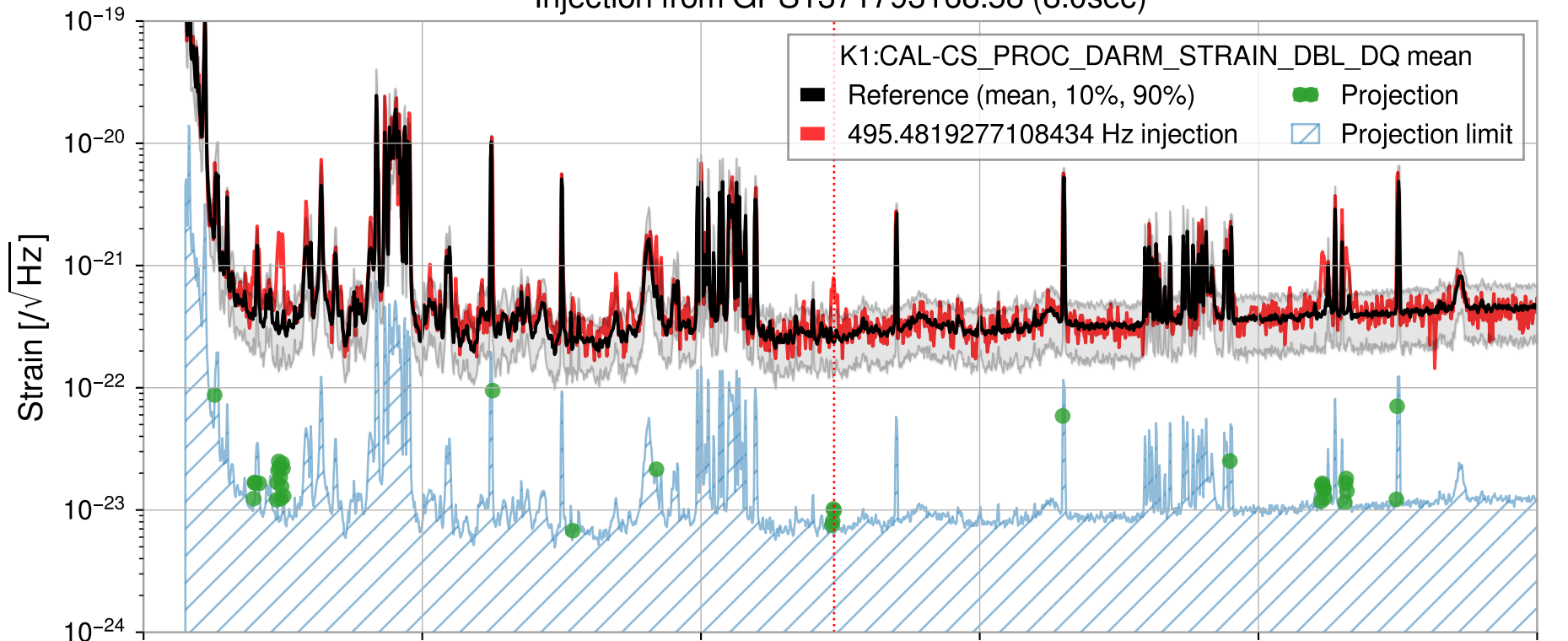
Injection from GPS1371793168.58 (8.0sec)
