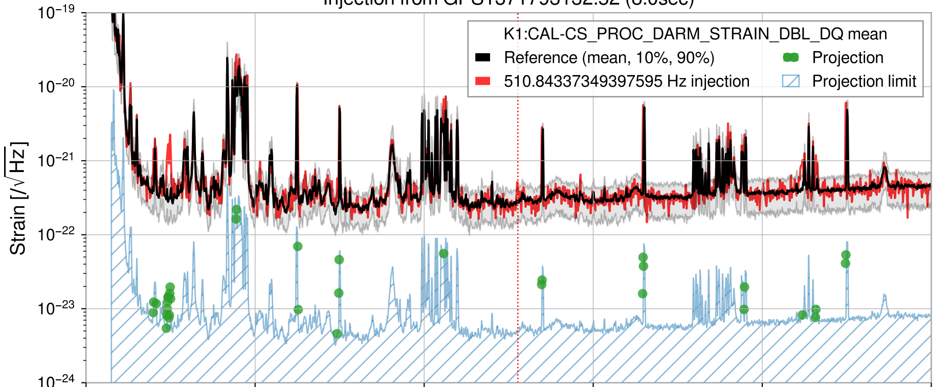
Injection from GPS1371793132.52 (8.0sec)
