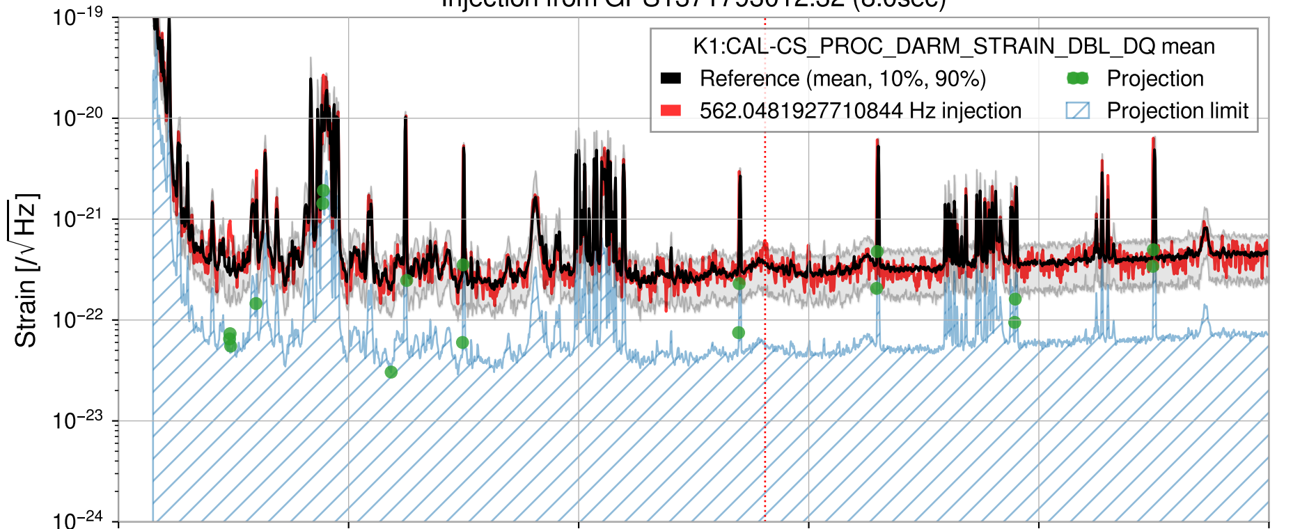
Injection from GPS1371793012.32 (8.0sec)
