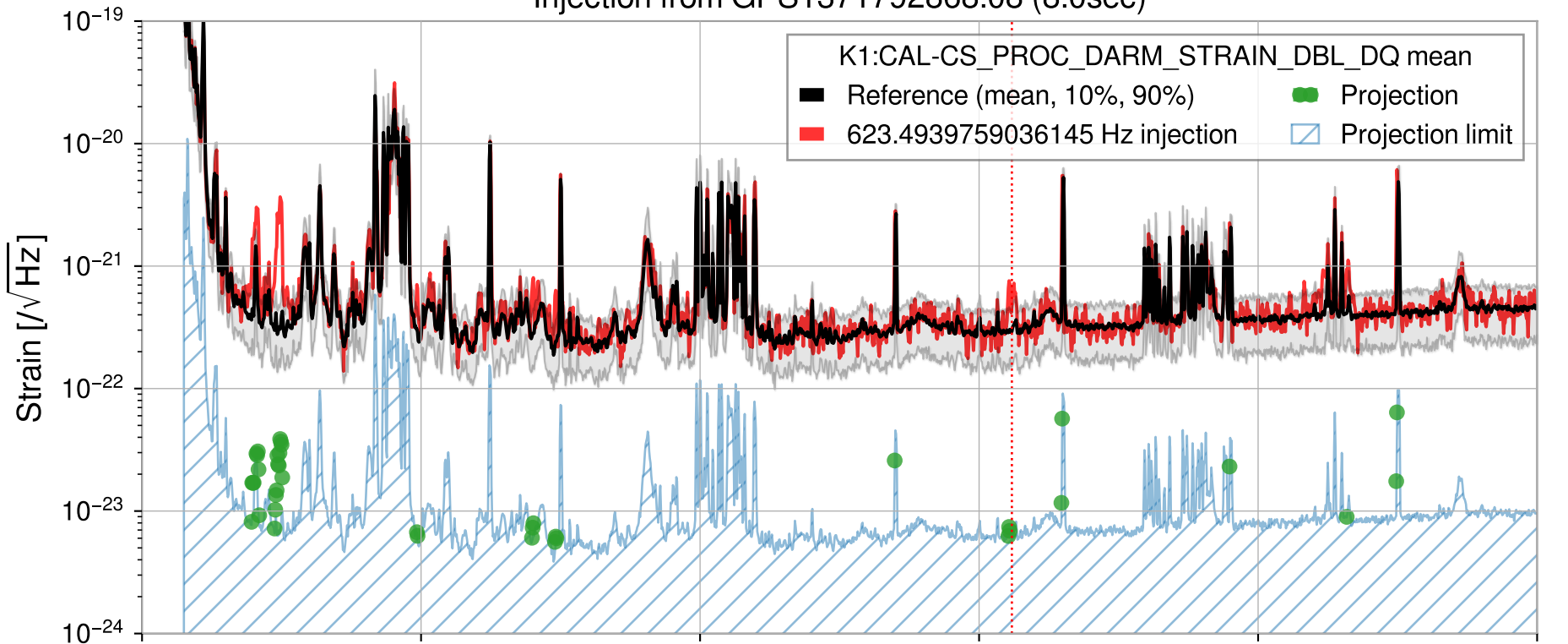
Injection from GPS1371792868.08 (8.0sec)
