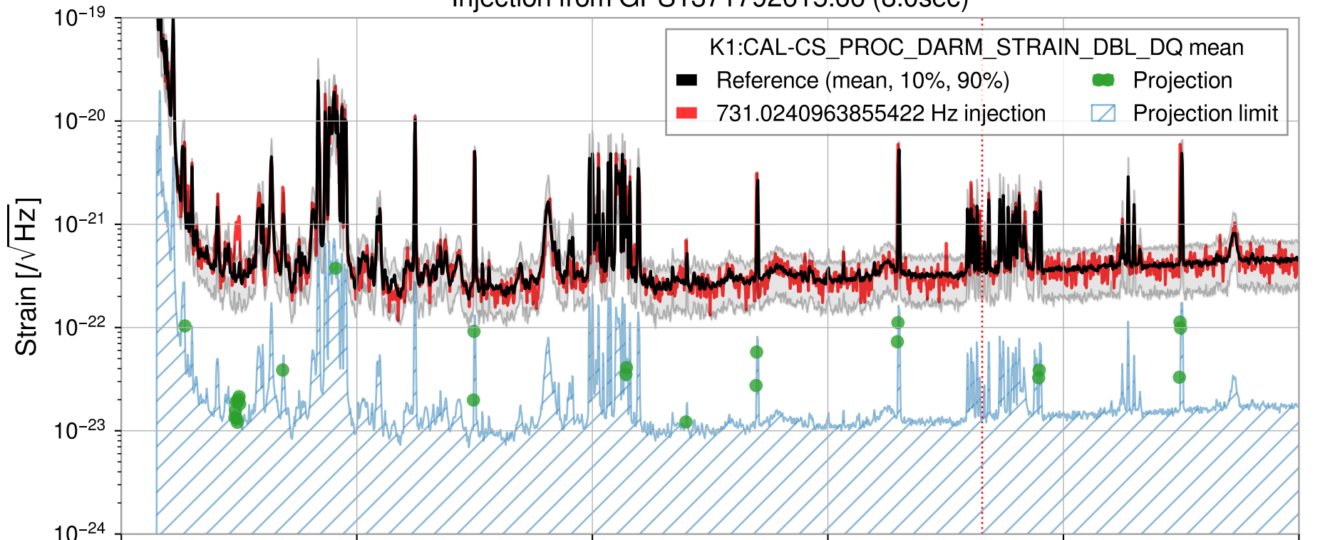
Injection from GPS1371792615.66 (8.0sec)
