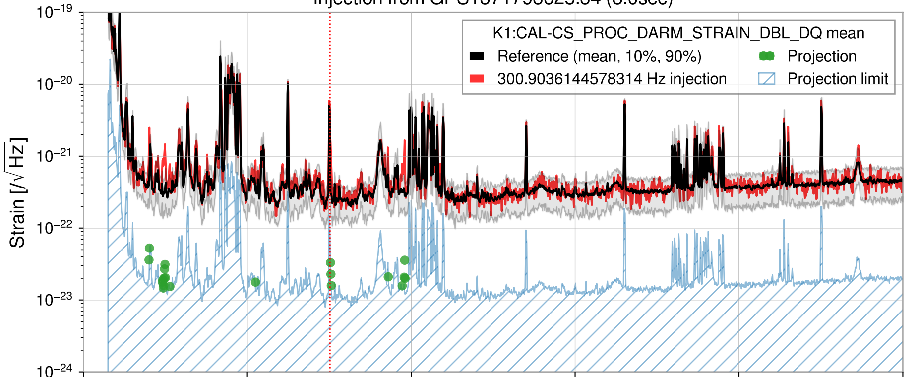
Injection from GPS1371793625.34 (8.0sec)
