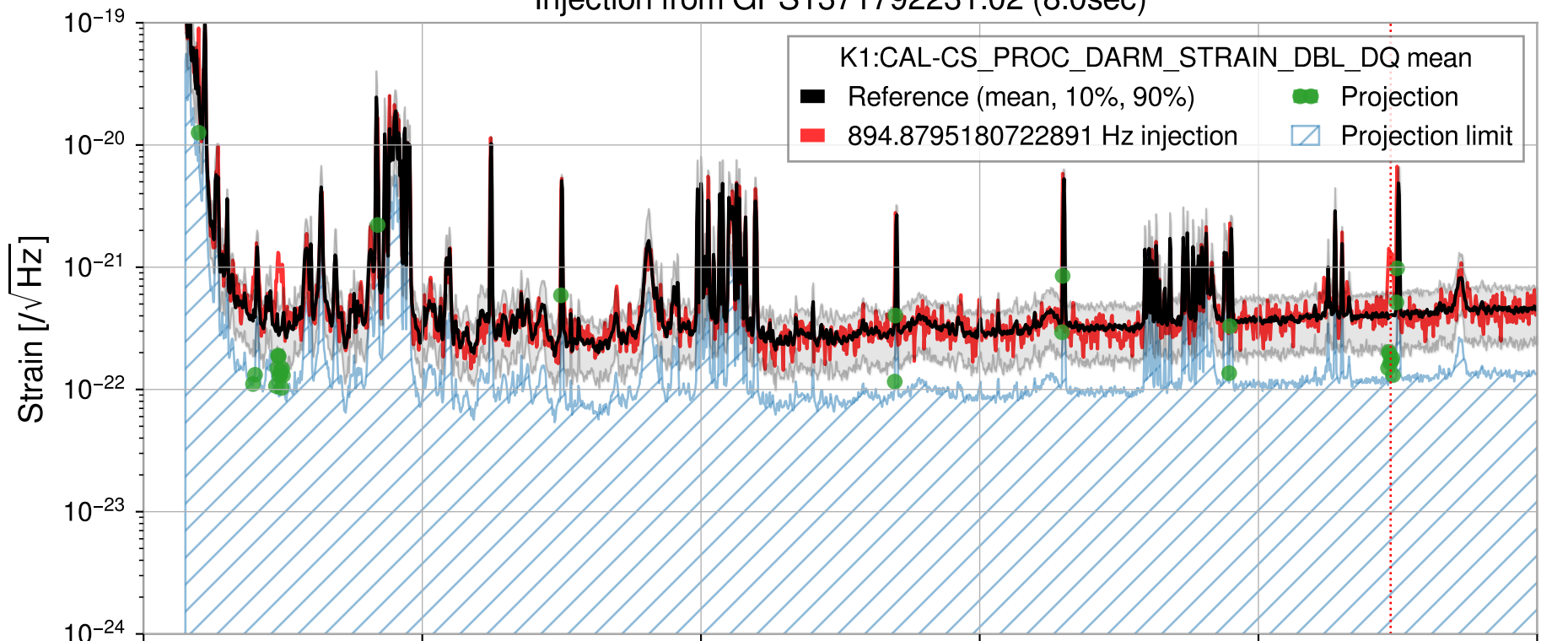
Injection from GPS1371792231.02 (8.0sec)
