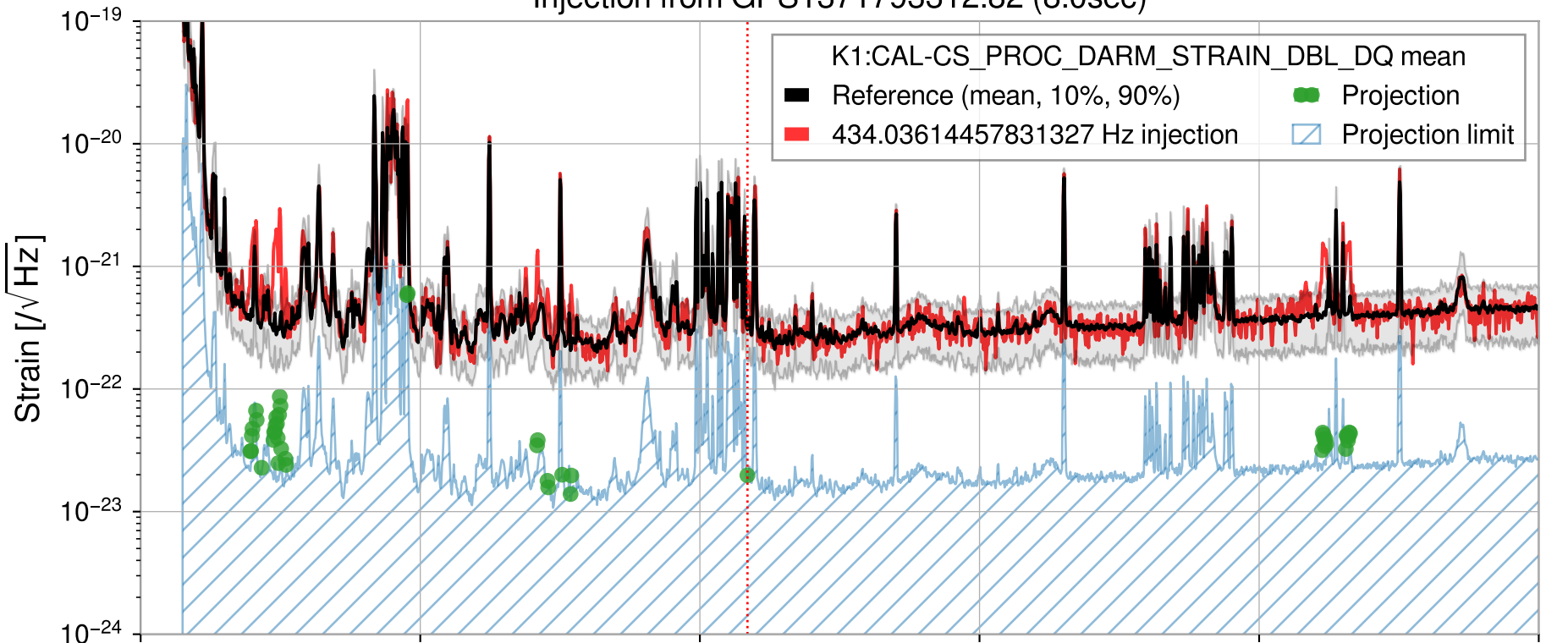
Injection from GPS1371793312.82 (8.0sec)
