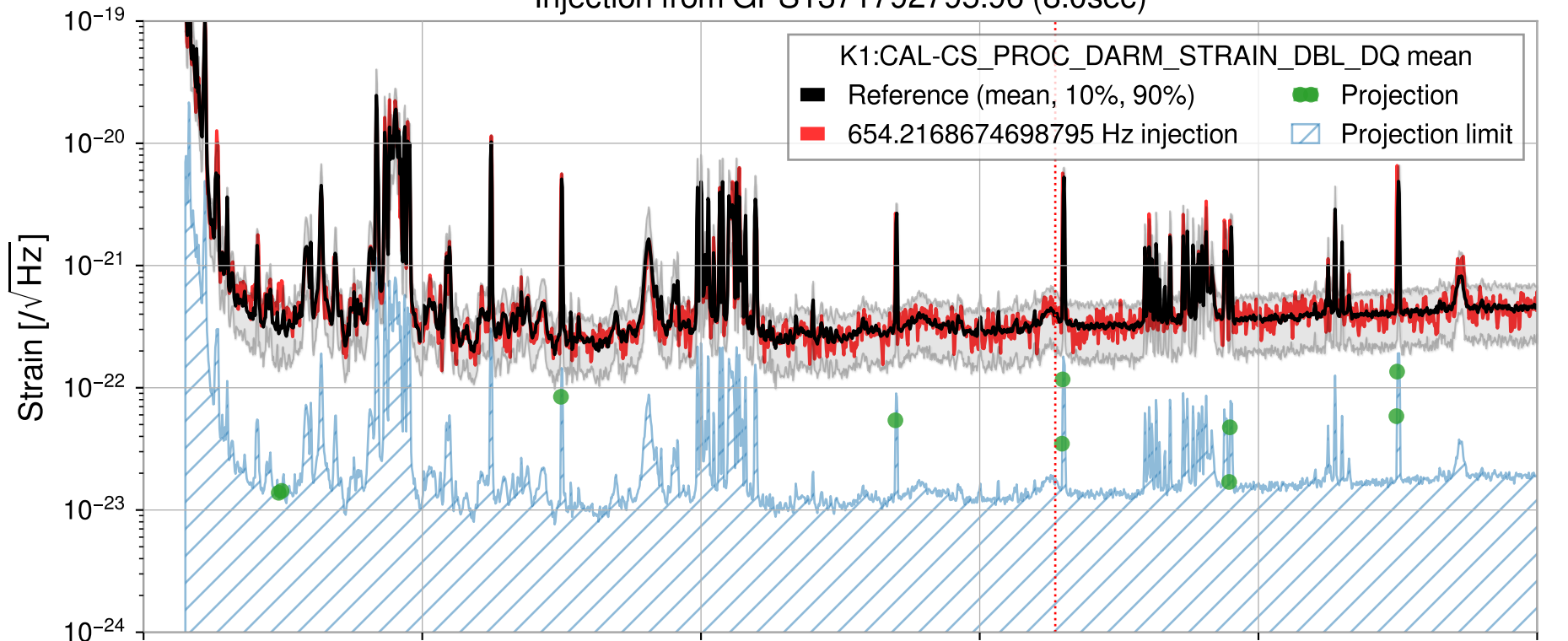
Injection from GPS1371792795.96 (8.0sec)
