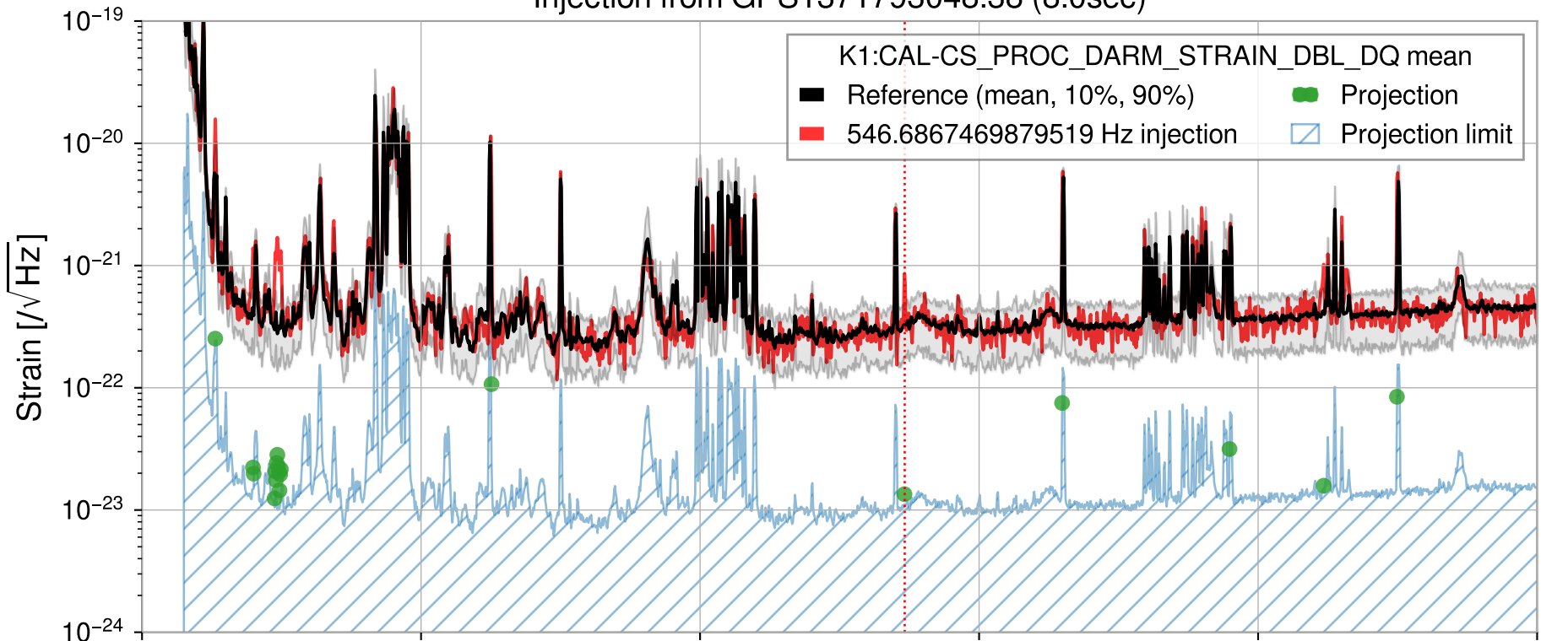
Injection from GPS1371793048.38 (8.0sec)
