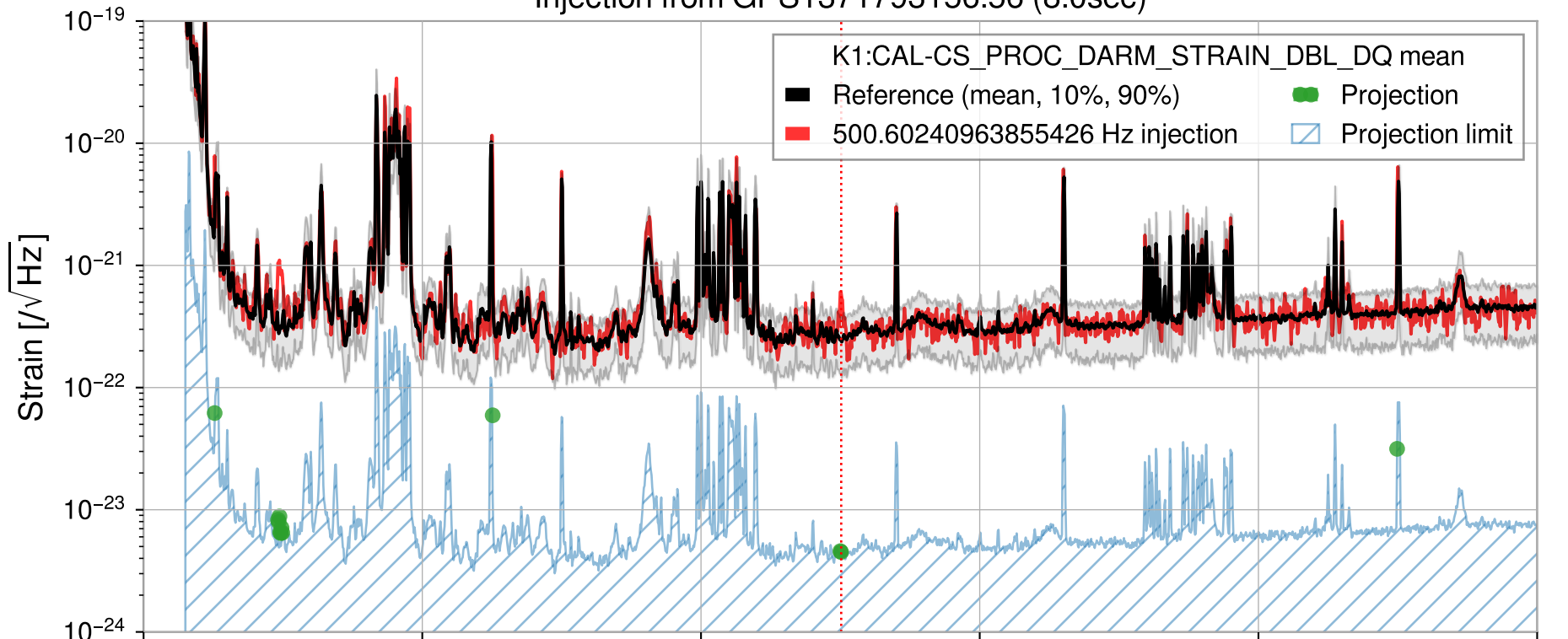
Injection from GPS1371793156.56 (8.0sec)
