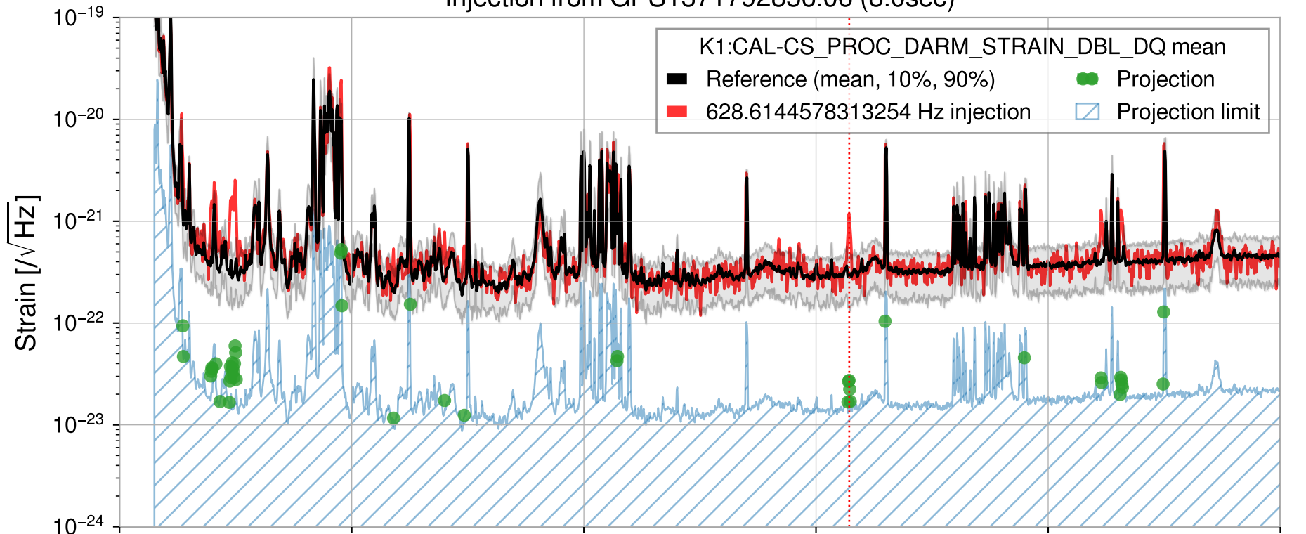
Injection from GPS1371792856.06 (8.0sec)
