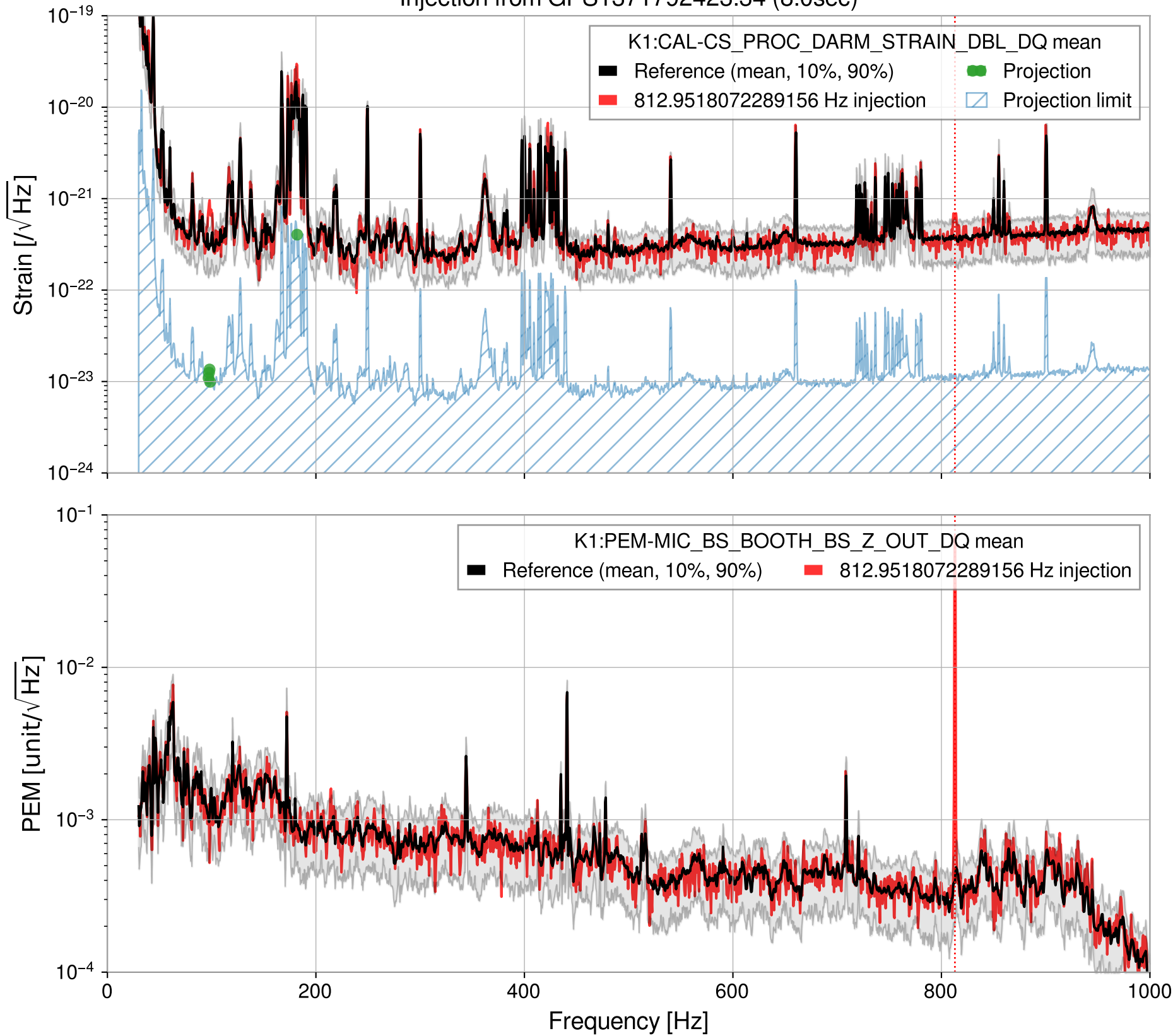
Injection from GPS1371792423.34 (8.0sec)
