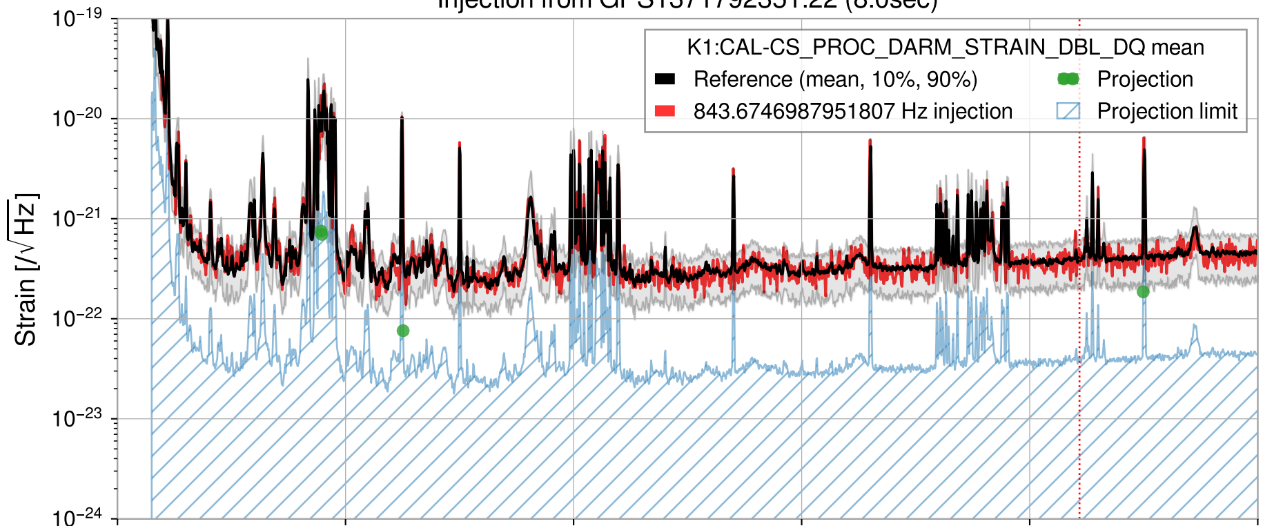
Injection from GPS1371792351.22 (8.0sec)
