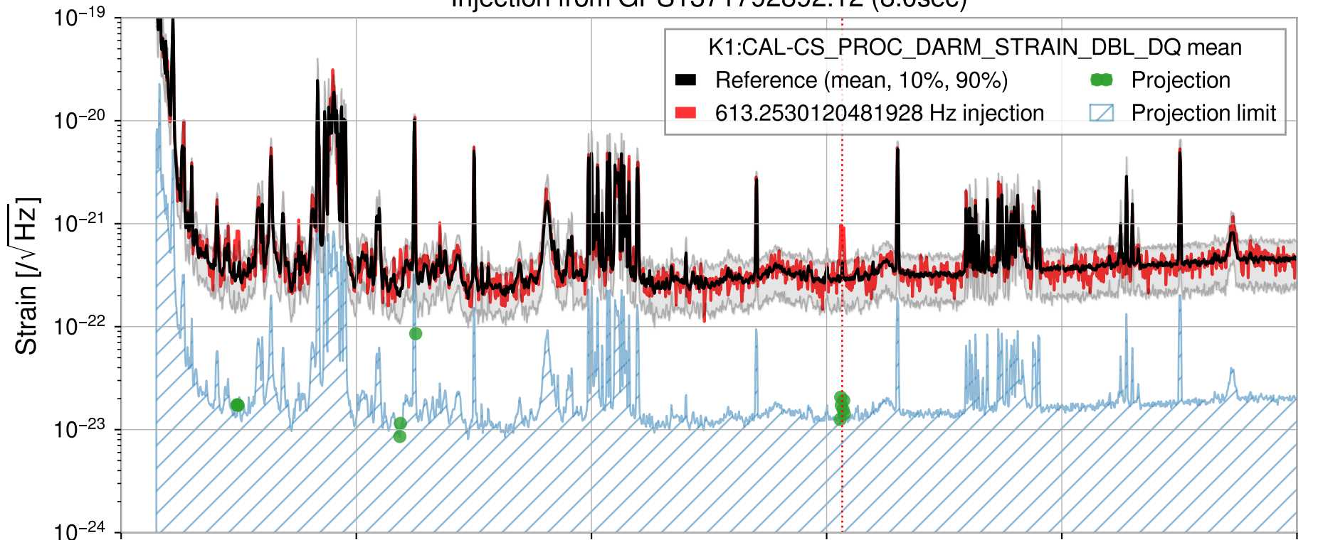
Injection from GPS1371792892.12 (8.0sec)
