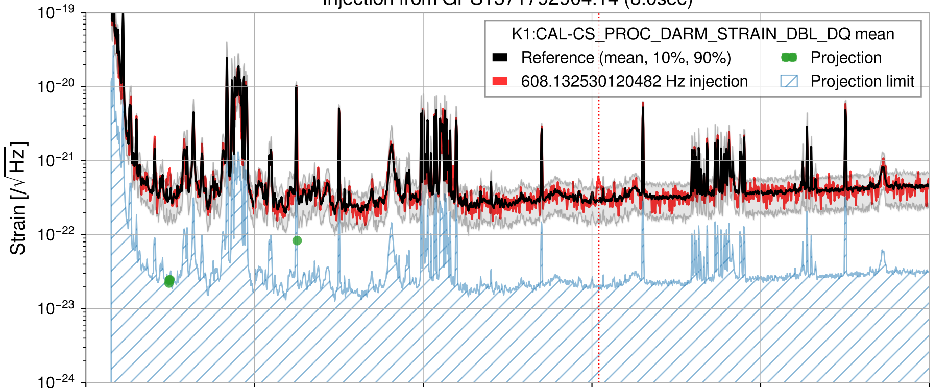
Injection from GPS1371792904.14 (8.0sec)
