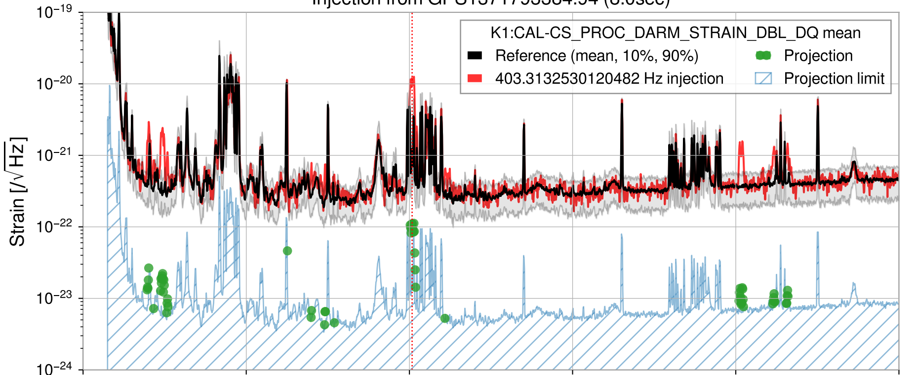
Injection from GPS1371793384.94 (8.0sec)
