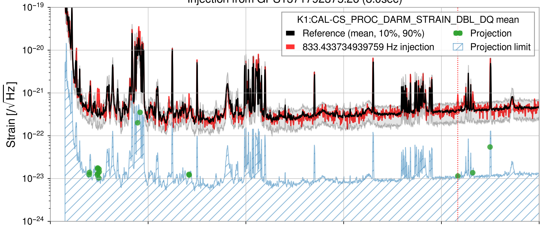
Injection from GPS1371792375.26 (8.0sec)
