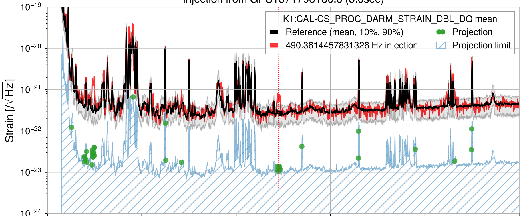
Injection from GPS1371793180.6 (8.0sec)
