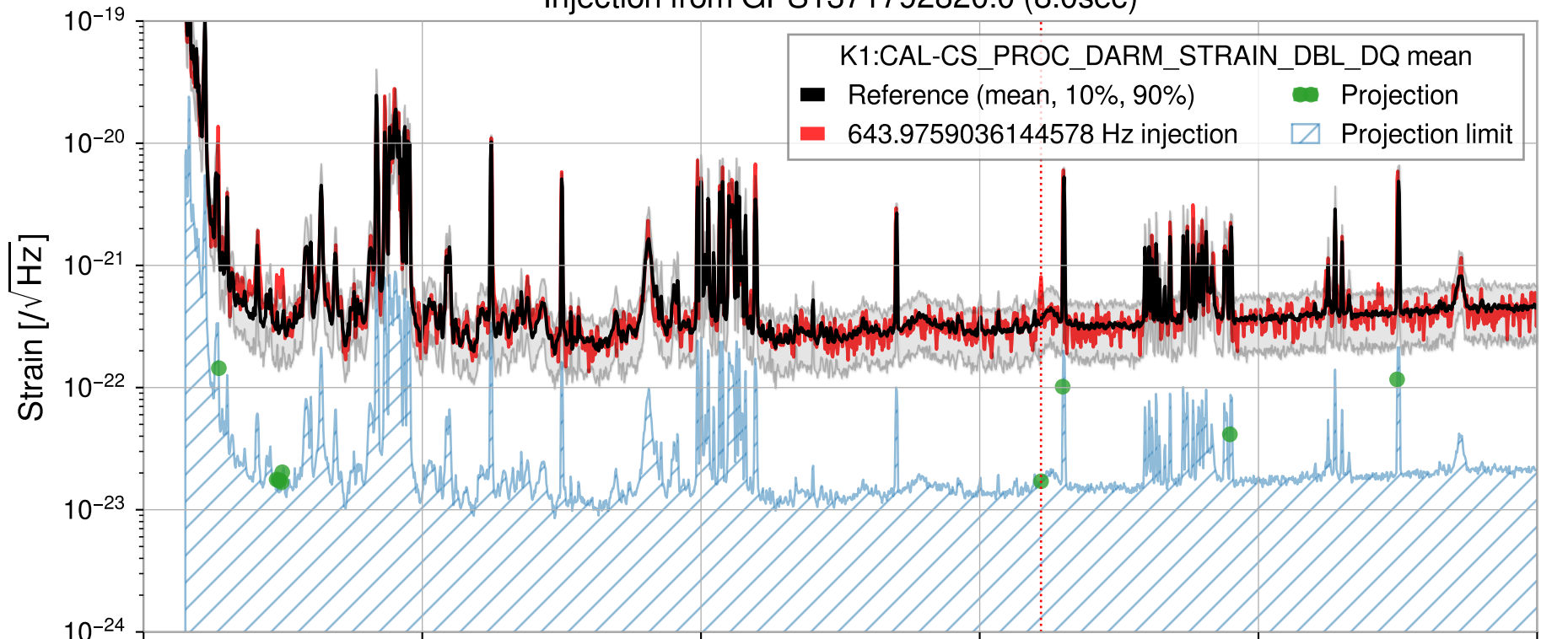
Injection from GPS1371792820.0 (8.0sec)
