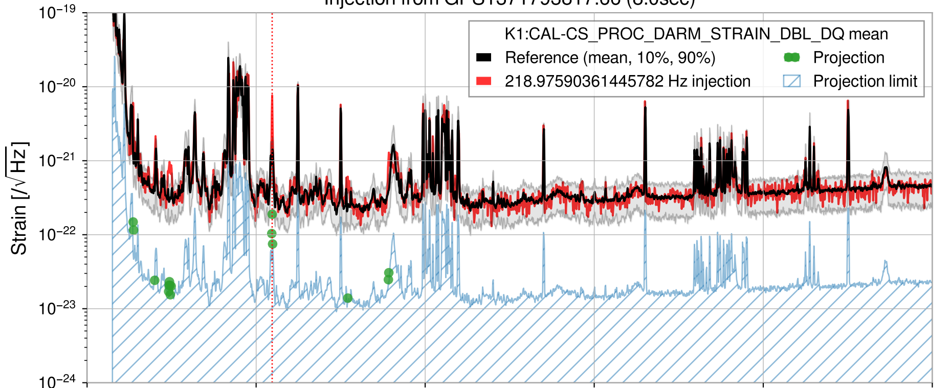
Injection from GPS1371793817.66 (8.0sec)
