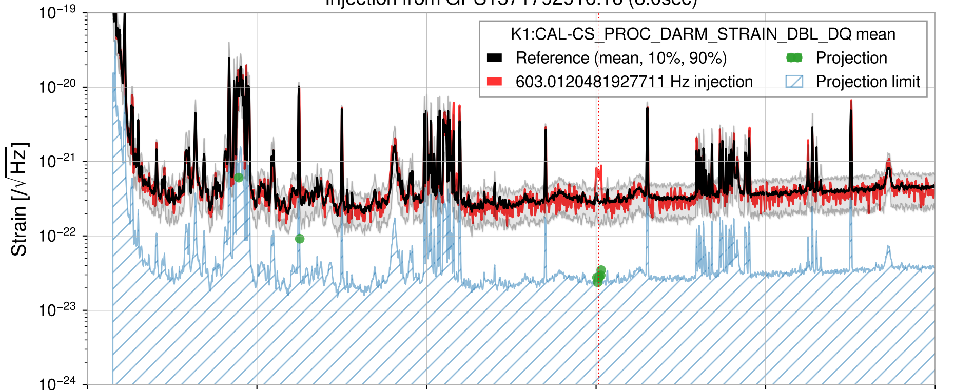
Injection from GPS1371792916.16 (8.0sec)
