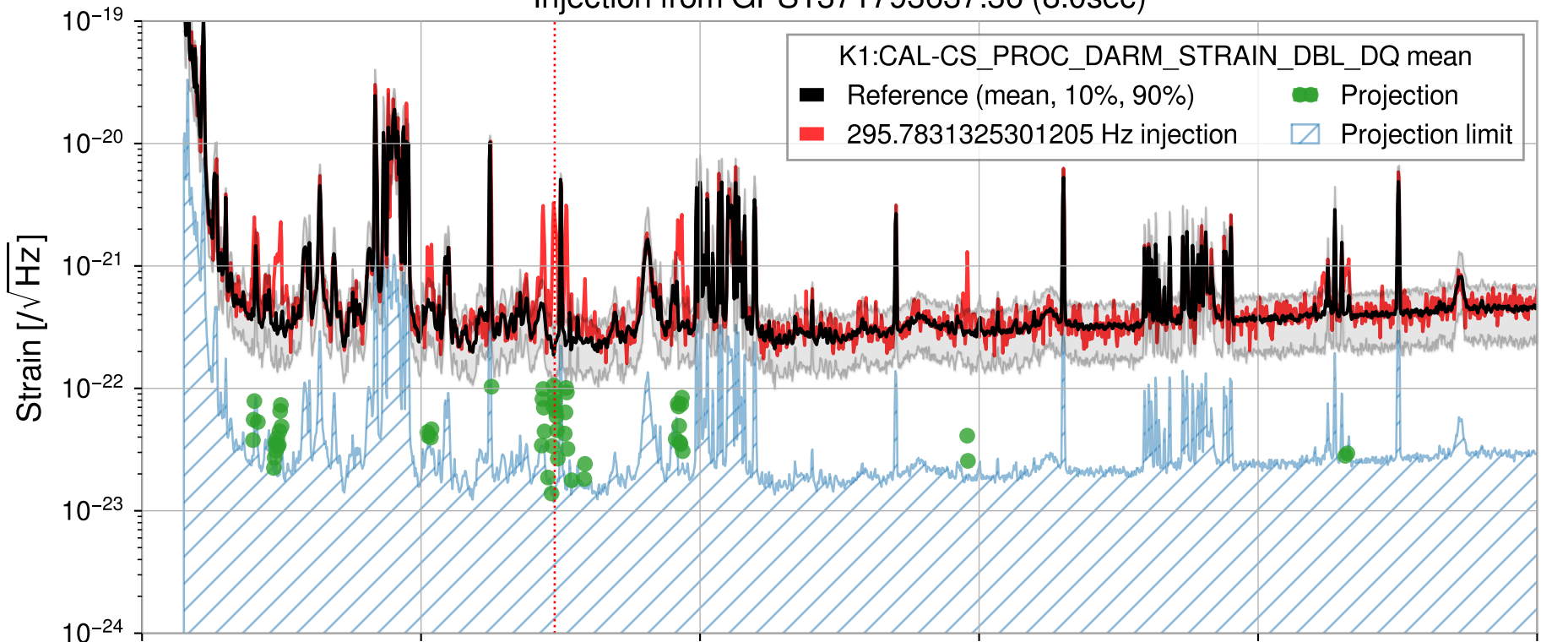
Injection from GPS1371793637.36 (8.0sec)
