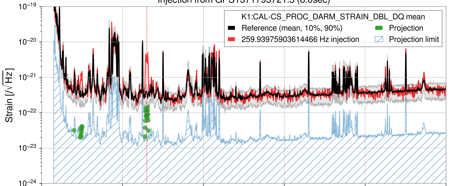
Injection from GPS1371793721.5 (8.0sec)
