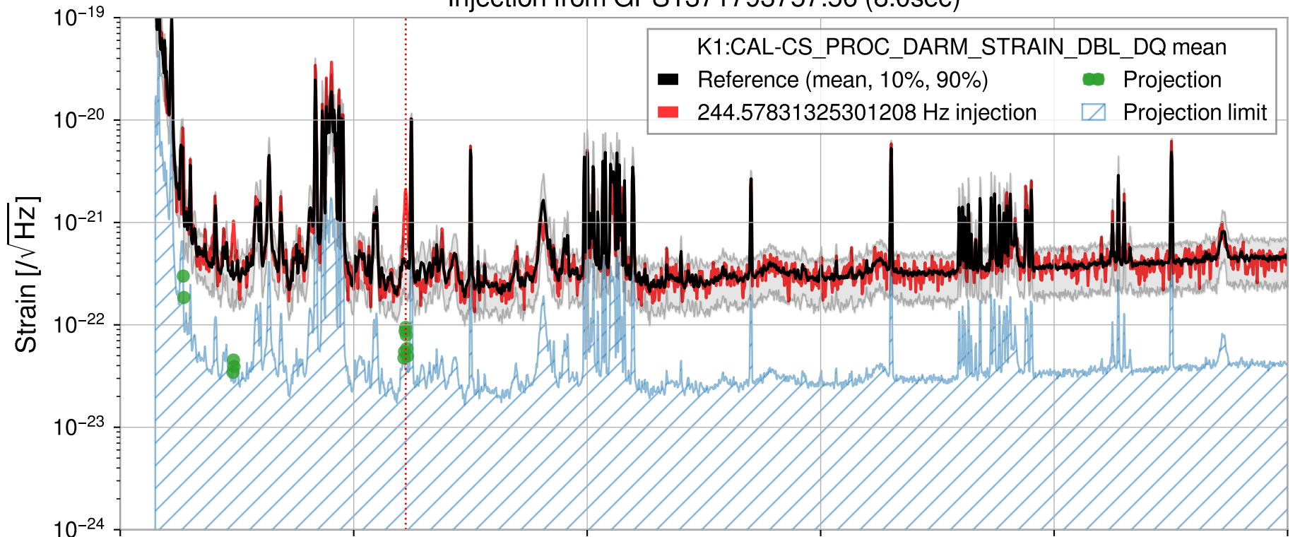
Injection from GPS1371793757.56 (8.0sec)
