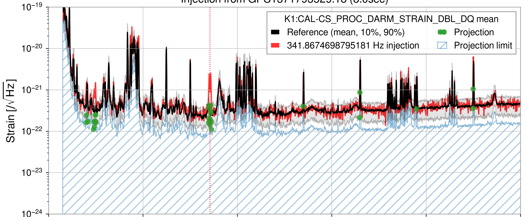
Injection from GPS1371793529.18 (8.0sec)
