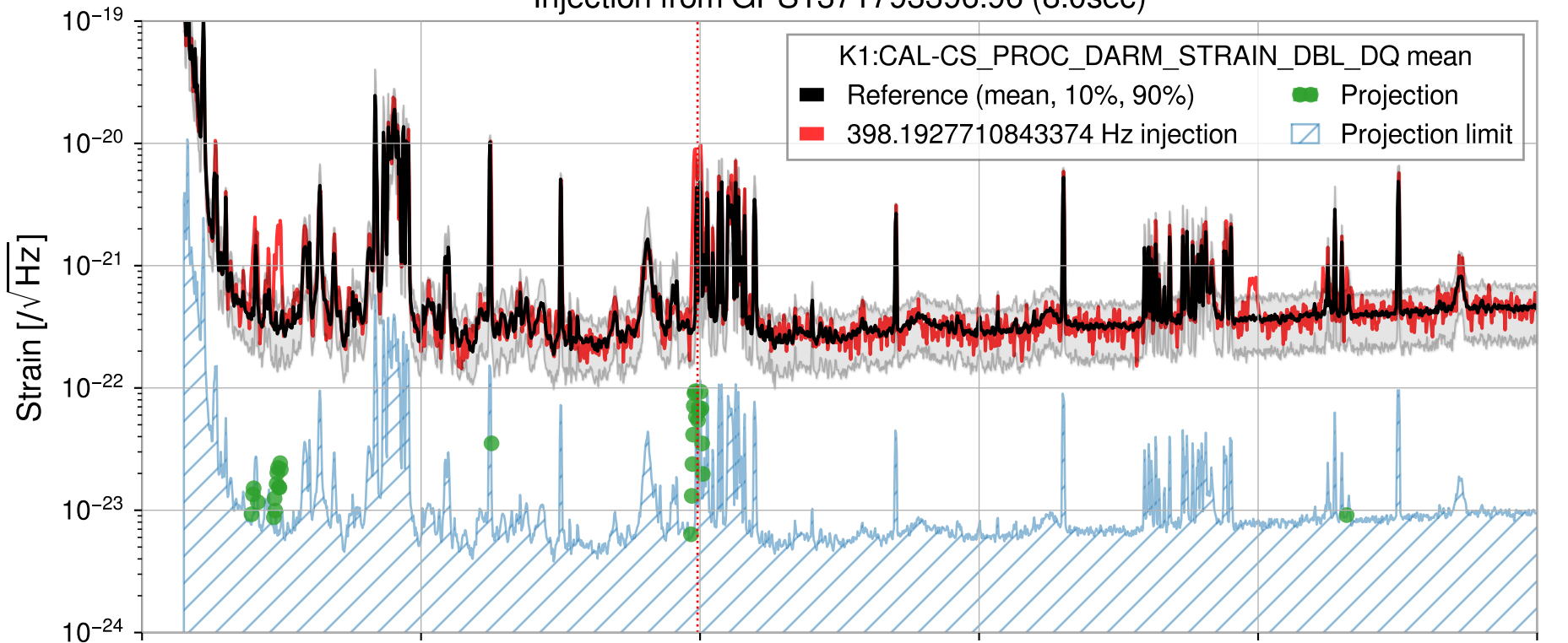
Injection from GPS1371793396.96 (8.0sec)
