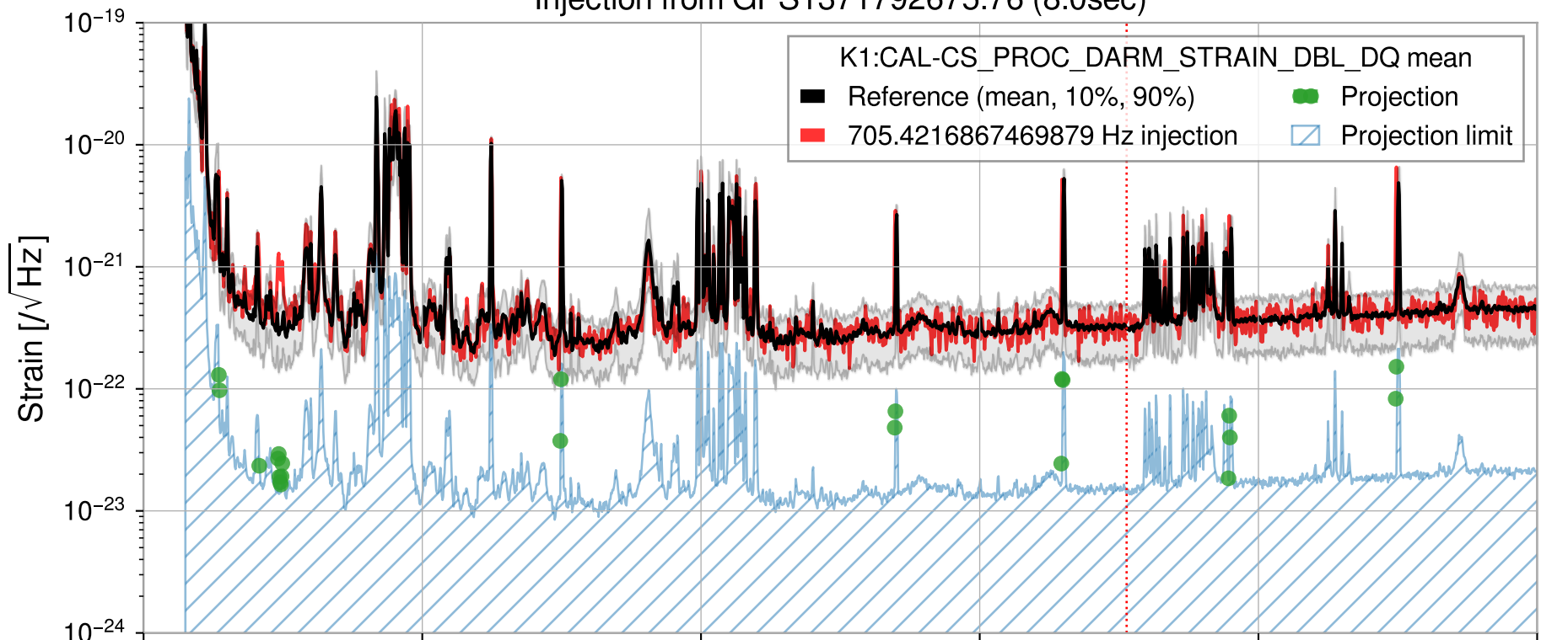
Injection from GPS1371792675.76 (8.0sec)
