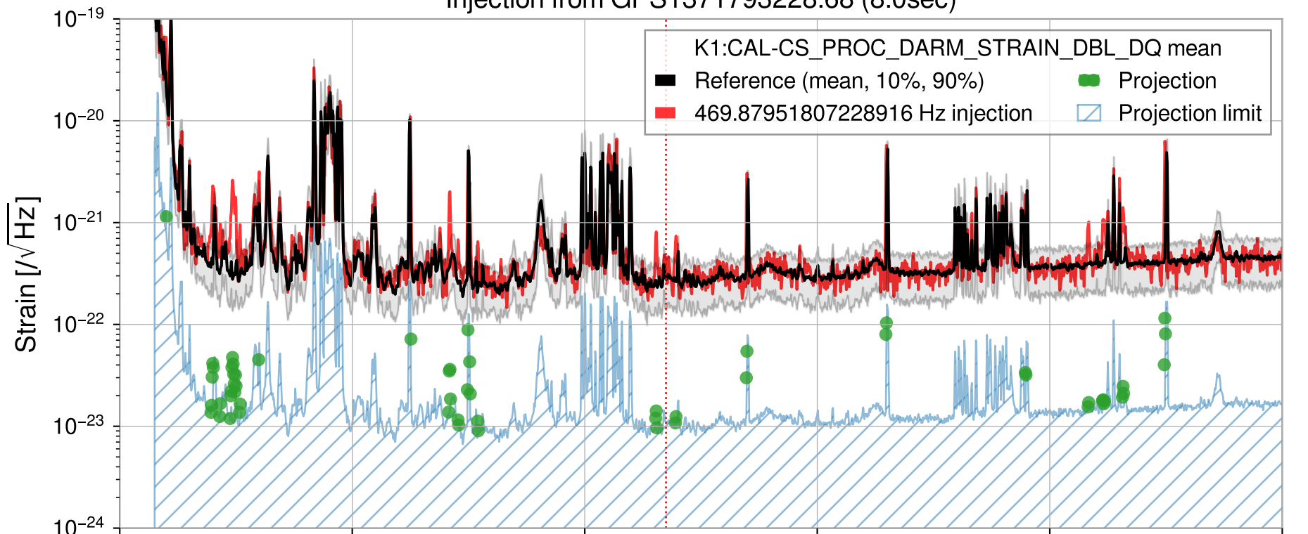
Injection from GPS1371793228.68 (8.0sec)
