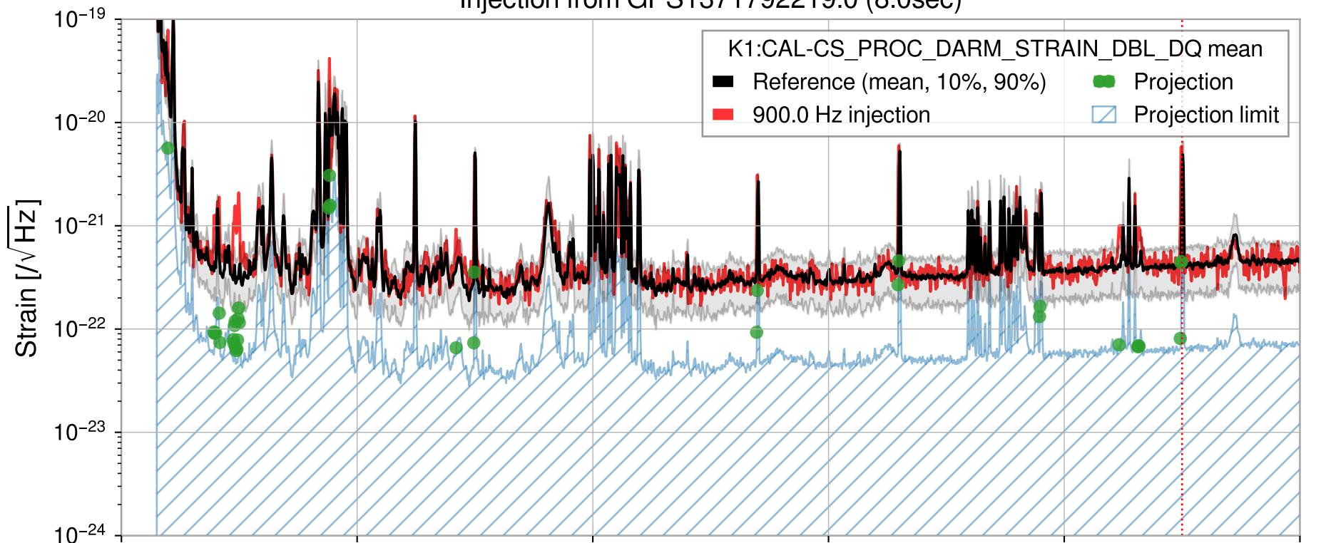
Injection from GPS1371792219.0 (8.0sec)
