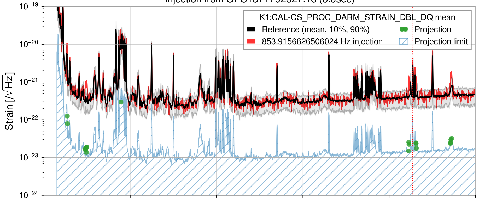
Injection from GPS1371792327.18 (8.0sec)
