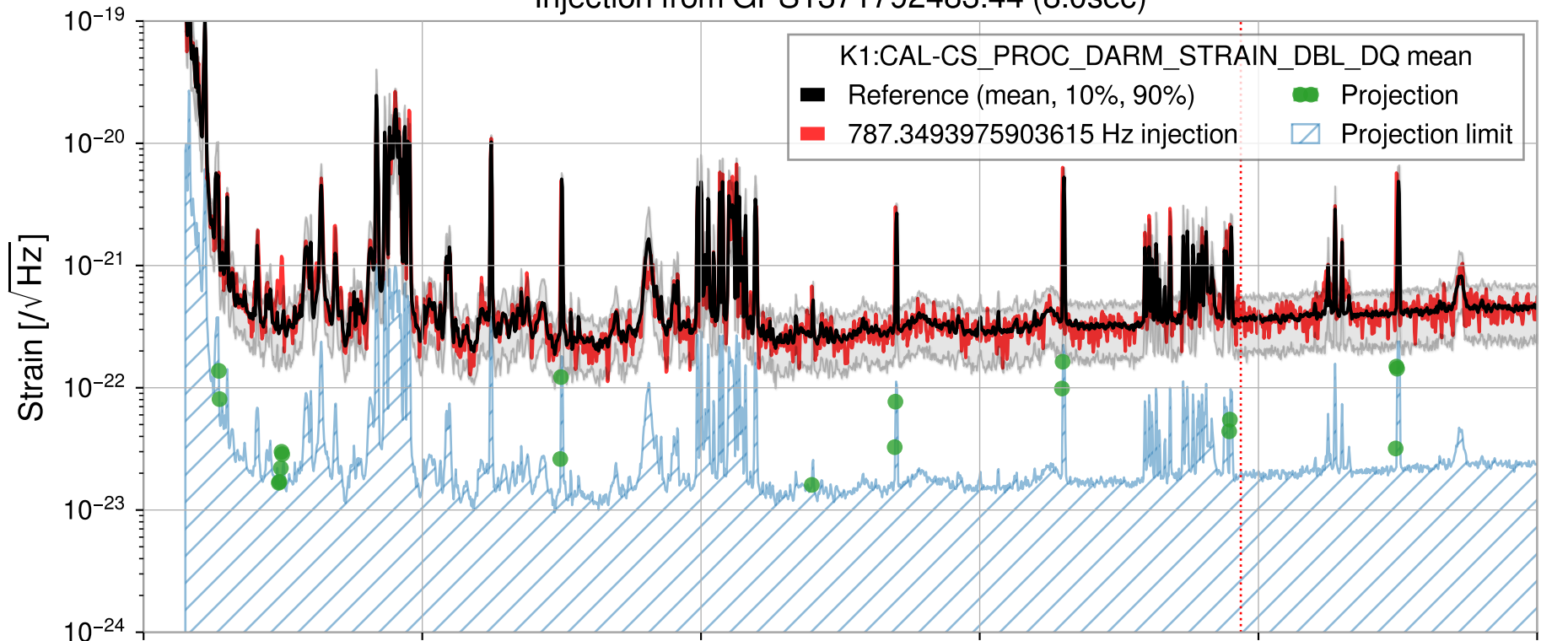
Injection from GPS1371792483.44 (8.0sec)
