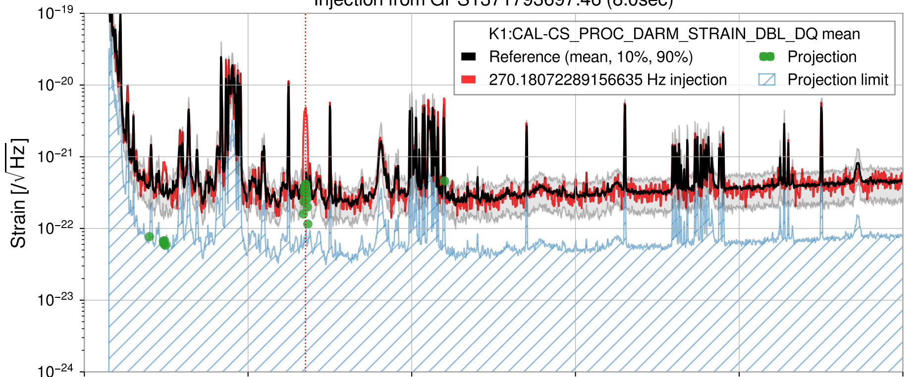
Injection from GPS1371793697.46 (8.0sec)
