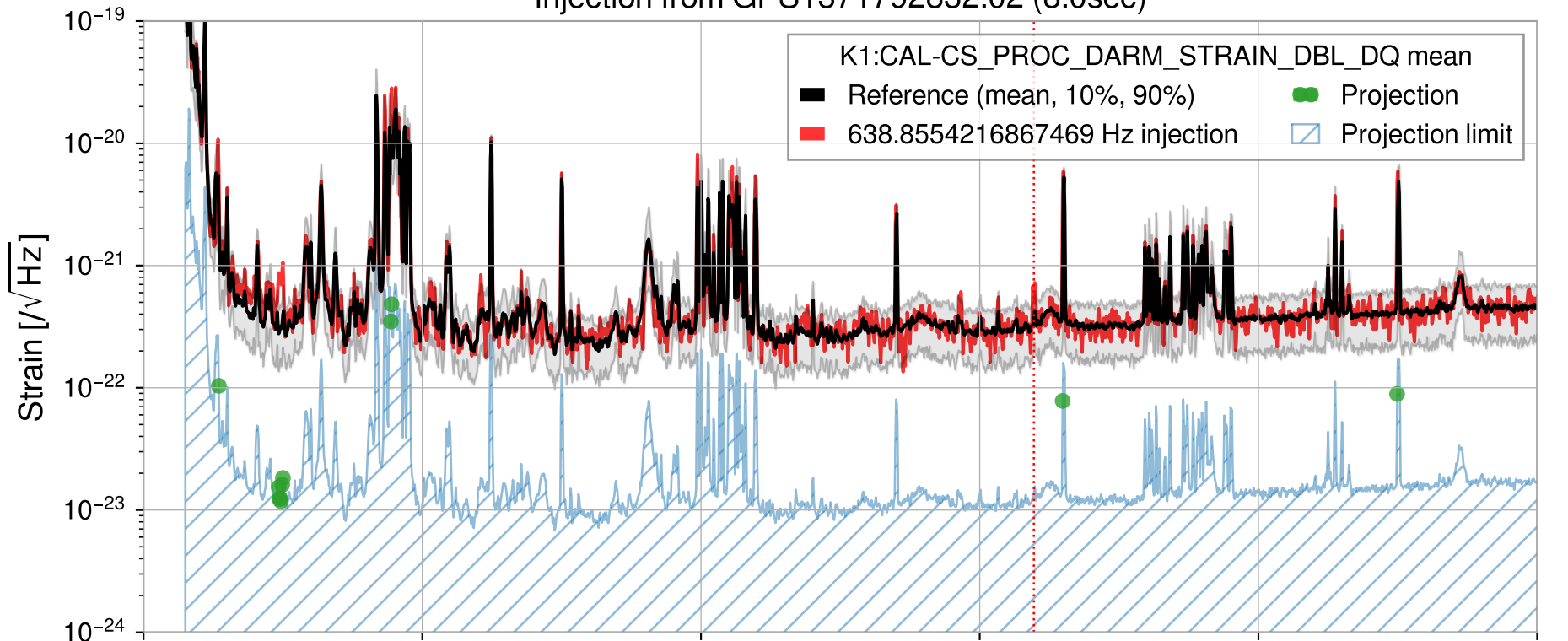
Injection from GPS1371792832.02 (8.0sec)
