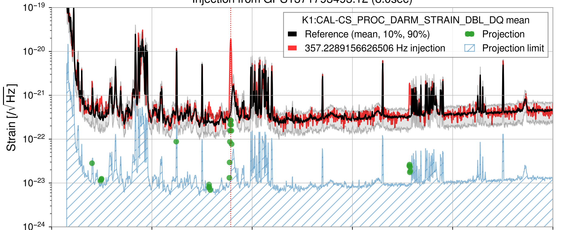
Injection from GPS1371793493.12 (8.0sec)
