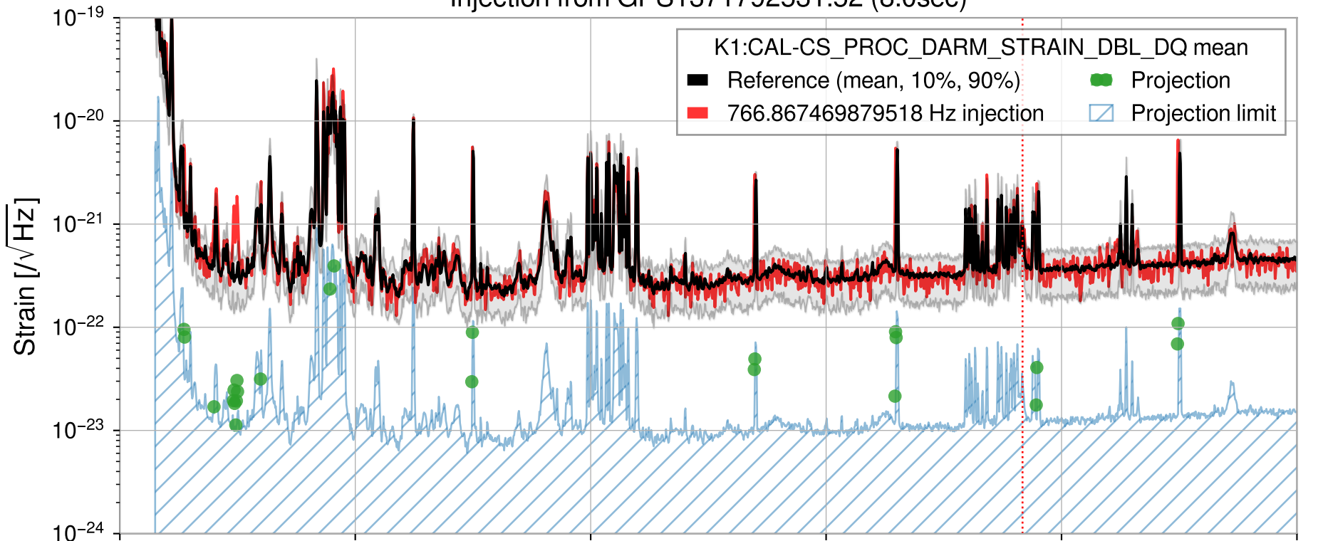
Injection from GPS1371792531.52 (8.0sec)
