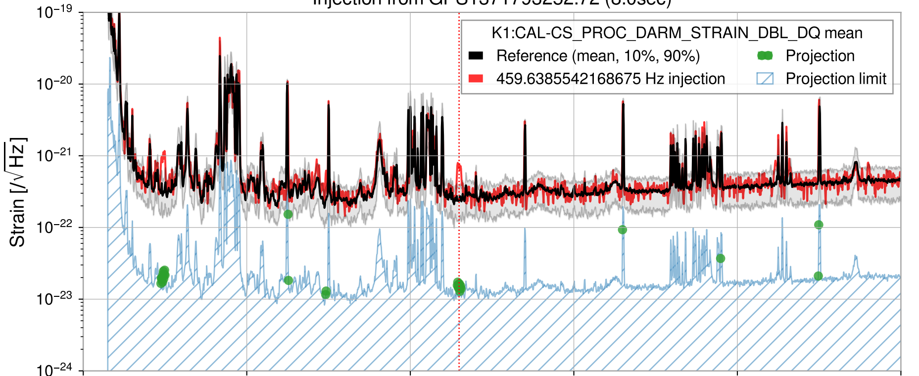
Injection from GPS1371793252.72 (8.0sec)
