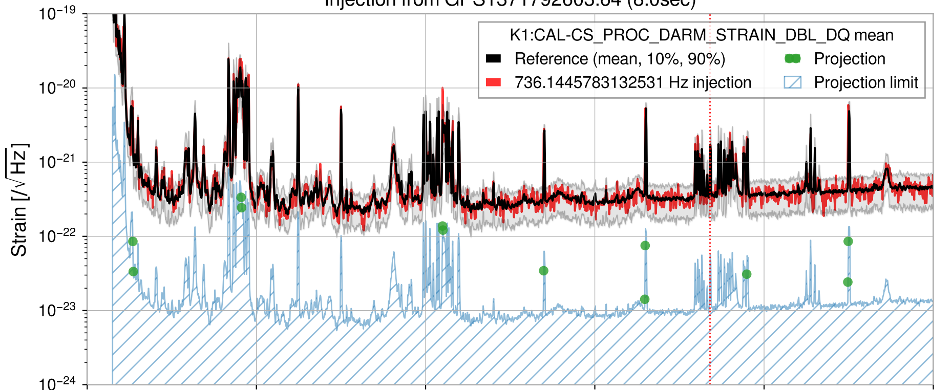
Injection from GPS1371792603.64 (8.0sec)
