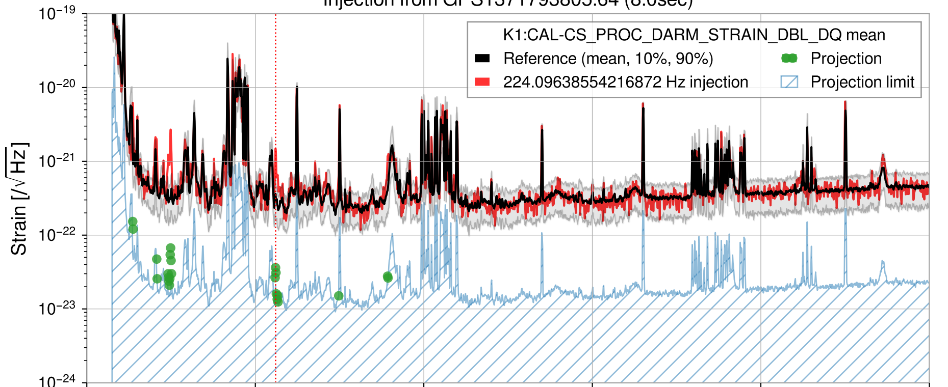
Injection from GPS1371793805.64 (8.0sec)
