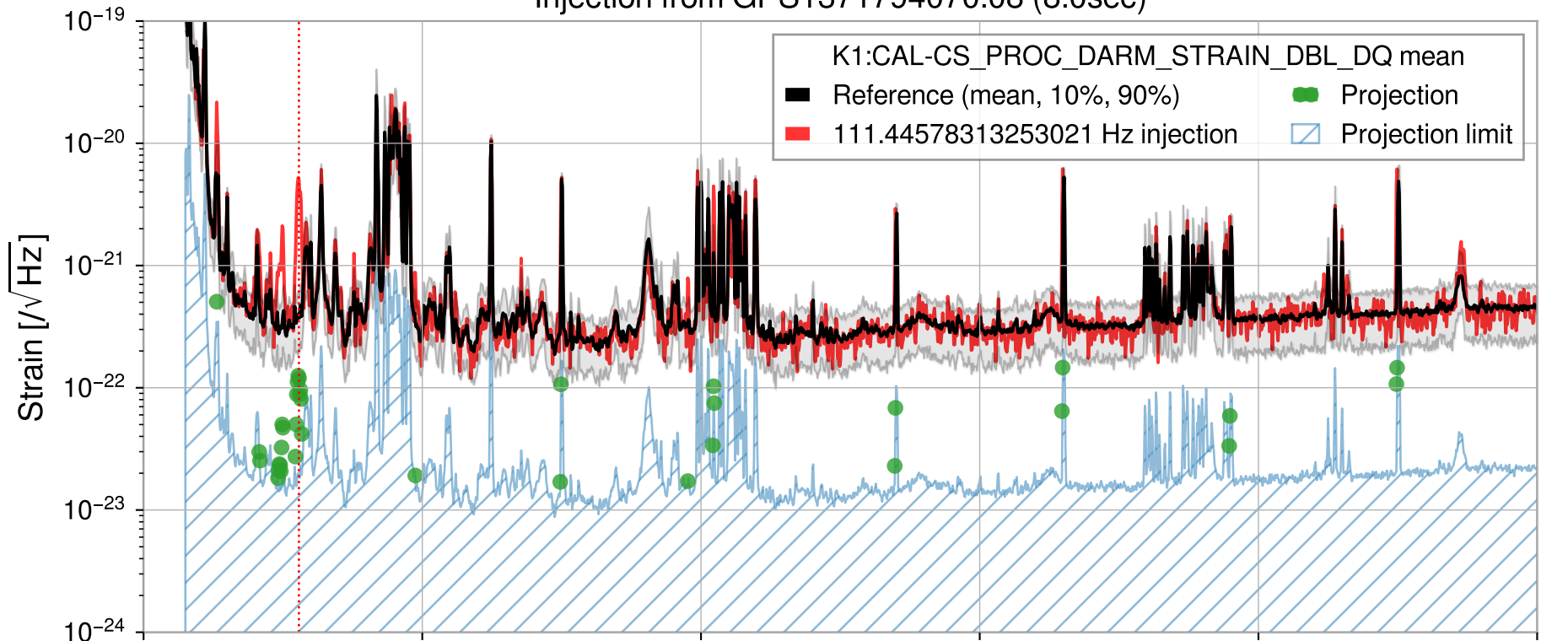
Injection from GPS1371794070.08 (8.0sec)
