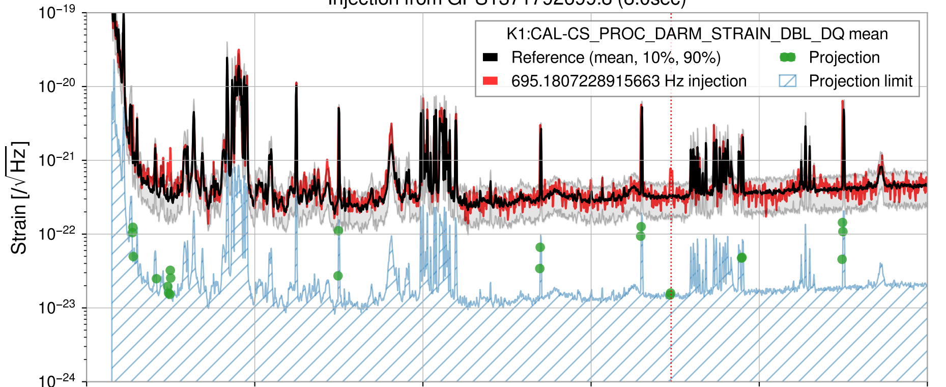
Injection from GPS1371792699.8 (8.0sec)
