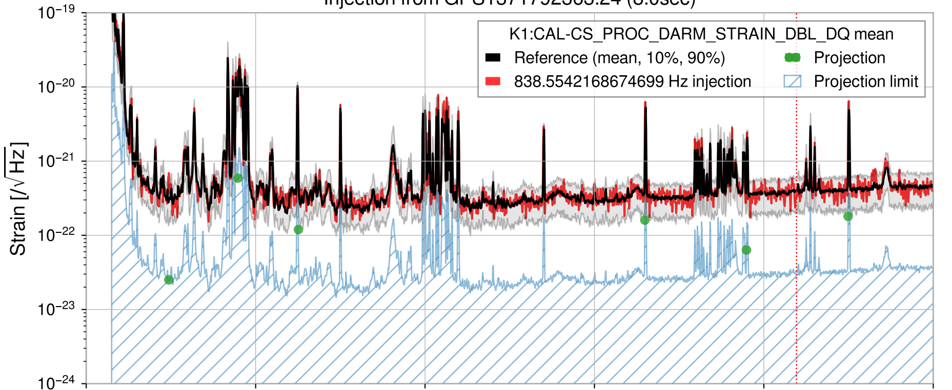
Injection from GPS1371792363.24 (8.0sec)
