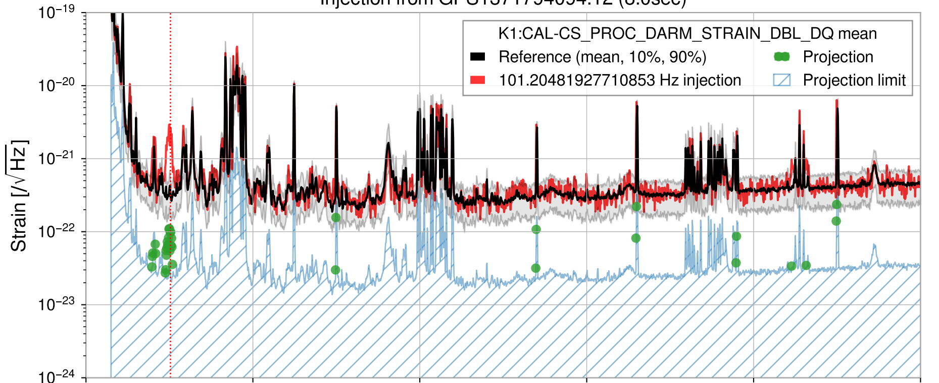
Injection from GPS1371794094.12 (8.0sec)
