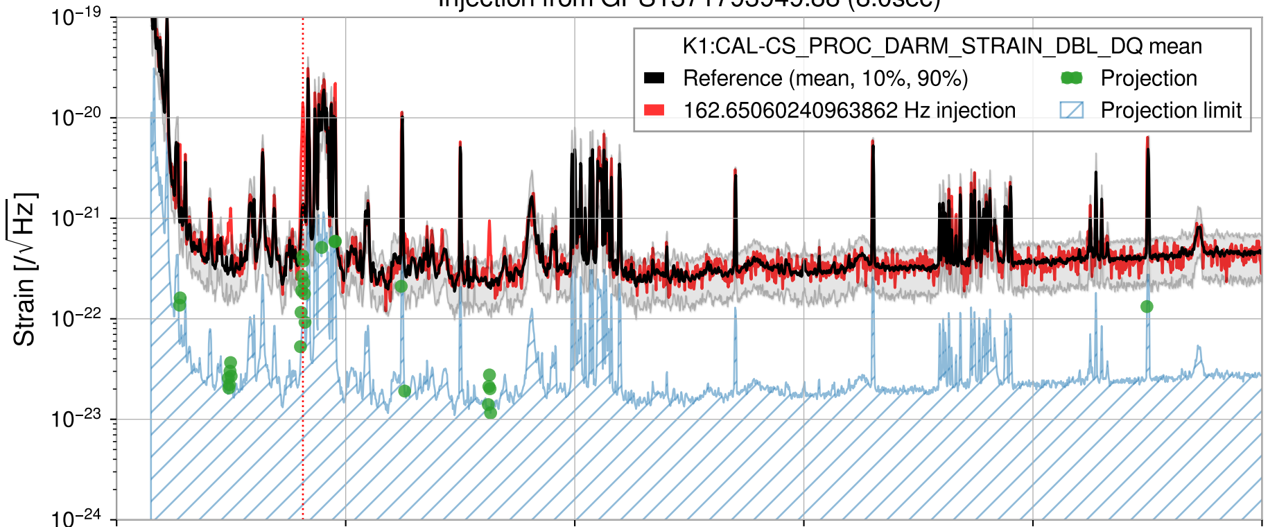
Injection from GPS1371793949.88 (8.0sec)
