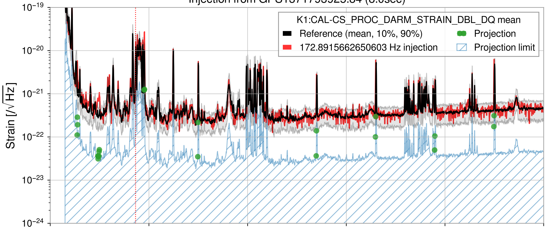
Injection from GPS1371793925.84 (8.0sec)
