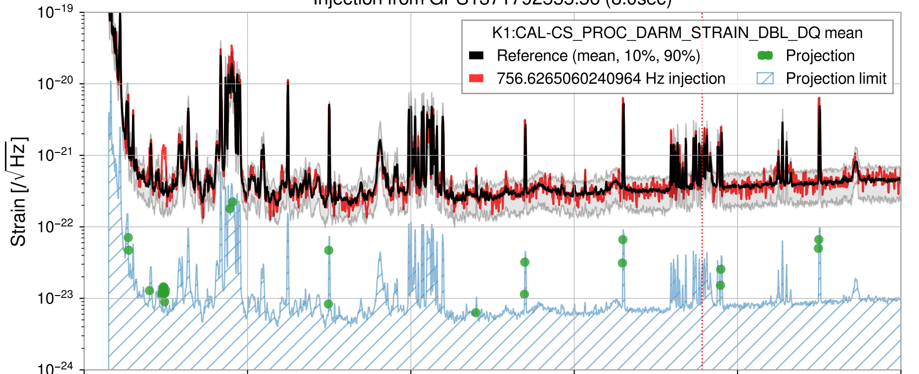
Injection from GPS1371792555.56 (8.0sec)
