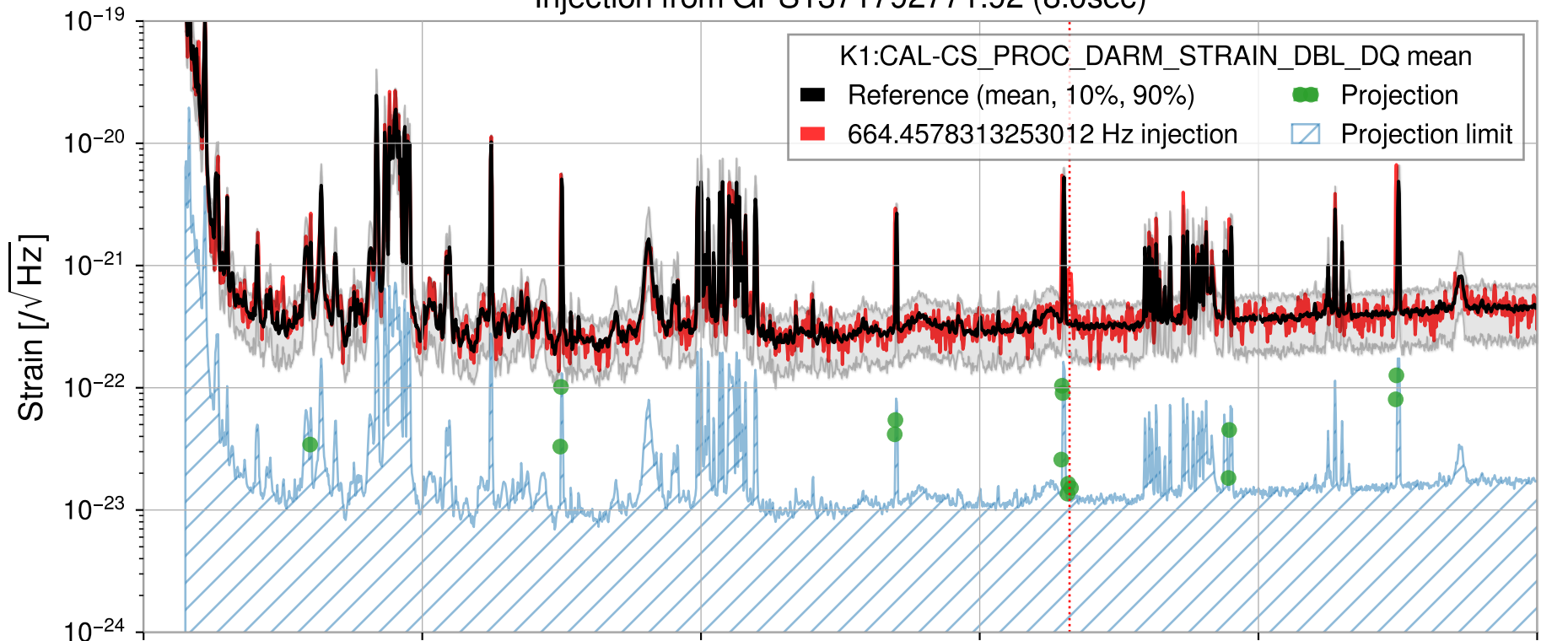
Injection from GPS1371792771.92 (8.0sec)
