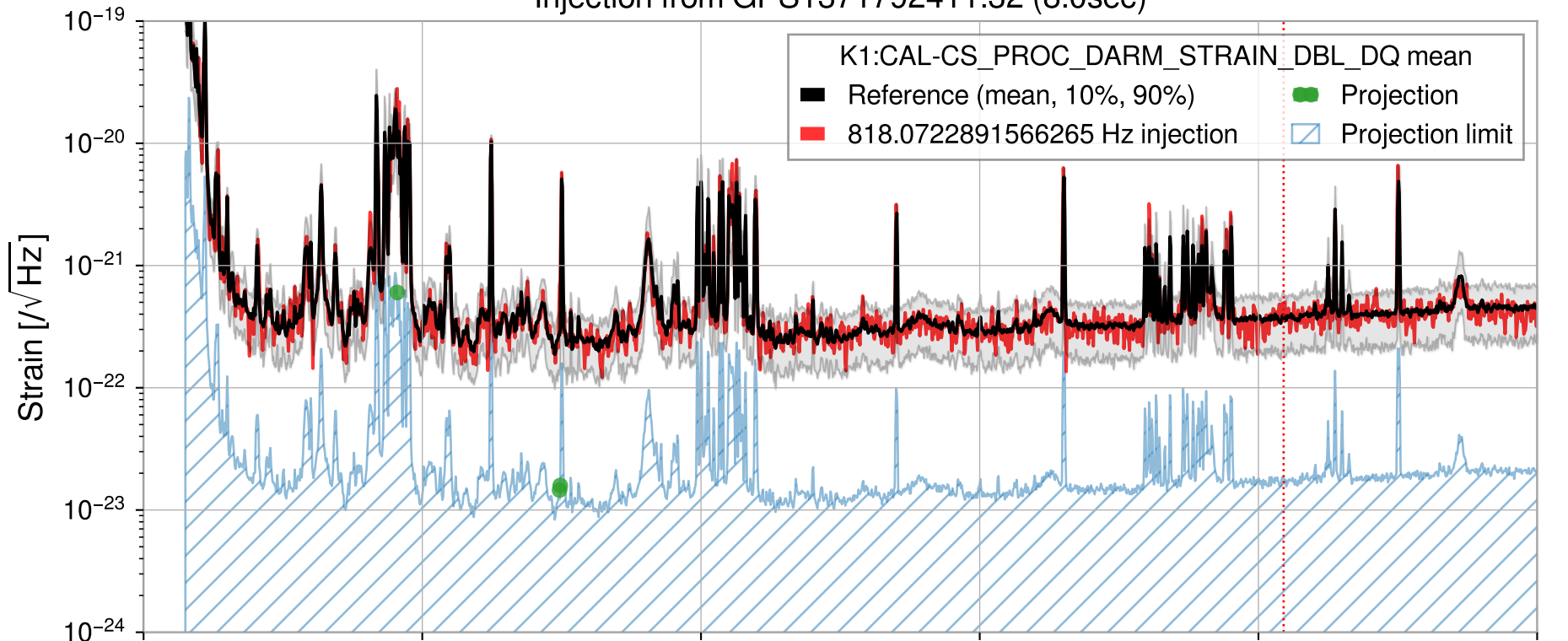
Injection from GPS1371792411.32 (8.0sec)
