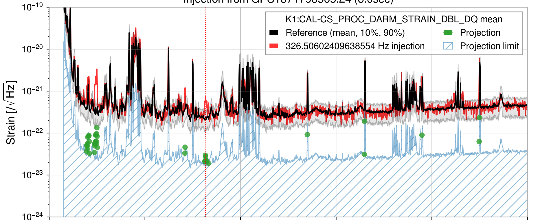
Injection from GPS1371793565.24 (8.0sec)
