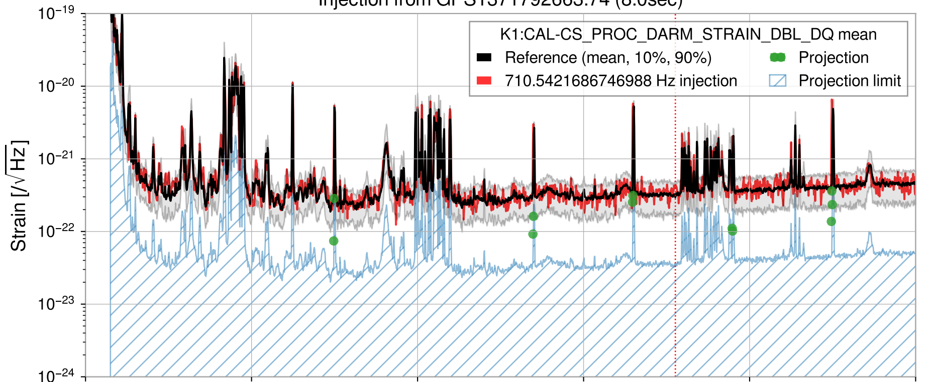
Injection from GPS1371792663.74 (8.0sec)
