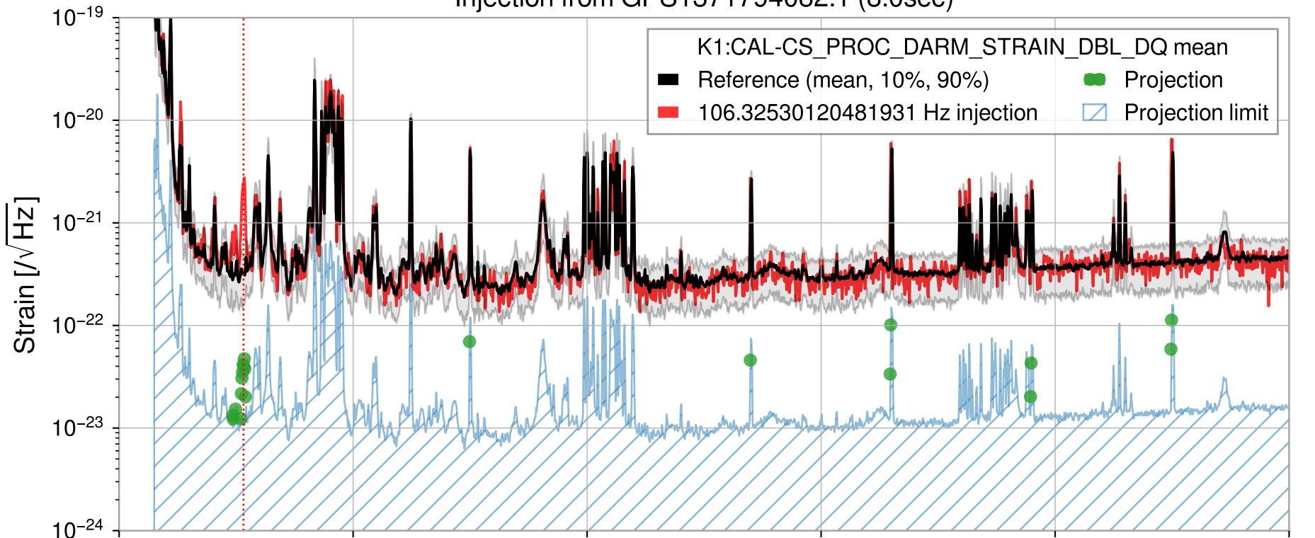
Injection from GPS1371794082.1 (8.0sec)
