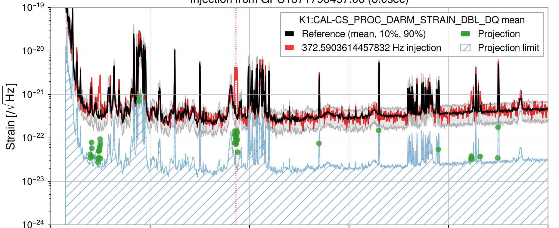
Injection from GPS1371793457.06 (8.0sec)
