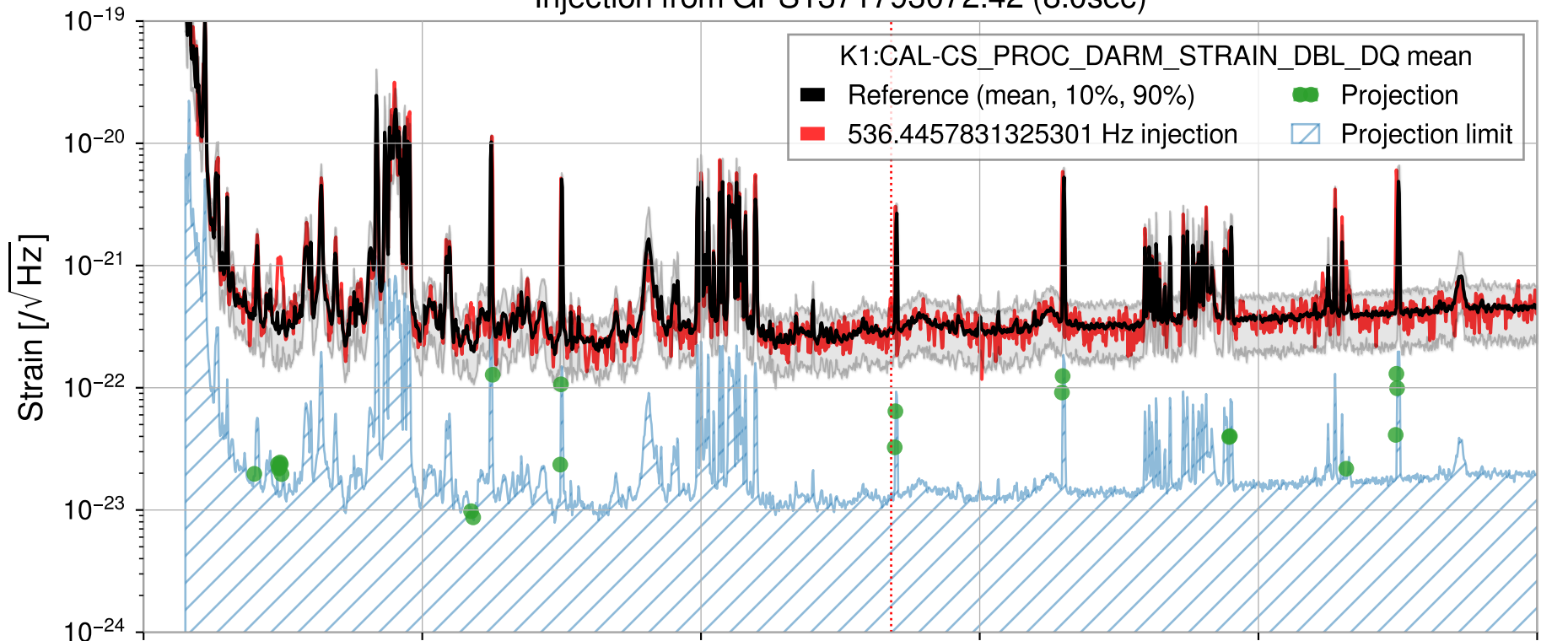
Injection from GPS1371793072.42 (8.0sec)
