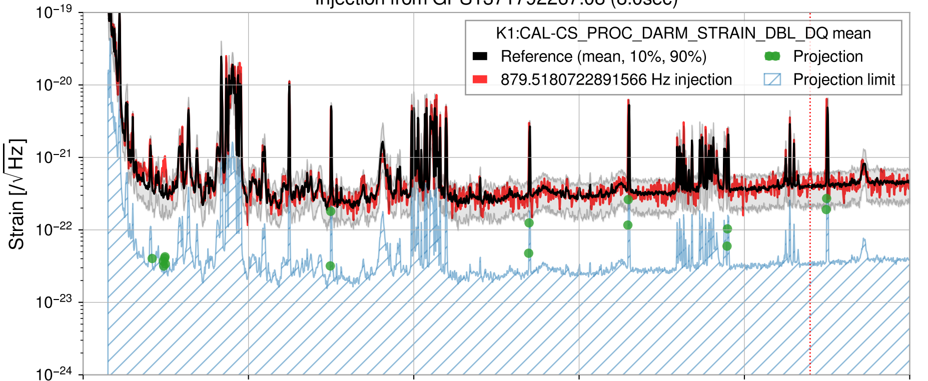
Injection from GPS1371792267.08 (8.0sec)
