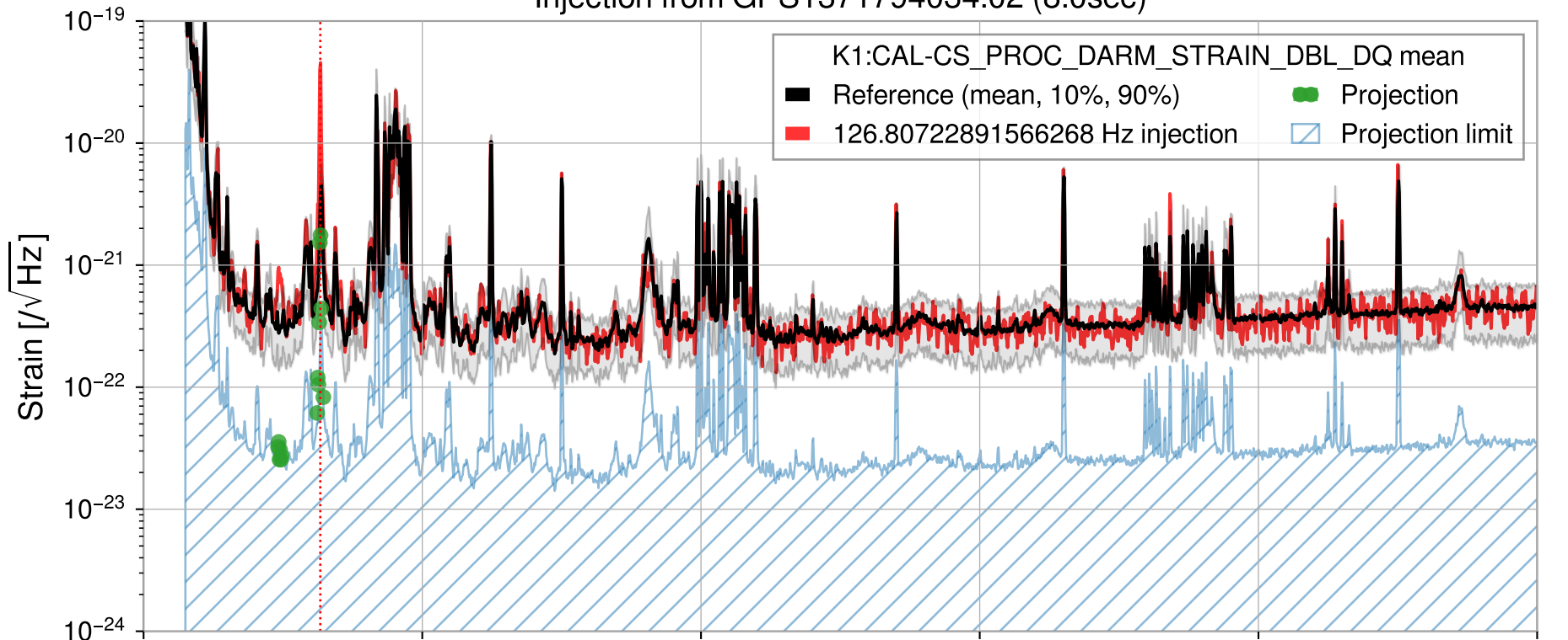
Injection from GPS1371794034.02 (8.0sec)
