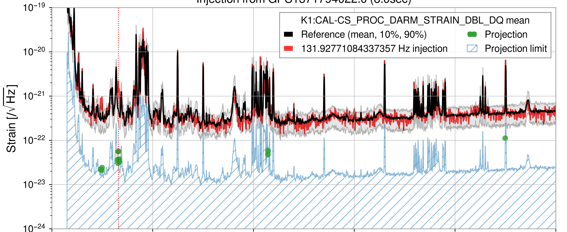
Injection from GPS1371794022.0 (8.0sec)
