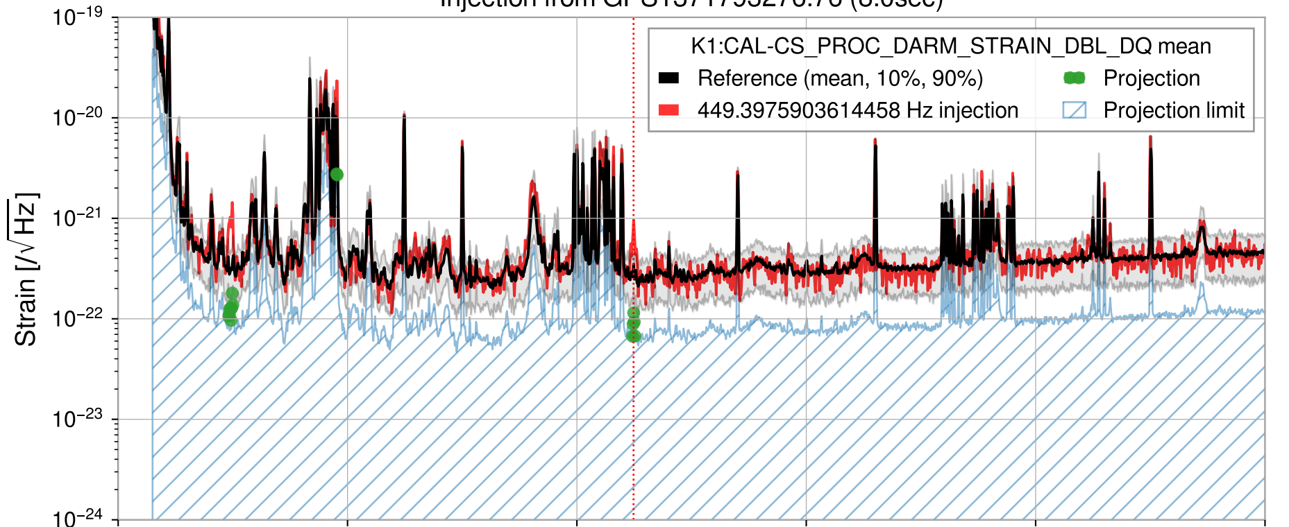
Injection from GPS1371793276.76 (8.0sec)
