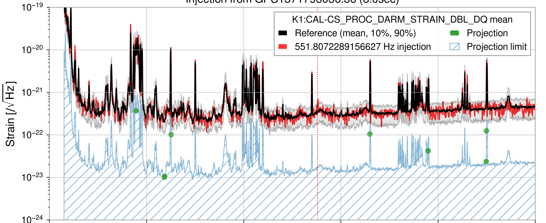
Injection from GPS1371793036.36 (8.0sec)
