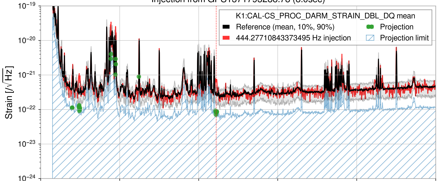
Injection from GPS1371793288.78 (8.0sec)
