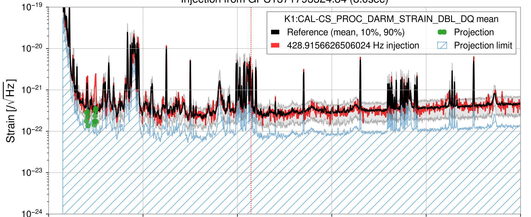
Injection from GPS1371793324.84 (8.0sec)
