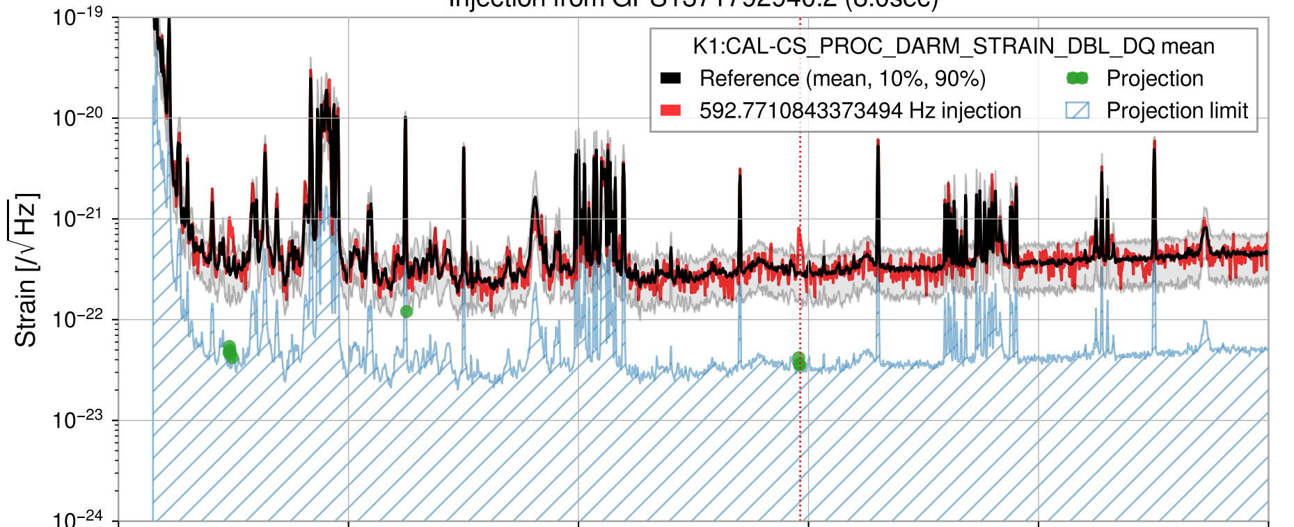
Injection from GPS1371792940.2 (8.0sec)
