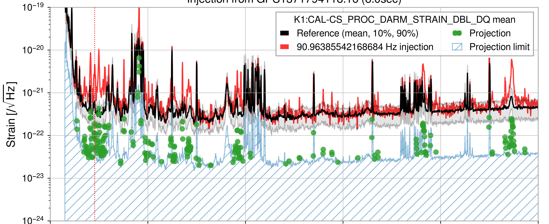
Injection from GPS1371794118.16 (8.0sec)
