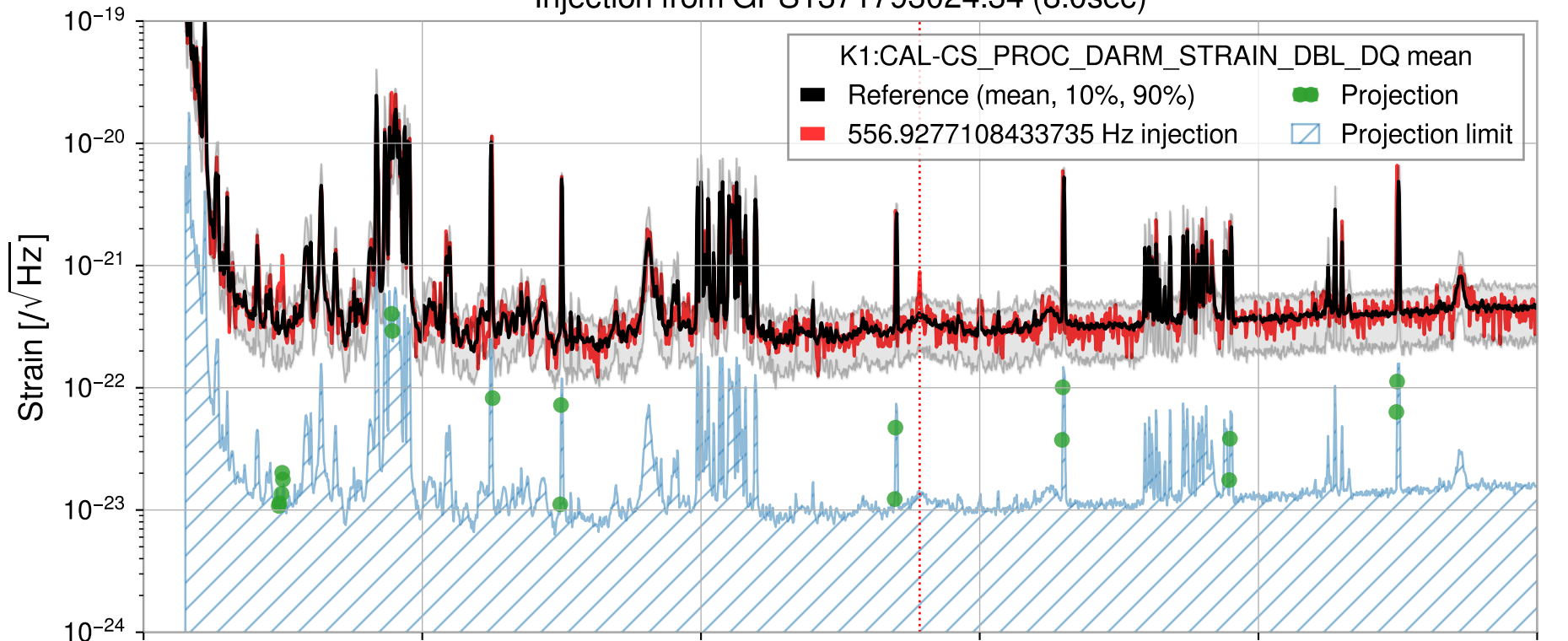
Injection from GPS1371793024.34 (8.0sec)
