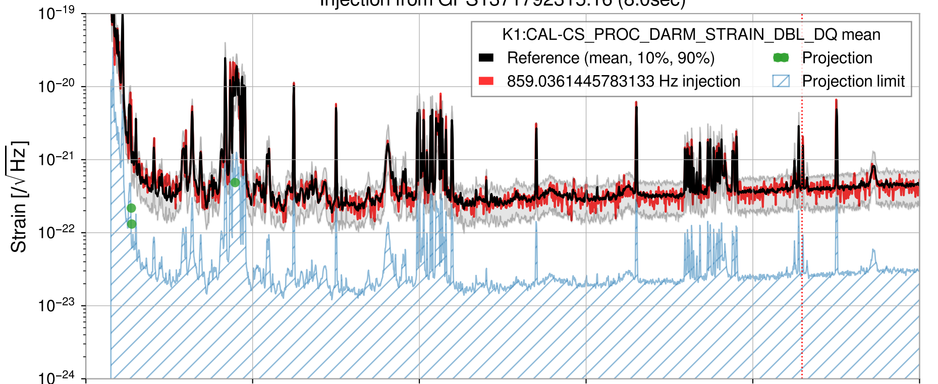
Injection from GPS1371792315.16 (8.0sec)
