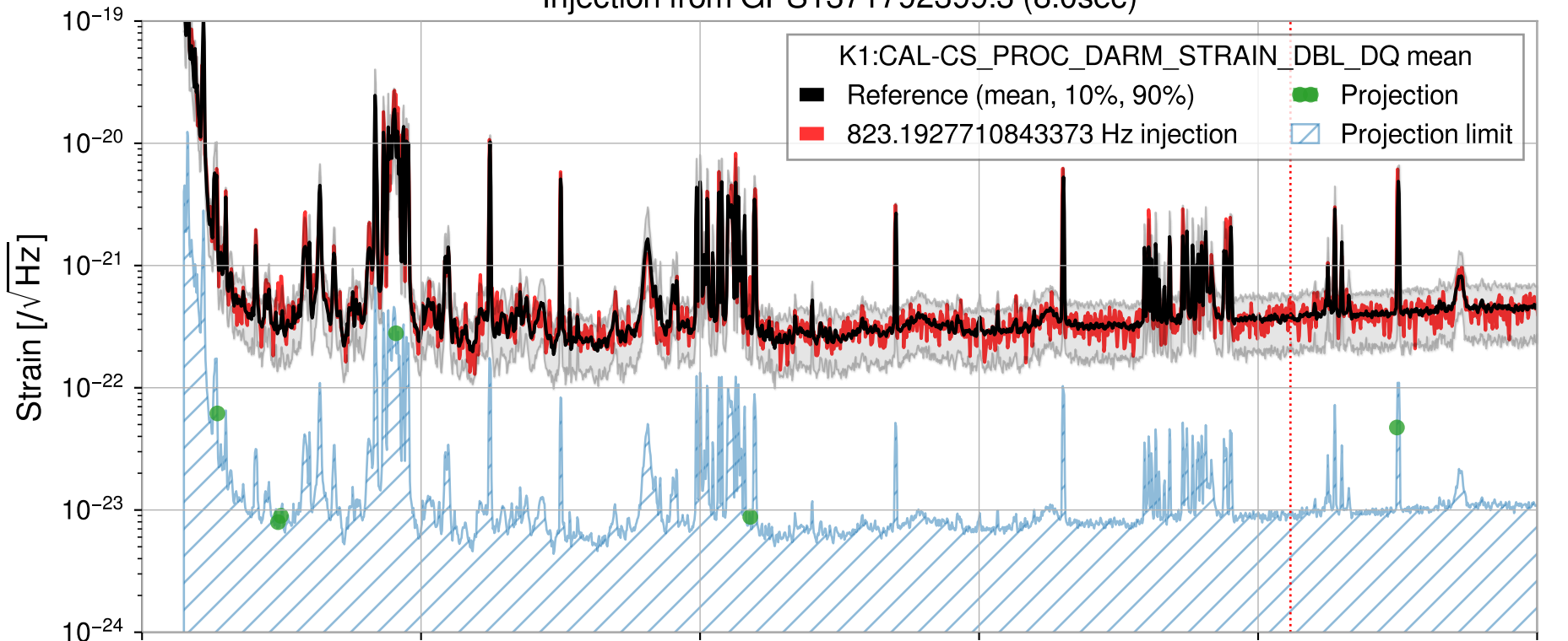
Injection from GPS1371792399.3 (8.0sec)
