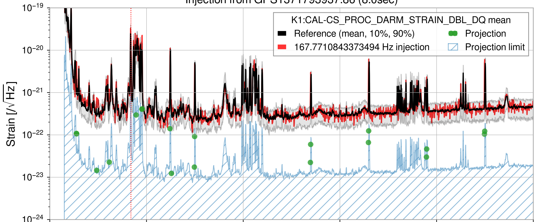
Injection from GPS1371793937.86 (8.0sec)
