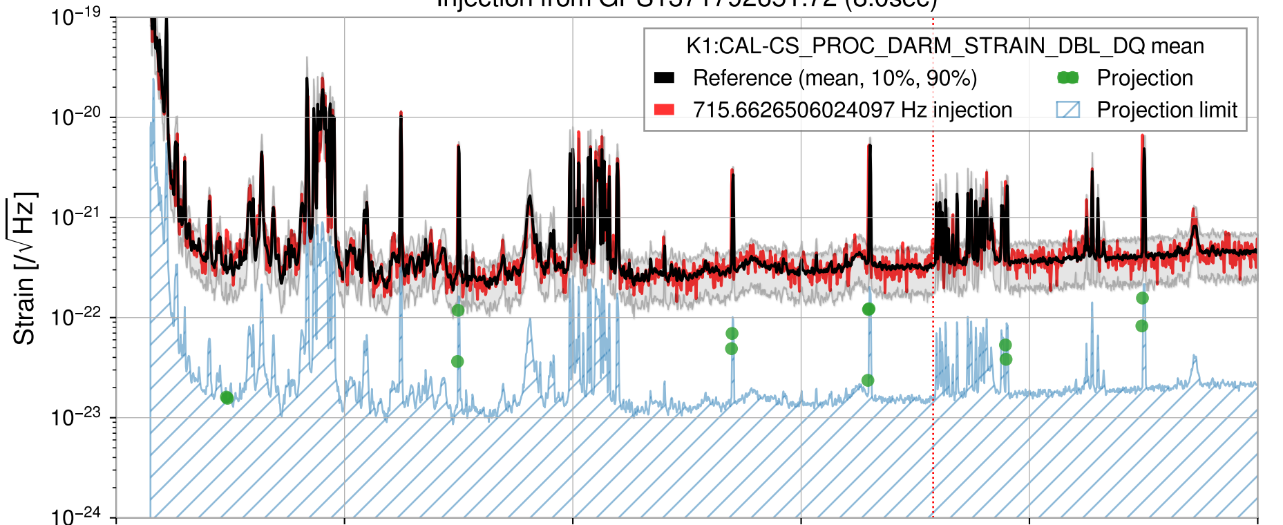
Injection from GPS1371792651.72 (8.0sec)
