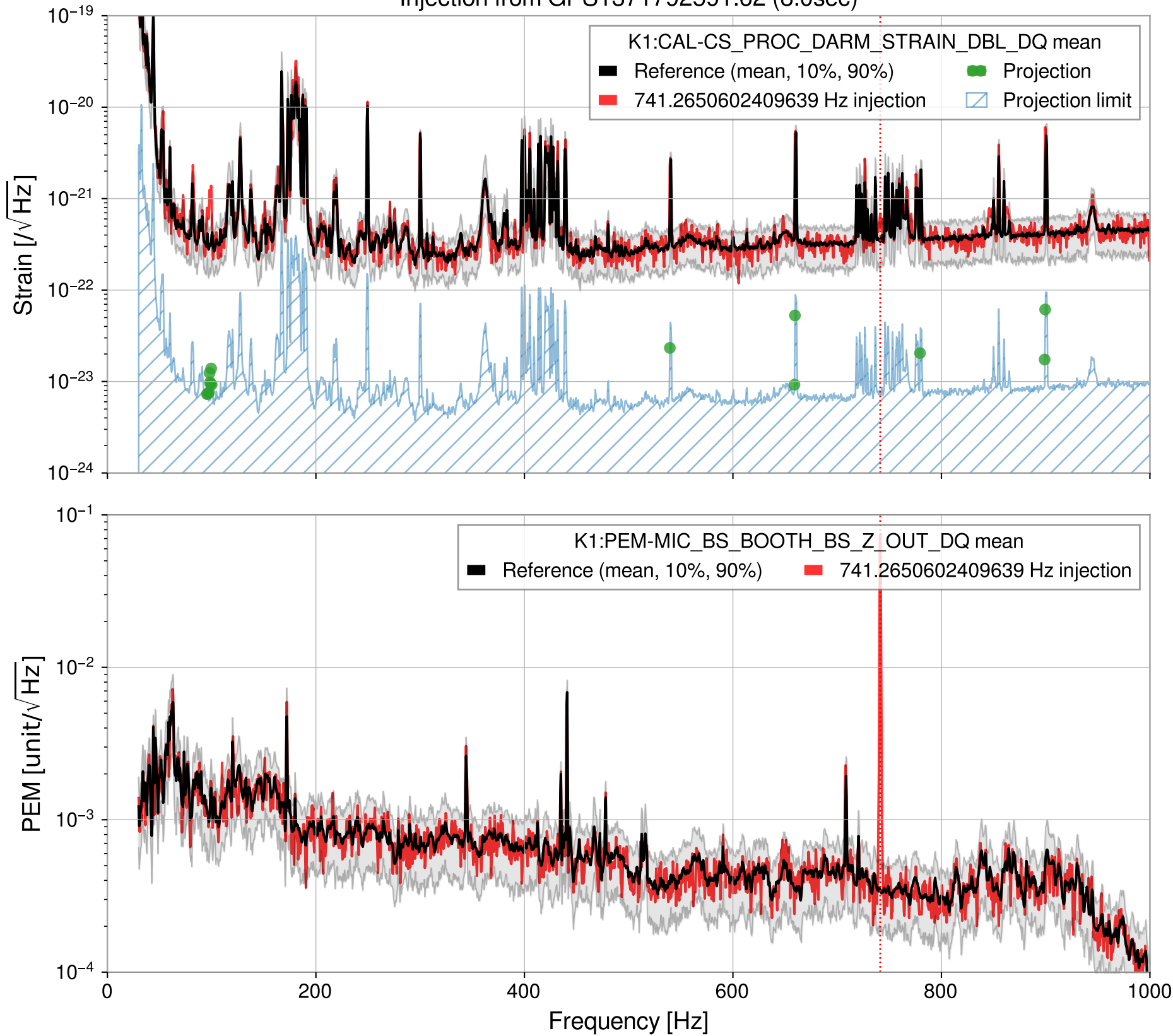
Injection from GPS1371792591.62 (8.0sec)
