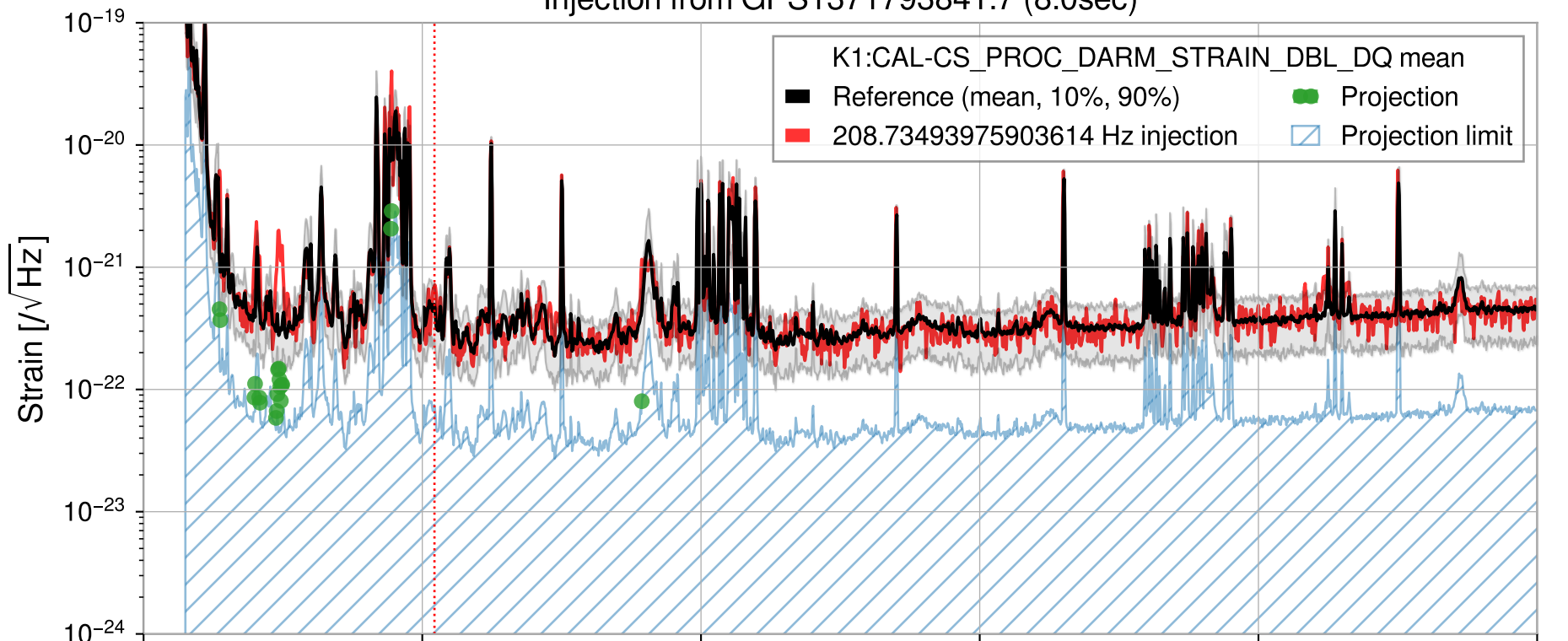
Injection from GPS1371793841.7 (8.0sec)
