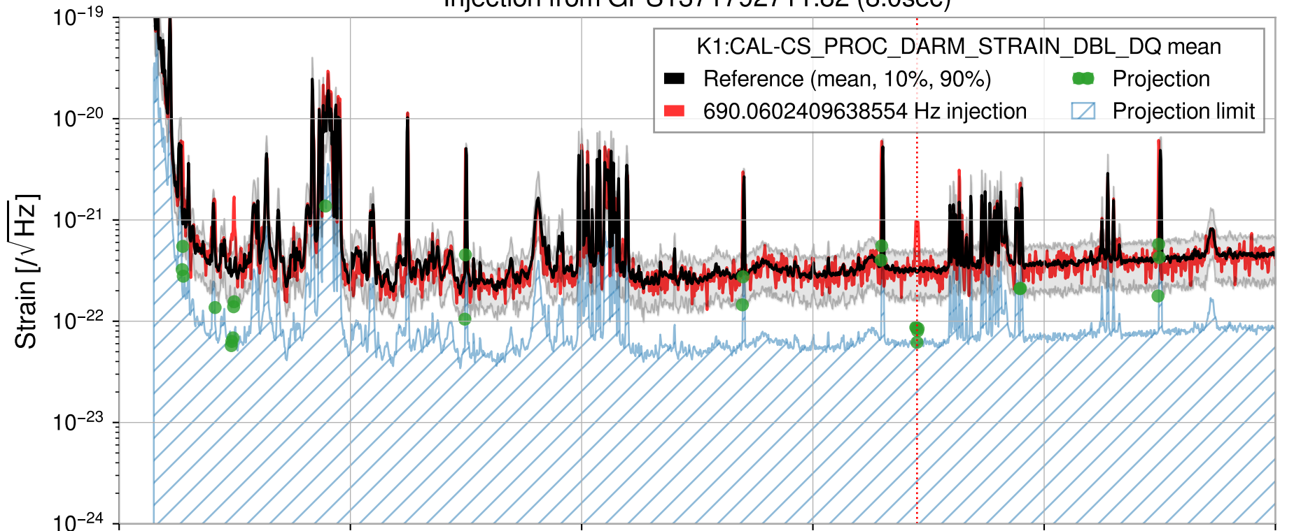
Injection from GPS1371792711.82 (8.0sec)
