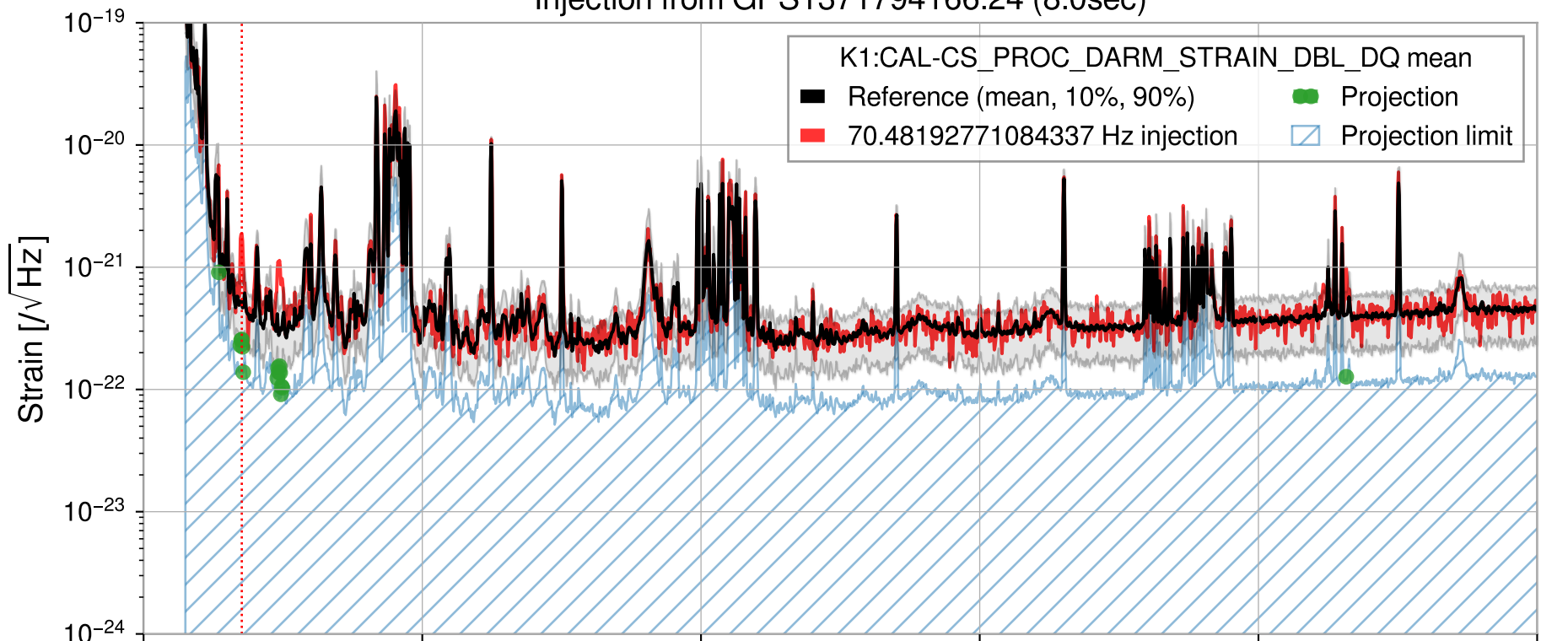
Injection from GPS1371794166.24 (8.0sec)
