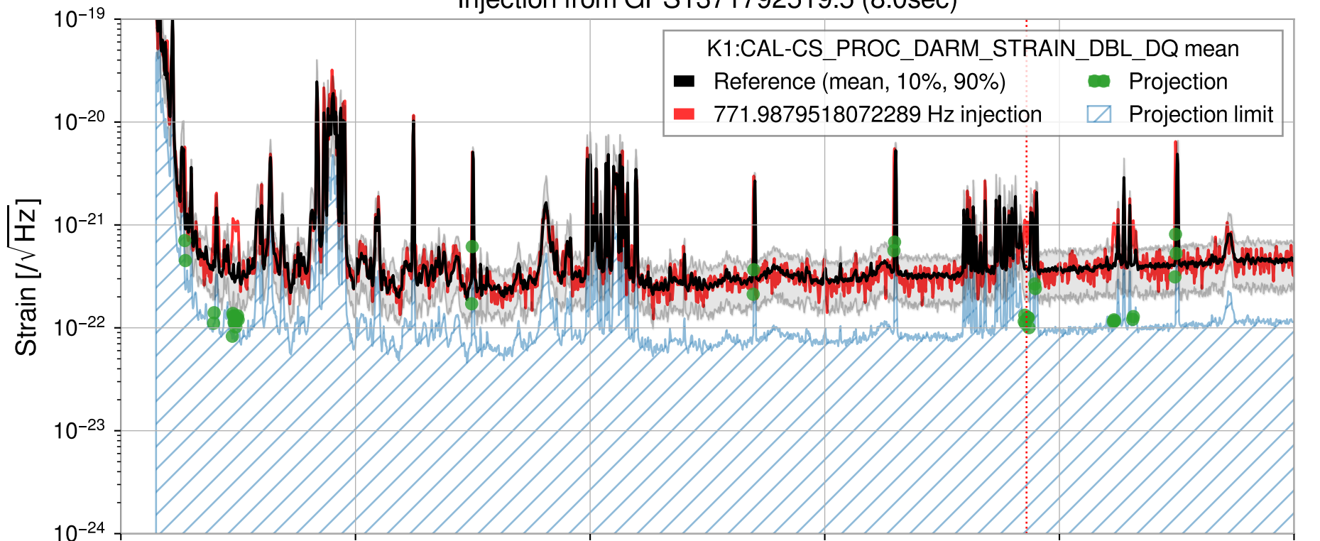
Injection from GPS1371792519.5 (8.0sec)
