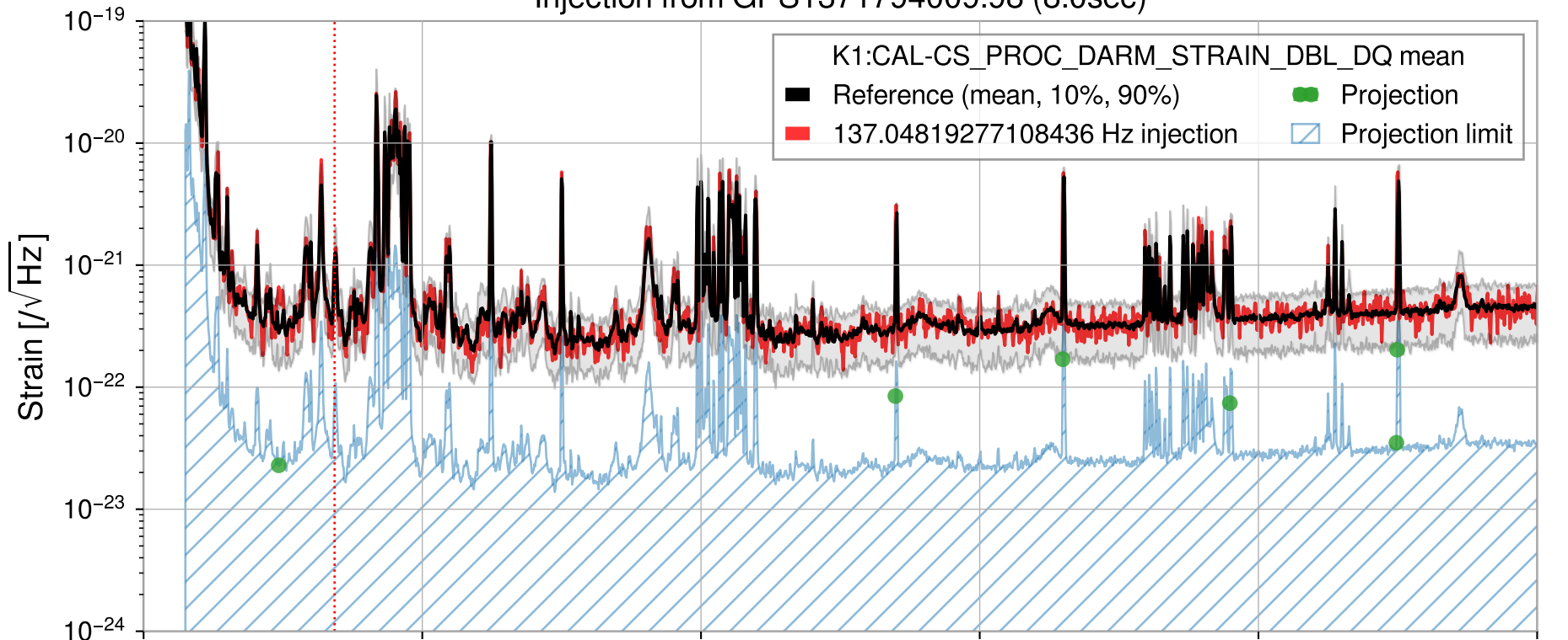
Injection from GPS1371794009.98 (8.0sec)
