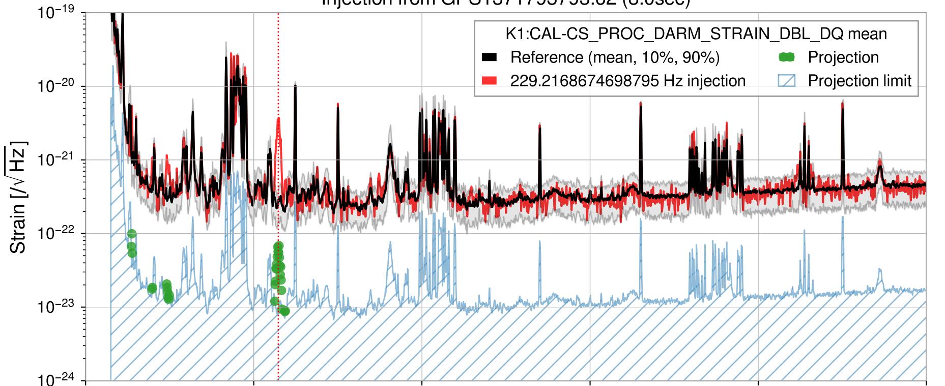
Injection from GPS1371793793.62 (8.0sec)
