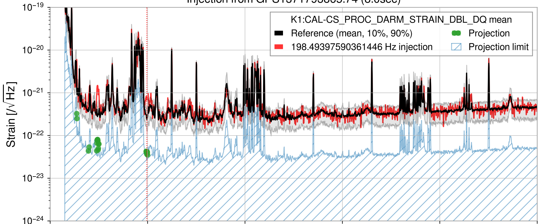
Injection from GPS1371793865.74 (8.0sec)
