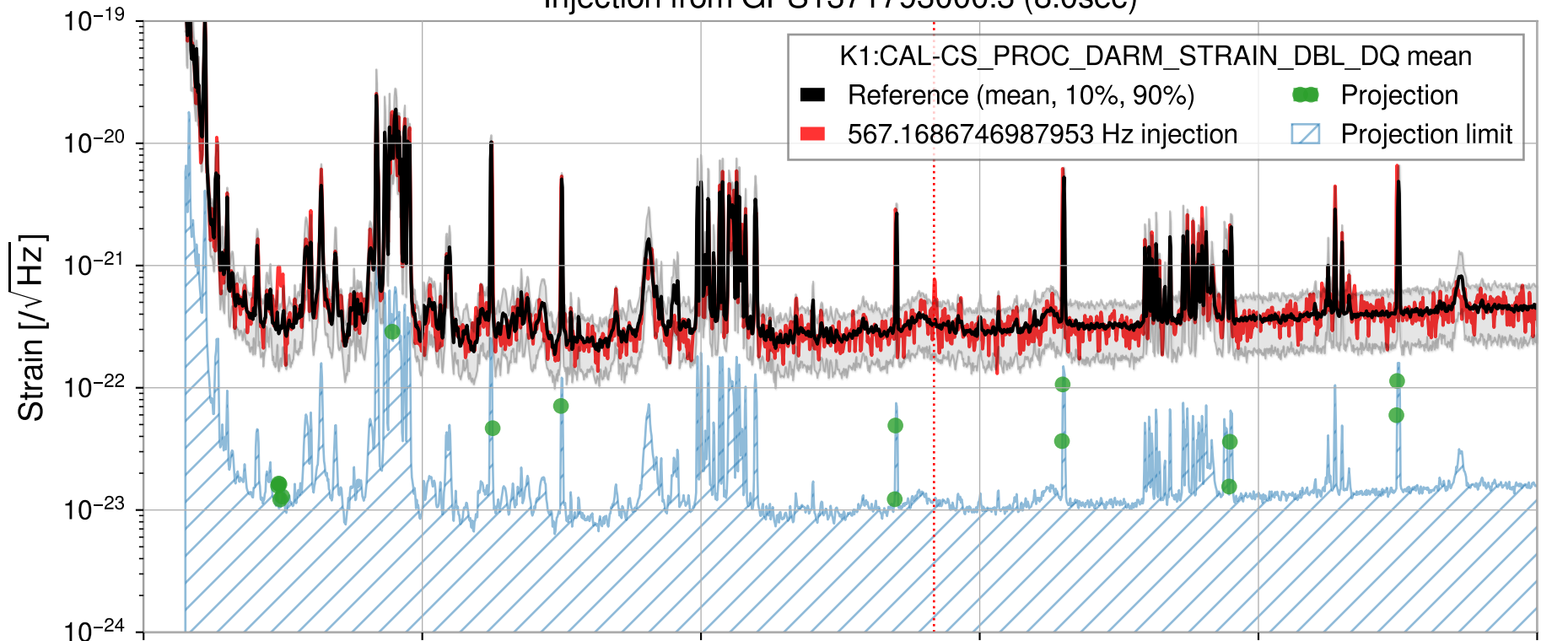
Injection from GPS1371793000.3 (8.0sec)
