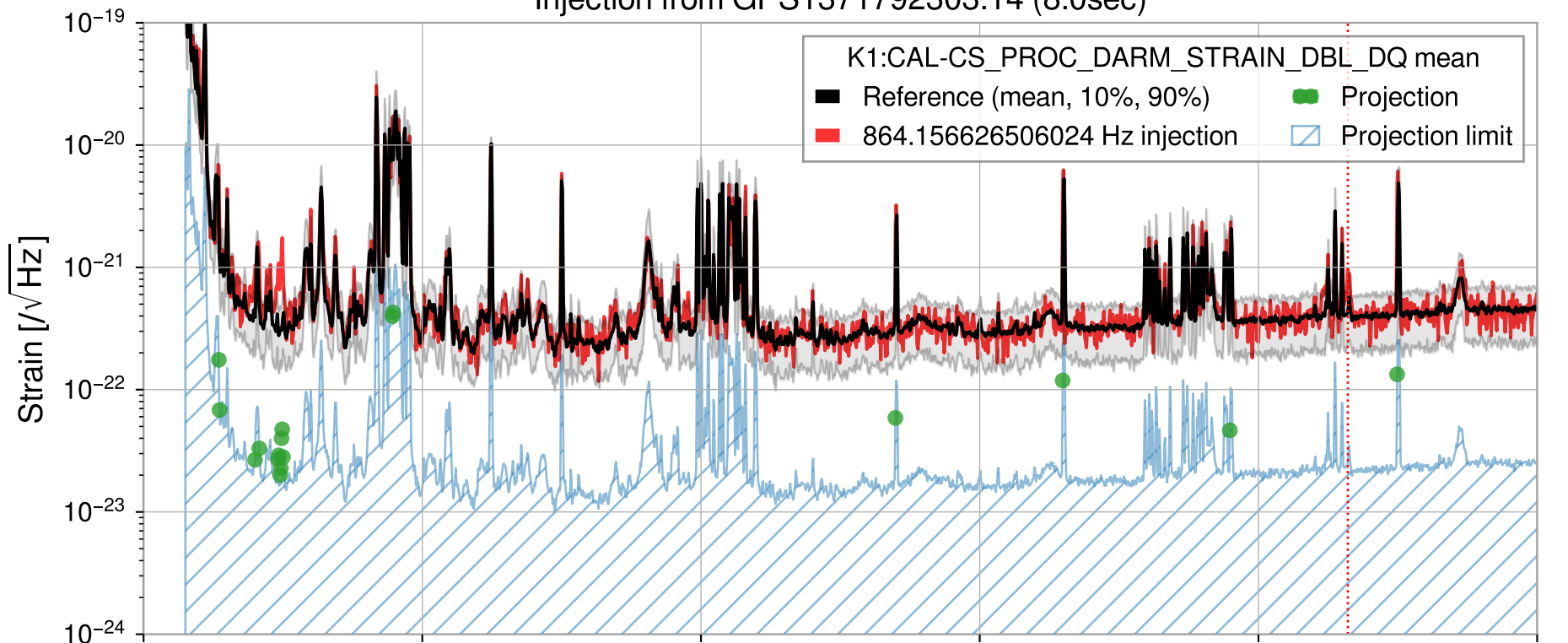
Injection from GPS1371792303.14 (8.0sec)
