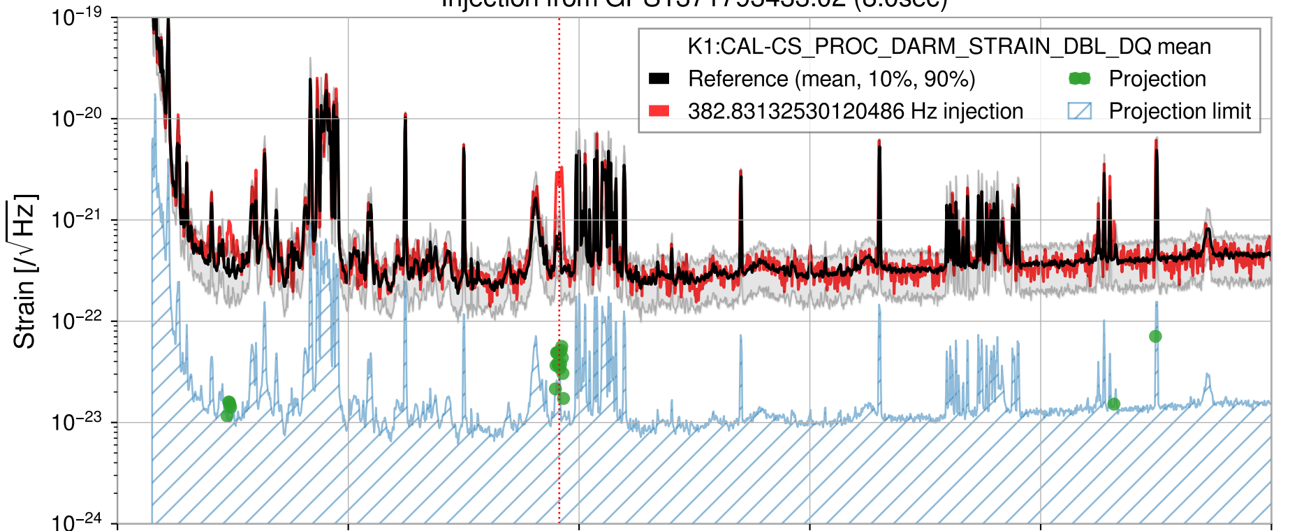
Injection from GPS1371793433.02 (8.0sec)
