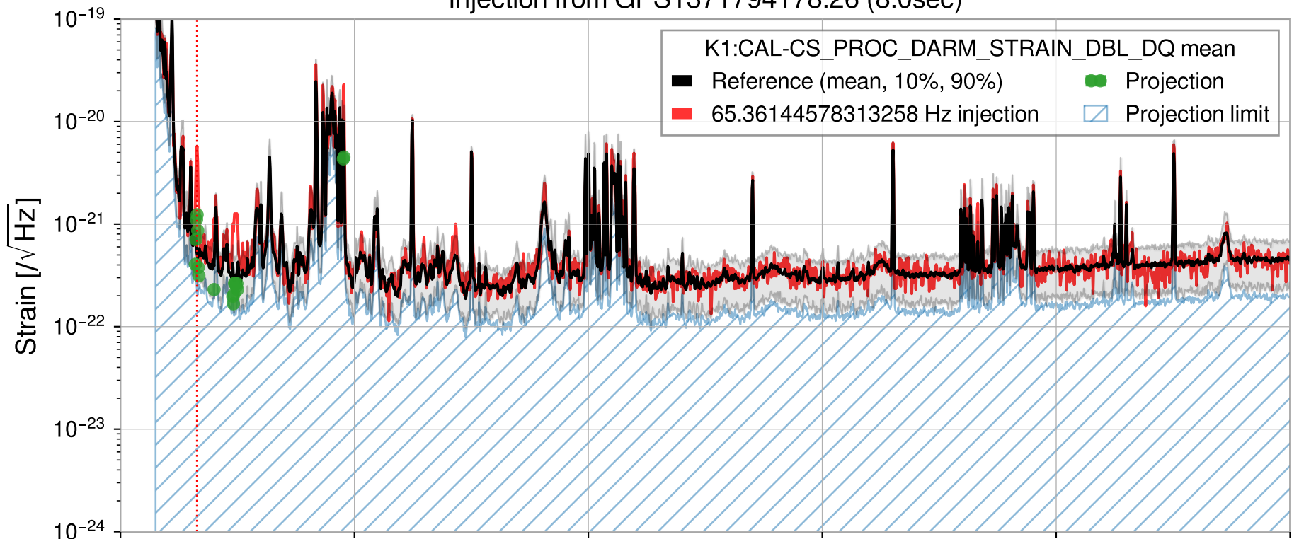
Injection from GPS1371794178.26 (8.0sec)
