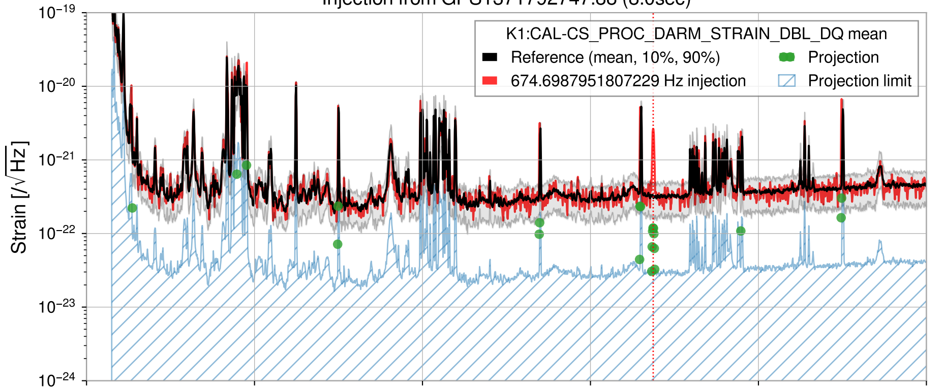
Injection from GPS1371792747.88 (8.0sec)
