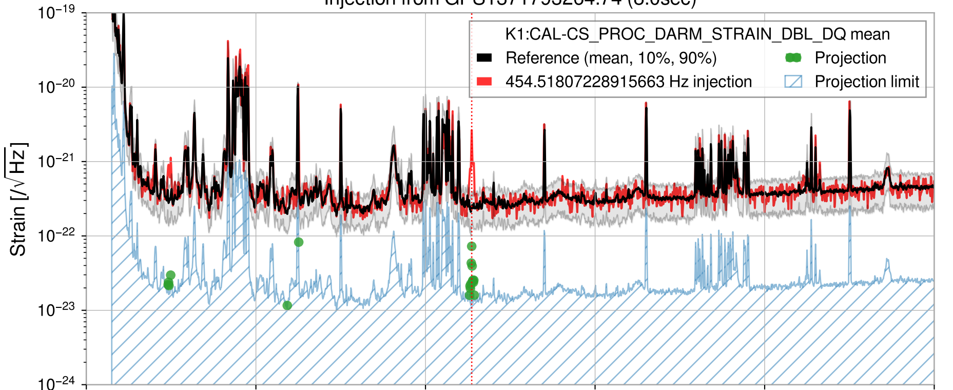
Injection from GPS1371793264.74 (8.0sec)
