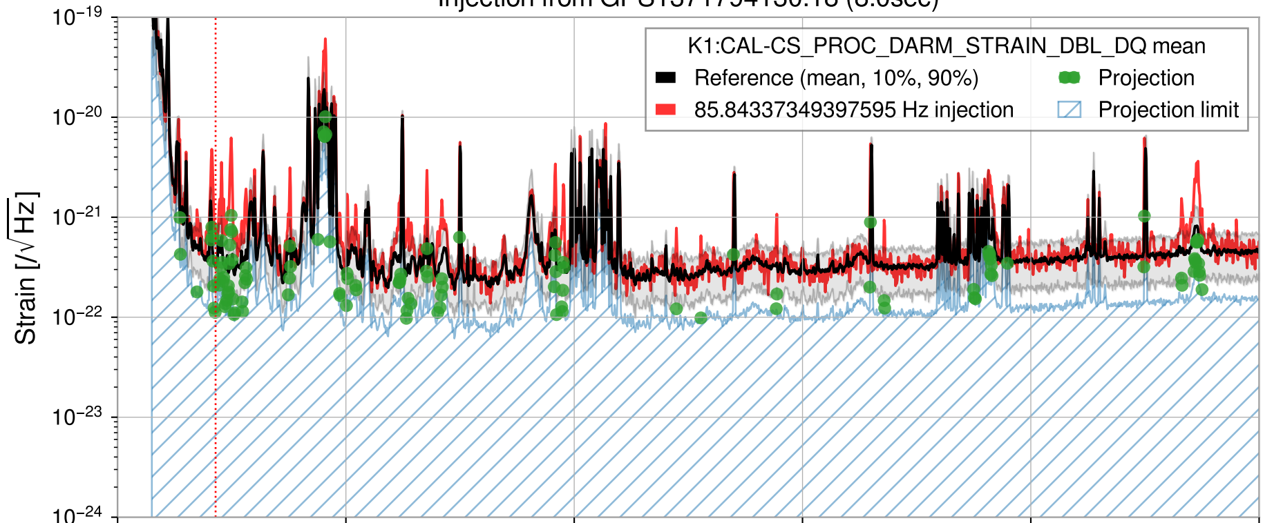
Injection from GPS1371794130.18 (8.0sec)
