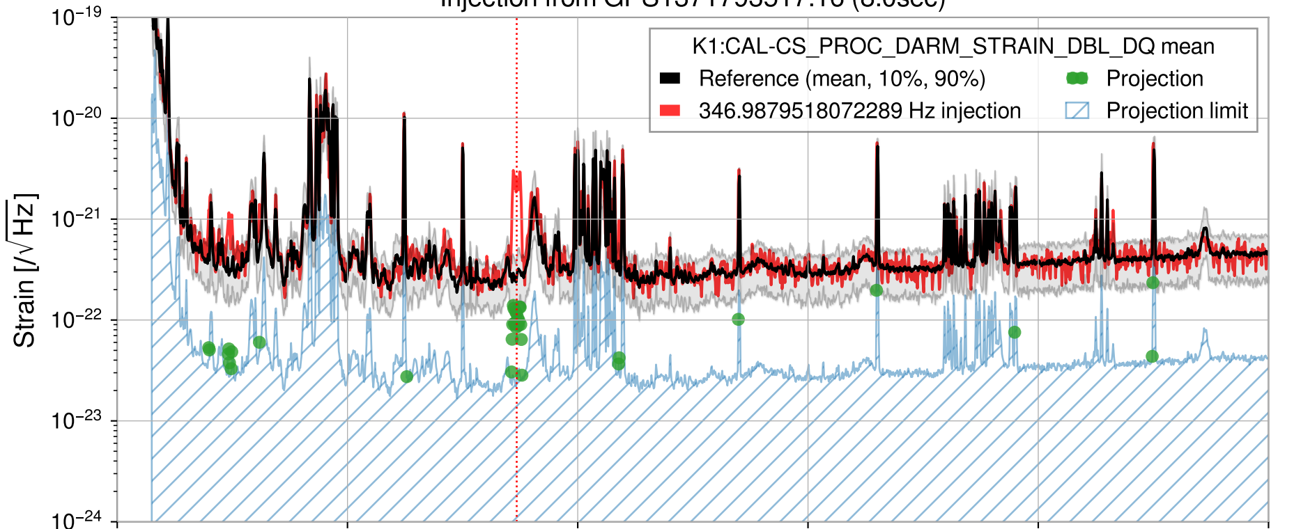
Injection from GPS1371793517.16 (8.0sec)
