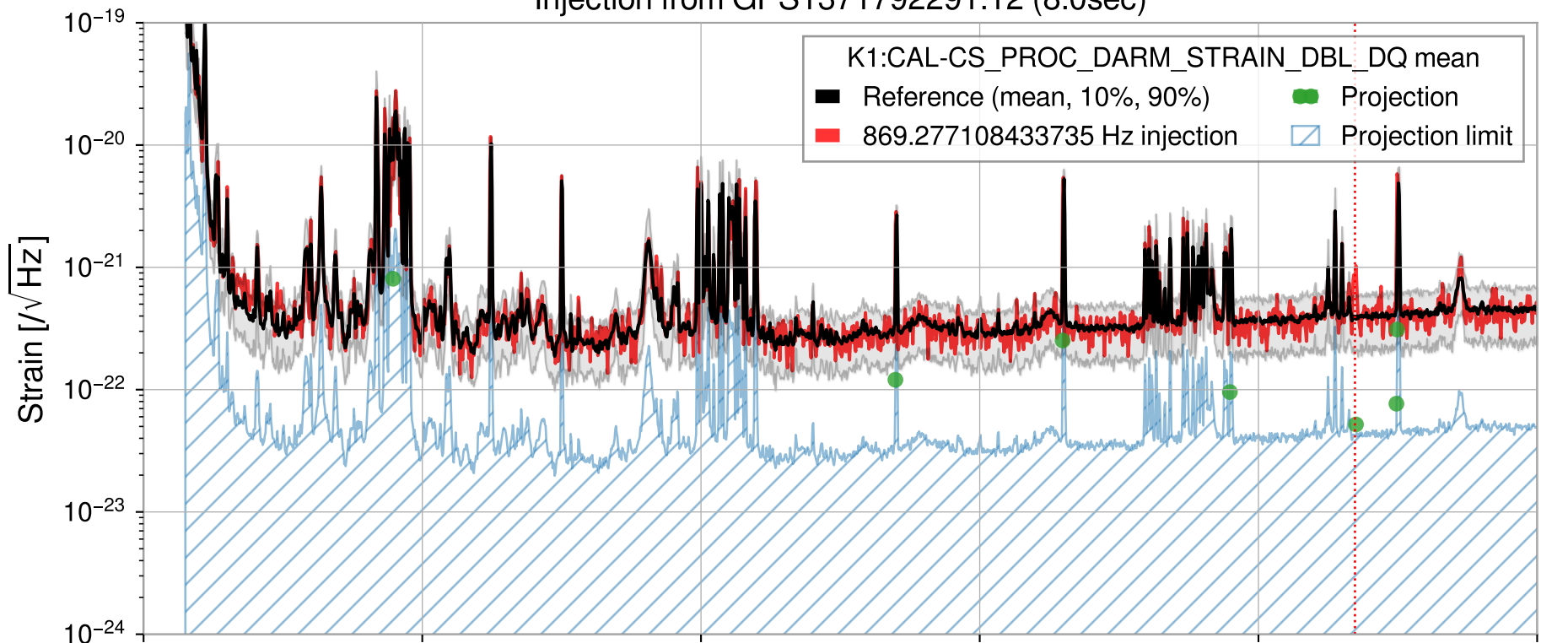
Injection from GPS1371792291.12 (8.0sec)
