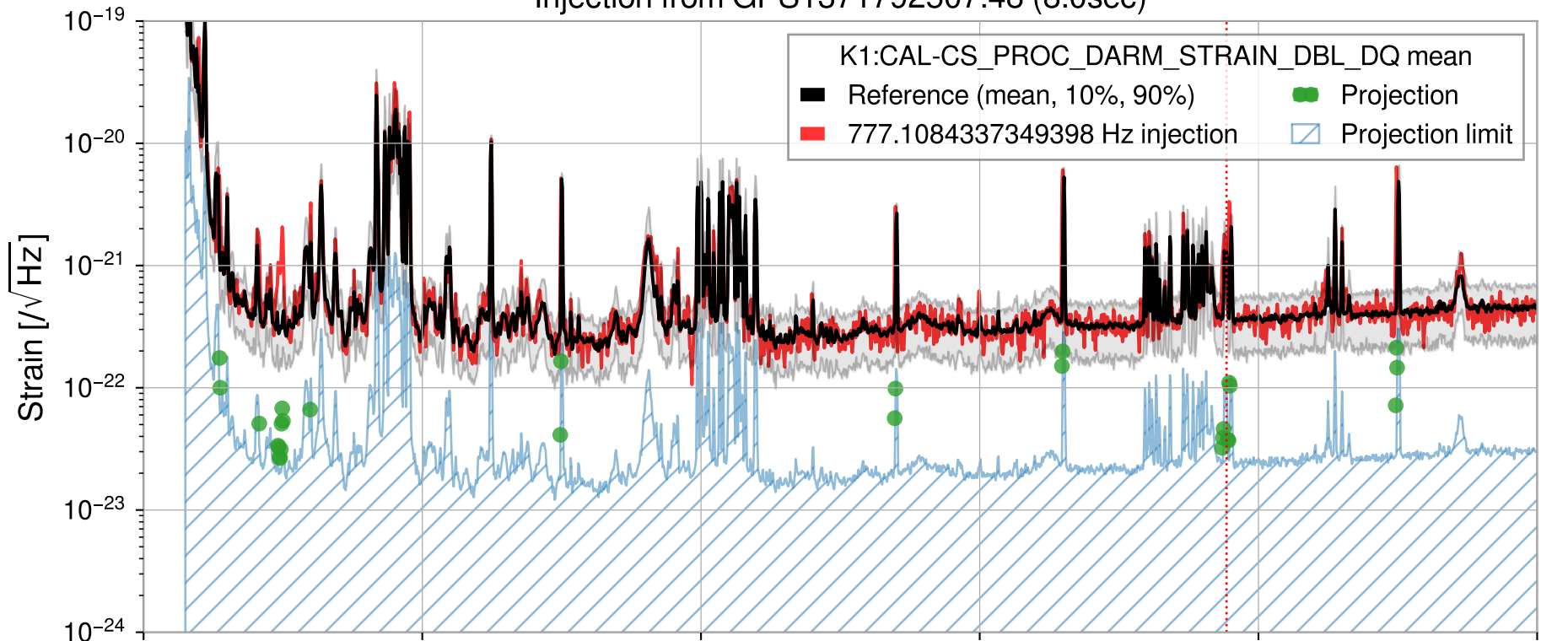
Injection from GPS1371792507.48 (8.0sec)
