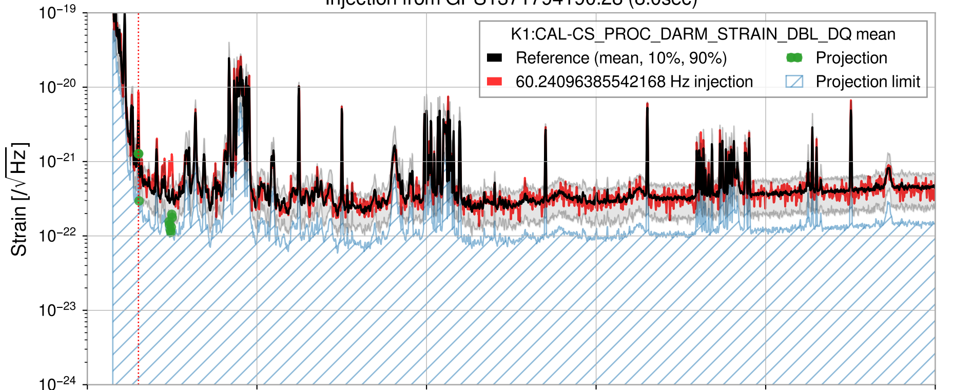
Injection from GPS1371794190.28 (8.0sec)
