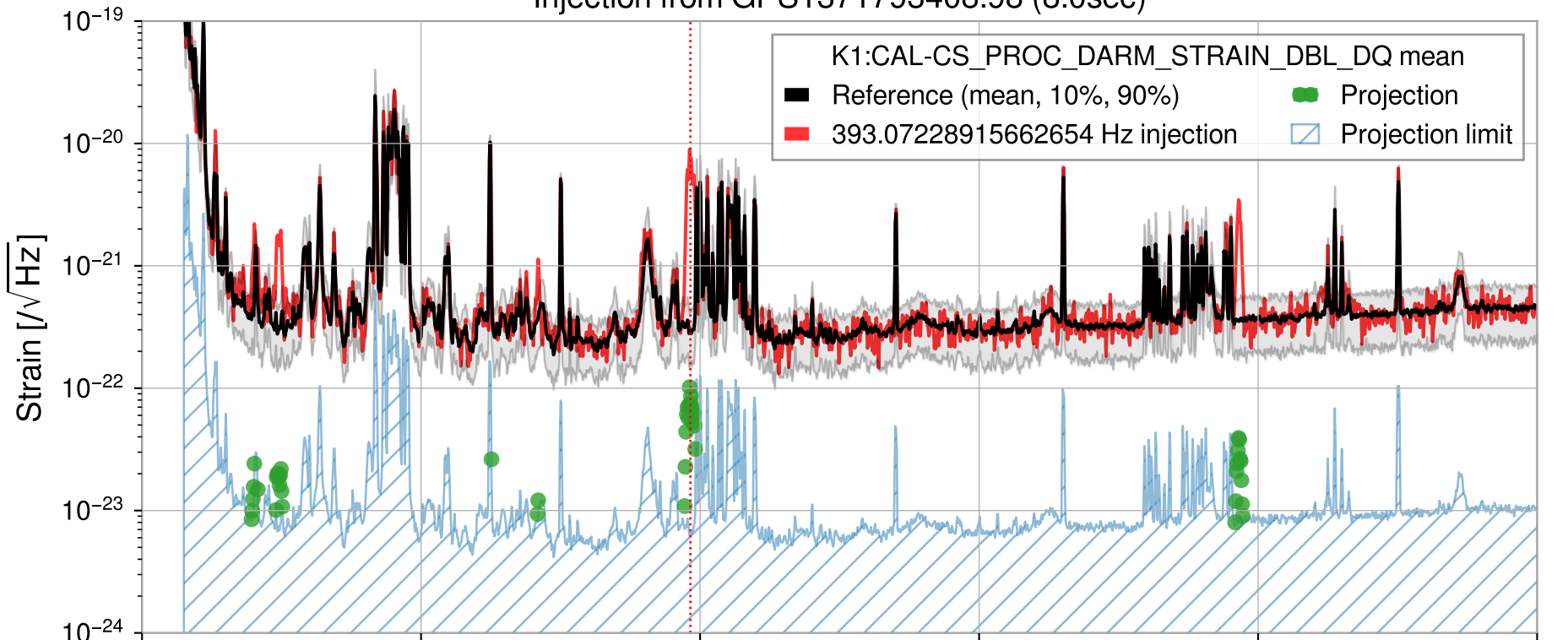
Injection from GPS1371793408.98 (8.0sec)
