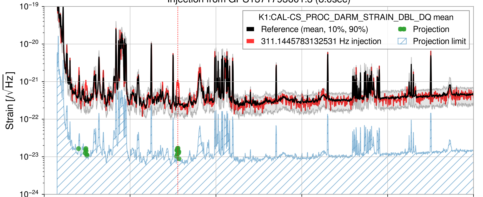
Injection from GPS1371793601.3 (8.0sec)
