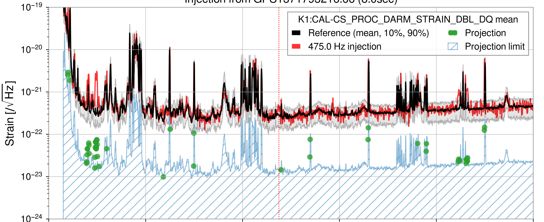
Injection from GPS1371793216.66 (8.0sec)
