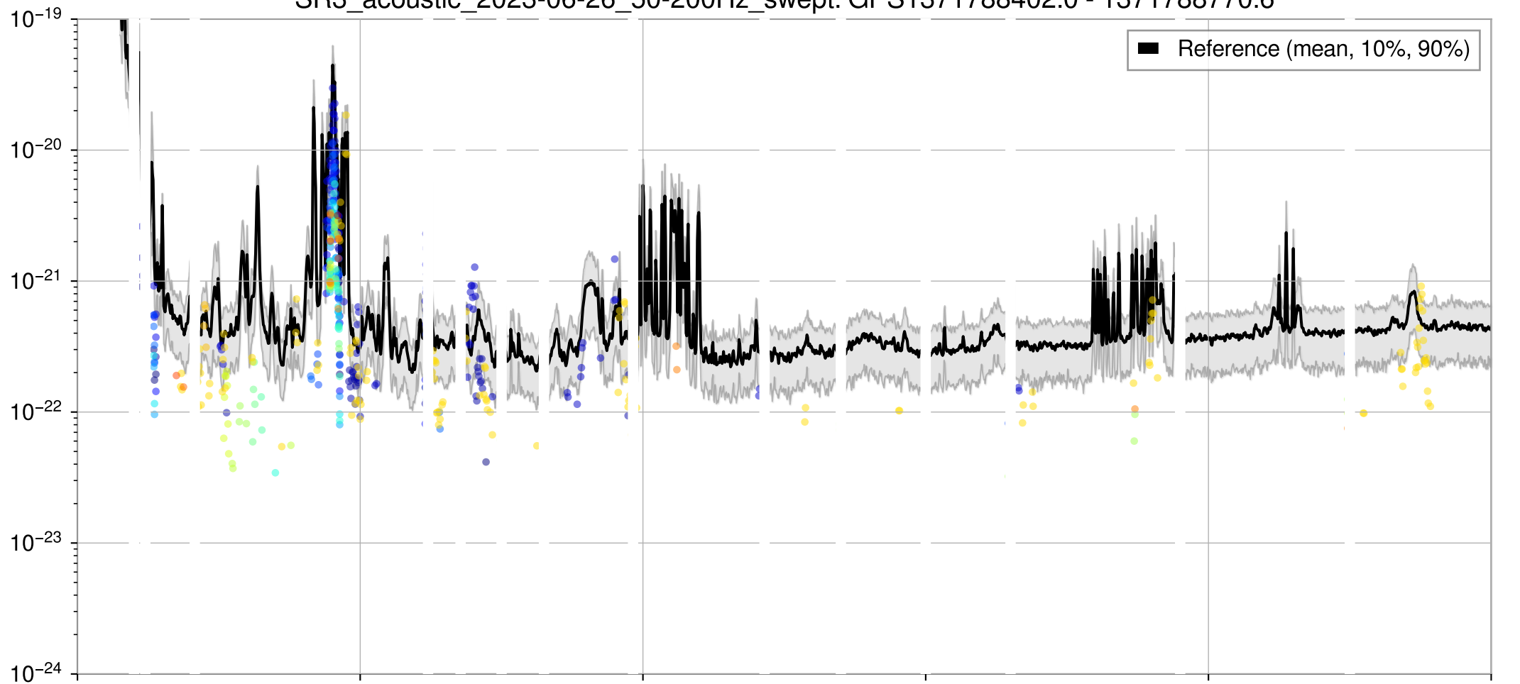
SR3_acoustic_2023-06-26_50-200Hz_swept: GPS1371788402.0 - 1371788770.6
