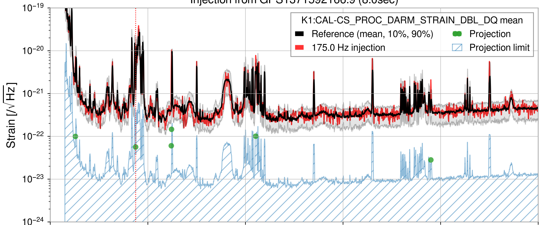
Injection from GPS1371592166.9 (8.0sec)
