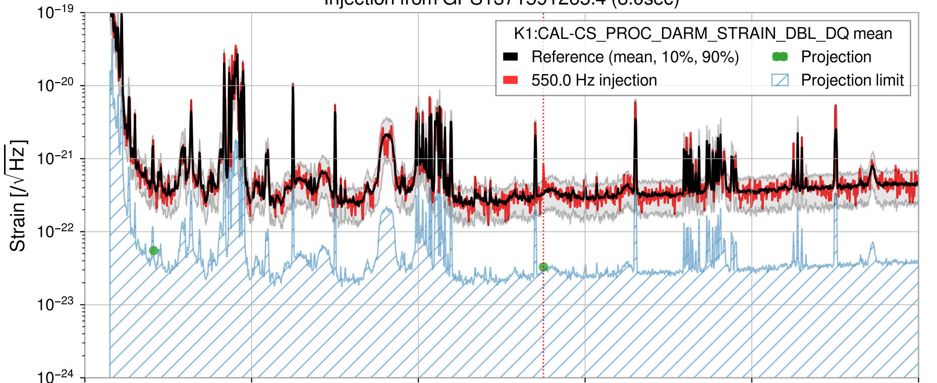
Injection from GPS1371591265.4 (8.0sec)
