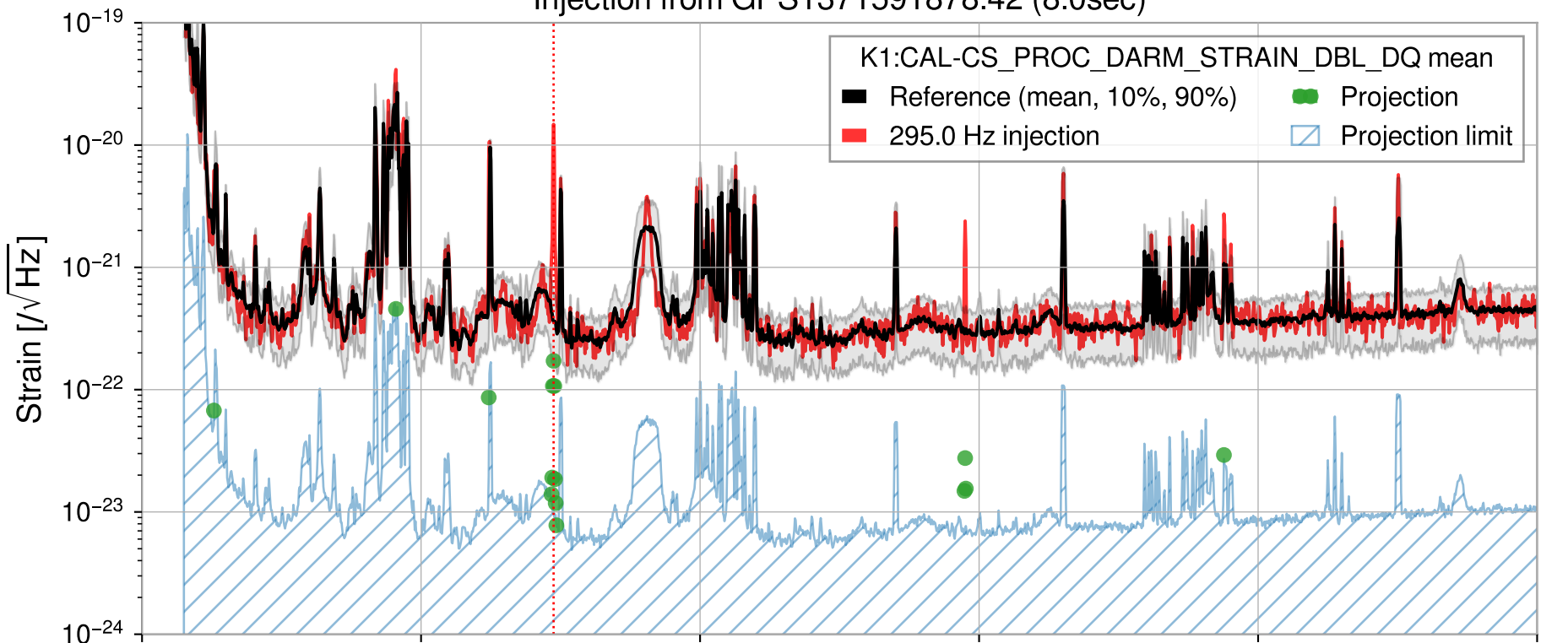
Injection from GPS1371591878.42 (8.0sec)
