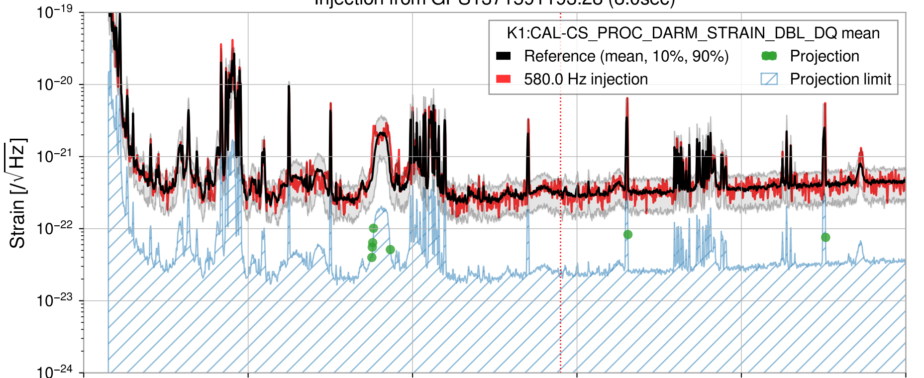
Injection from GPS1371591193.28 (8.0sec)
