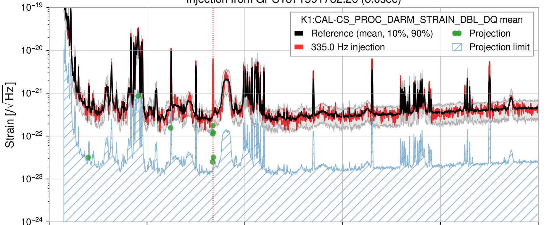
Injection from GPS1371591782.26 (8.0sec)
