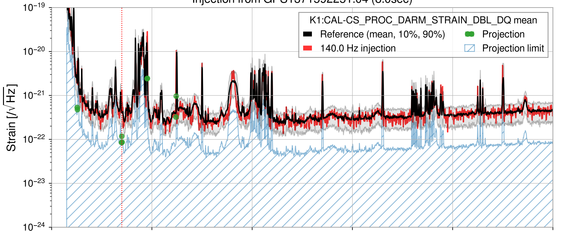
Injection from GPS1371592251.04 (8.0sec)
