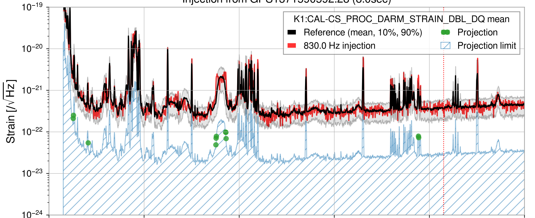
Injection from GPS1371590592.28 (8.0sec)
