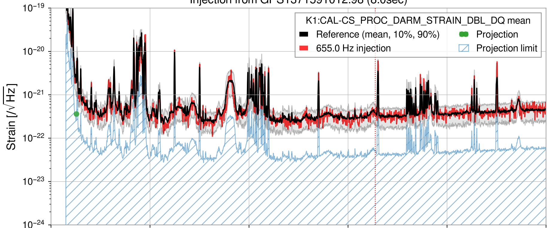
Injection from GPS1371591012.98 (8.0sec)
