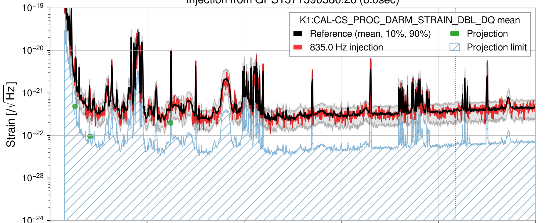
Injection from GPS1371590580.26 (8.0sec)
