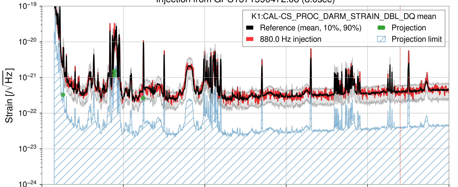
Injection from GPS1371590472.08 (8.0sec)
