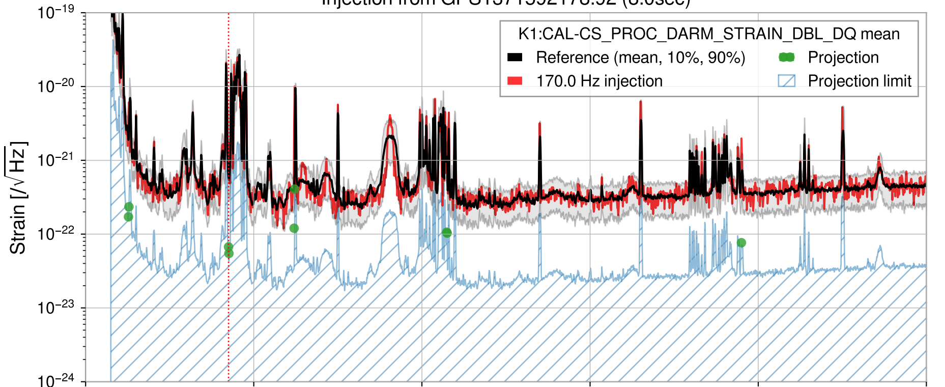
Injection from GPS1371592178.92 (8.0sec)
