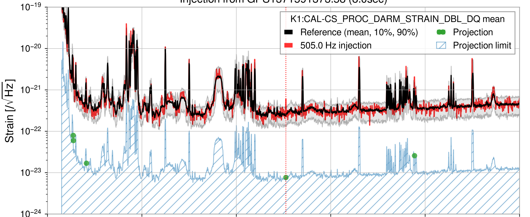
Injection from GPS1371591373.58 (8.0sec)
