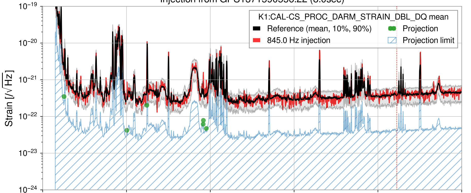
Injection from GPS1371590556.22 (8.0sec)
