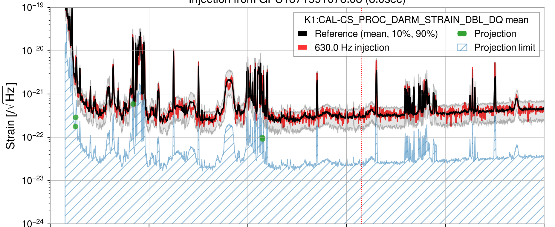
Injection from GPS1371591073.08 (8.0sec)
