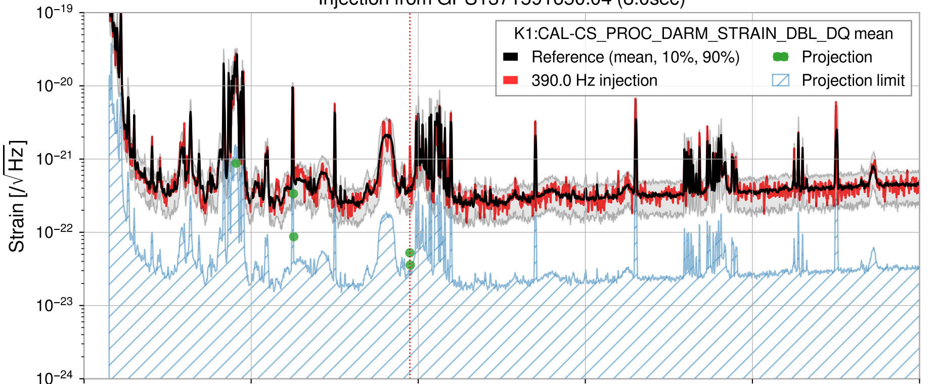
Injection from GPS1371591650.04 (8.0sec)
