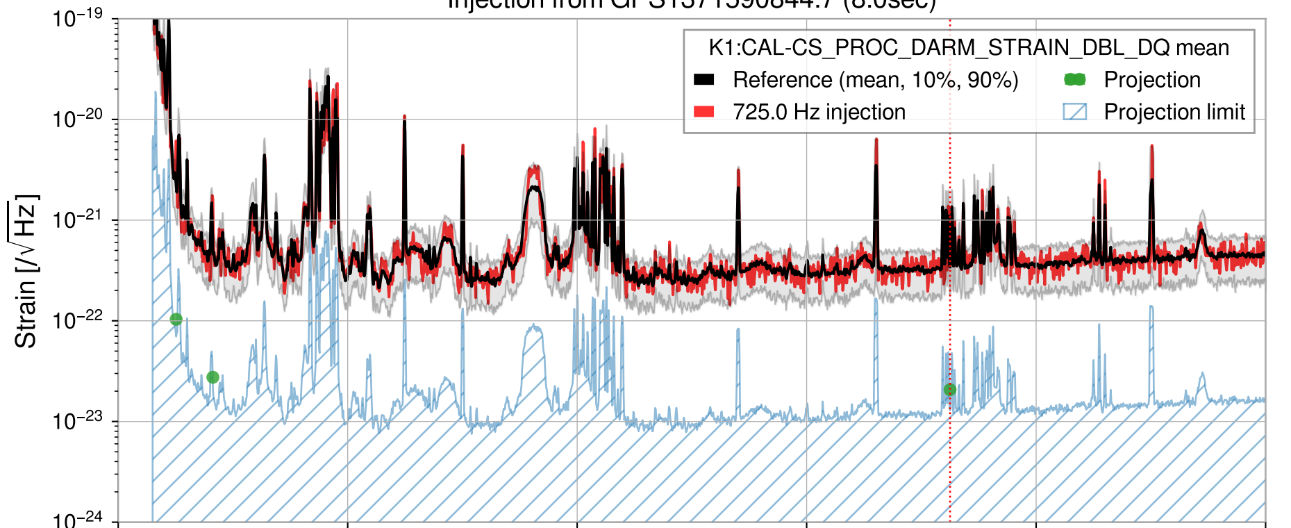
Injection from GPS1371590844.7 (8.0sec)
