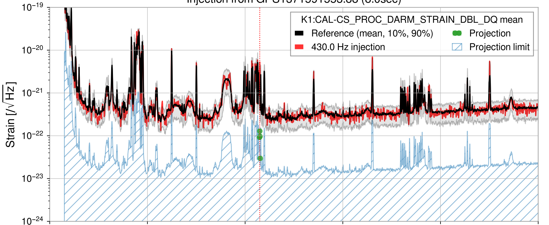
Injection from GPS1371591553.88 (8.0sec)
