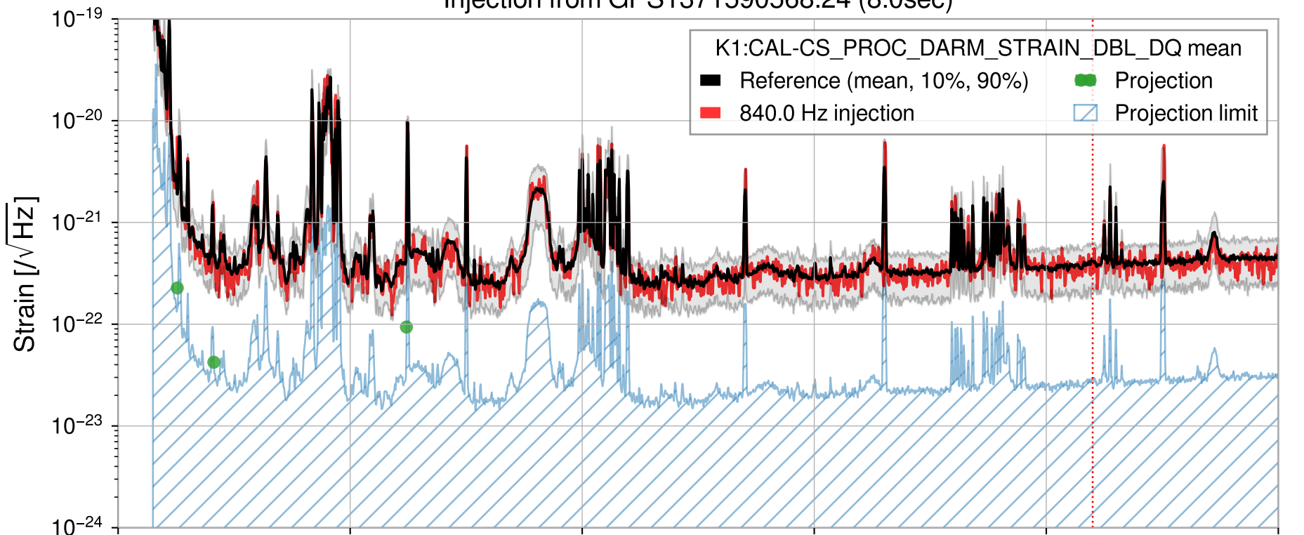
Injection from GPS1371590568.24 (8.0sec)
