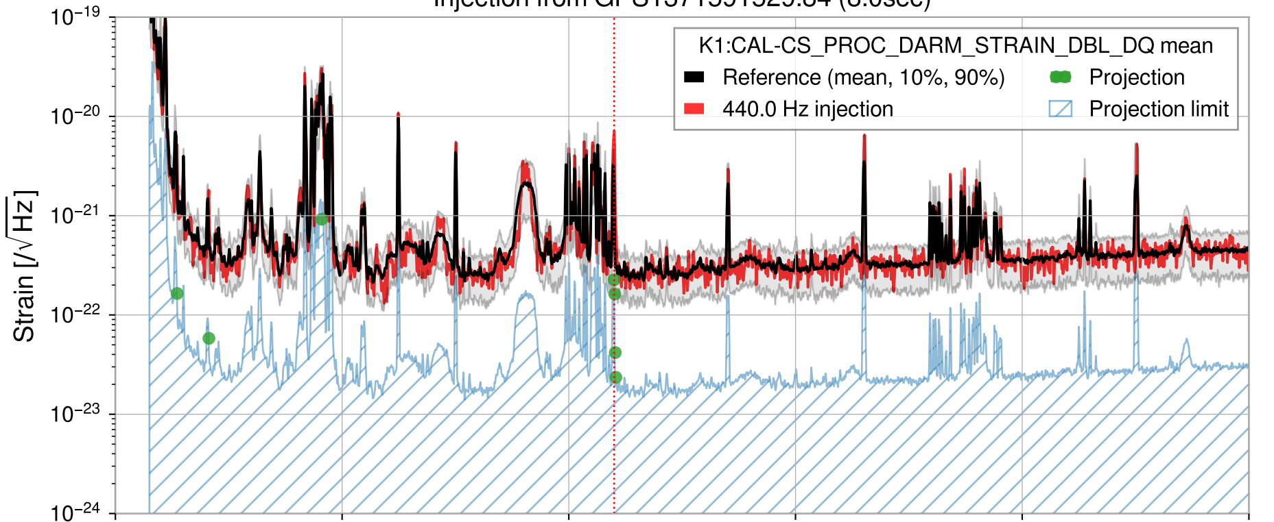
Injection from GPS1371591529.84 (8.0sec)
