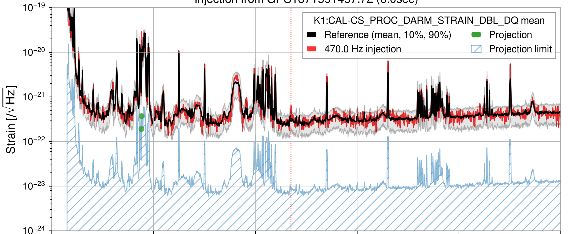
Injection from GPS1371591457.72 (8.0sec)
