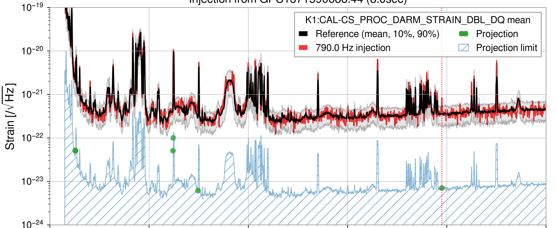
Injection from GPS1371590688.44 (8.0sec)
