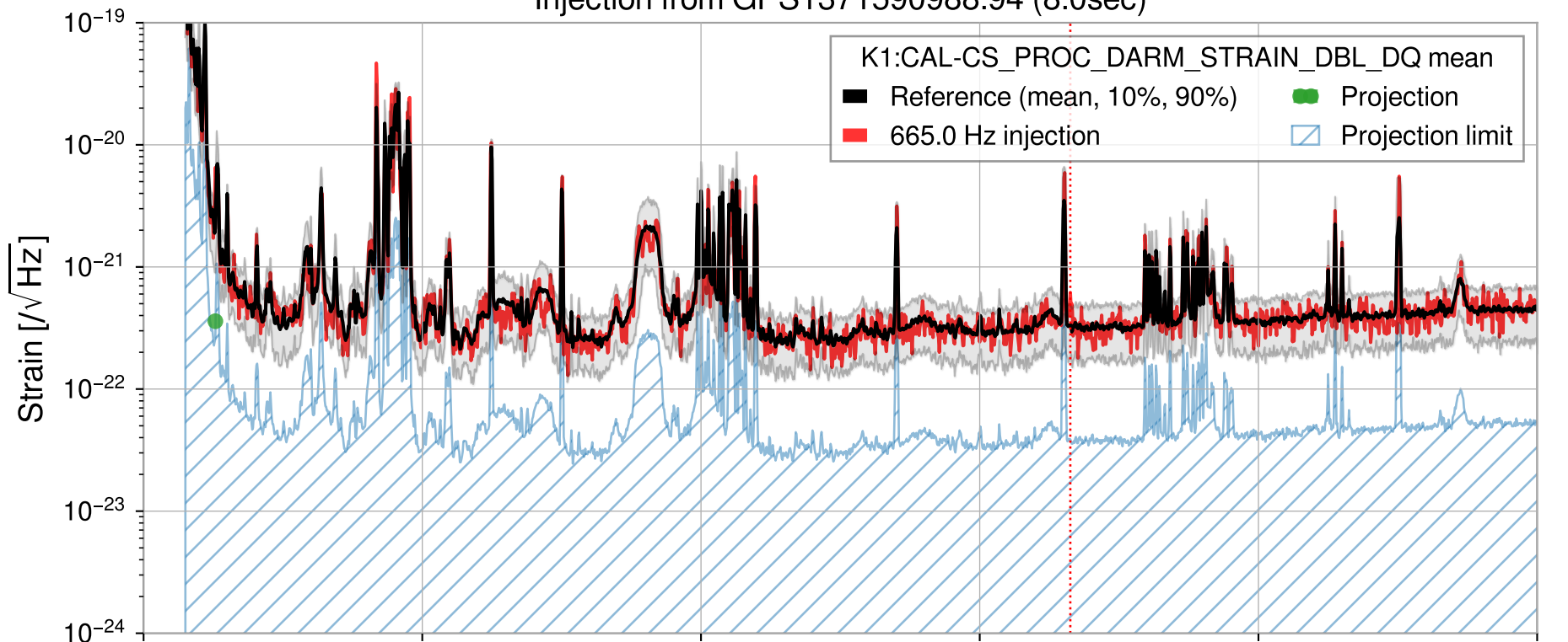
Injection from GPS1371590988.94 (8.0sec)
