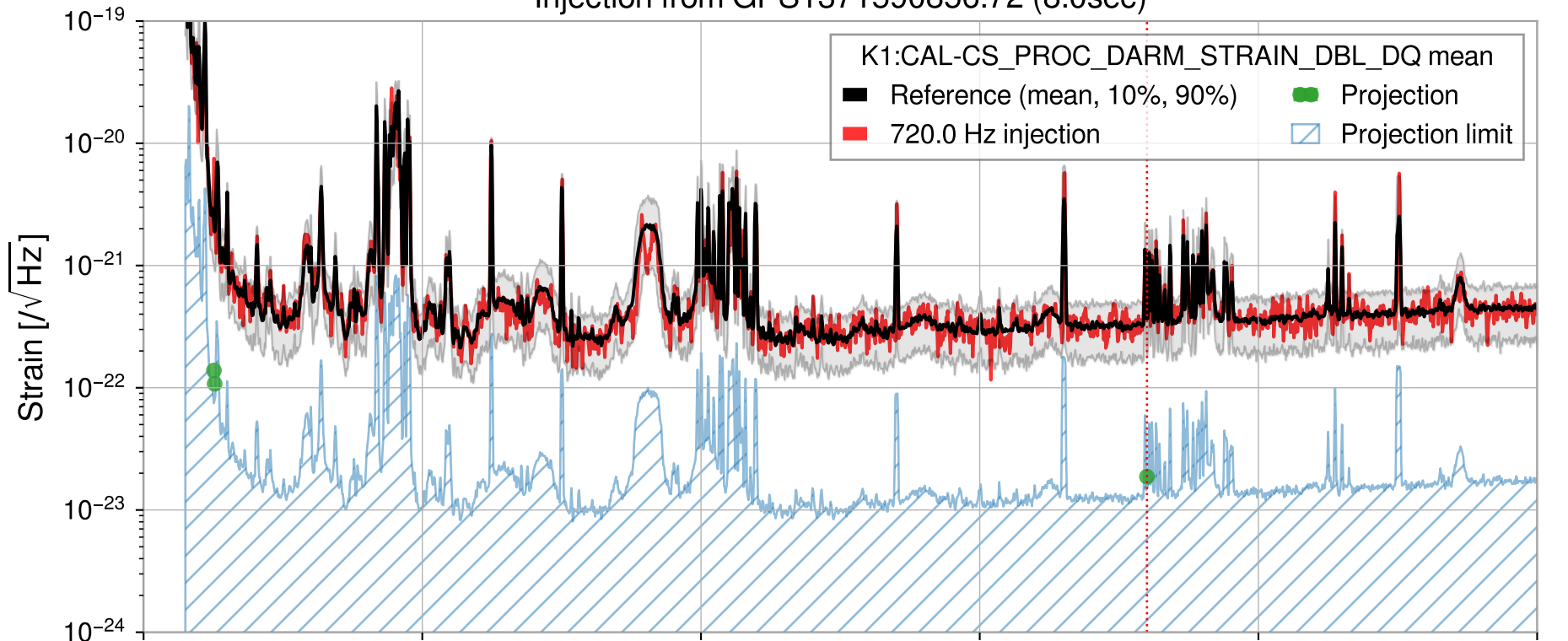
Injection from GPS1371590856.72 (8.0sec)
