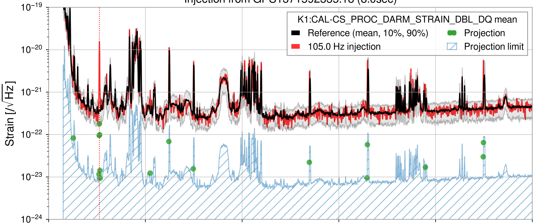
Injection from GPS1371592335.18 (8.0sec)
