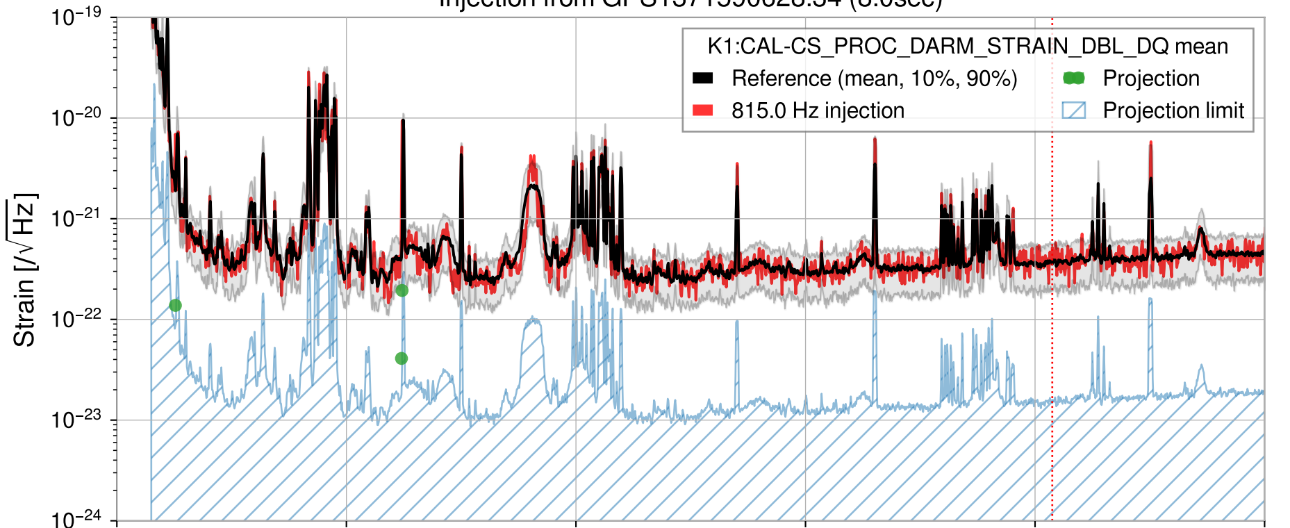
Injection from GPS1371590628.34 (8.0sec)
