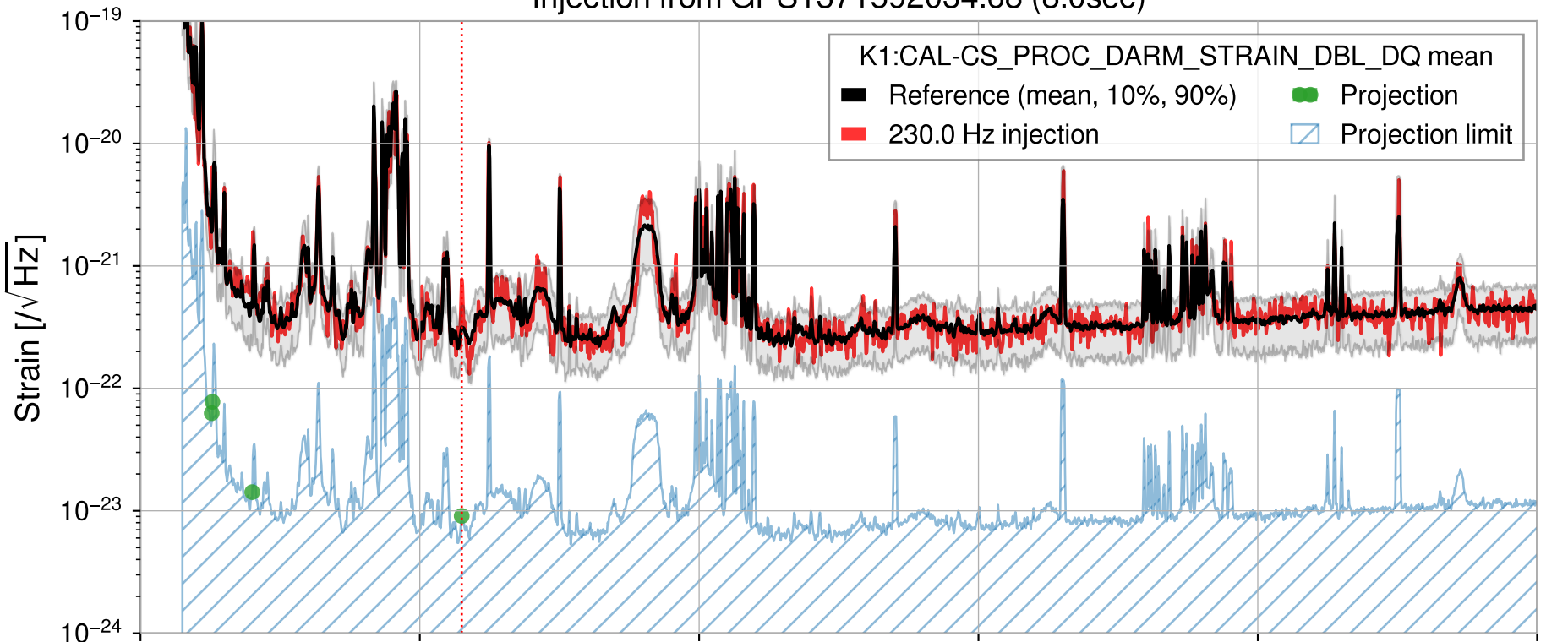
Injection from GPS1371592034.68 (8.0sec)
