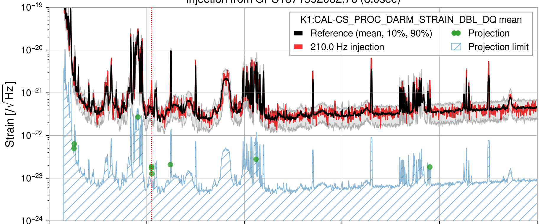
Injection from GPS1371592082.76 (8.0sec)
