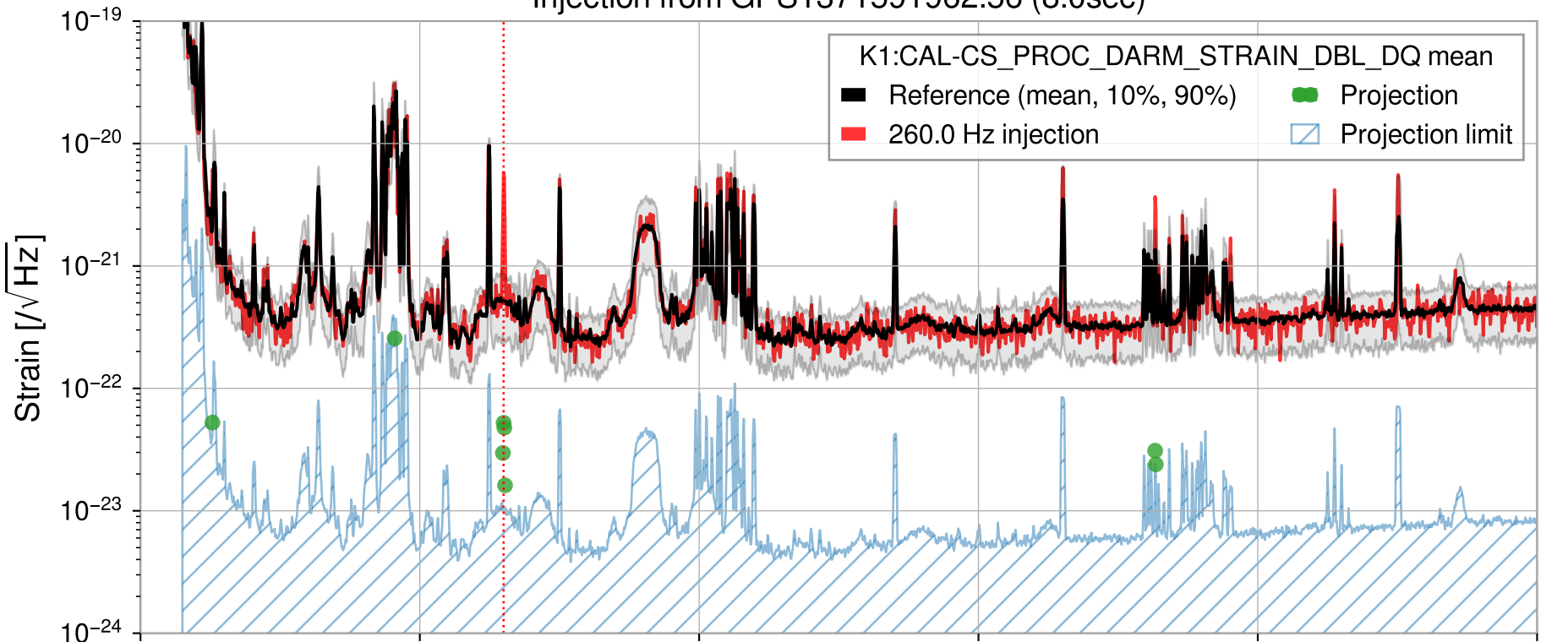
Injection from GPS1371591962.56 (8.0sec)
