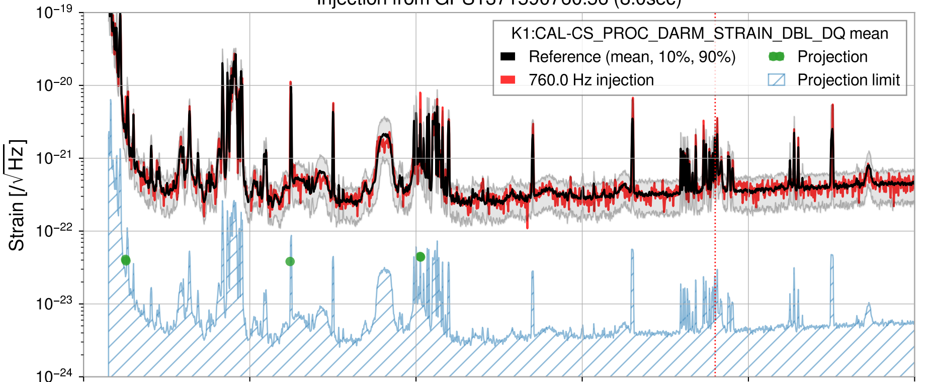
Injection from GPS1371590760.56 (8.0sec)
