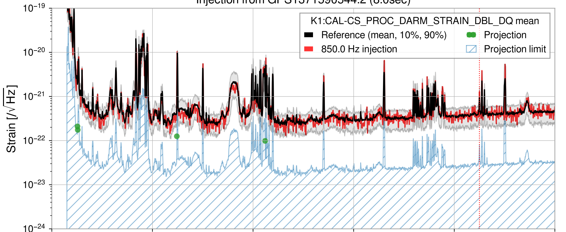
Injection from GPS1371590544.2 (8.0sec)
