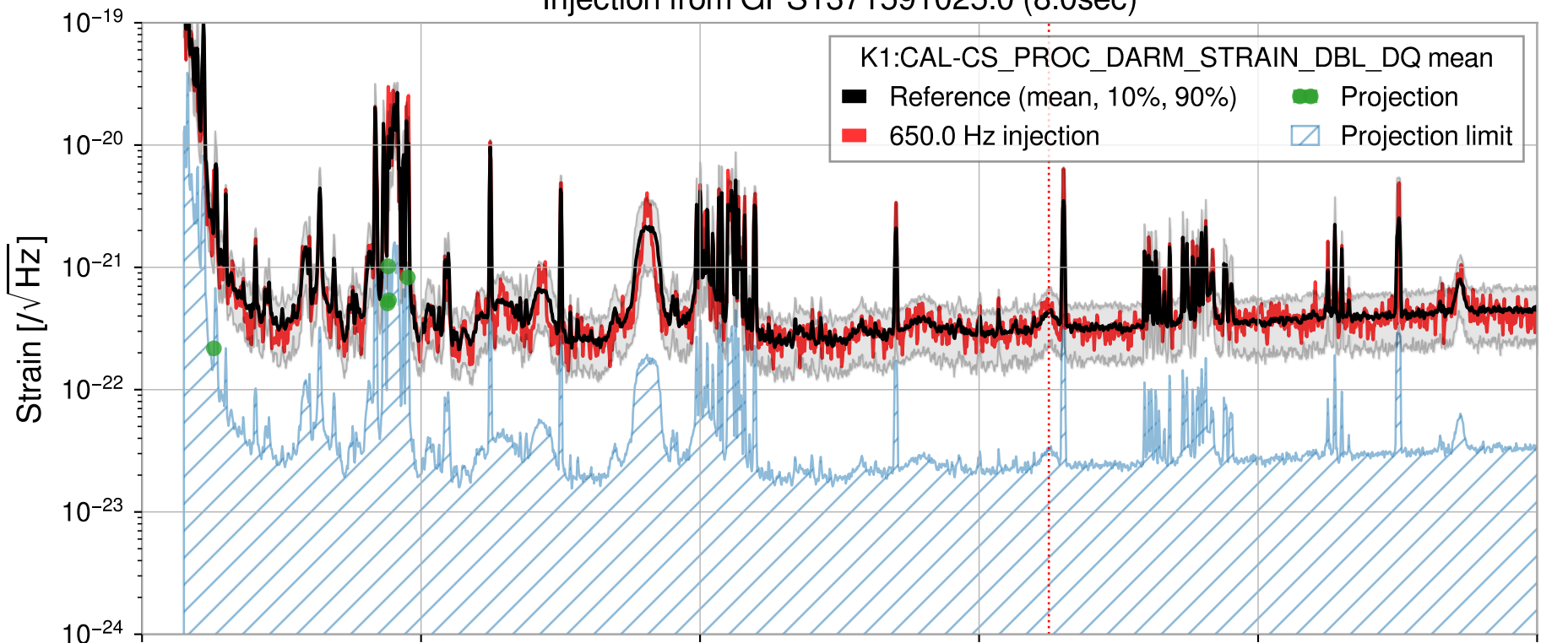
Injection from GPS1371591025.0 (8.0sec)
