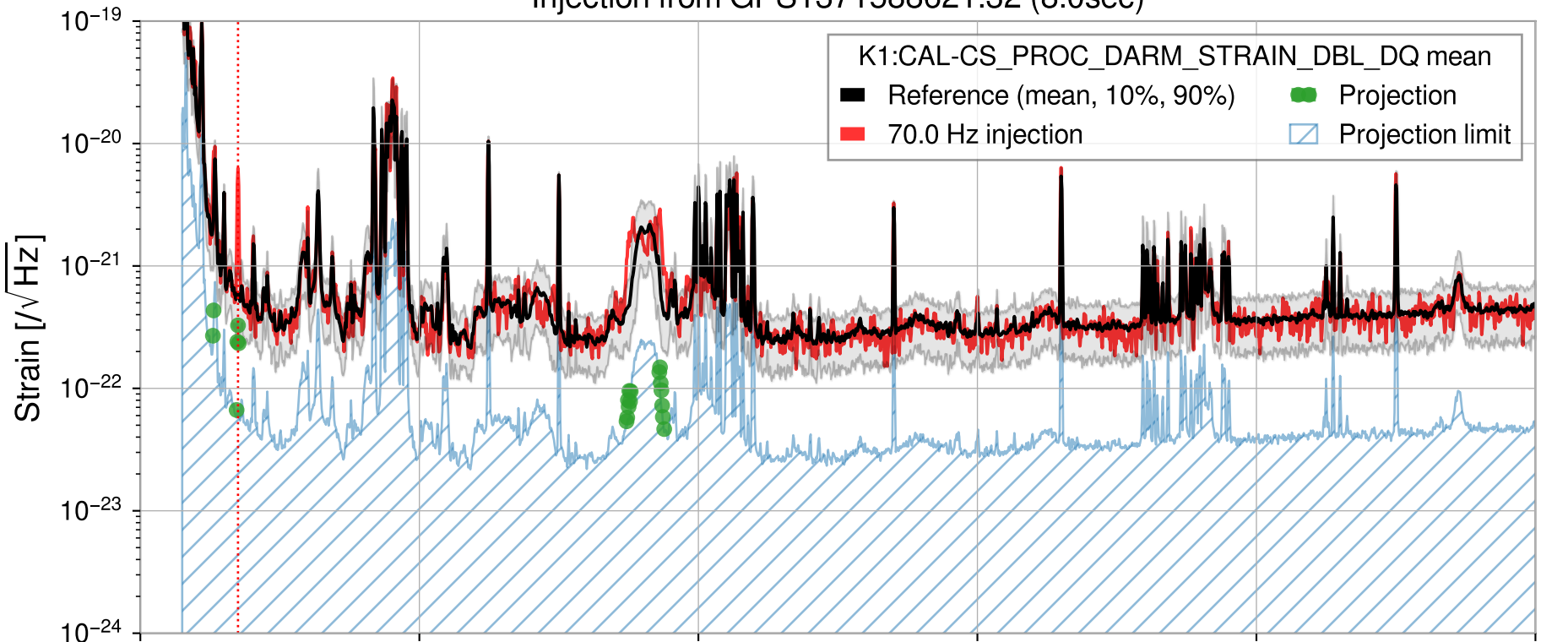
Injection from GPS1371588621.32 (8.0sec)
