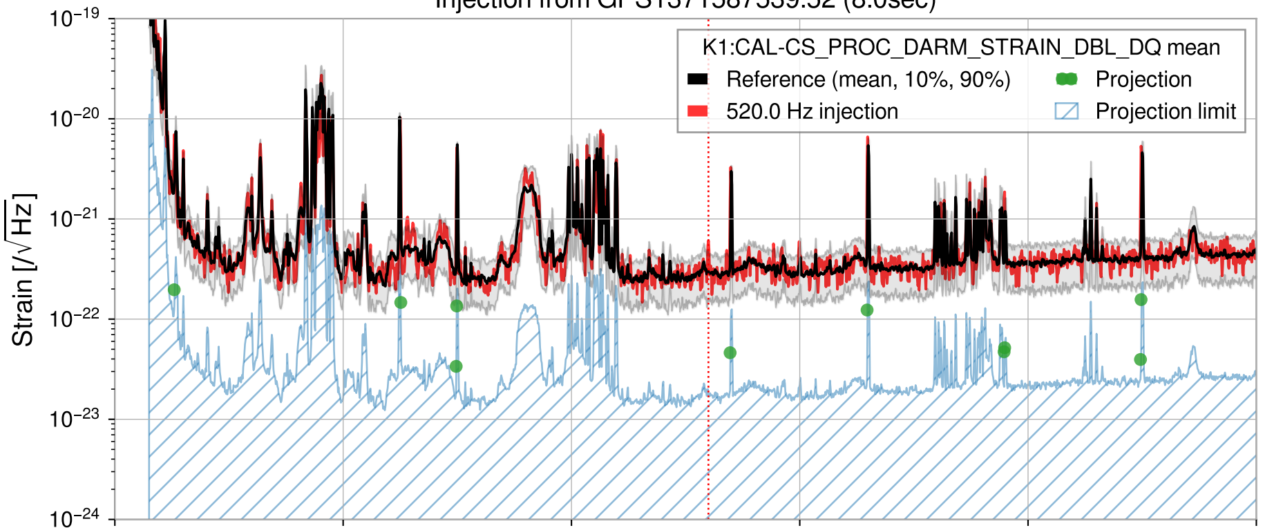
Injection from GPS1371587539.52 (8.0sec)
