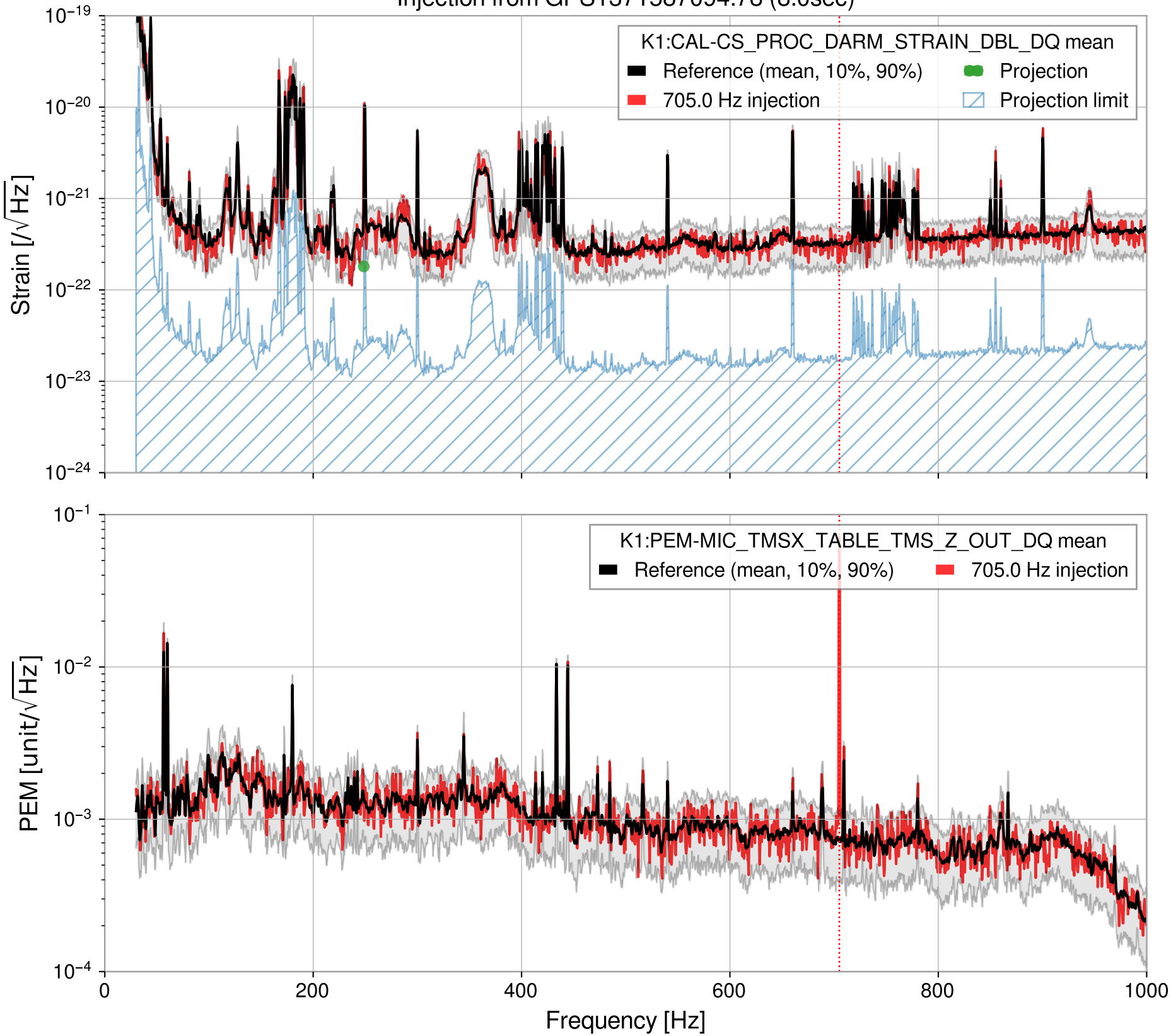
Injection from GPS1371587094.78 (8.0sec)
