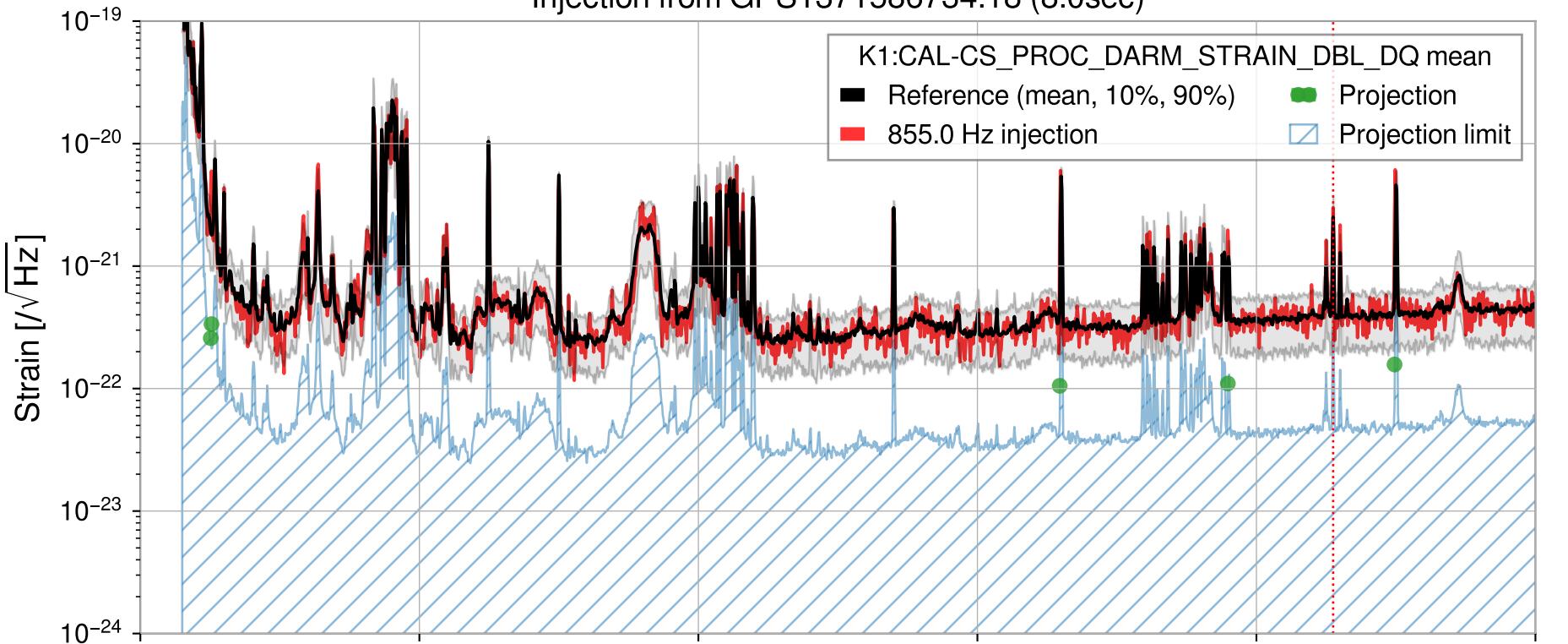
Injection from GPS1371586734.18 (8.0sec)
