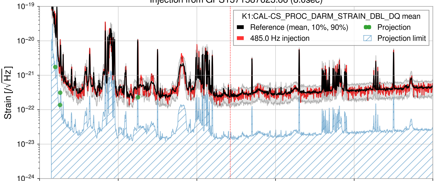
Injection from GPS1371587623.66 (8.0sec)
