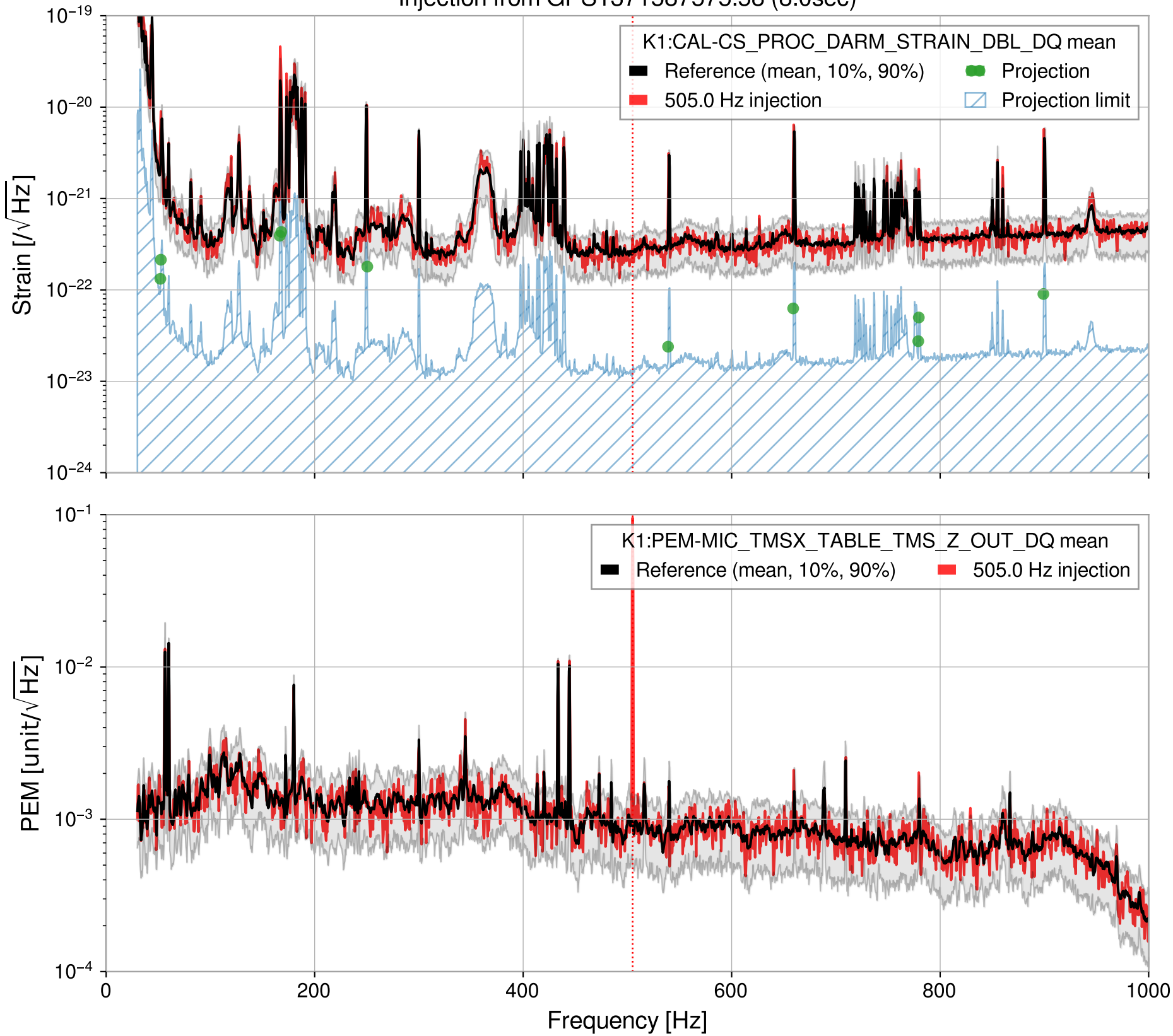
Injection from GPS1371587575.58 (8.0sec)
