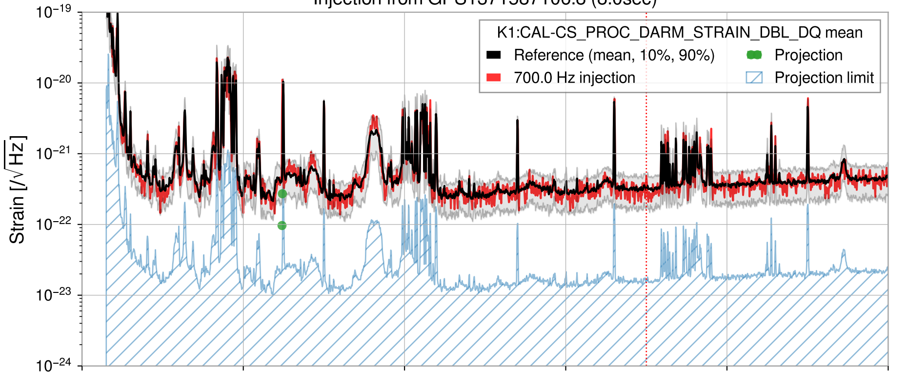
Injection from GPS1371587106.8 (8.0sec)
