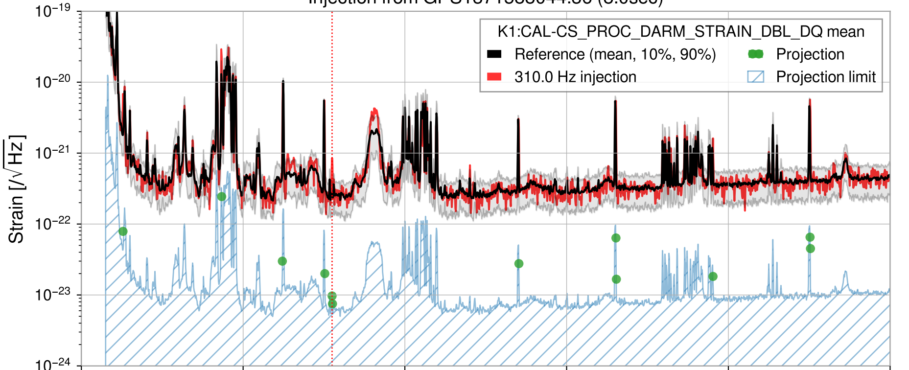
Injection from GPS1371588044.36 (8.0sec)
