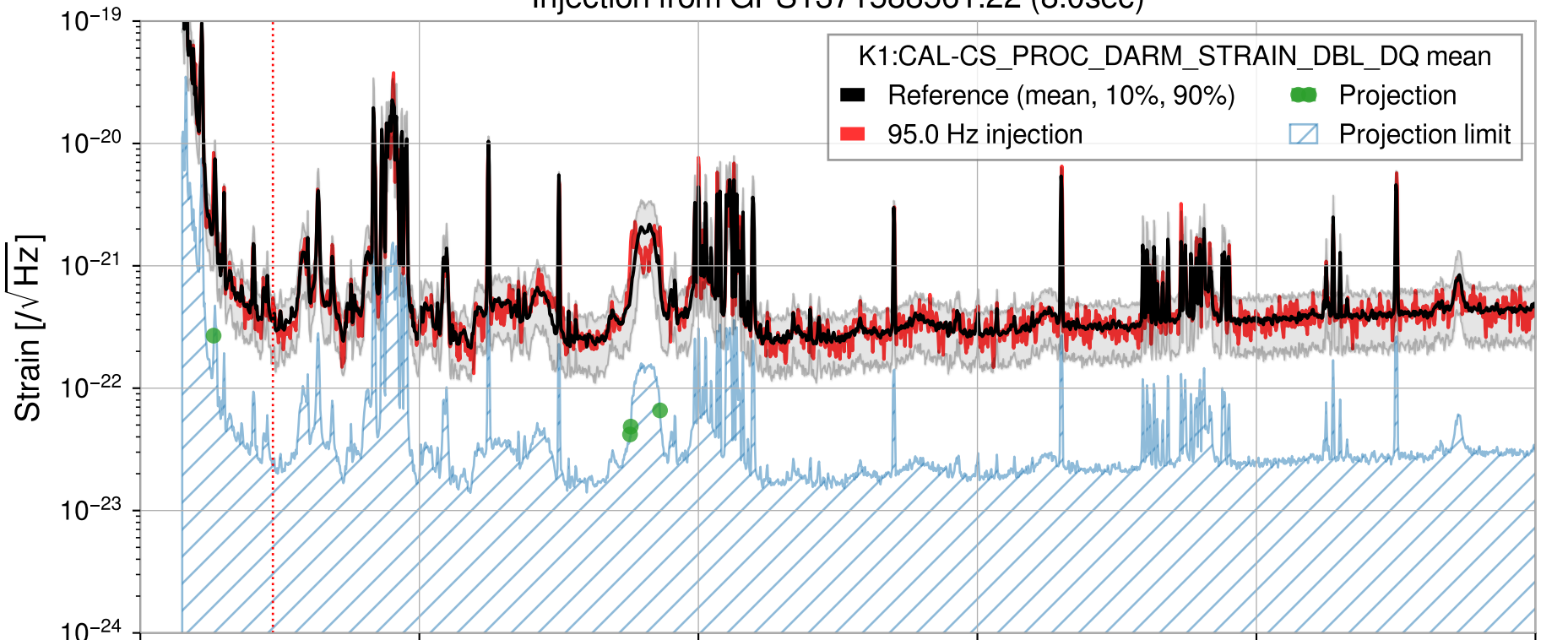
Injection from GPS1371588561.22 (8.0sec)
