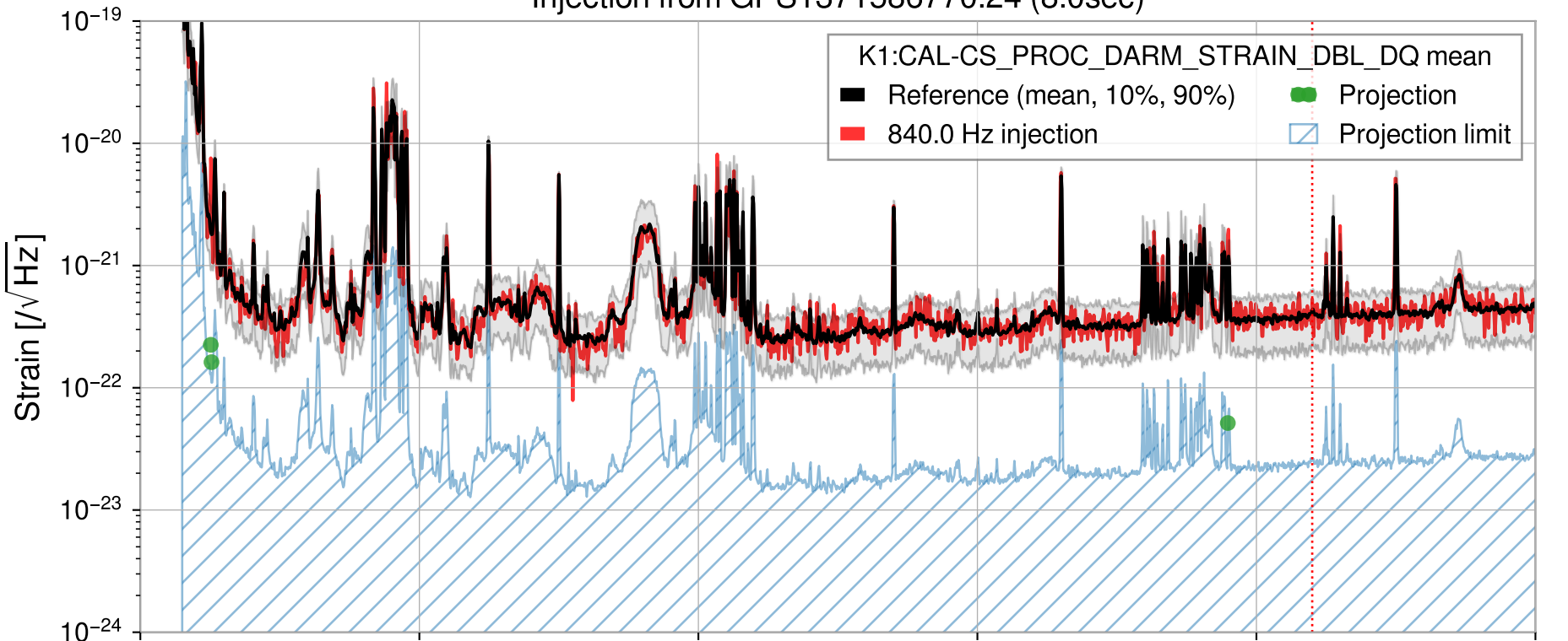
Injection from GPS1371586770.24 (8.0sec)
