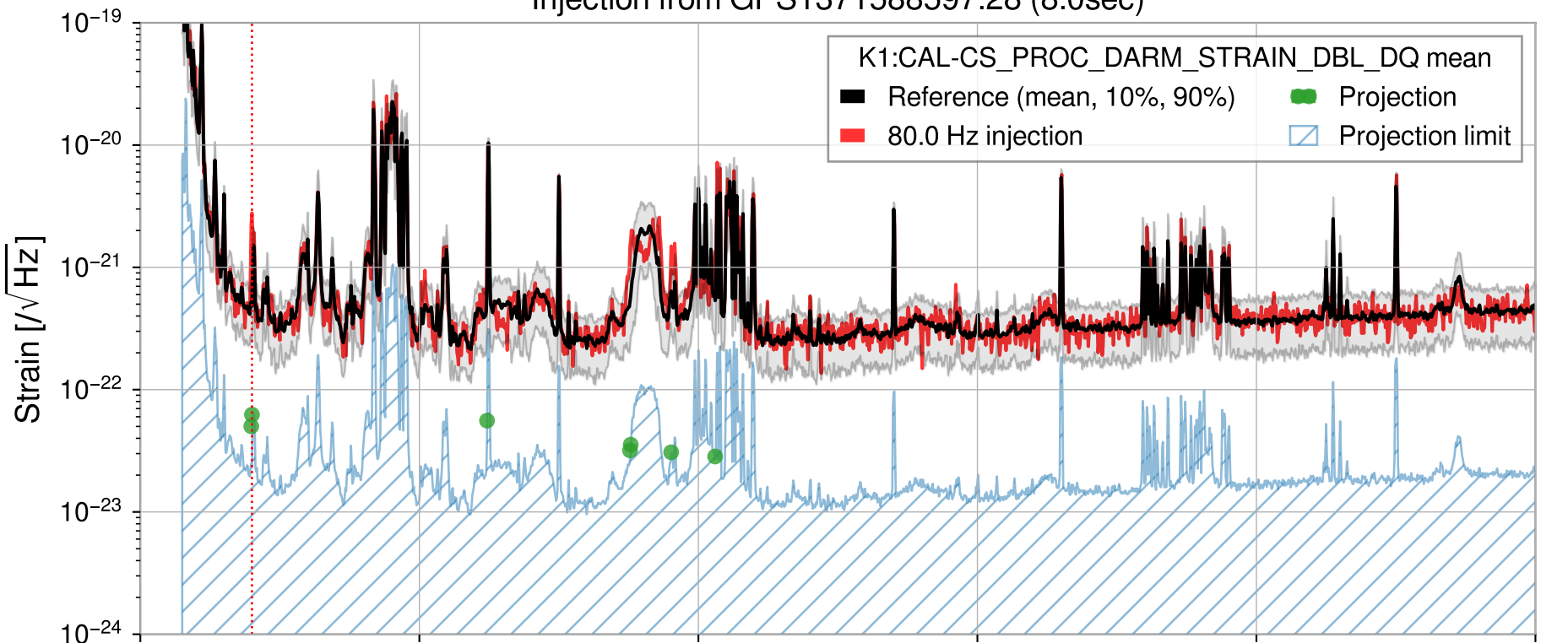
Injection from GPS1371588597.28 (8.0sec)
