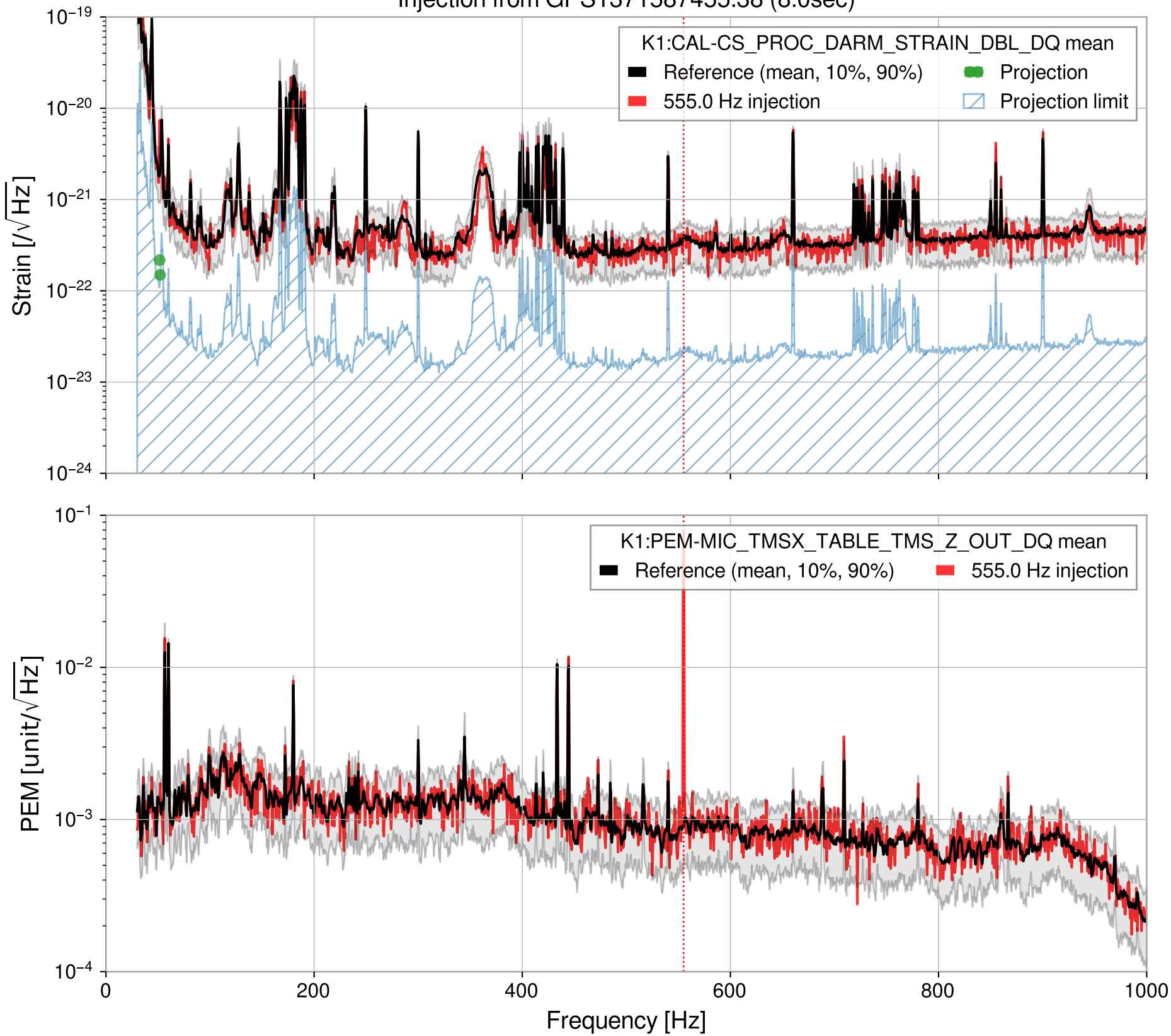
Injection from GPS1371587455.38 (8.0sec)
