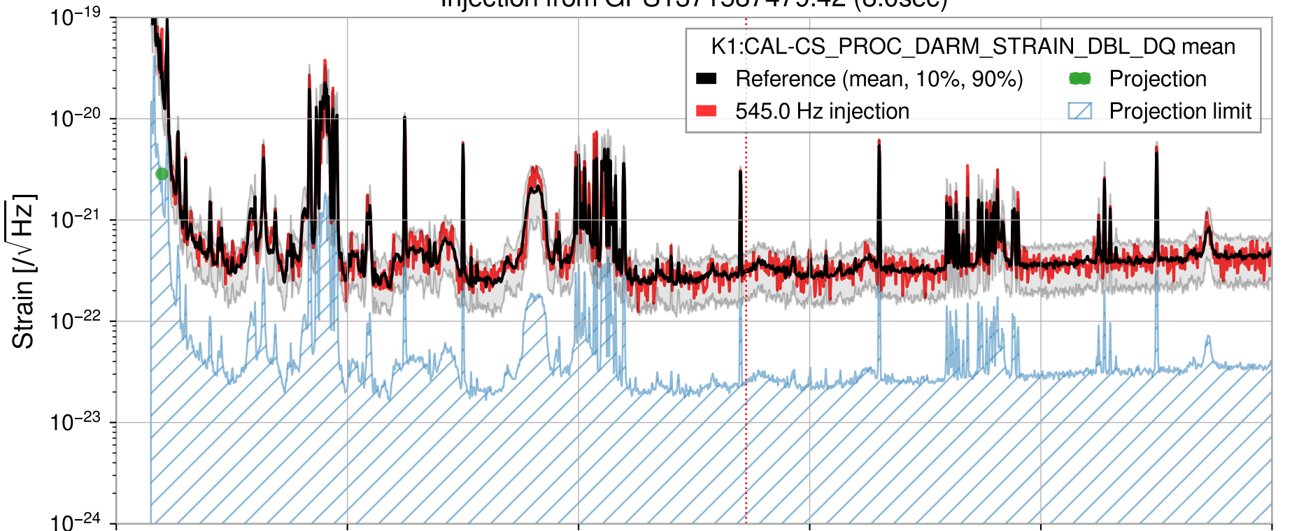
Injection from GPS1371587479.42 (8.0sec)
