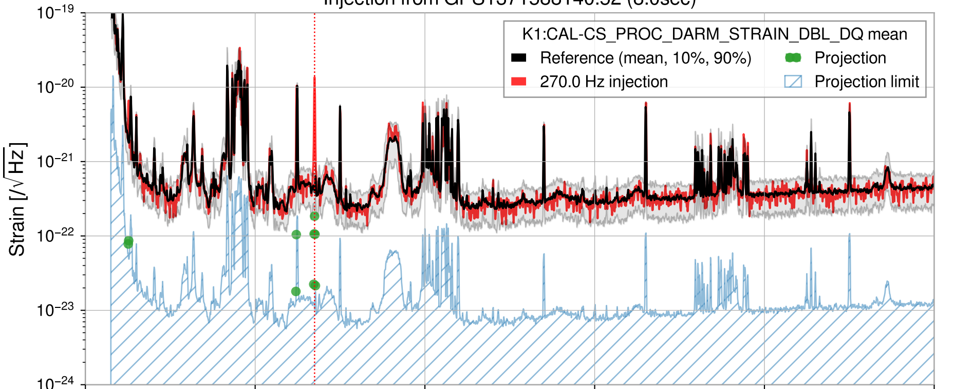
Injection from GPS1371588140.52 (8.0sec)
