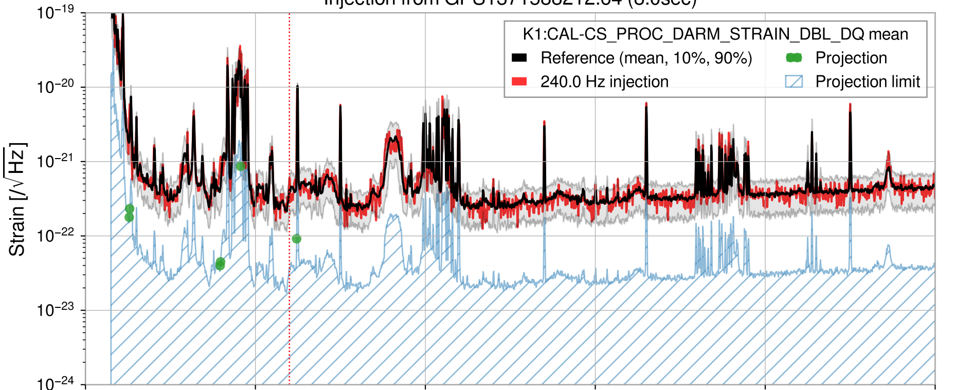
Injection from GPS1371588212.64 (8.0sec)
