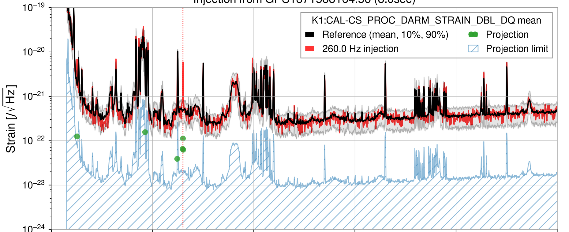
Injection from GPS1371588164.56 (8.0sec)
