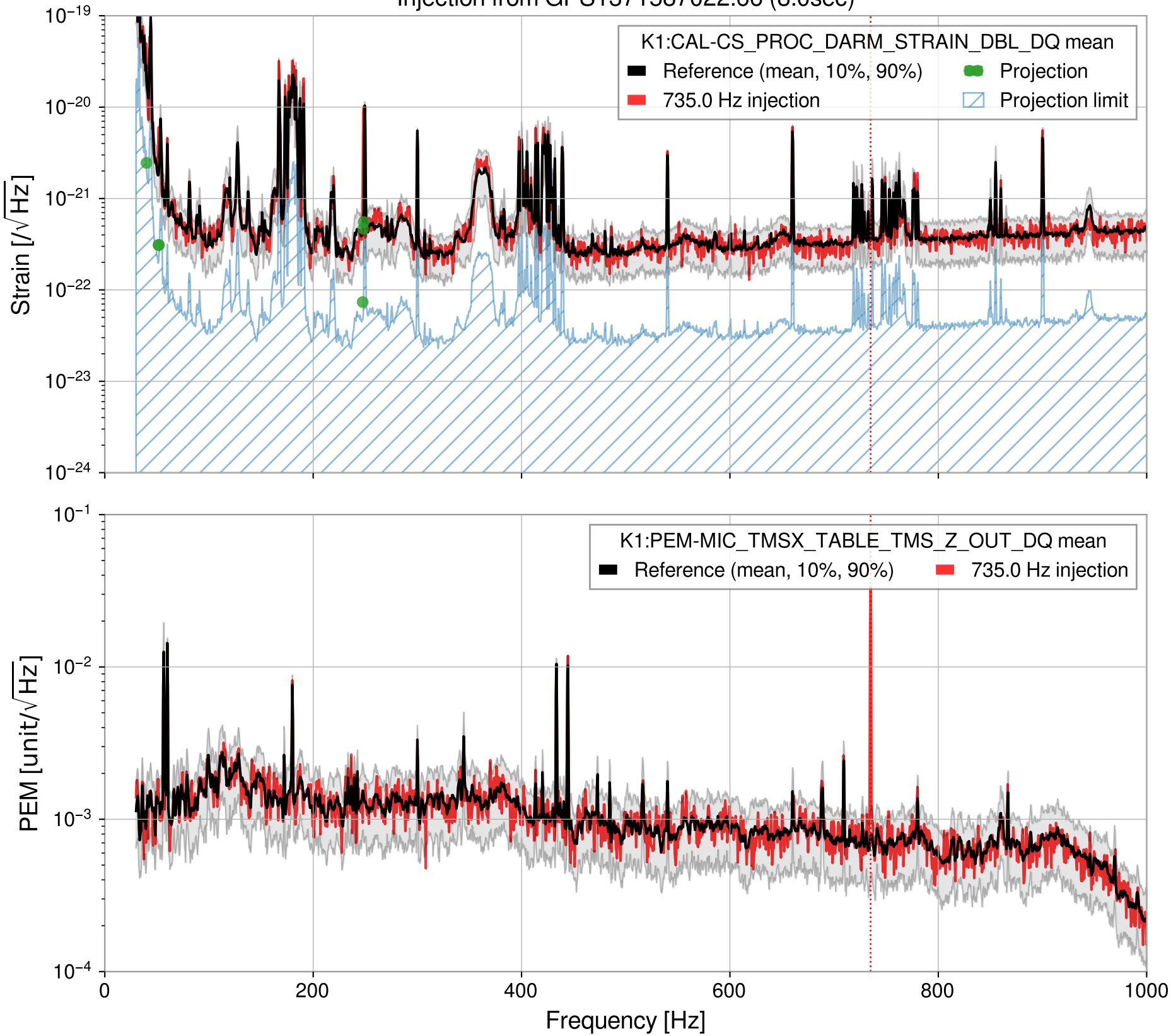
Injection from GPS1371587022.66 (8.0sec)
