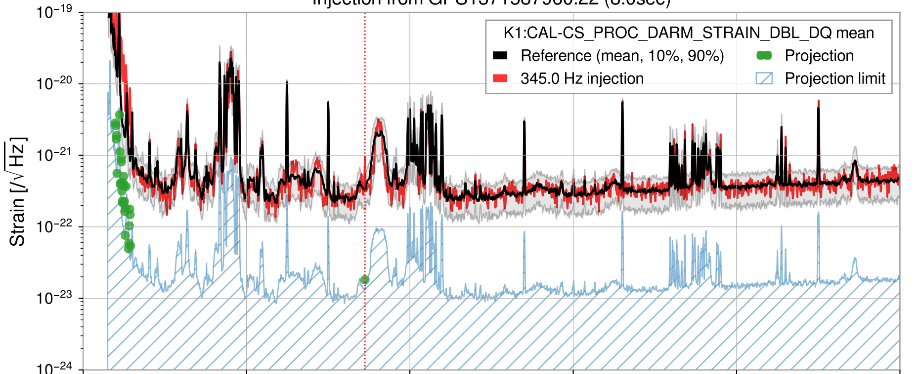
Injection from GPS1371587960.22 (8.0sec)
