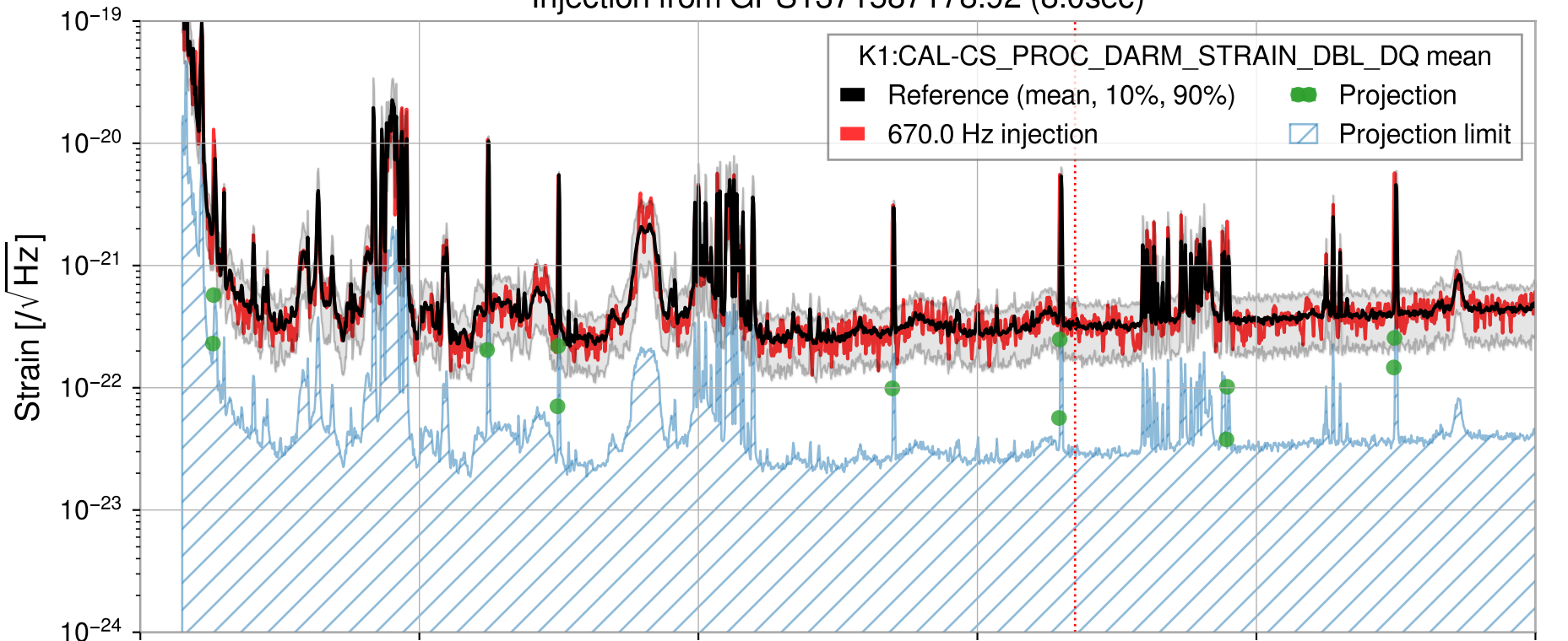
Injection from GPS1371587178.92 (8.0sec)
