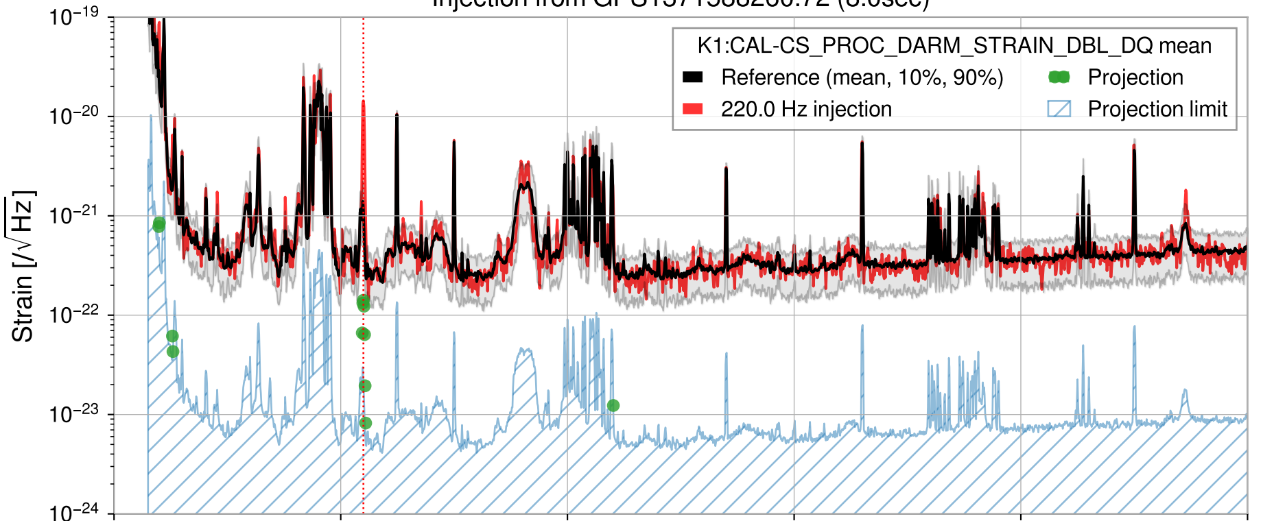
Injection from GPS1371588260.72 (8.0sec)
