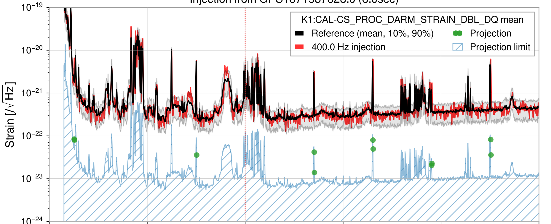
Injection from GPS1371587828.0 (8.0sec)
