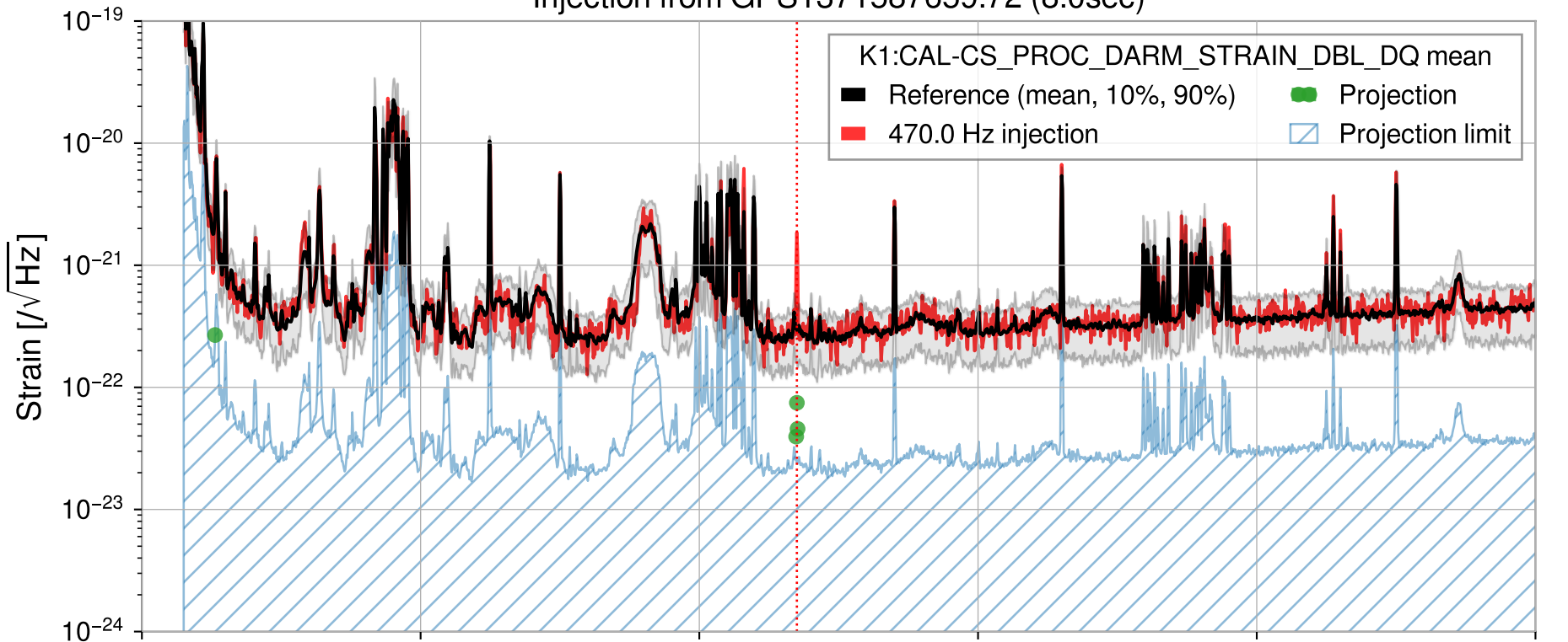
Injection from GPS1371587659.72 (8.0sec)
