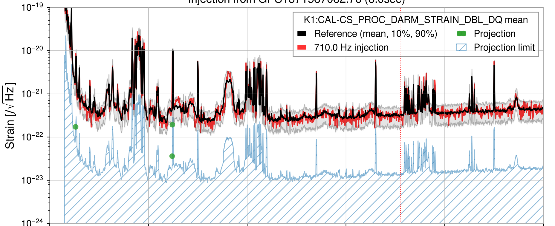
Injection from GPS1371587082.76 (8.0sec)
