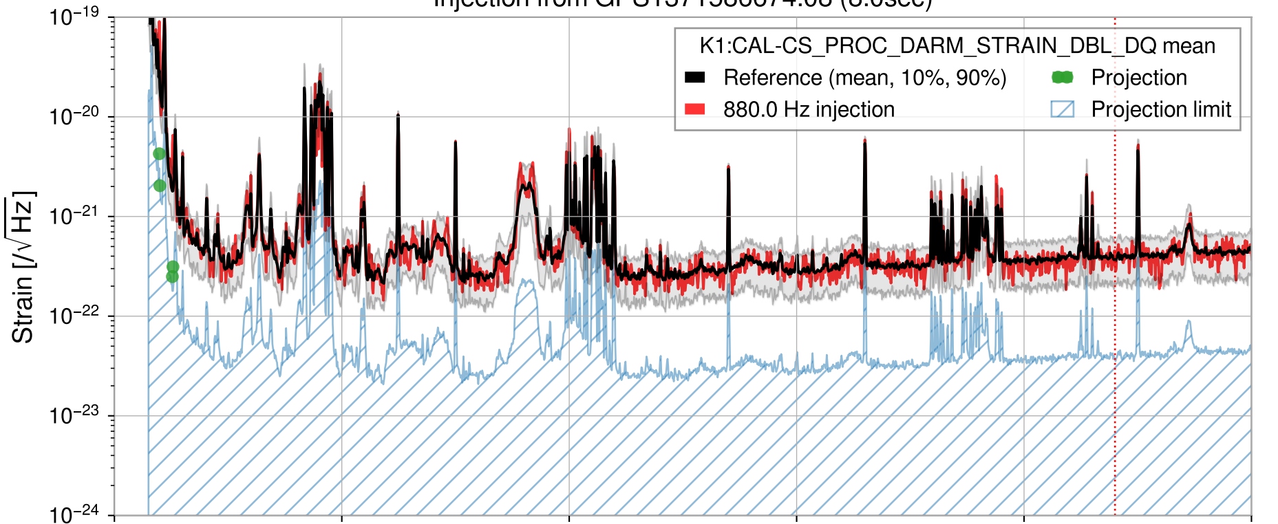
Injection from GPS1371586674.08 (8.0sec)
