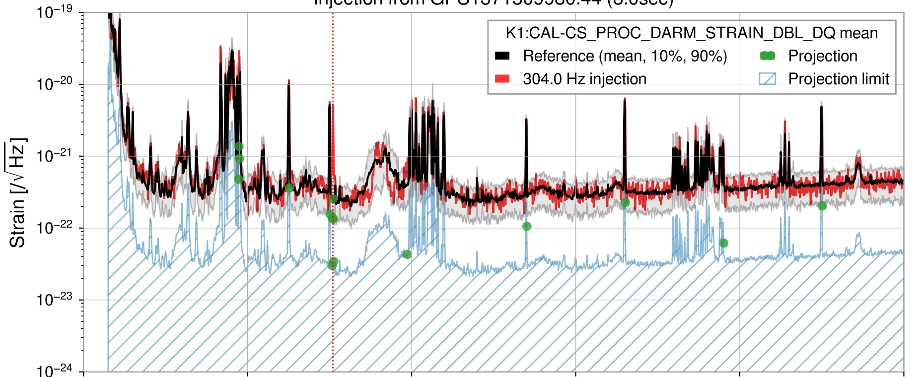
Injection from GPS1371509980.44 (8.0sec)
