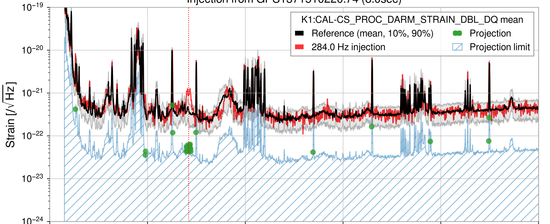
Injection from GPS1371510220.74 (8.0sec)
