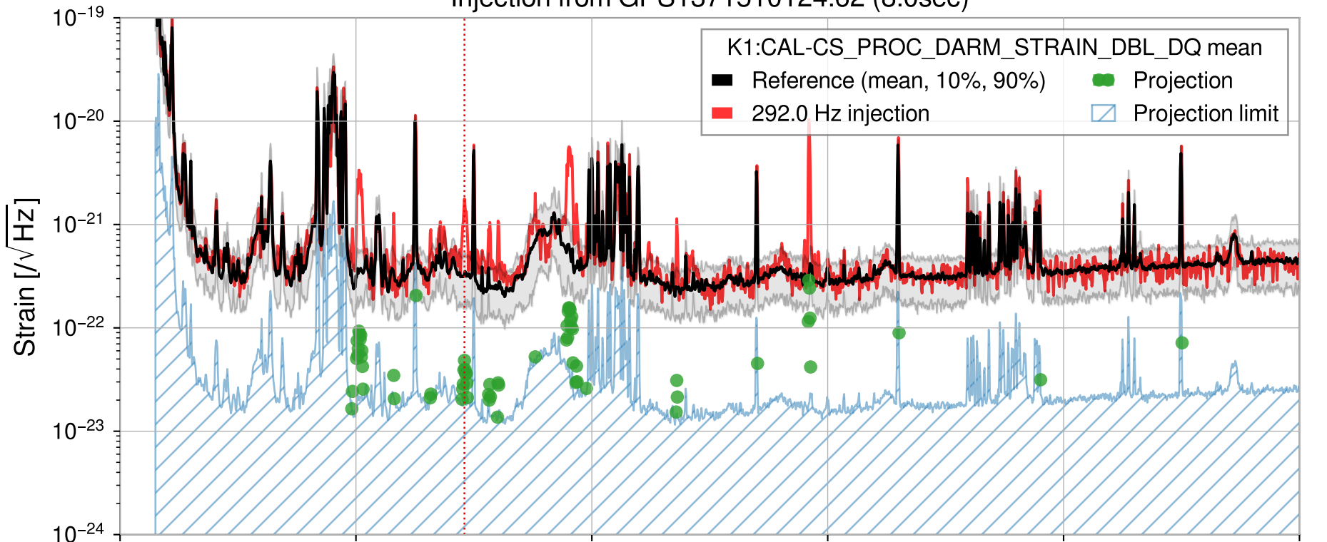
Injection from GPS1371510124.62 (8.0sec)
