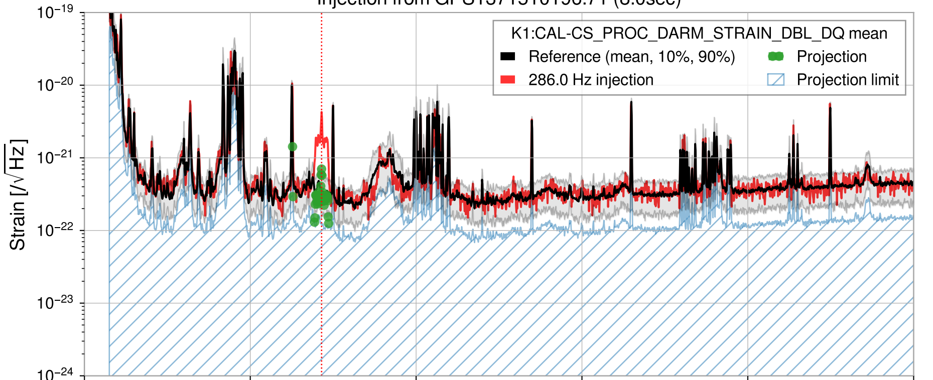
Injection from GPS1371510196.71 (8.0sec)
