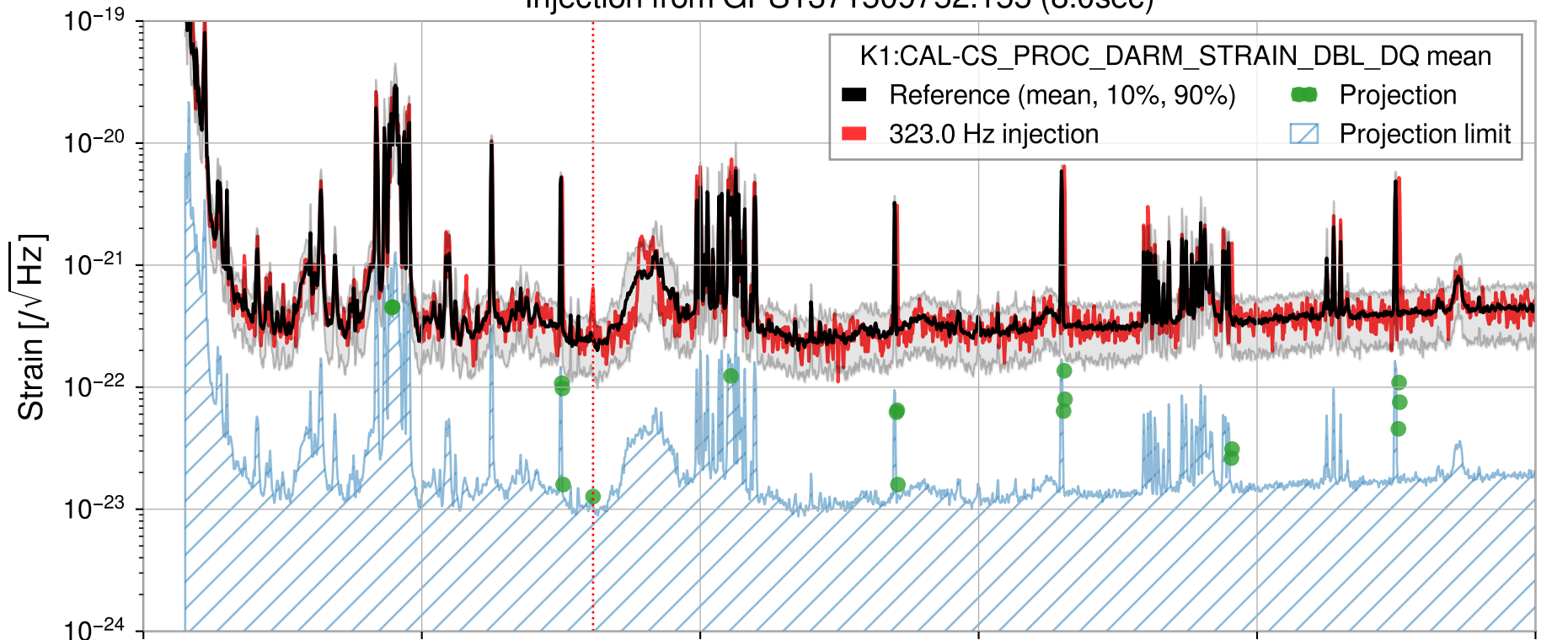
Injection from GPS1371509752.155 (8.0sec)
