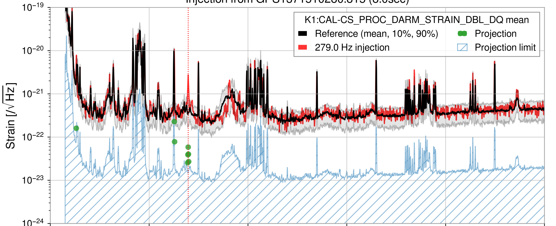
Injection from GPS1371510280.815 (8.0sec)
