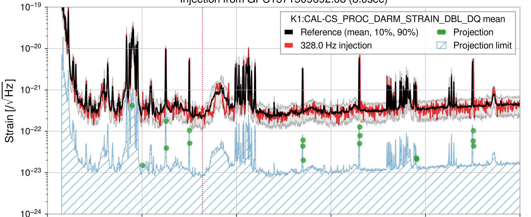
Injection from GPS1371509692.08 (8.0sec)
