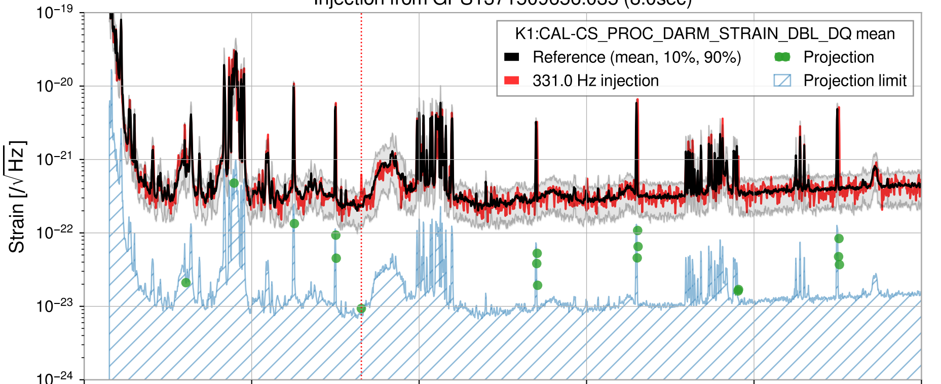
Injection from GPS1371509656.035 (8.0sec)
