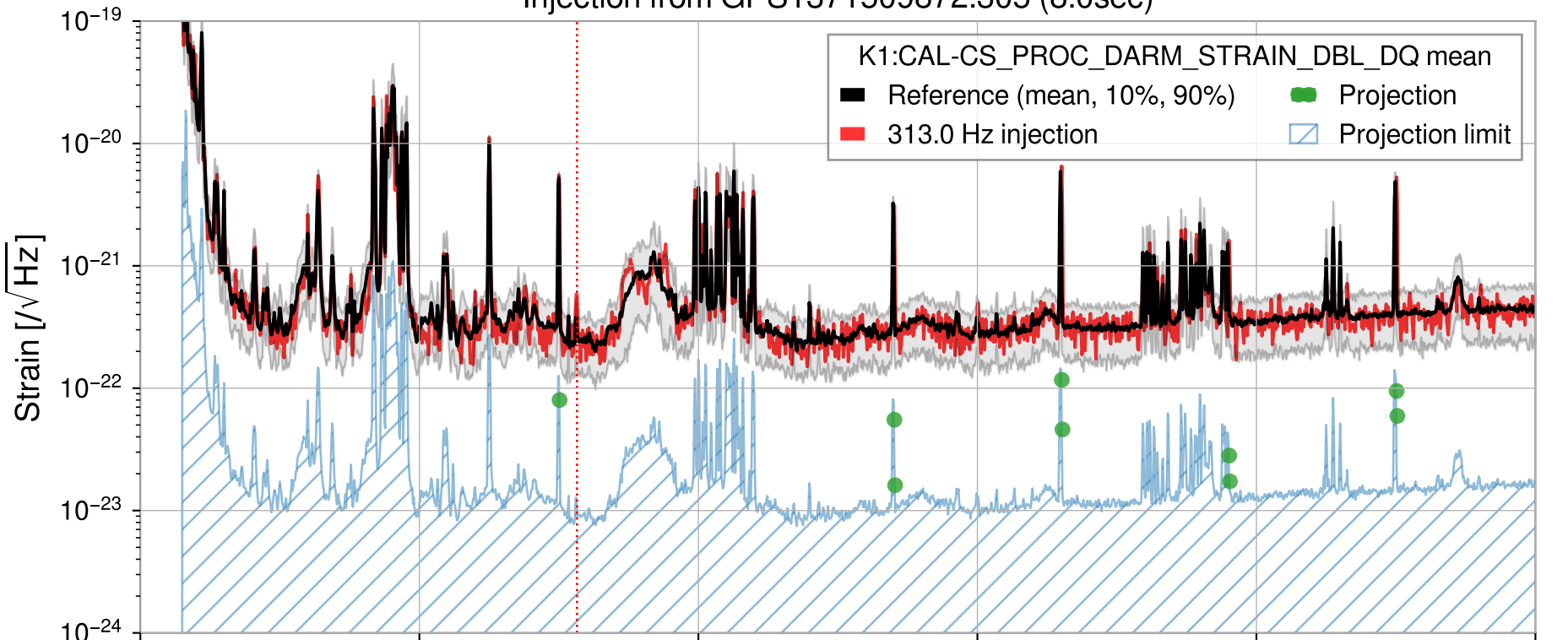
Injection from GPS1371509872.305 (8.0sec)
