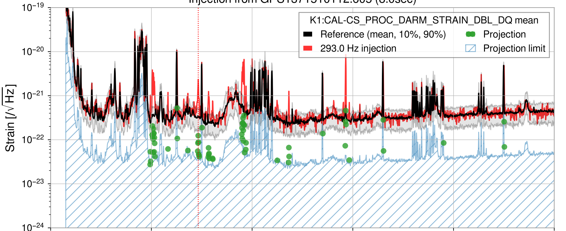
Injection from GPS1371510112.605 (8.0sec)
