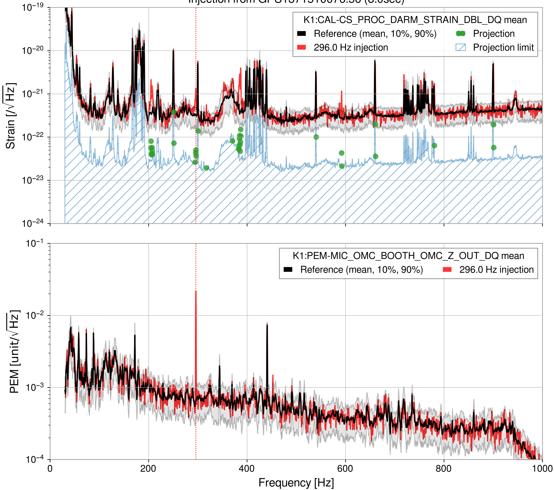
Injection from GPS1371510076.56 (8.0sec)
