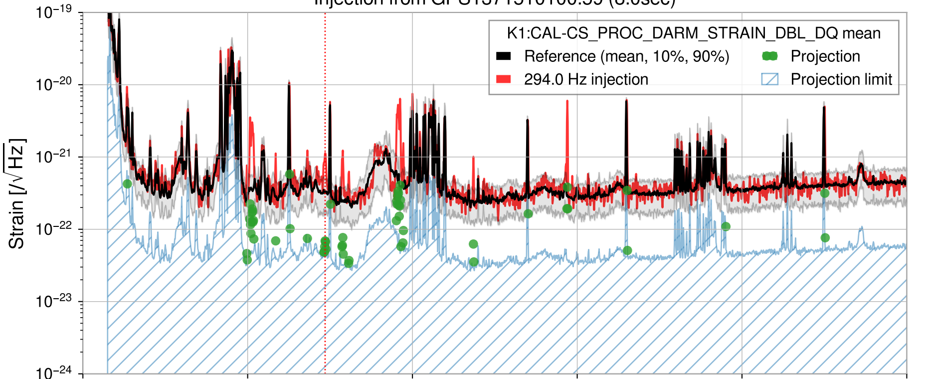
Injection from GPS1371510100.59 (8.0sec)
