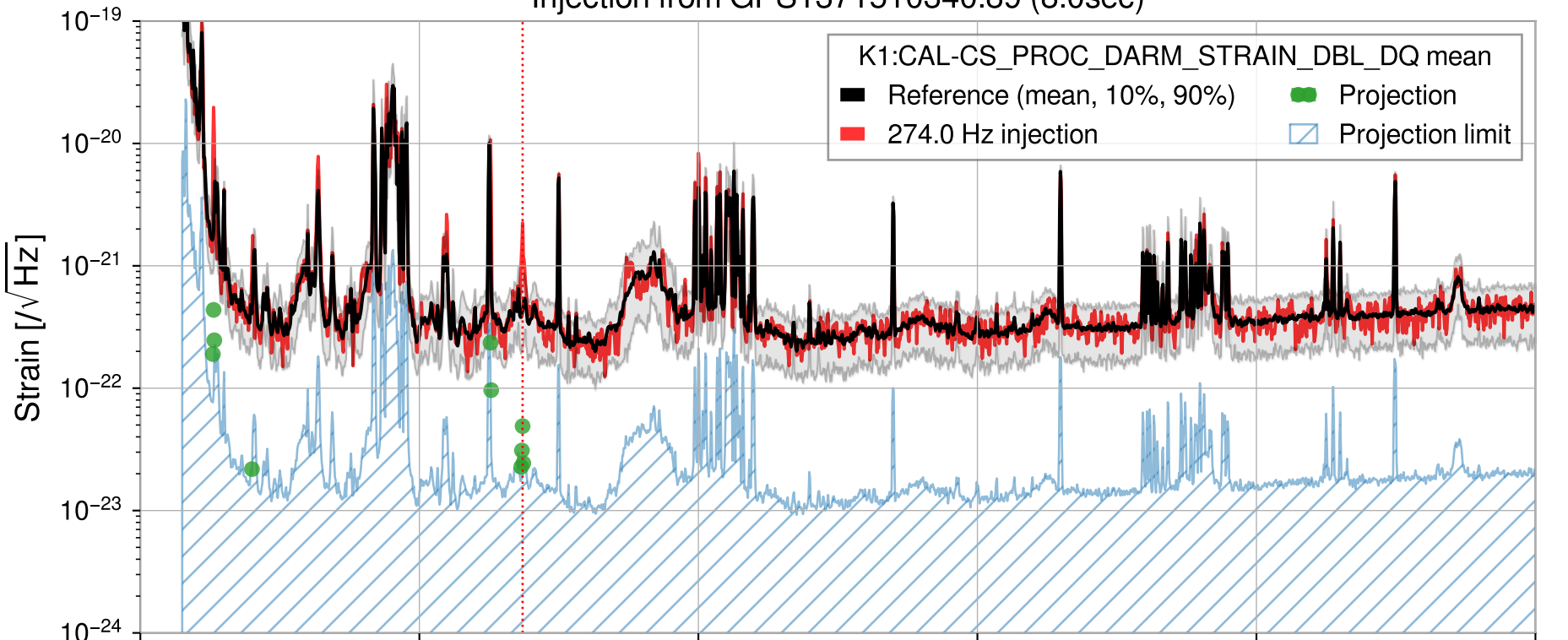
Injection from GPS1371510340.89 (8.0sec)
