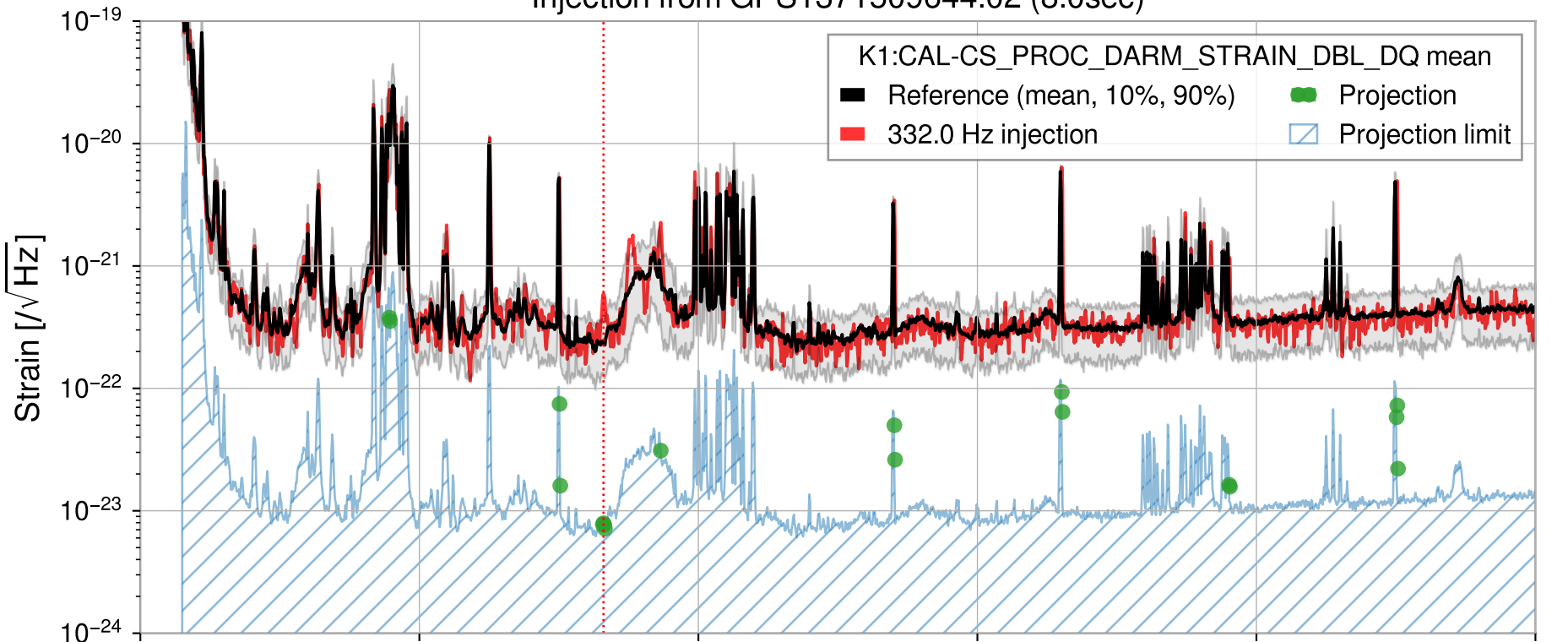
Injection from GPS1371509644.02 (8.0sec)
