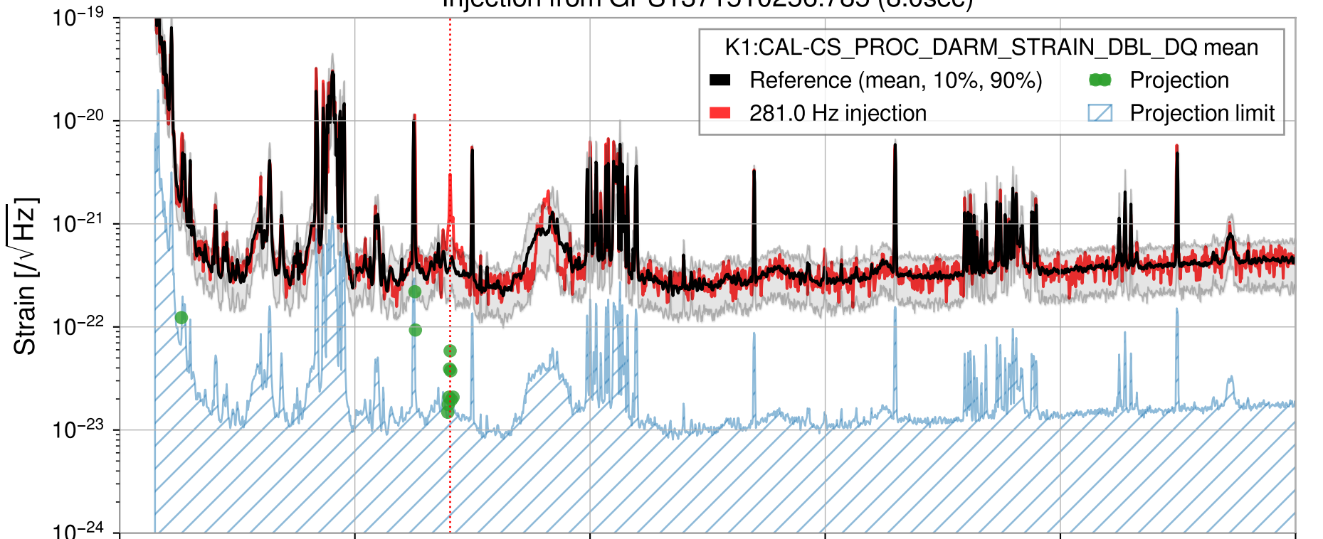
Injection from GPS1371510256.785 (8.0sec)
