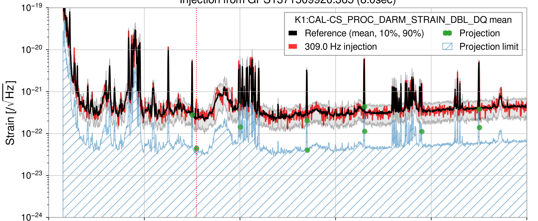
Injection from GPS1371509920.365 (8.0sec)
