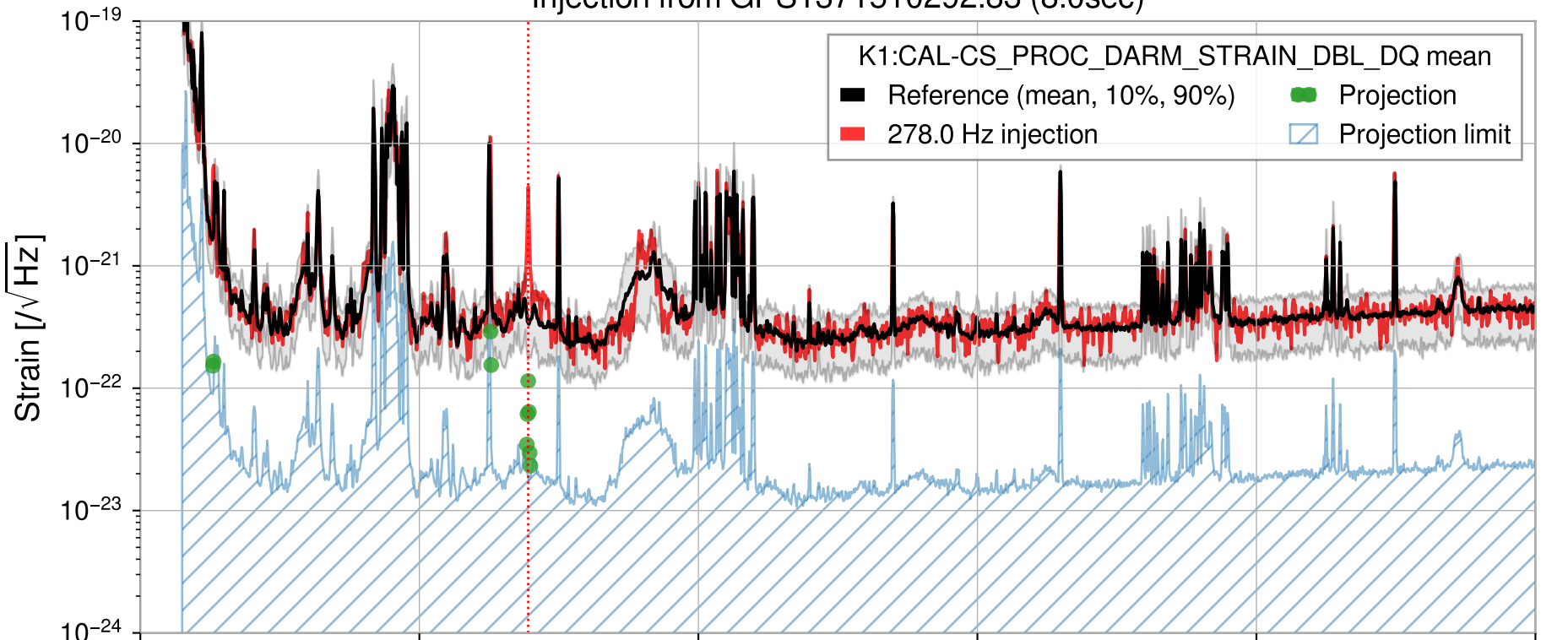
Injection from GPS1371510292.83 (8.0sec)
