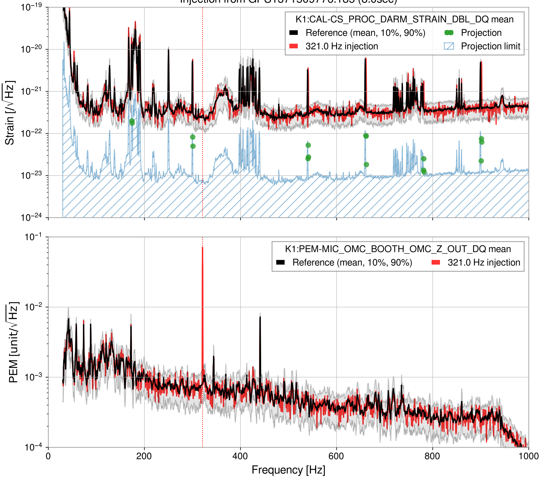
Injection from GPS1371509776.185 (8.0sec)
