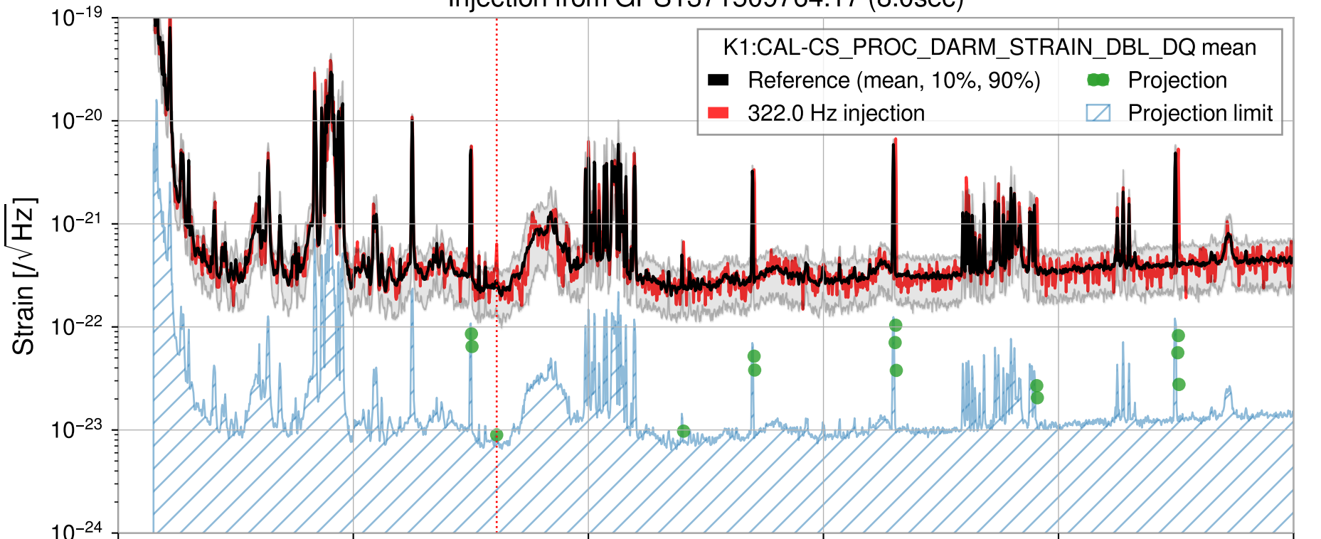
Injection from GPS1371509764.17 (8.0sec)
