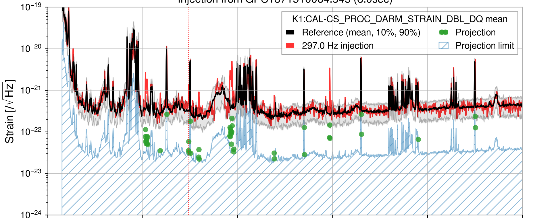
Injection from GPS1371510064.545 (8.0sec)
