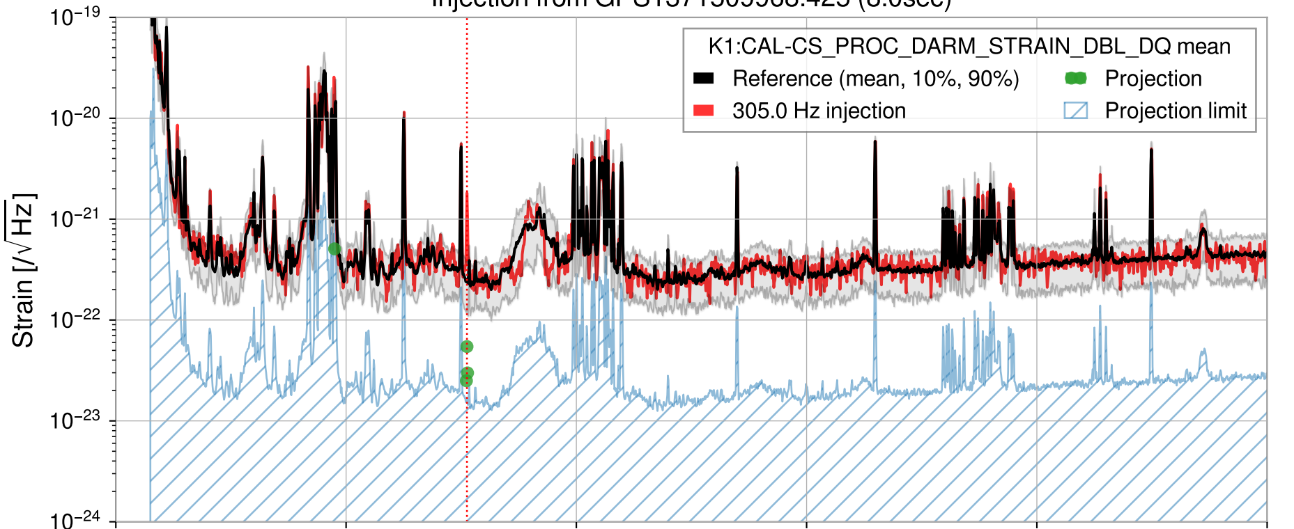
Injection from GPS1371509968.425 (8.0sec)
