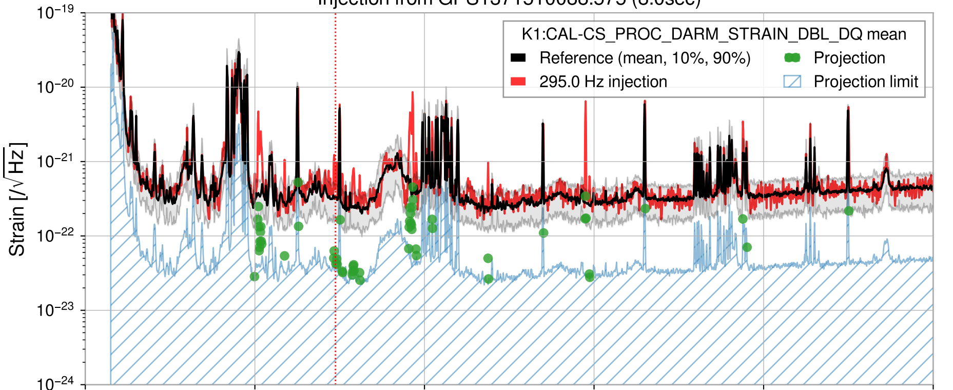
Injection from GPS1371510088.575 (8.0sec)
