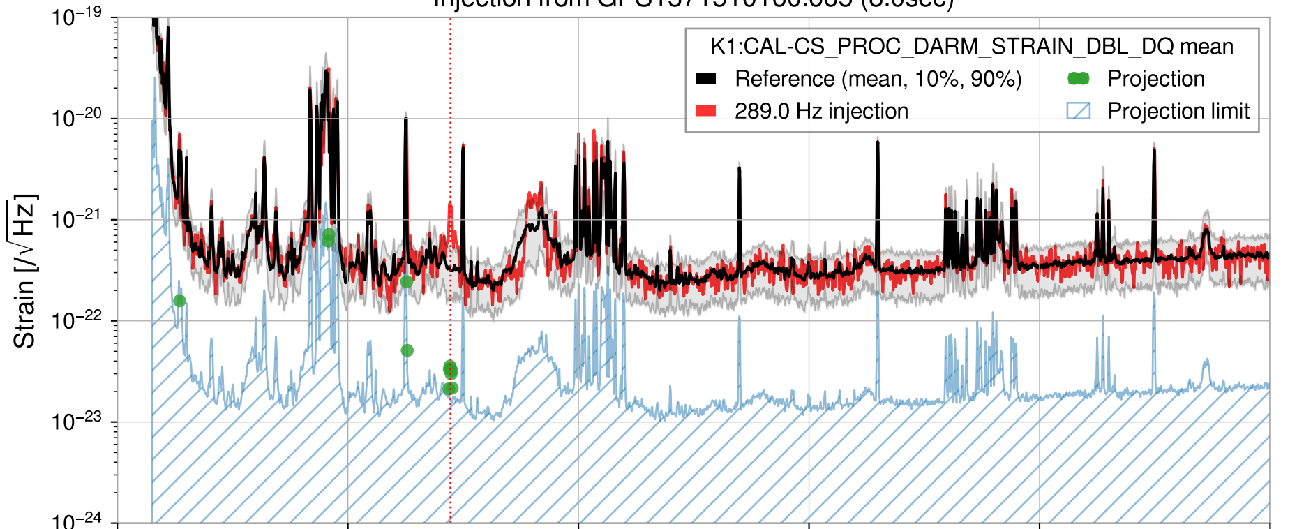
Injection from GPS1371510160.665 (8.0sec)
