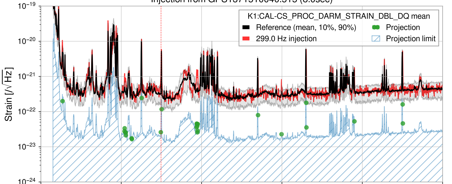
Injection from GPS1371510040.515 (8.0sec)
