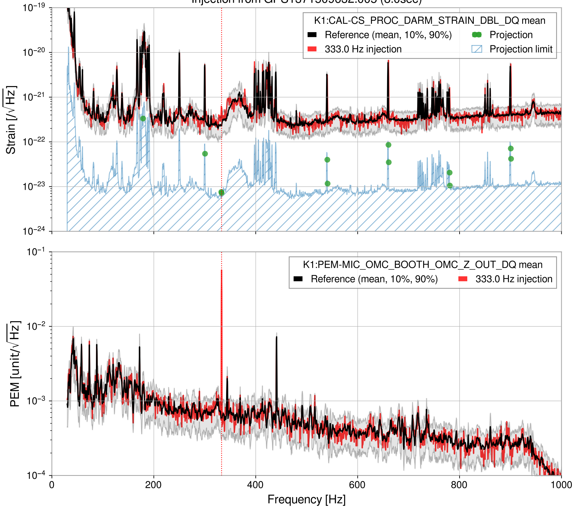
Injection from GPS1371509632.005 (8.0sec)
