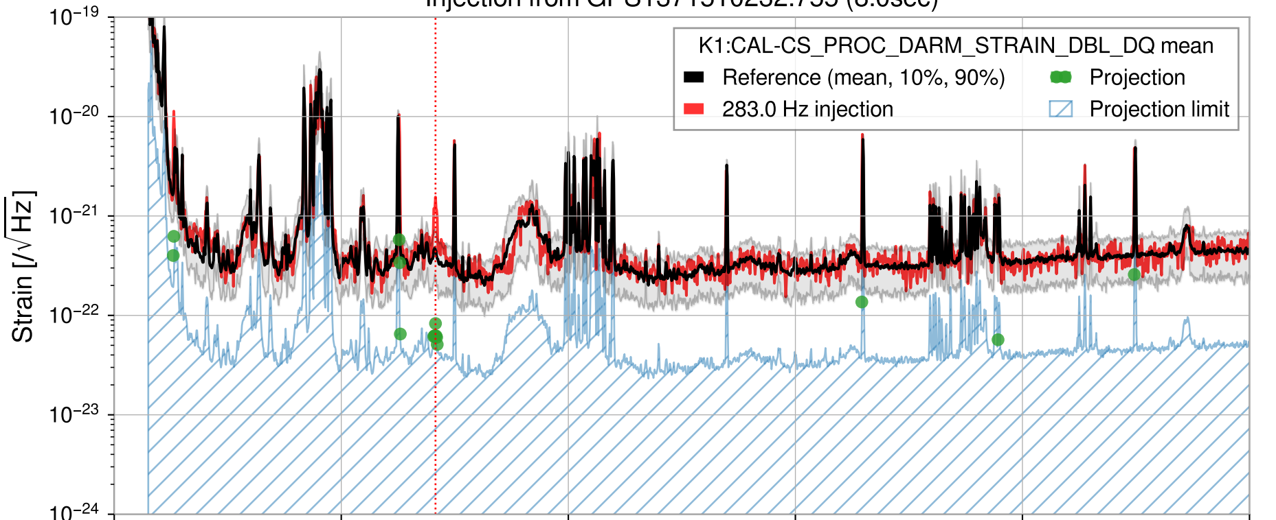
Injection from GPS1371510232.755 (8.0sec)
