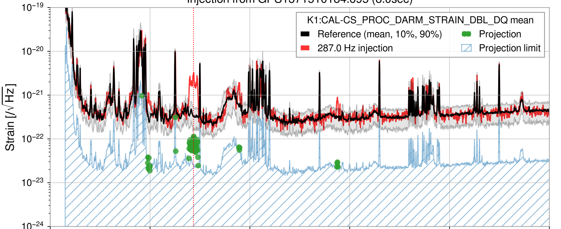
Injection from GPS1371510184.695 (8.0sec)
