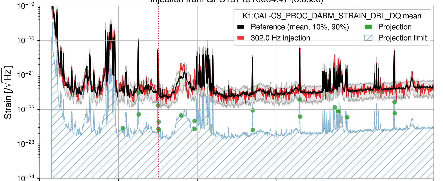
Injection from GPS1371510004.47 (8.0sec)
