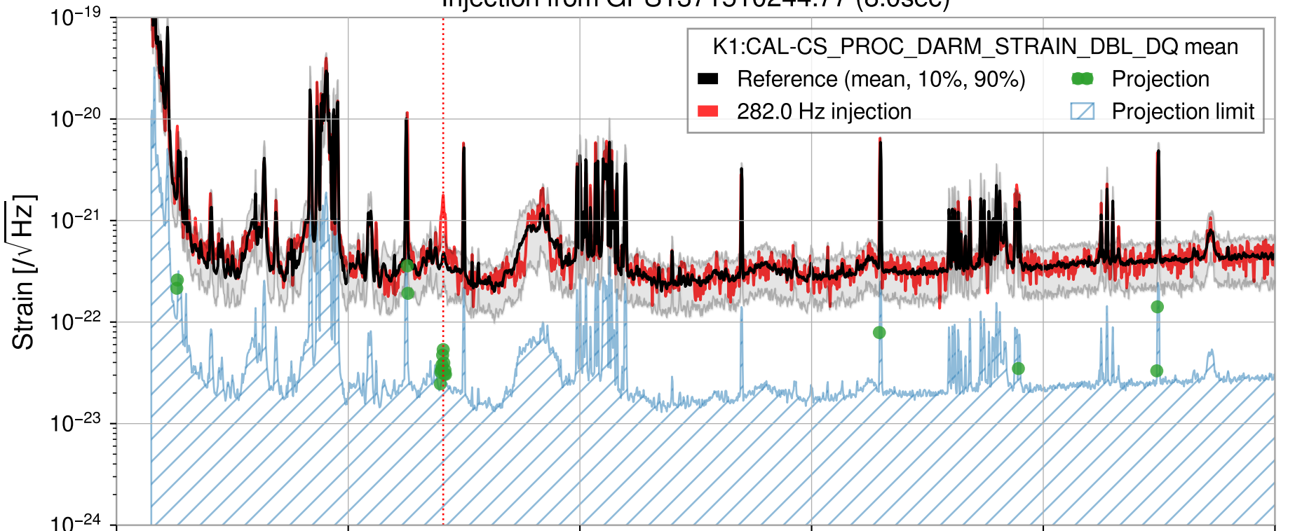
Injection from GPS1371510244.77 (8.0sec)
