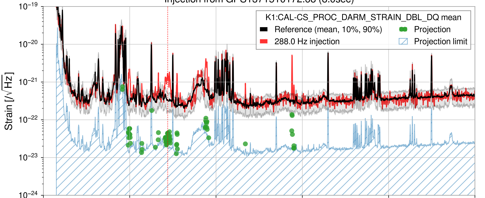
Injection from GPS1371510172.68 (8.0sec)
