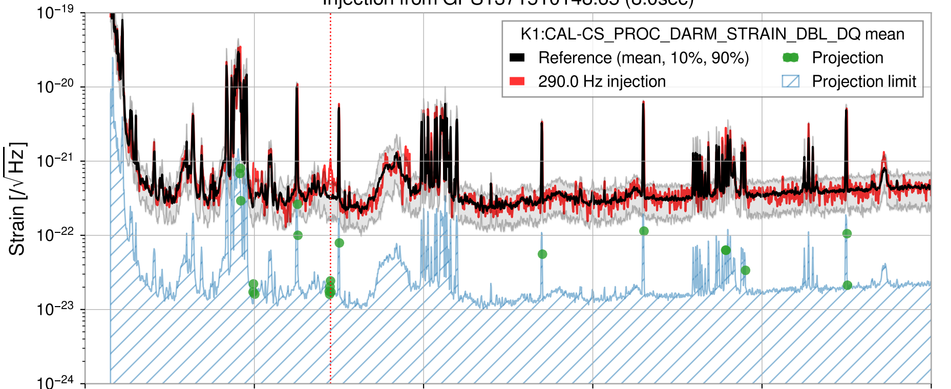
Injection from GPS1371510148.65 (8.0sec)
