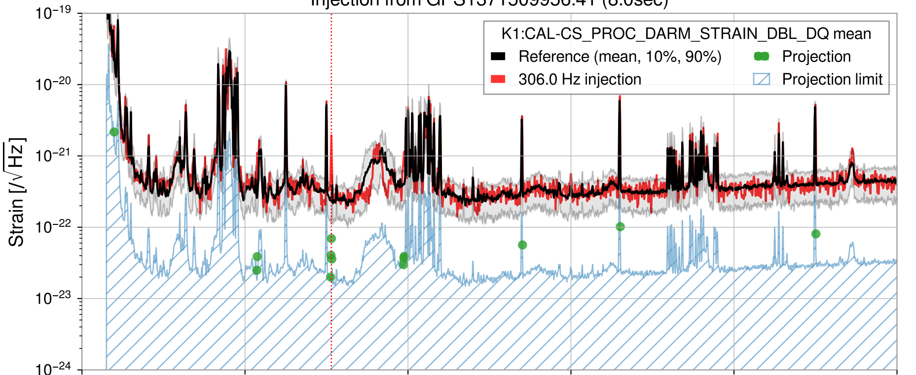
Injection from GPS1371509956.41 (8.0sec)
