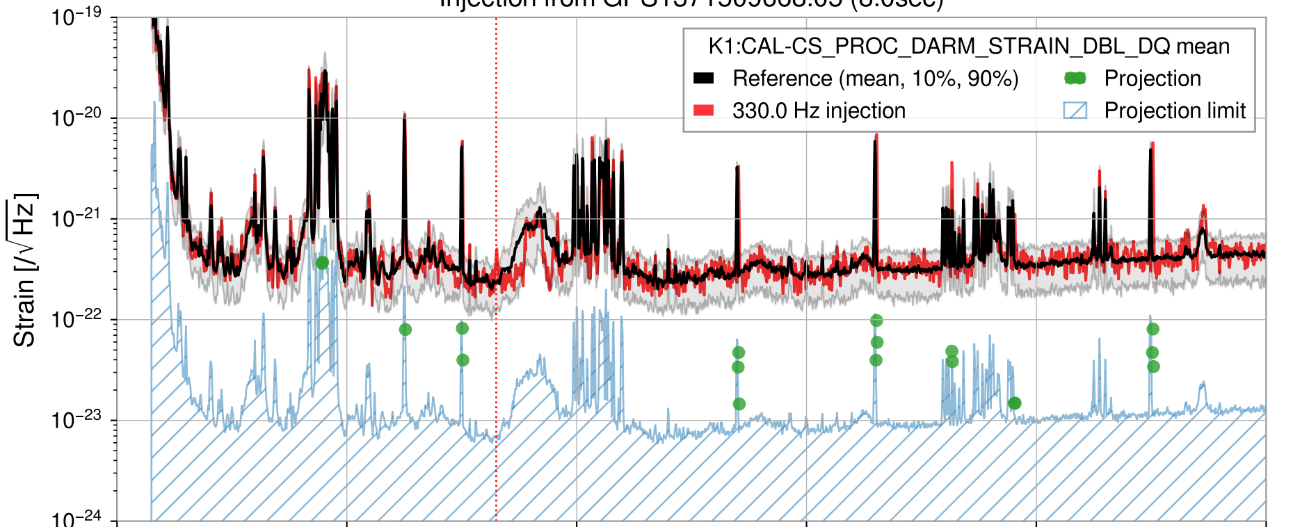
Injection from GPS1371509668.05 (8.0sec)
