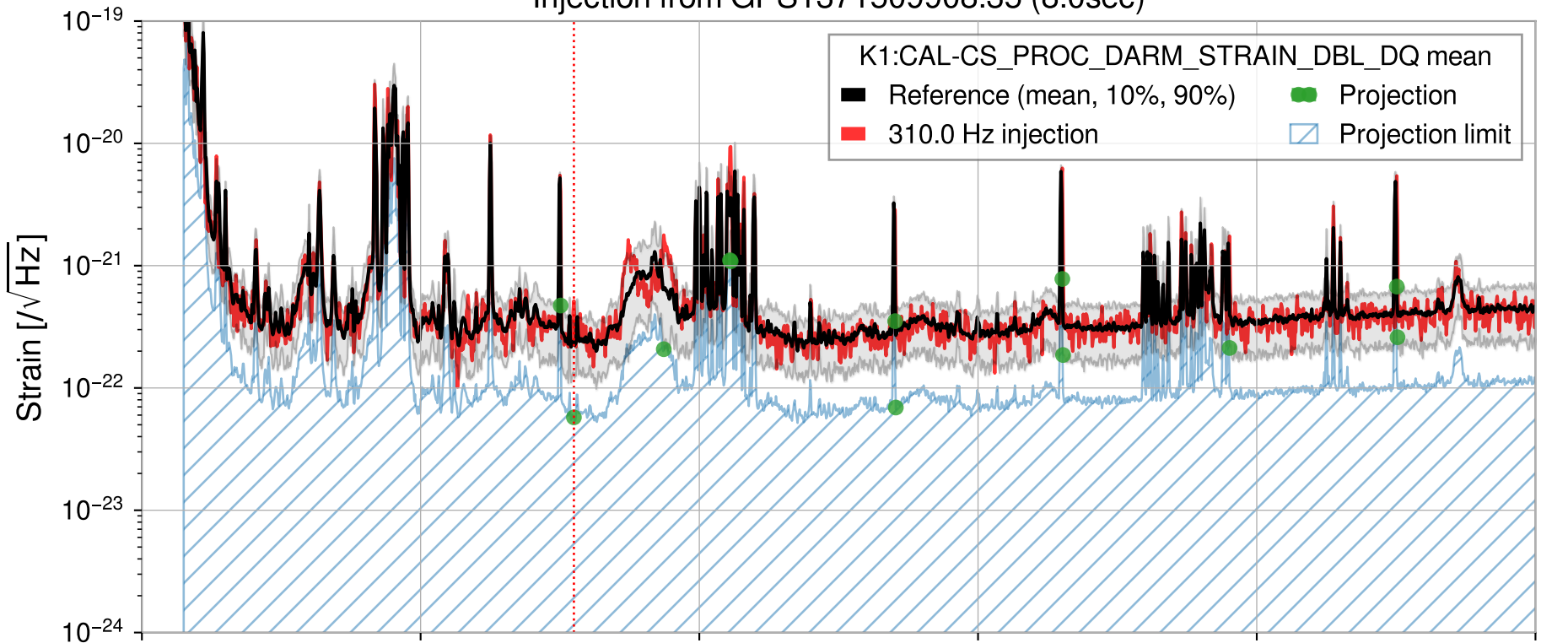
Injection from GPS1371509908.35 (8.0sec)
