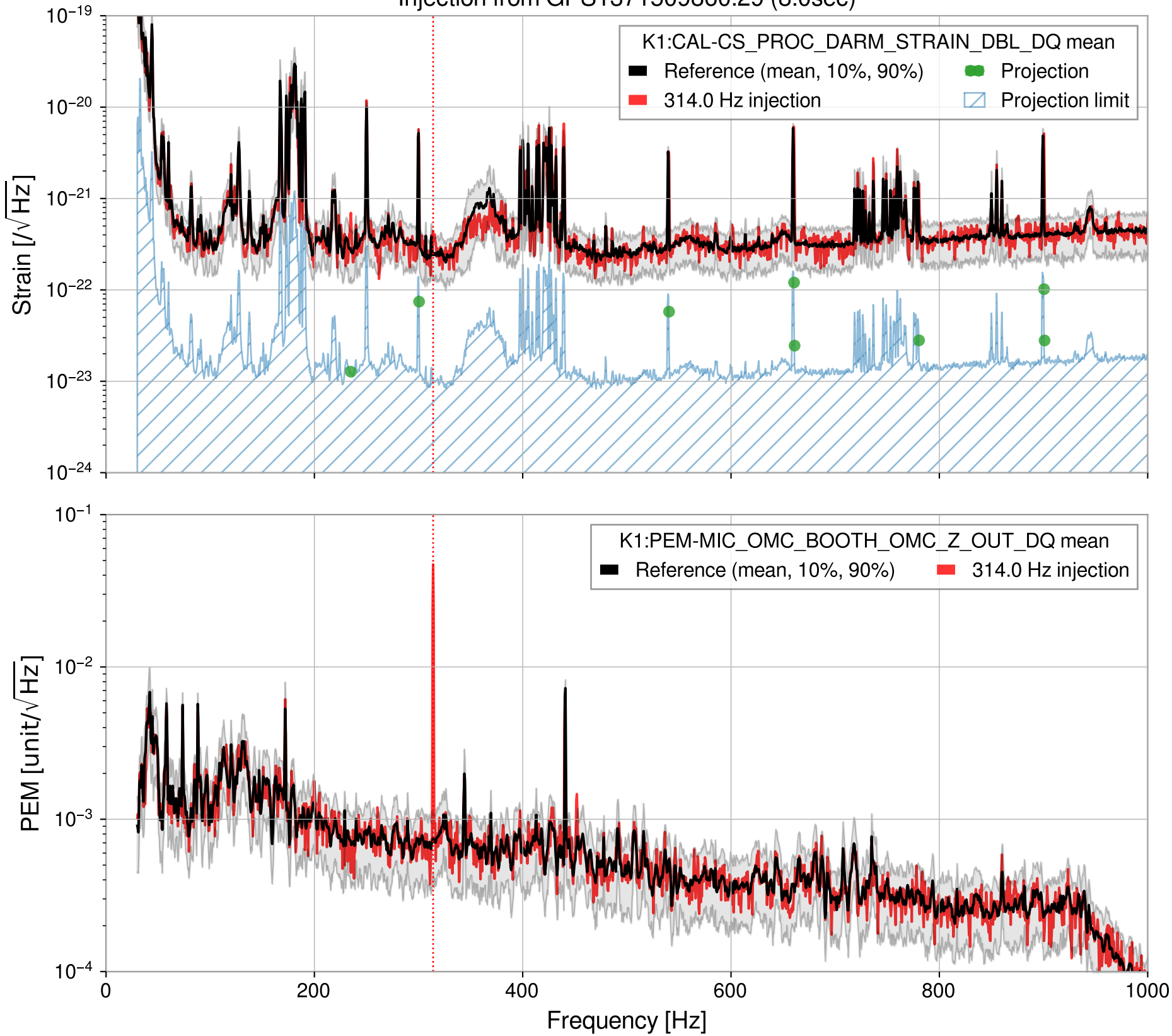
Injection from GPS1371509860.29 (8.0sec)
