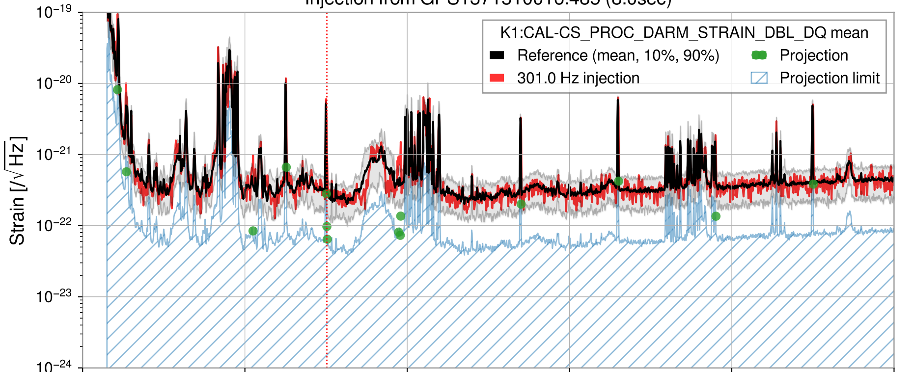
Injection from GPS1371510016.485 (8.0sec)
