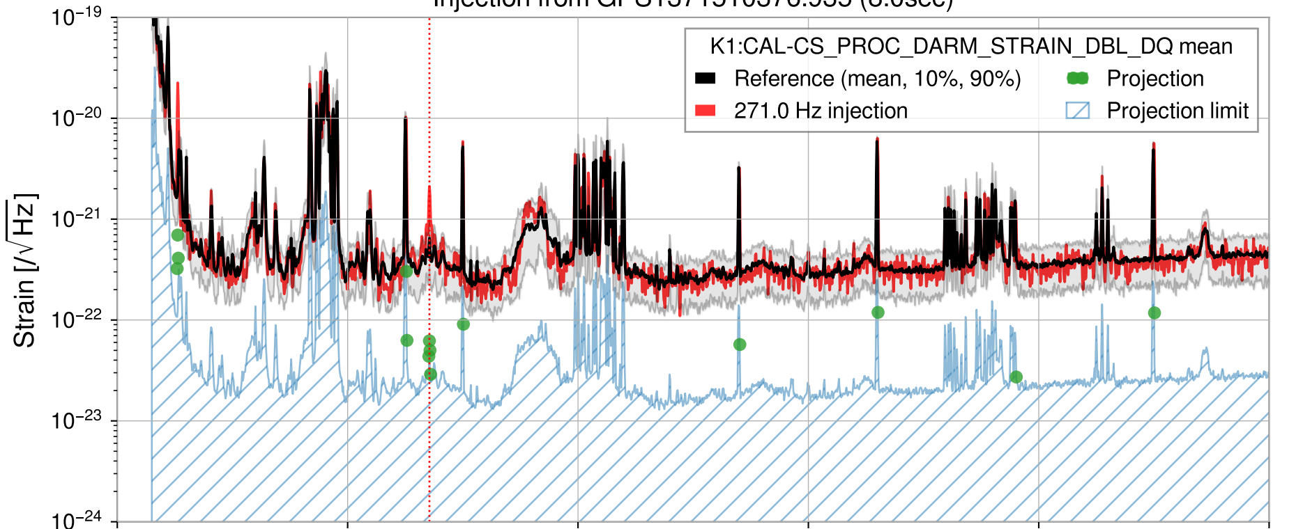
Injection from GPS1371510376.935 (8.0sec)
