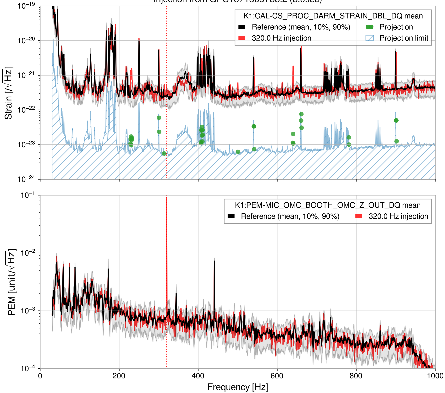
Injection from GPS1371509788.2 (8.0sec)
