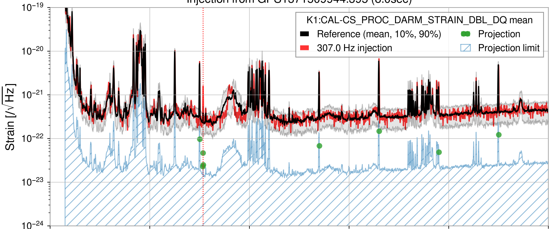
Injection from GPS1371509944.395 (8.0sec)
