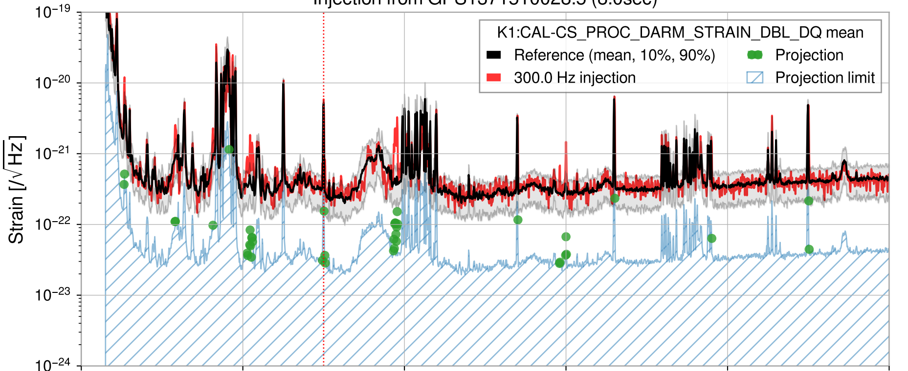
Injection from GPS1371510028.5 (8.0sec)
