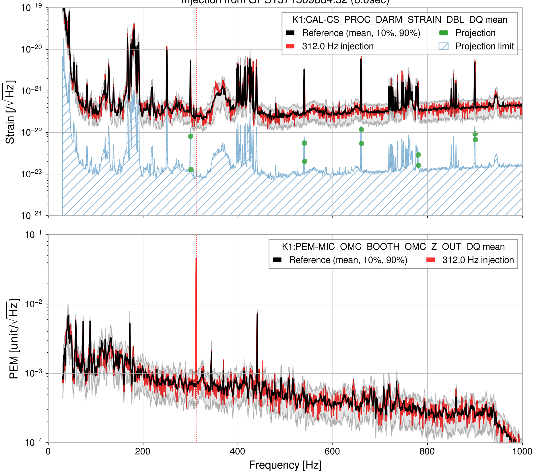
Injection from GPS1371509884.32 (8.0sec)
