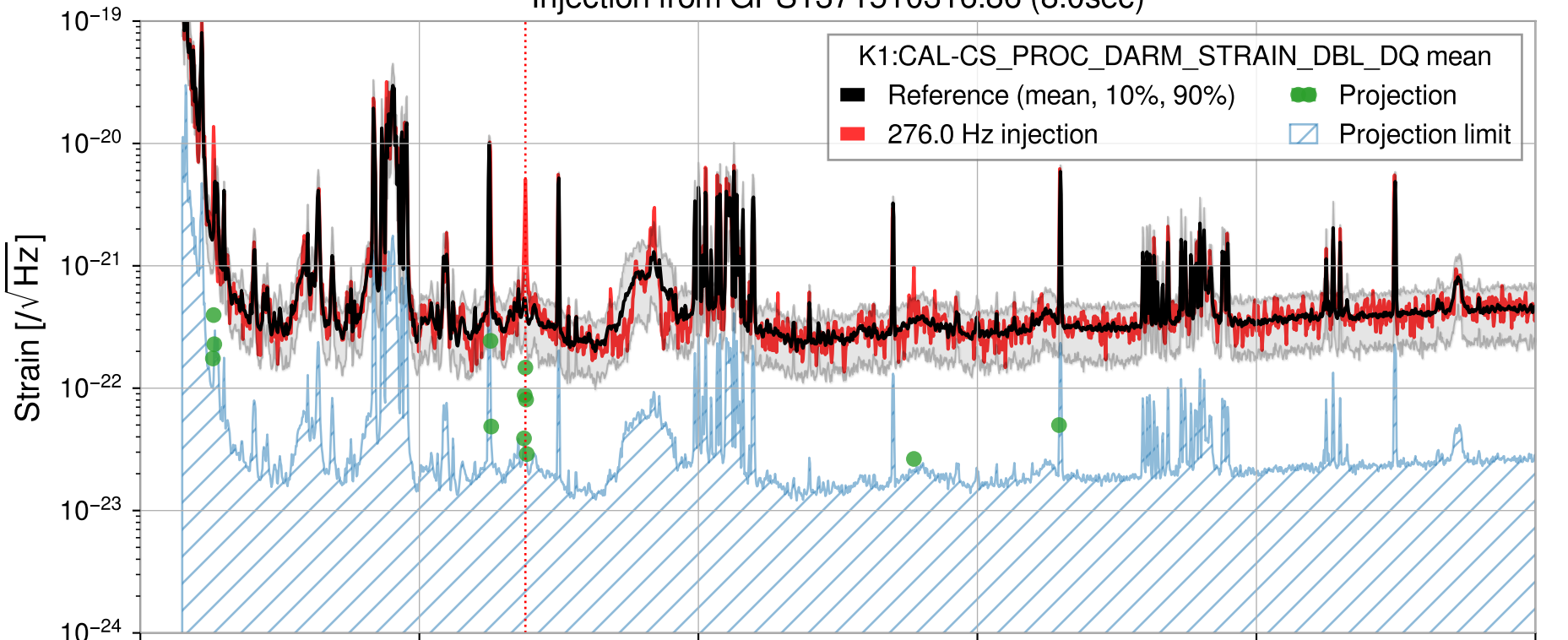
Injection from GPS1371510316.86 (8.0sec)
