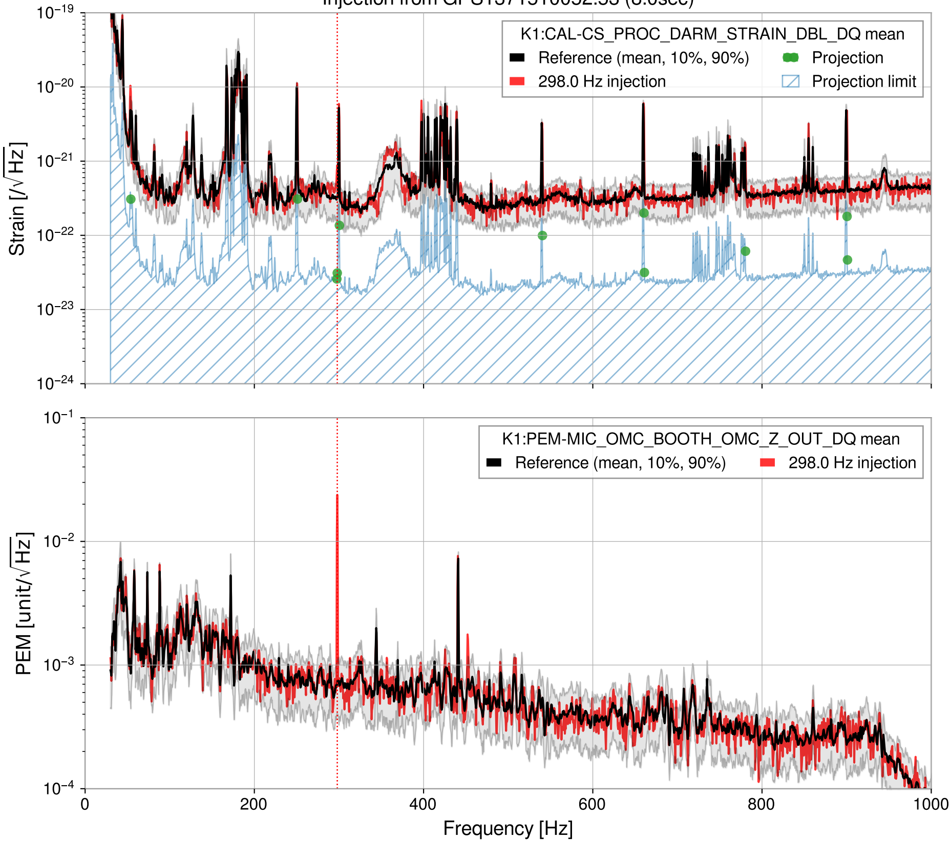
Injection from GPS1371510052.53 (8.0sec)
