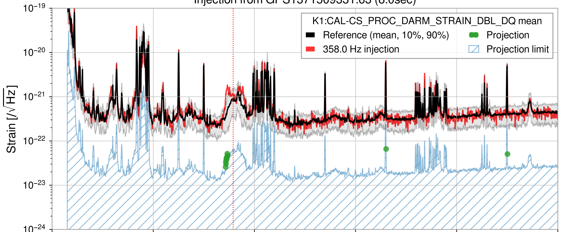
Injection from GPS1371509331.63 (8.0sec)
