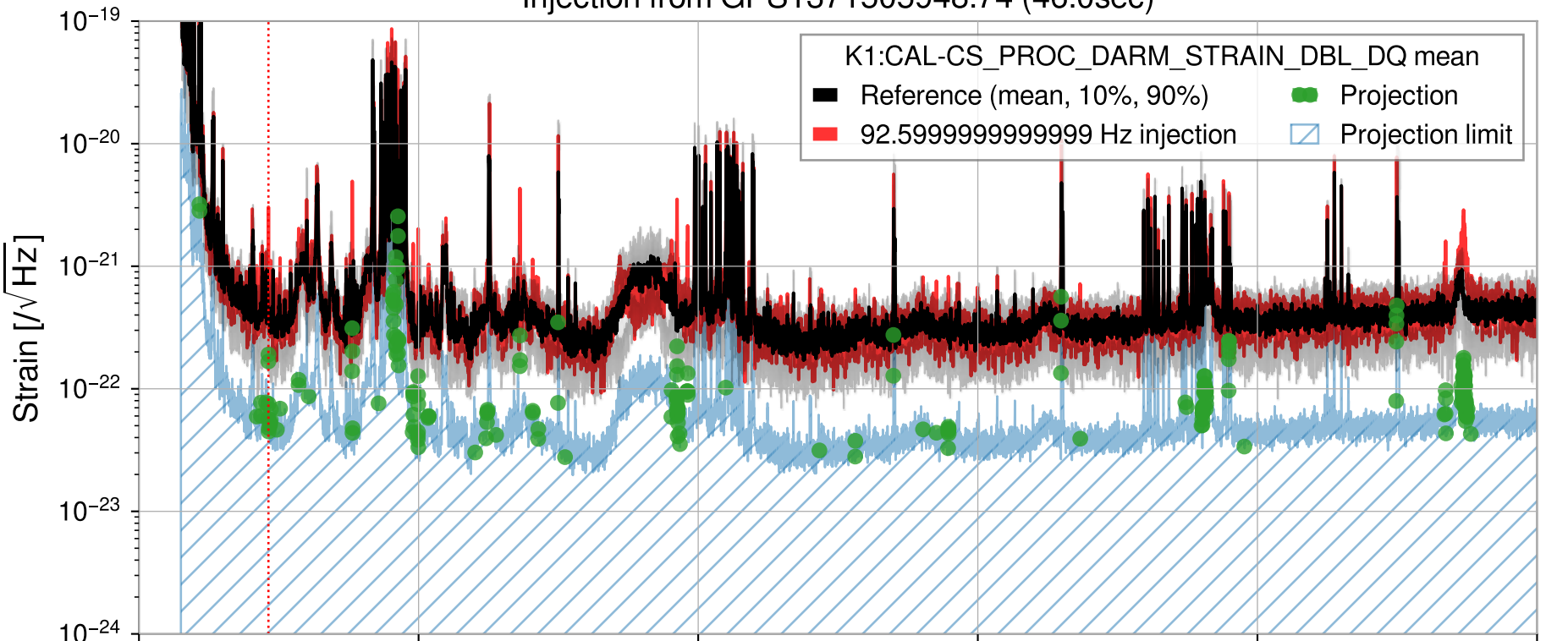
Injection from GPS1371505948.74 (46.0sec)
