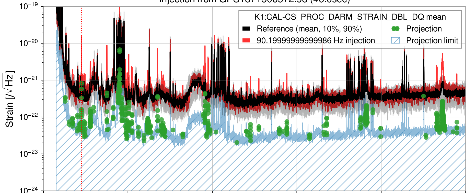
Injection from GPS1371506572.98 (46.0sec)
