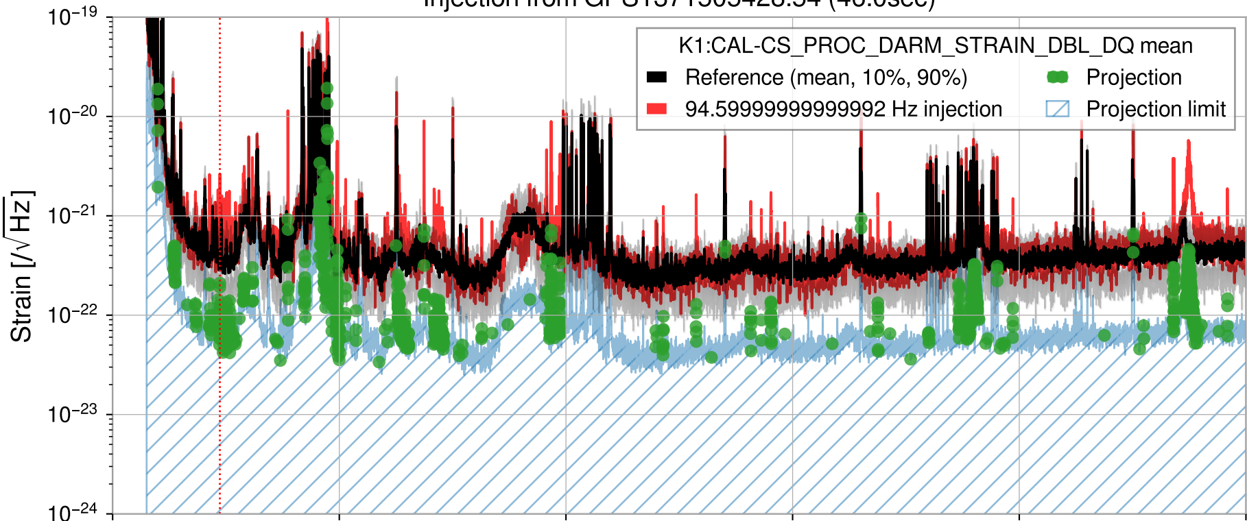
Injection from GPS1371505428.54 (46.0sec)
