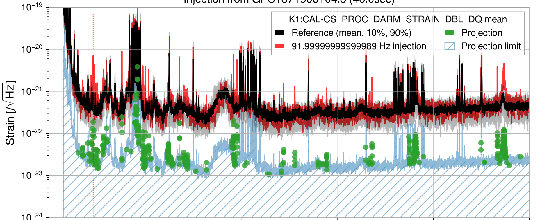
Injection from GPS1371506104.8 (46.0sec)
