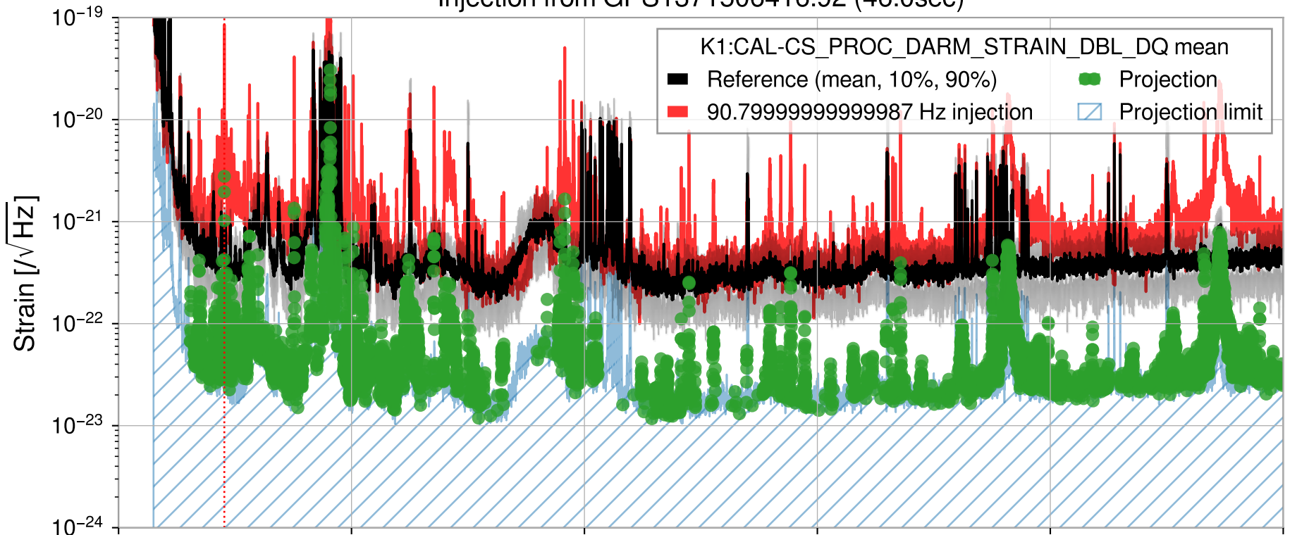
Injection from GPS1371506416.92 (46.0sec)
