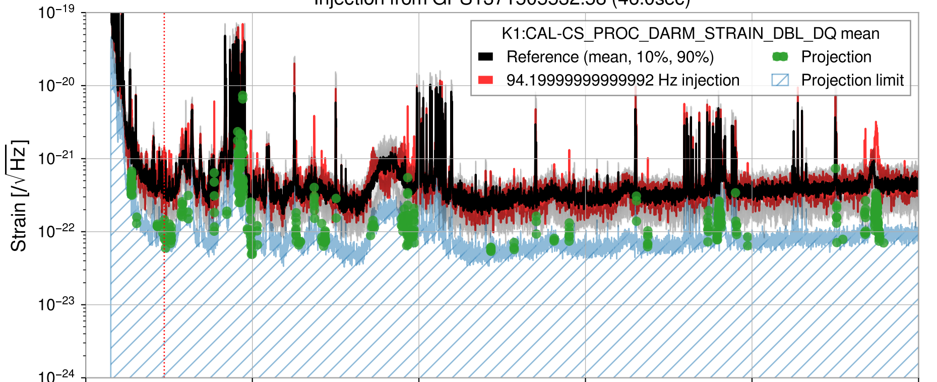
Injection from GPS1371505532.58 (46.0sec)
