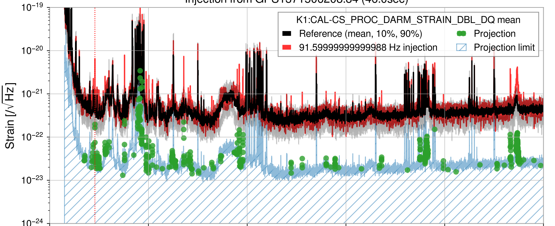
Injection from GPS1371506208.84 (46.0sec)
