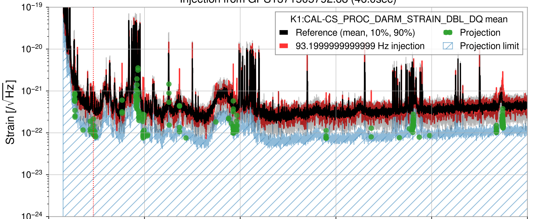
Injection from GPS1371505792.68 (46.0sec)
