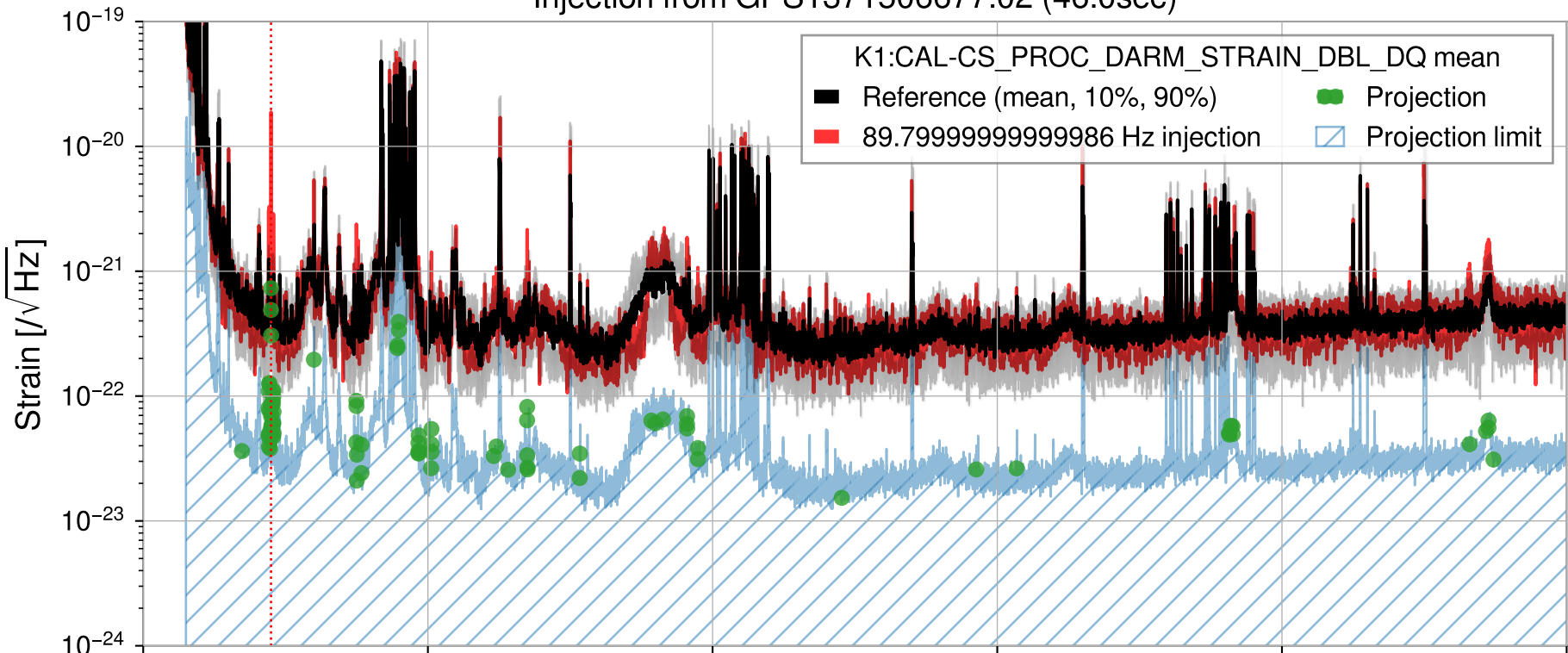
Injection from GPS1371506677.02 (46.0sec)
