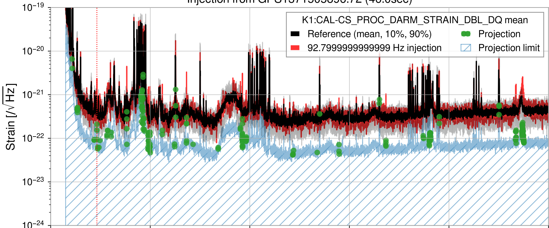
Injection from GPS1371505896.72 (46.0sec)
