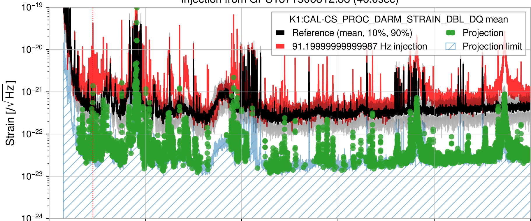
Injection from GPS1371506312.88 (46.0sec)
