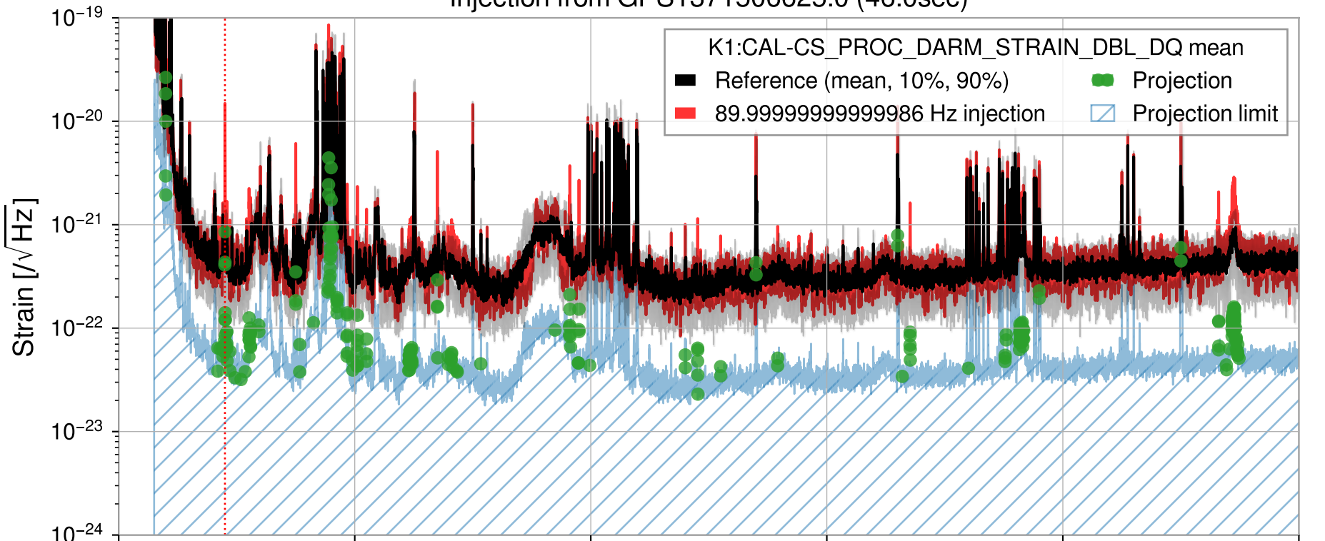
Injection from GPS1371506625.0 (46.0sec)
