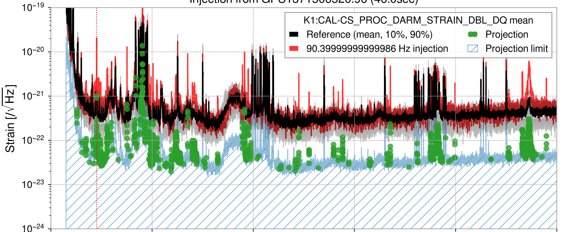
Injection from GPS1371506520.96 (46.0sec)
