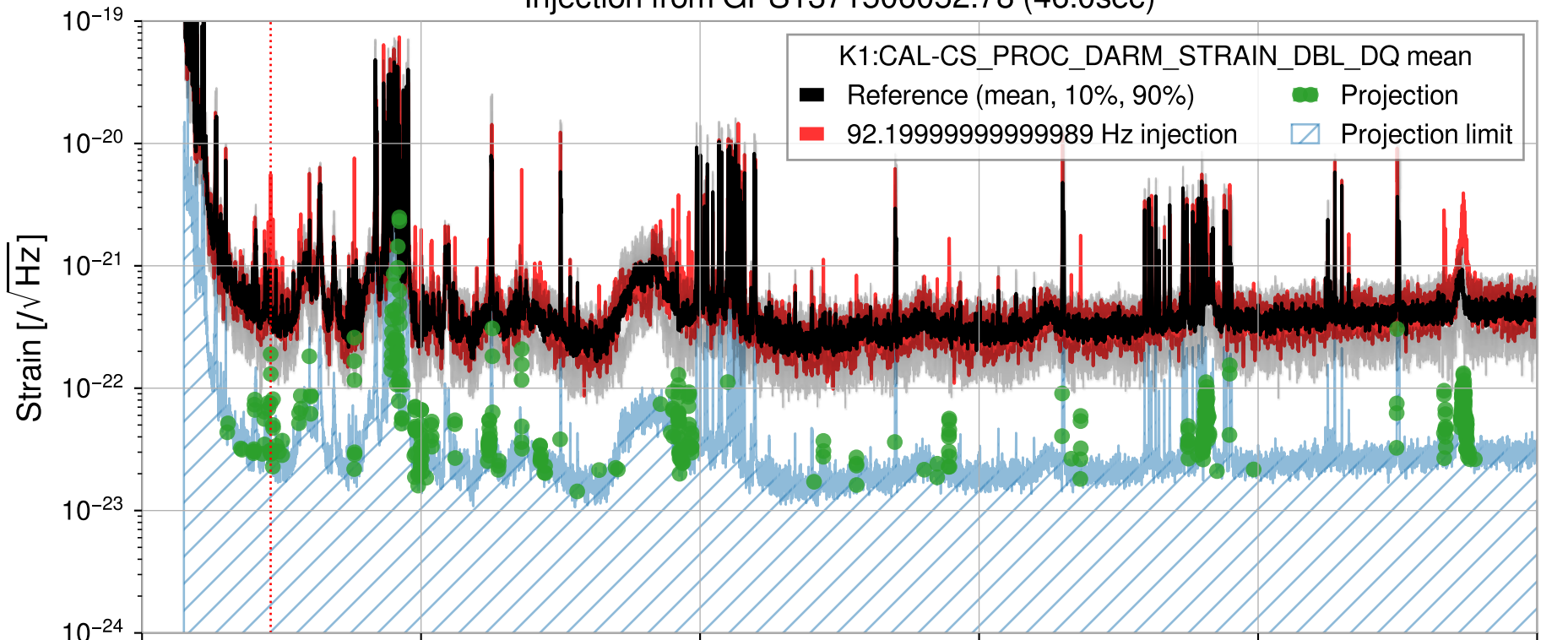
Injection from GPS1371506052.78 (46.0sec)
