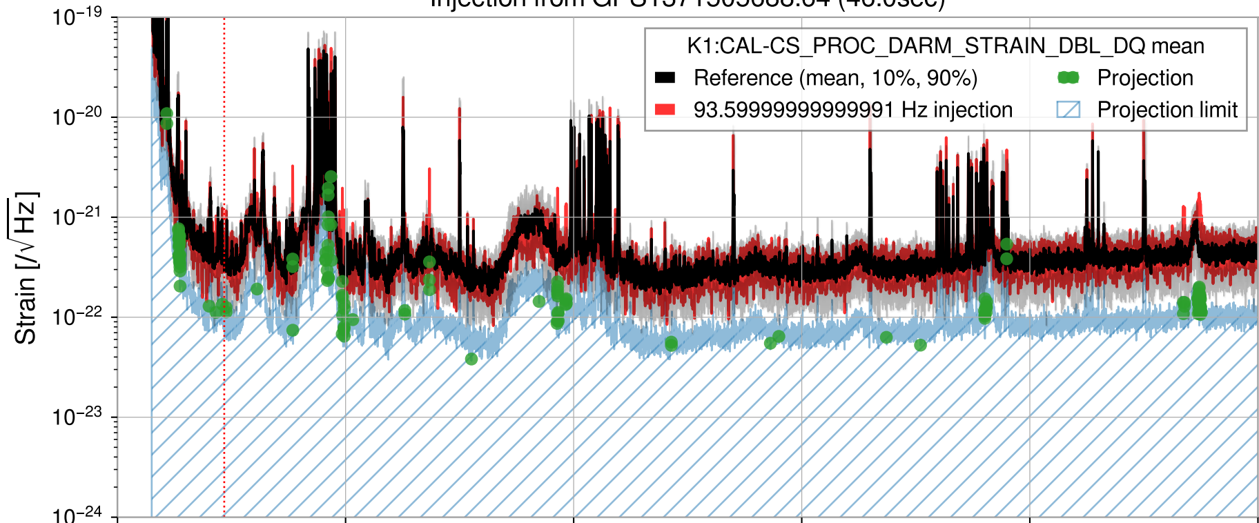
Injection from GPS1371505688.64 (46.0sec)
