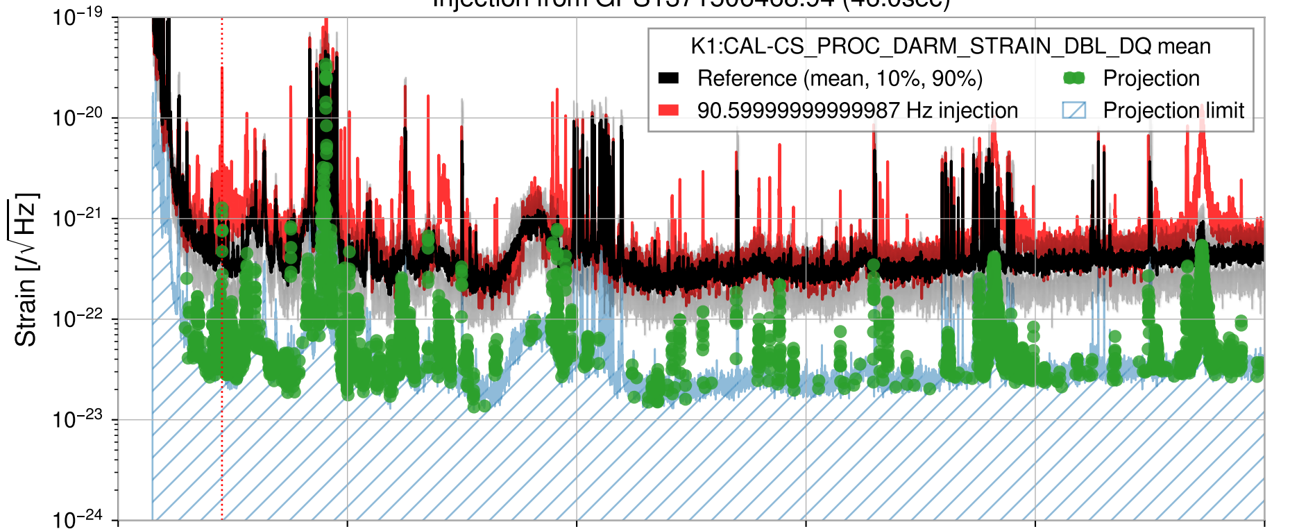
Injection from GPS1371506468.94 (46.0sec)
