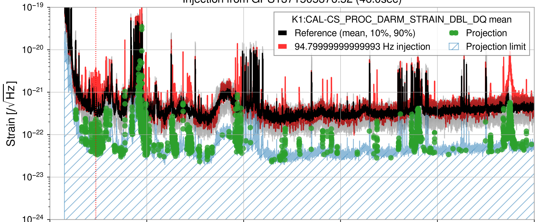
Injection from GPS1371505376.52 (46.0sec)
