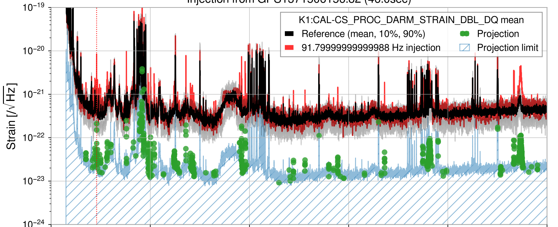
Injection from GPS1371506156.82 (46.0sec)
