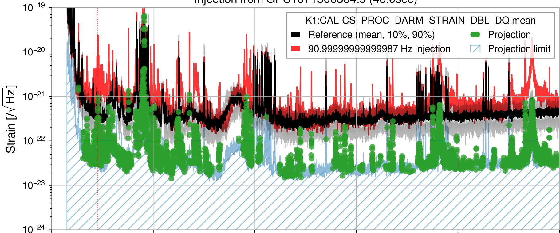
Injection from GPS1371506364.9 (46.0sec)
