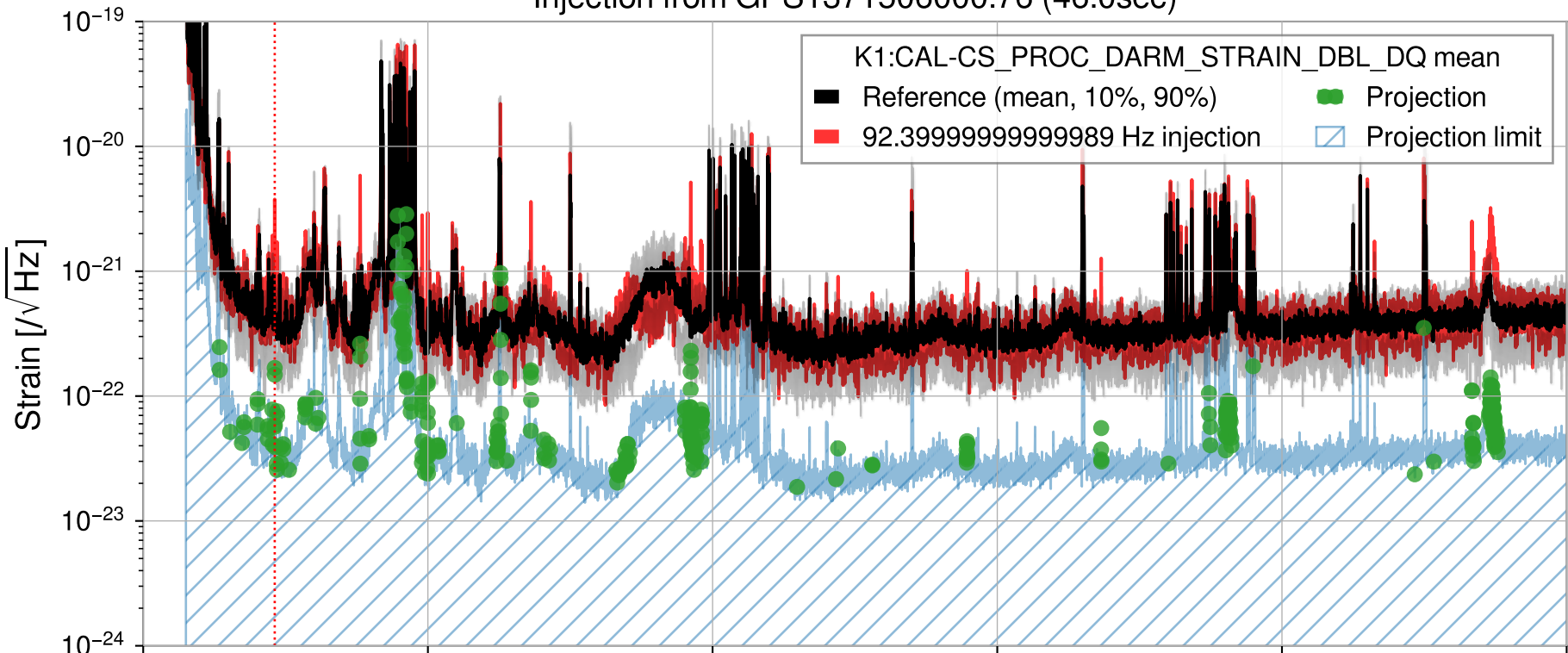
Injection from GPS1371506000.76 (46.0sec)
