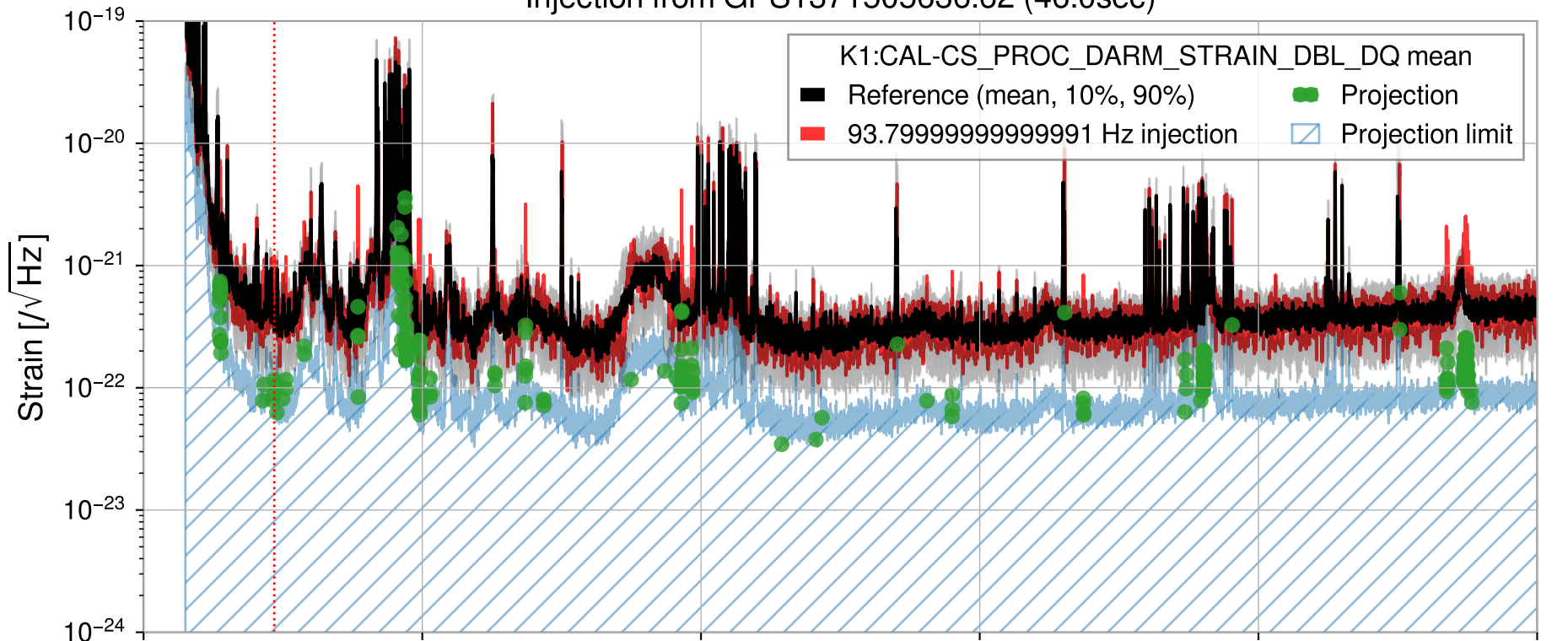
Injection from GPS1371505636.62 (46.0sec)
