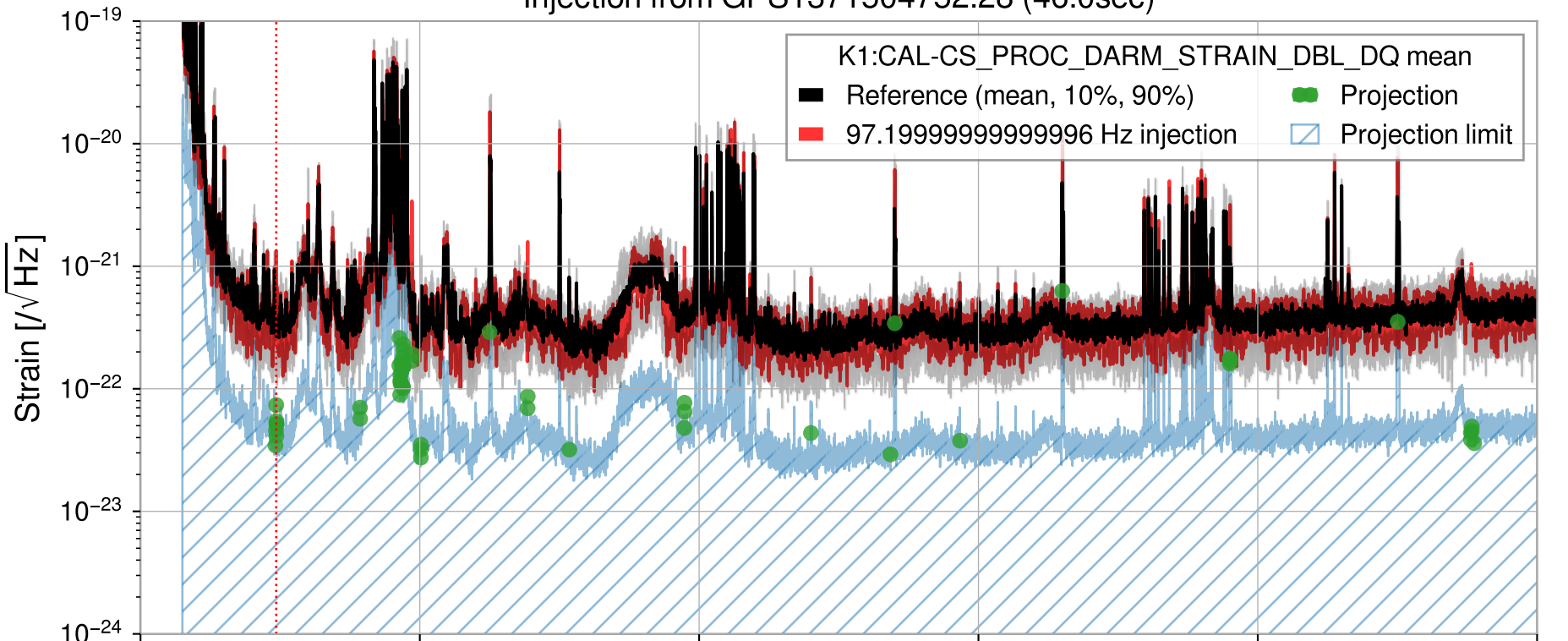
Injection from GPS1371504752.28 (46.0sec)
