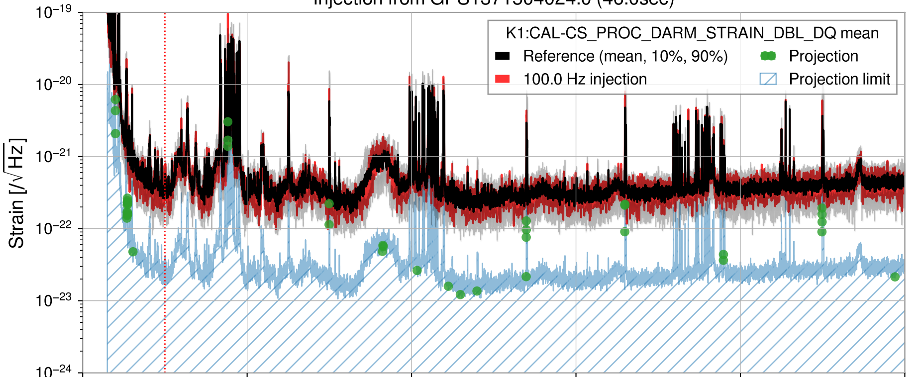
Injection from GPS1371504024.0 (46.0sec)
