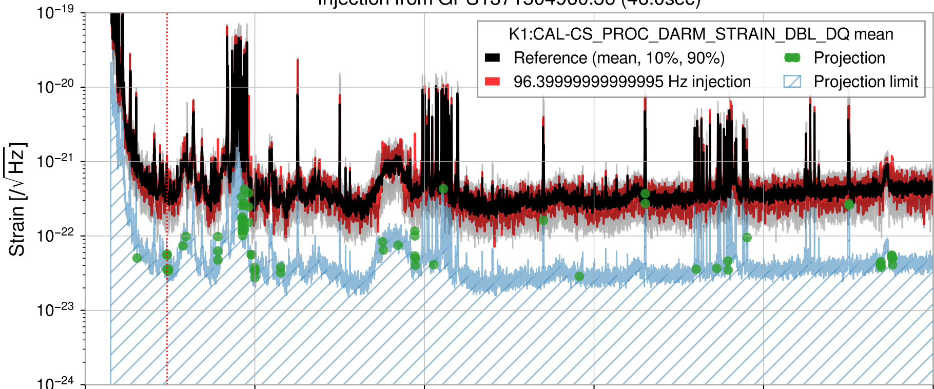
Injection from GPS1371504960.36 (46.0sec)
