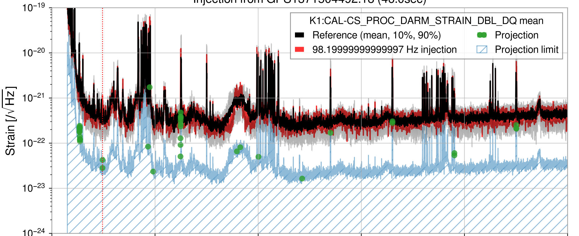
Injection from GPS1371504492.18 (46.0sec)
