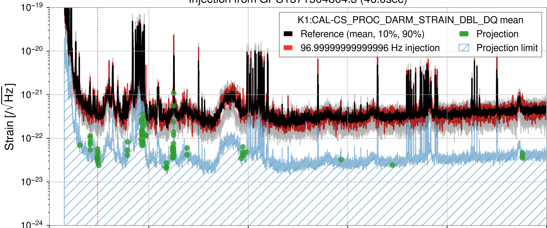
Injection from GPS1371504804.3 (46.0sec)
