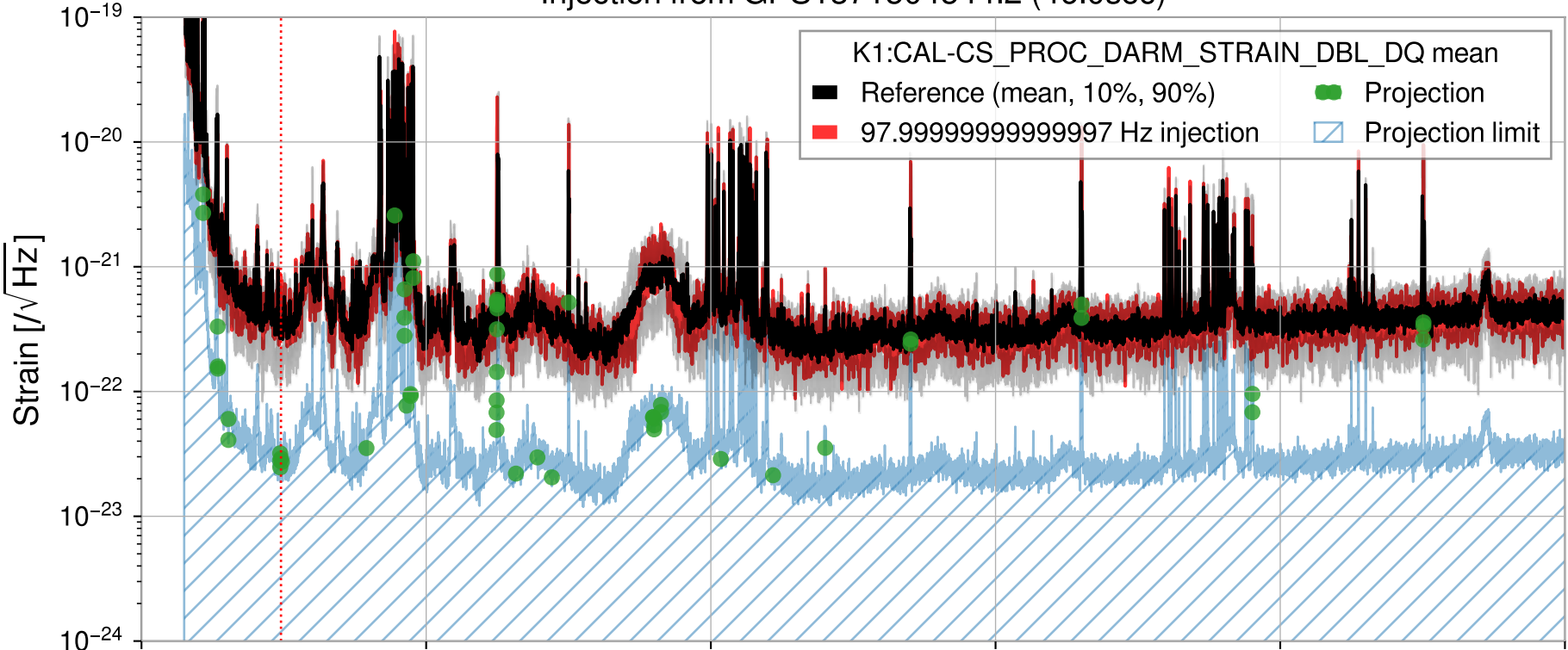
Injection from GPS1371504544.2 (46.0sec)
