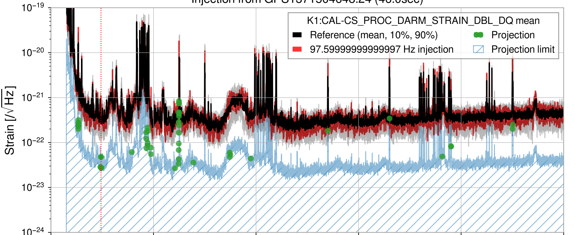
Injection from GPS1371504648.24 (46.0sec)
