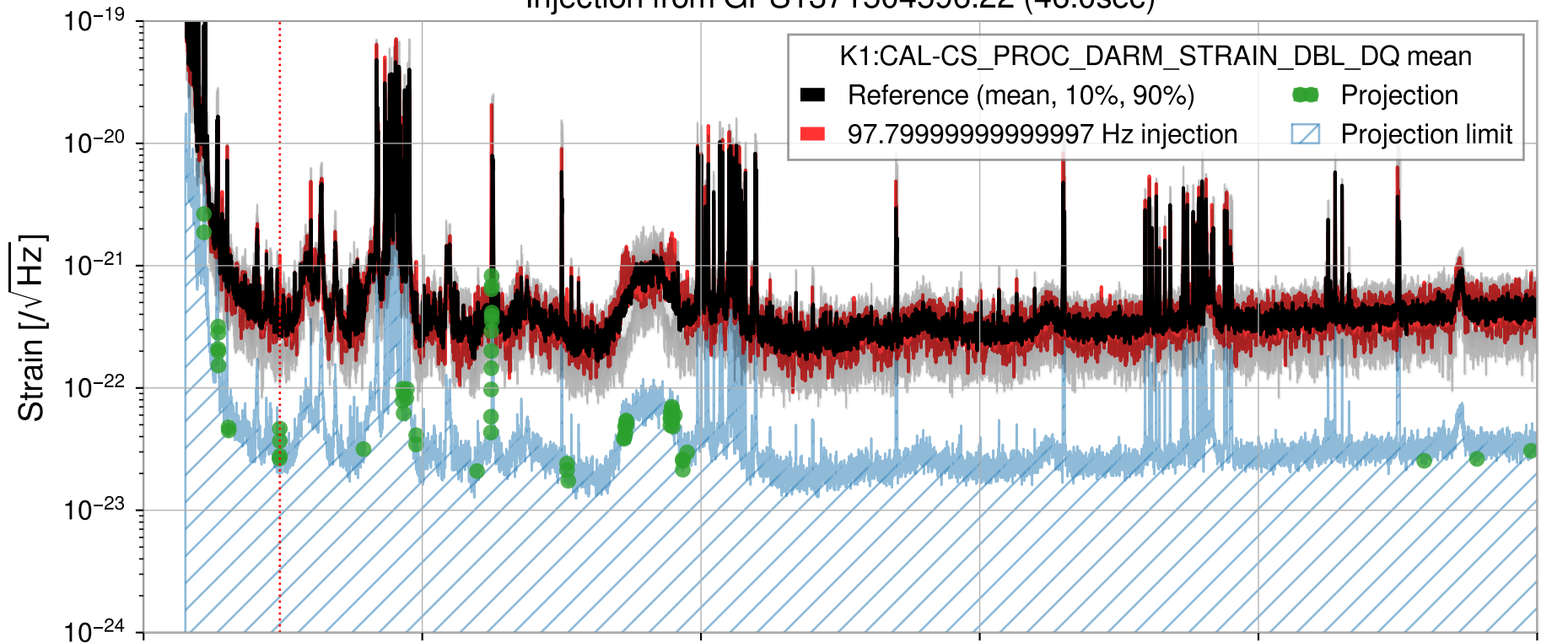
Injection from GPS1371504596.22 (46.0sec)
