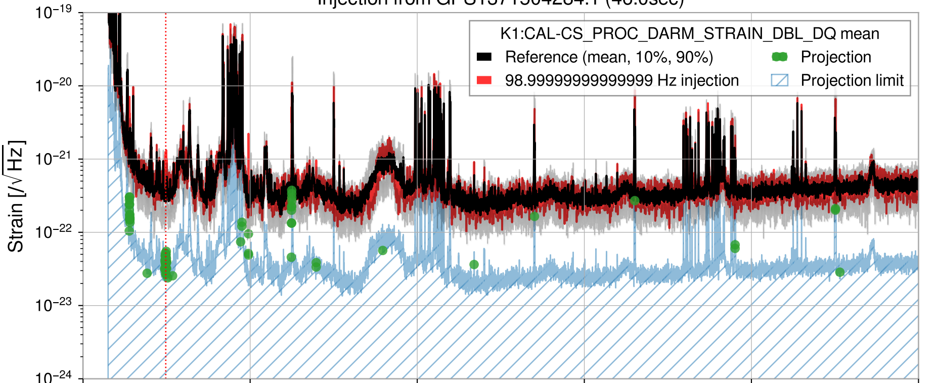
Injection from GPS1371504284.1 (46.0sec)
