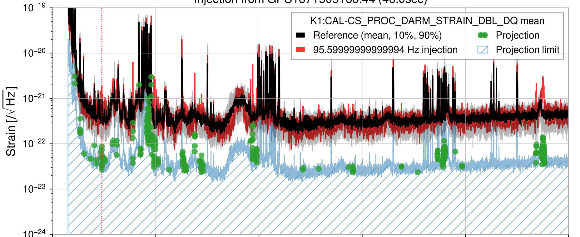
Injection from GPS1371505168.44 (46.0sec)
