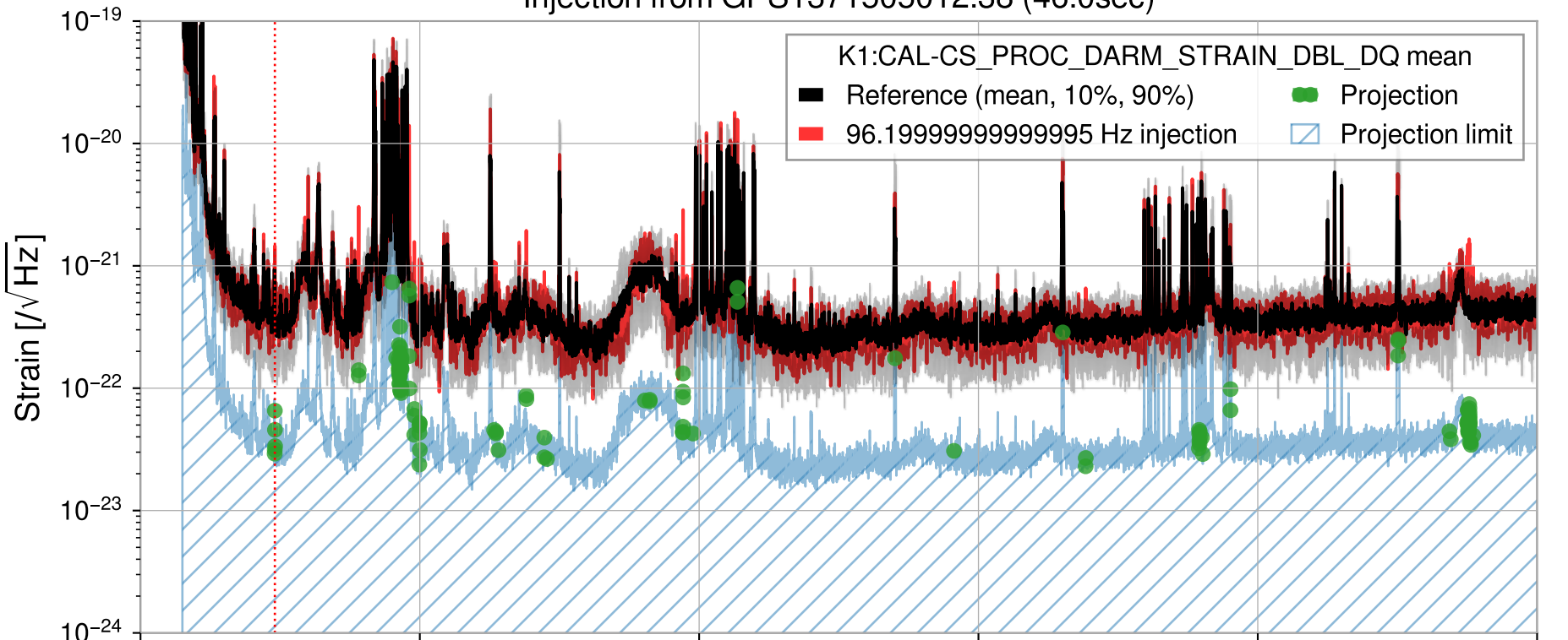
Injection from GPS1371505012.38 (46.0sec)
