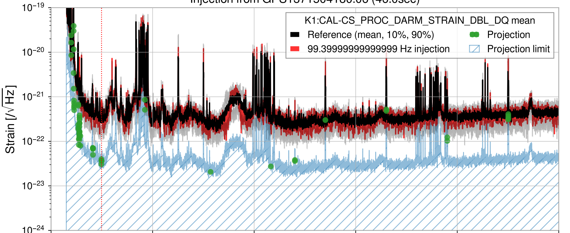
Injection from GPS1371504180.06 (46.0sec)
