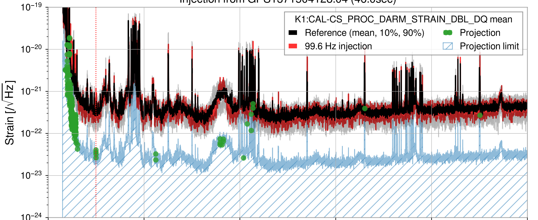
Injection from GPS1371504128.04 (46.0sec)
