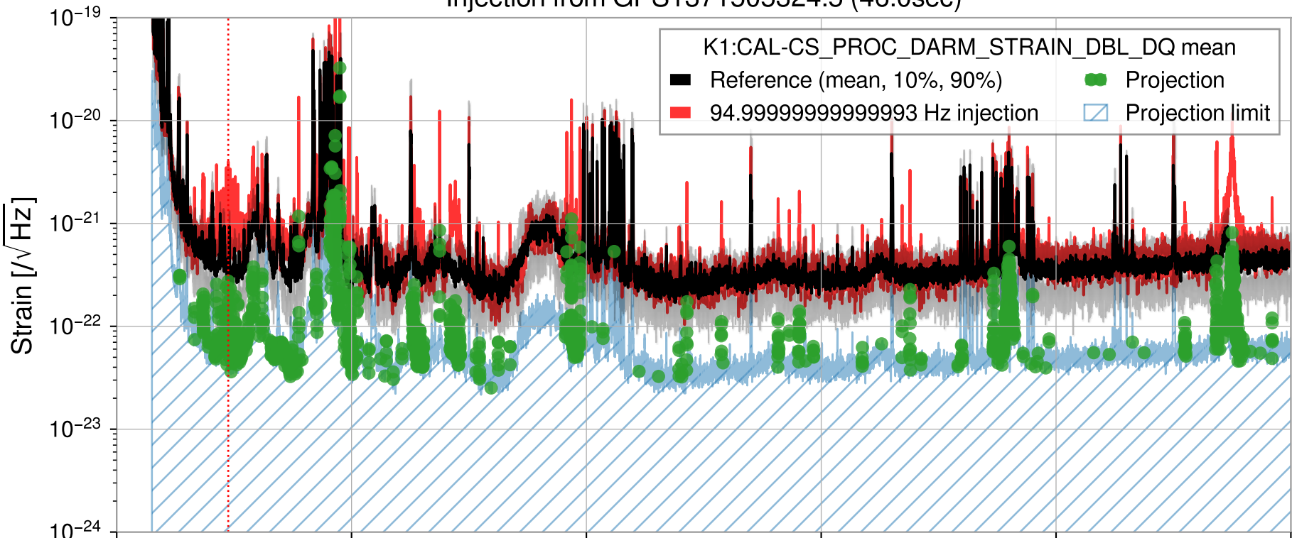
Injection from GPS1371505324.5 (46.0sec)
