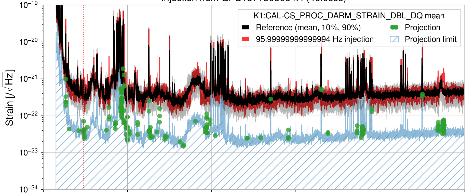
Injection from GPS1371505064.4 (46.0sec)
