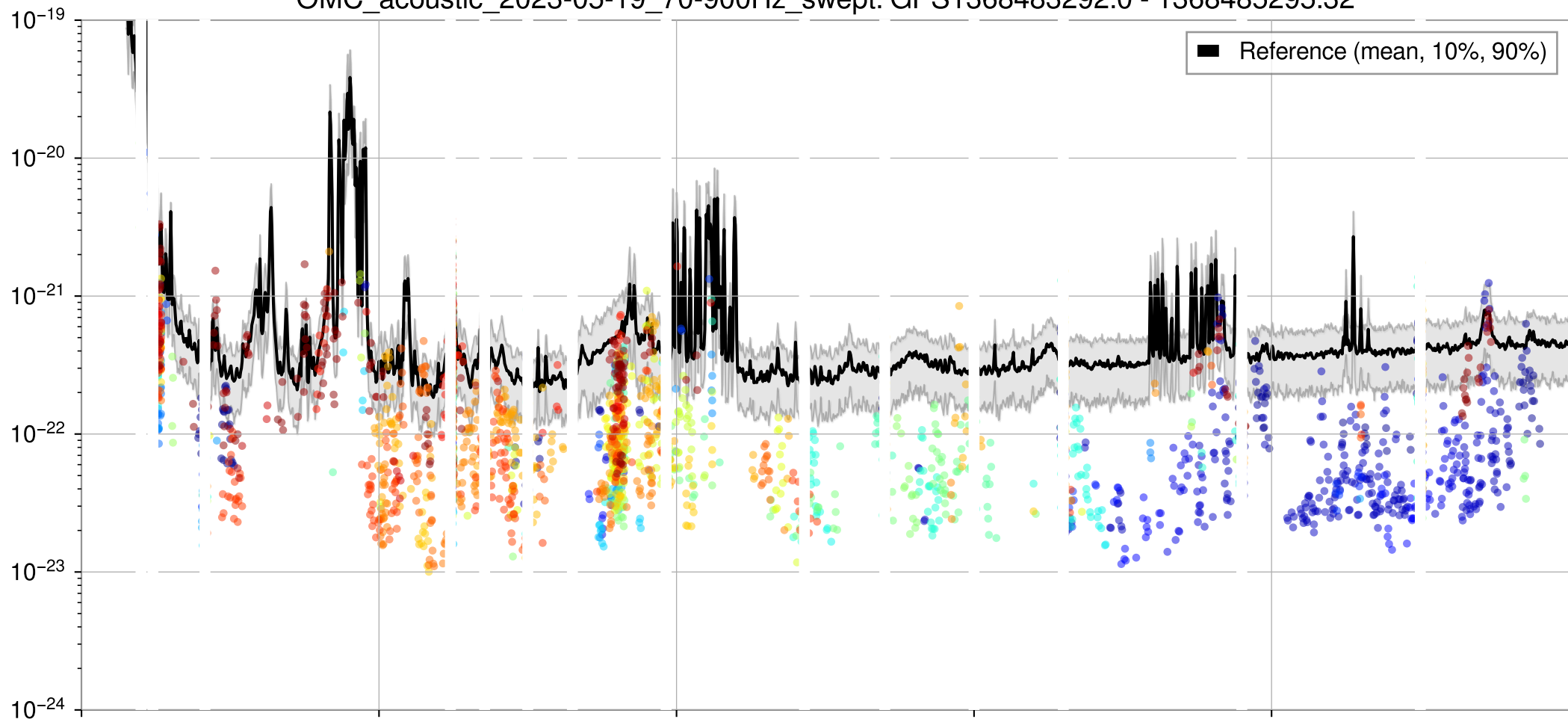
OMC_acoustic_2023-05-19_70-900Hz_swept: GPS1368483292.0 - 1368485295.32
