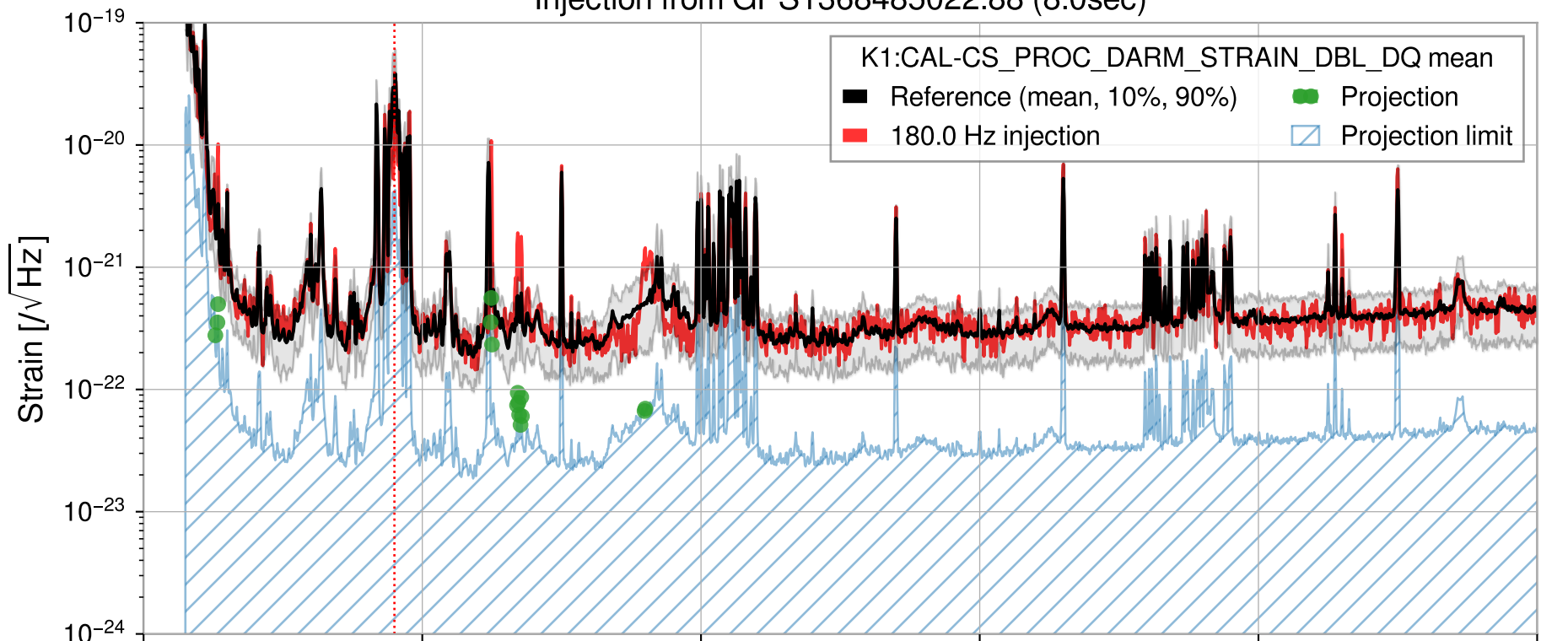
Injection from GPS1368485022.88 (8.0sec)
