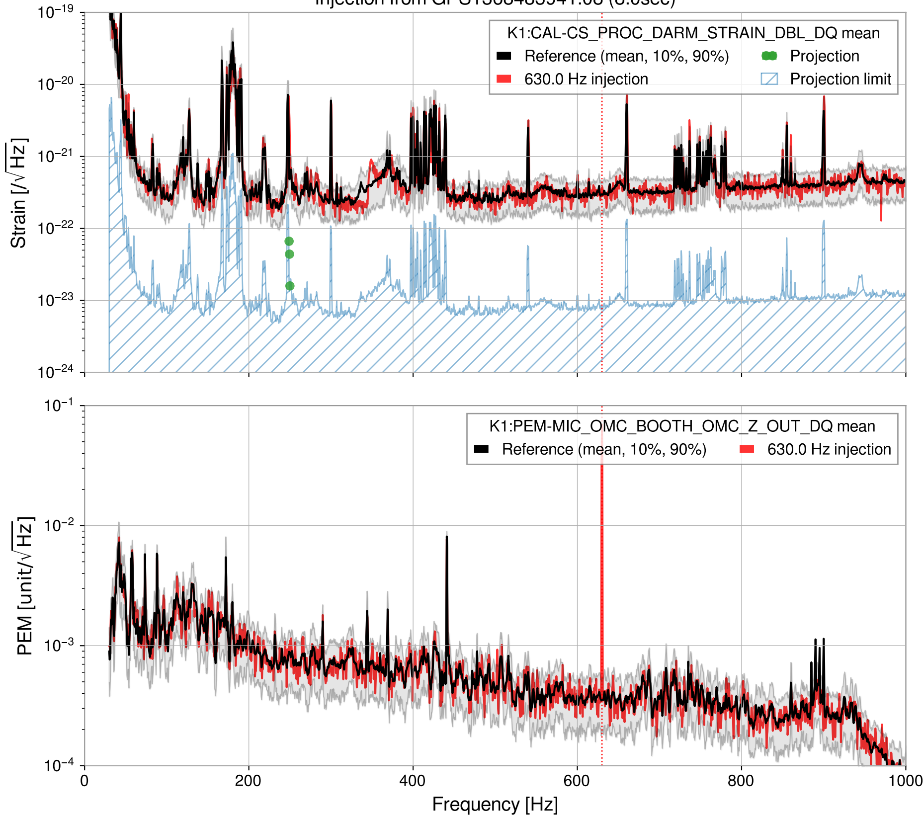
Injection from GPS1368483941.08 (8.0sec)
