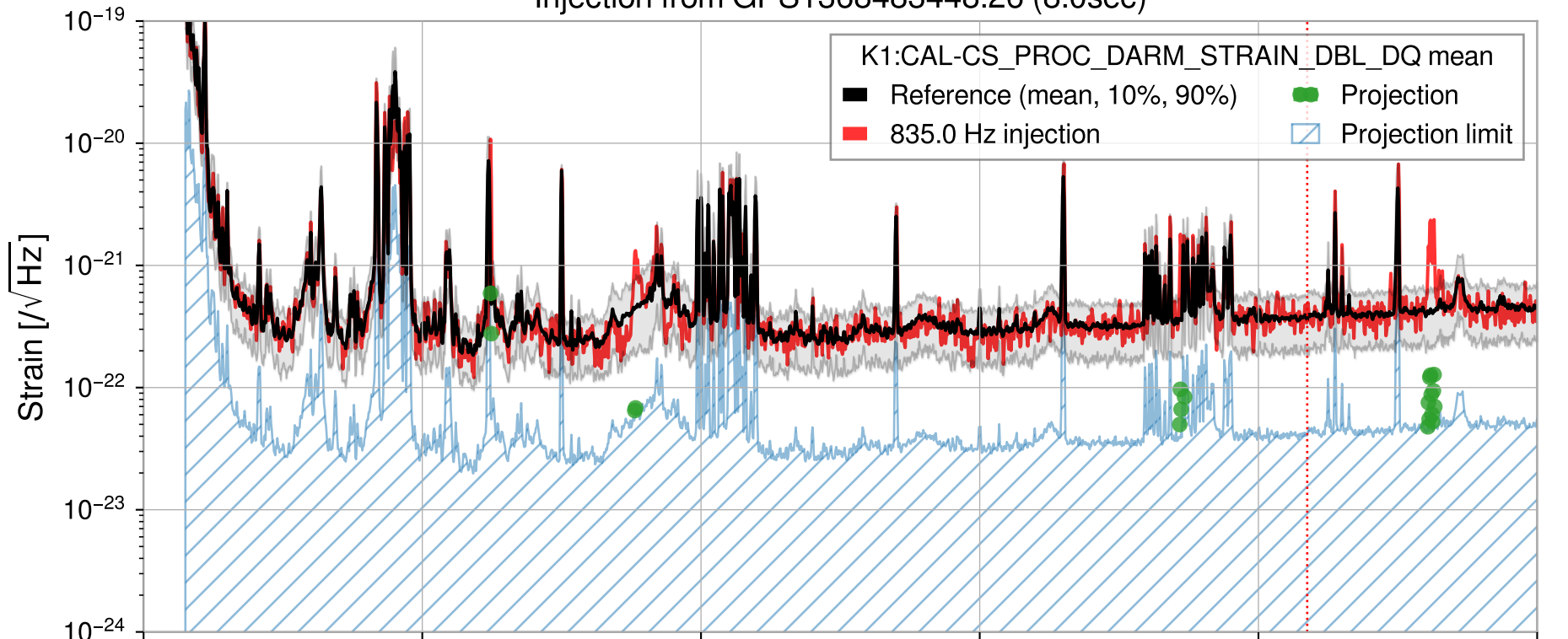
Injection from GPS1368483448.26 (8.0sec)
