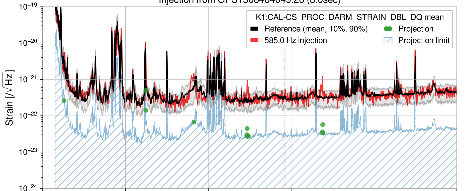
Injection from GPS1368484049.26 (8.0sec)
