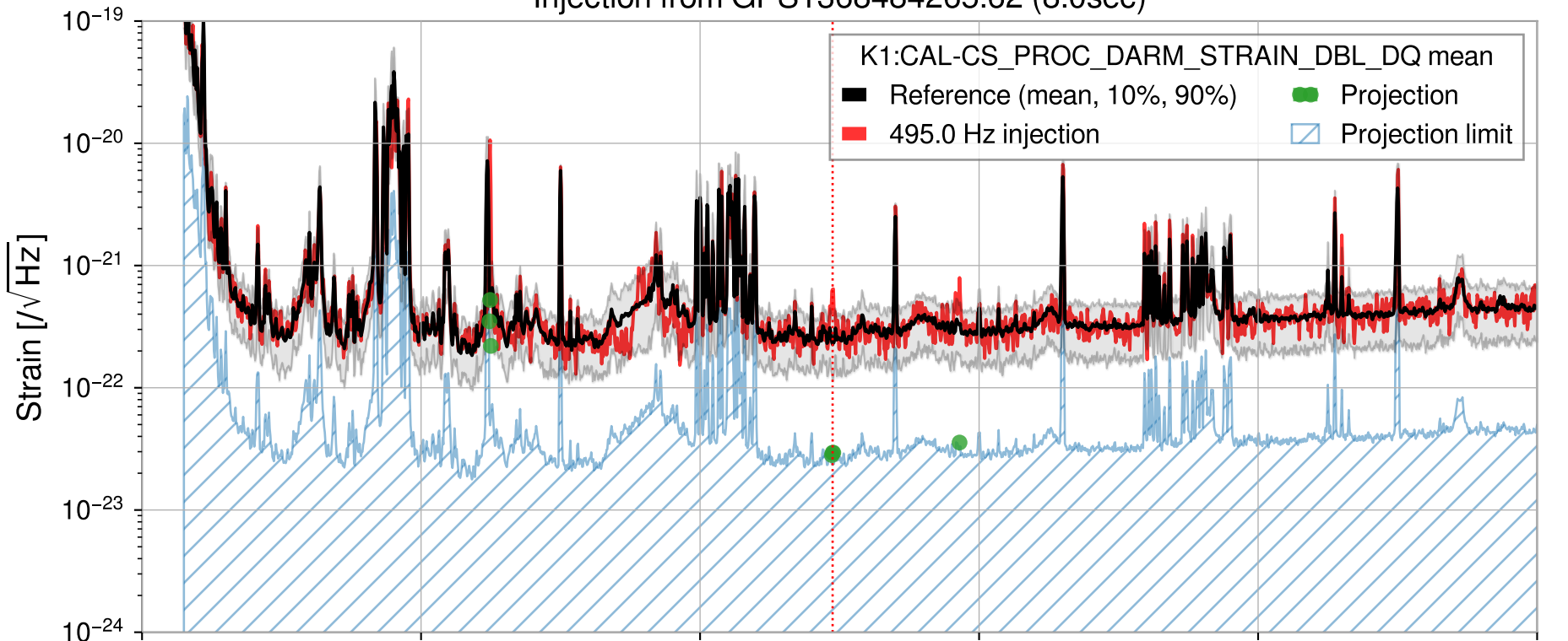
Injection from GPS1368484265.62 (8.0sec)
