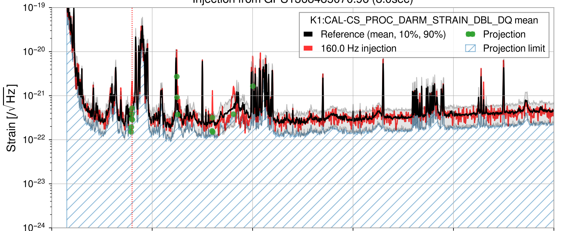
Injection from GPS1368485070.96 (8.0sec)
