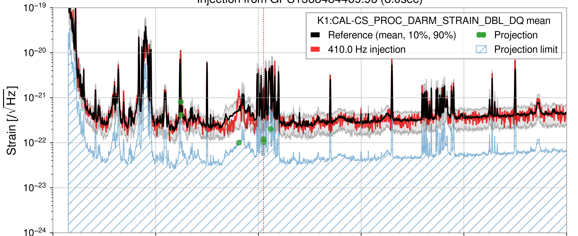
Injection from GPS1368484469.96 (8.0sec)
