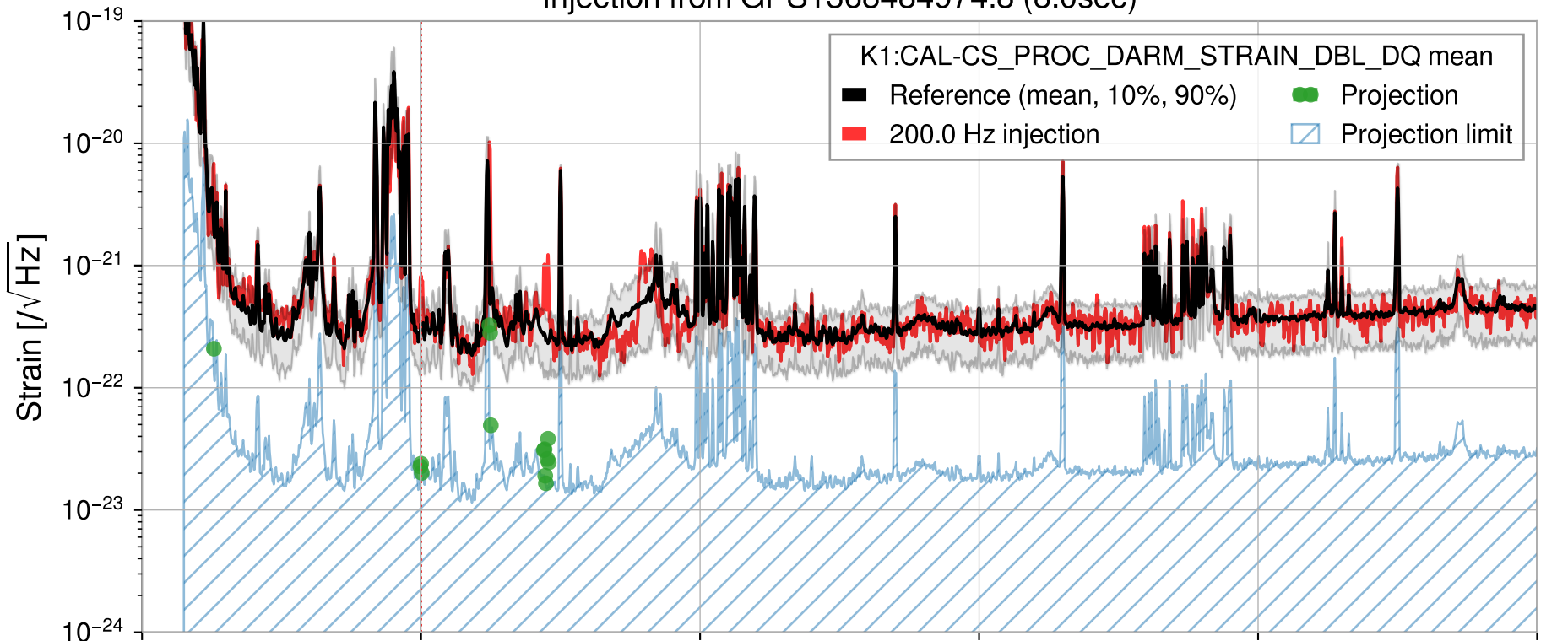
Injection from GPS1368484974.8 (8.0sec)
