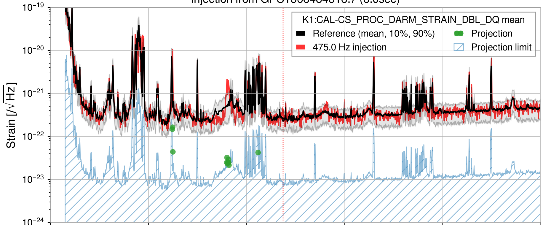
Injection from GPS1368484313.7 (8.0sec)
