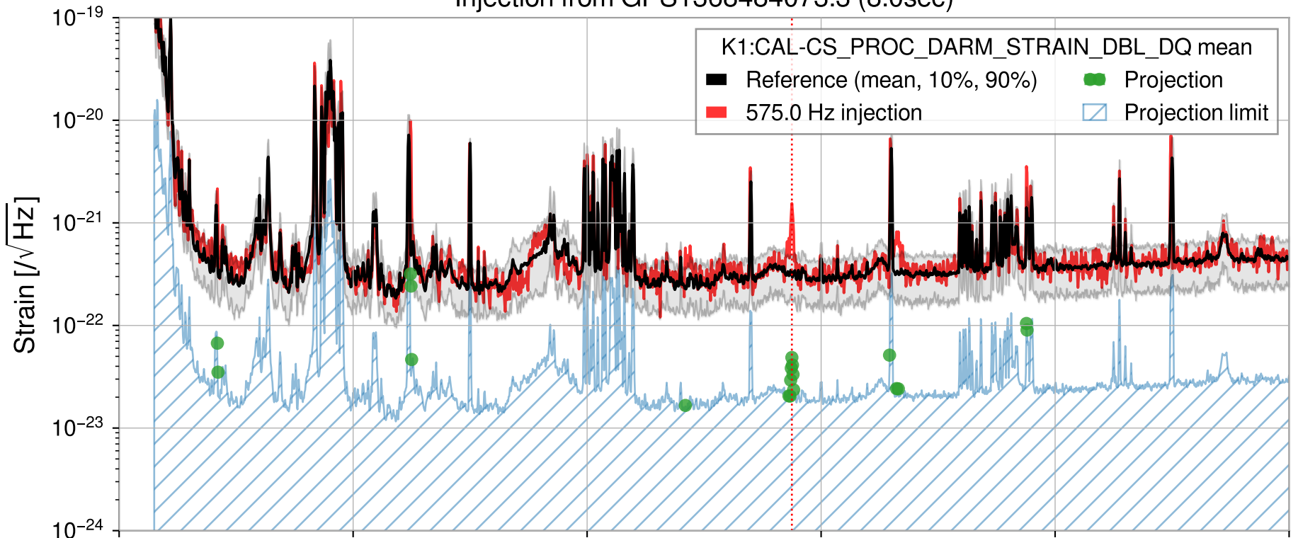
Injection from GPS1368484073.3 (8.0sec)
