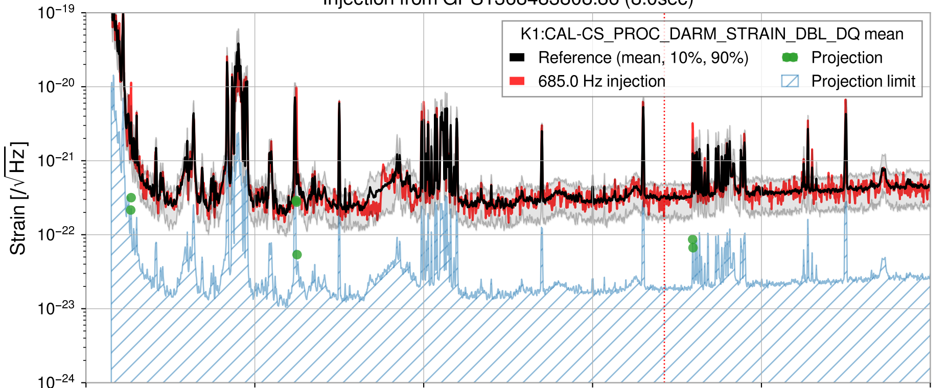
Injection from GPS1368483808.86 (8.0sec)
