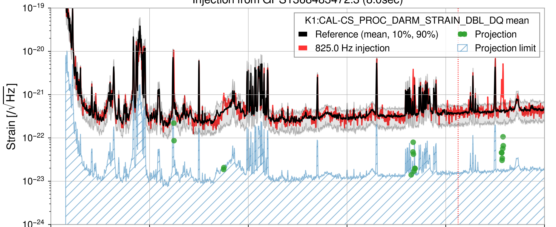
Injection from GPS1368483472.3 (8.0sec)
