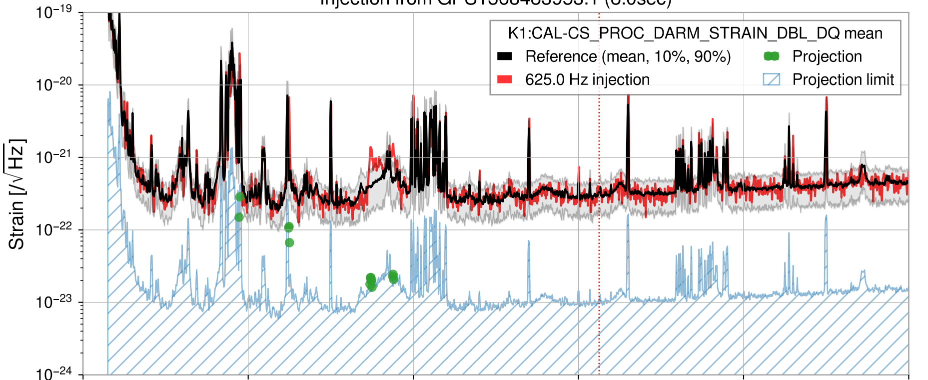
Injection from GPS1368483953.1 (8.0sec)
