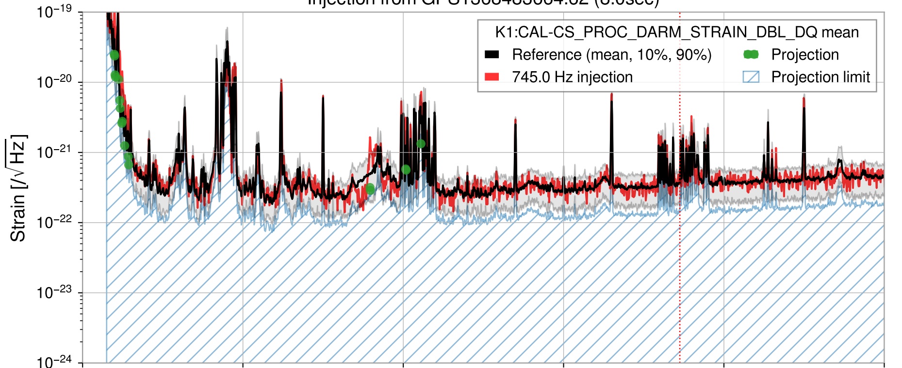
Injection from GPS1368483664.62 (8.0sec)
