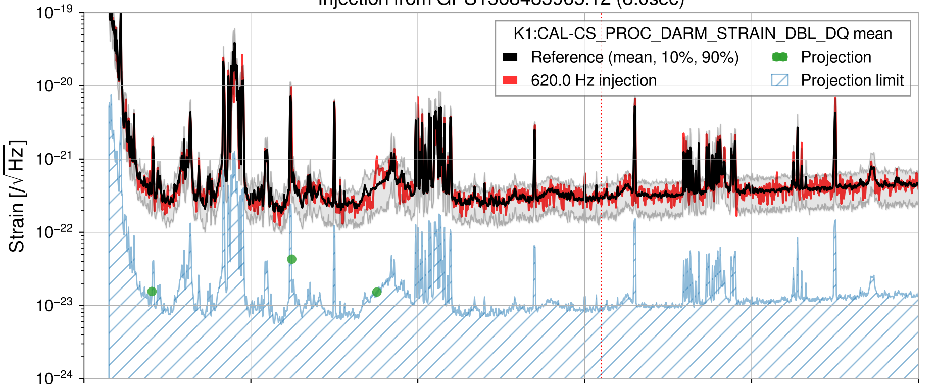
Injection from GPS1368483965.12 (8.0sec)
