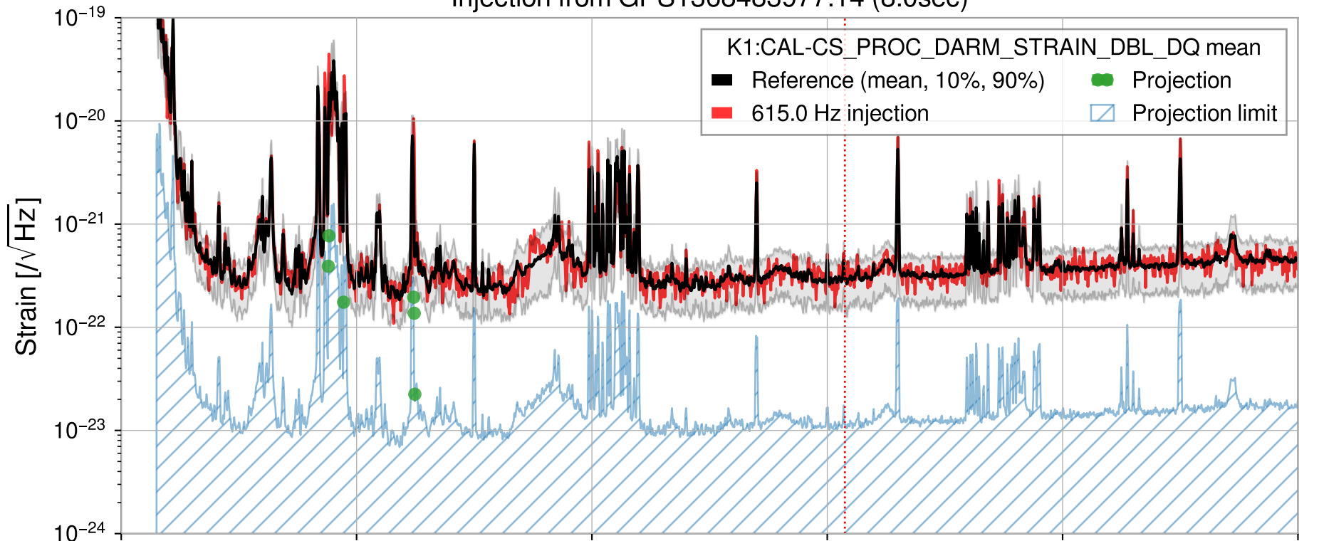
Injection from GPS1368483977.14 (8.0sec)
