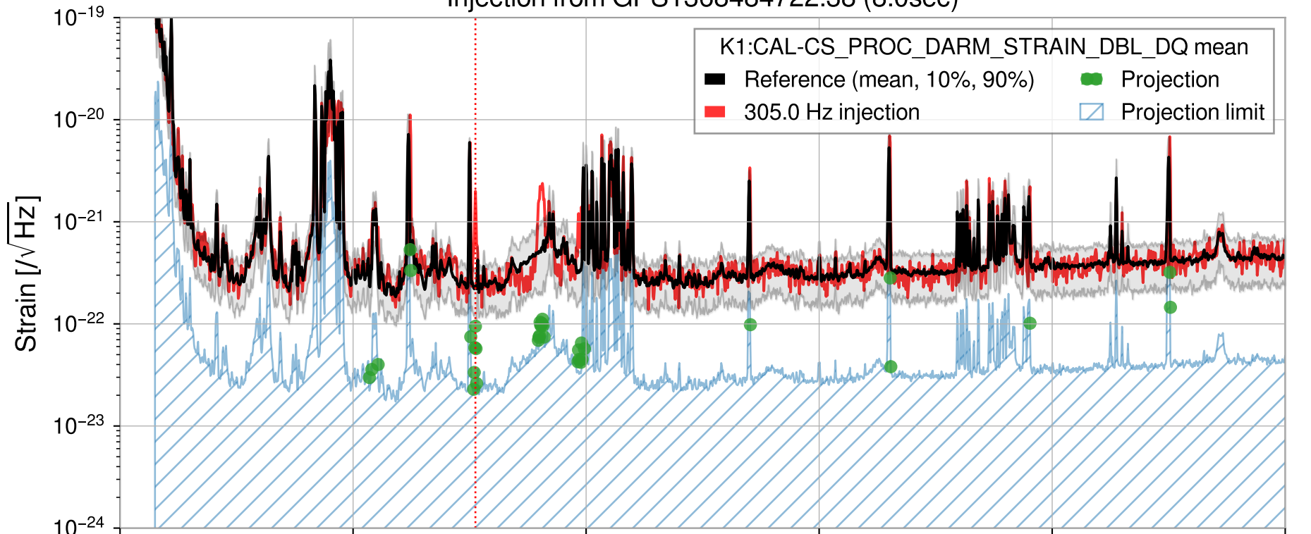
Injection from GPS1368484722.38 (8.0sec)
