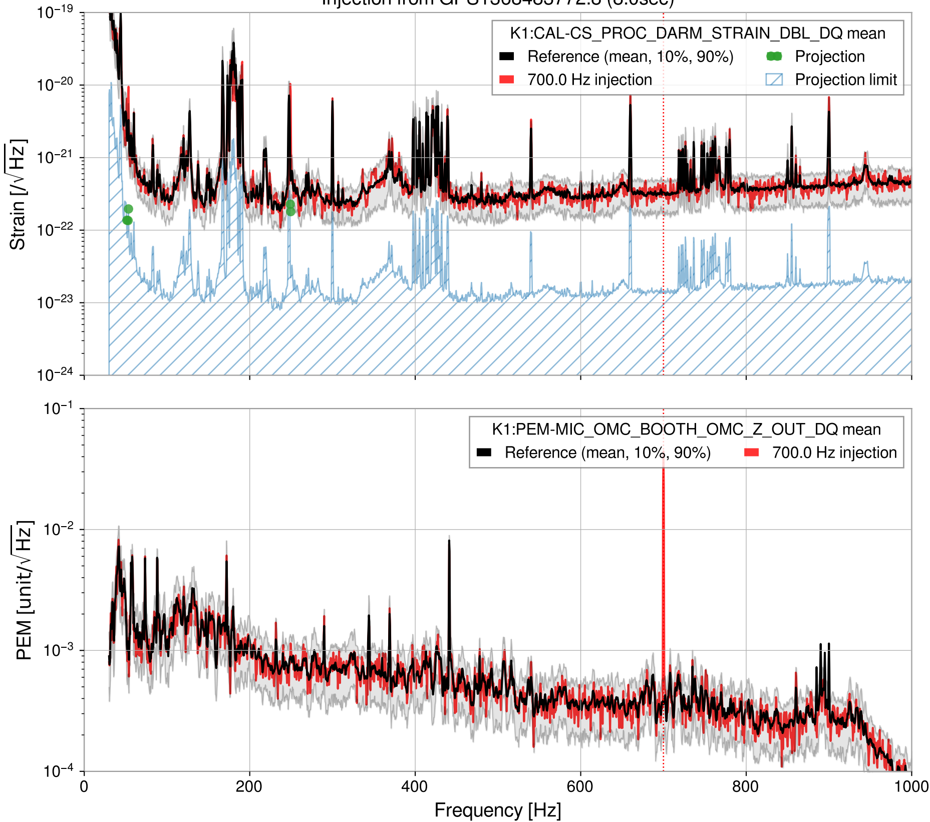
Injection from GPS1368483772.8 (8.0sec)
