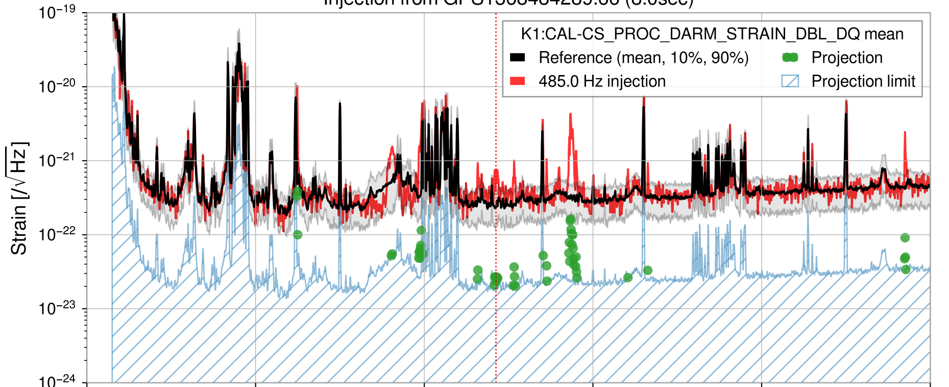
Injection from GPS1368484289.66 (8.0sec)
