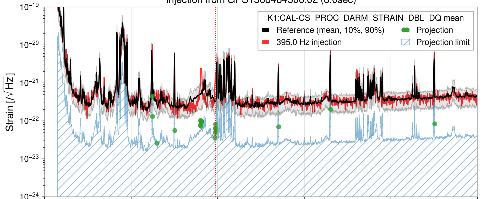
Injection from GPS1368484506.02 (8.0sec)
