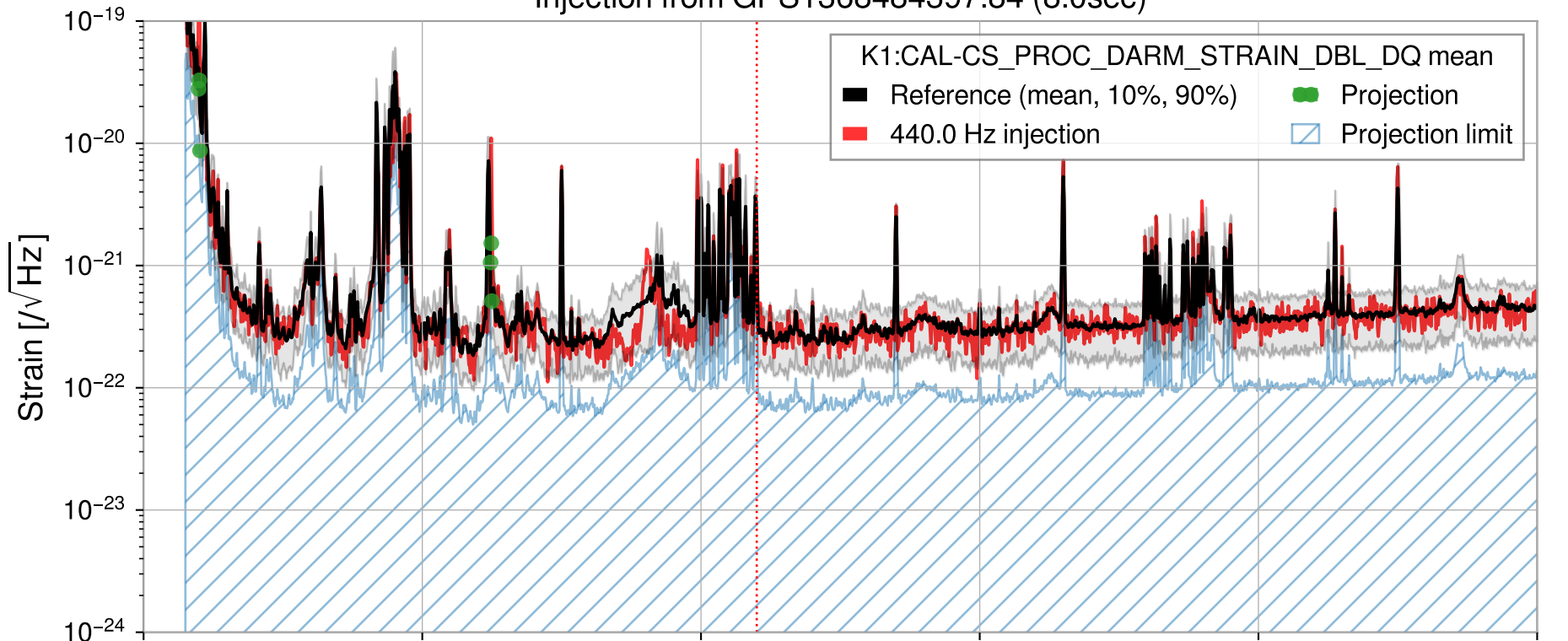
Injection from GPS1368484397.84 (8.0sec)
