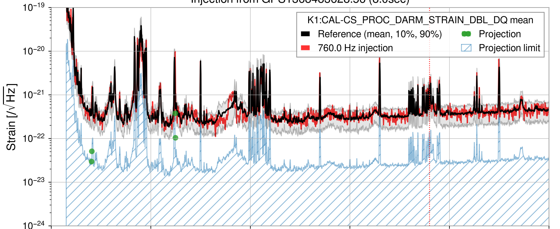
Injection from GPS1368483628.56 (8.0sec)
