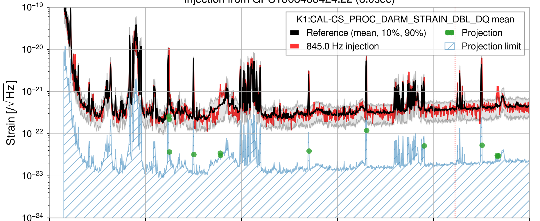
Injection from GPS1368483424.22 (8.0sec)
