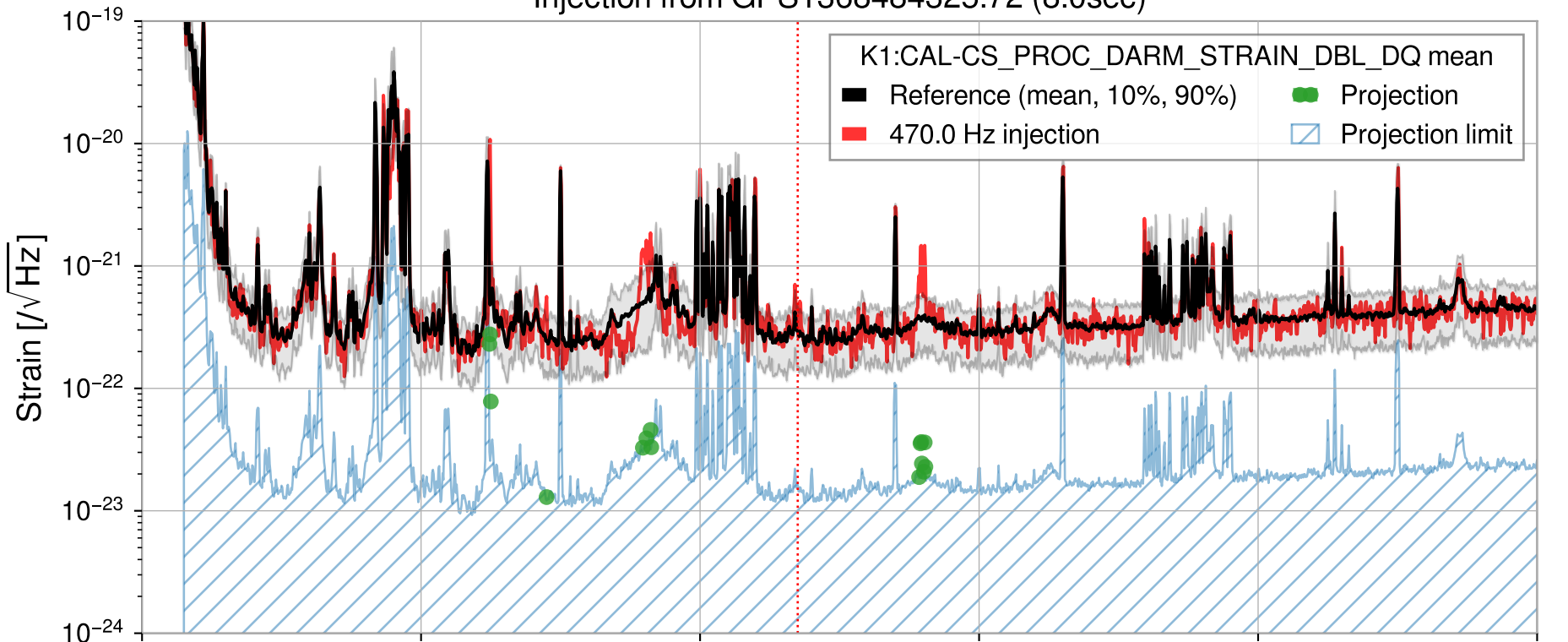
Injection from GPS1368484325.72 (8.0sec)
