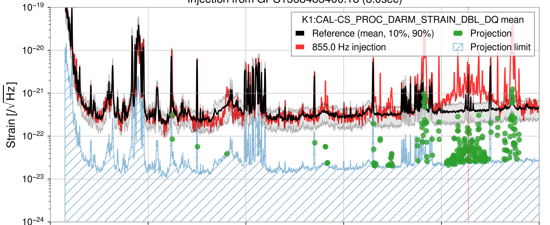
Injection from GPS1368483400.18 (8.0sec)
