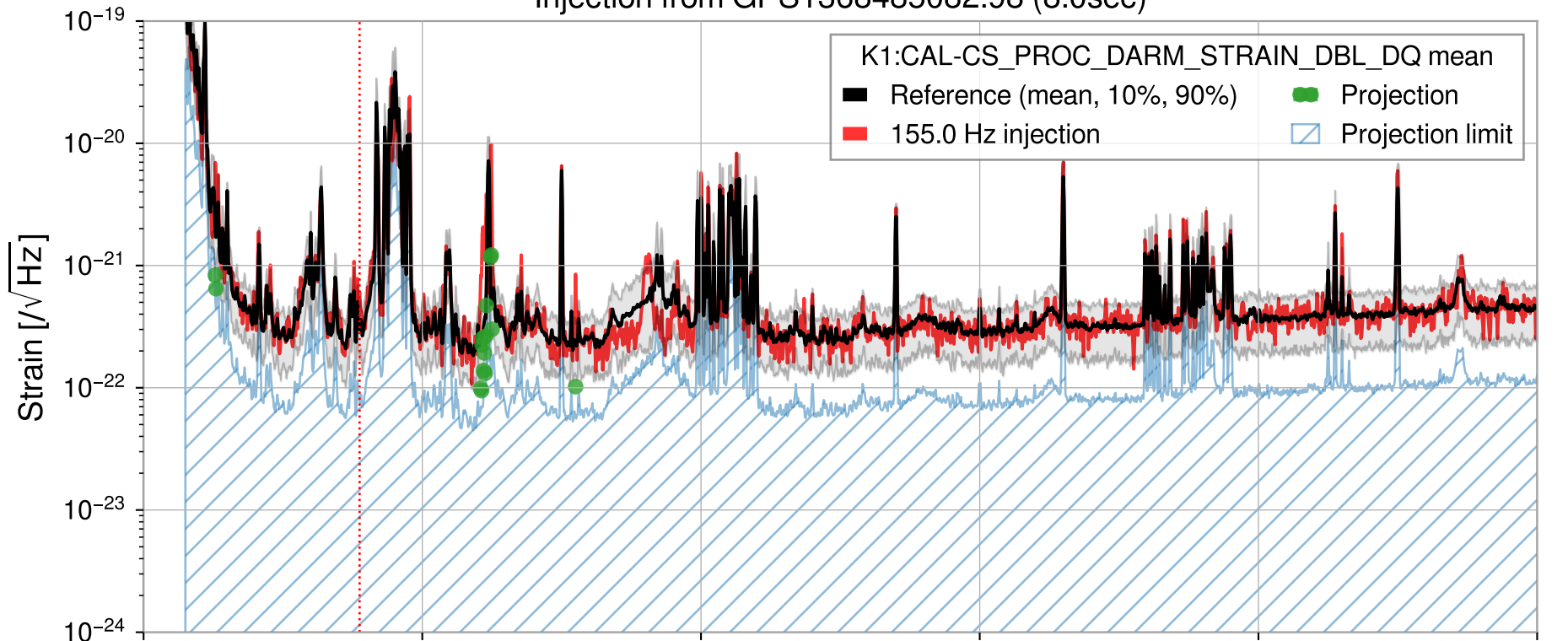
Injection from GPS1368485082.98 (8.0sec)
