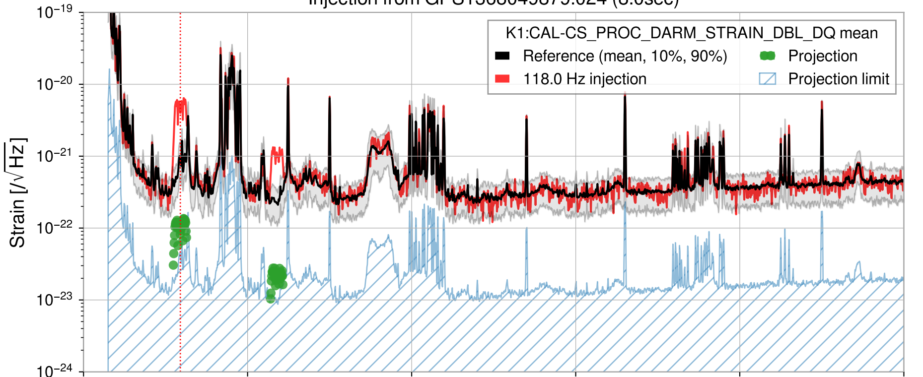
Injection from GPS1368049879.024 (8.0sec)
