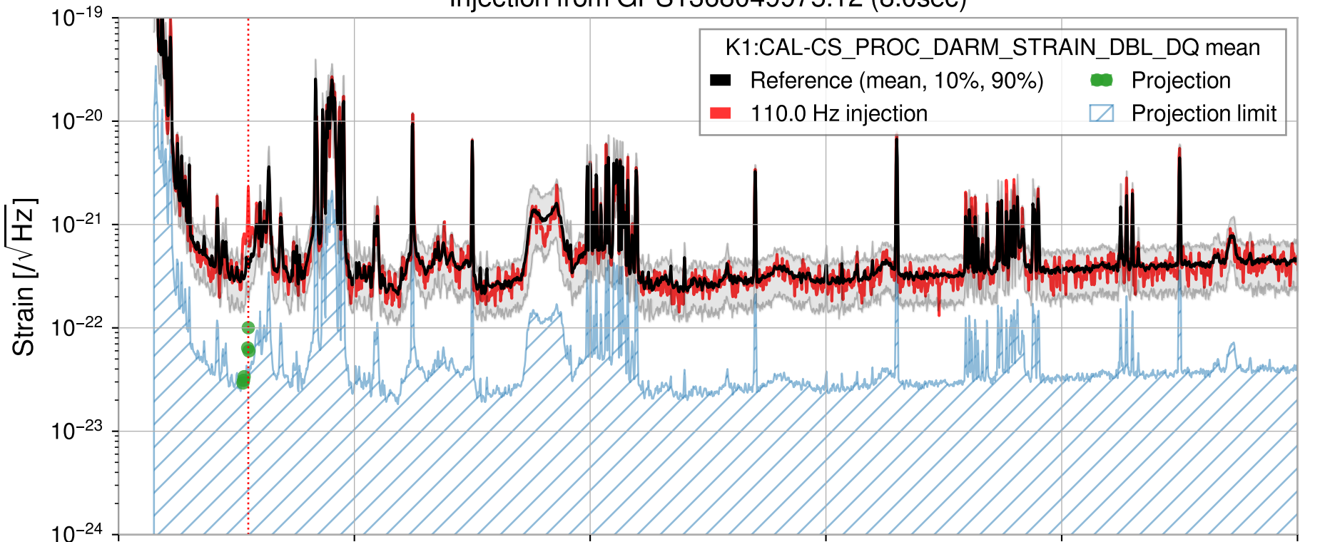
Injection from GPS1368049975.12 (8.0sec)
