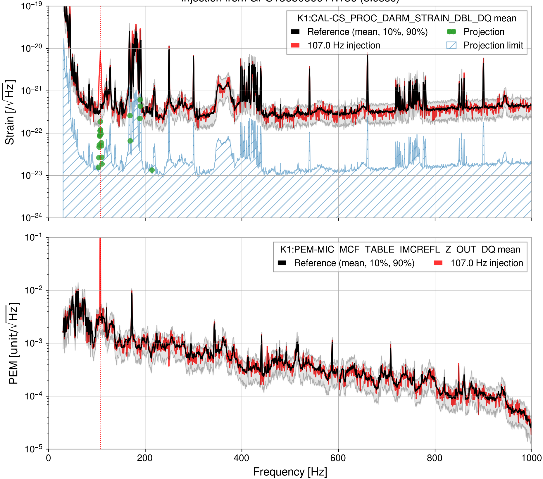
Injection from GPS1368050011.156 (8.0sec)
