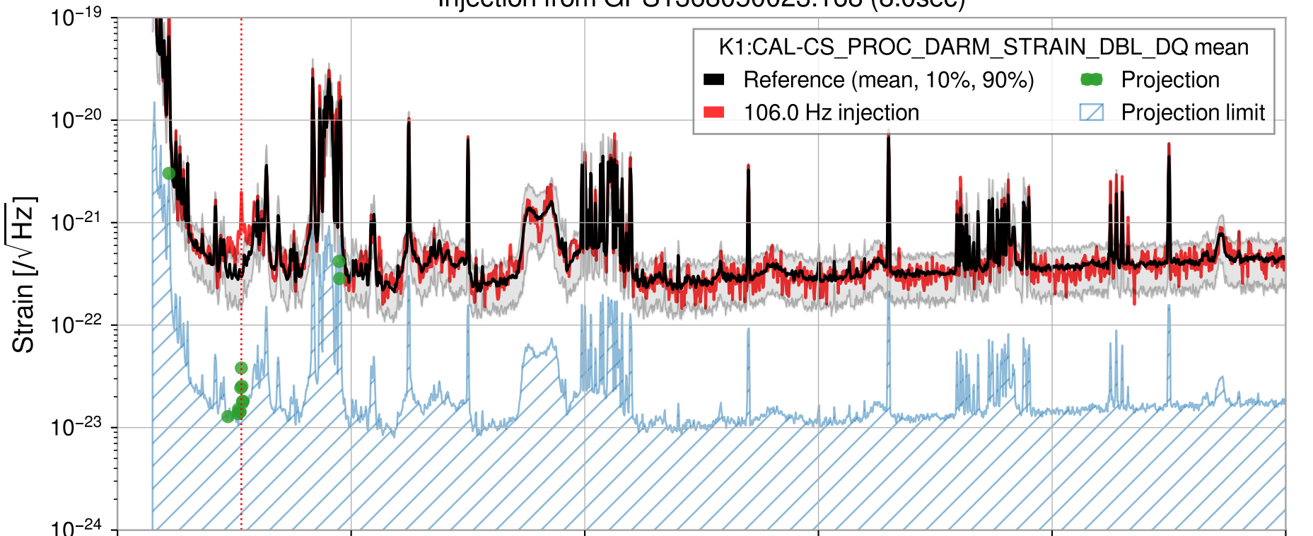
Injection from GPS1368050023.168 (8.0sec)
