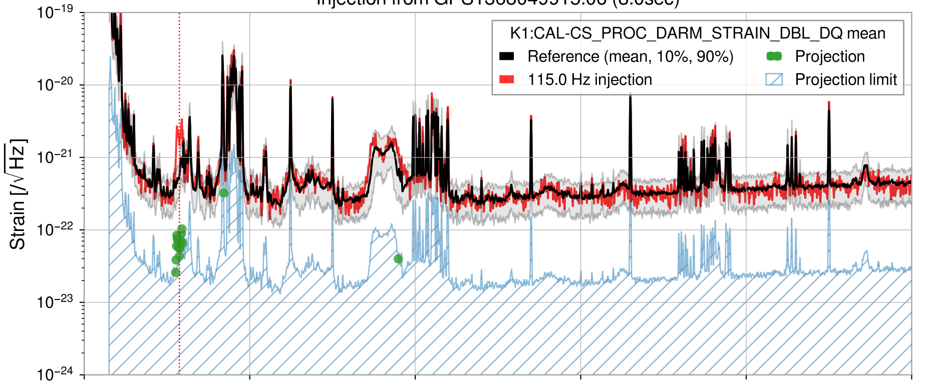
Injection from GPS1368049915.06 (8.0sec)
