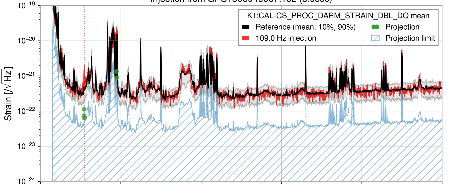
Injection from GPS1368049987.132 (8.0sec)
