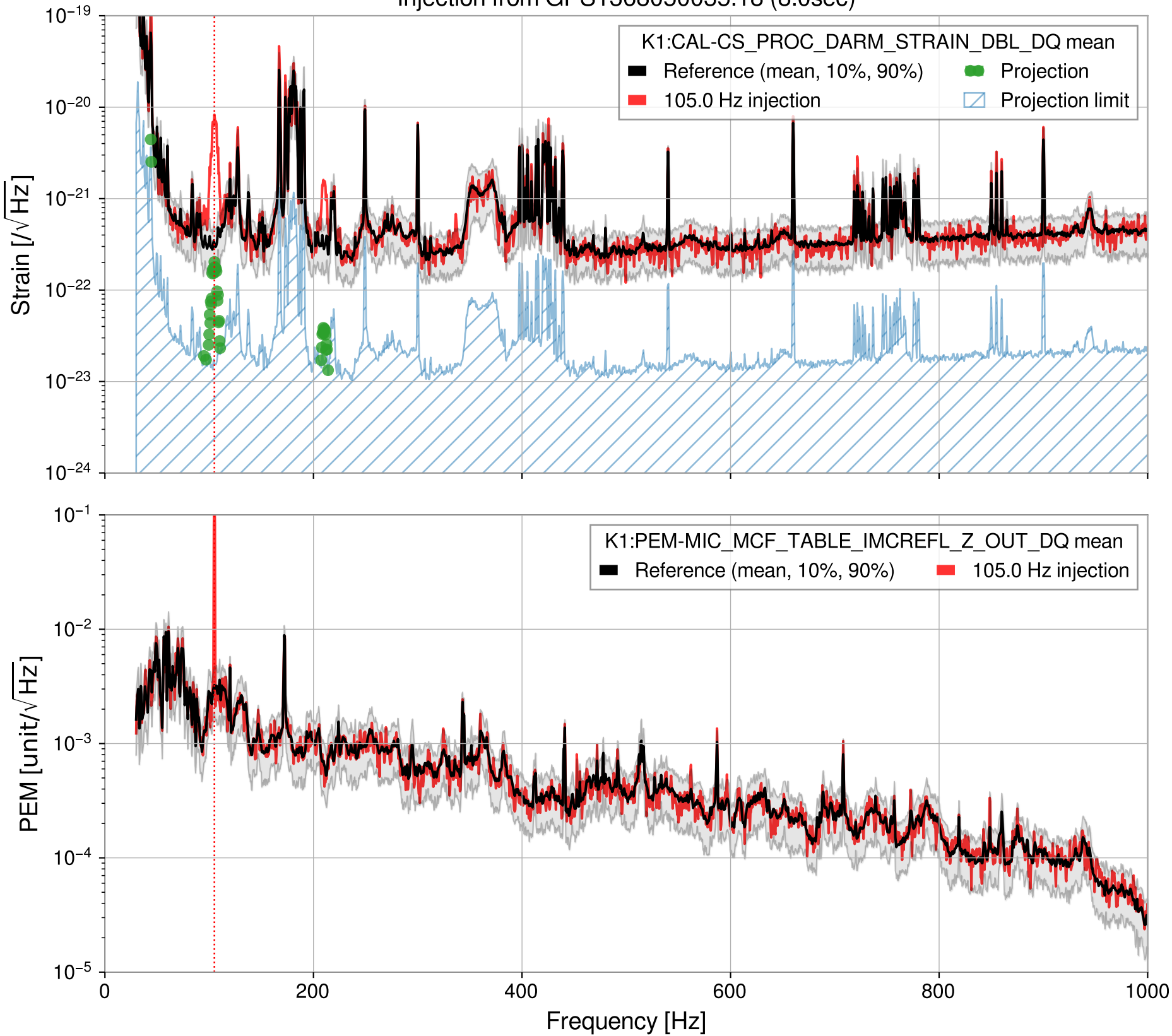
Injection from GPS1368050035.18 (8.0sec)
