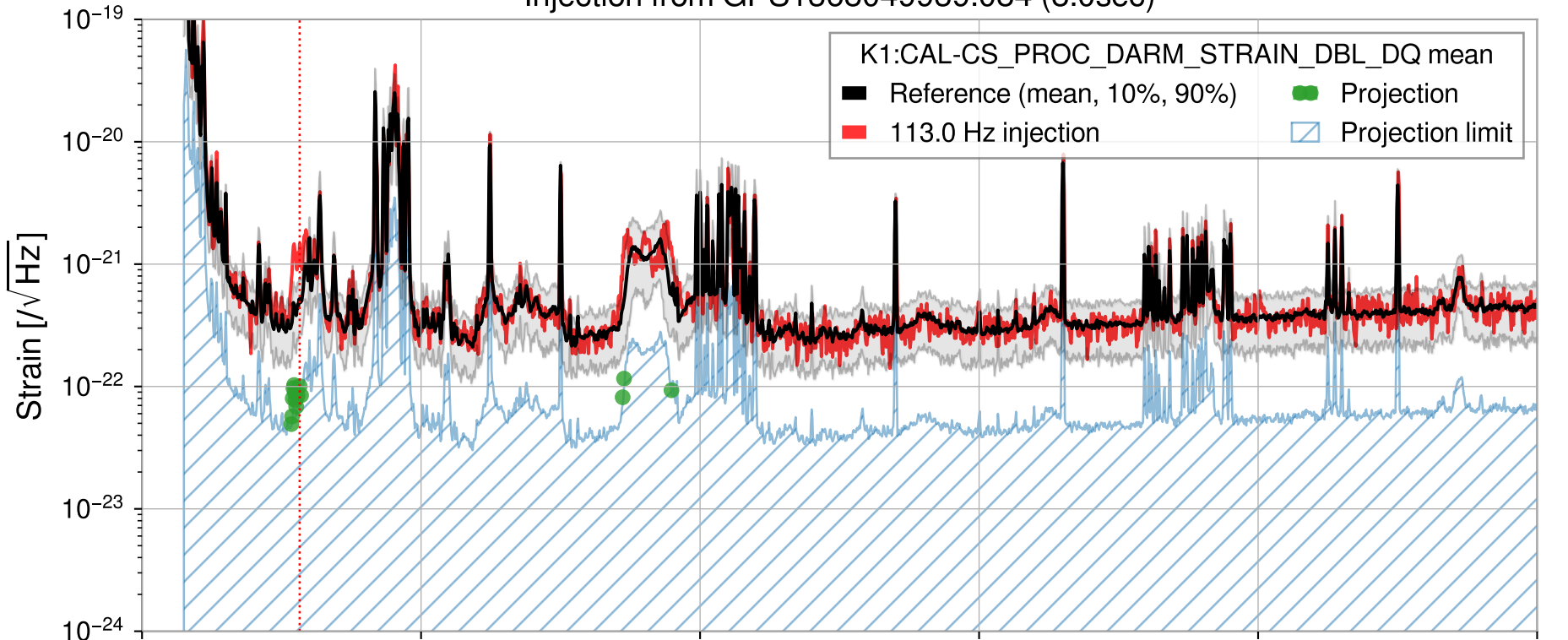
Injection from GPS1368049939.084 (8.0sec)
