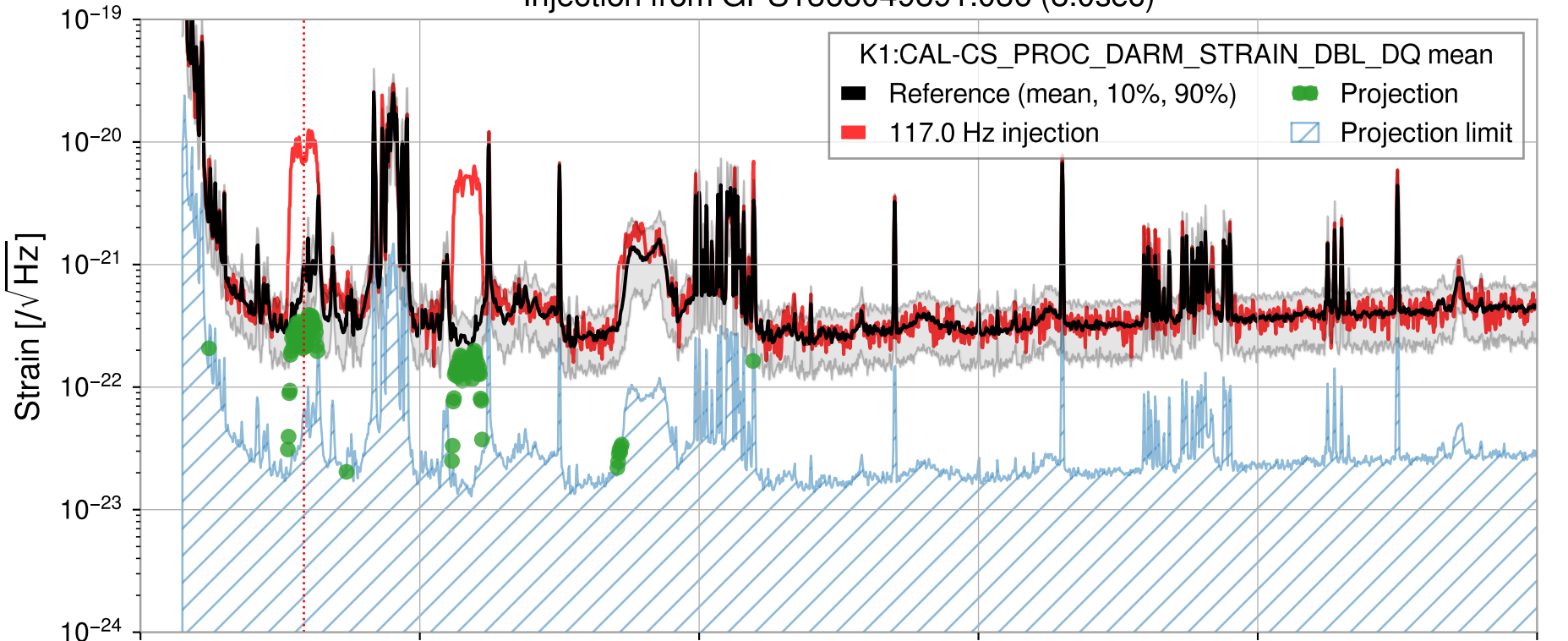
Injection from GPS1368049891.036 (8.0sec)
