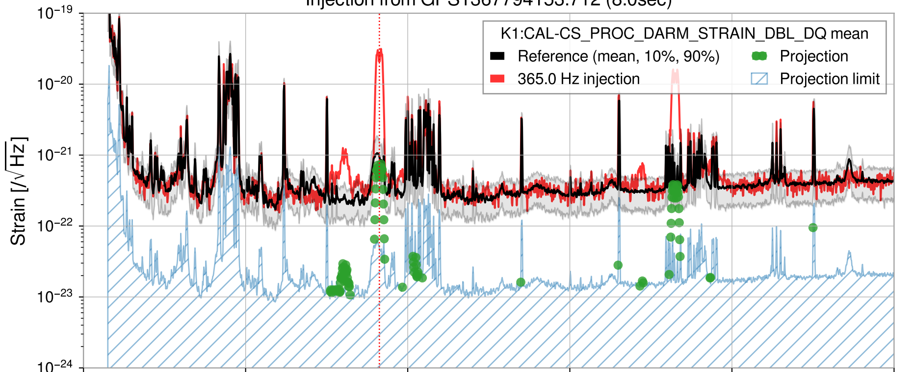
Injection from GPS1367794153.712 (8.0sec)
