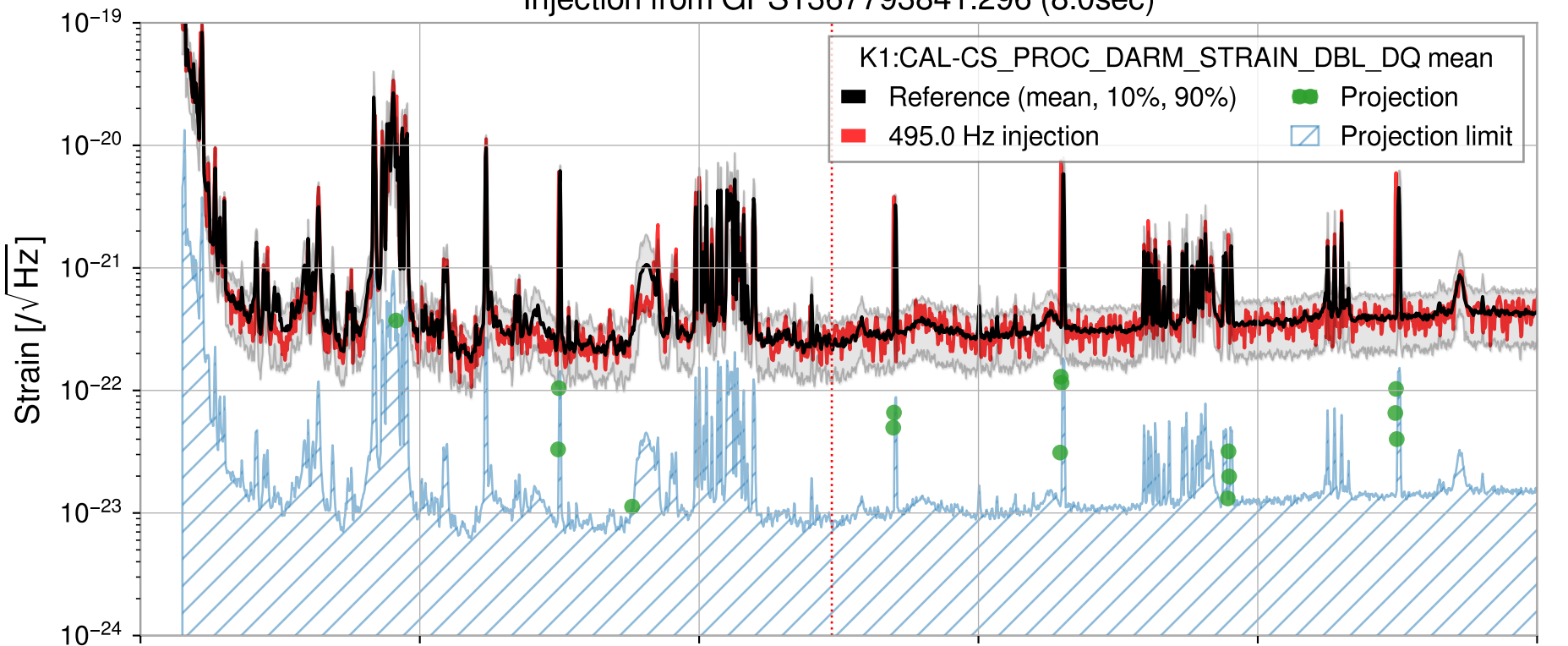
Injection from GPS1367793841.296 (8.0sec)
