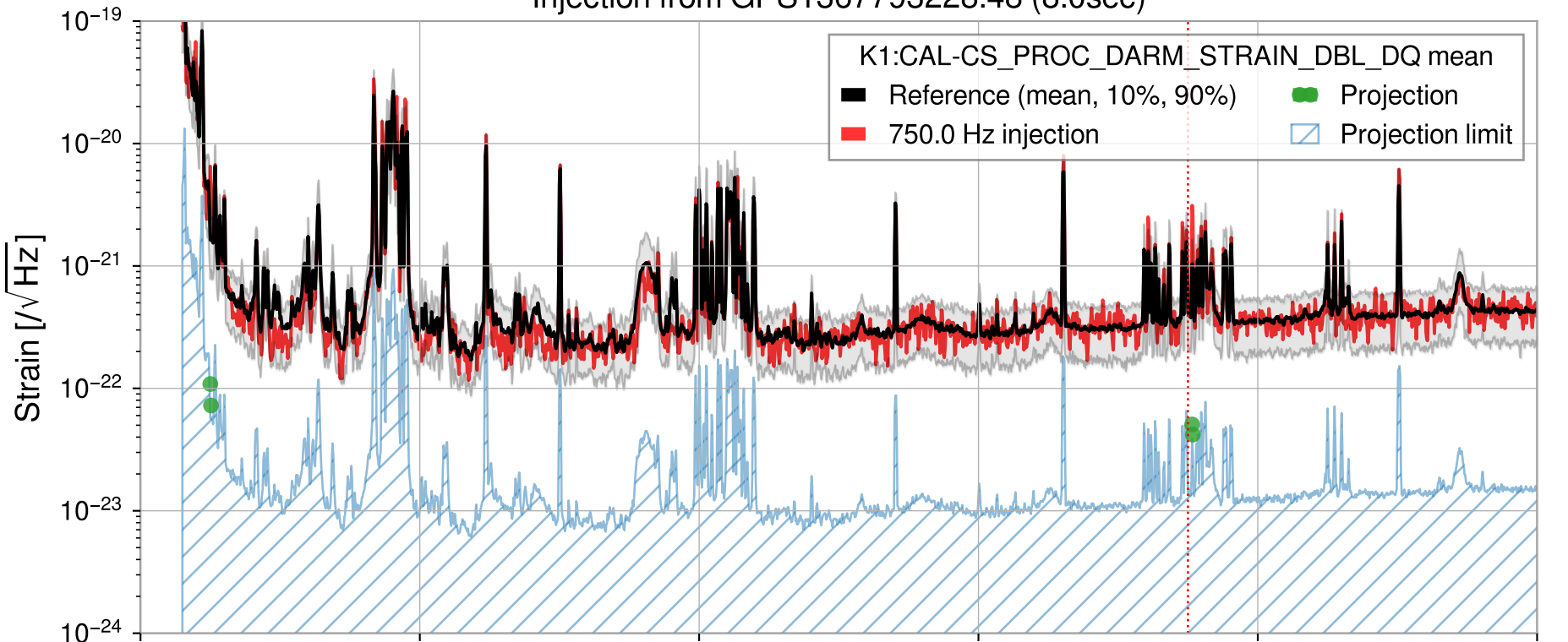
Injection from GPS1367793228.48 (8.0sec)
