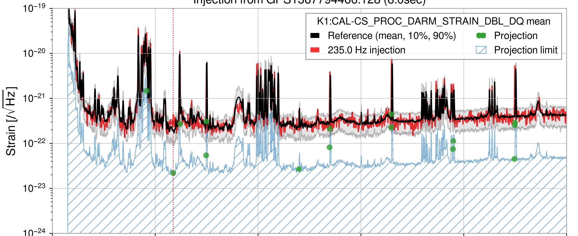
Injection from GPS1367794466.128 (8.0sec)
