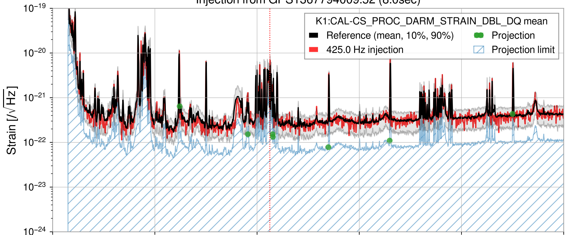
Injection from GPS1367794009.52 (8.0sec)
