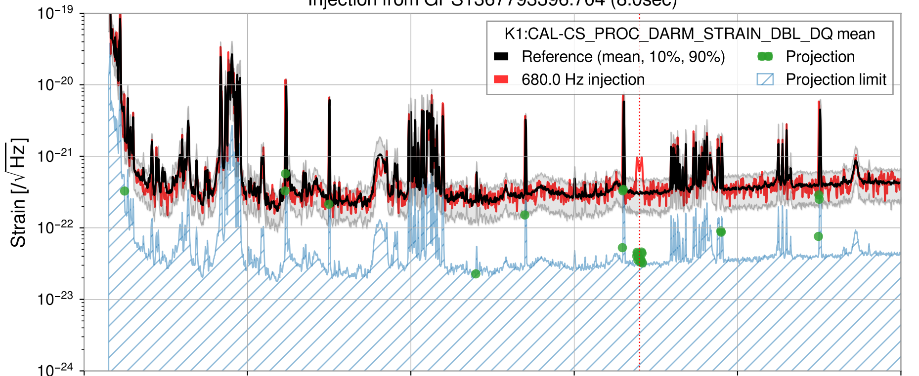
Injection from GPS1367793396.704 (8.0sec)
