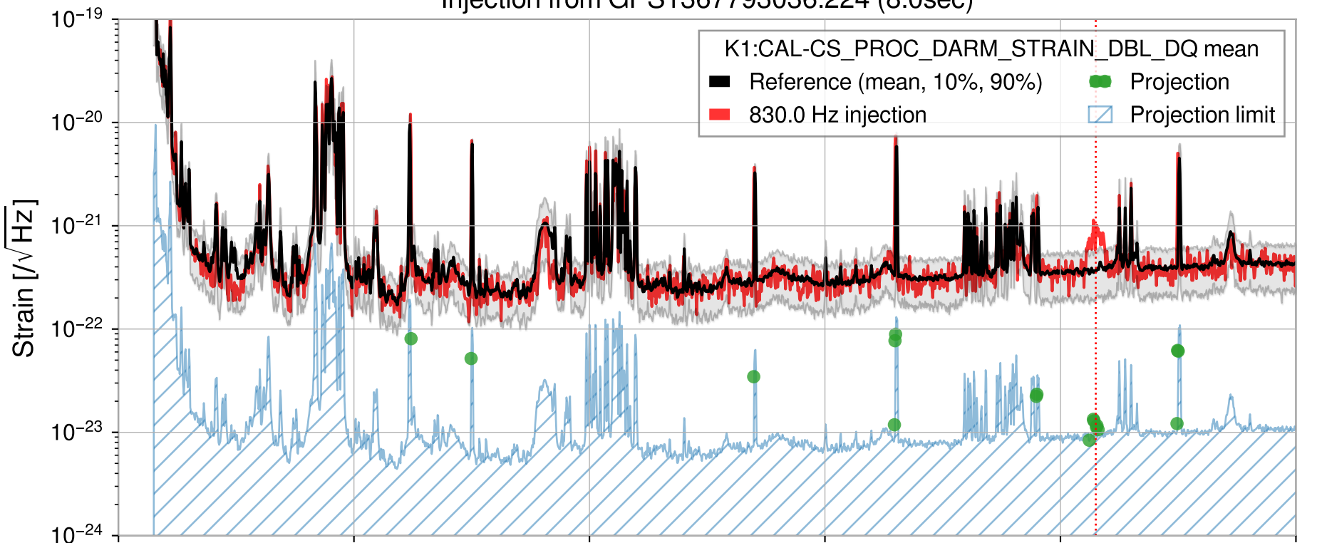
Injection from GPS1367793036.224 (8.0sec)
