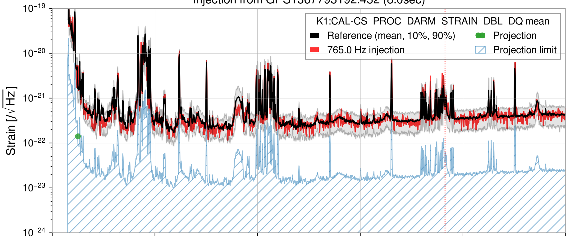
Injection from GPS1367793192.432 (8.0sec)
