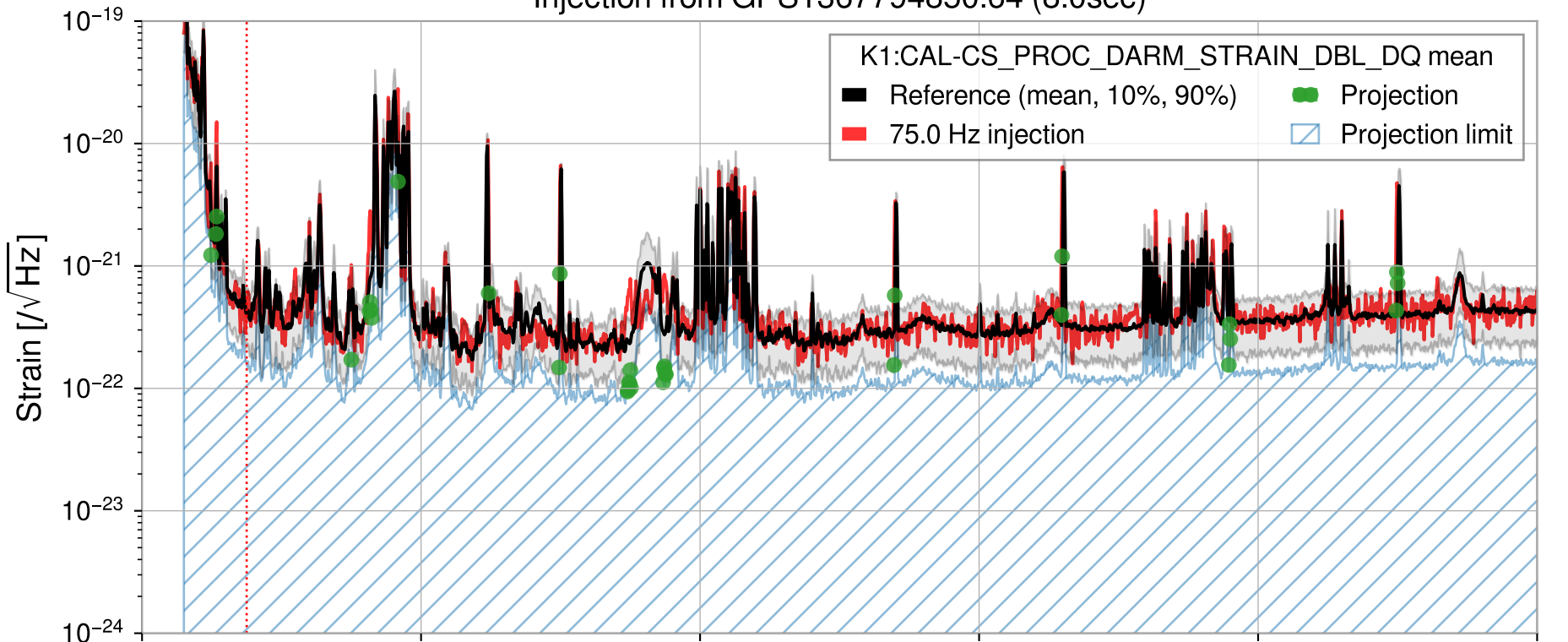
Injection from GPS1367794850.64 (8.0sec)
