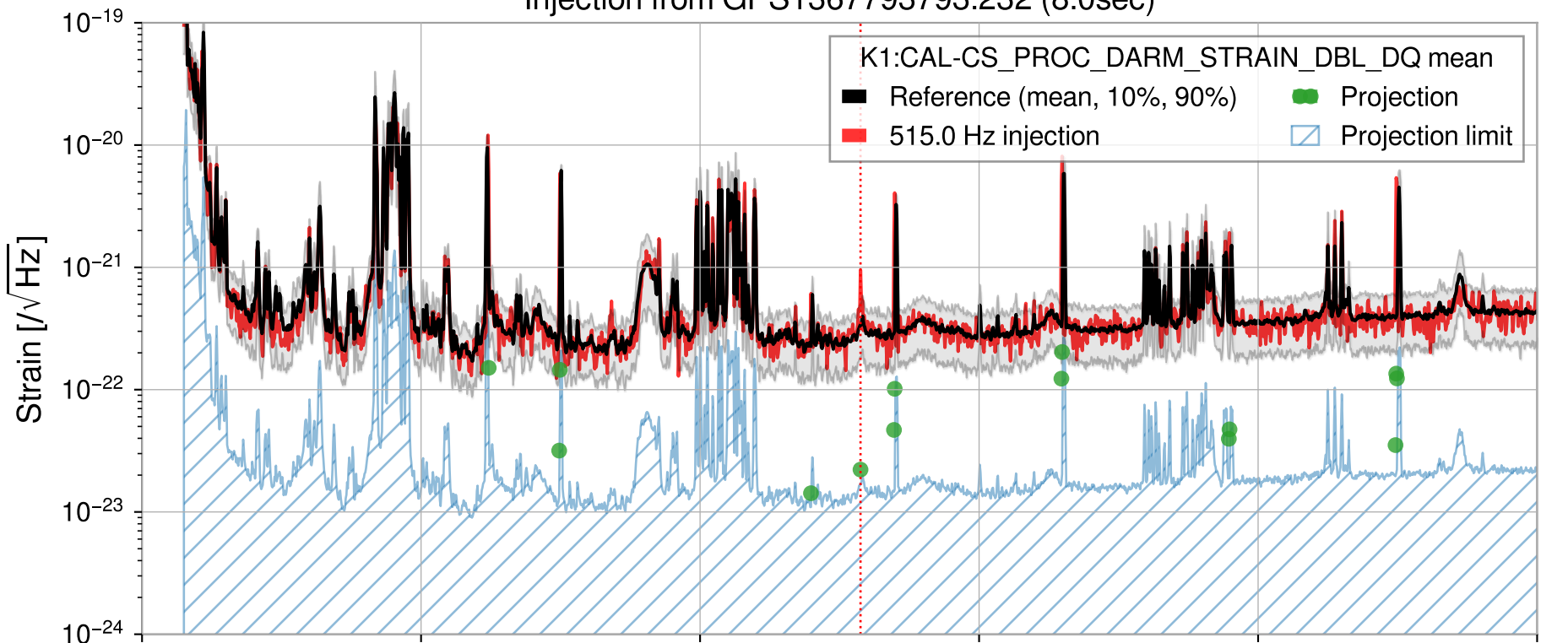
Injection from GPS1367793793.232 (8.0sec)
