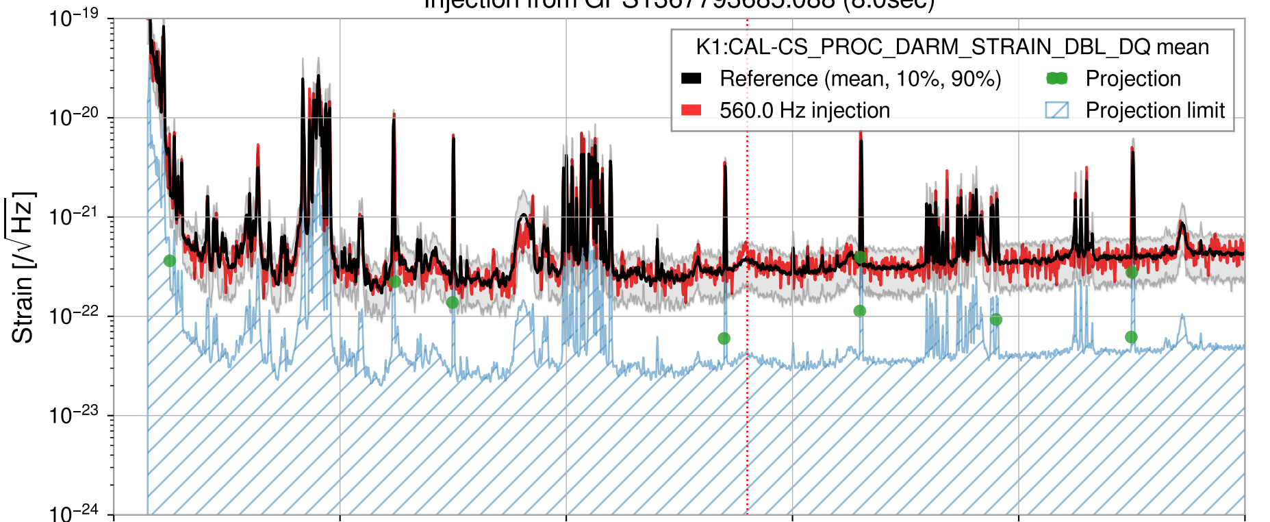
Injection from GPS1367793685.088 (8.0sec)
