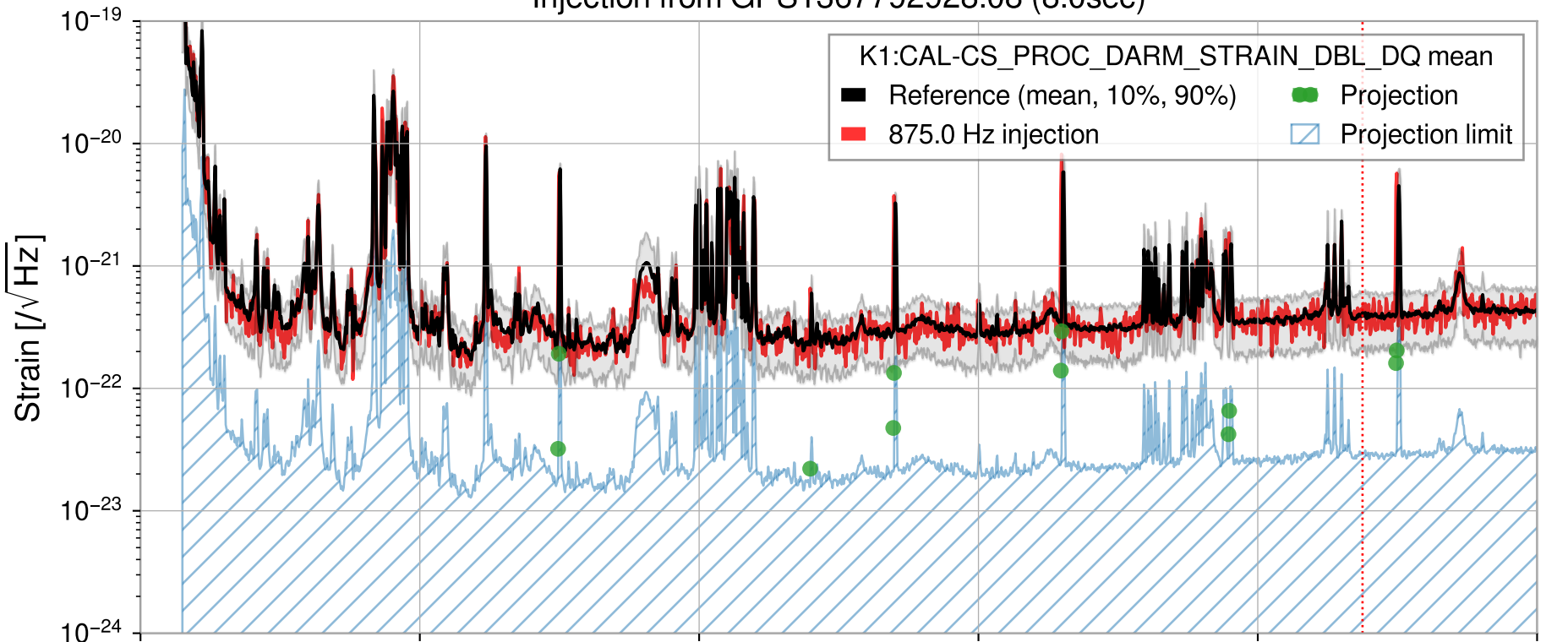
Injection from GPS1367792928.08 (8.0sec)
