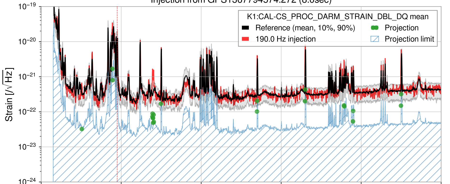
Injection from GPS1367794574.272 (8.0sec)
