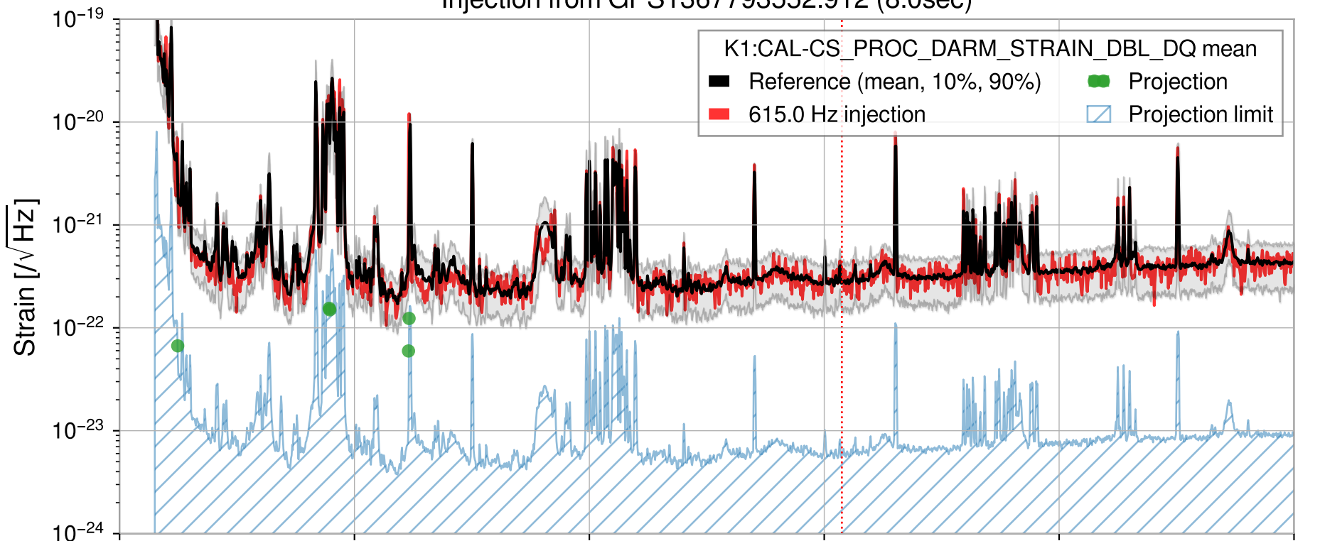
Injection from GPS1367793552.912 (8.0sec)
