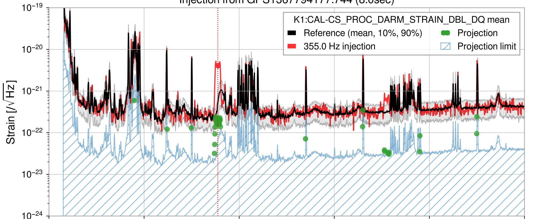
Injection from GPS1367794177.744 (8.0sec)
