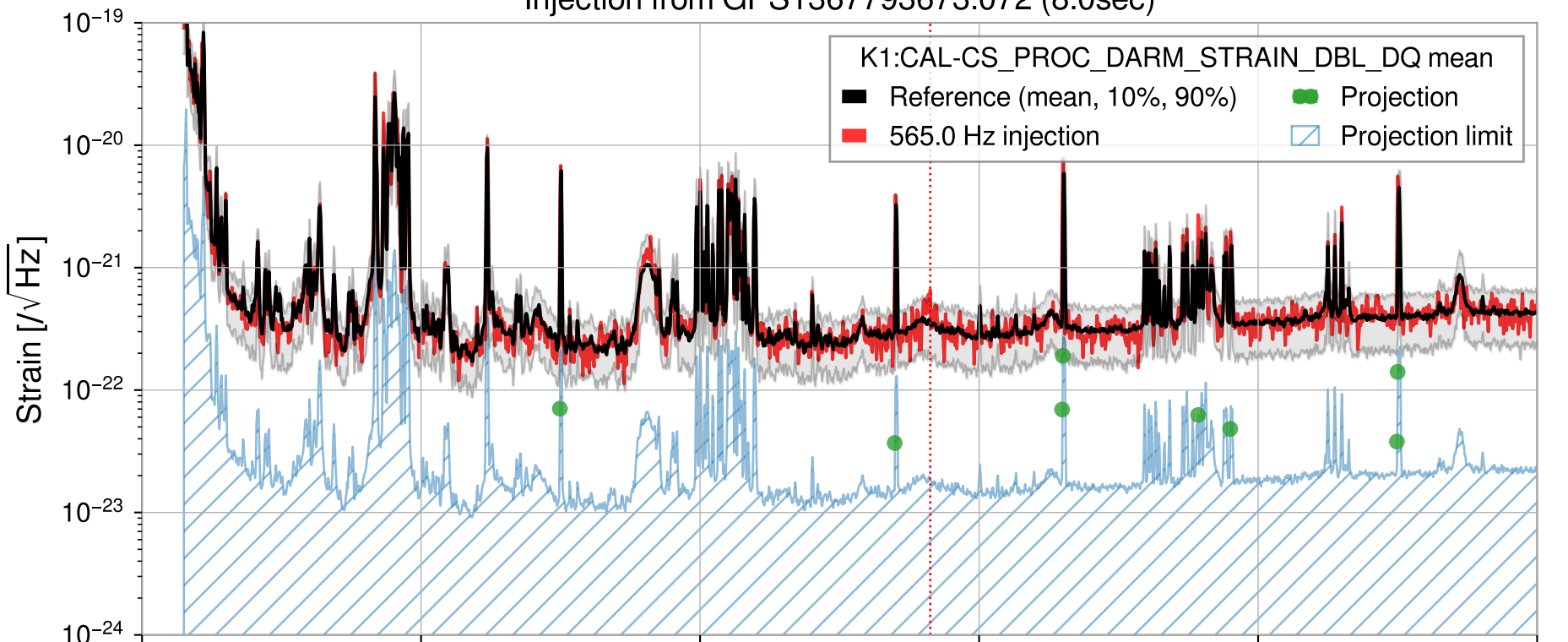
Injection from GPS1367793673.072 (8.0sec)
