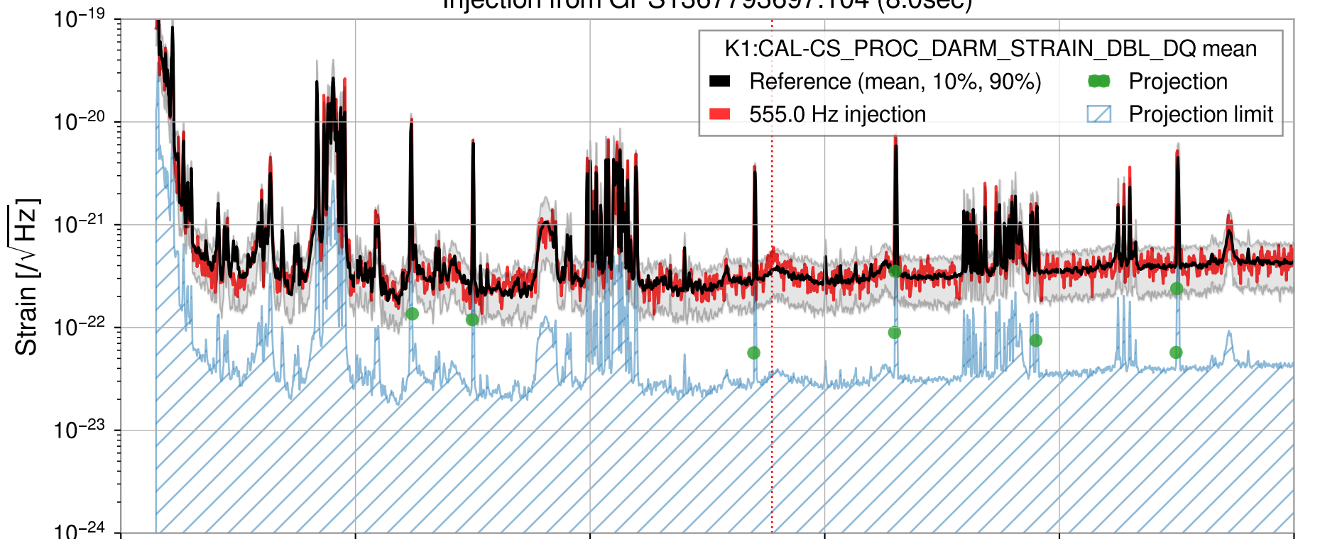
Injection from GPS1367793697.104 (8.0sec)
