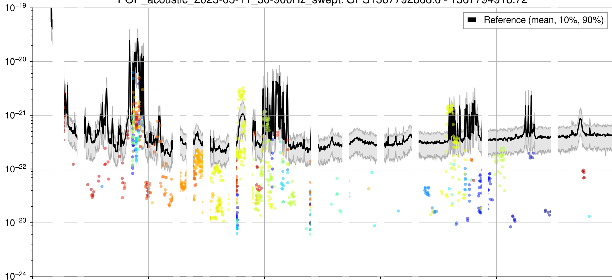
POP_acoustic_2023-05-11_50-900Hz_swept: GPS1367792868.0 - 1367794918.72
