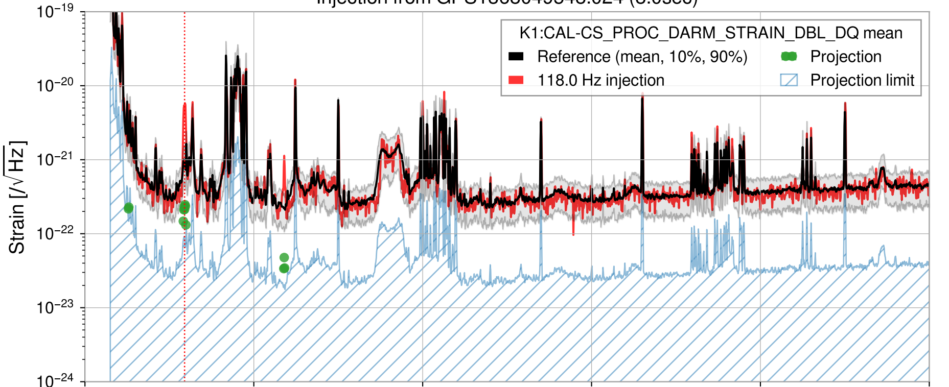
Injection from GPS1368049548.024 (8.0sec)
