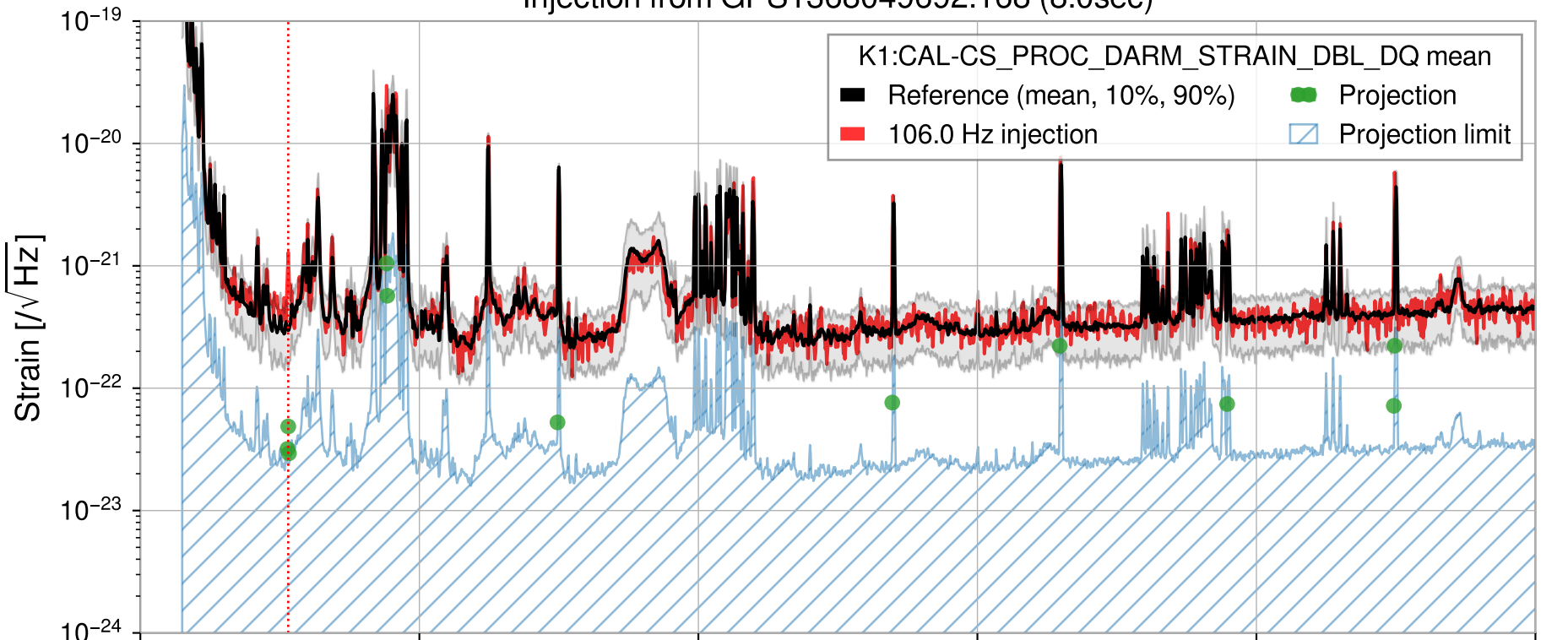
Injection from GPS1368049692.168 (8.0sec)
