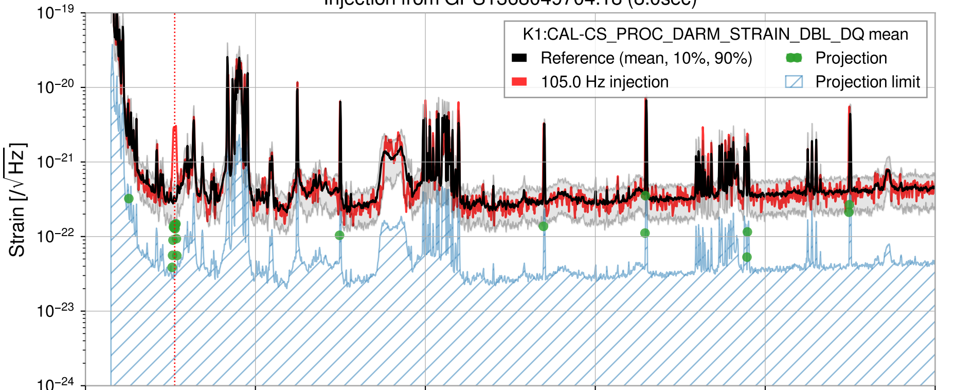
Injection from GPS1368049704.18 (8.0sec)
