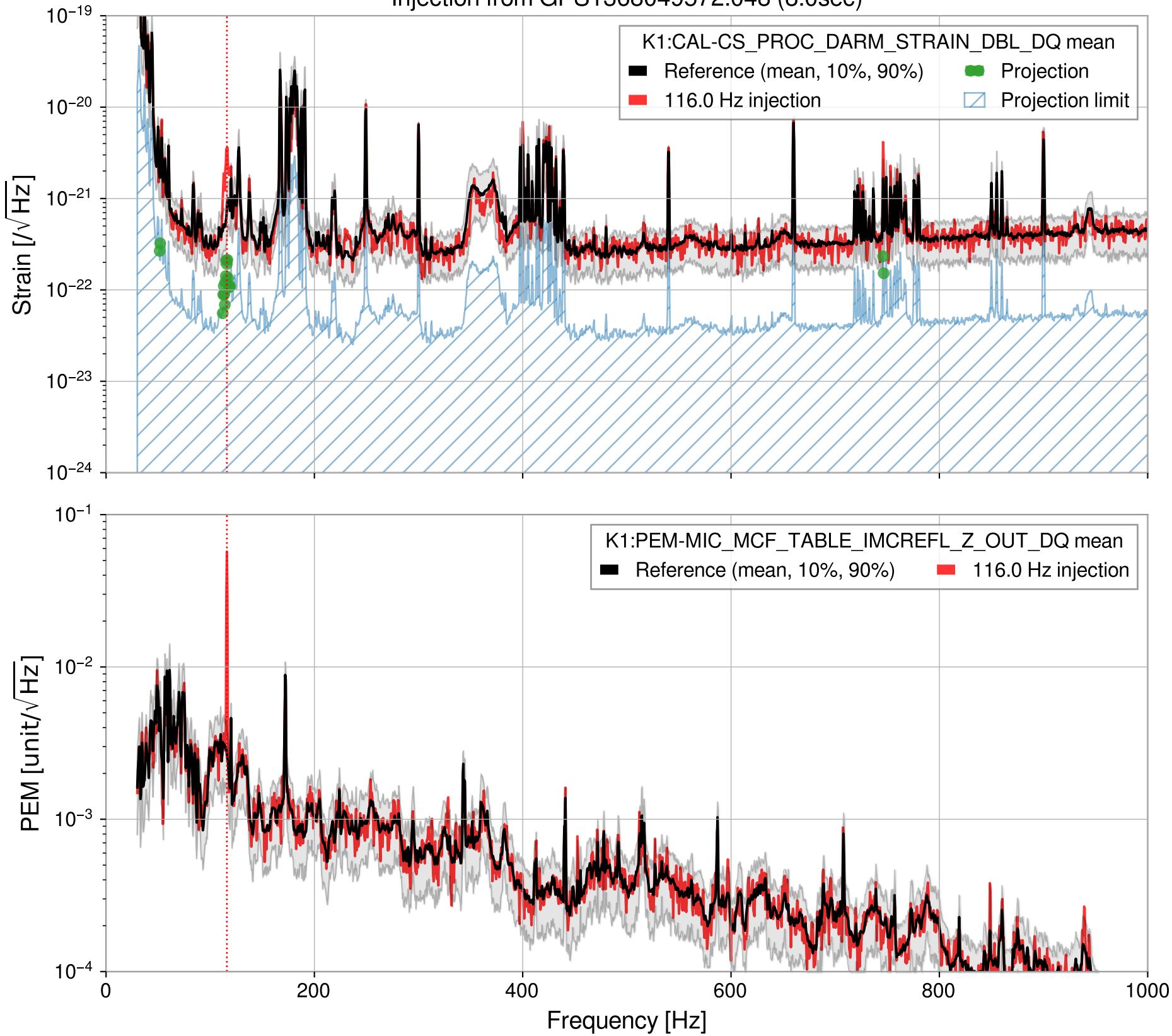
Injection from GPS1368049572.048 (8.0sec)
