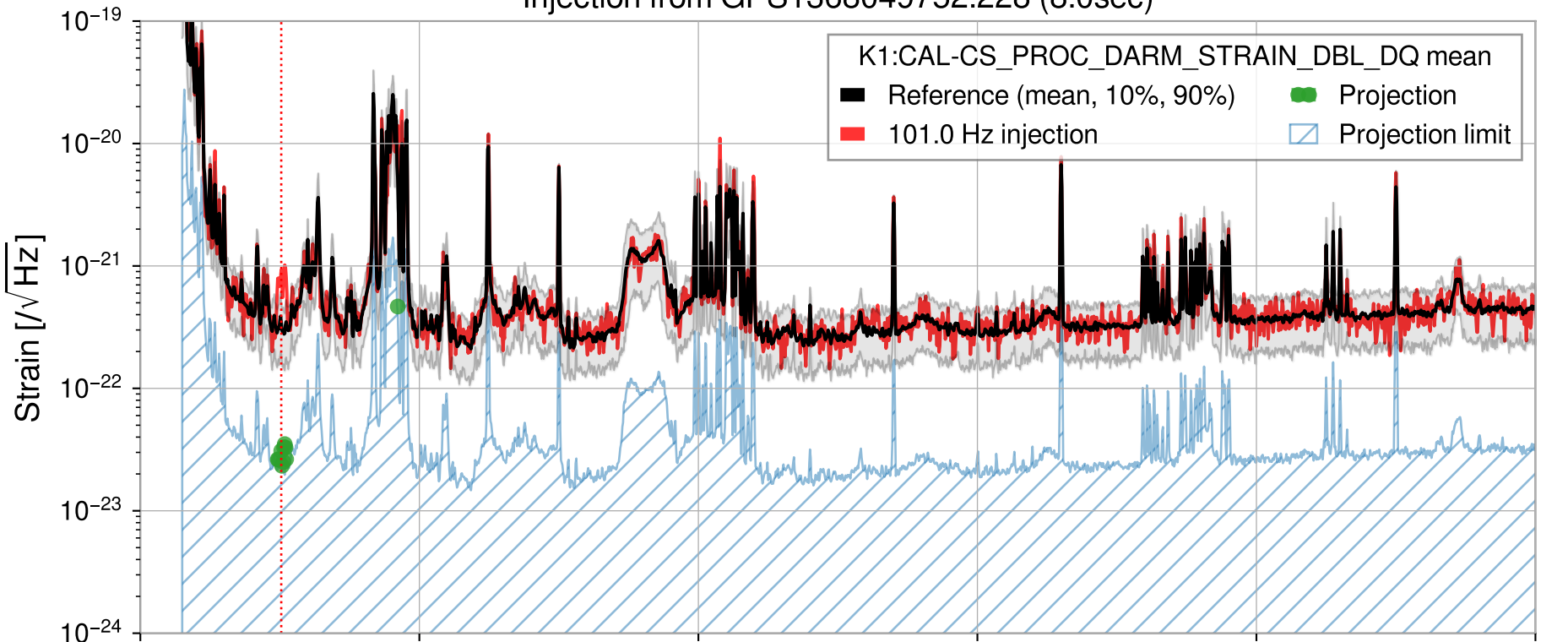
Injection from GPS1368049752.228 (8.0sec)
