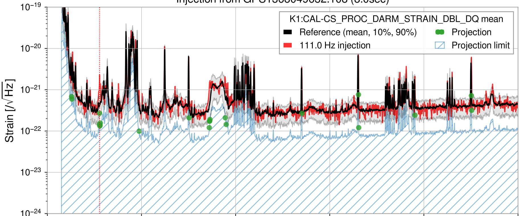
Injection from GPS1368049632.108 (8.0sec)
