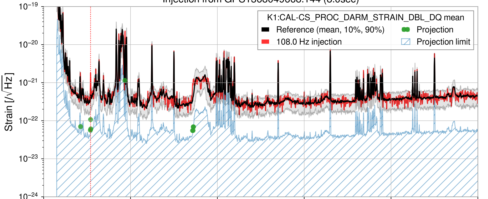
Injection from GPS1368049668.144 (8.0sec)
