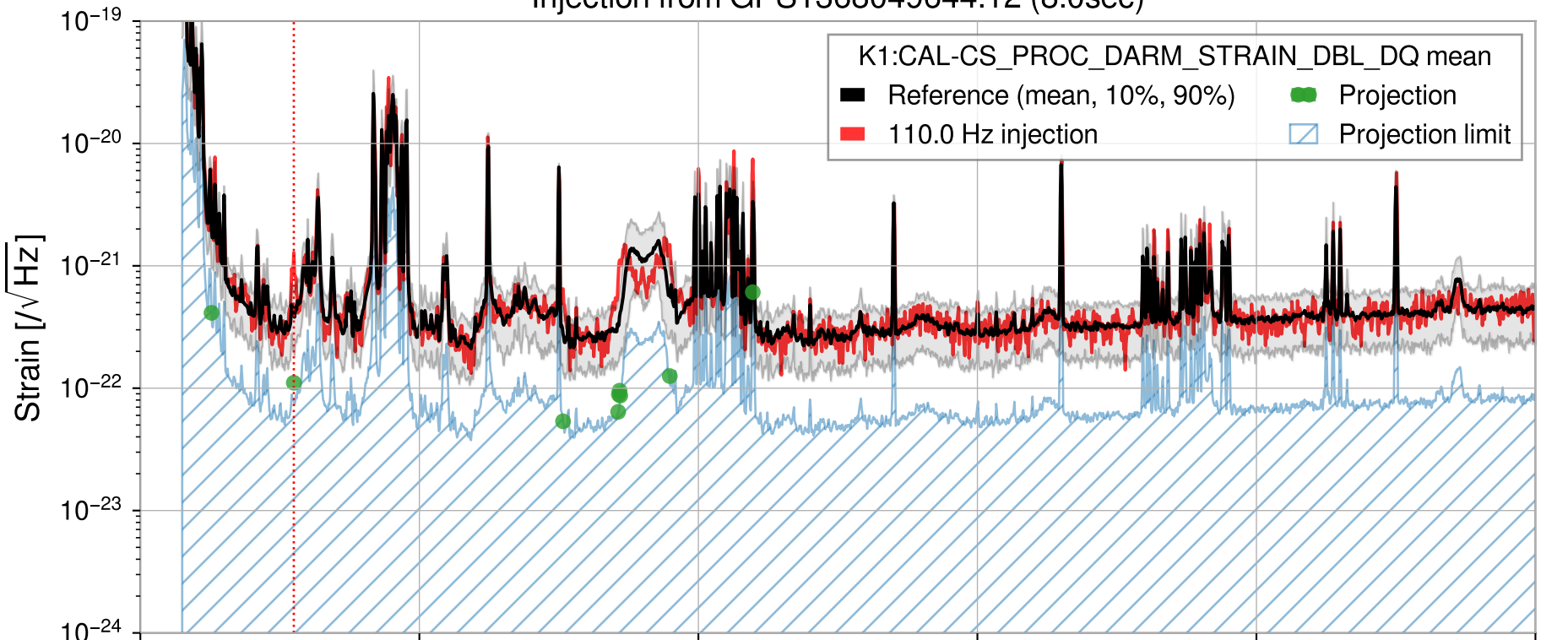
Injection from GPS1368049644.12 (8.0sec)
