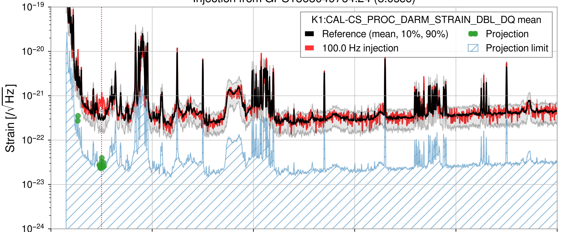
Injection from GPS1368049764.24 (8.0sec)
