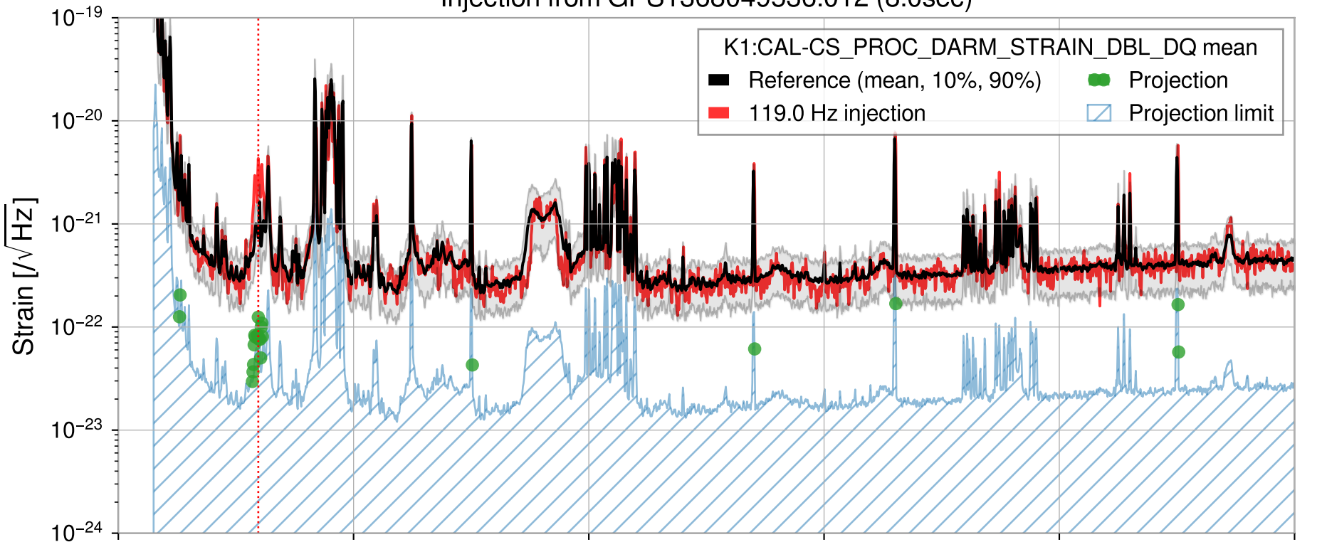
Injection from GPS1368049536.012 (8.0sec)
