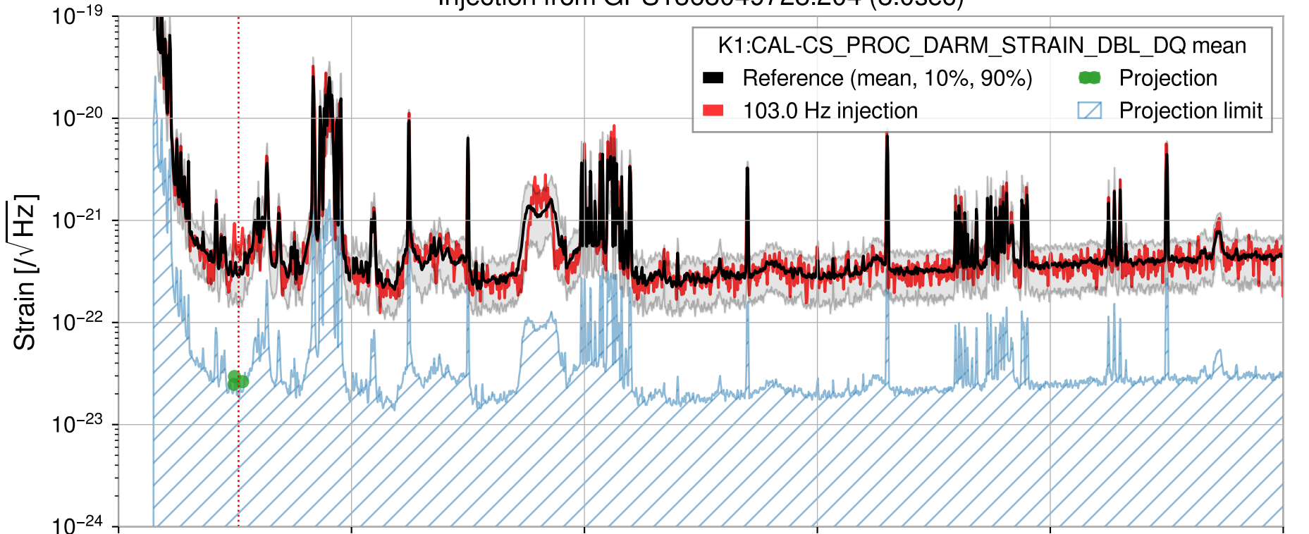
Injection from GPS1368049728.204 (8.0sec)
