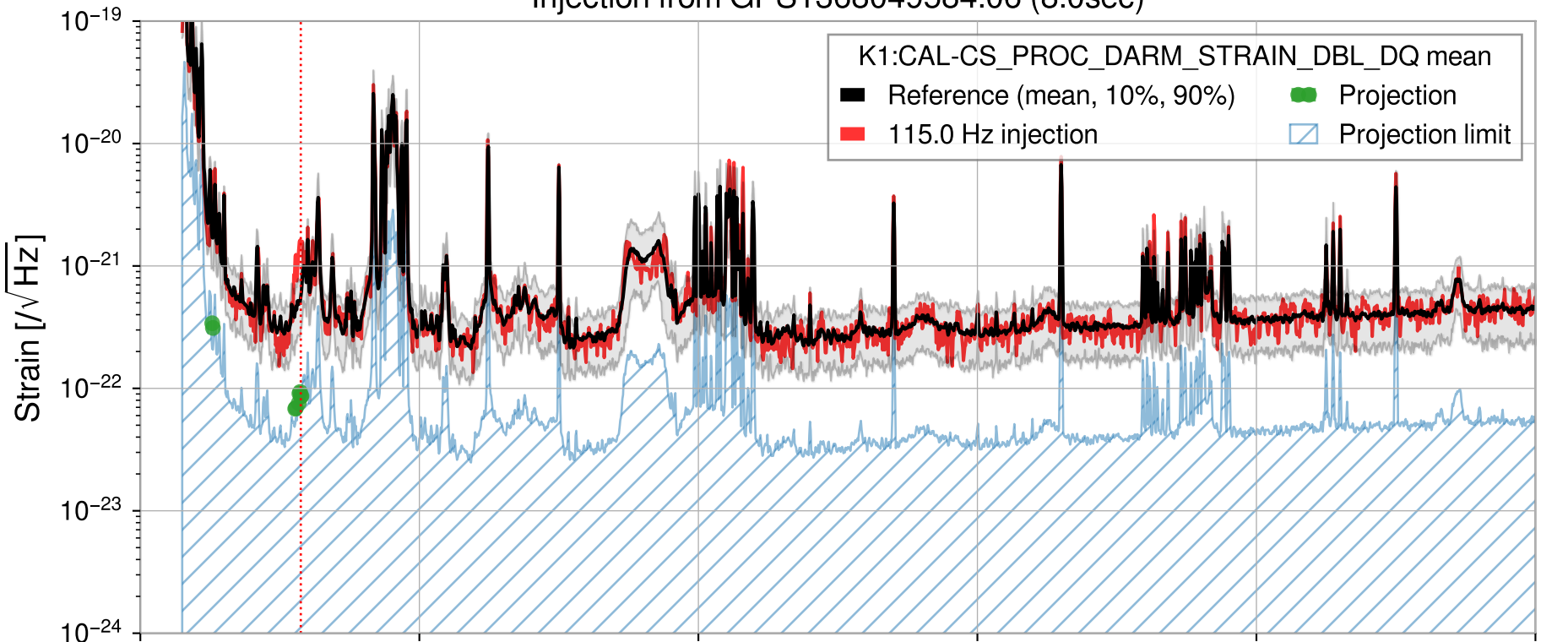
Injection from GPS1368049584.06 (8.0sec)
