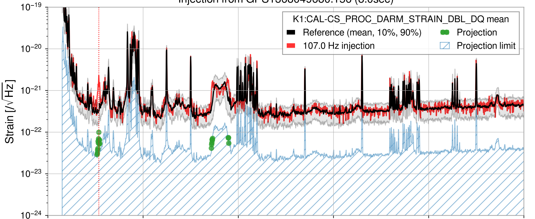
Injection from GPS1368049680.156 (8.0sec)
