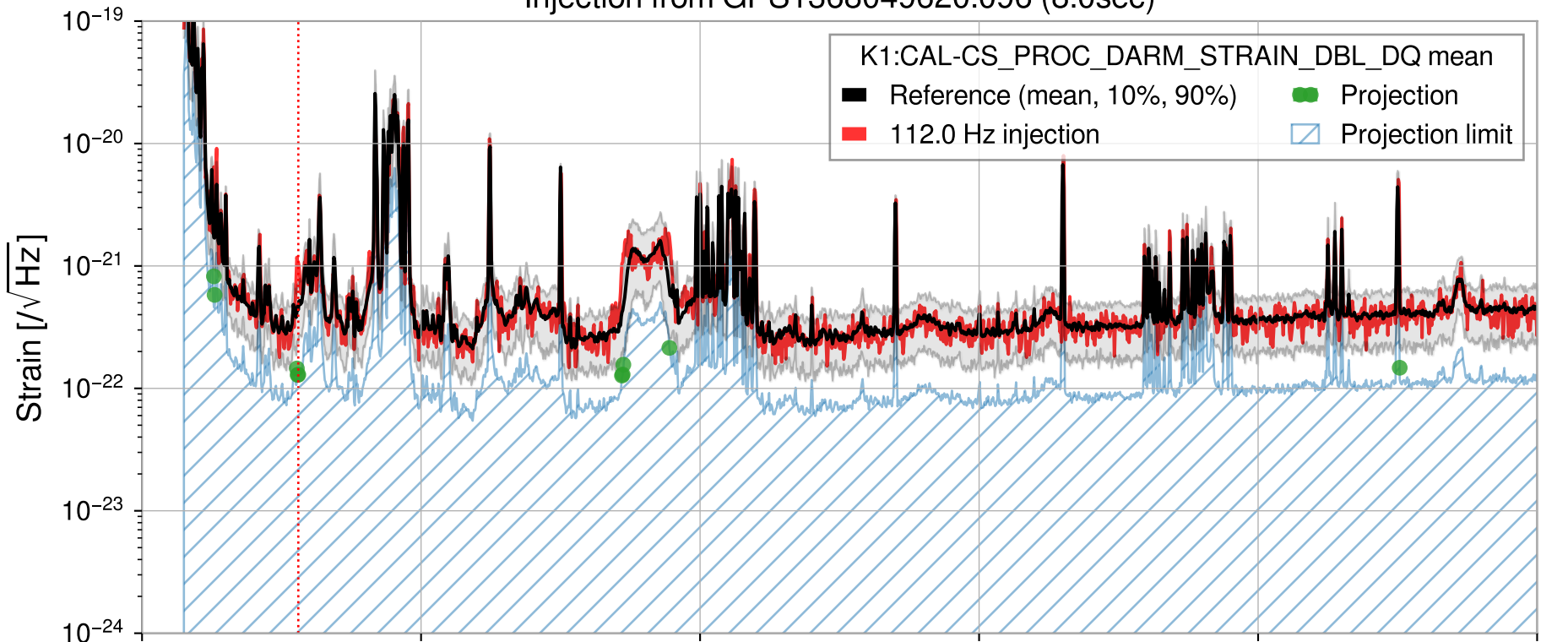
Injection from GPS1368049620.096 (8.0sec)
