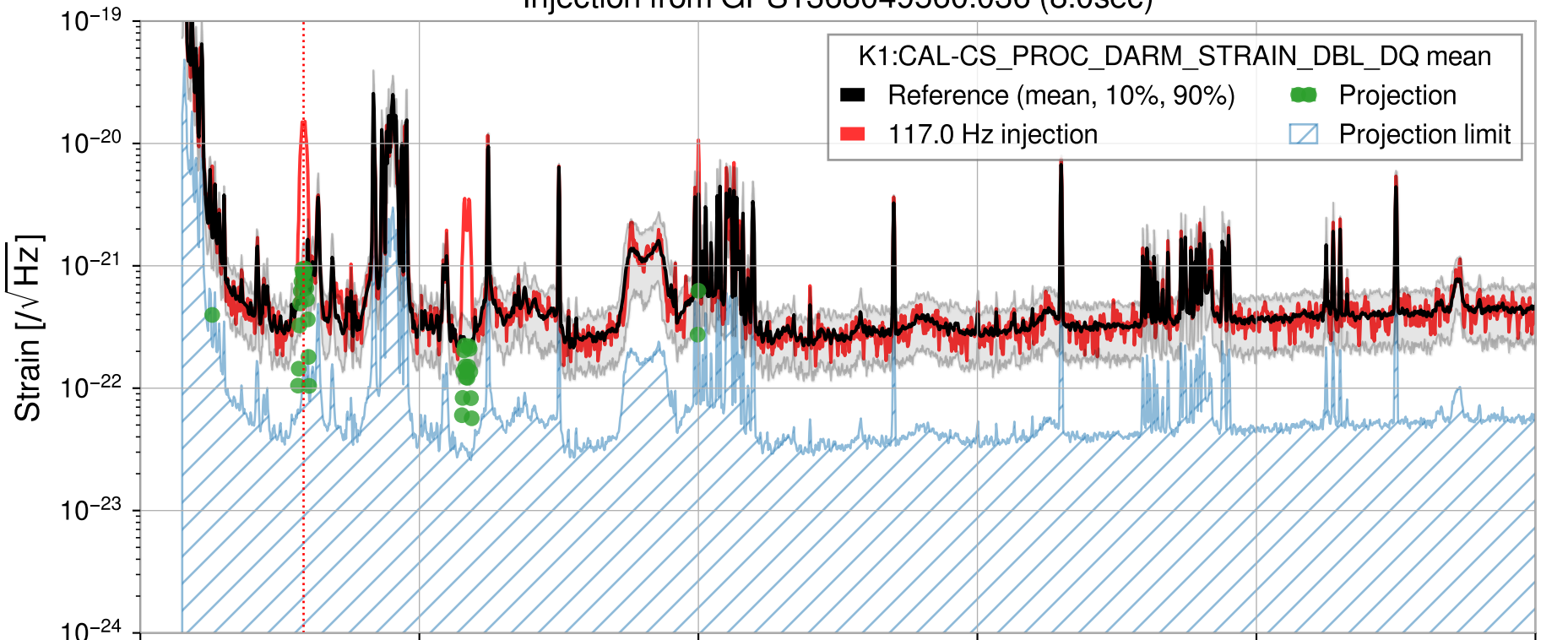
Injection from GPS1368049560.036 (8.0sec)
