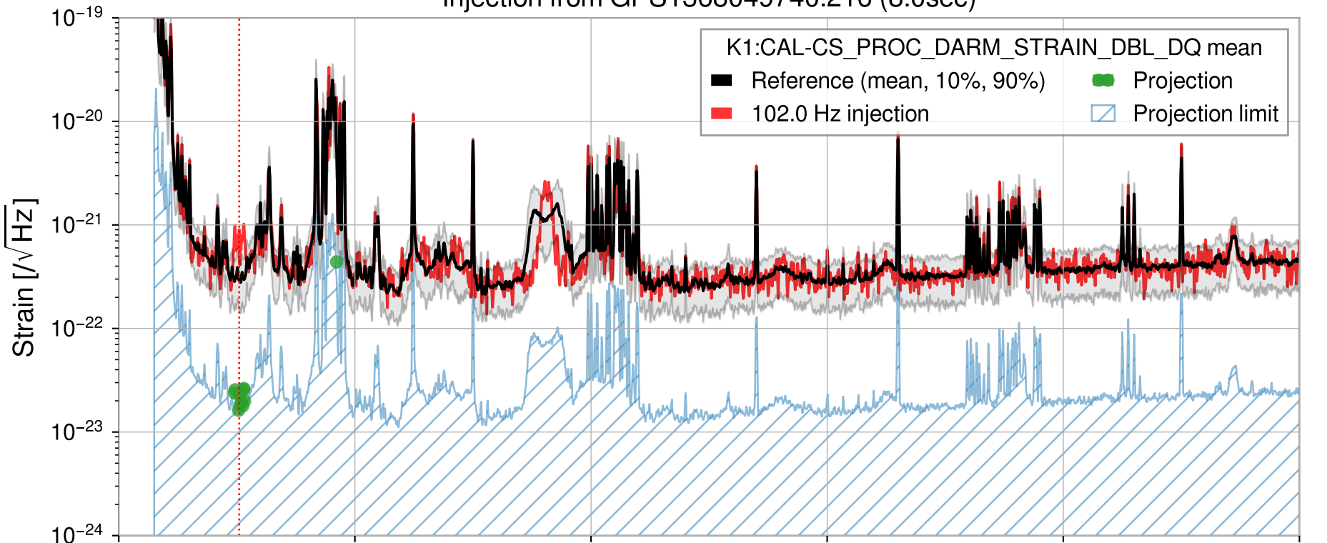
Injection from GPS1368049740.216 (8.0sec)
