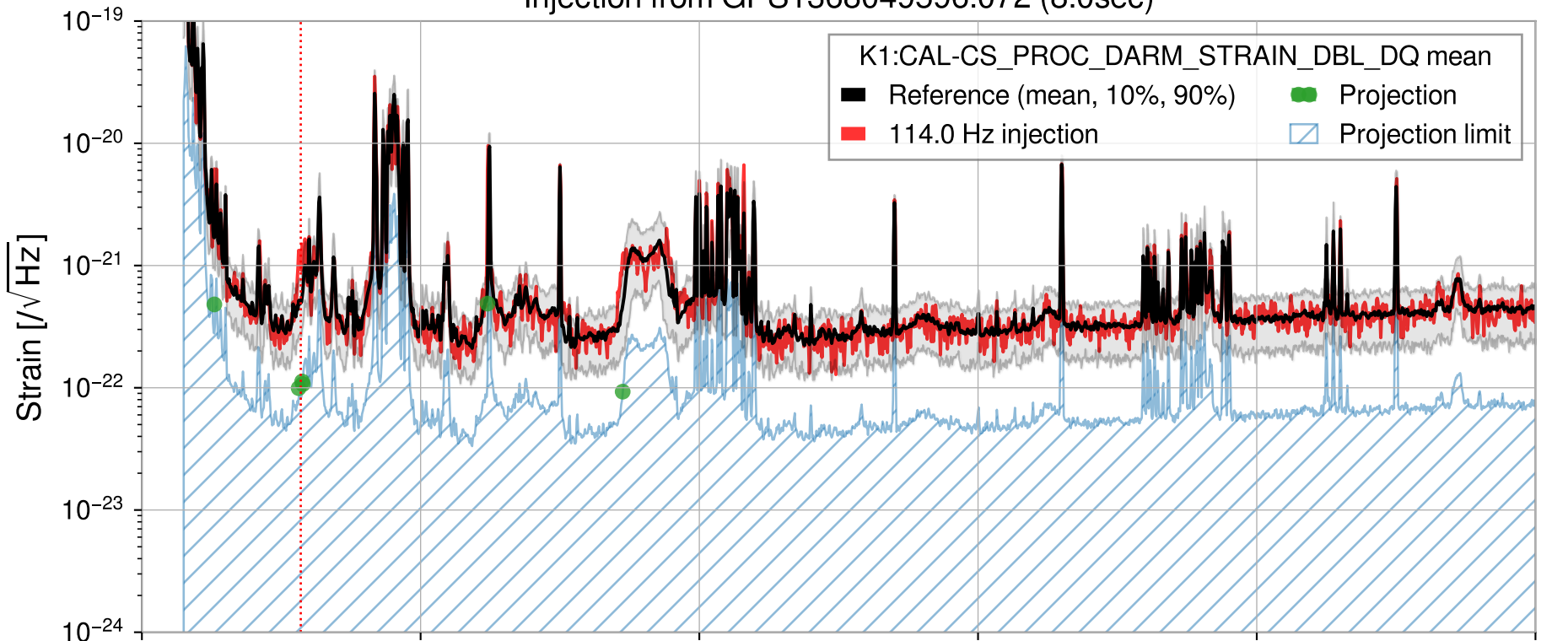
Injection from GPS1368049596.072 (8.0sec)
