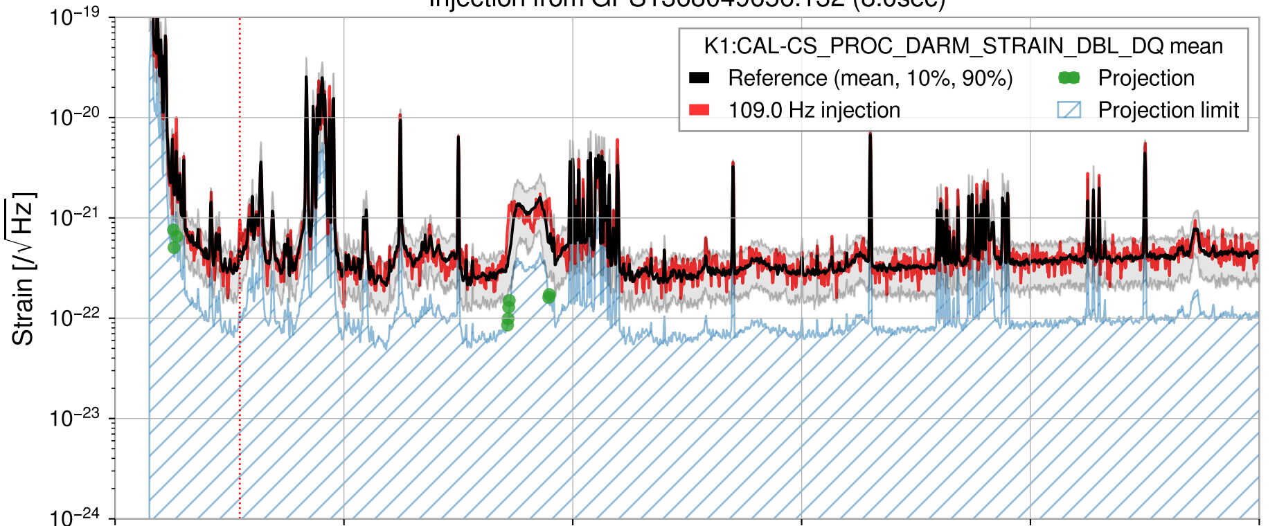
Injection from GPS1368049656.132 (8.0sec)
