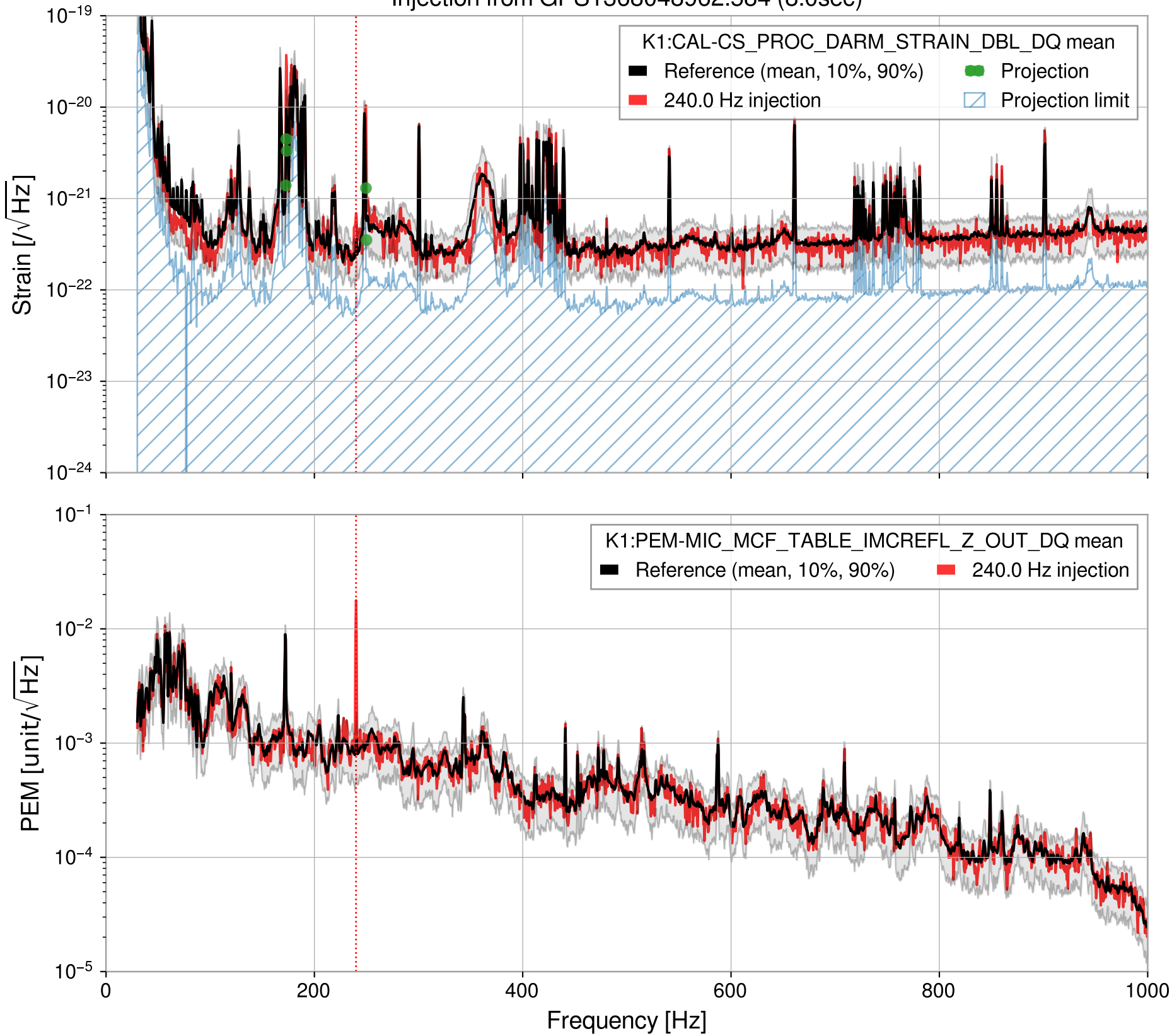
Injection from GPS1368048962.584 (8.0sec)
