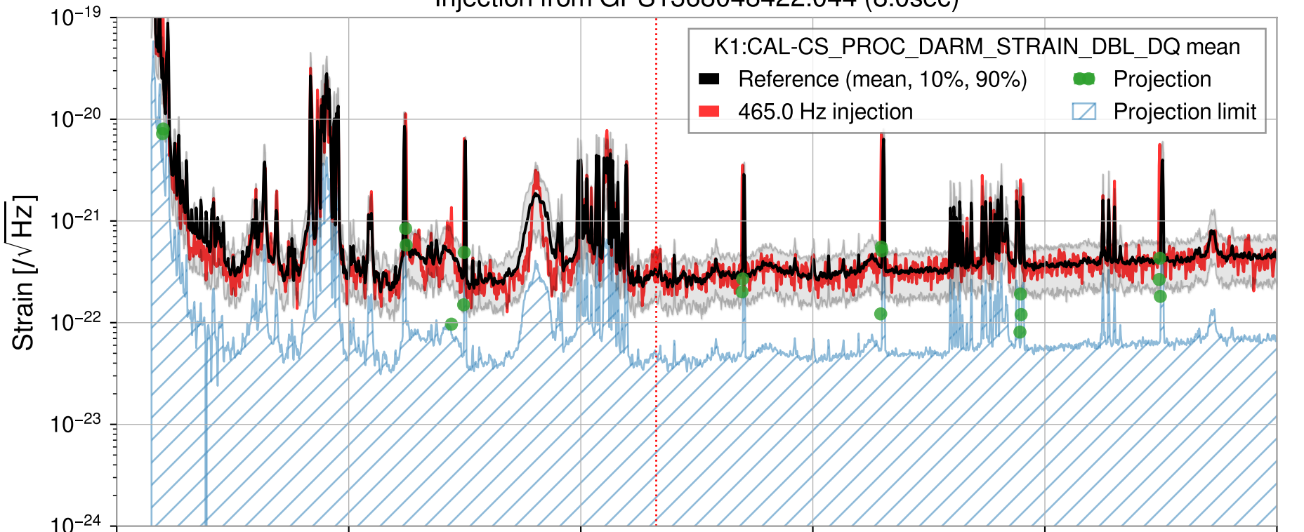
Injection from GPS1368048422.044 (8.0sec)
