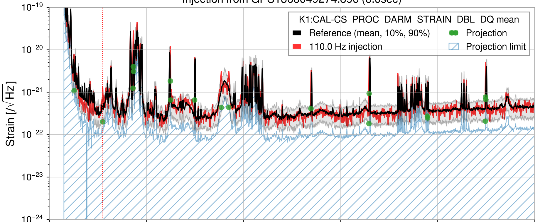
Injection from GPS1368049274.896 (8.0sec)
