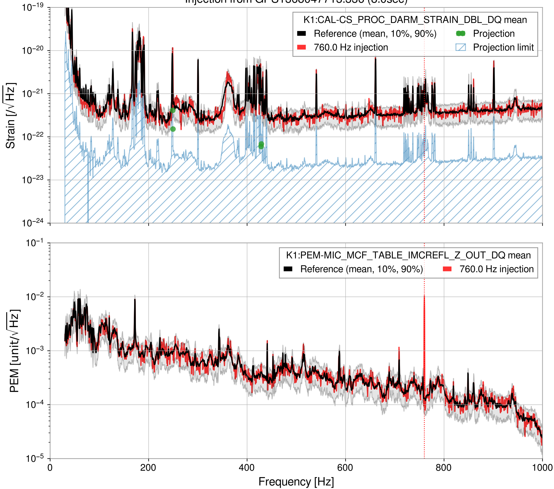
Injection from GPS1368047713.336 (8.0sec)
