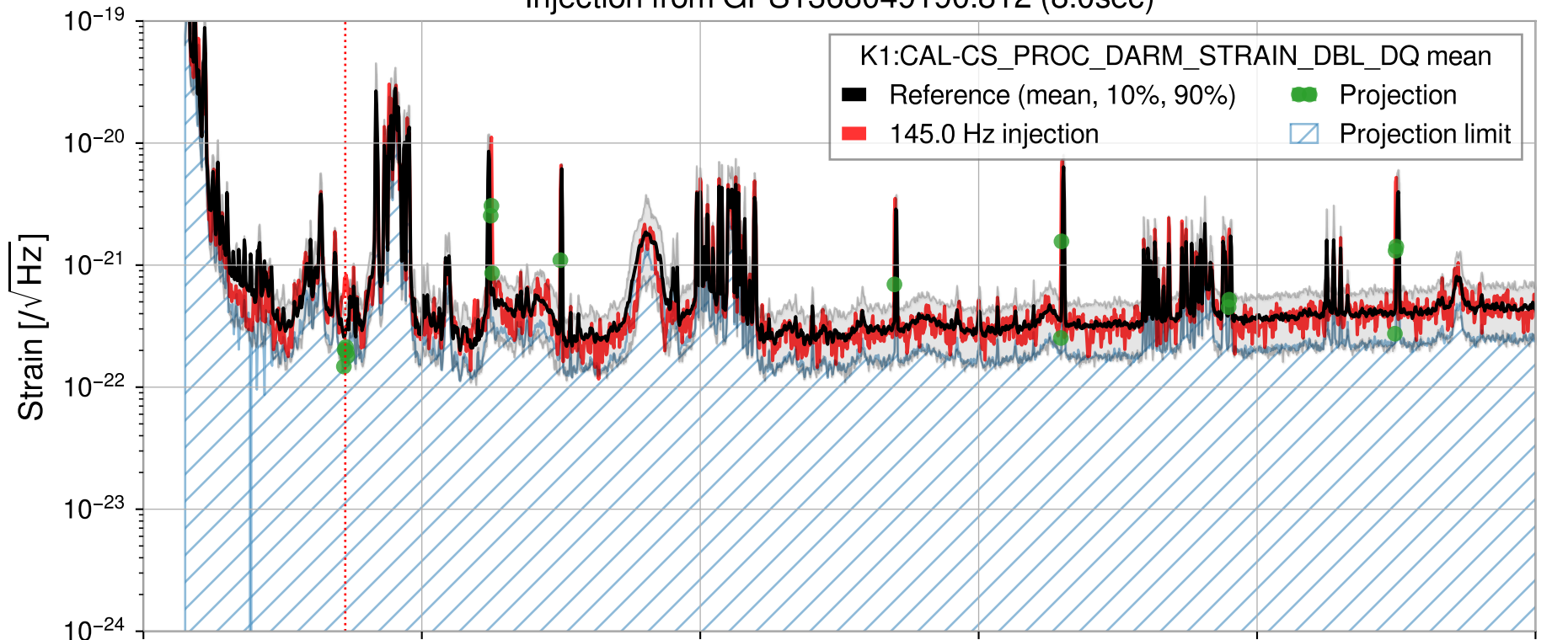
Injection from GPS1368049190.812 (8.0sec)
