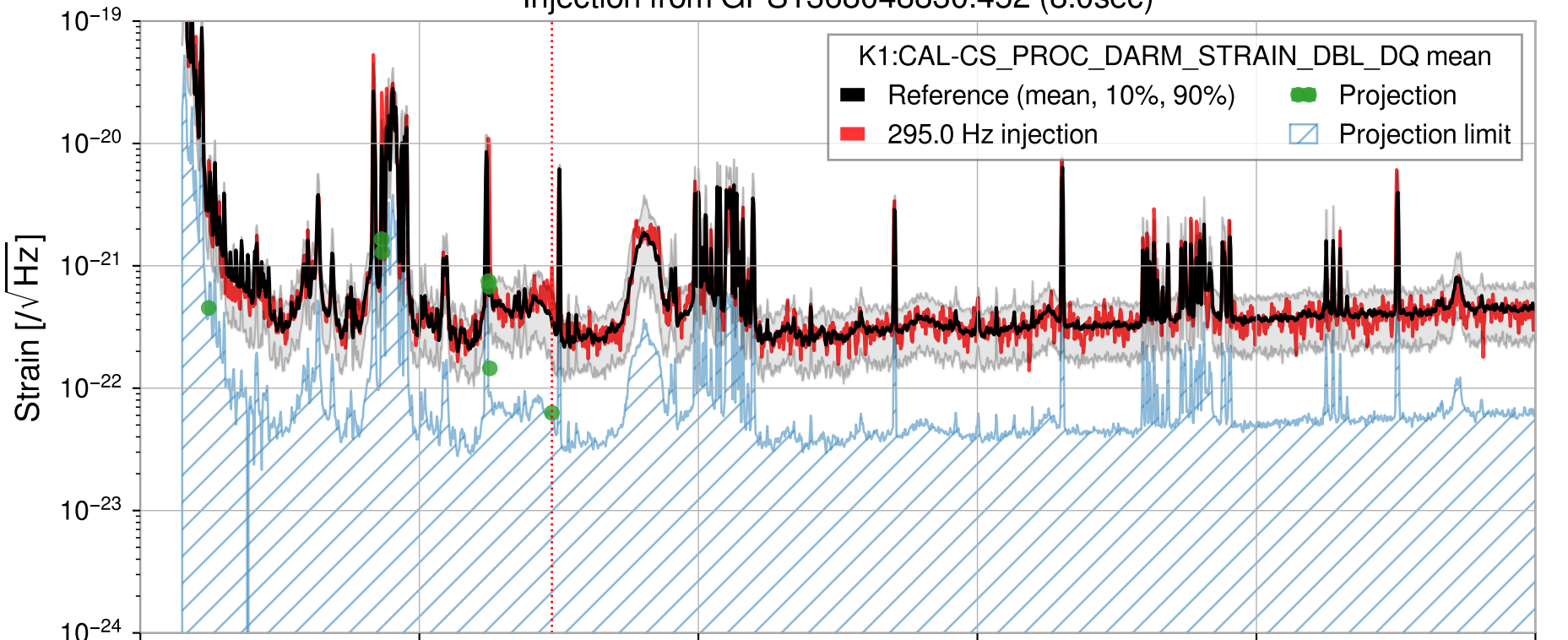
Injection from GPS1368048830.452 (8.0sec)
