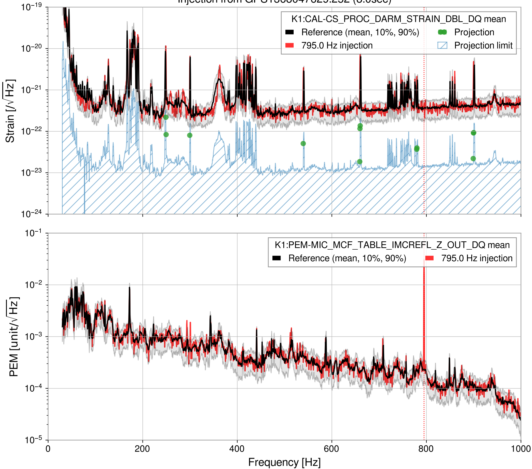
Injection from GPS1368047629.252 (8.0sec)
