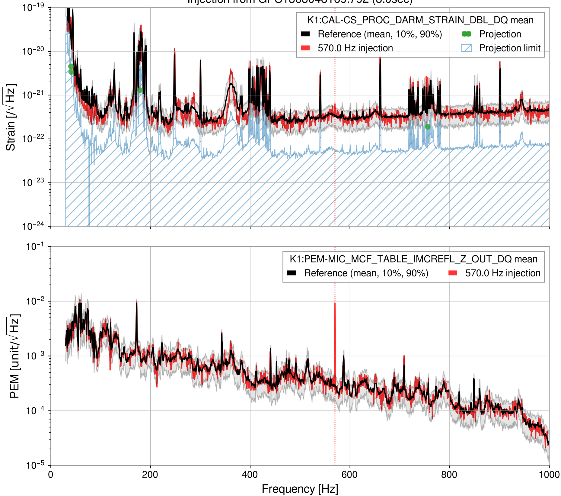
Injection from GPS1368048169.792 (8.0sec)
