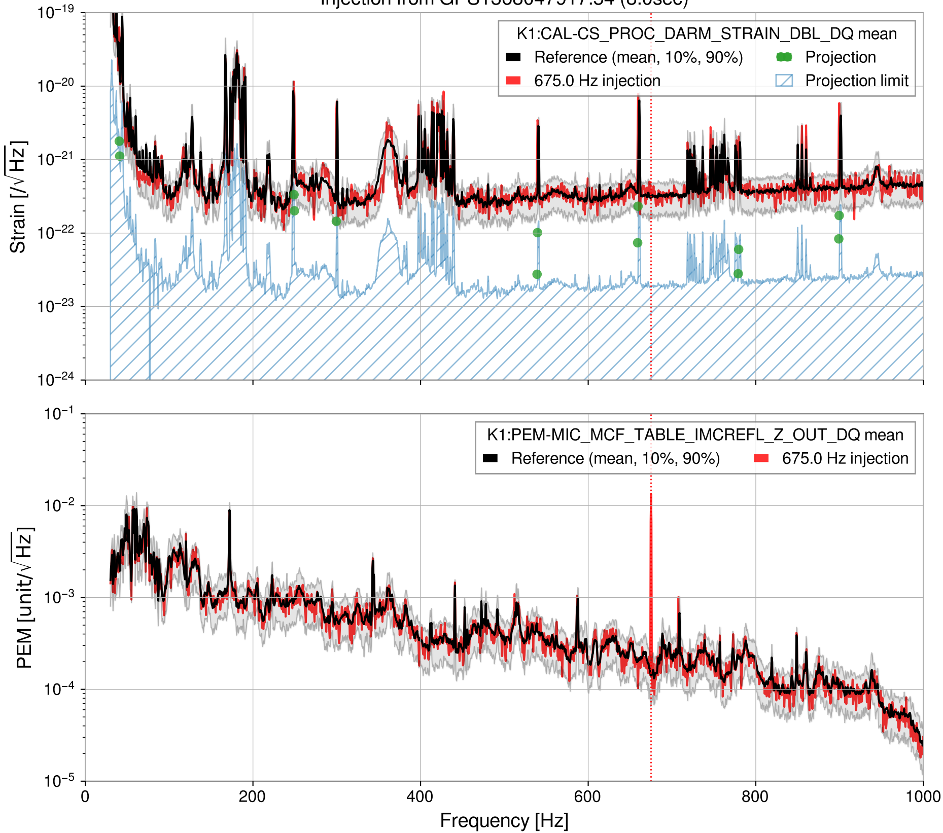
Injection from GPS1368047917.54 (8.0sec)
