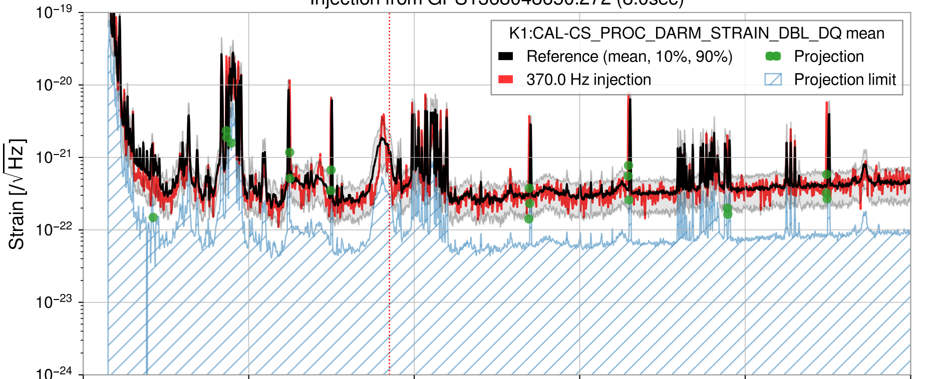
Injection from GPS1368048650.272 (8.0sec)
