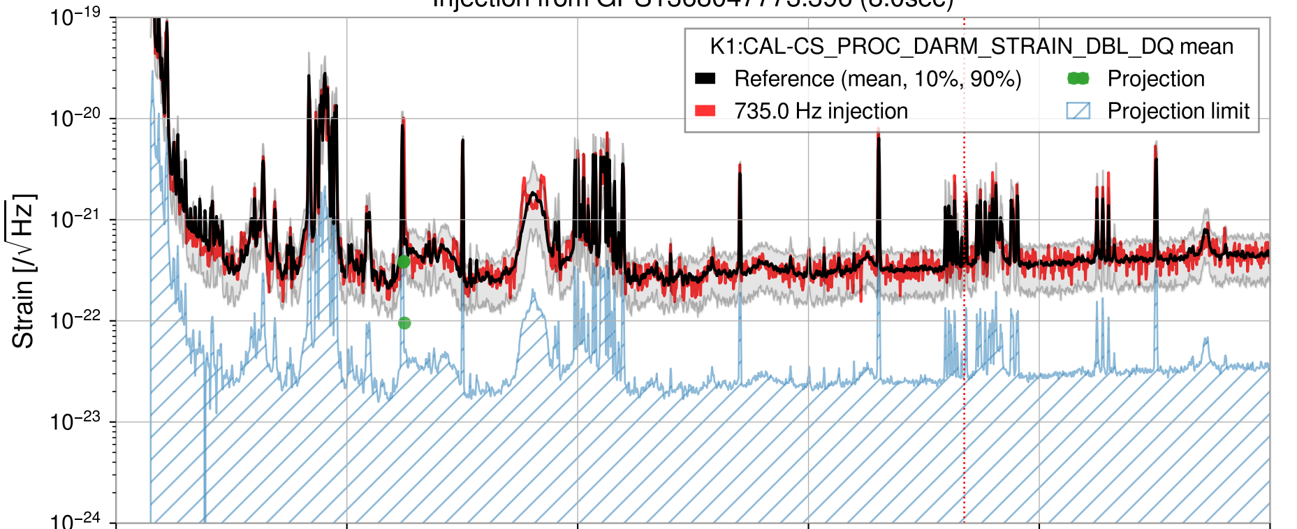
Injection from GPS1368047773.396 (8.0sec)
