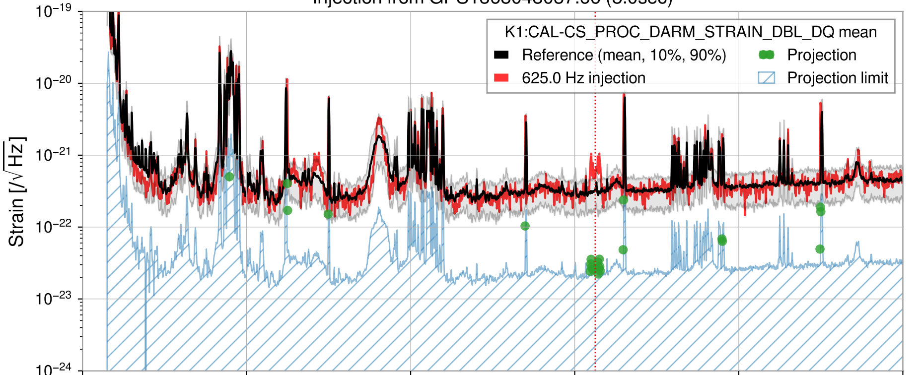
Injection from GPS1368048037.66 (8.0sec)
