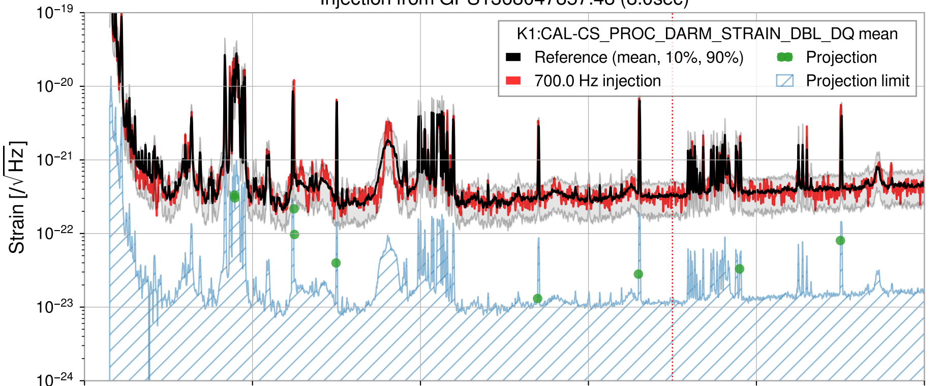
Injection from GPS1368047857.48 (8.0sec)
