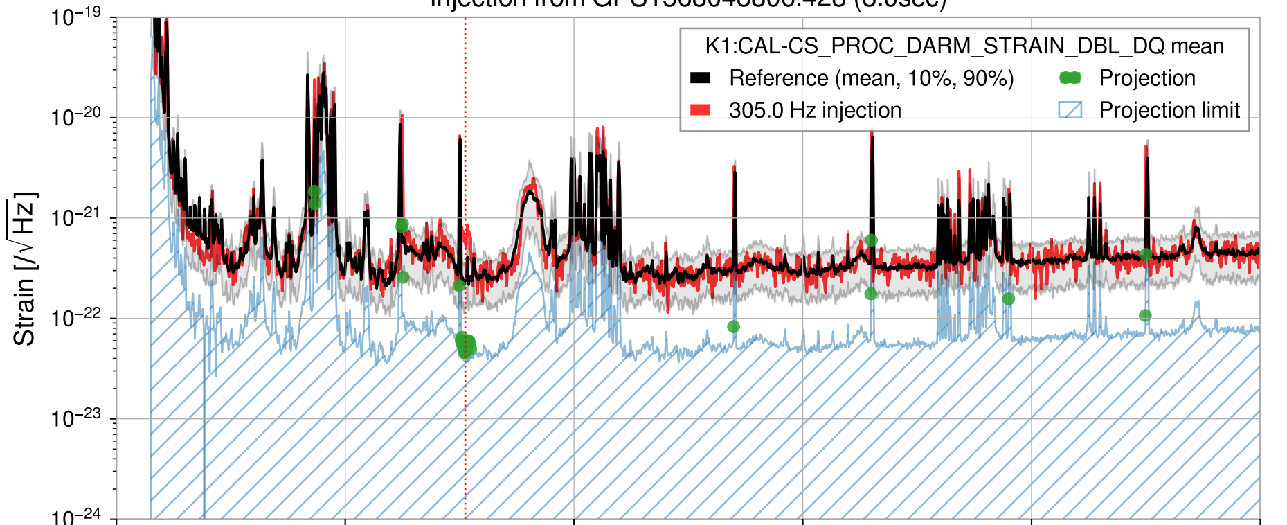
Injection from GPS1368048806.428 (8.0sec)
