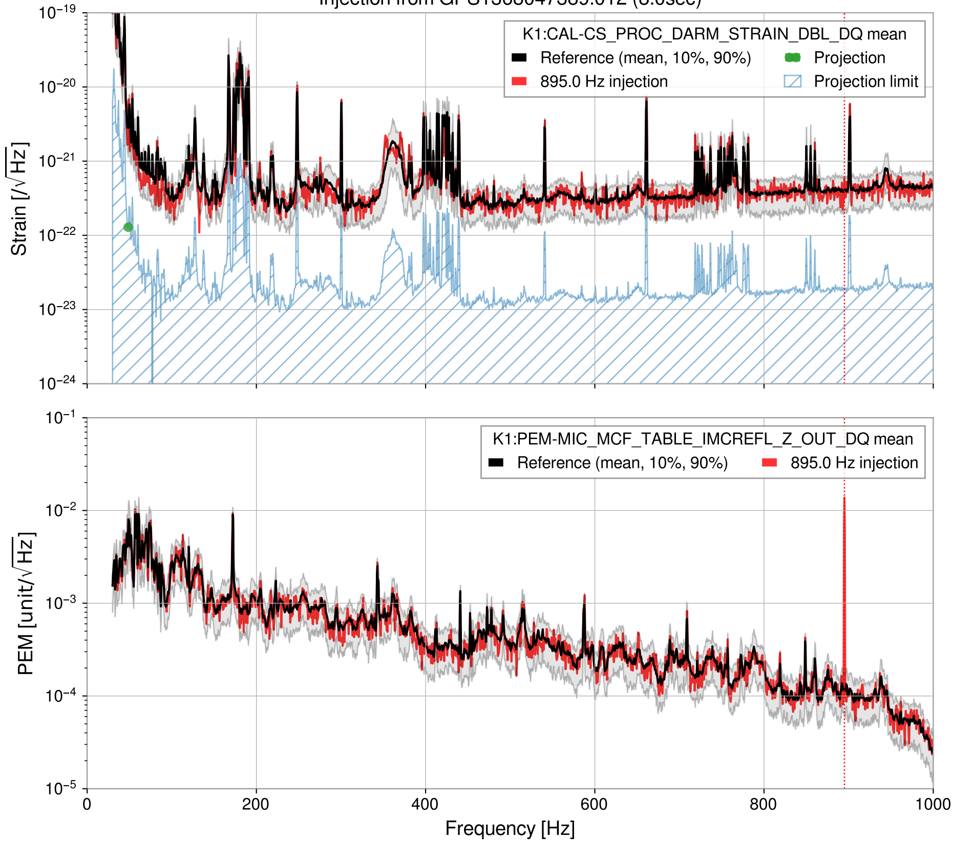
Injection from GPS1368047389.012 (8.0sec)
