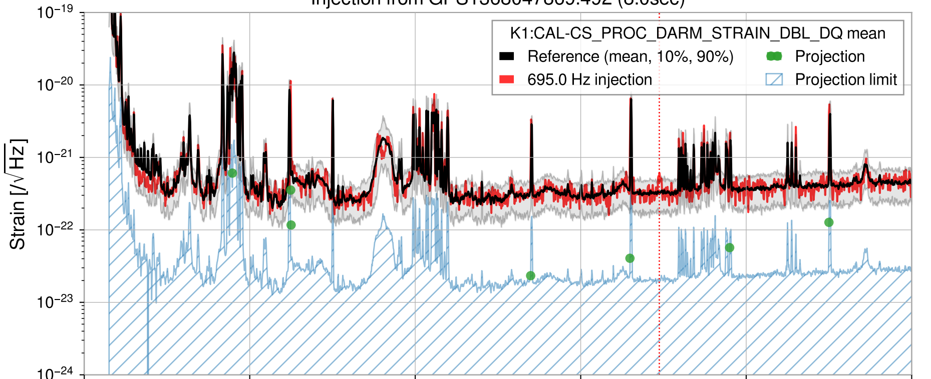
Injection from GPS1368047869.492 (8.0sec)
