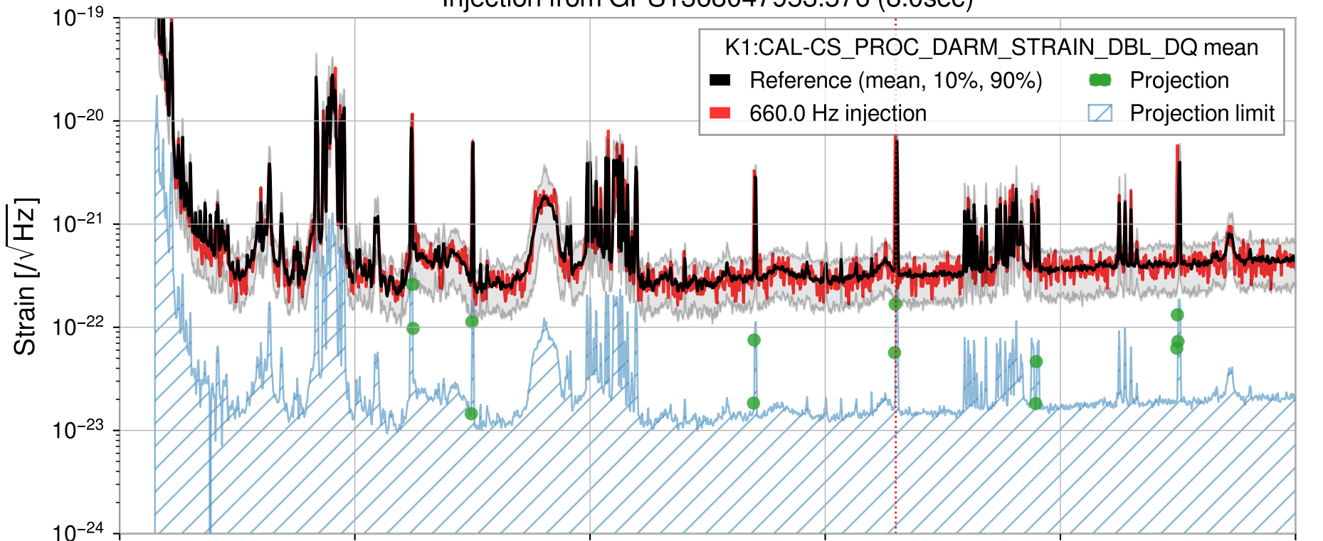
Injection from GPS1368047953.576 (8.0sec)
