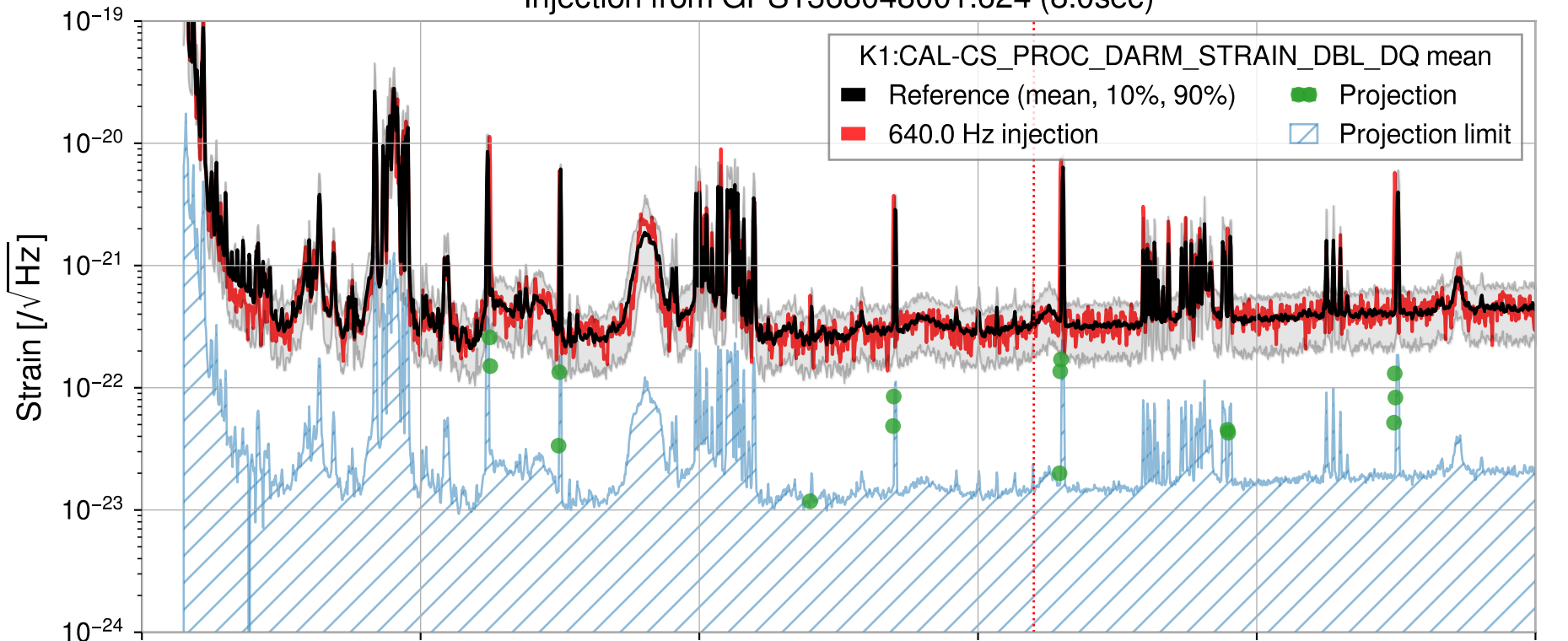
Injection from GPS1368048001.624 (8.0sec)
