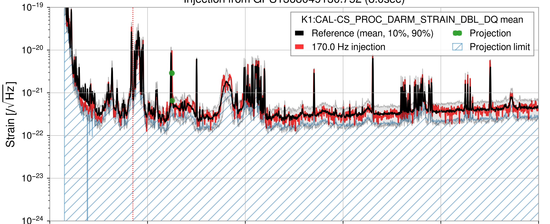
Injection from GPS1368049130.752 (8.0sec)
