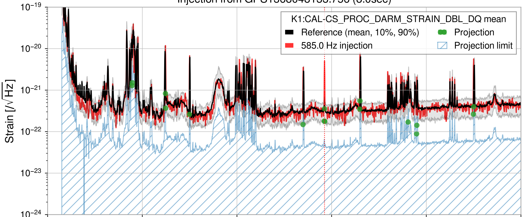
Injection from GPS1368048133.756 (8.0sec)
