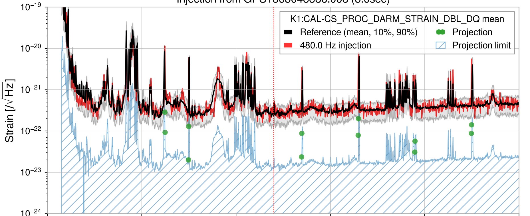
Injection from GPS1368048386.008 (8.0sec)
