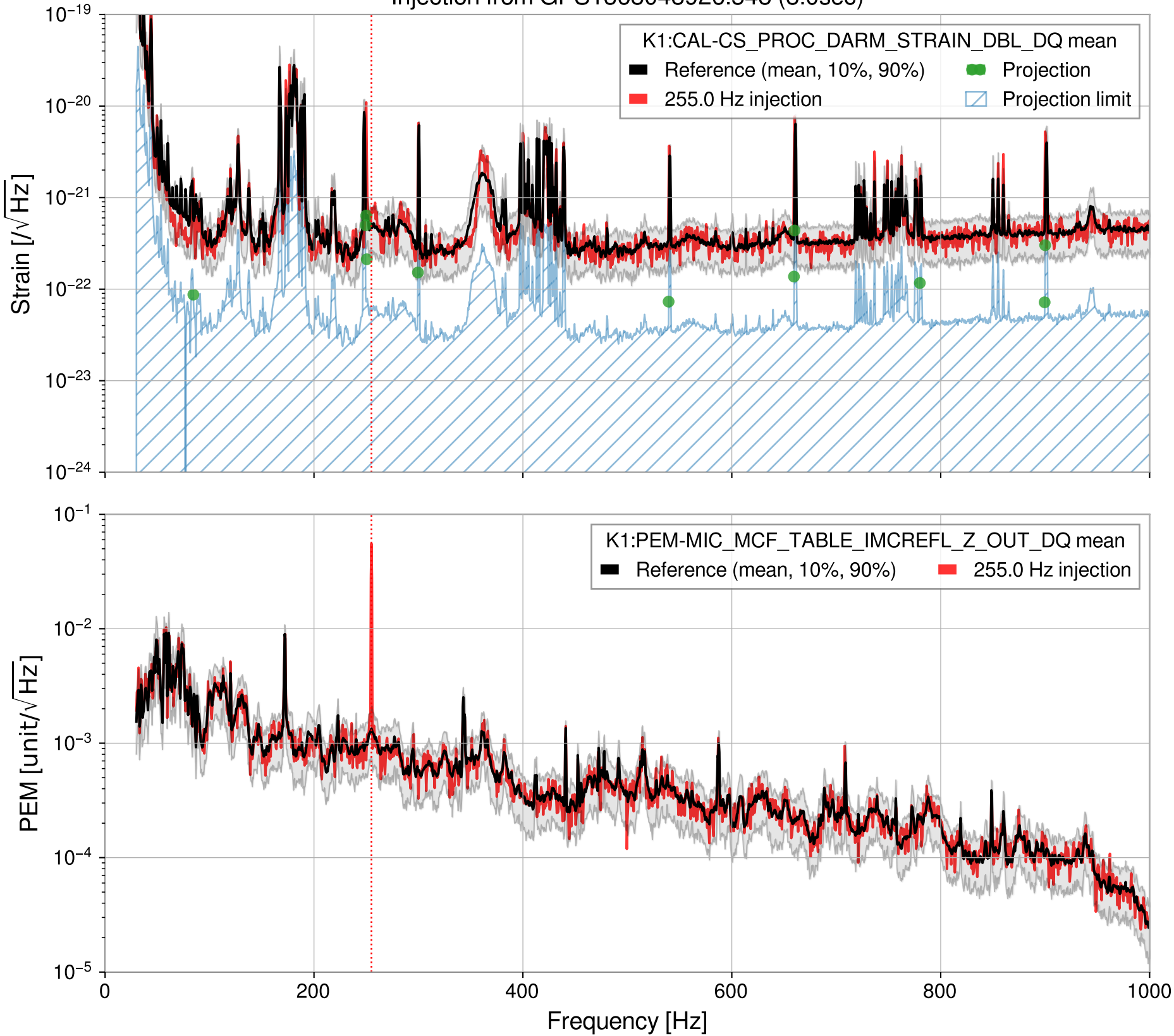
Injection from GPS1368048926.548 (8.0sec)
