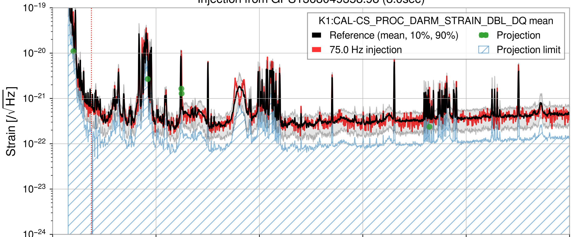
Injection from GPS1368049358.98 (8.0sec)
