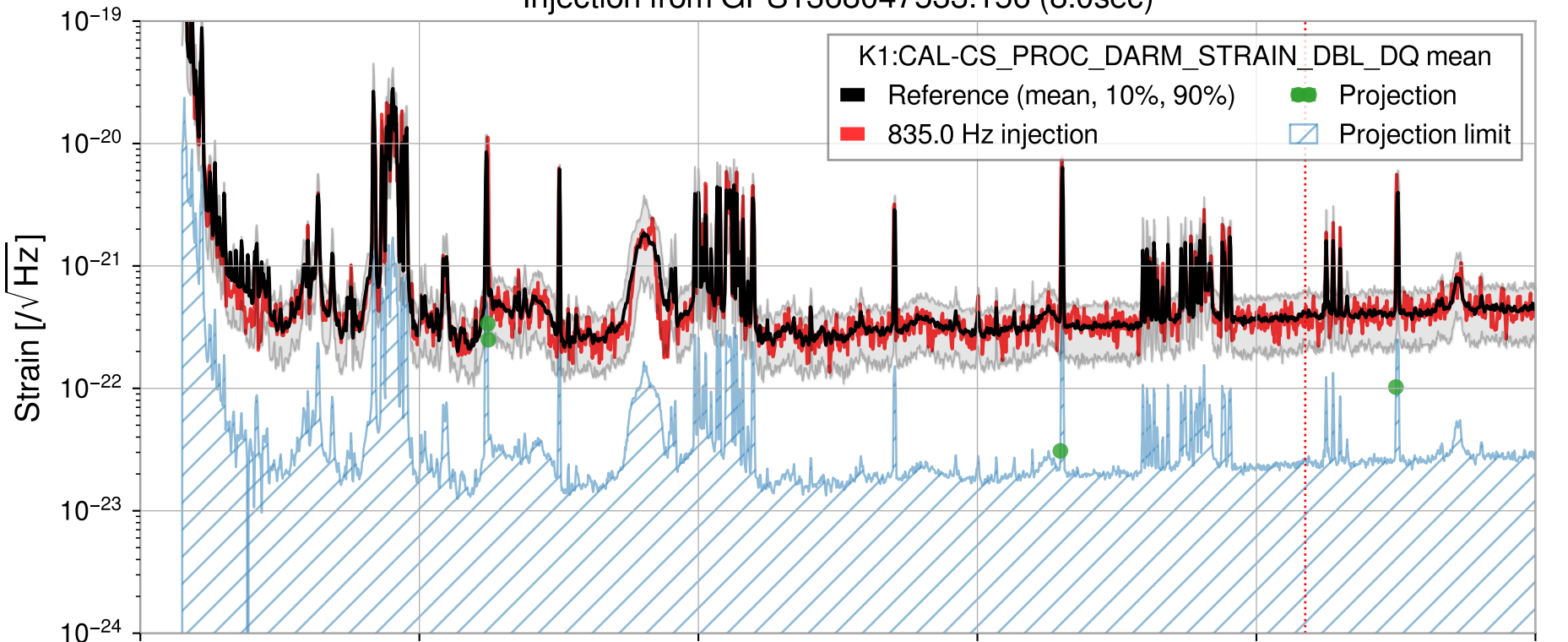
Injection from GPS1368047533.156 (8.0sec)
