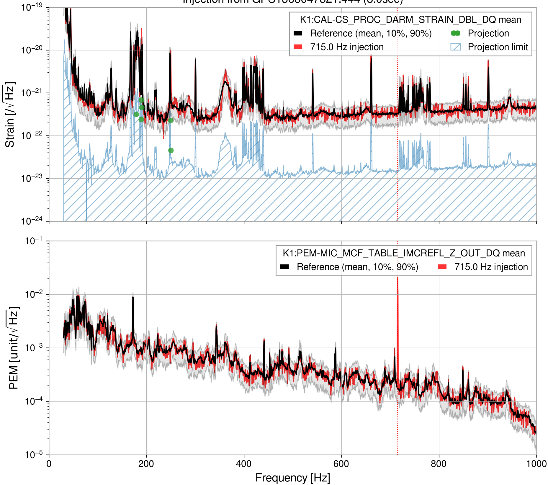
Injection from GPS1368047821.444 (8.0sec)
