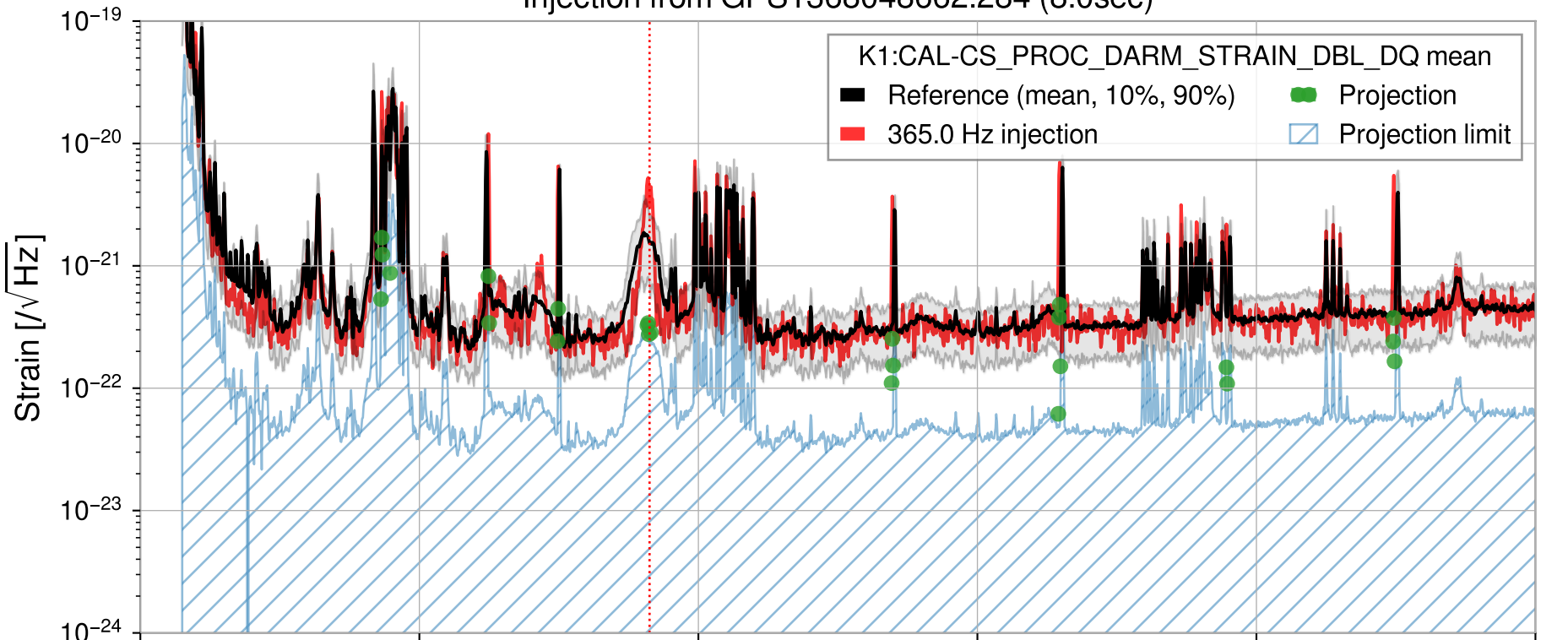
Injection from GPS1368048662.284 (8.0sec)
