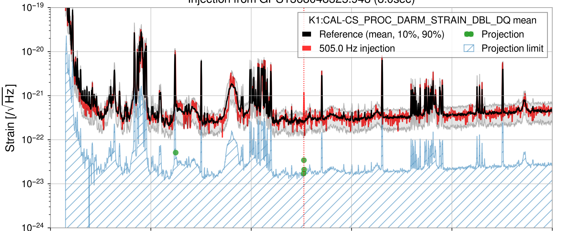
Injection from GPS1368048325.948 (8.0sec)
