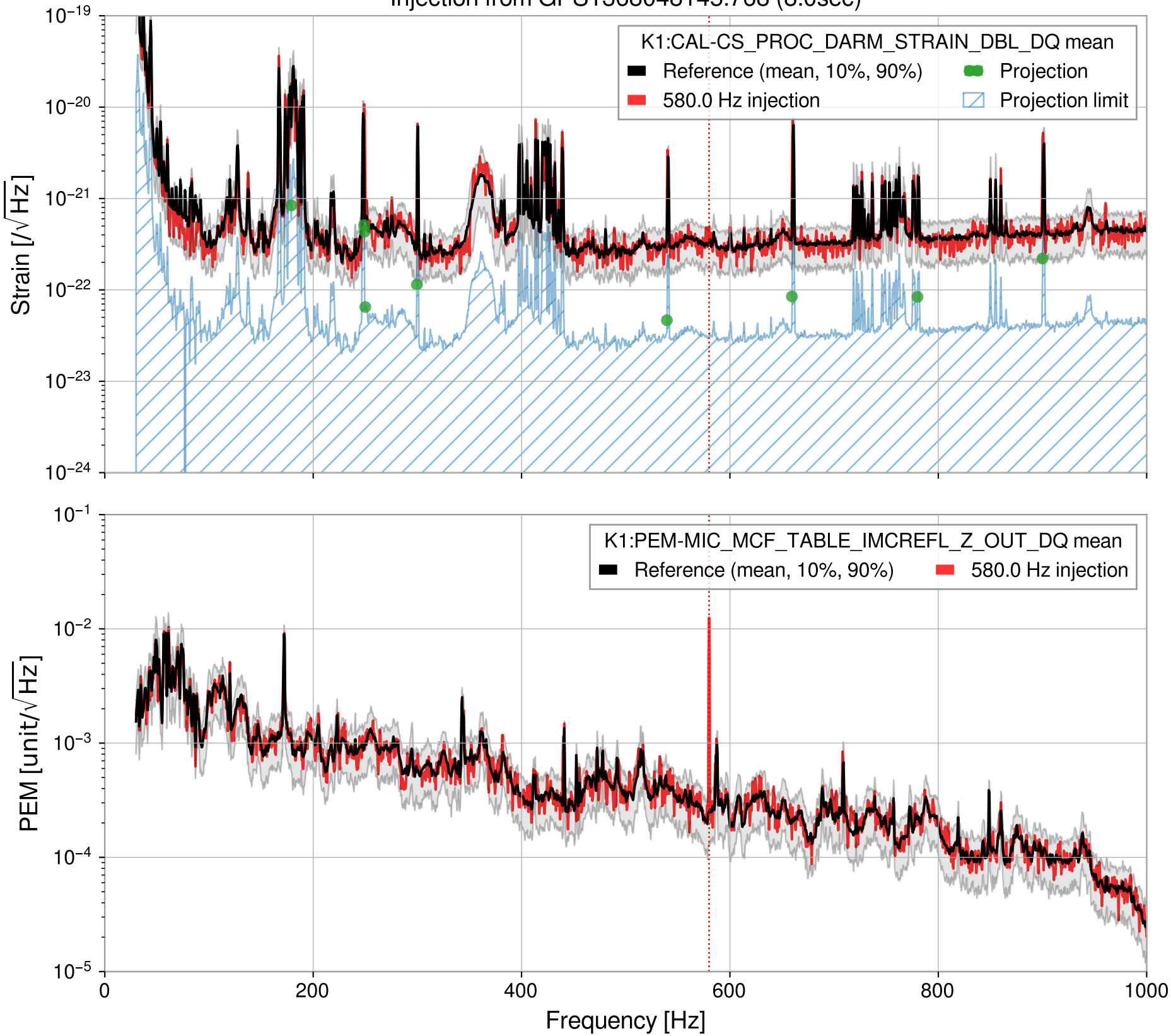
Injection from GPS1368048145.768 (8.0sec)
