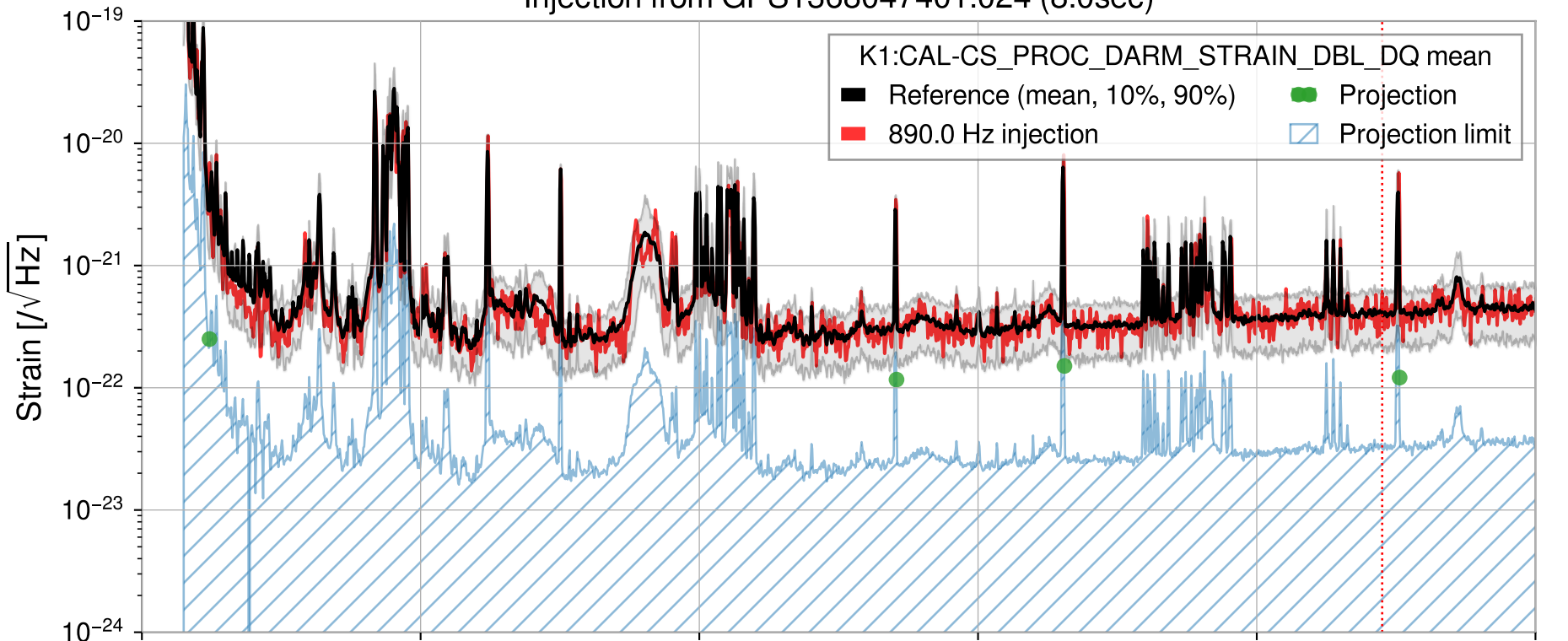
Injection from GPS1368047401.024 (8.0sec)
