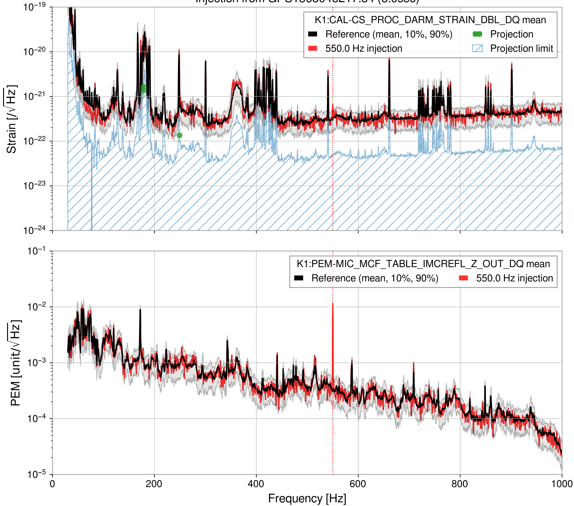
Injection from GPS1368048217.84 (8.0sec)
