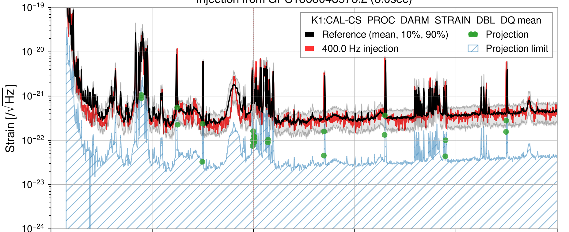
Injection from GPS1368048578.2 (8.0sec)
