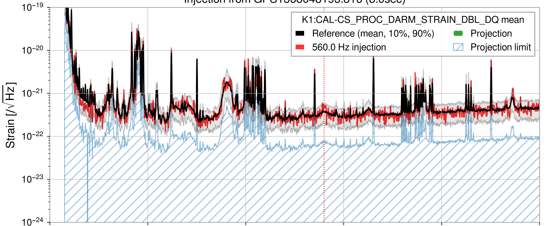
Injection from GPS1368048193.816 (8.0sec)
