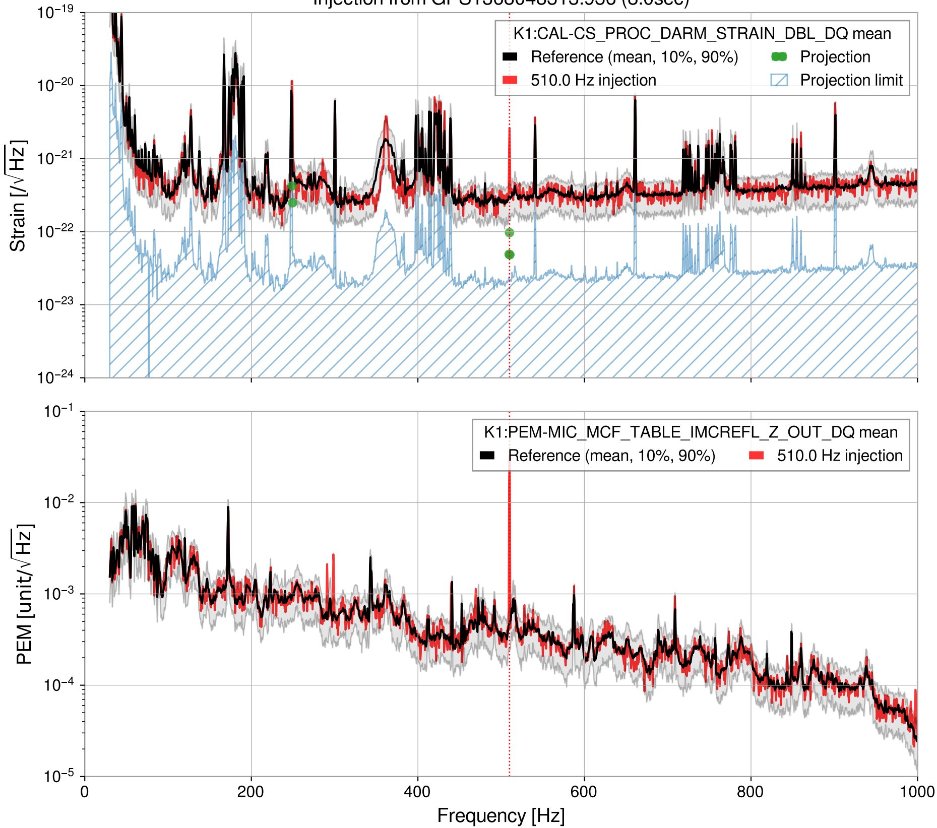
Injection from GPS1368048313.936 (8.0sec)
