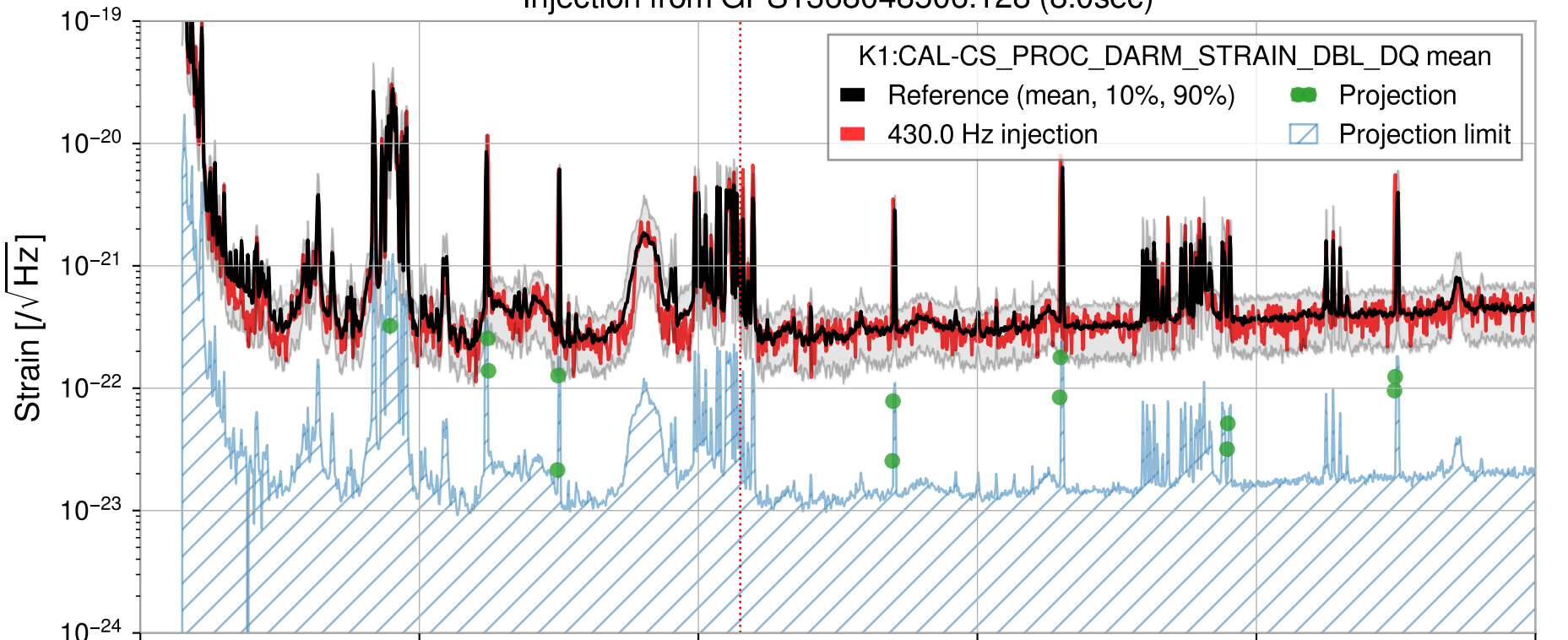
Injection from GPS1368048506.128 (8.0sec)
