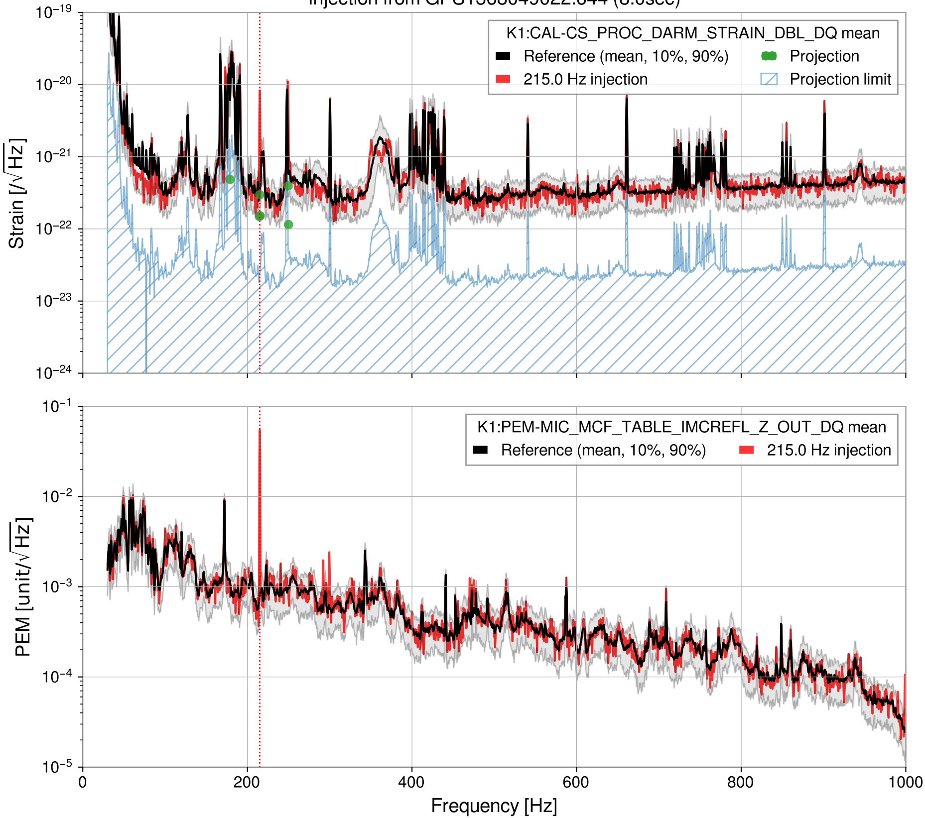
Injection from GPS1368049022.644 (8.0sec)
