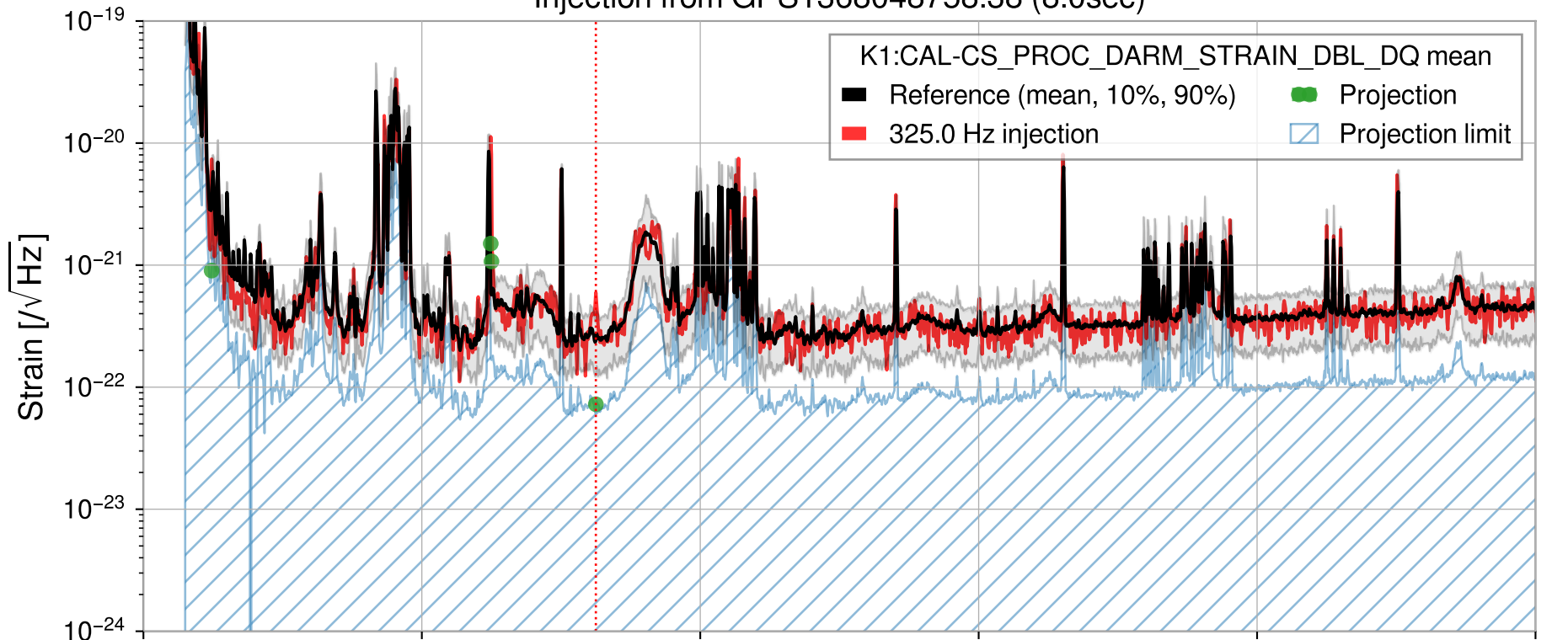
Injection from GPS1368048758.38 (8.0sec)
