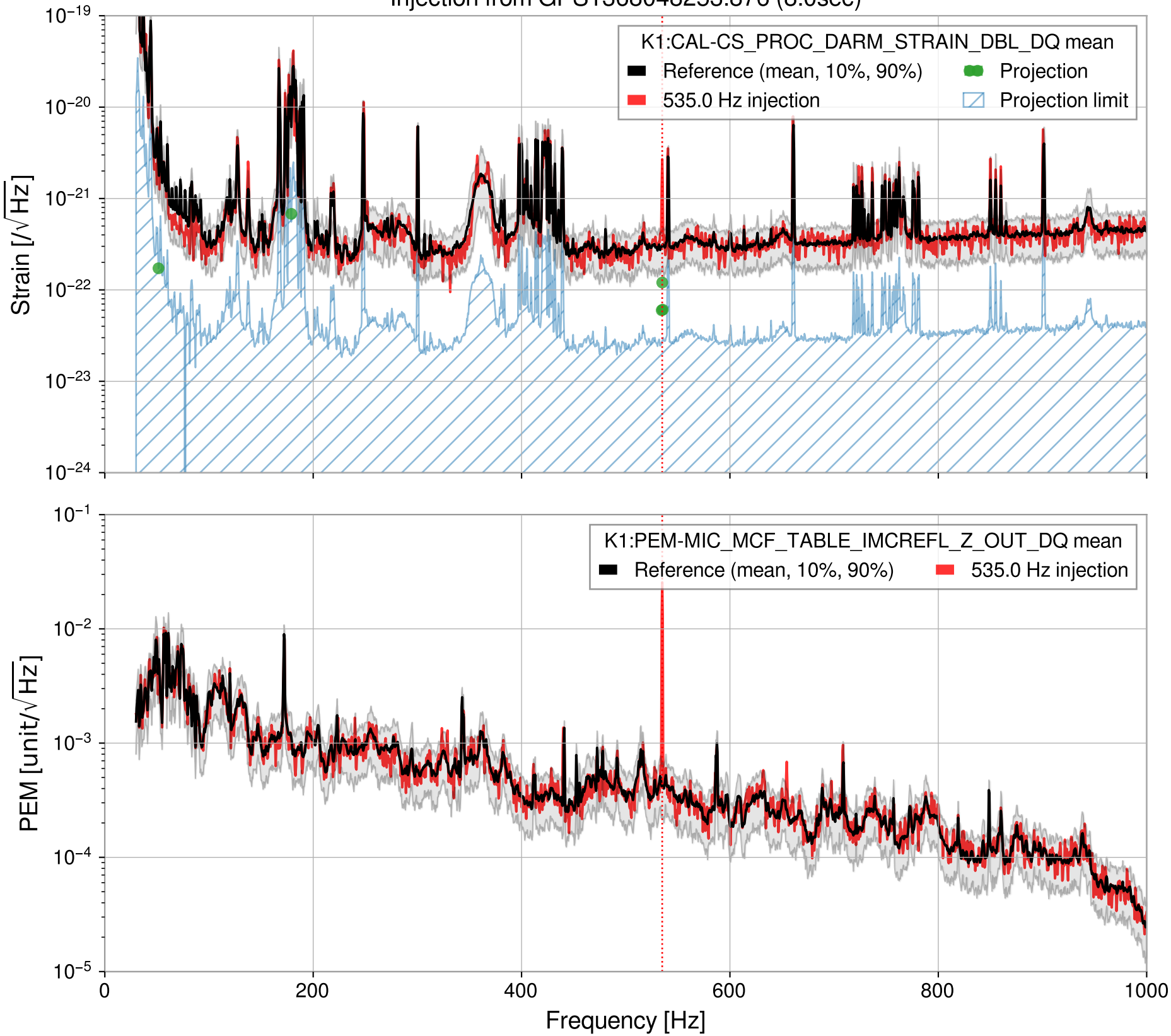
Injection from GPS1368048253.876 (8.0sec)
