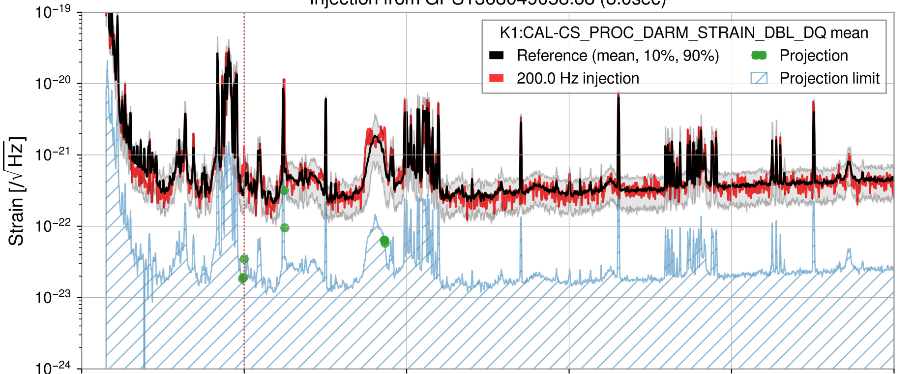
Injection from GPS1368049058.68 (8.0sec)
