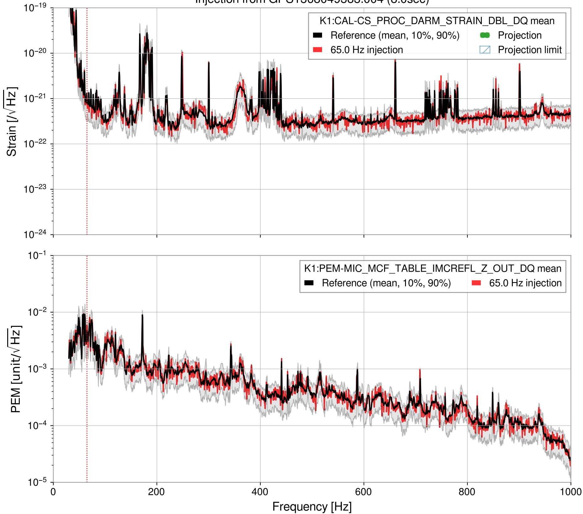
Injection from GPS1368049383.004 (8.0sec)
