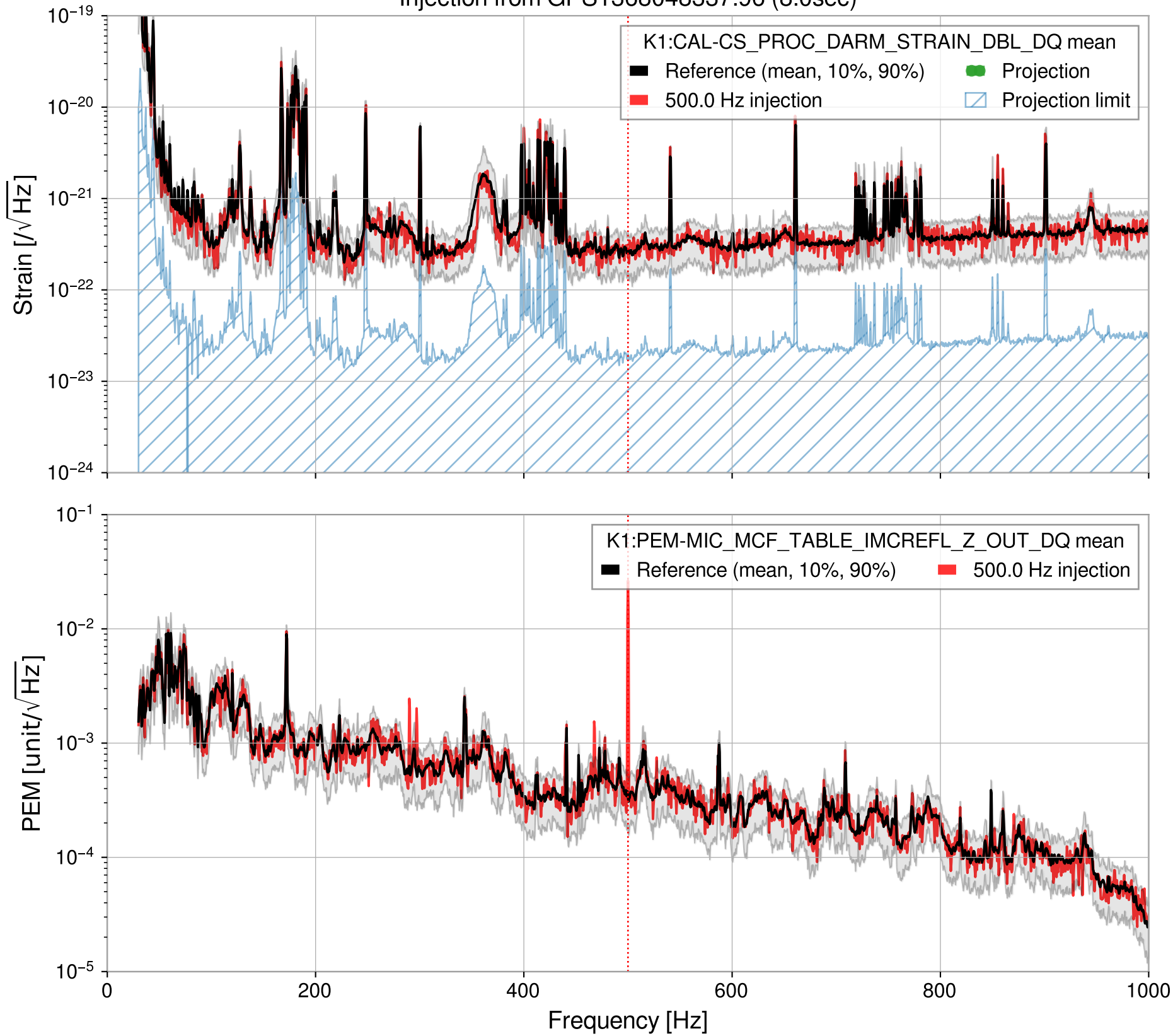
Injection from GPS1368048337.96 (8.0sec)
