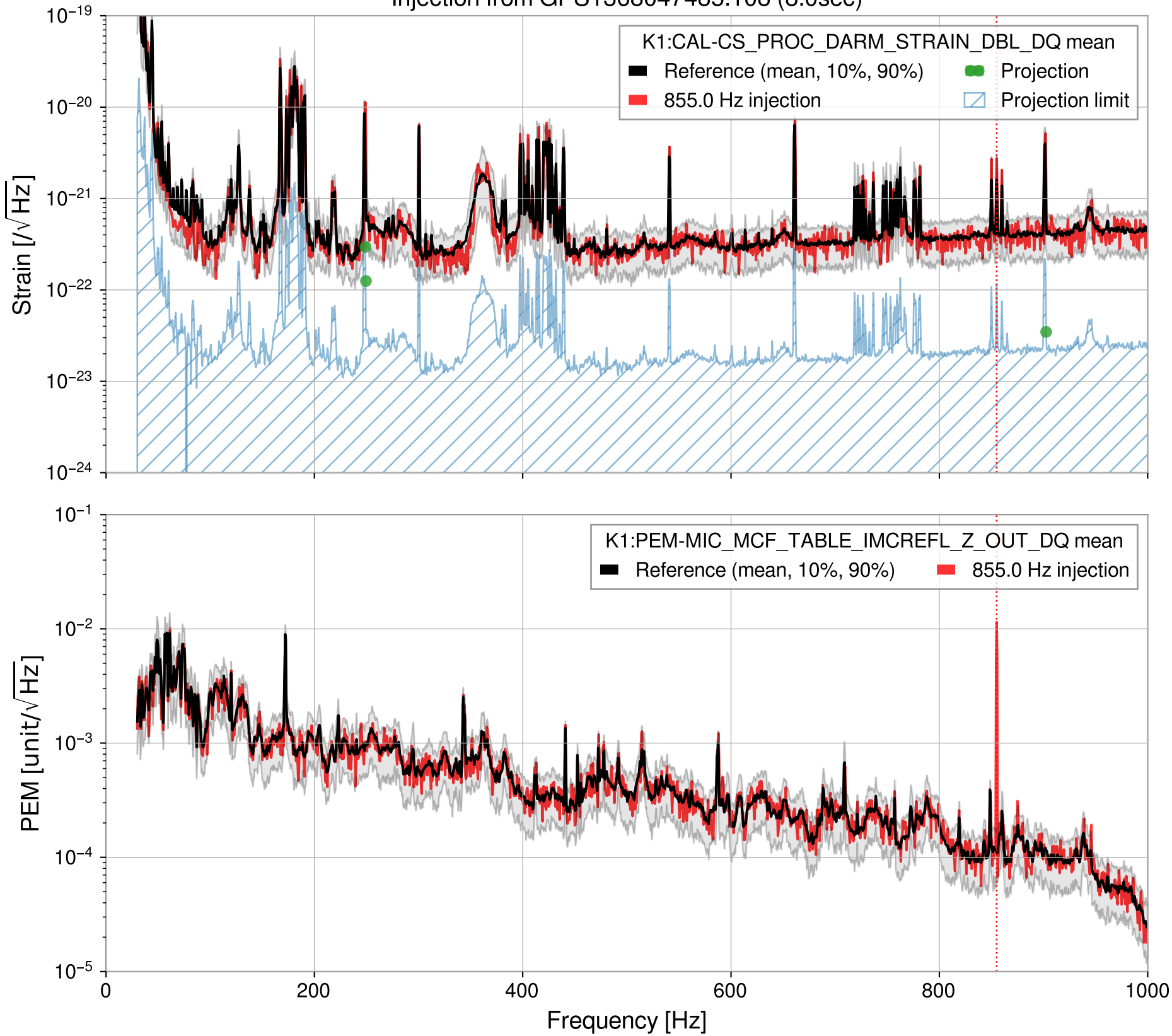
Injection from GPS1368047485.108 (8.0sec)
