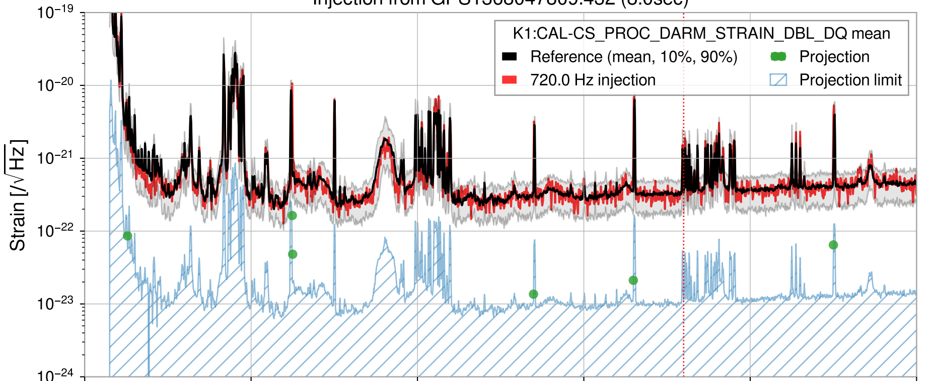
Injection from GPS1368047809.432 (8.0sec)
