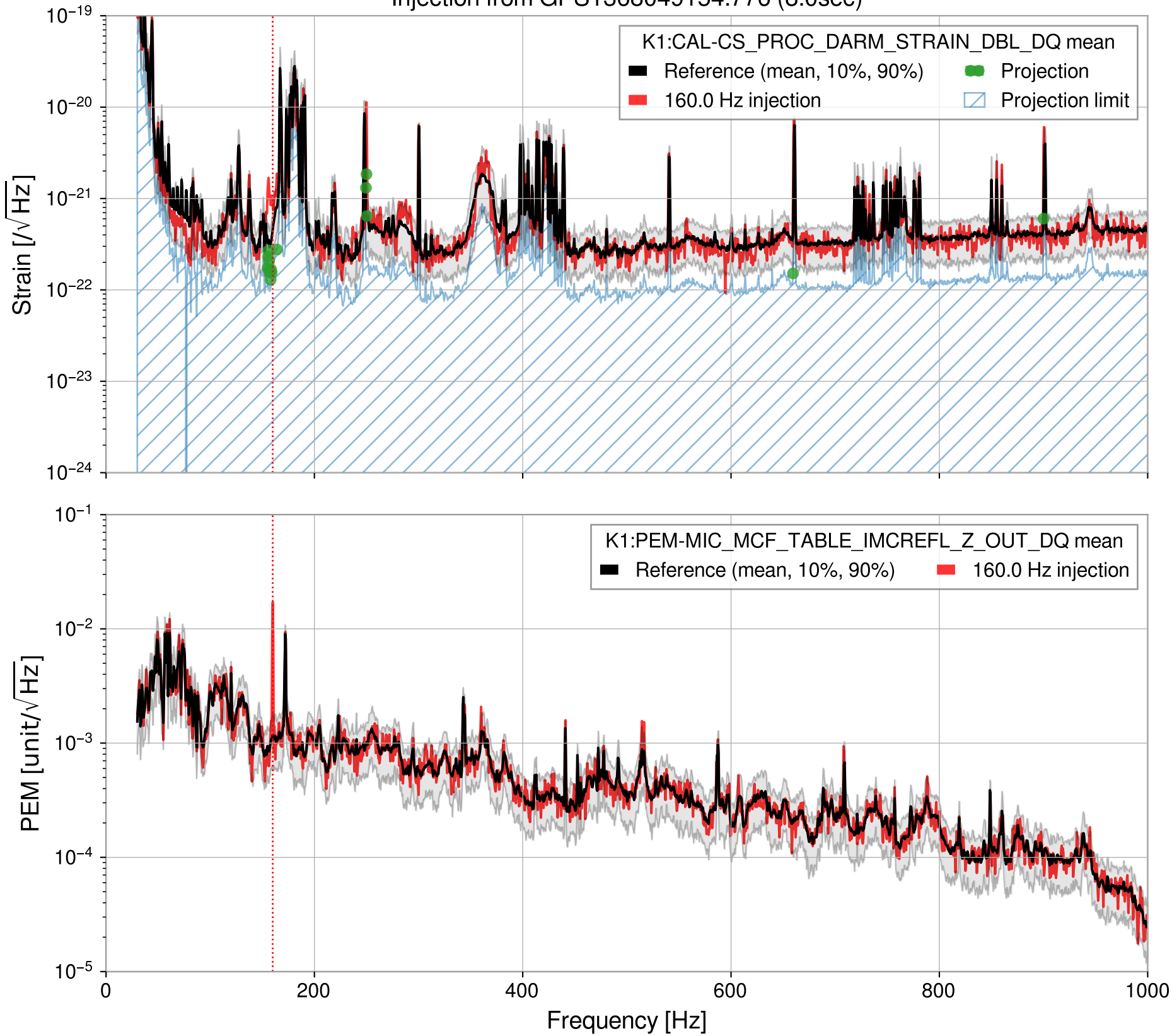
Injection from GPS1368049154.776 (8.0sec)
