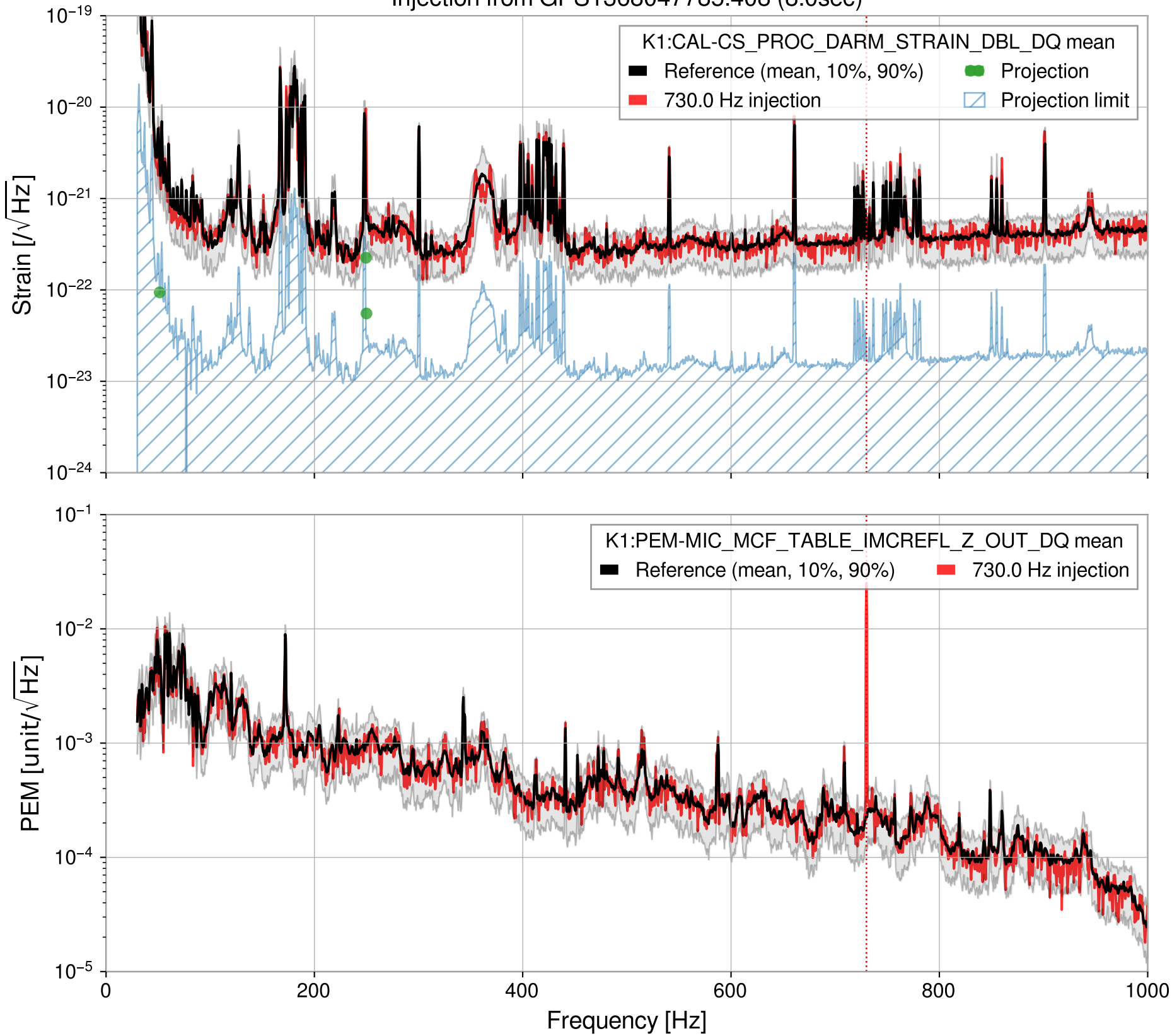
Injection from GPS1368047785.408 (8.0sec)
