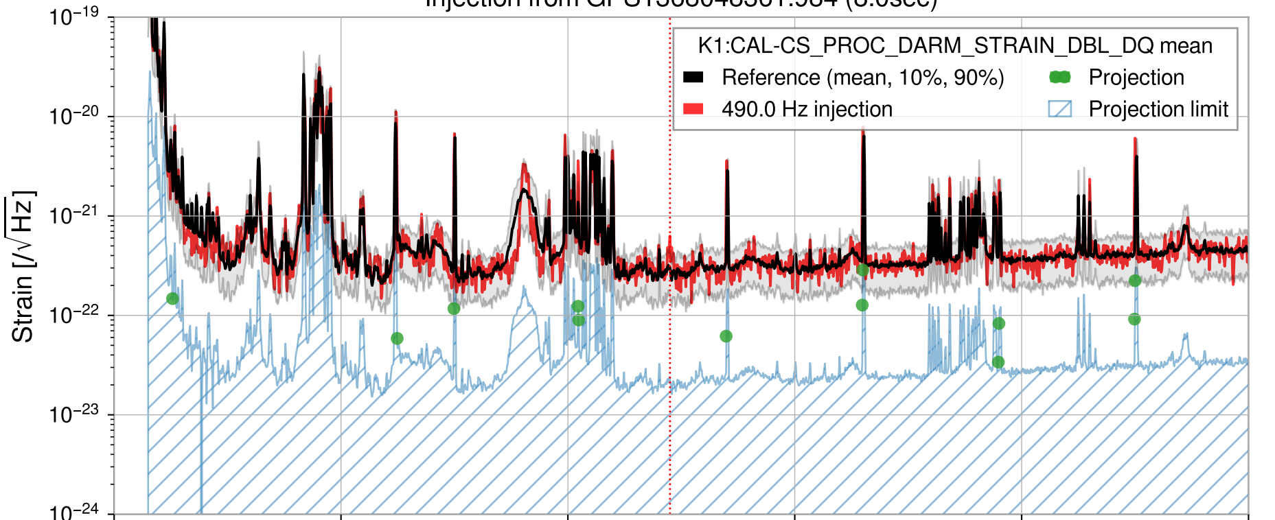
Injection from GPS1368048361.984 (8.0sec)
