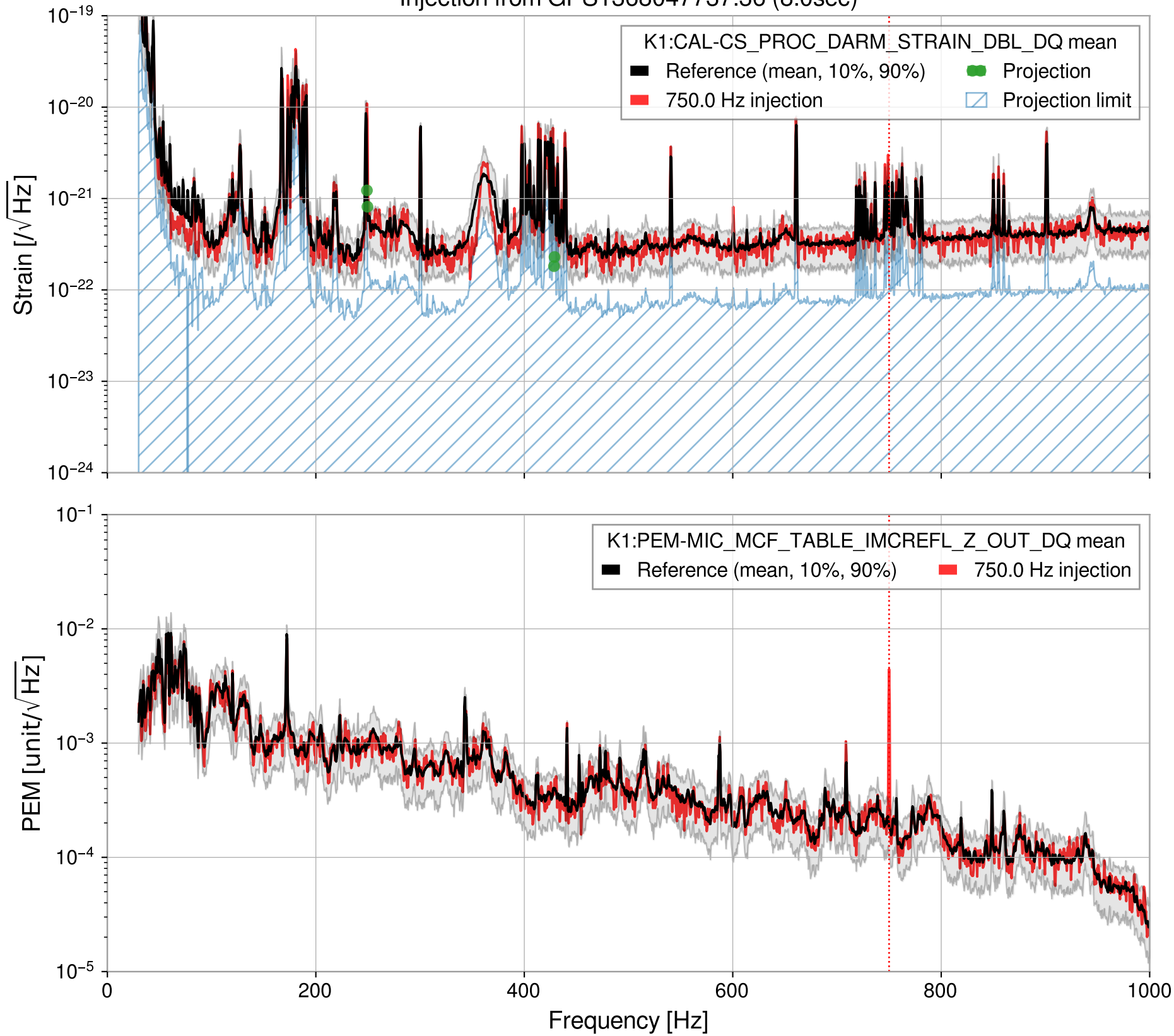
Injection from GPS1368047737.36 (8.0sec)
