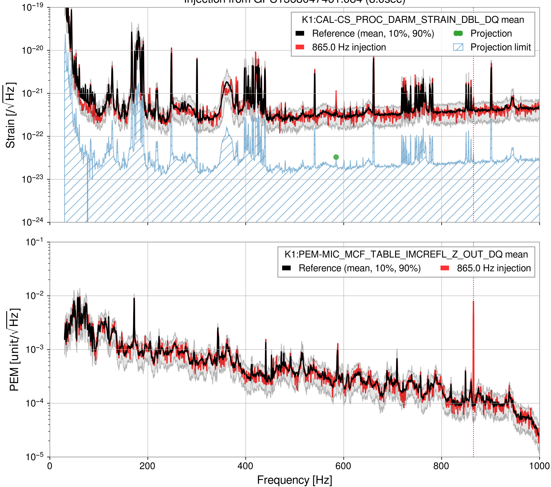
Injection from GPS1368047461.084 (8.0sec)
