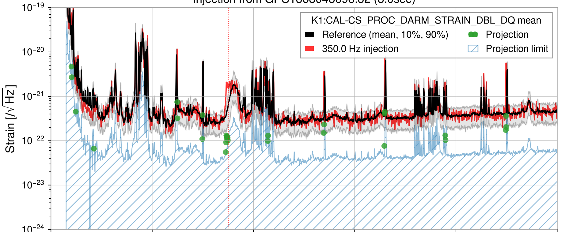
Injection from GPS1368048698.32 (8.0sec)
