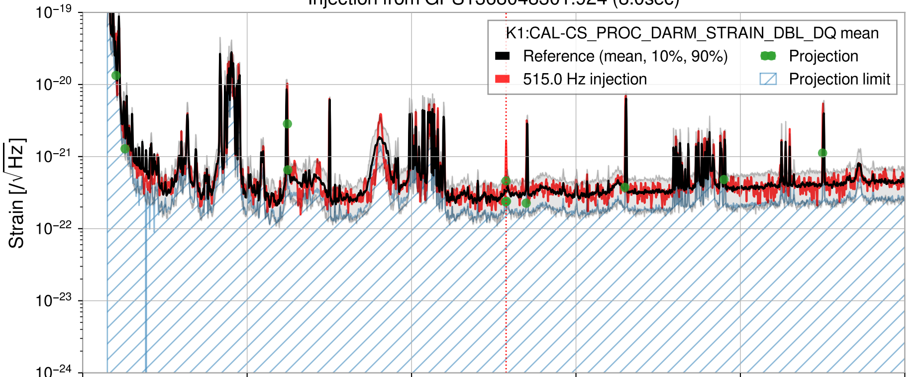
Injection from GPS1368048301.924 (8.0sec)
