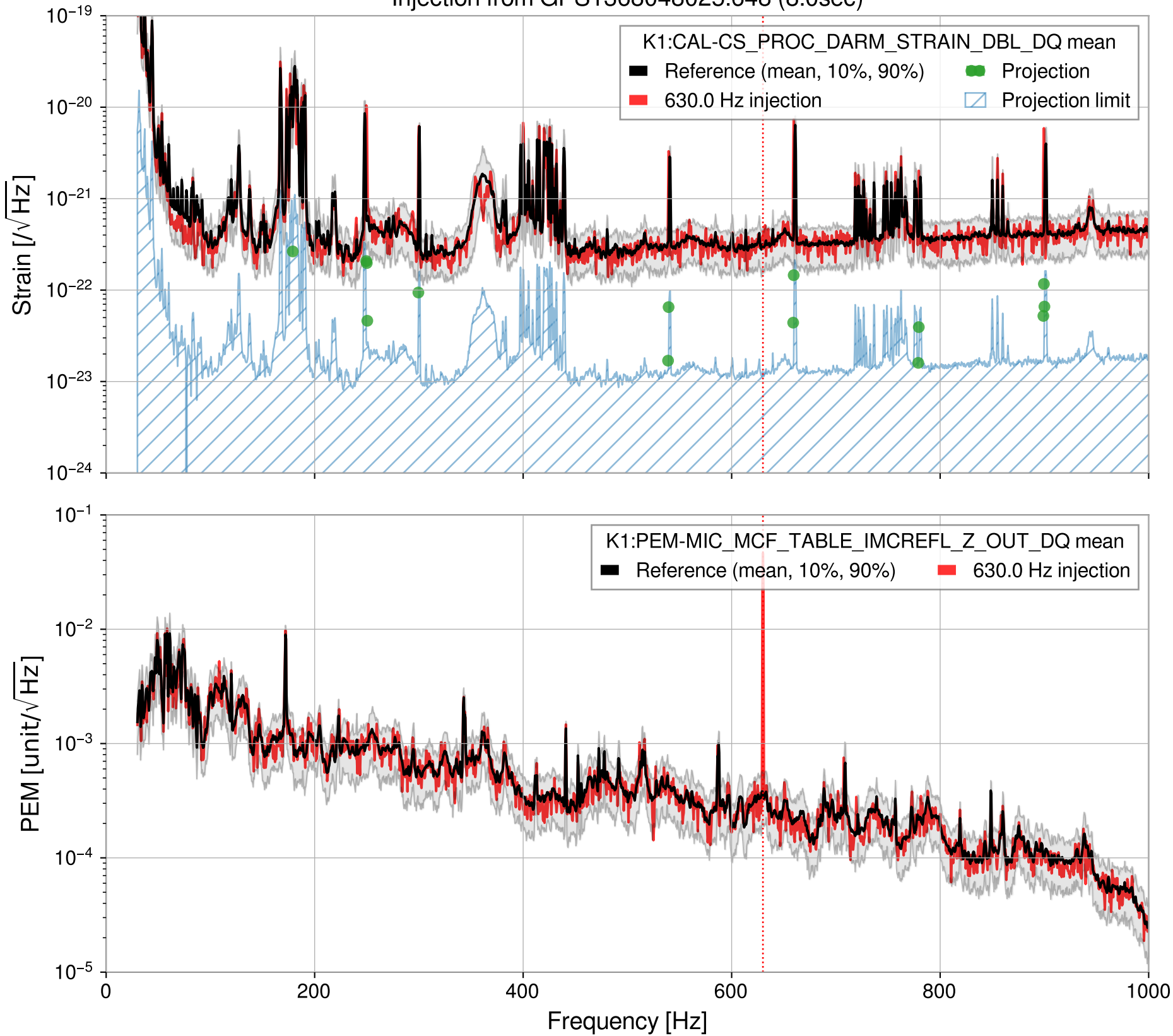
Injection from GPS1368048025.648 (8.0sec)
