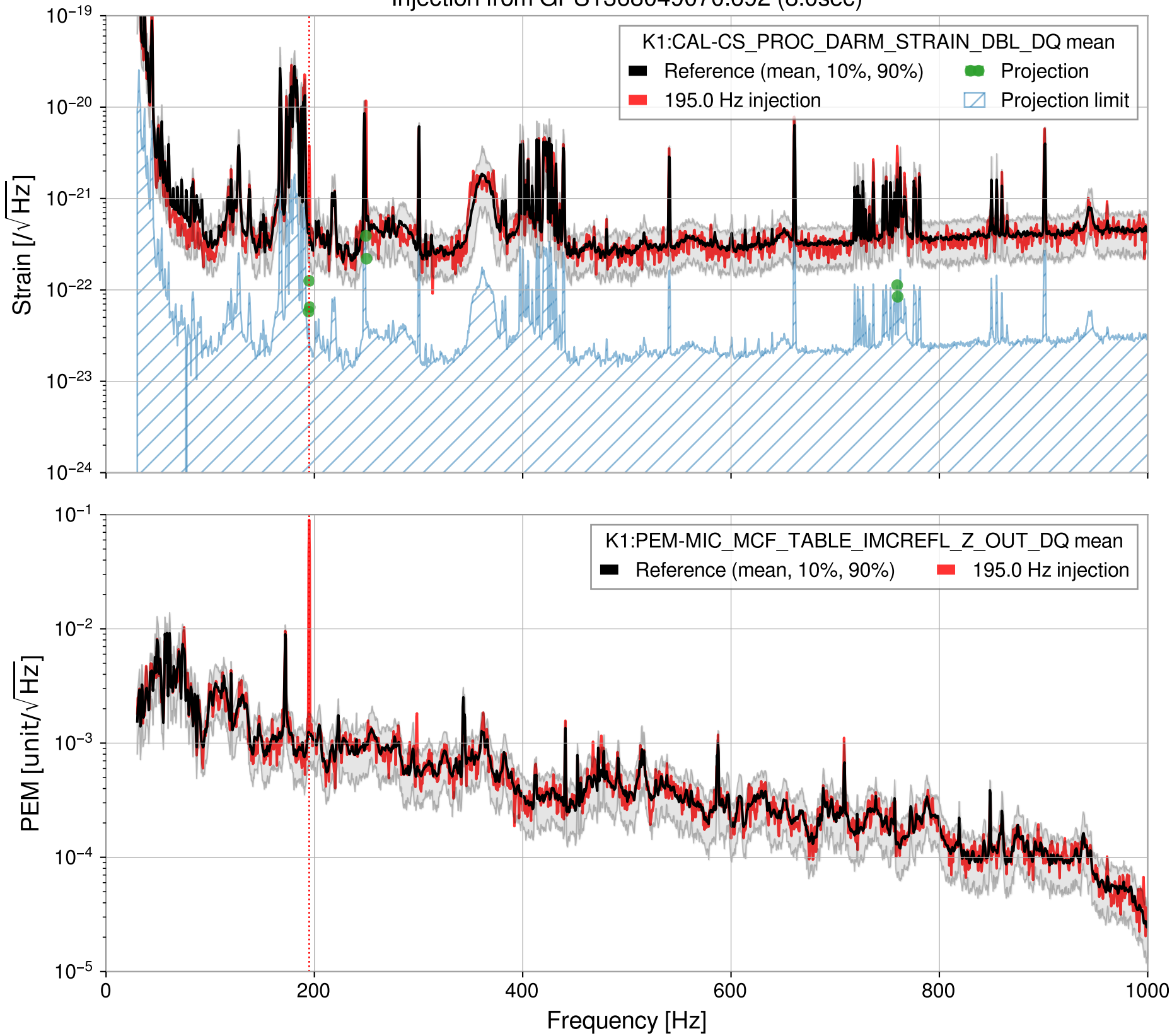
Injection from GPS1368049070.692 (8.0sec)
