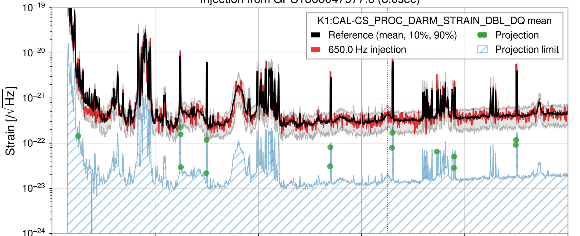
Injection from GPS1368047977.6 (8.0sec)
