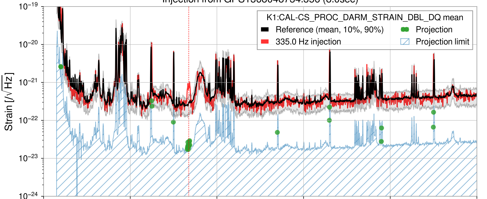
Injection from GPS1368048734.356 (8.0sec)
