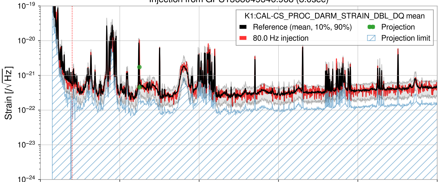
Injection from GPS1368049346.968 (8.0sec)
