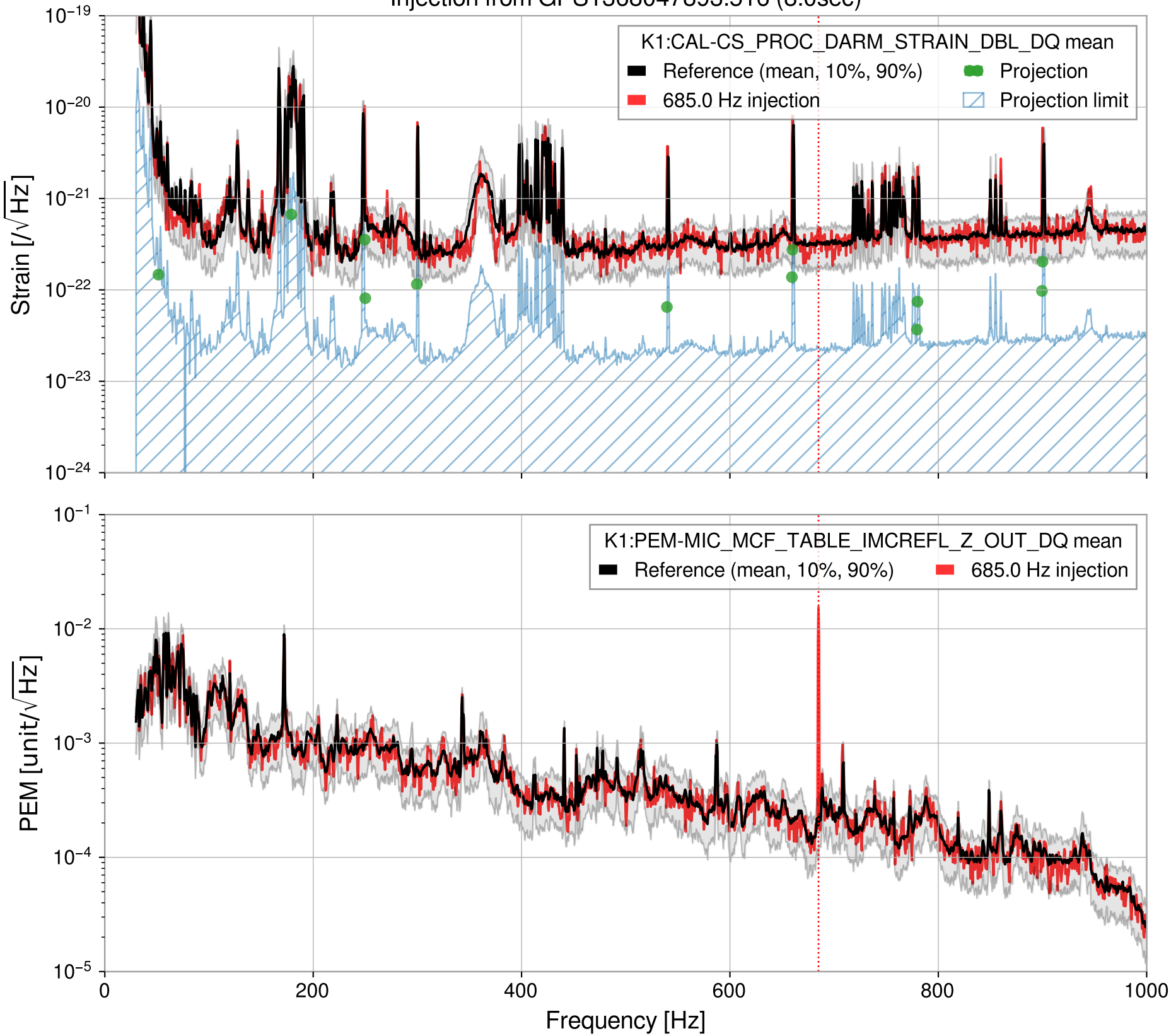
Injection from GPS1368047893.516 (8.0sec)
