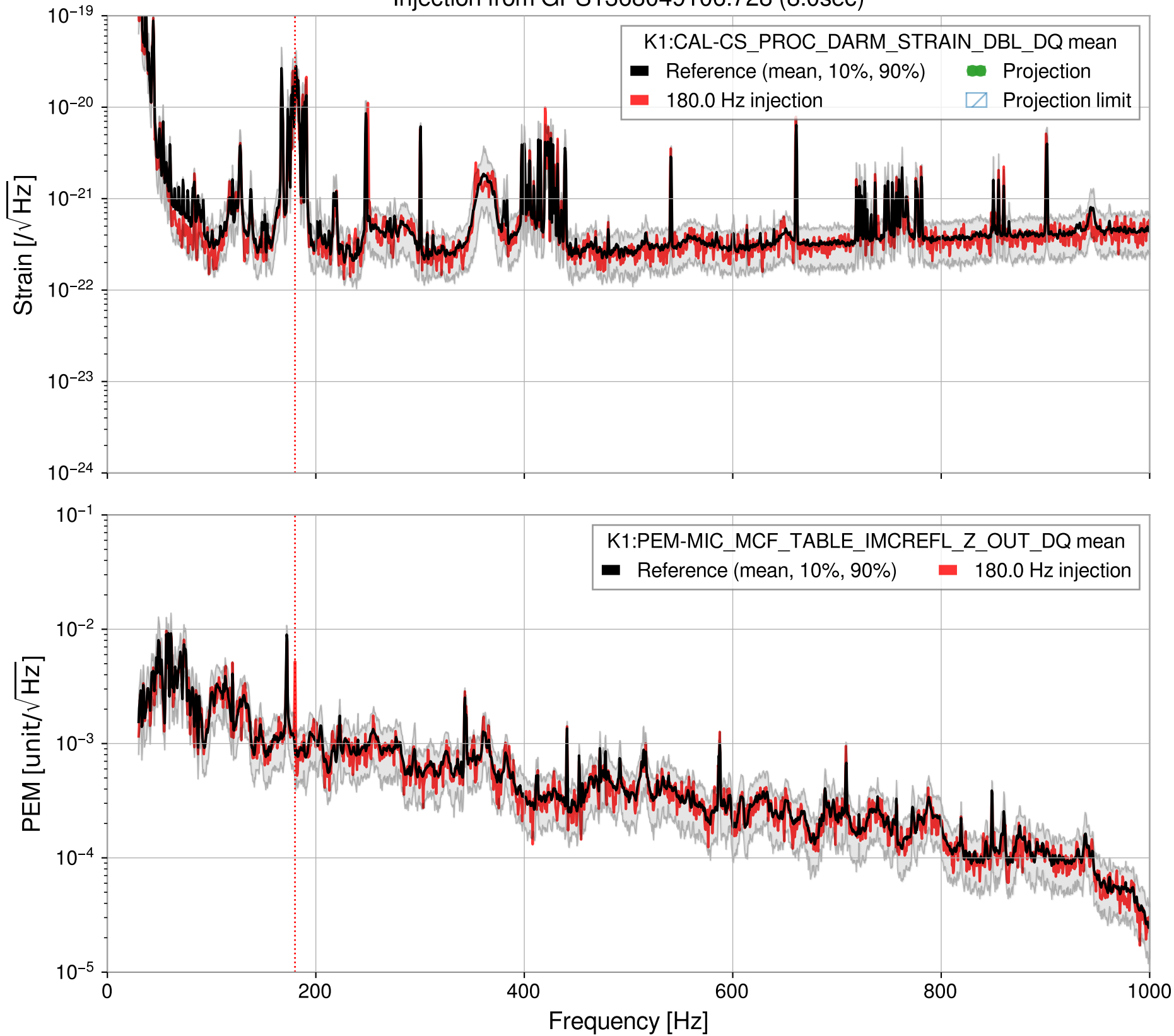
Injection from GPS1368049106.728 (8.0sec)
