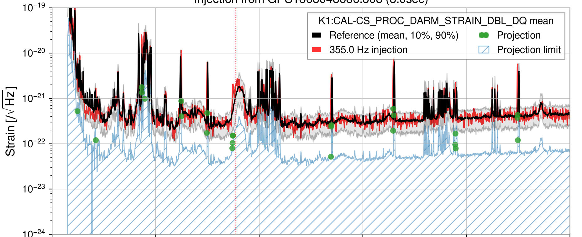
Injection from GPS1368048686.308 (8.0sec)
