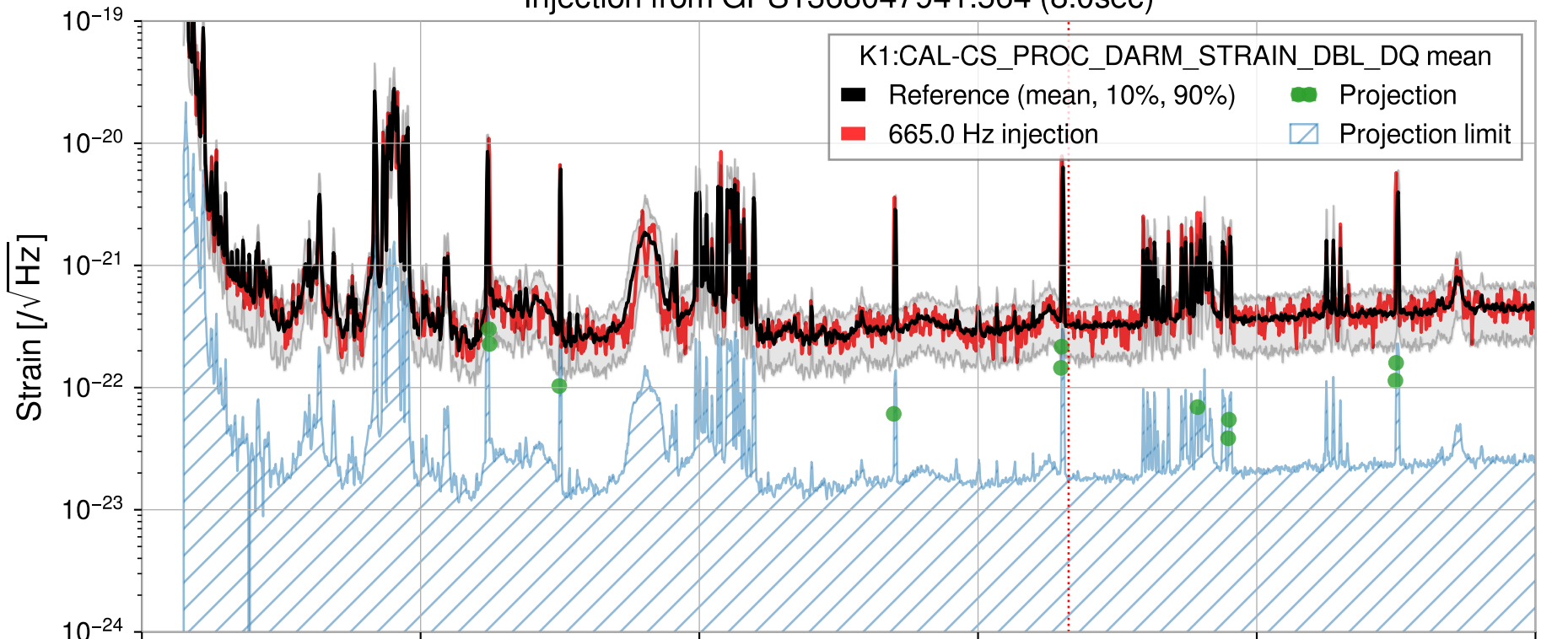
Injection from GPS1368047941.564 (8.0sec)
