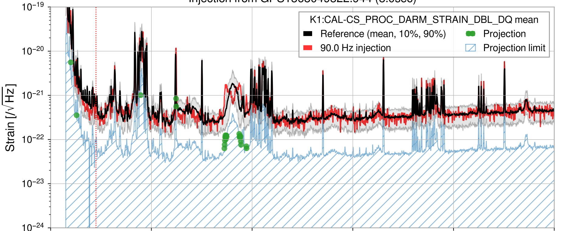
Injection from GPS1368049322.944 (8.0sec)
