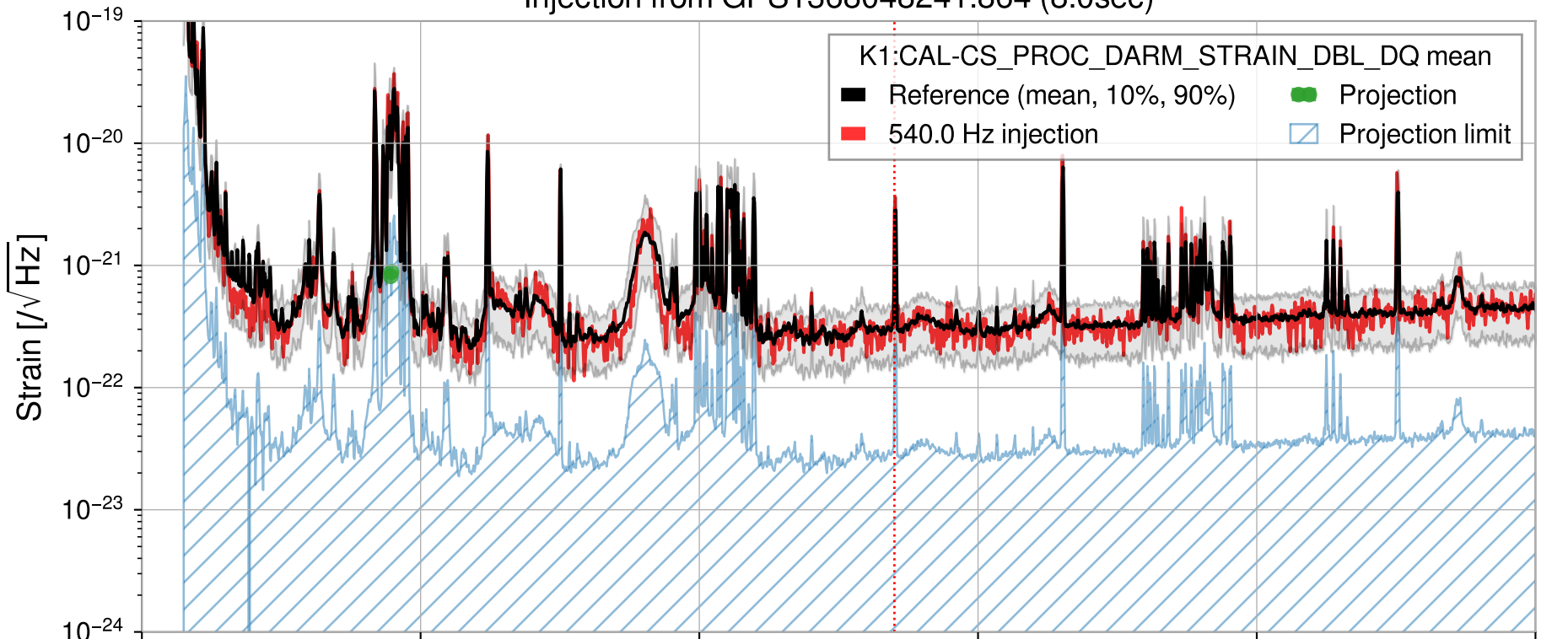
Injection from GPS1368048241.864 (8.0sec)
