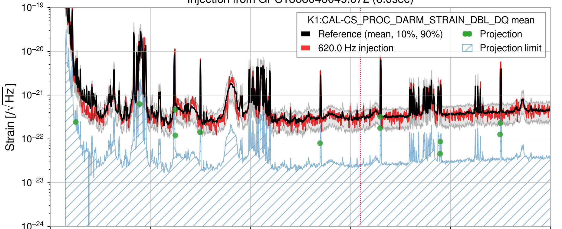
Injection from GPS1368048049.672 (8.0sec)
