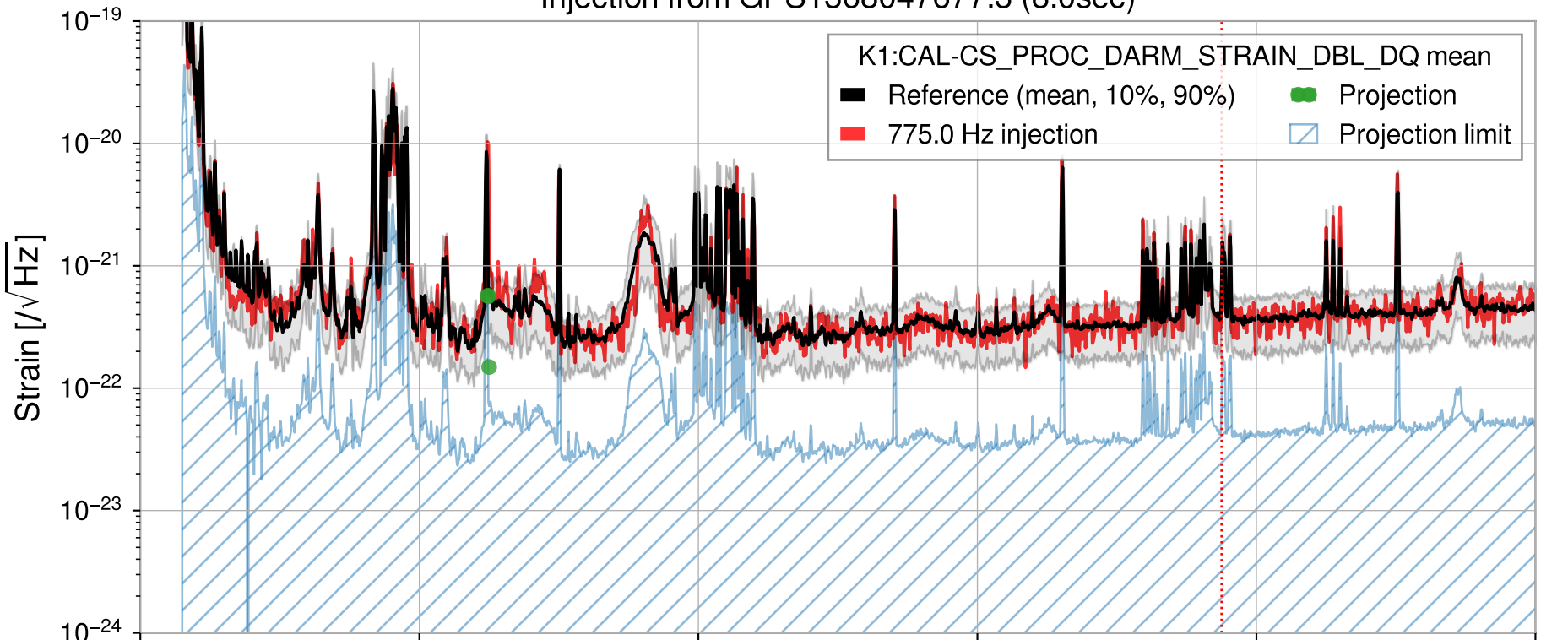
Injection from GPS1368047677.3 (8.0sec)
