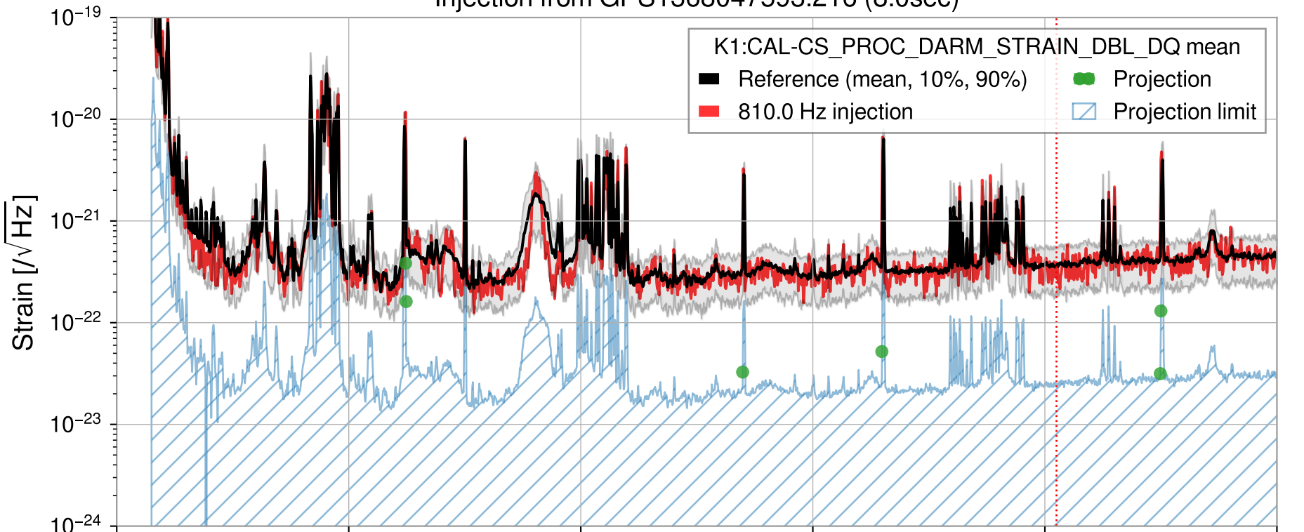
Injection from GPS1368047593.216 (8.0sec)
