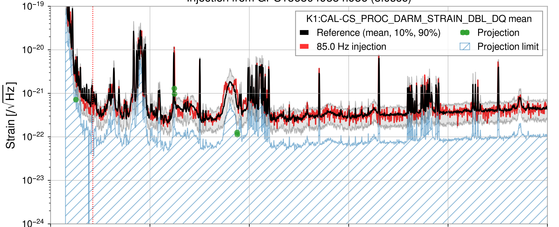
Injection from GPS1368049334.956 (8.0sec)
