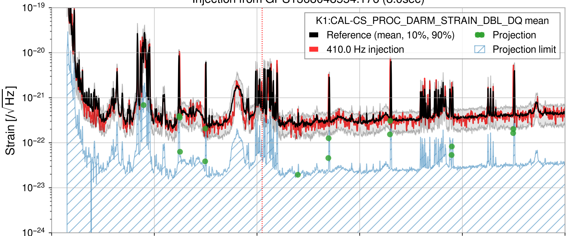
Injection from GPS1368048554.176 (8.0sec)
