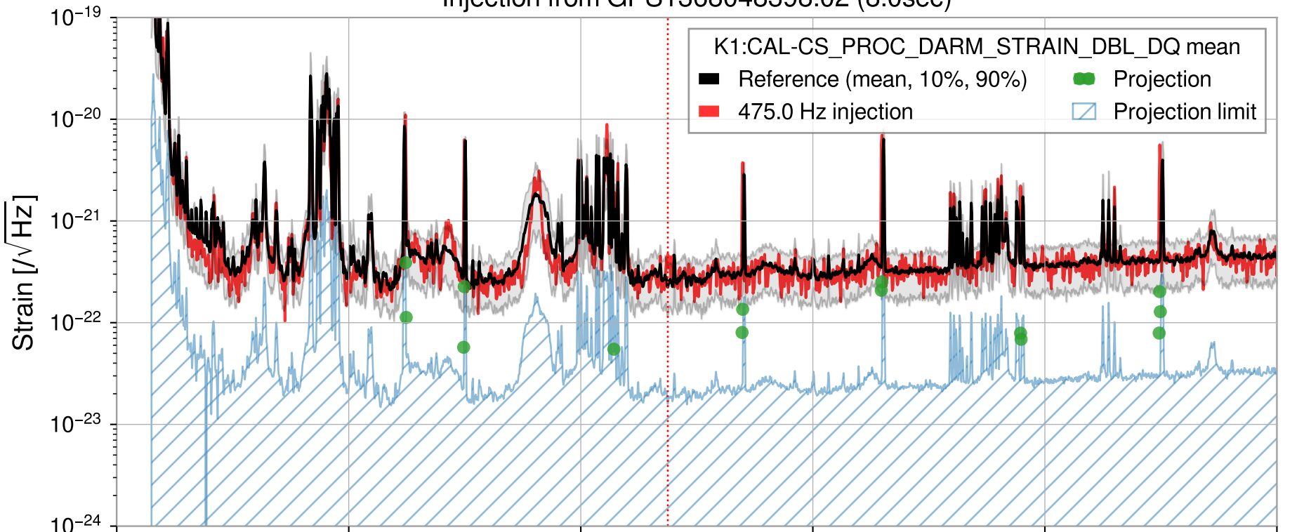
Injection from GPS1368048398.02 (8.0sec)
