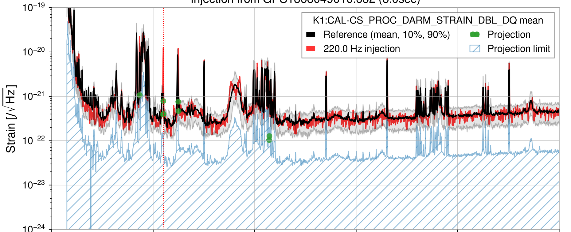
Injection from GPS1368049010.632 (8.0sec)
