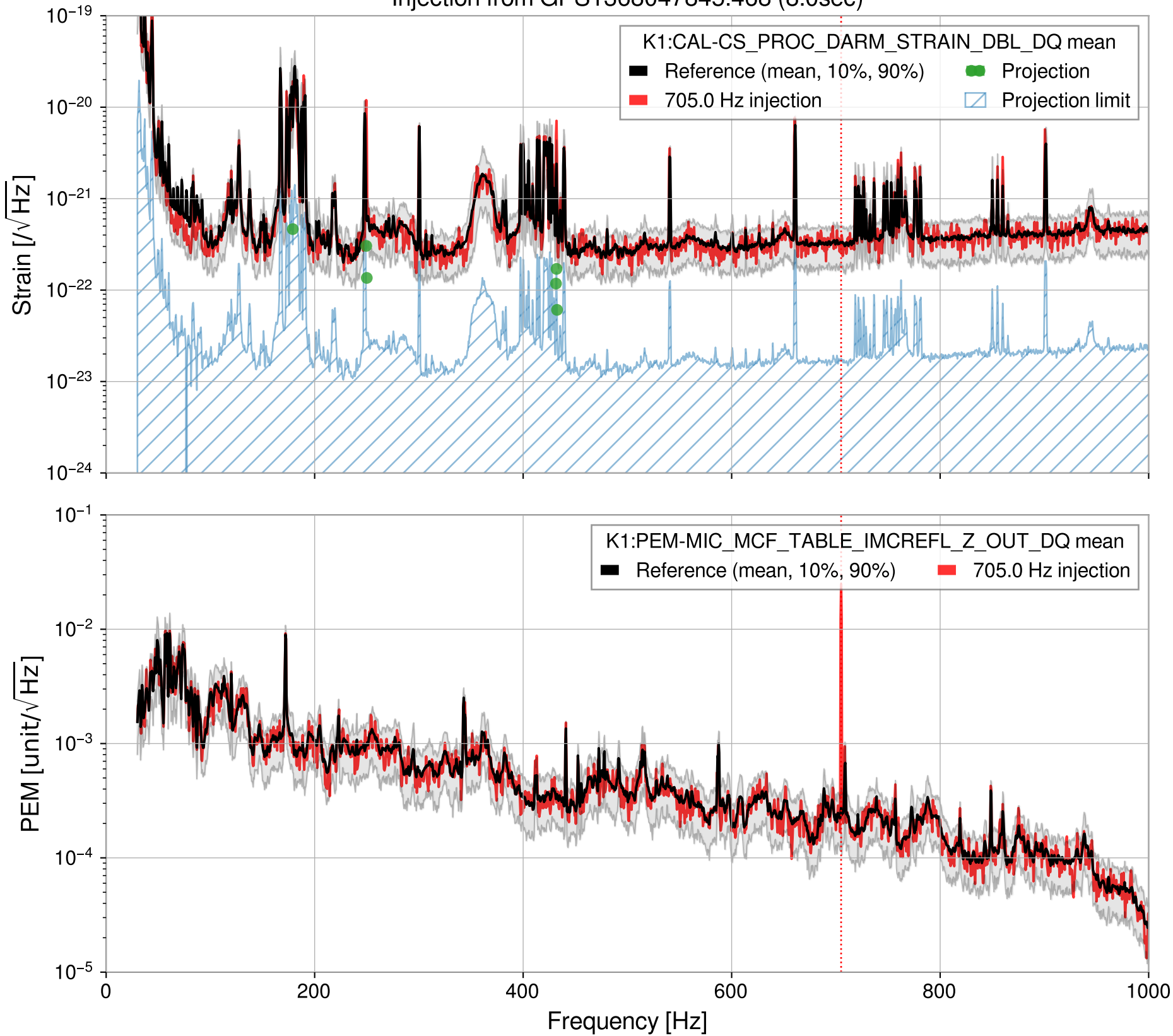
Injection from GPS1368047845.468 (8.0sec)
