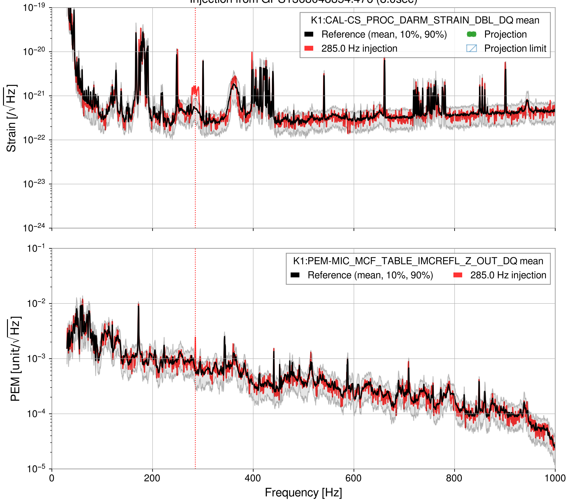
Injection from GPS1368048854.476 (8.0sec)
