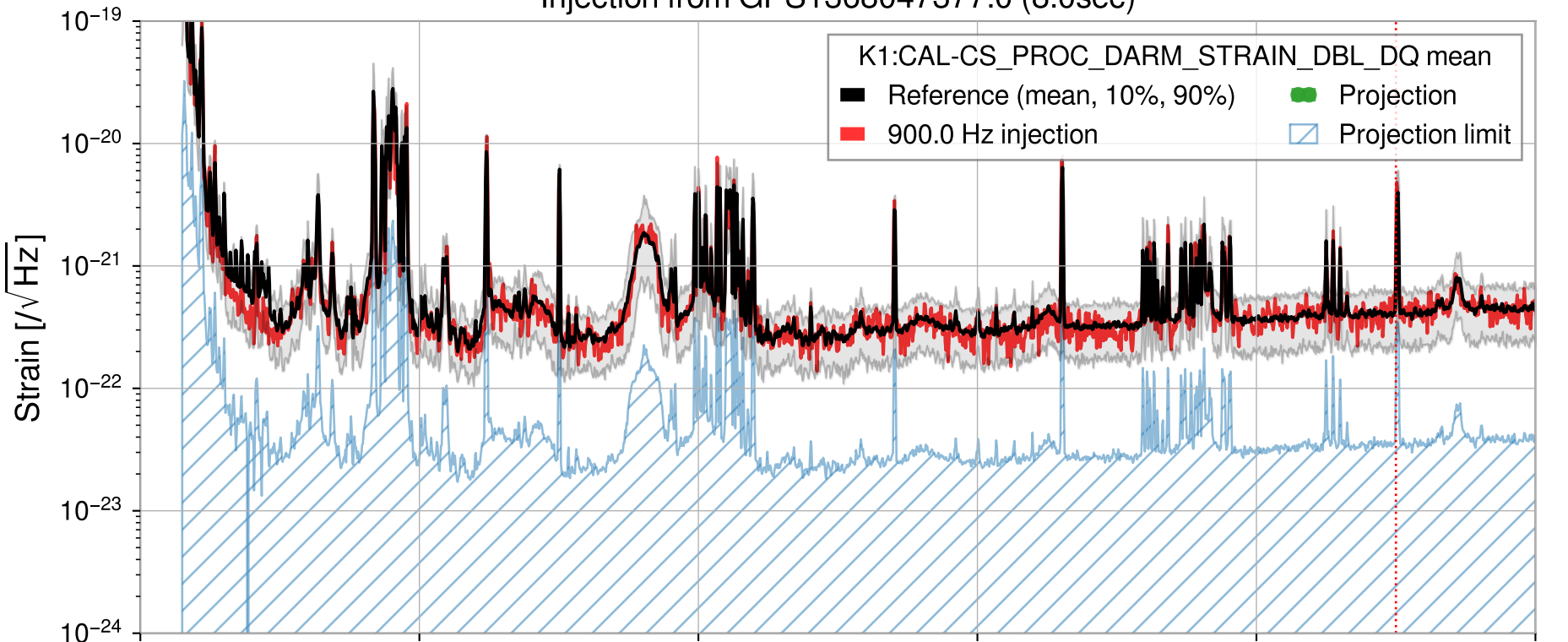
Injection from GPS1368047377.0 (8.0sec)
