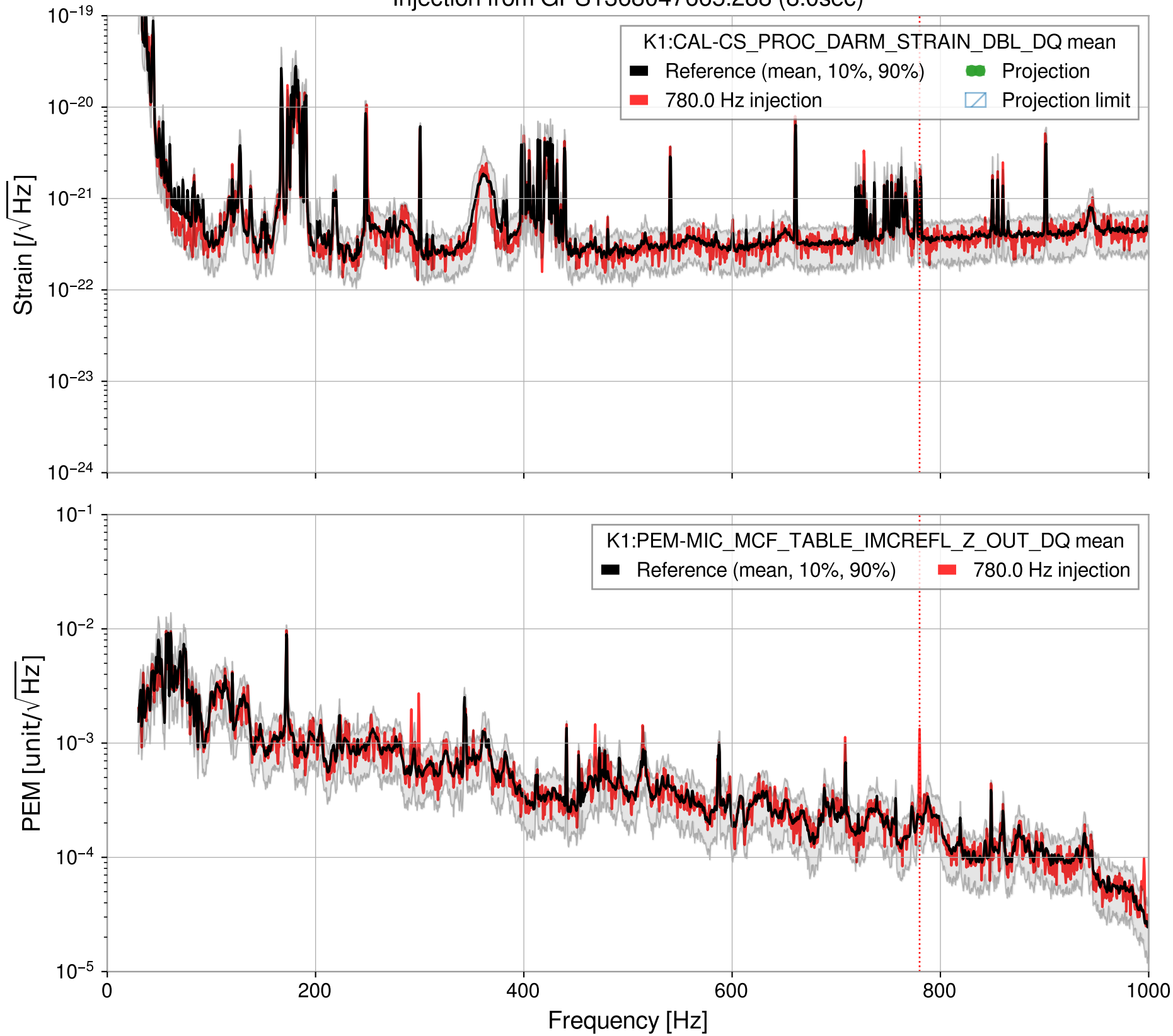
Injection from GPS1368047665.288 (8.0sec)
