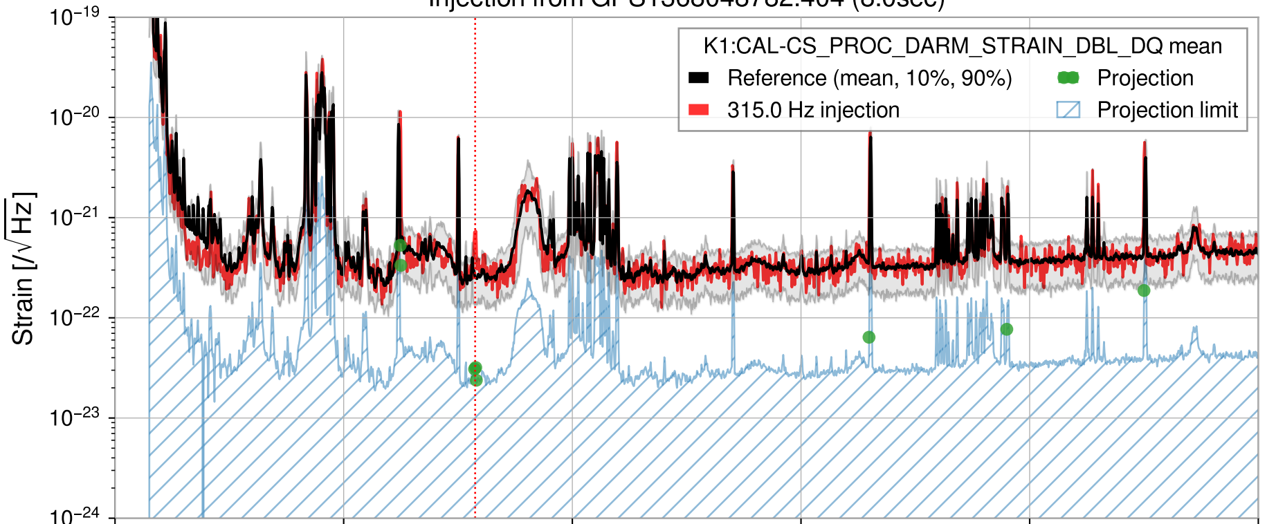
Injection from GPS1368048782.404 (8.0sec)
