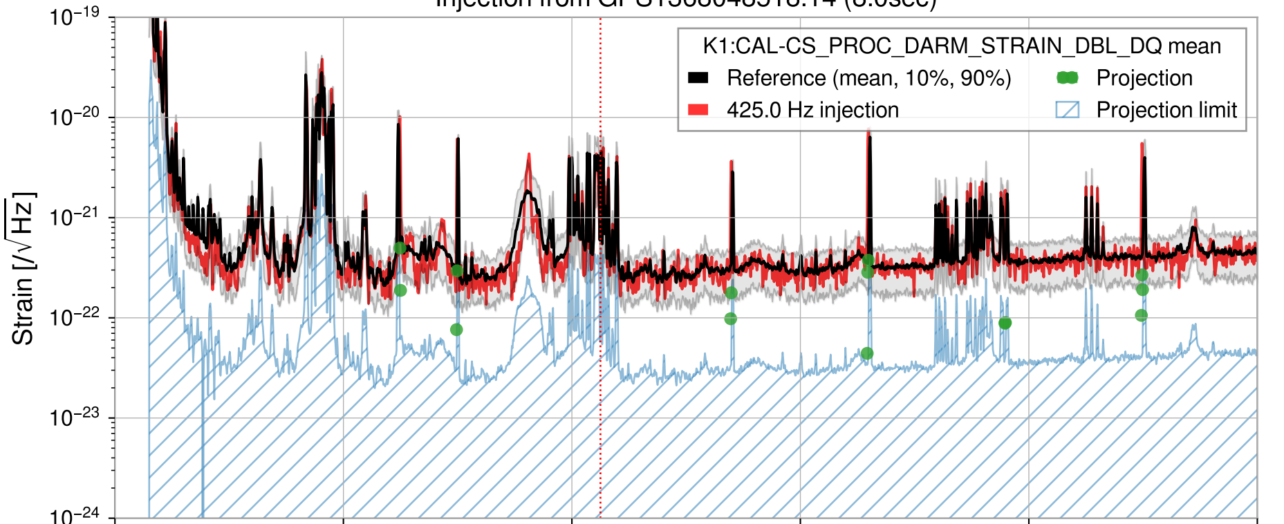
Injection from GPS1368048518.14 (8.0sec)
