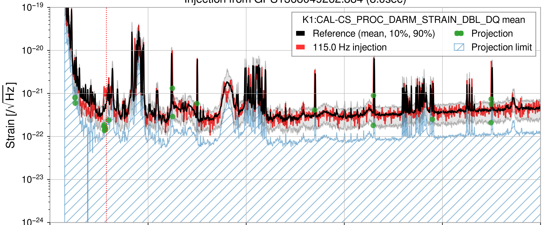
Injection from GPS1368049262.884 (8.0sec)
