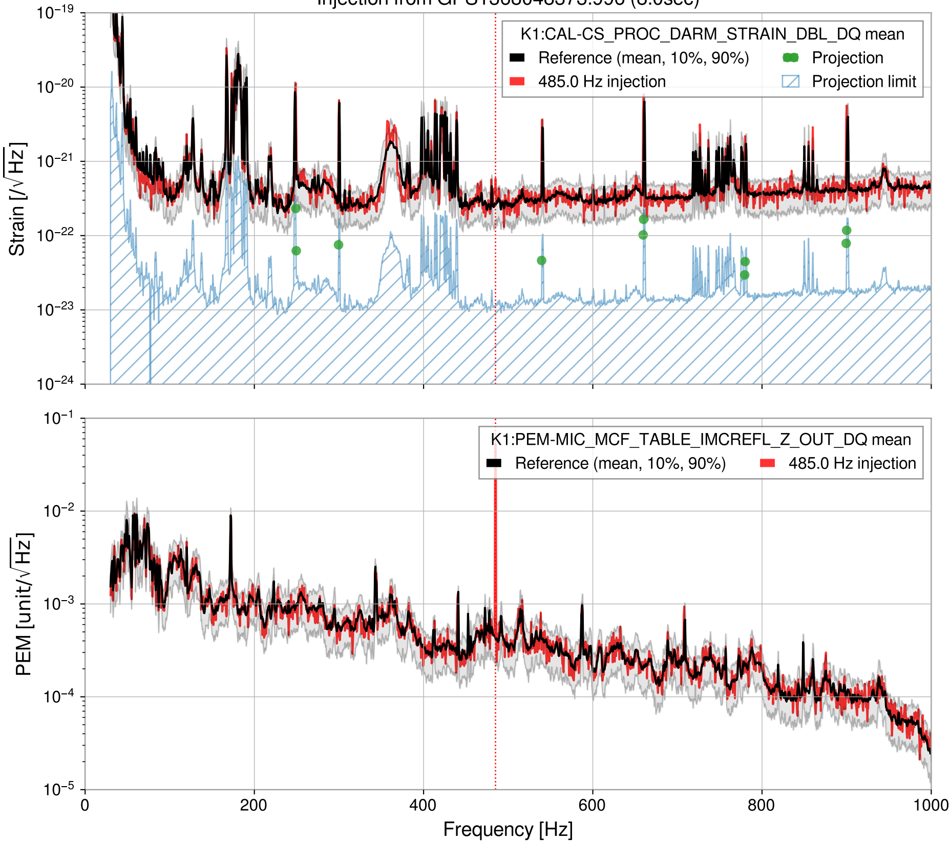
Injection from GPS1368048373.996 (8.0sec)
