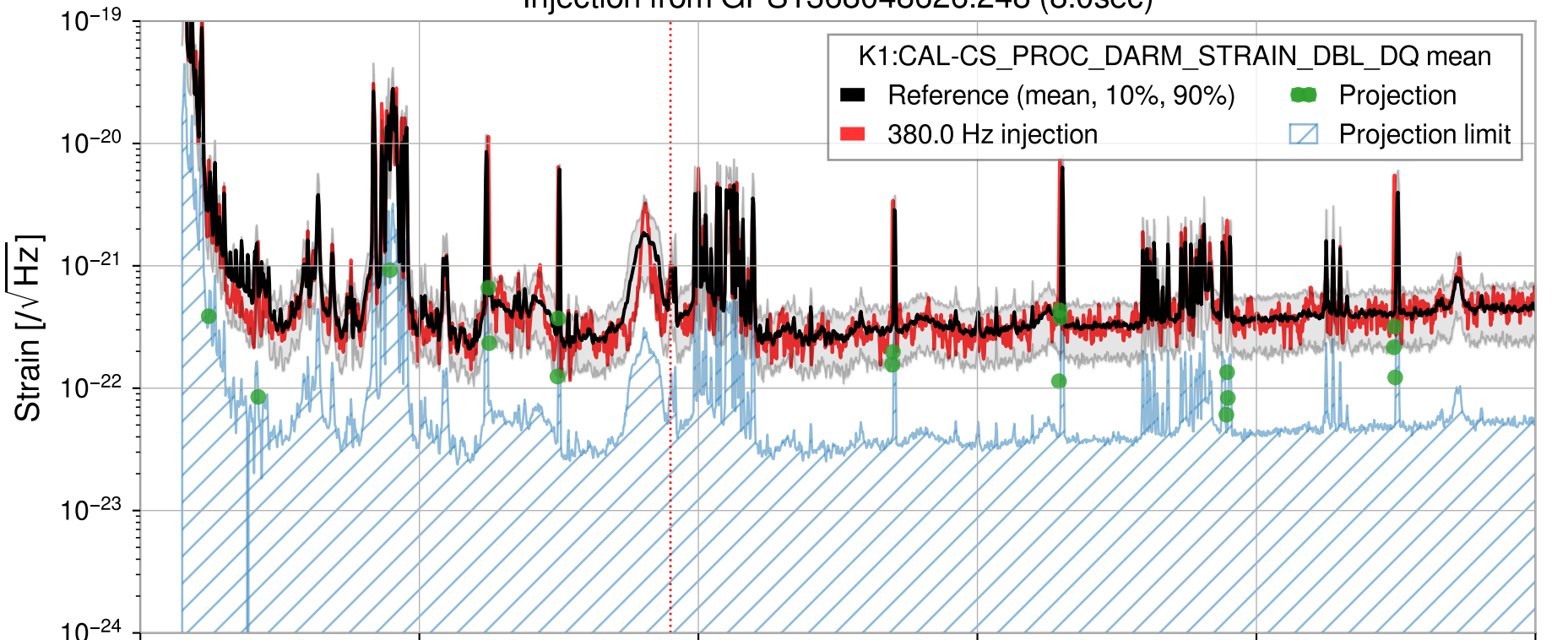
Injection from GPS1368048626.248 (8.0sec)
