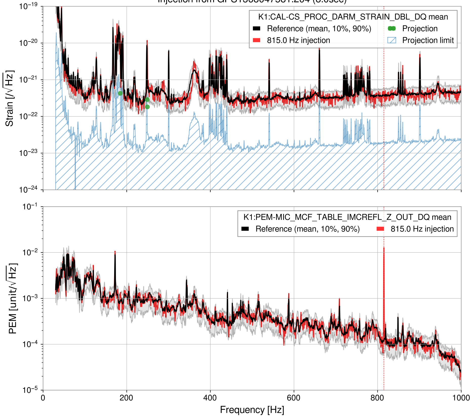
Injection from GPS1368047581.204 (8.0sec)
