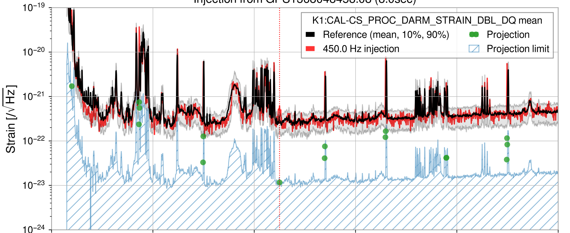
Injection from GPS1368048458.08 (8.0sec)
