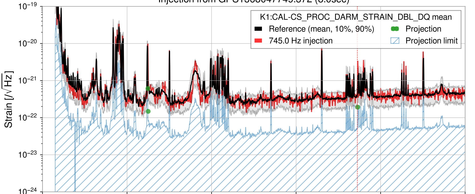
Injection from GPS1368047749.372 (8.0sec)
