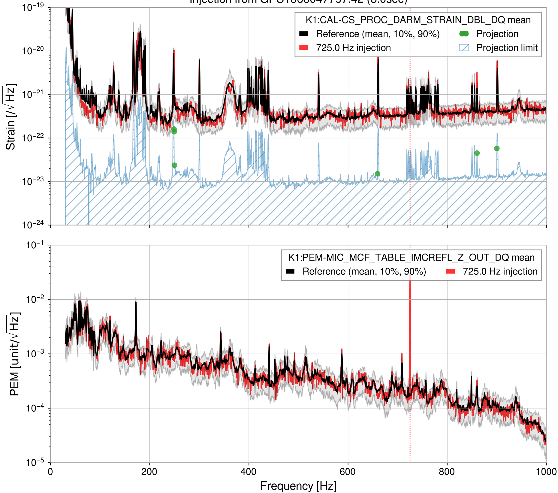
Injection from GPS1368047797.42 (8.0sec)
