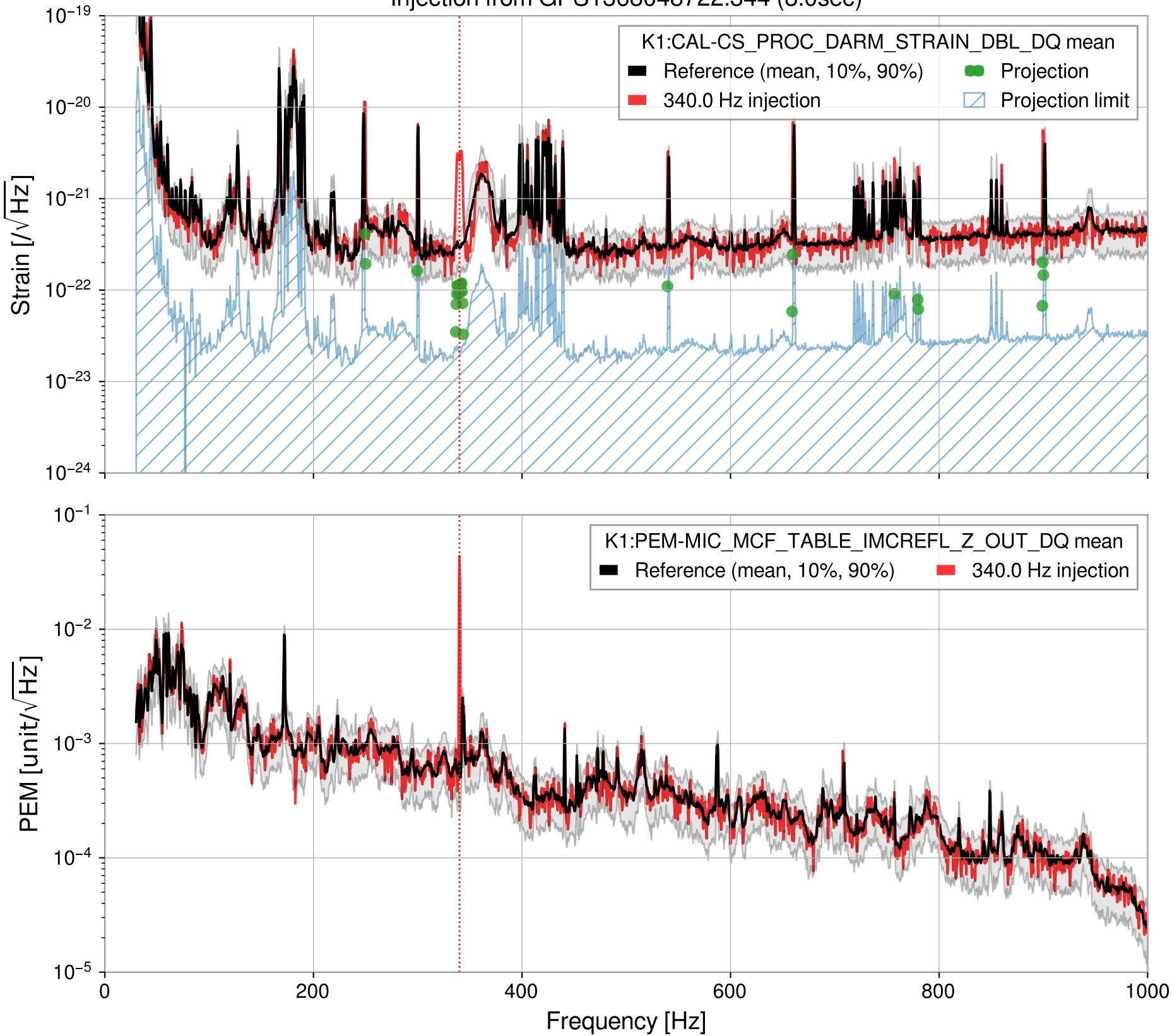
Injection from GPS1368048722.344 (8.0sec)
