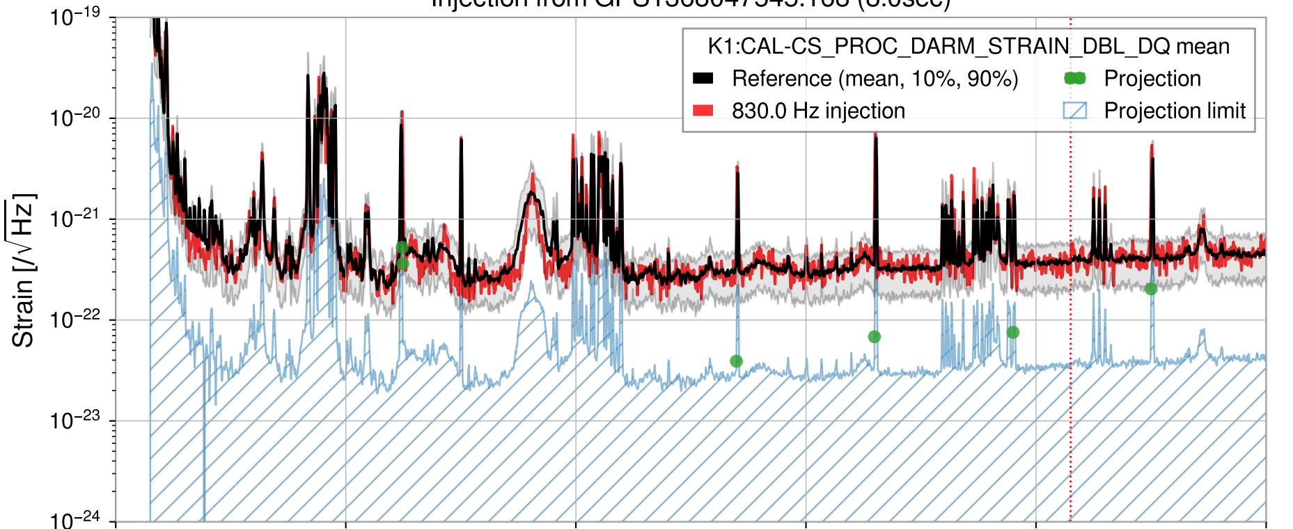
Injection from GPS1368047545.168 (8.0sec)
