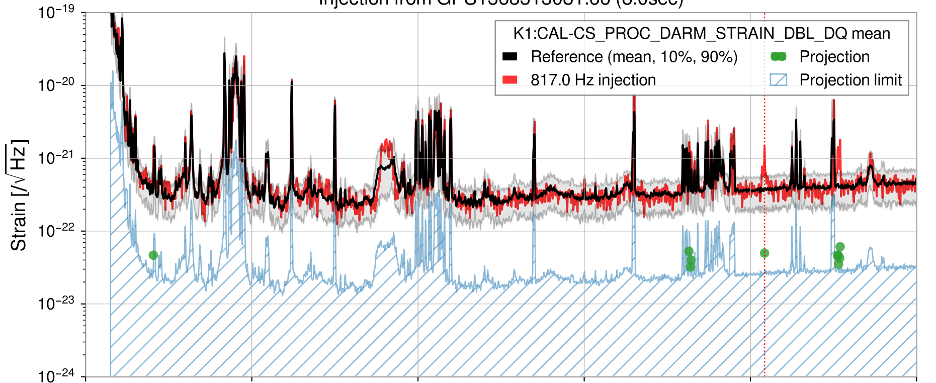
Injection from GPS1368313081.66 (8.0sec)
