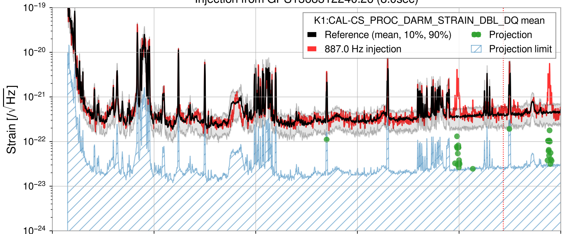
Injection from GPS1368312240.26 (8.0sec)
