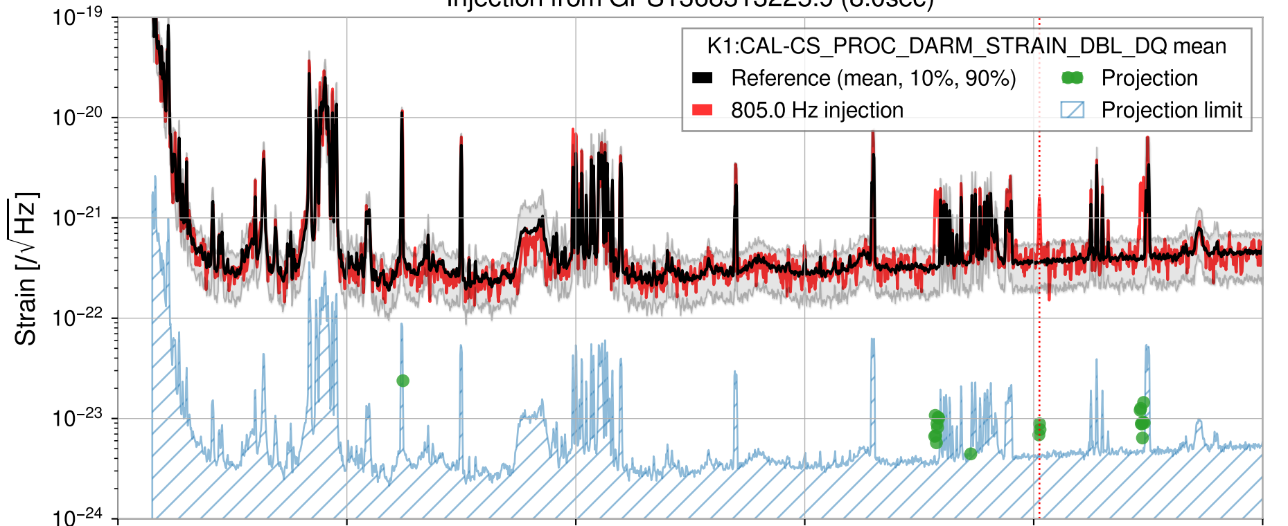
Injection from GPS1368313225.9 (8.0sec)
