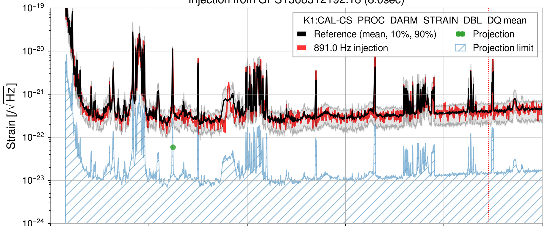
Injection from GPS1368312192.18 (8.0sec)
