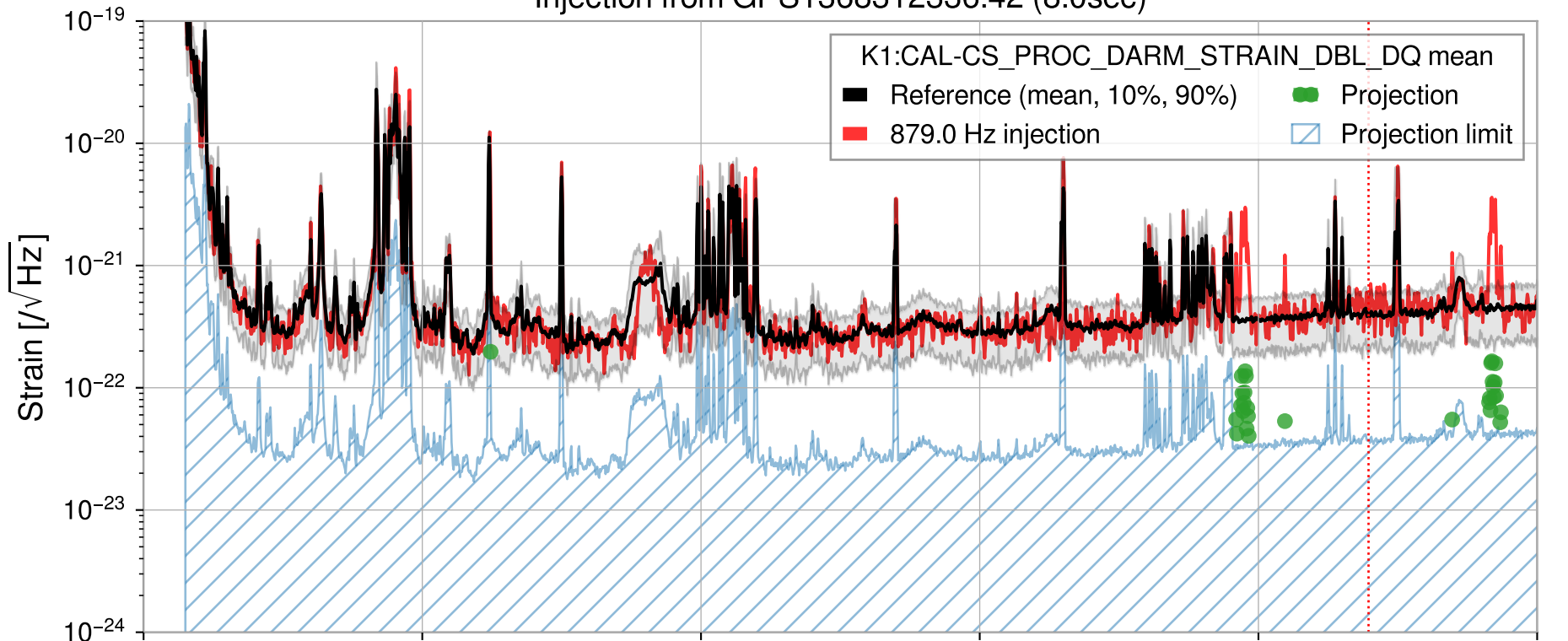
Injection from GPS1368312336.42 (8.0sec)
