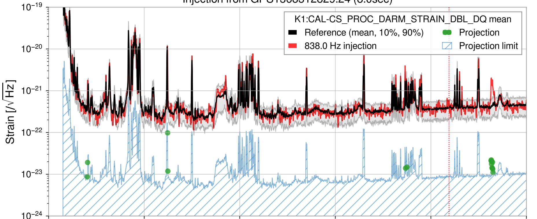
Injection from GPS1368312829.24 (8.0sec)
