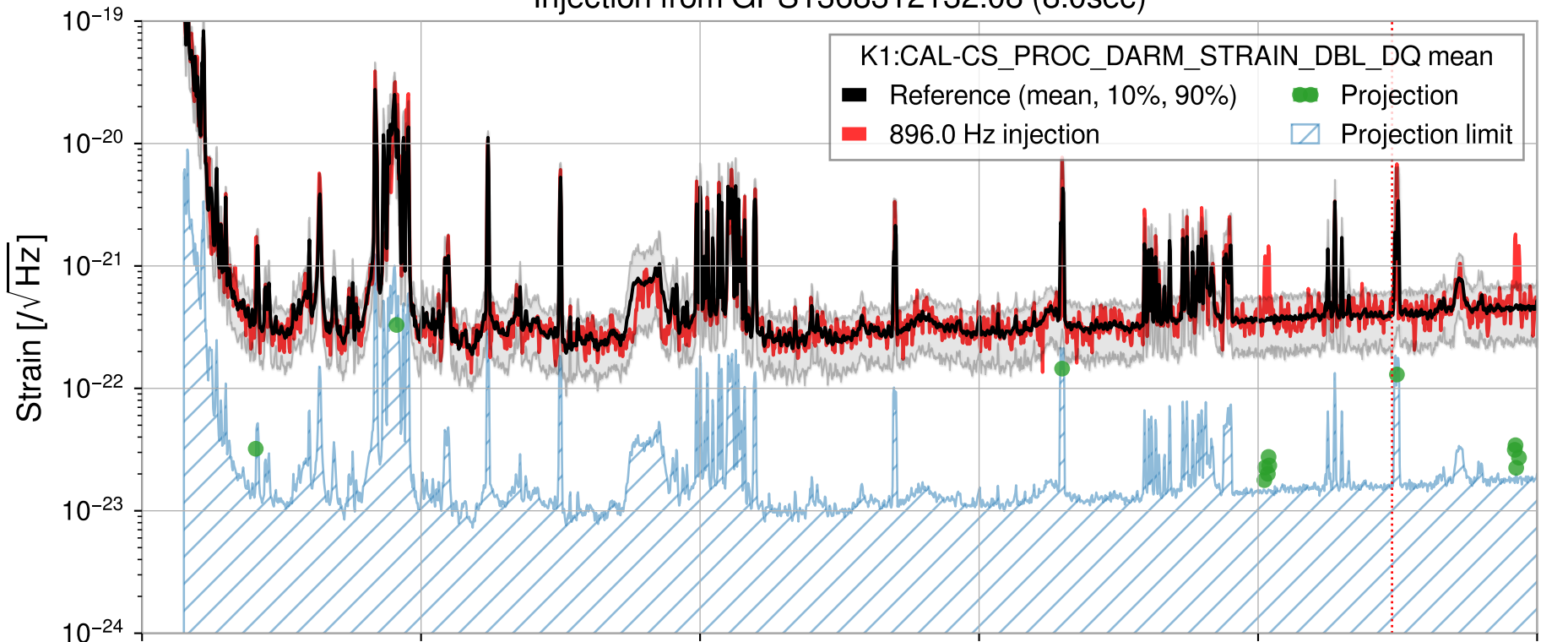
Injection from GPS1368312132.08 (8.0sec)
