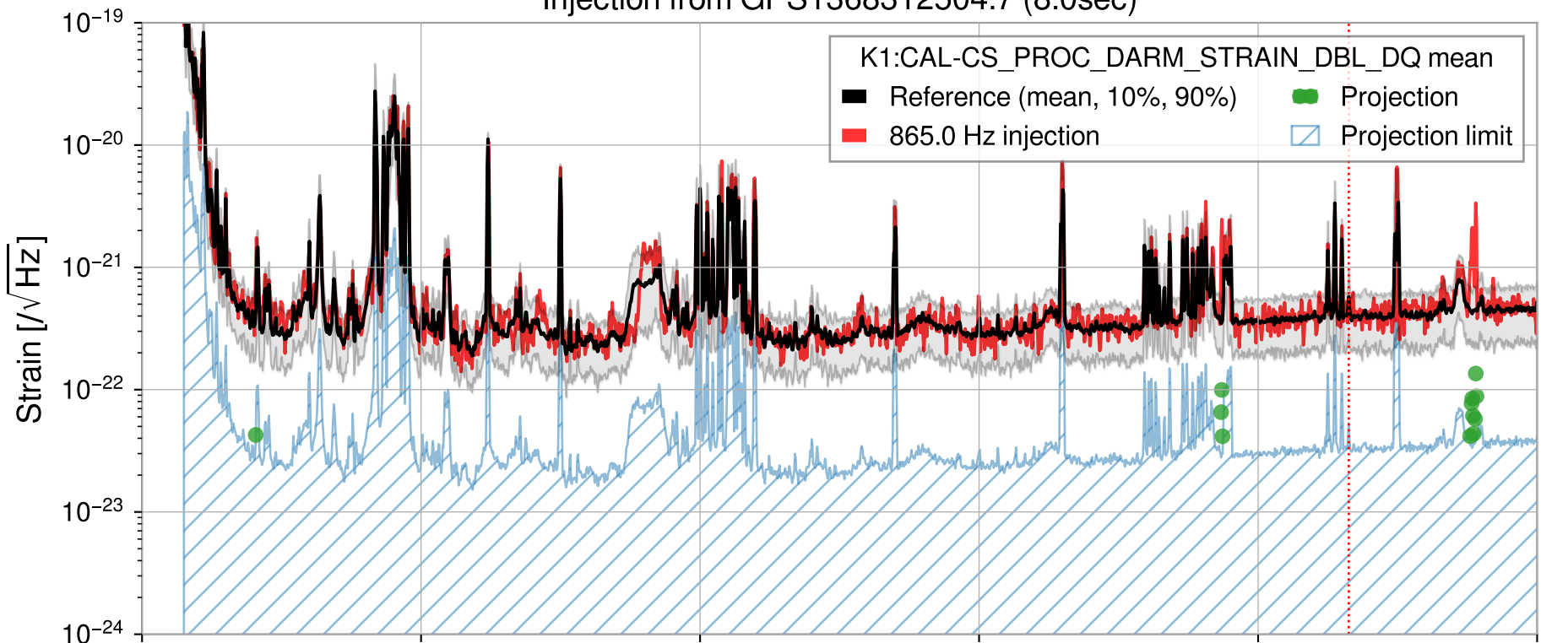
Injection from GPS1368312504.7 (8.0sec)
