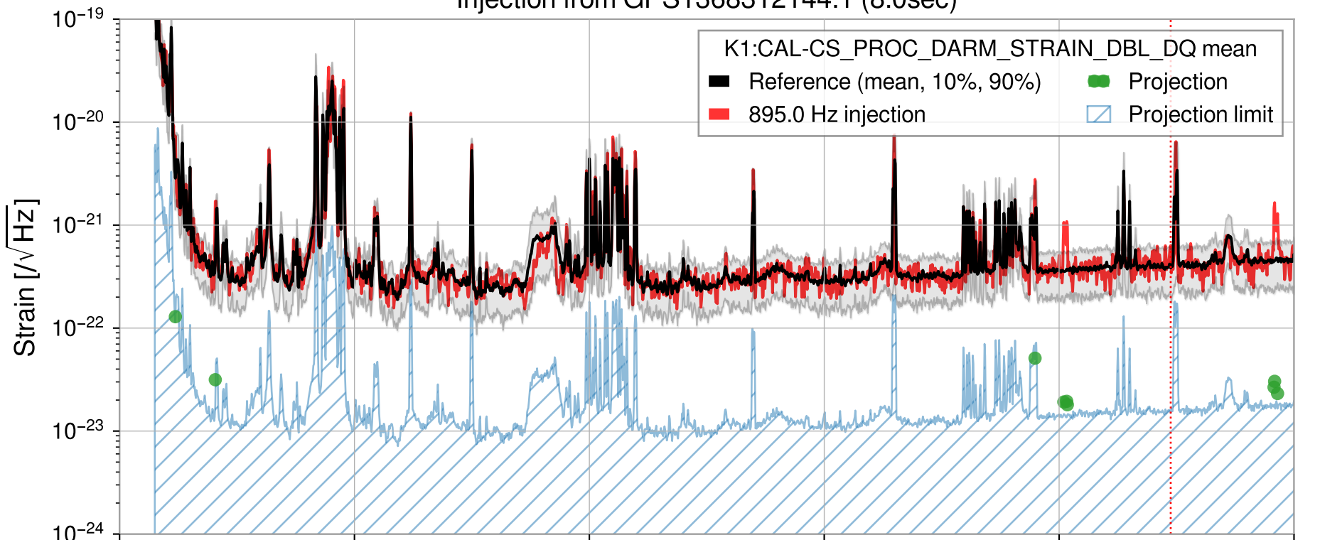
Injection from GPS1368312144.1 (8.0sec)
