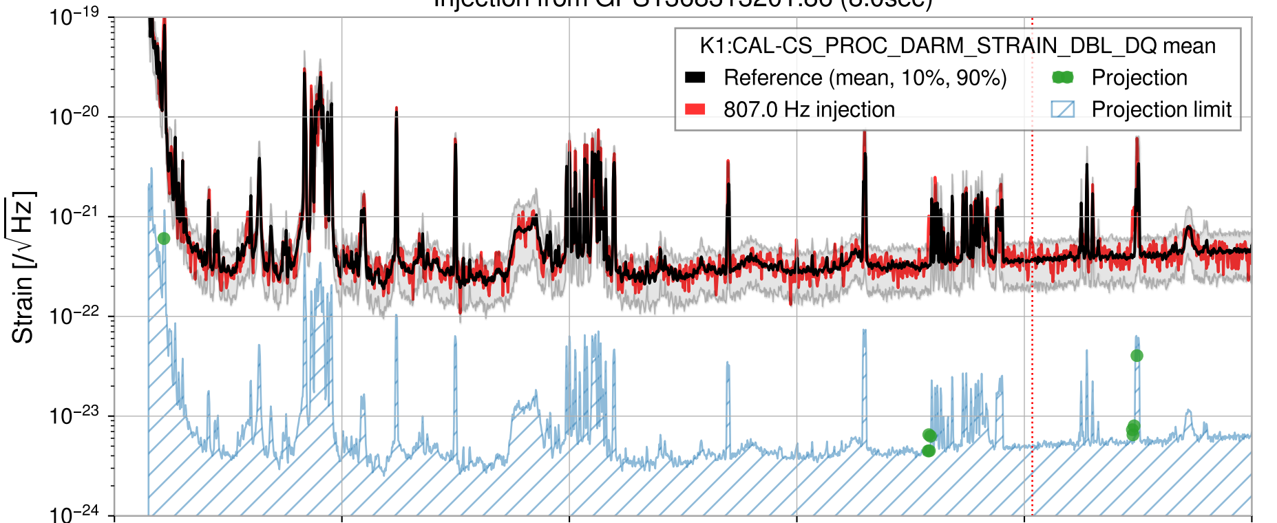
Injection from GPS1368313201.86 (8.0sec)
