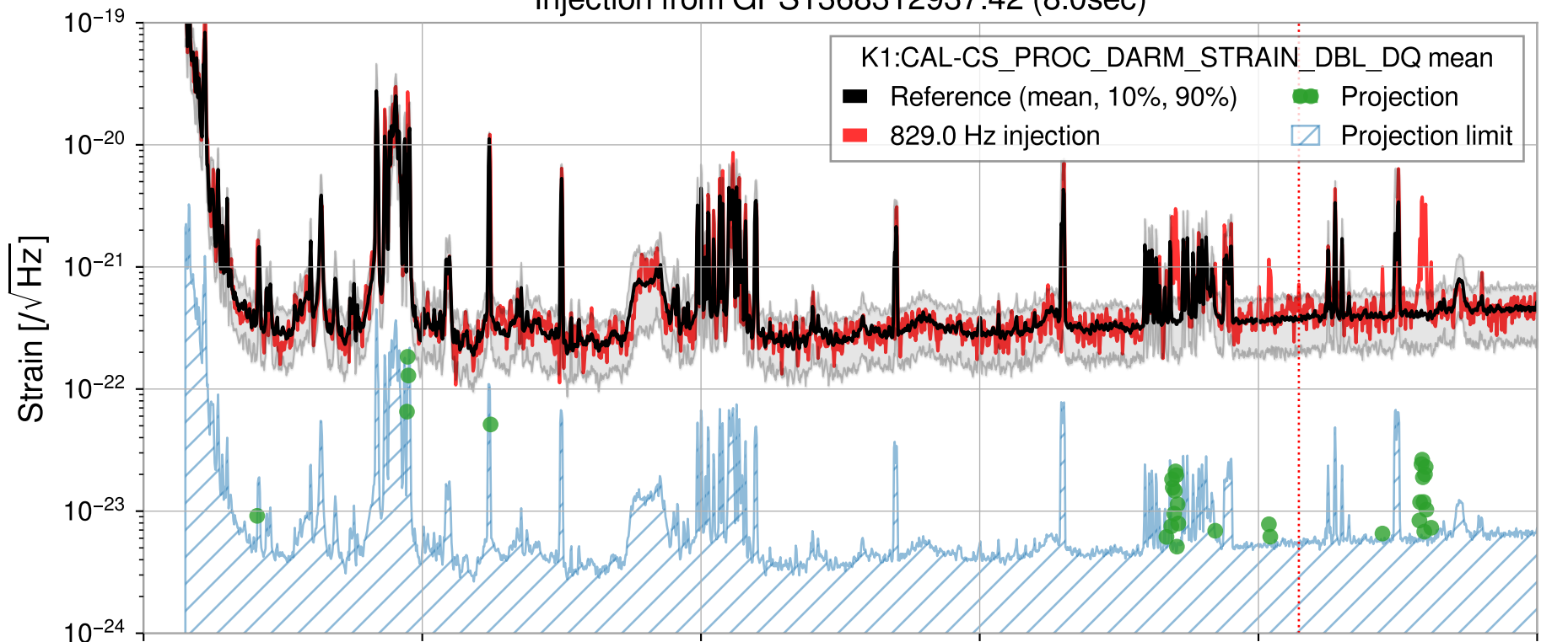
Injection from GPS1368312937.42 (8.0sec)
