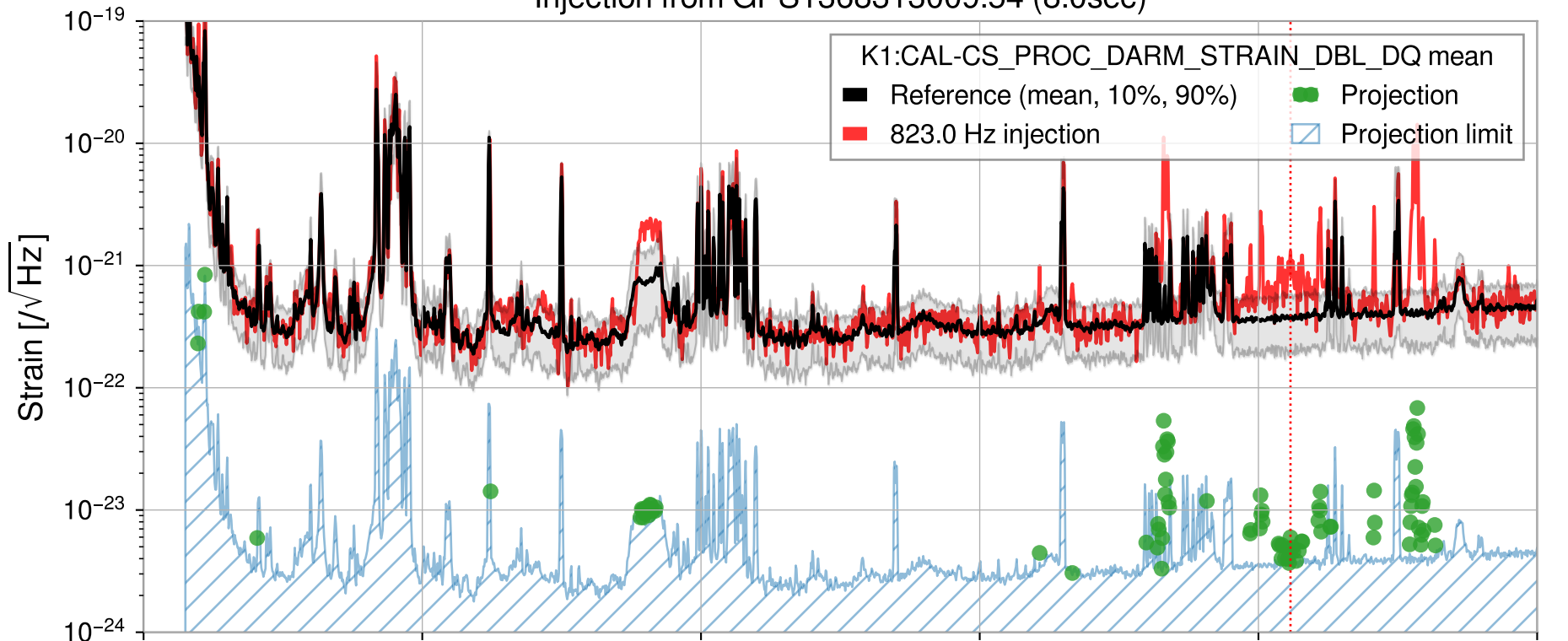
Injection from GPS1368313009.54 (8.0sec)
