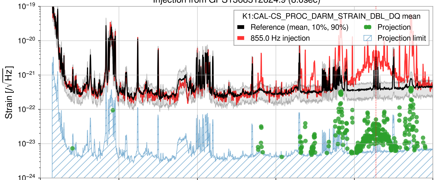
Injection from GPS1368312624.9 (8.0sec)
