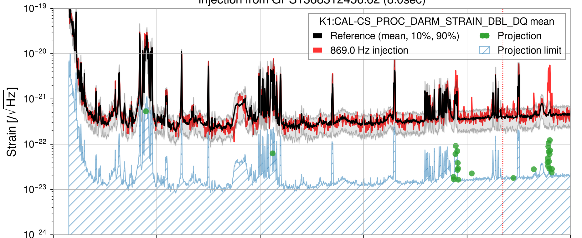
Injection from GPS1368312456.62 (8.0sec)
