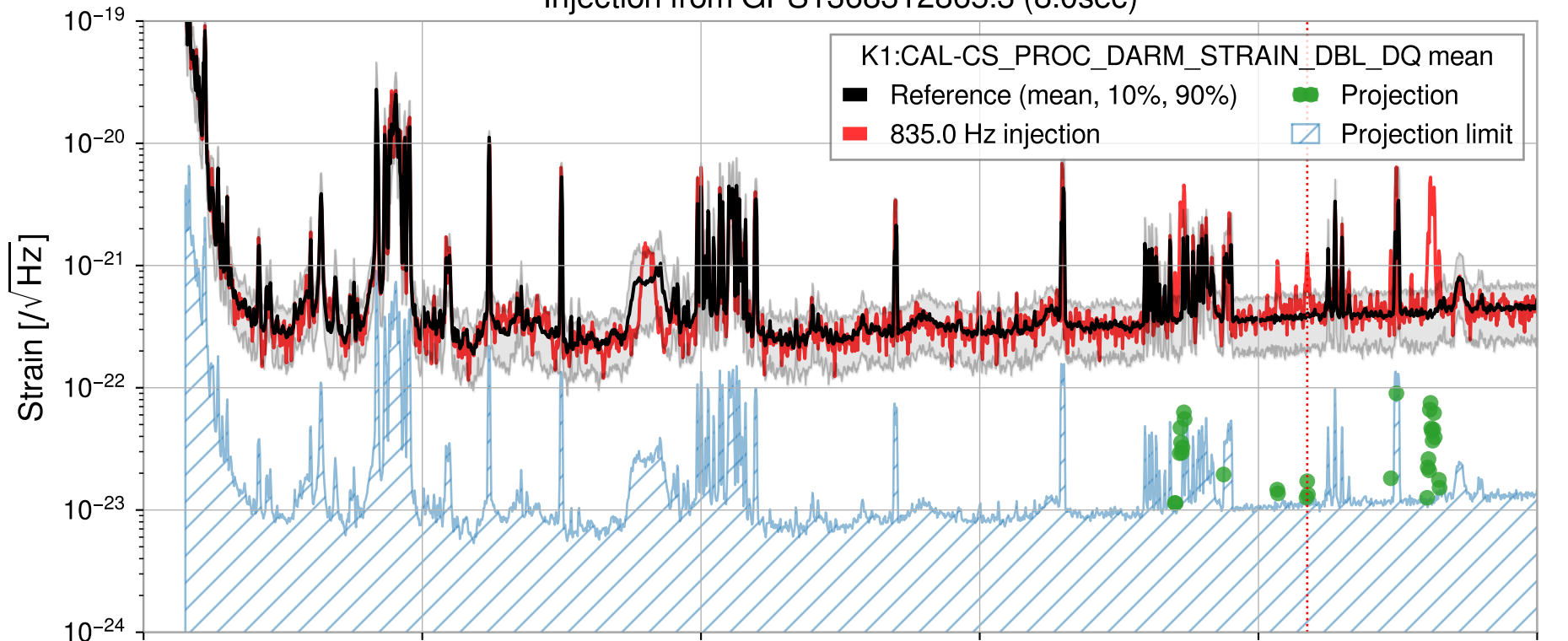
Injection from GPS1368312865.3 (8.0sec)
