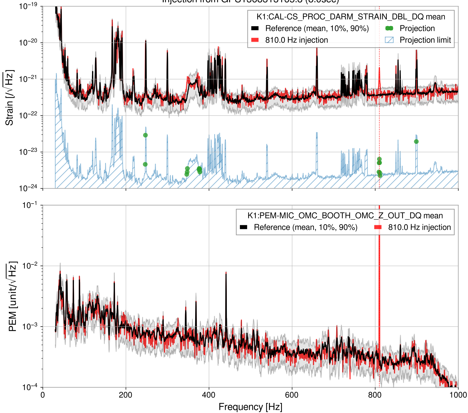
Injection from GPS1368313165.8 (8.0sec)
