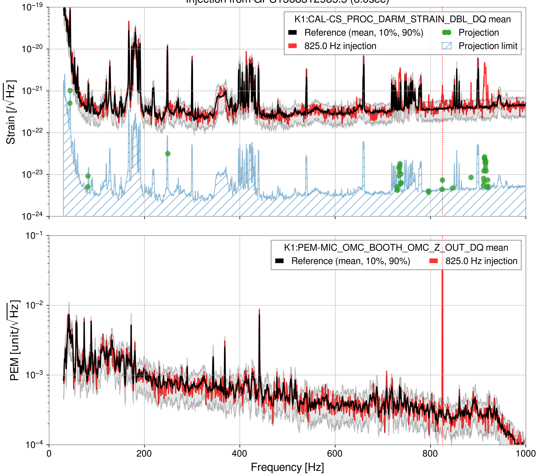
Injection from GPS1368312985.5 (8.0sec)
