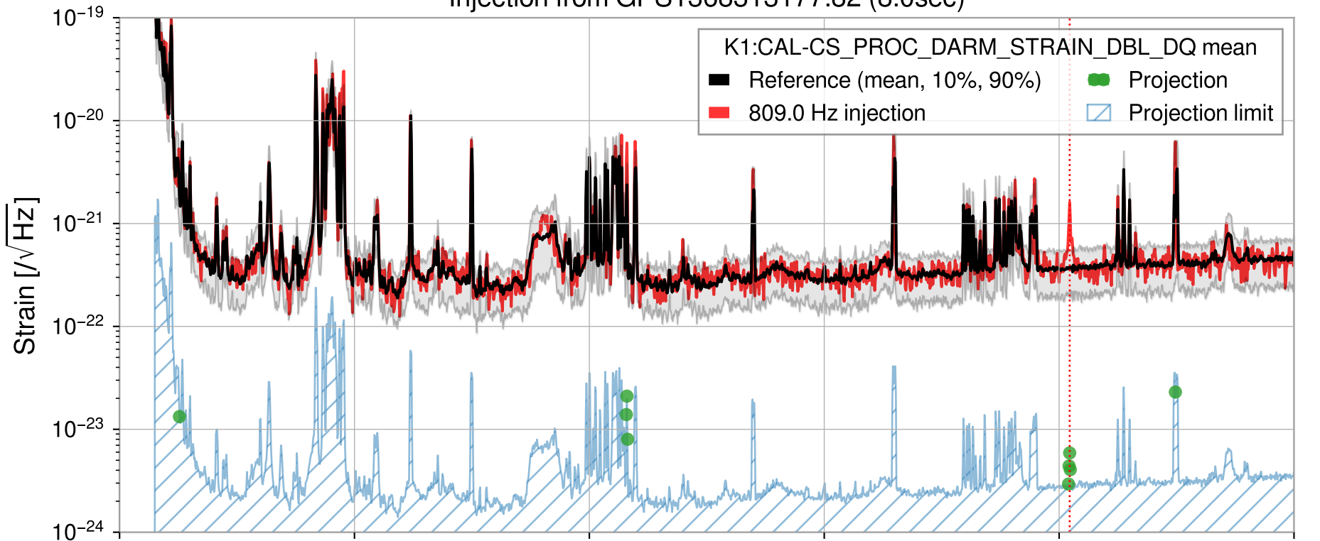
Injection from GPS1368313177.82 (8.0sec)
