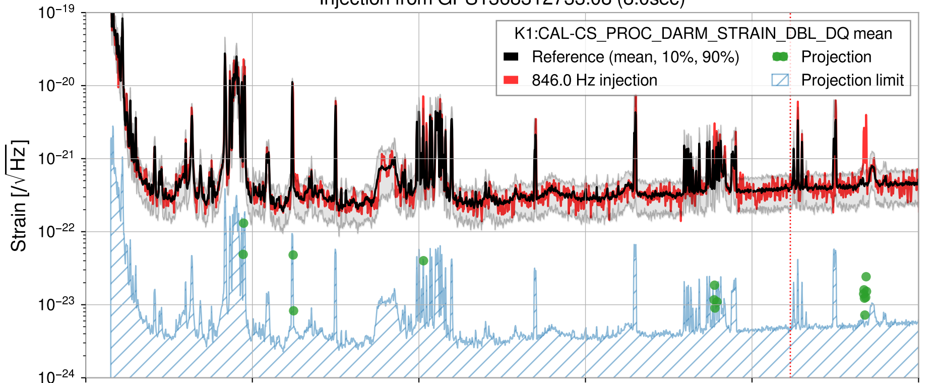
Injection from GPS1368312733.08 (8.0sec)
