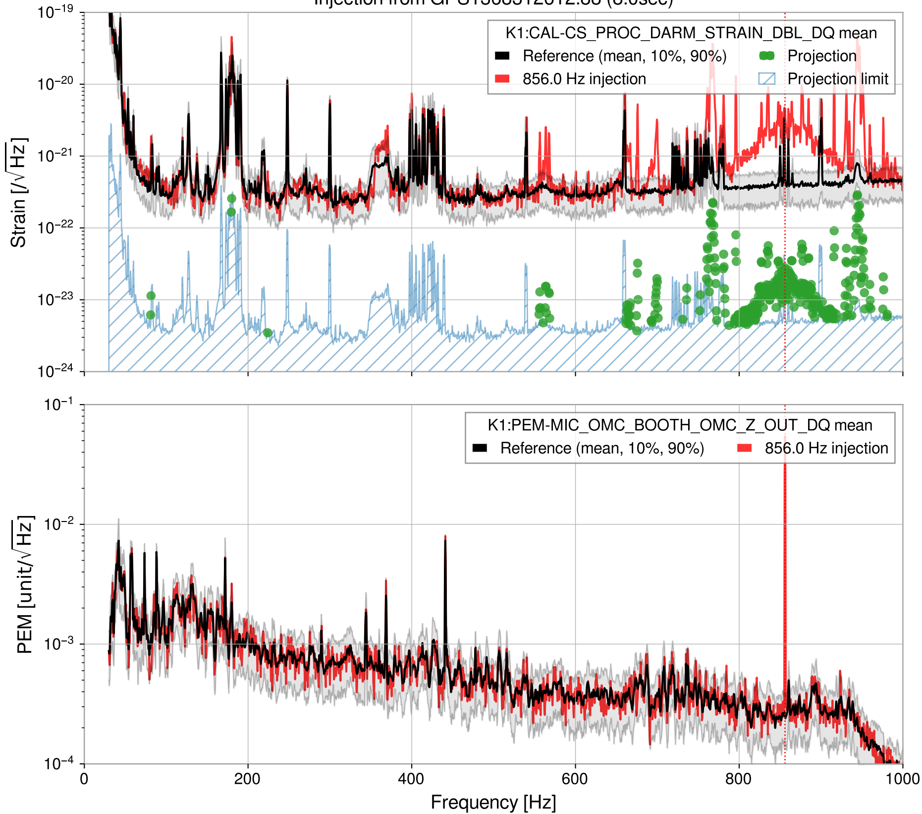
Injection from GPS1368312612.88 (8.0sec)
