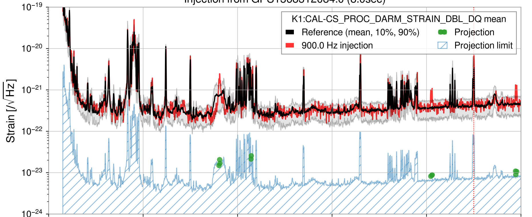
Injection from GPS1368312084.0 (8.0sec)
