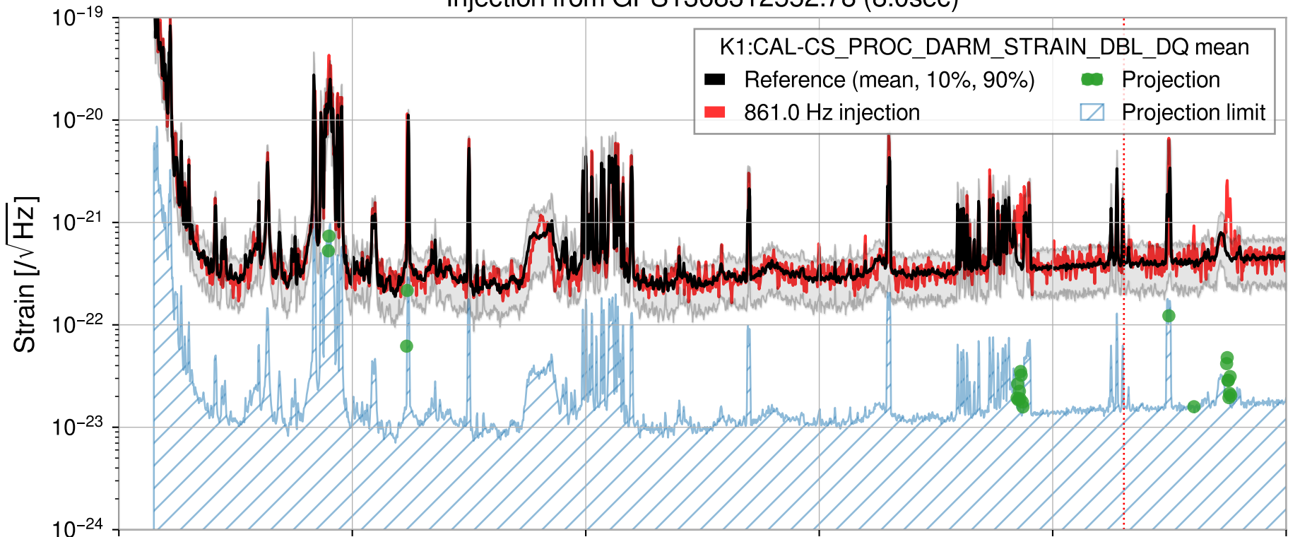
Injection from GPS1368312552.78 (8.0sec)
