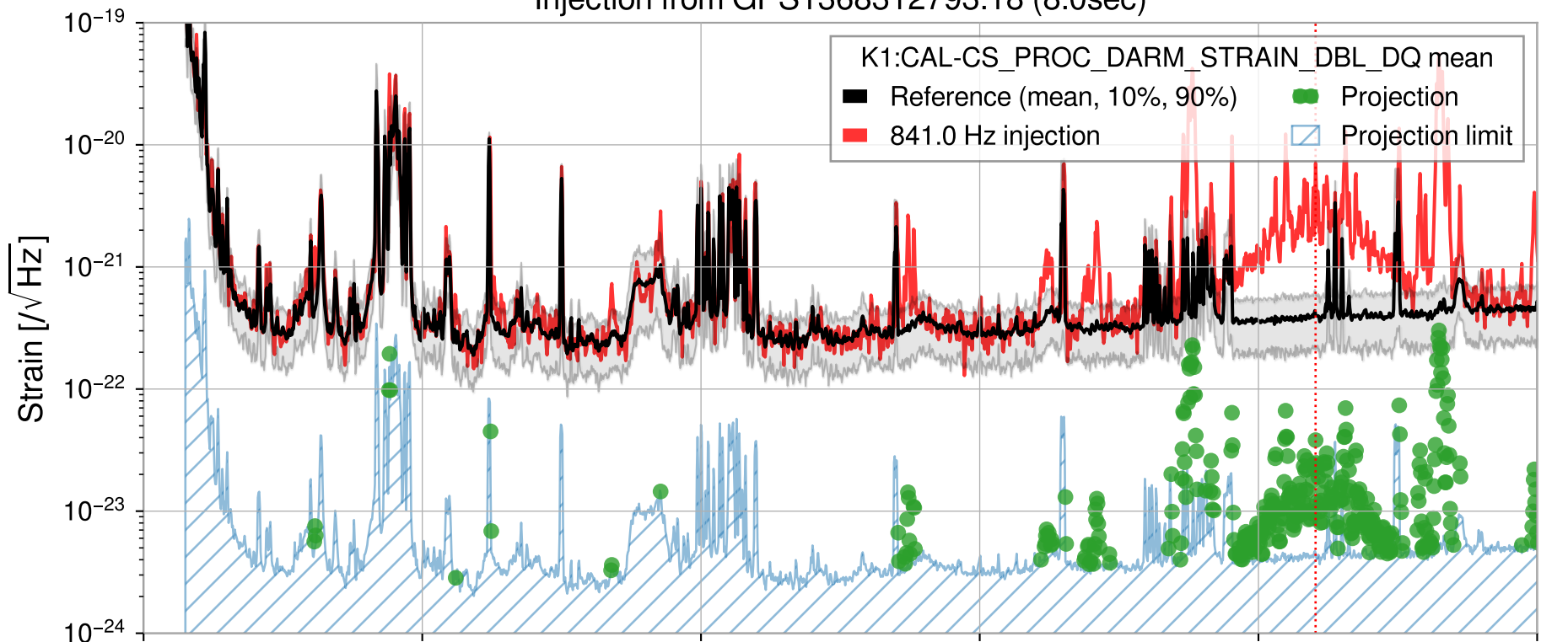
Injection from GPS1368312793.18 (8.0sec)
