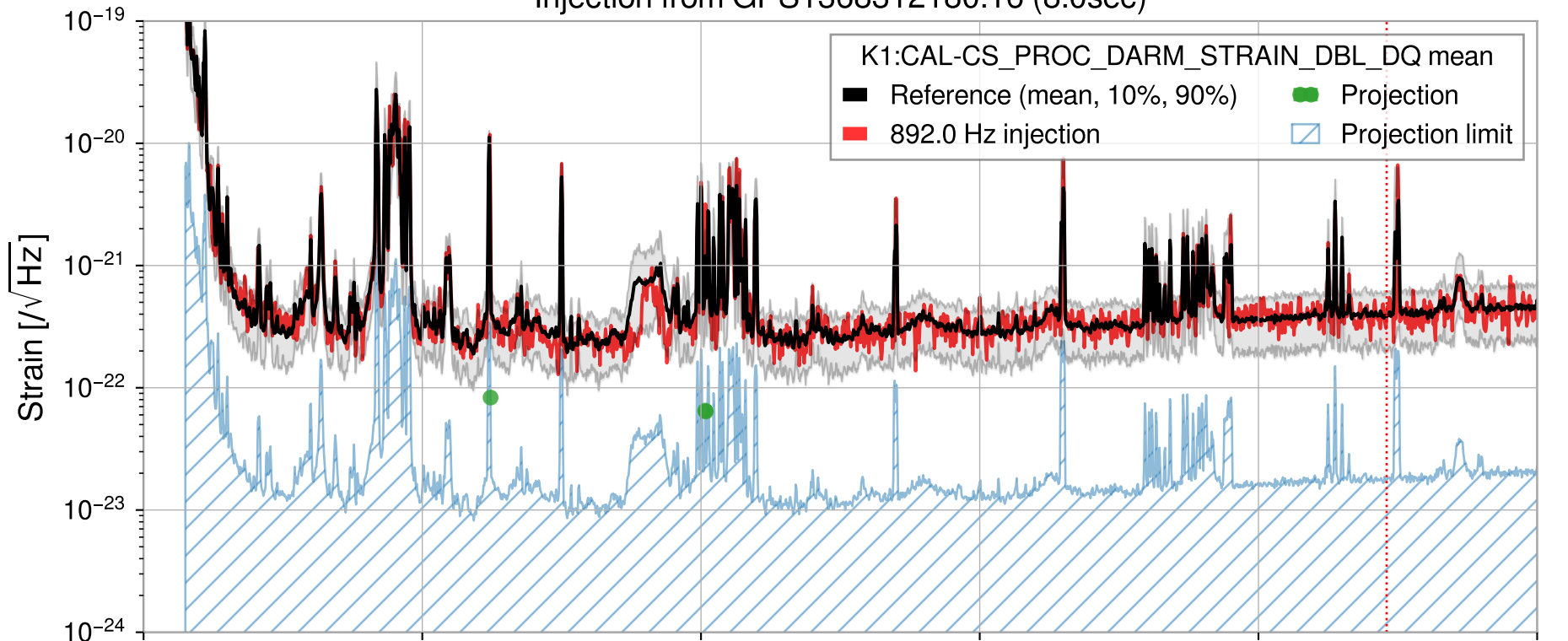
Injection from GPS1368312180.16 (8.0sec)
