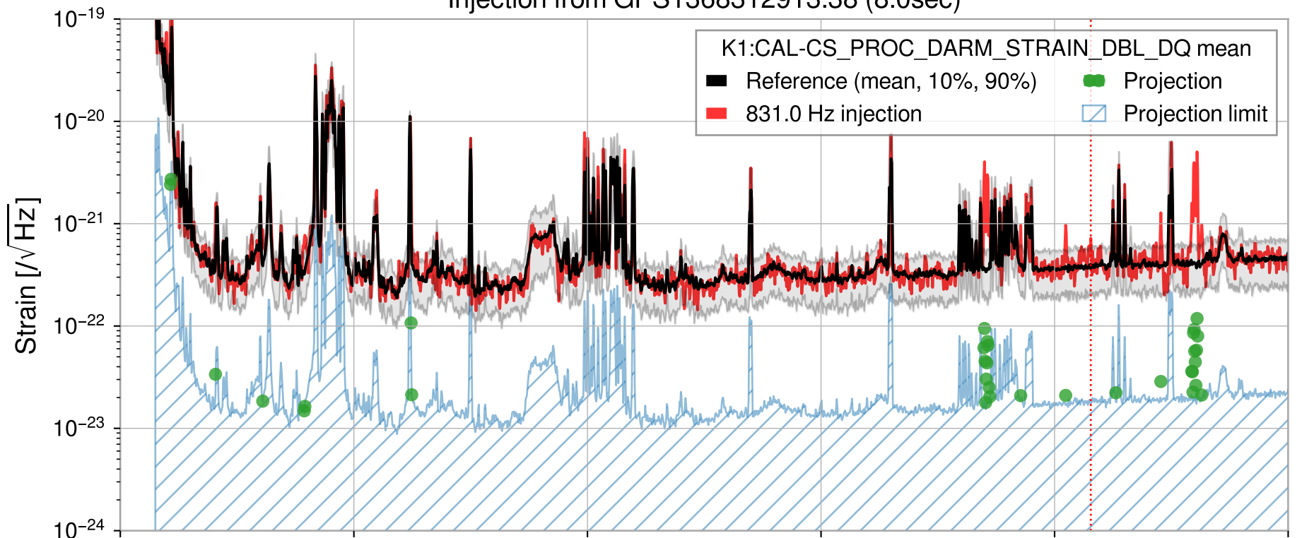
Injection from GPS1368312913.38 (8.0sec)
