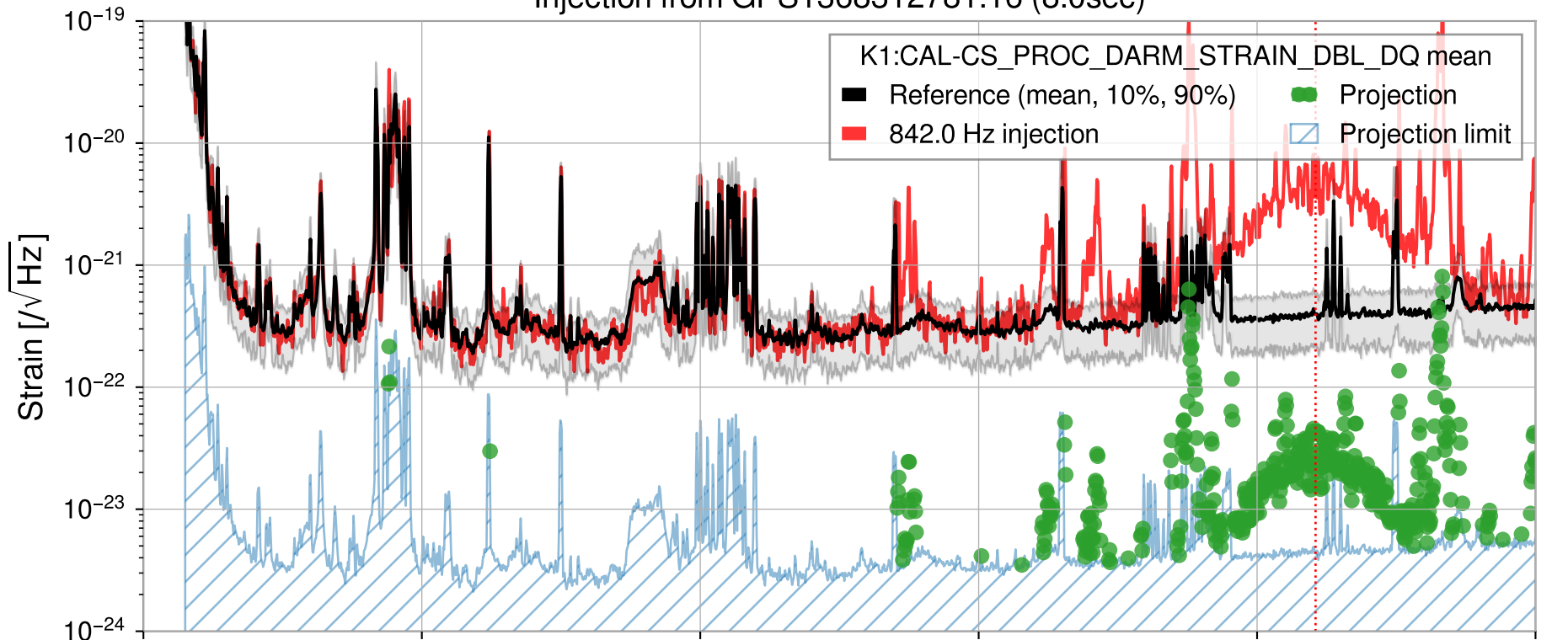
Injection from GPS1368312781.16 (8.0sec)
