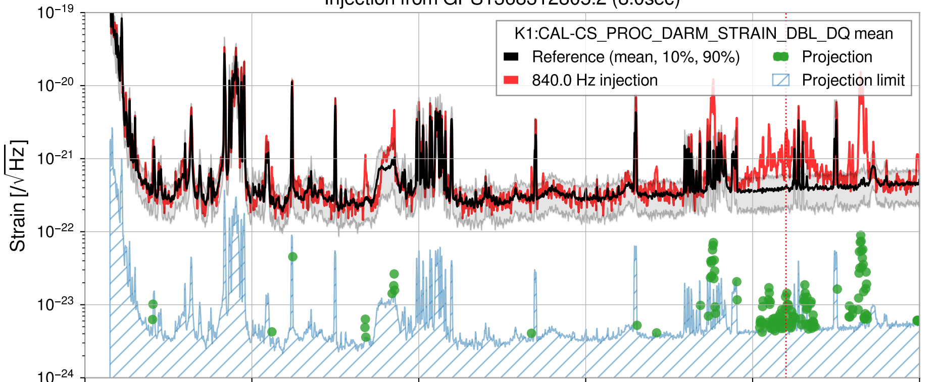
Injection from GPS1368312805.2 (8.0sec)
