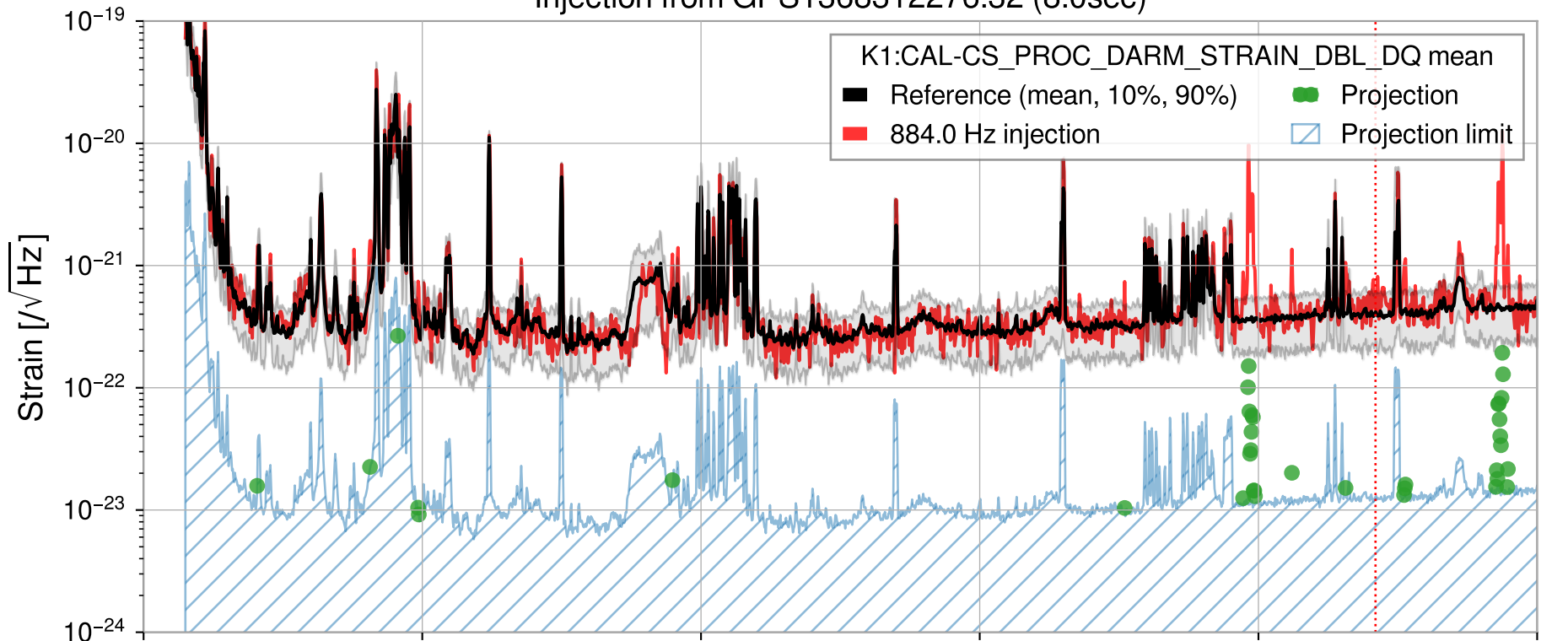
Injection from GPS1368312276.32 (8.0sec)
