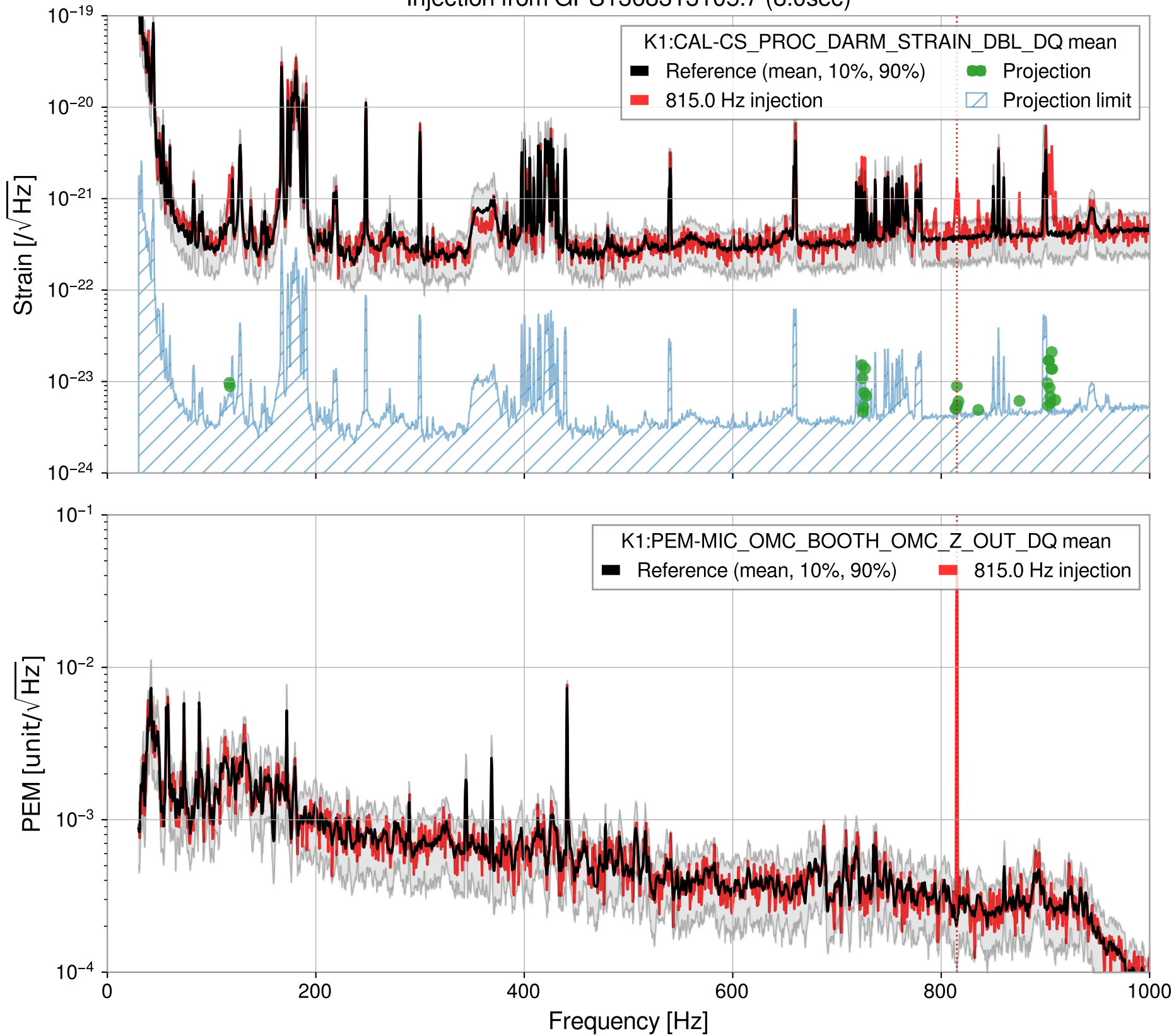
Injection from GPS1368313105.7 (8.0sec)
