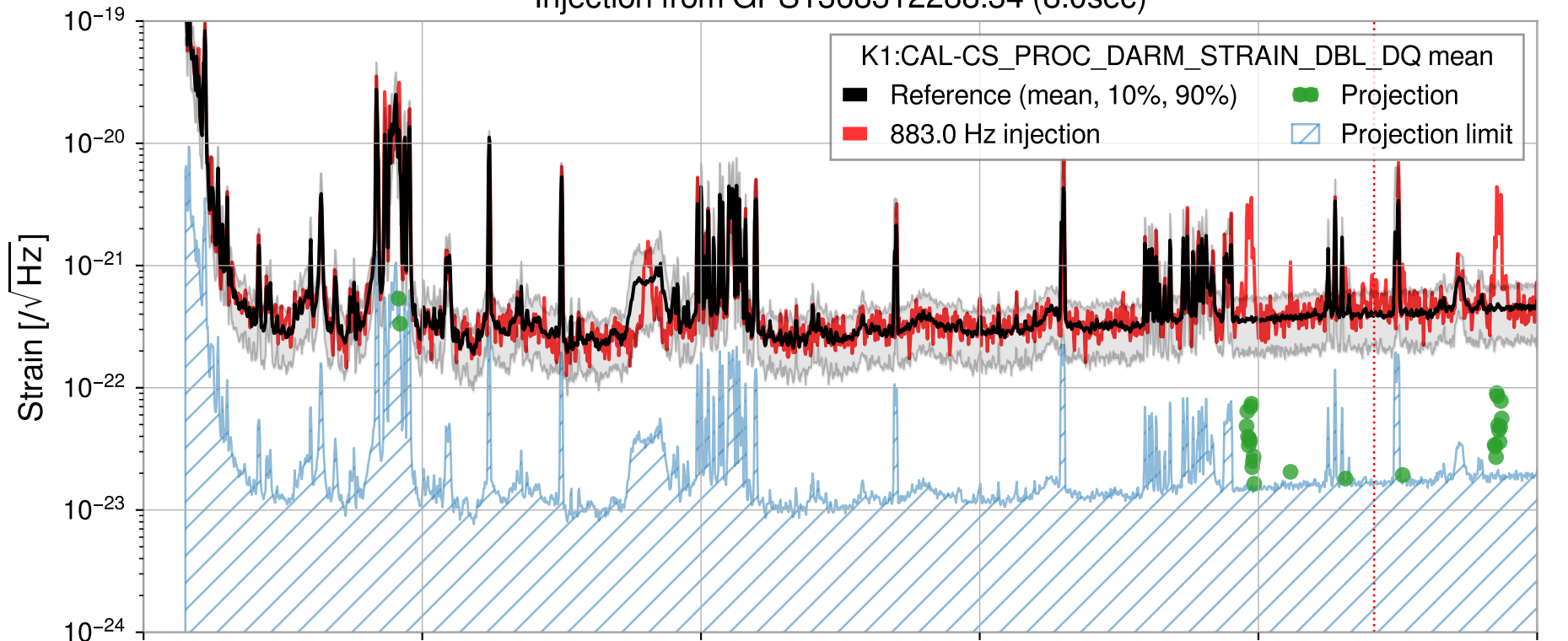
Injection from GPS1368312288.34 (8.0sec)
