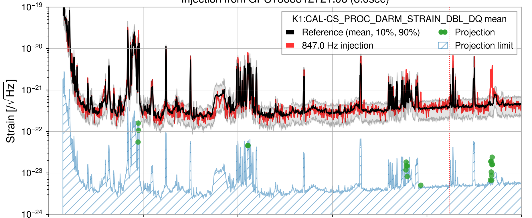
Injection from GPS1368312721.06 (8.0sec)
