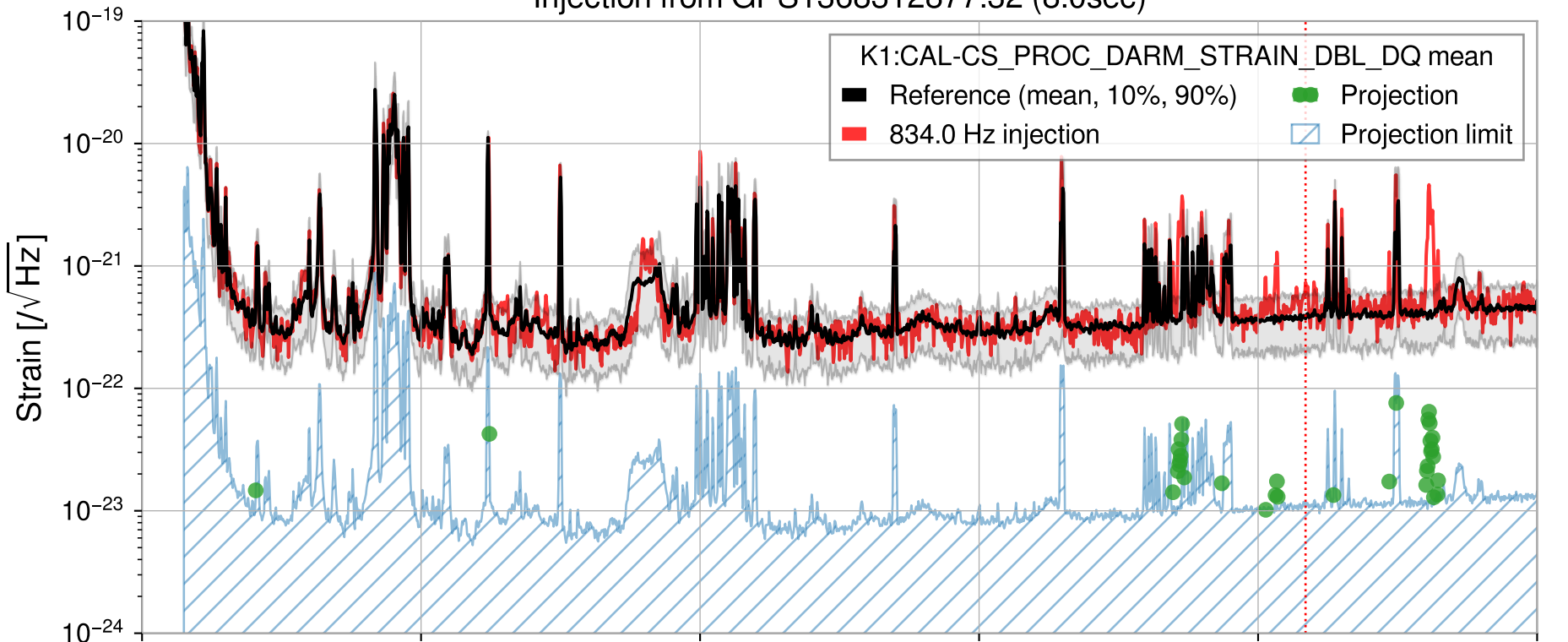
Injection from GPS1368312877.32 (8.0sec)
