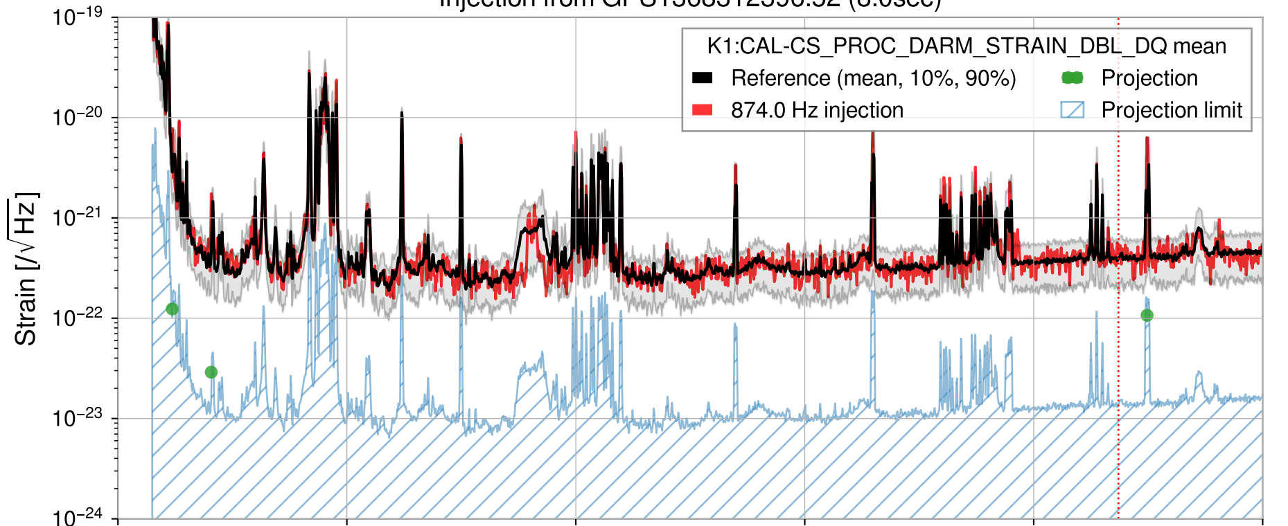
Injection from GPS1368312396.52 (8.0sec)
