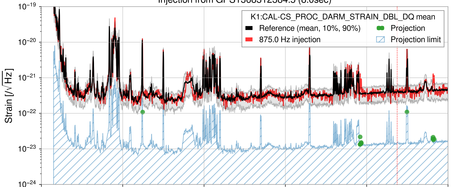
Injection from GPS1368312384.5 (8.0sec)
