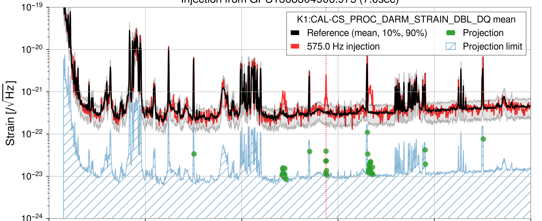
Injection from GPS1368304906.975 (7.0sec)
