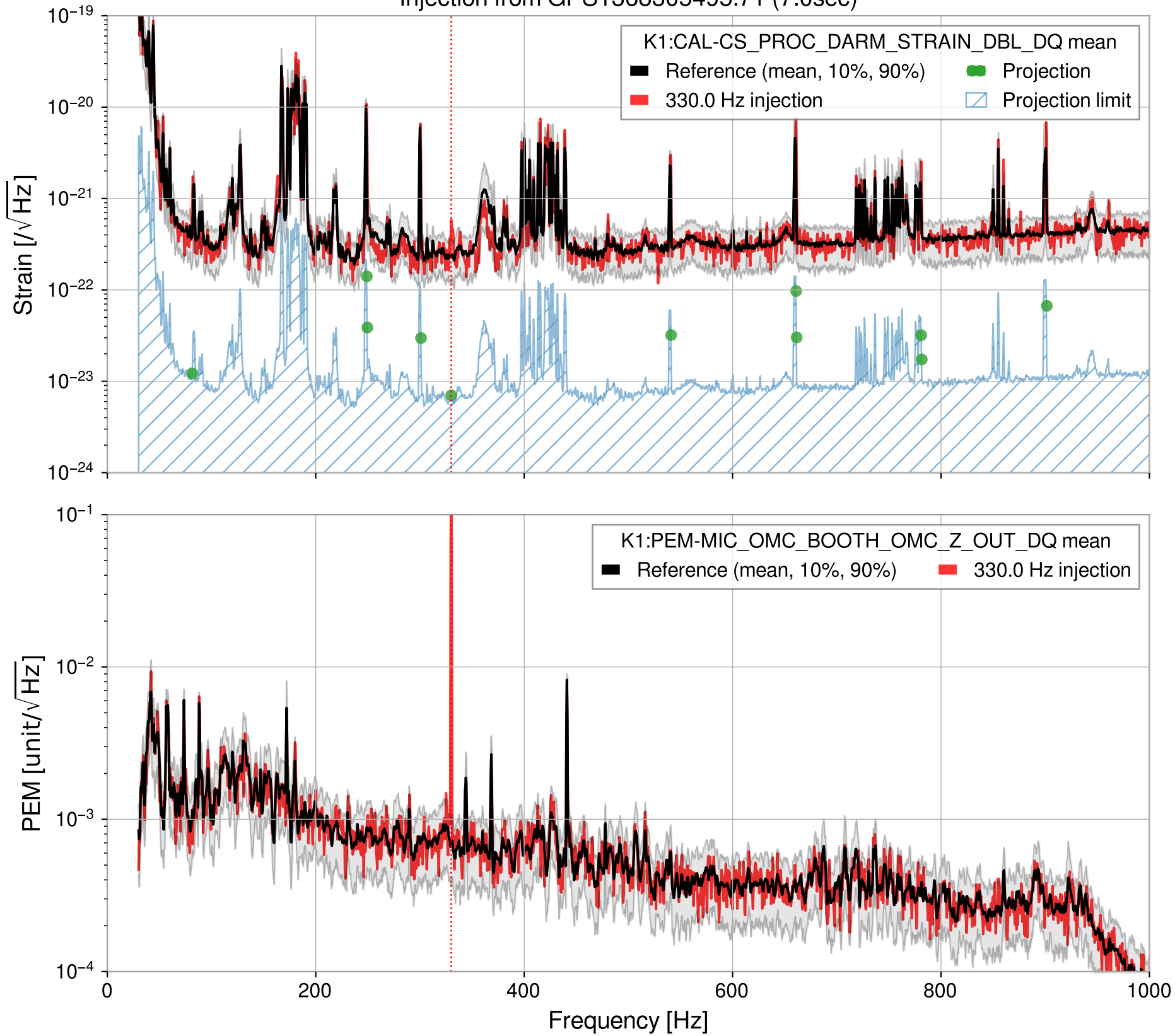
Injection from GPS1368305495.71 (7.0sec)
