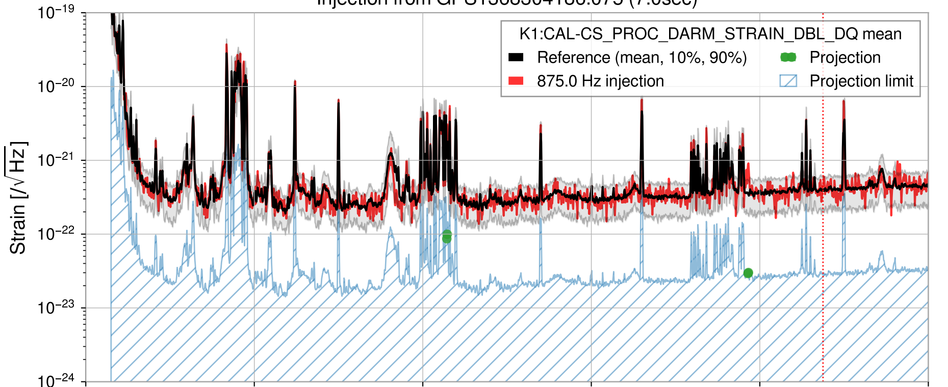
Injection from GPS1368304186.075 (7.0sec)
