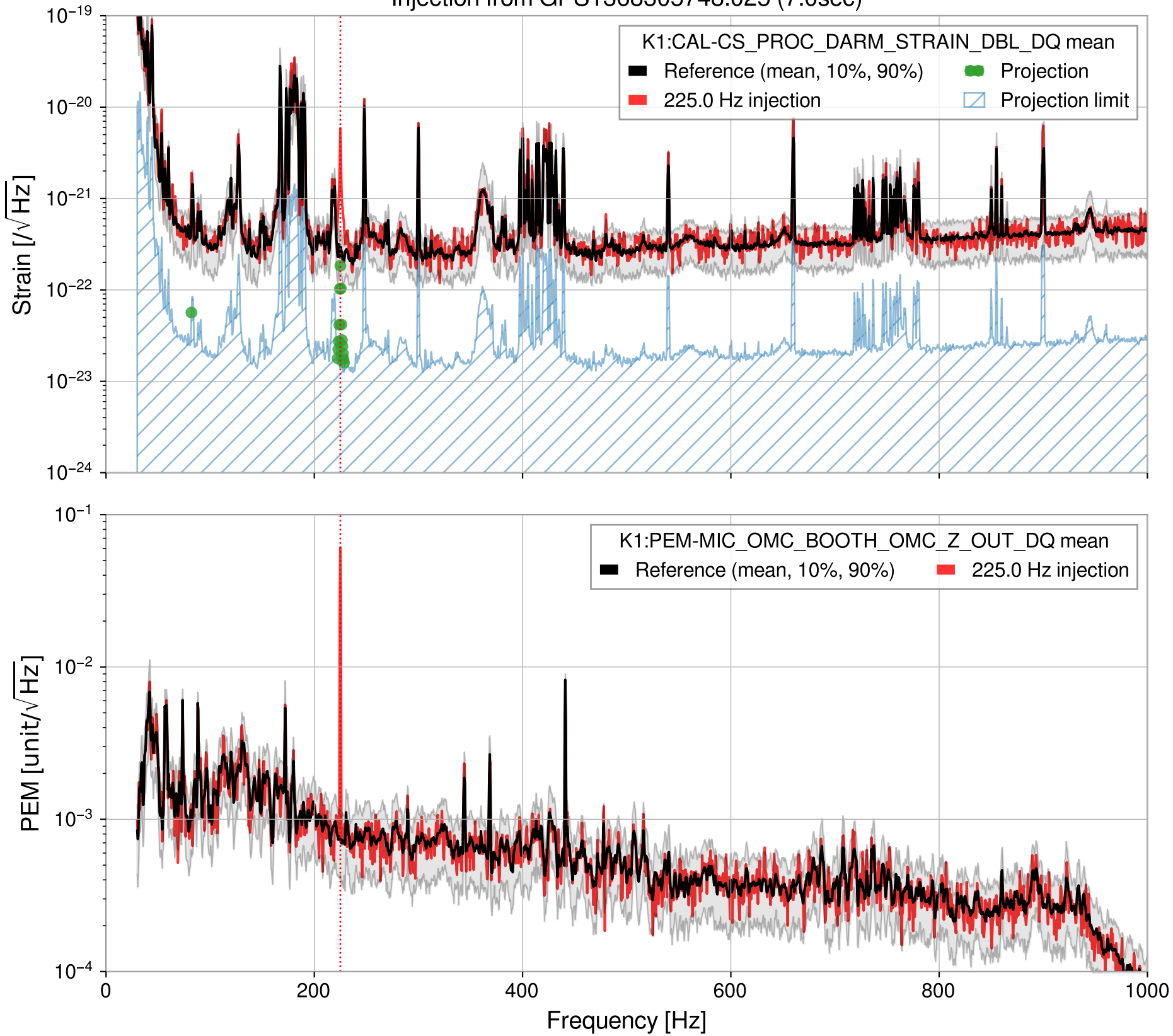
Injection from GPS1368305748.025 (7.0sec)
