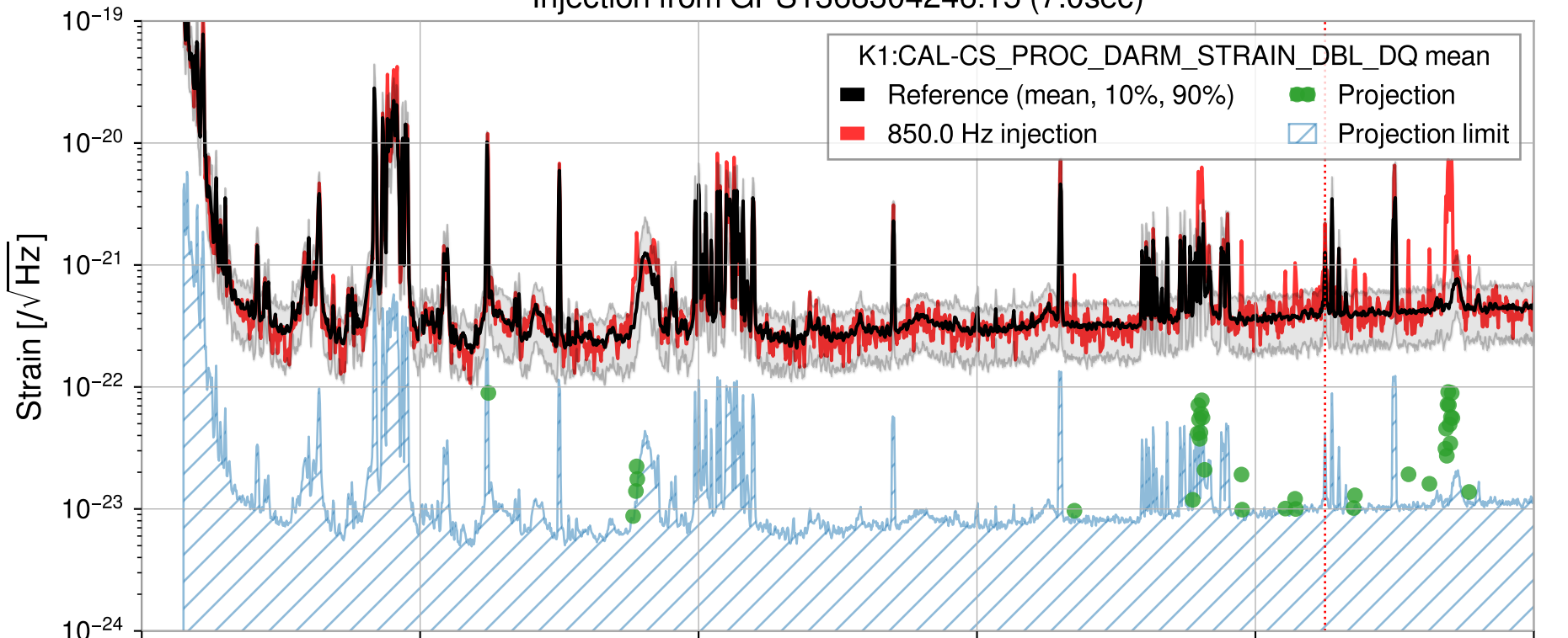
Injection from GPS1368304246.15 (7.0sec)
