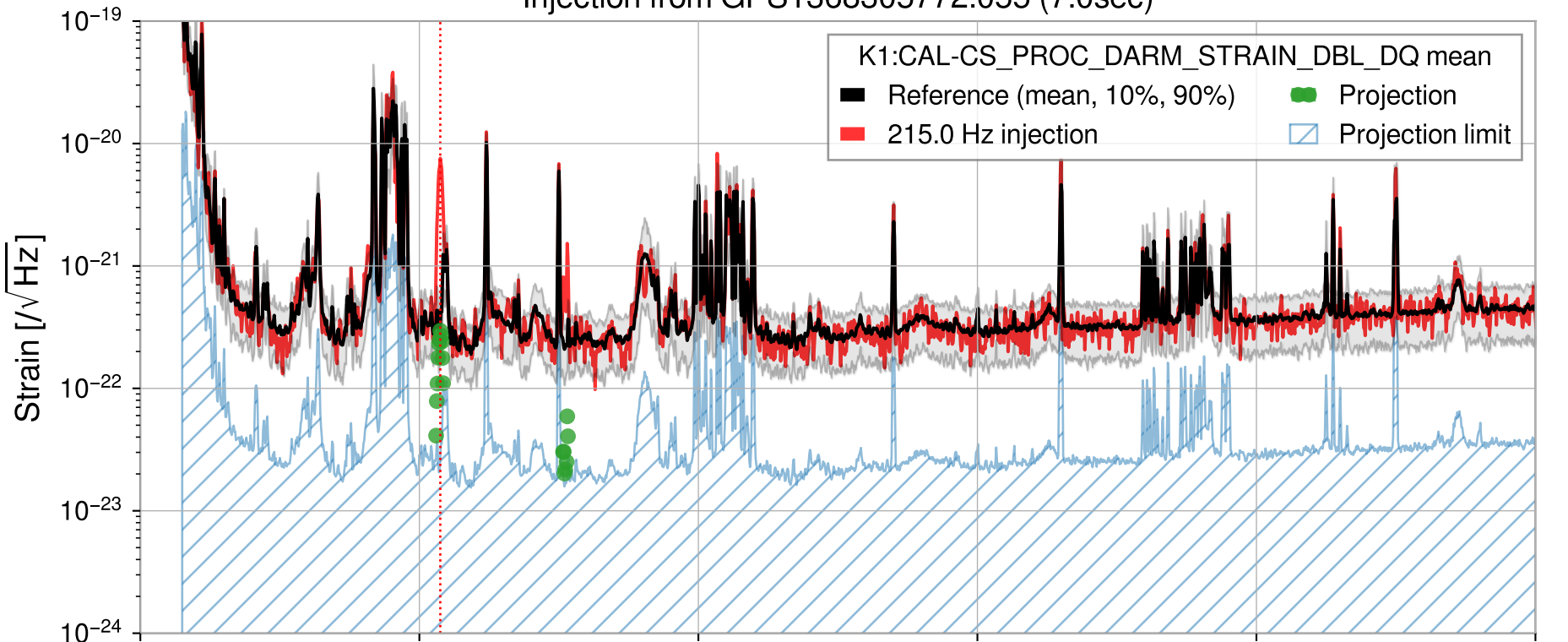
Injection from GPS1368305772.055 (7.0sec)
