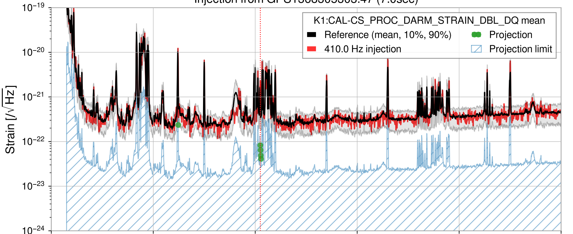
Injection from GPS1368305303.47 (7.0sec)
