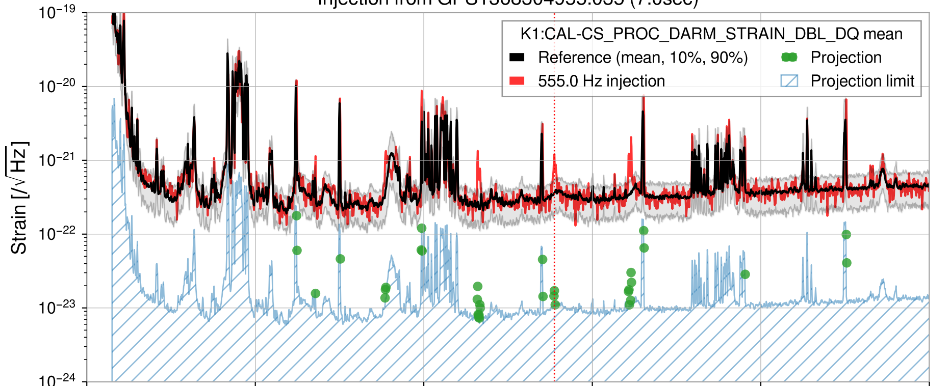
Injection from GPS1368304955.035 (7.0sec)
