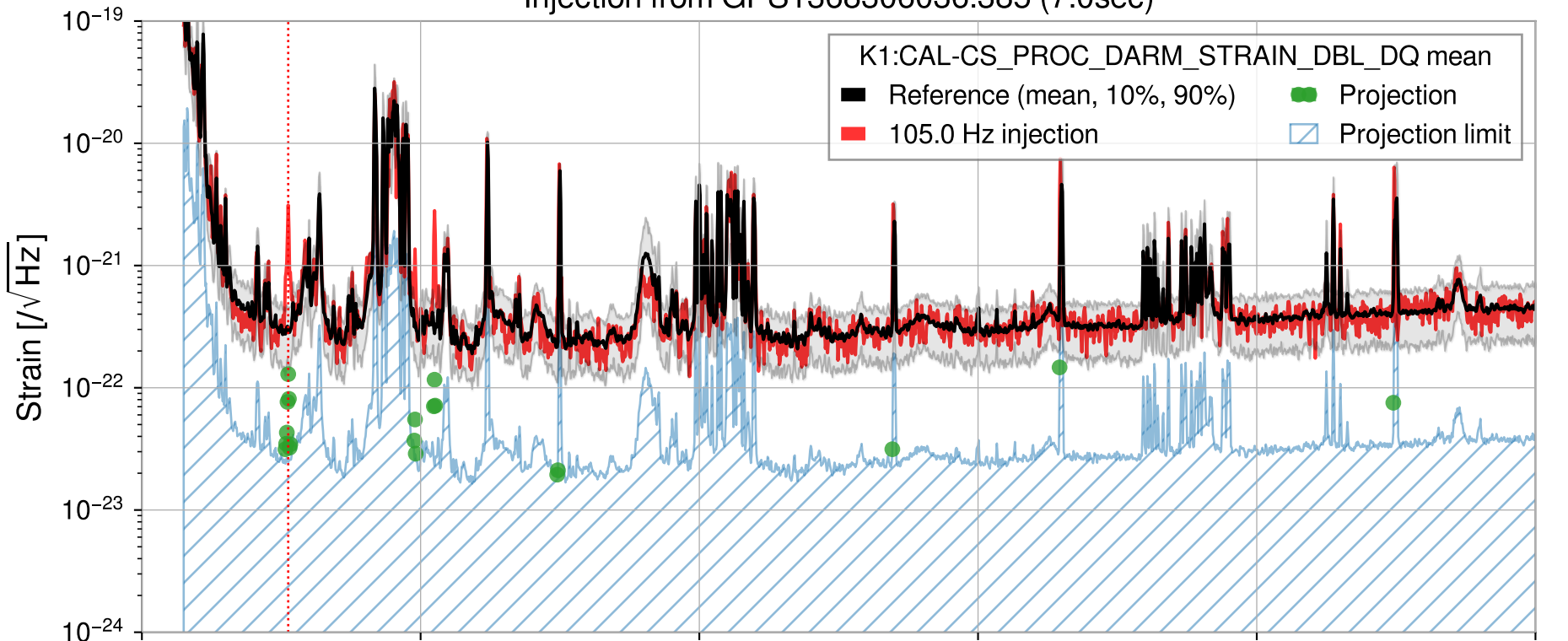
Injection from GPS1368306036.385 (7.0sec)
