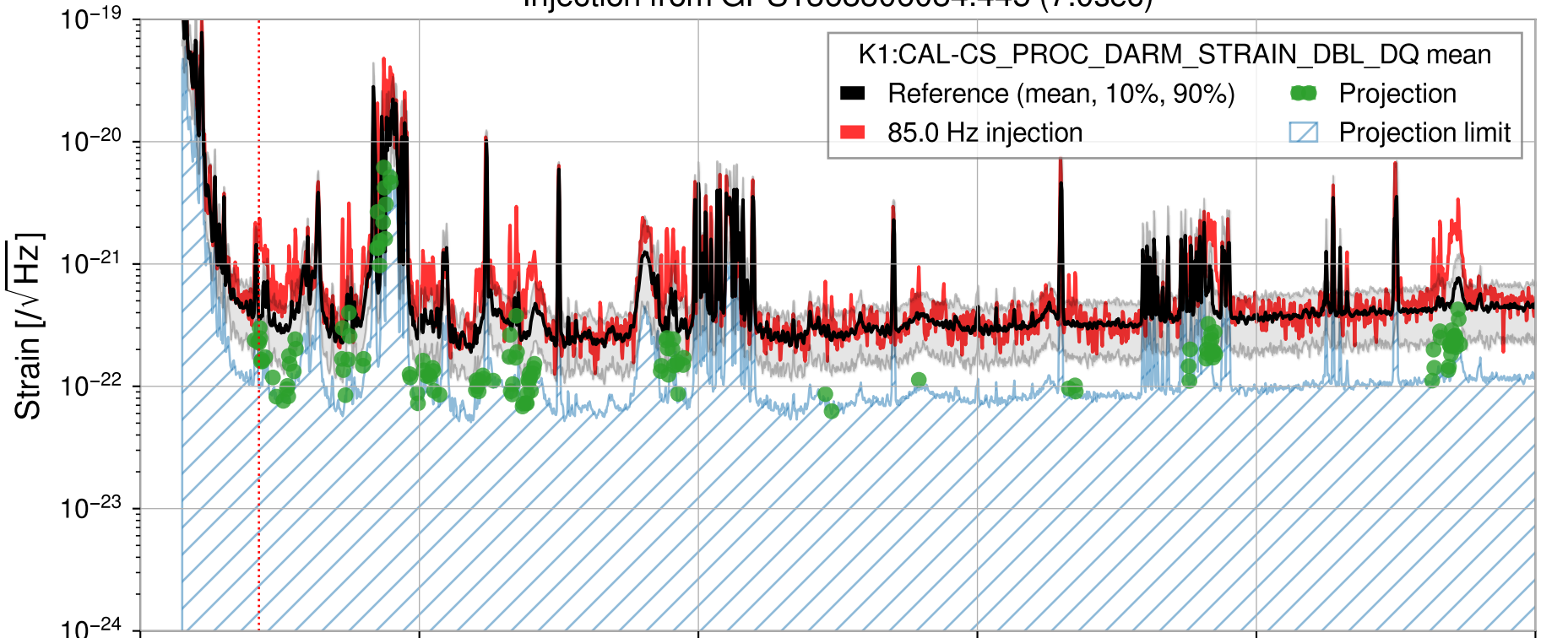
Injection from GPS1368306084.445 (7.0sec)
