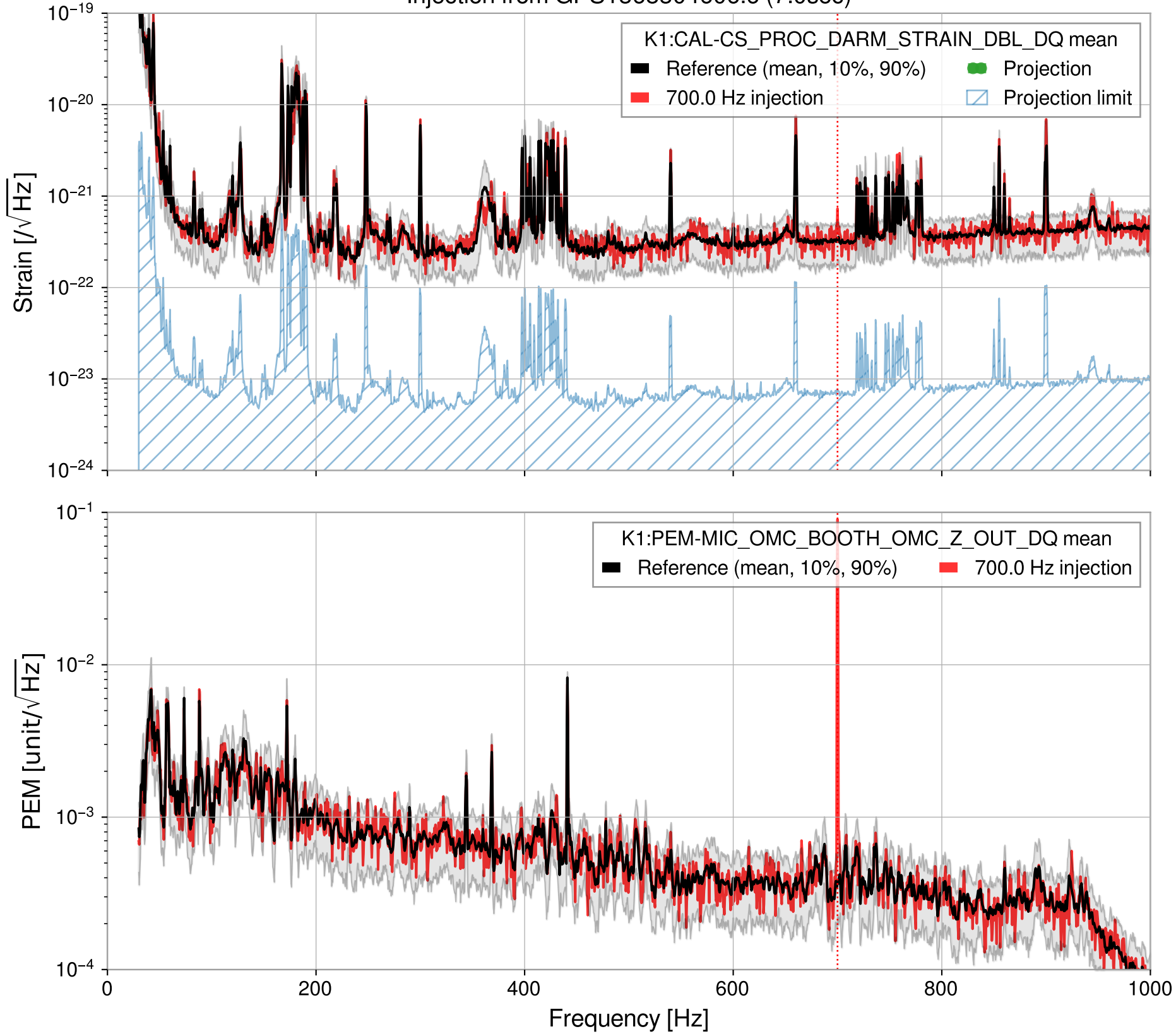
Injection from GPS1368304606.6 (7.0sec)
