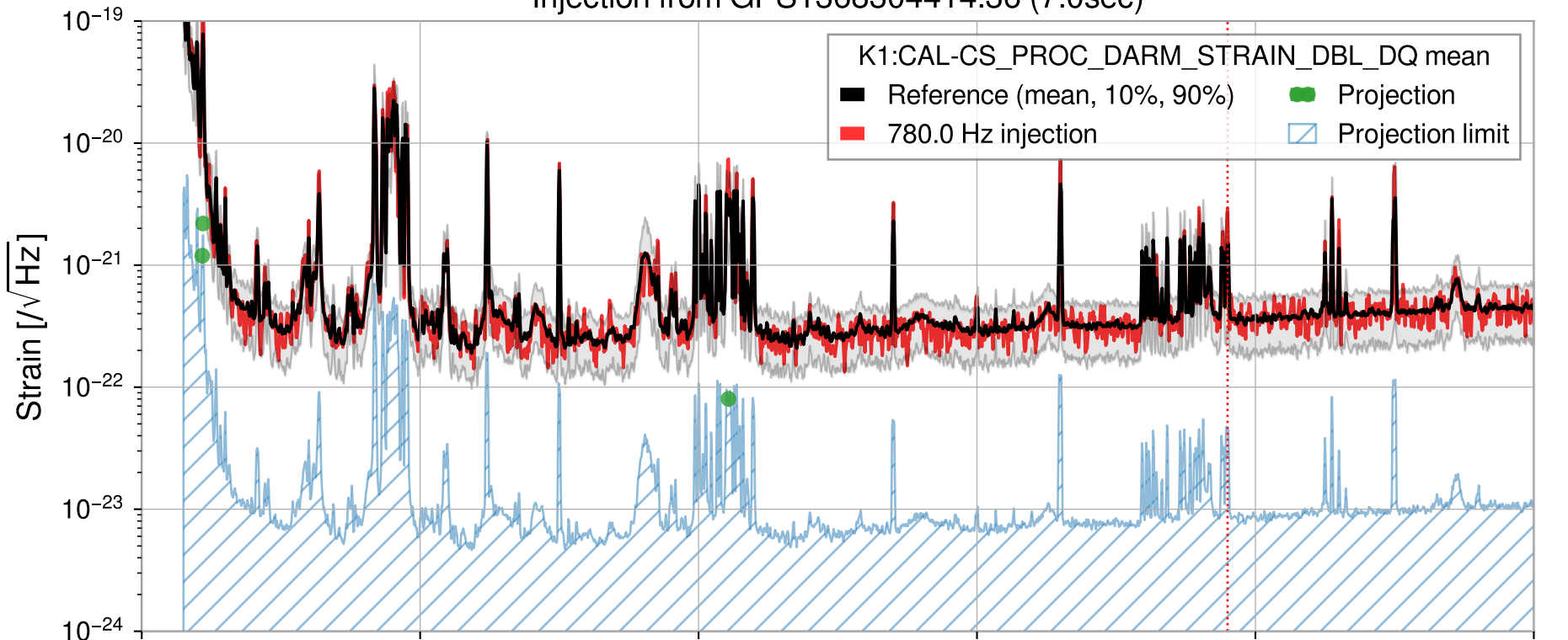
Injection from GPS1368304414.36 (7.0sec)
