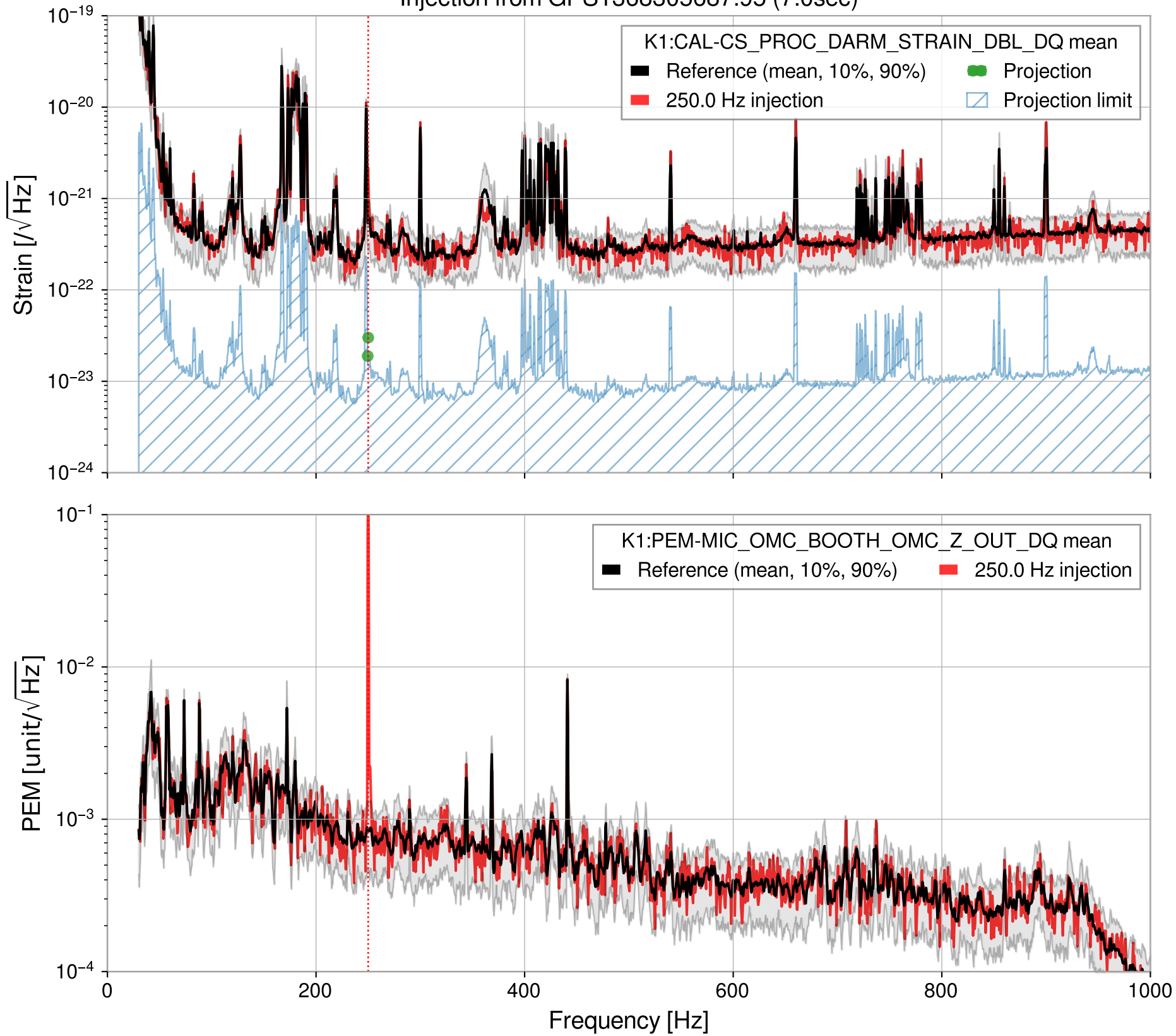
Injection from GPS1368305687.95 (7.0sec)
