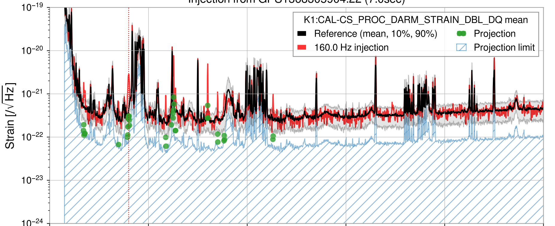
Injection from GPS1368305904.22 (7.0sec)
