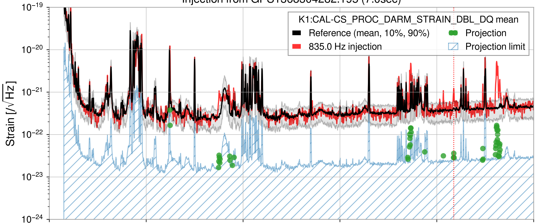
Injection from GPS1368304282.195 (7.0sec)
