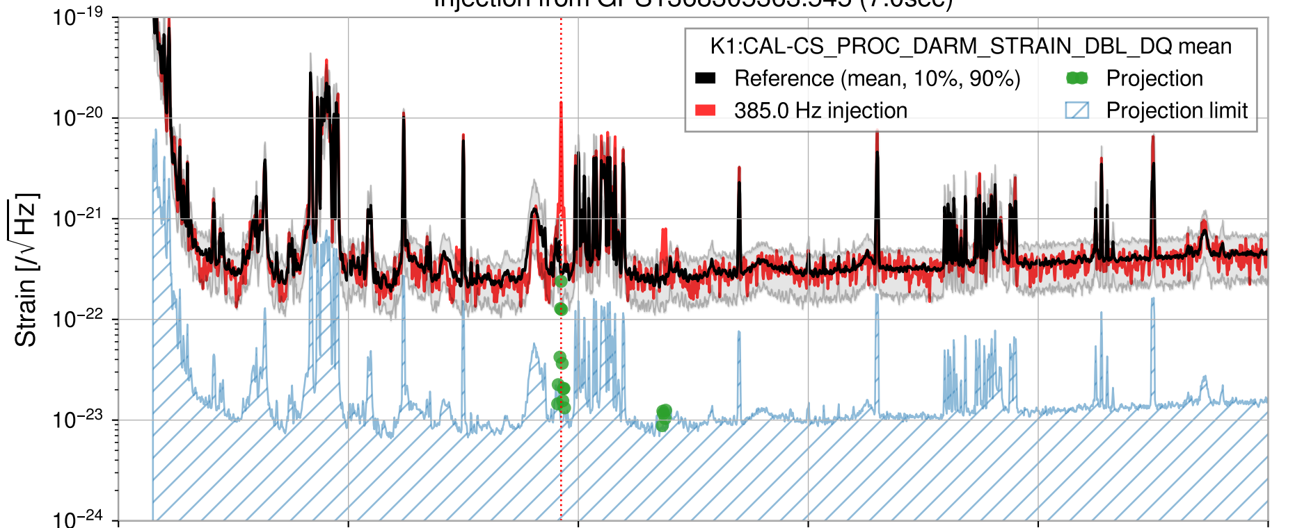
Injection from GPS1368305363.545 (7.0sec)
