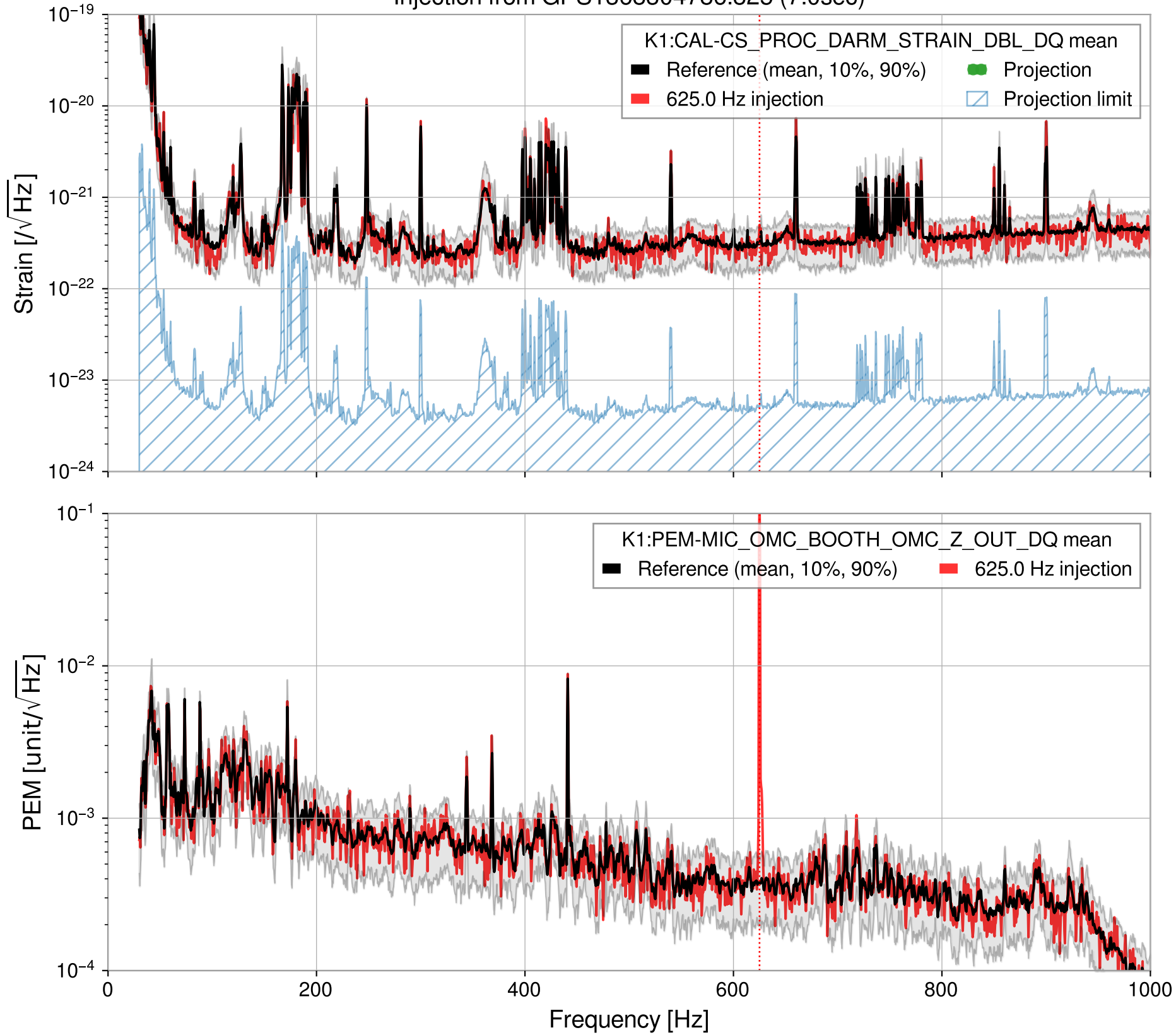
Injection from GPS1368304786.825 (7.0sec)
