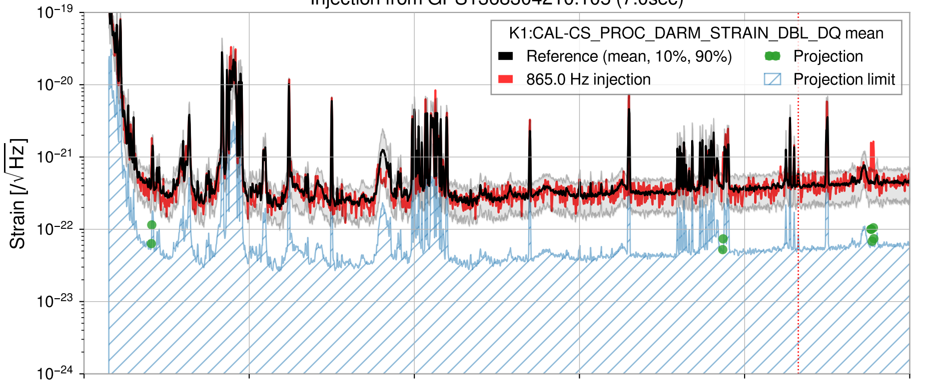
Injection from GPS1368304210.105 (7.0sec)
