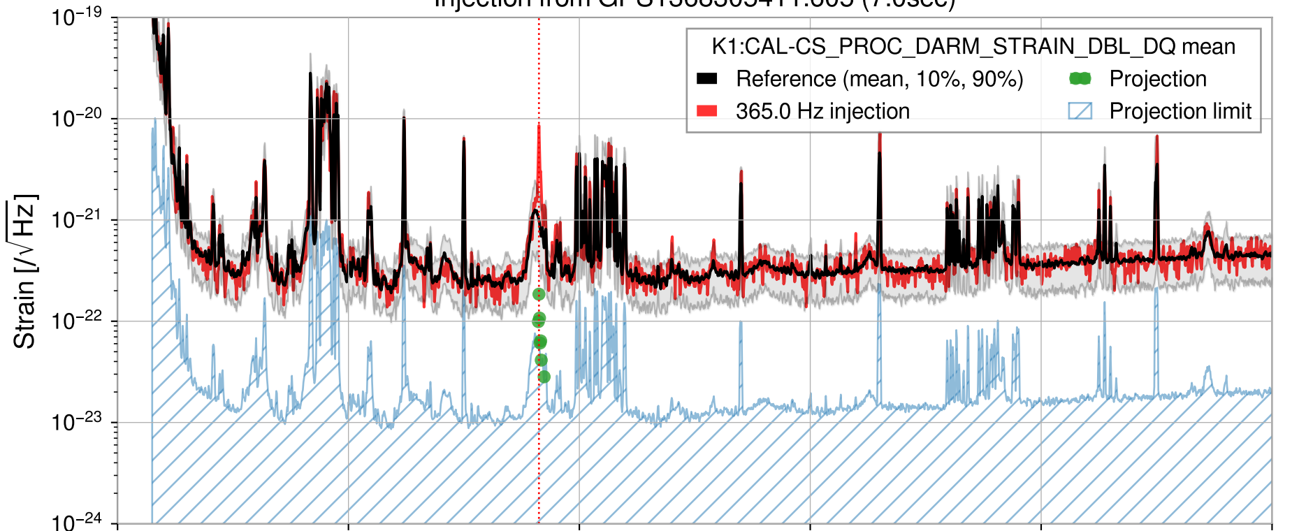
Injection from GPS1368305411.605 (7.0sec)
