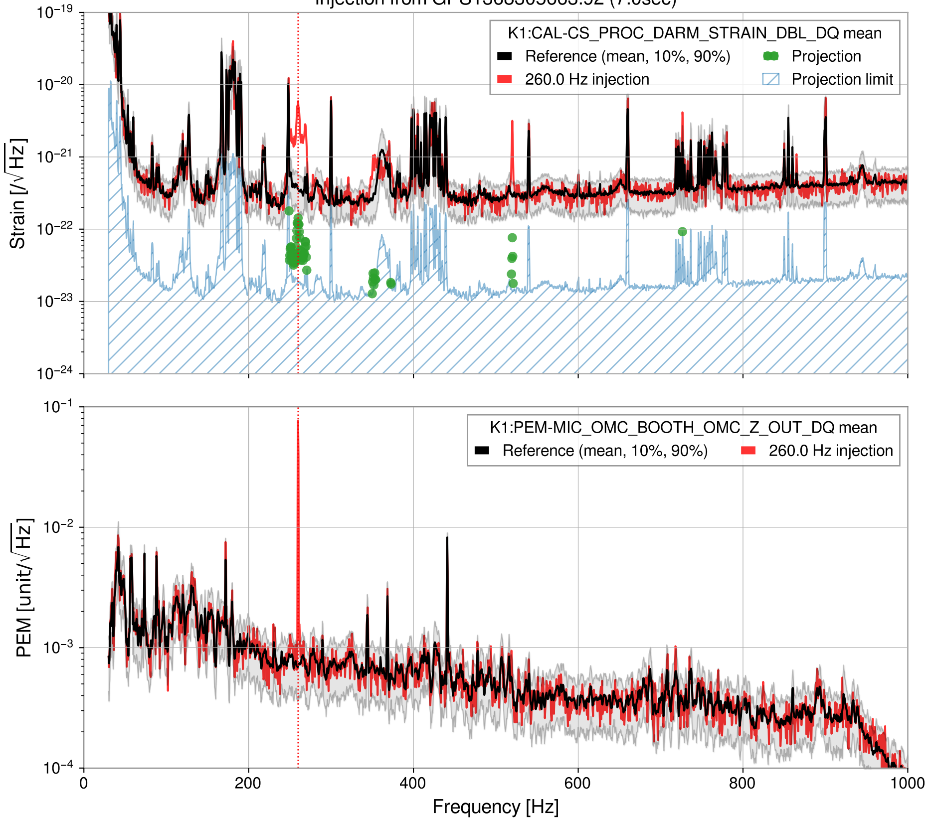
Injection from GPS1368305663.92 (7.0sec)
