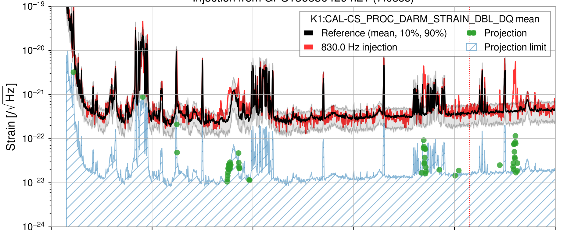
Injection from GPS1368304294.21 (7.0sec)
