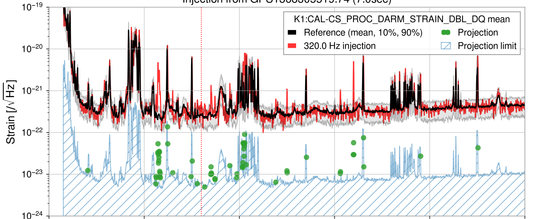
Injection from GPS1368305519.74 (7.0sec)
