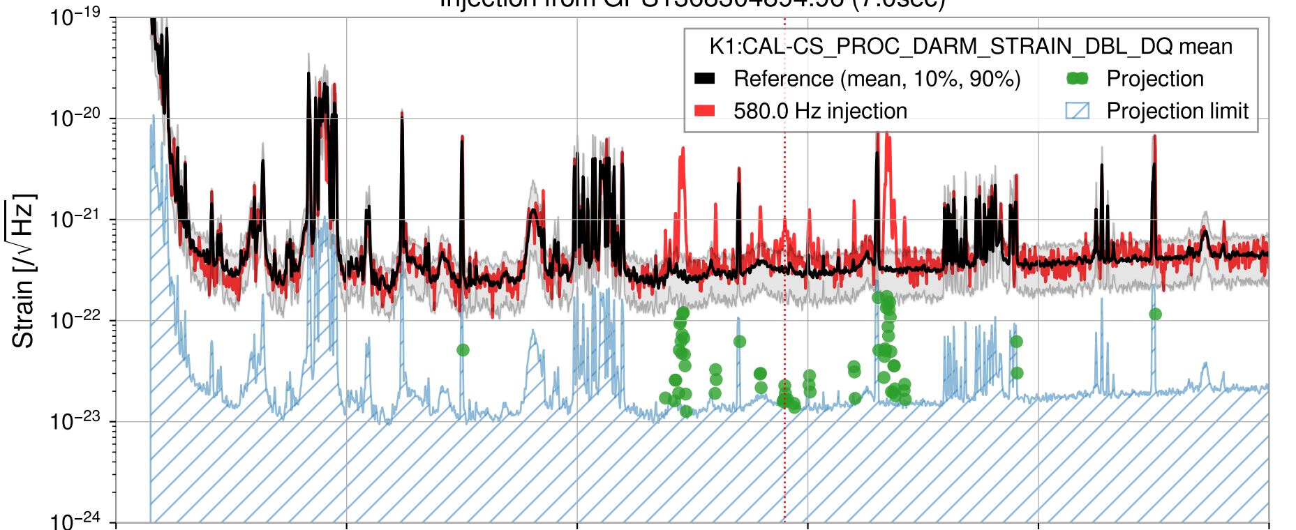
Injection from GPS1368304894.96 (7.0sec)
