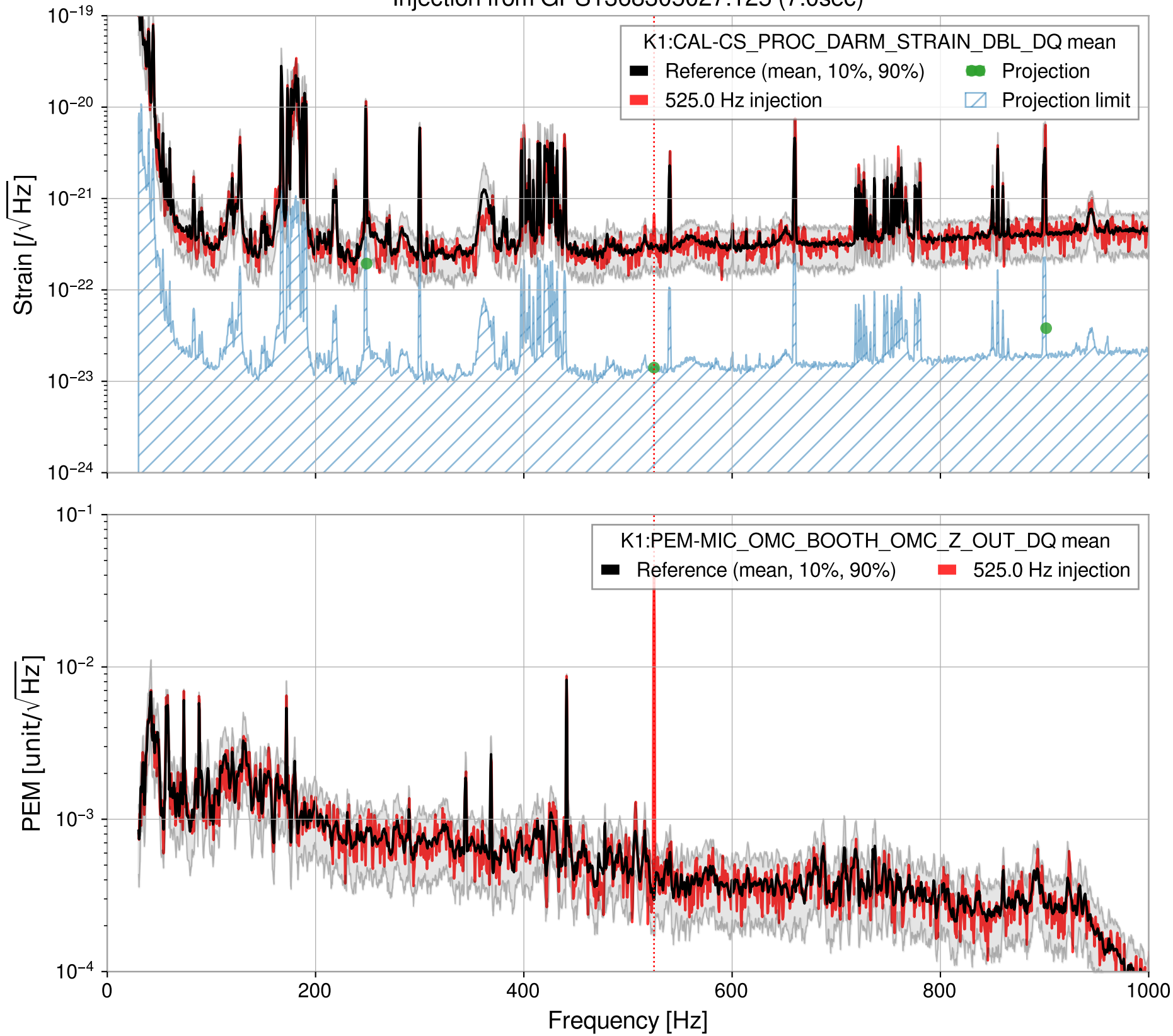
Injection from GPS1368305027.125 (7.0sec)
