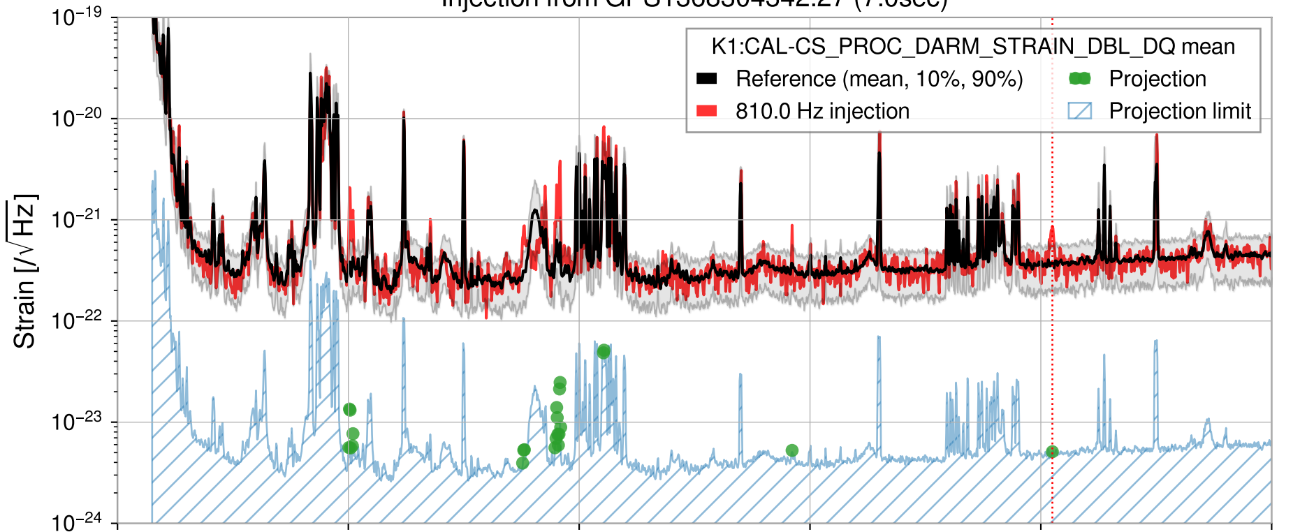
Injection from GPS1368304342.27 (7.0sec)
