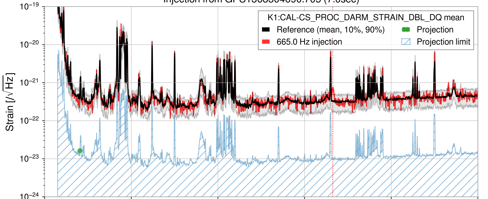
Injection from GPS1368304690.705 (7.0sec)
