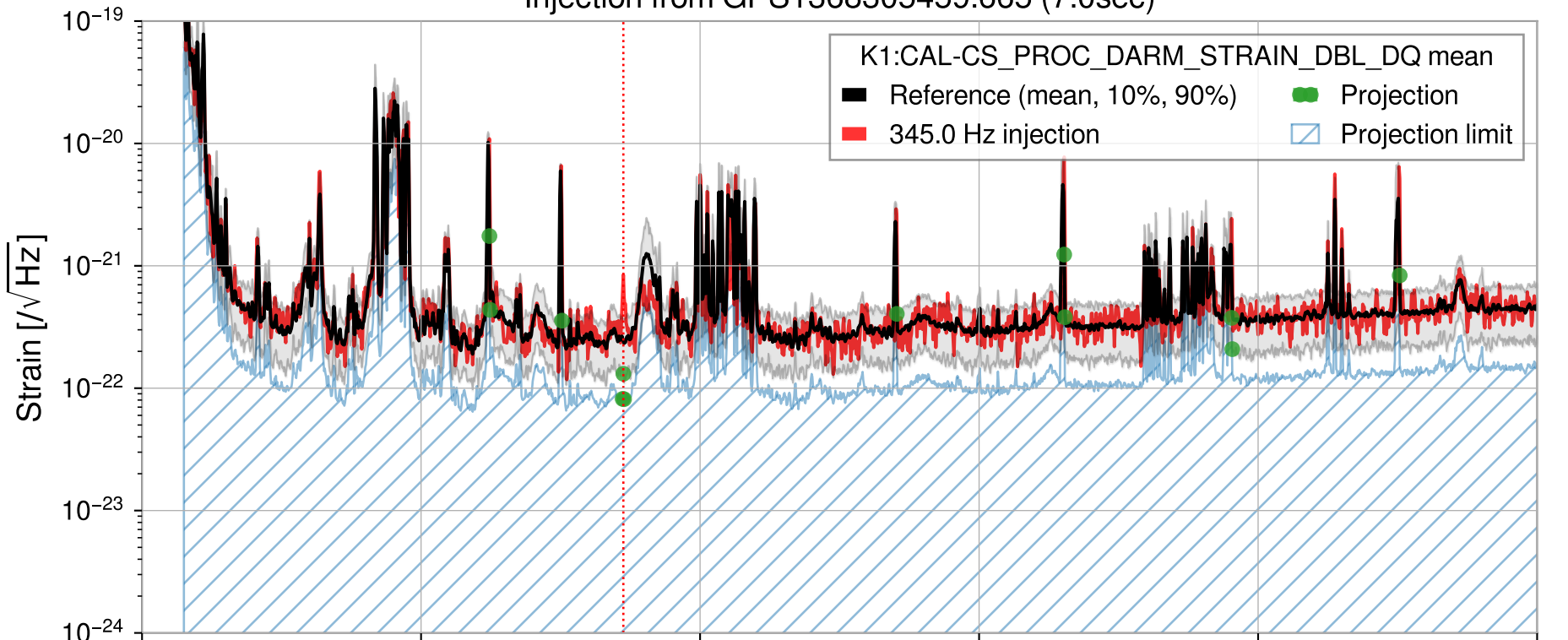
Injection from GPS1368305459.665 (7.0sec)
