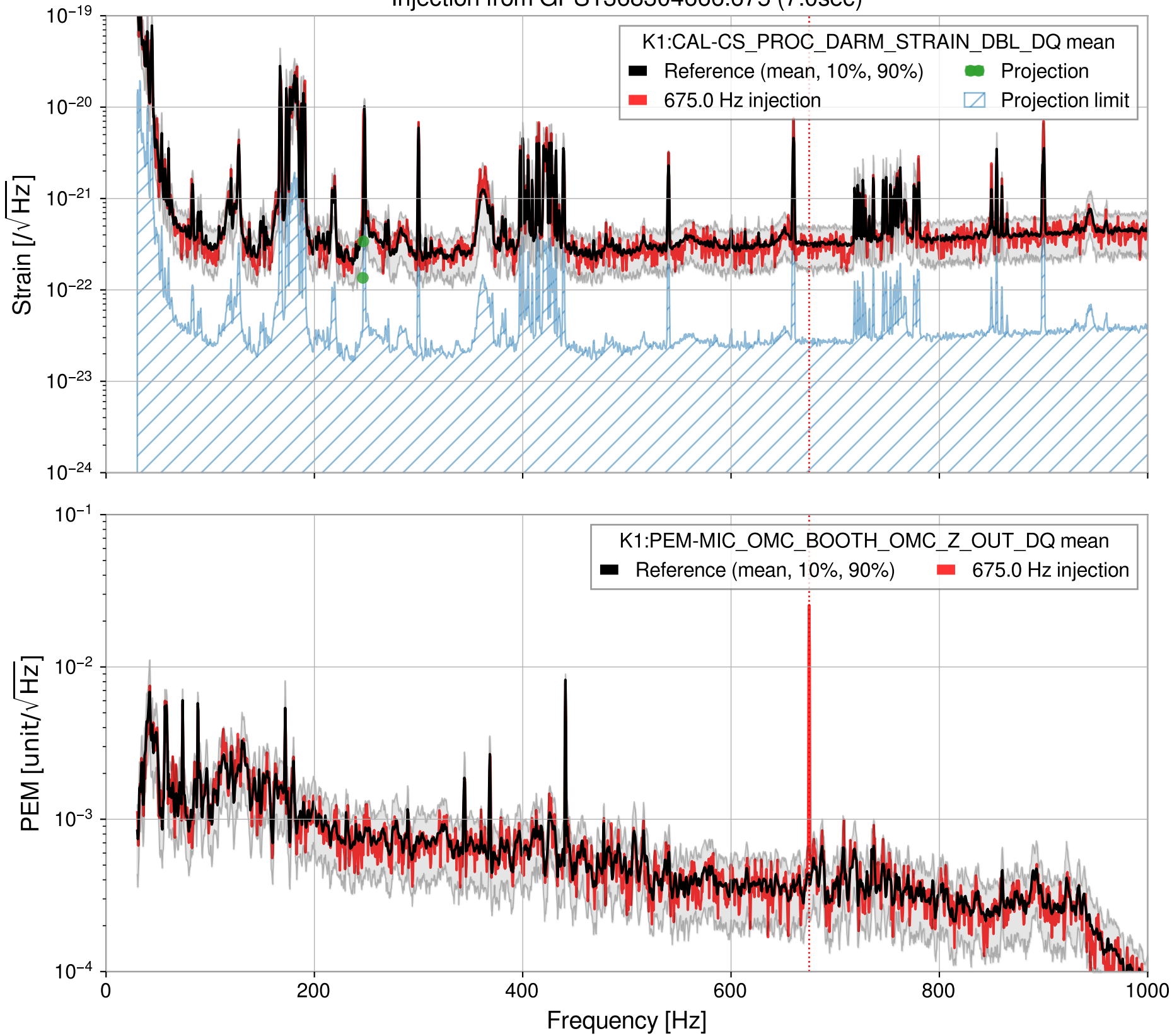
Injection from GPS1368304666.675 (7.0sec)
