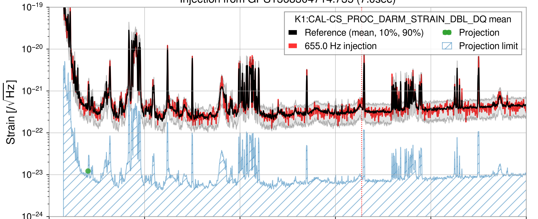
Injection from GPS1368304714.735 (7.0sec)
