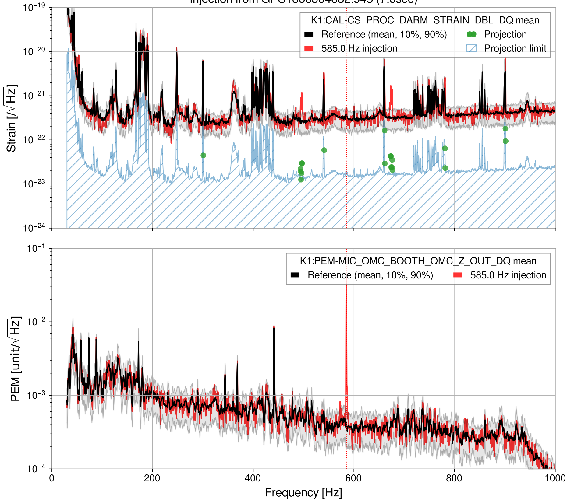
Injection from GPS136830482.945 (7.0sec)
