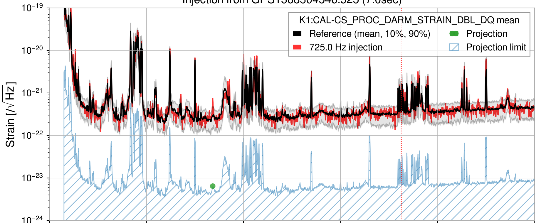
Injection from GPS1368304546.525 (7.0sec)
