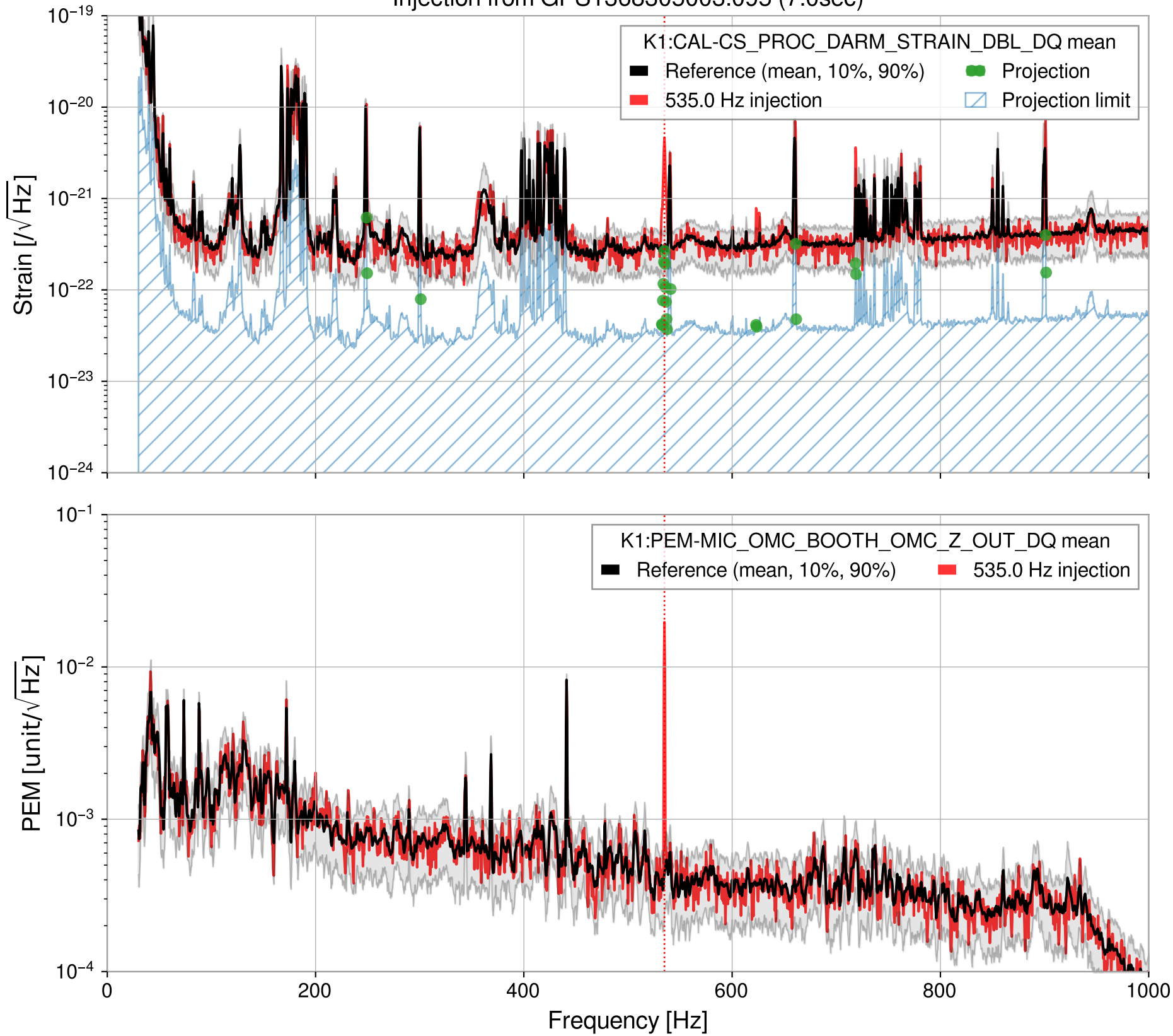
Injection from GPS1368305003.095 (7.0sec)
