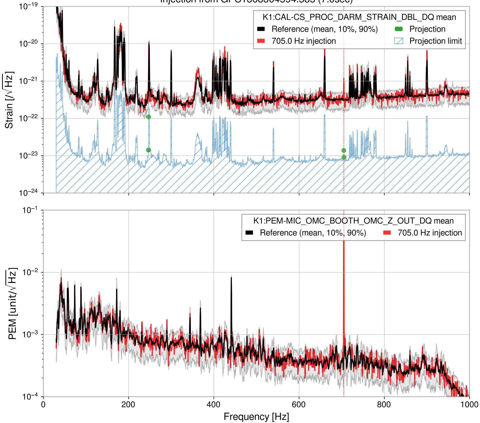
Injection from GPS1368304594.585 (7.0sec)
