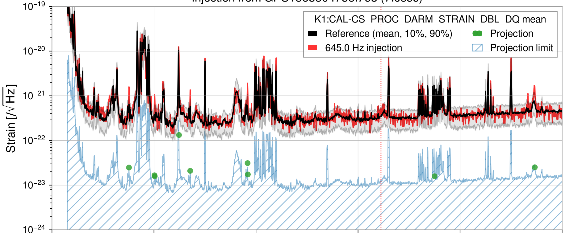
Injection from GPS1368304738.765 (7.0sec)
