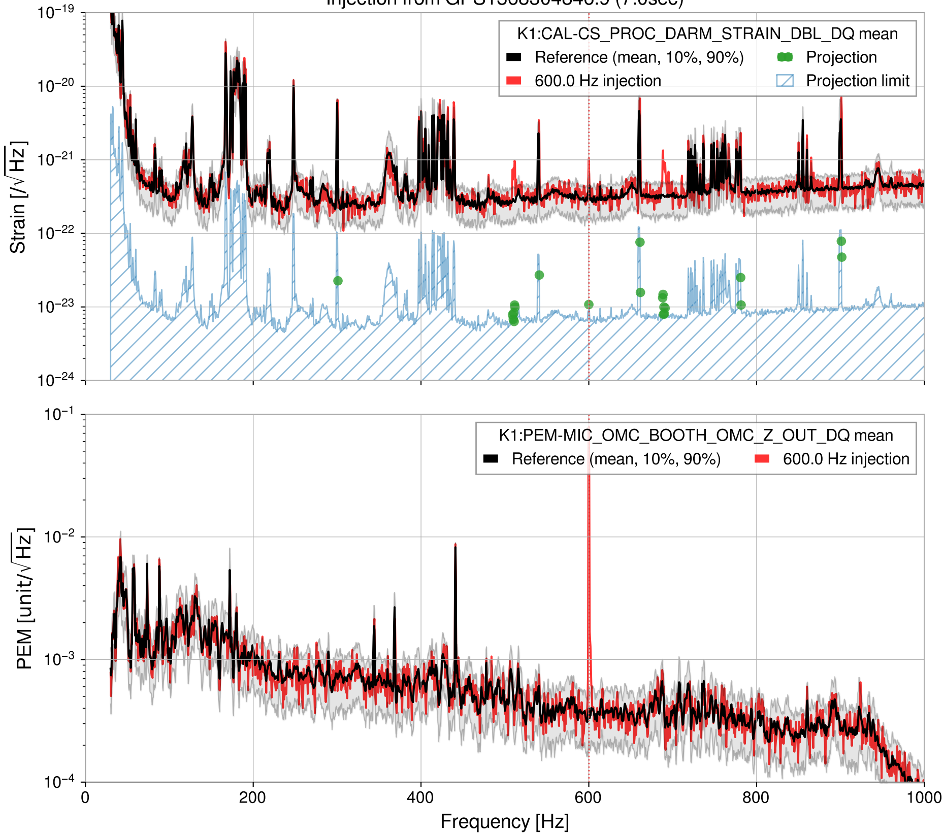
Injection from GPS1368304846.9 (7.0sec)
