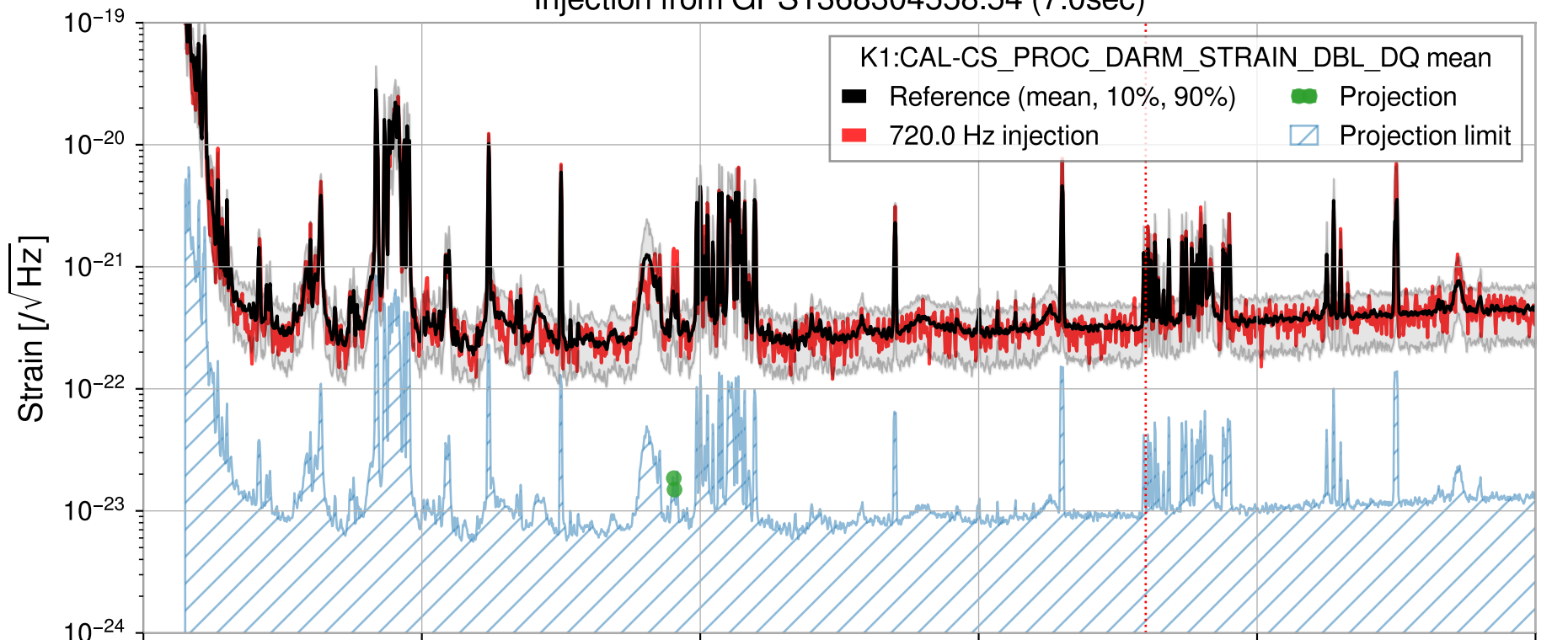
Injection from GPS1368304558.54 (7.0sec)
