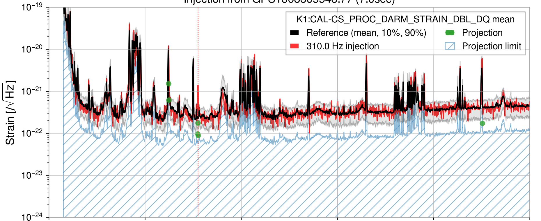
Injection from GPS1368305543.77 (7.0sec)
