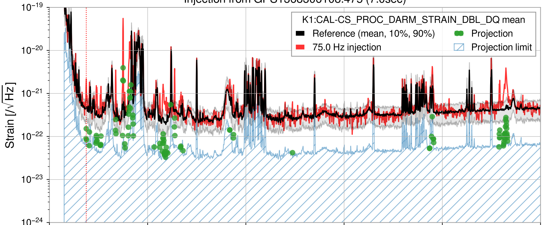
Injection from GPS1368306108.475 (7.0sec)
