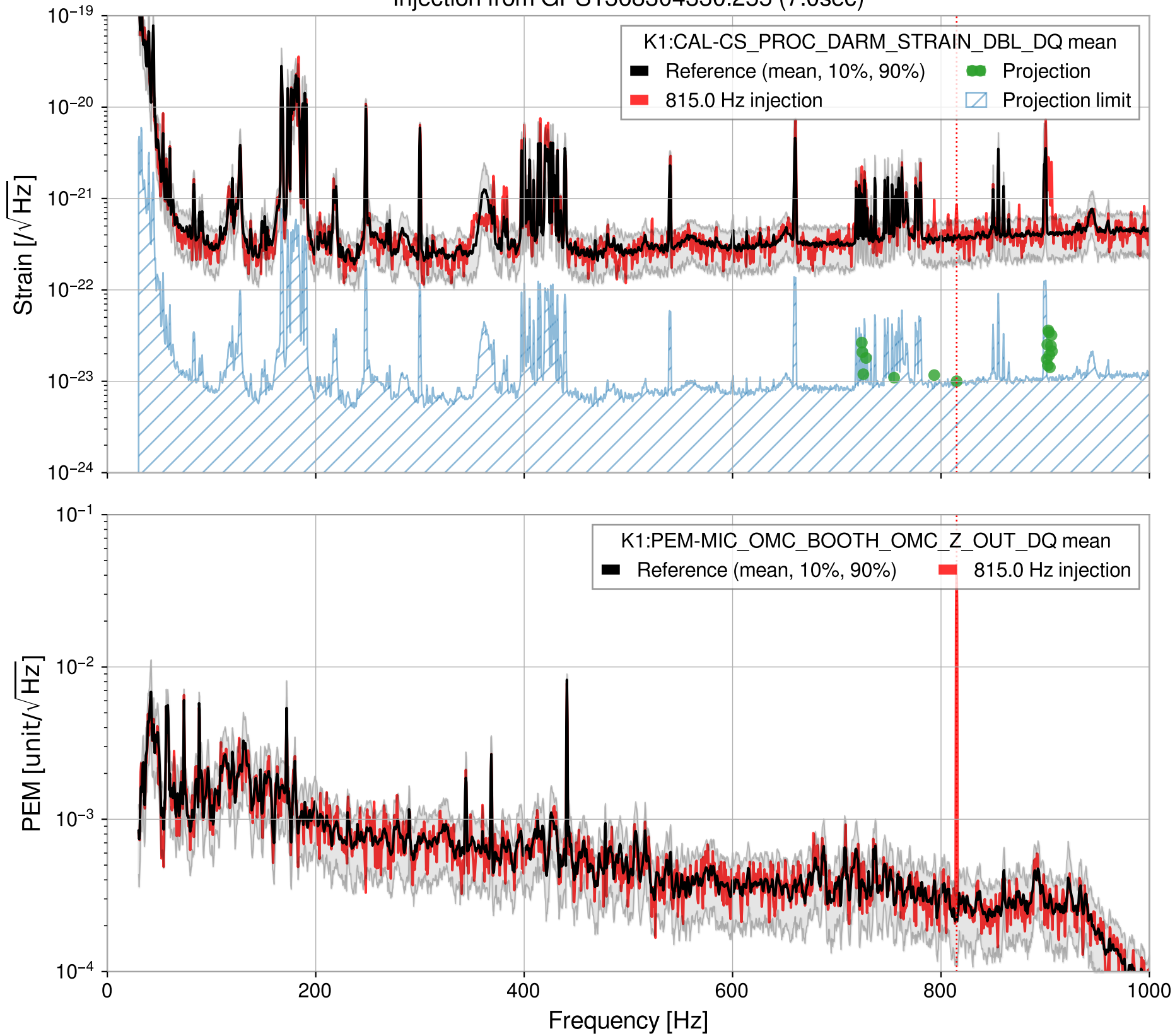
Injection from GPS1368304330.255 (7.0sec)
