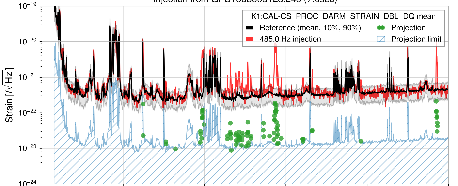
Injection from GPS1368305123.245 (7.0sec)
