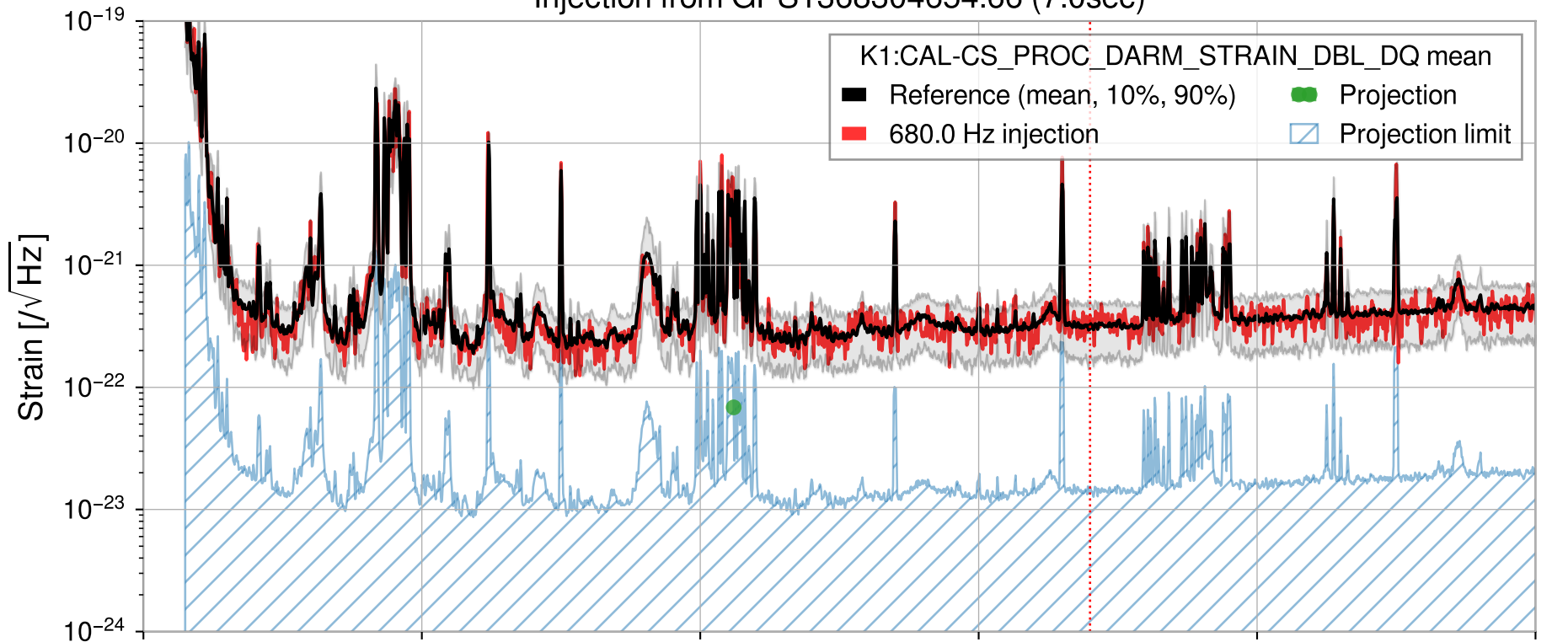
Injection from GPS1368304654.66 (7.0sec)
