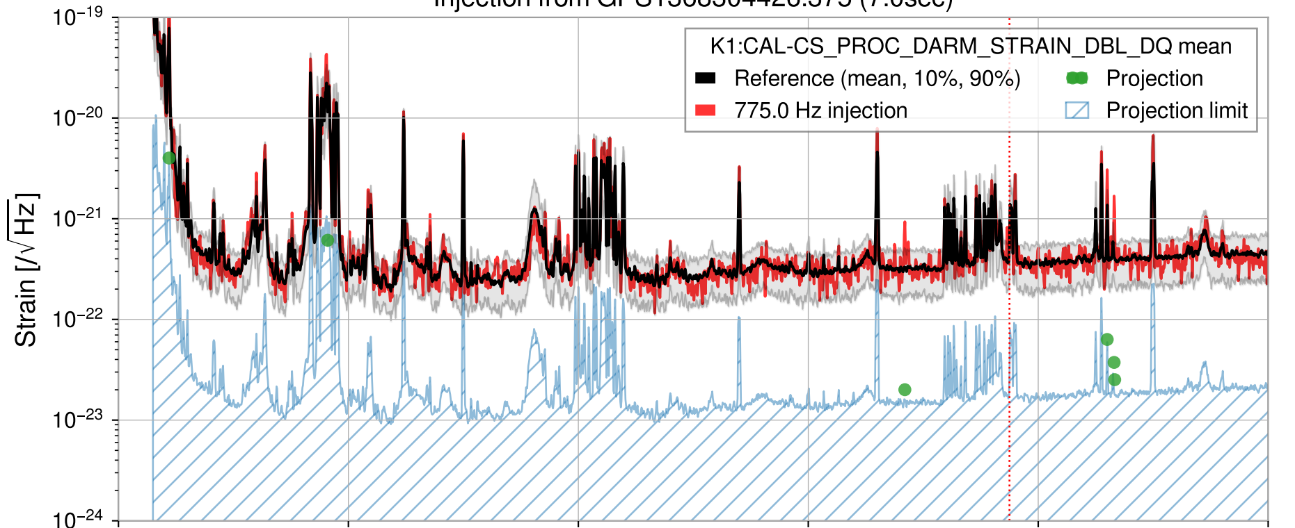
Injection from GPS1368304426.375 (7.0sec)
