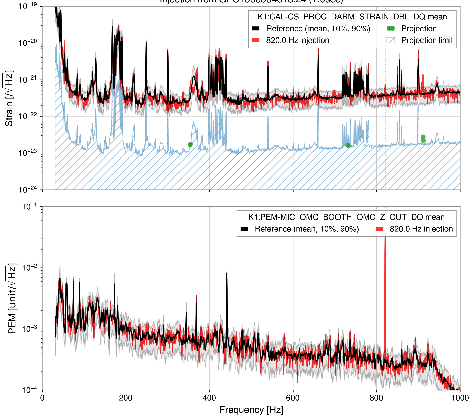
Injection from GPS1368304318.24 (7.0sec)
