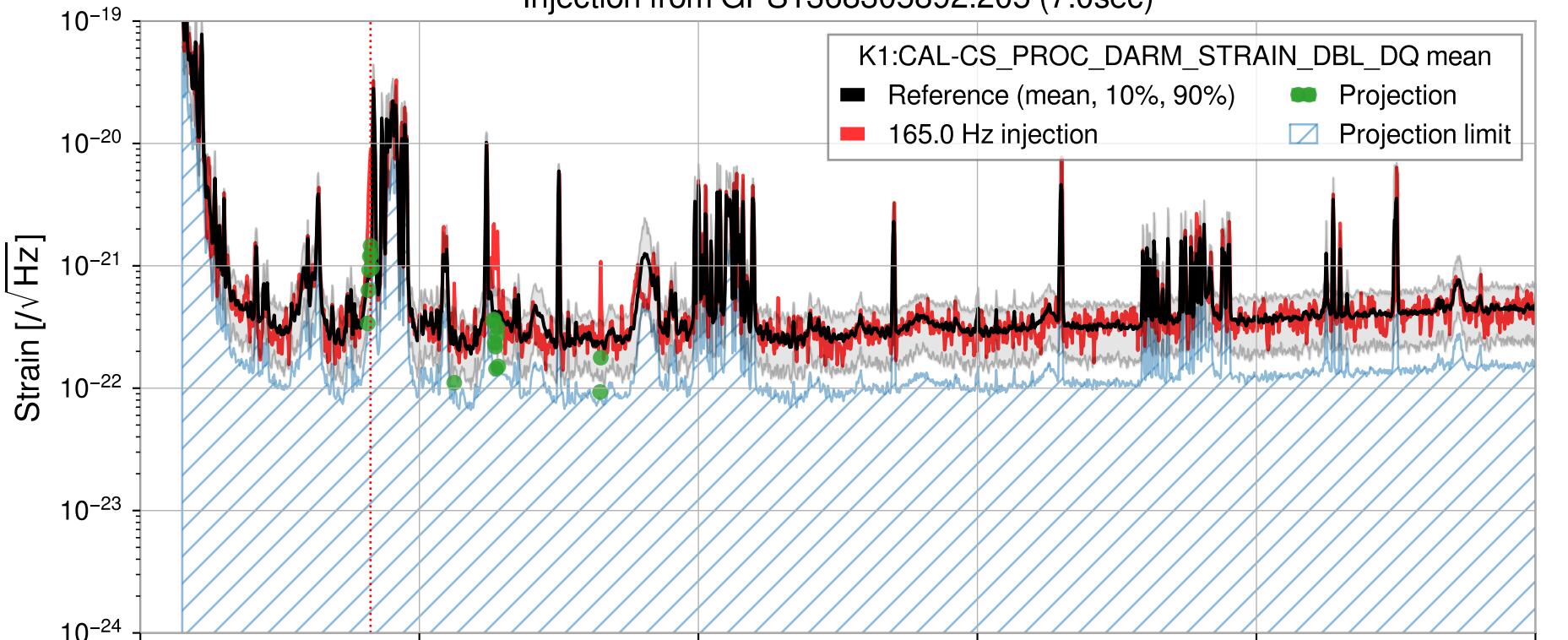
Injection from GPS1368305892.205 (7.0sec)
