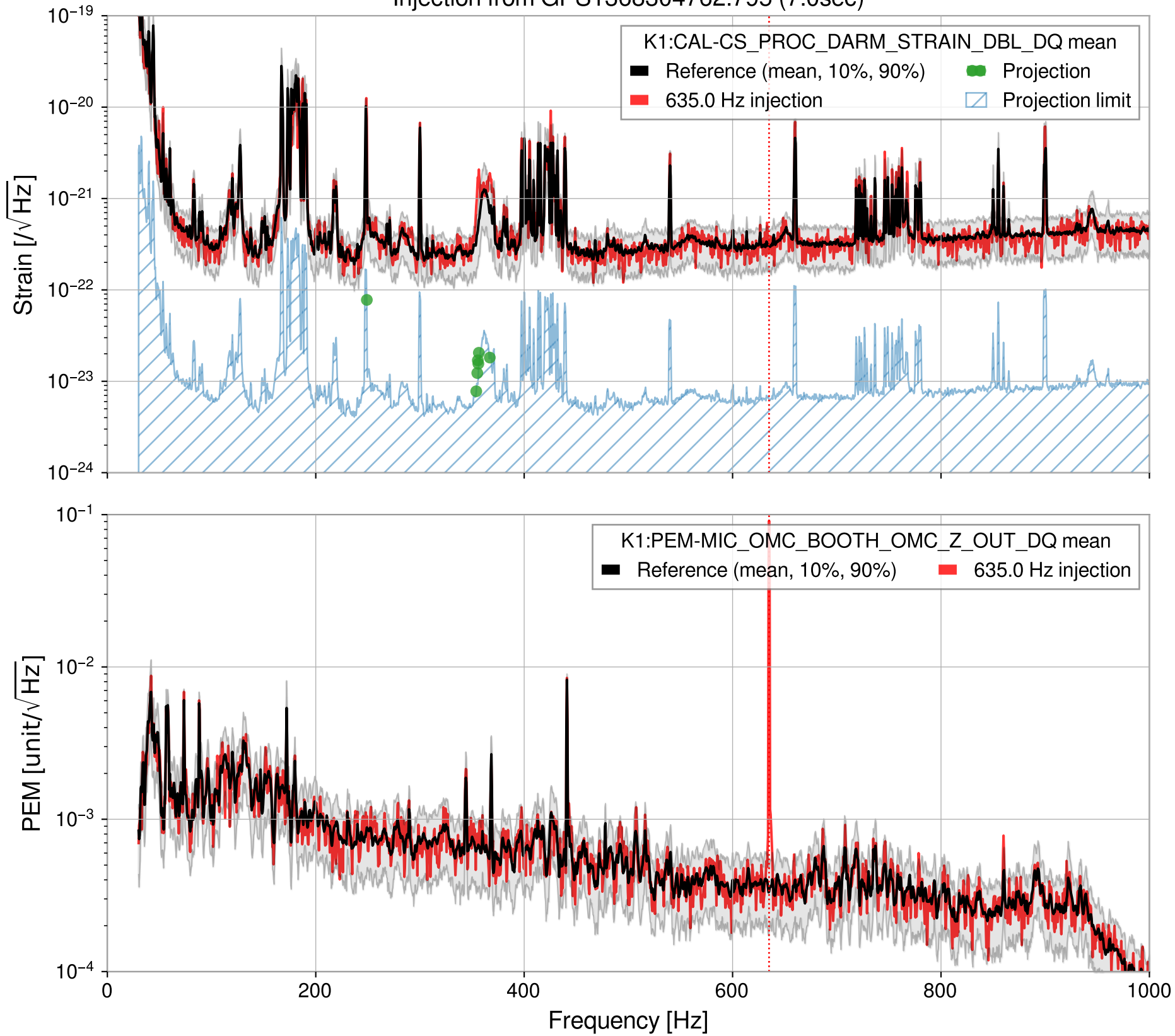
Injection from GPS1368304762.795 (7.0sec)
