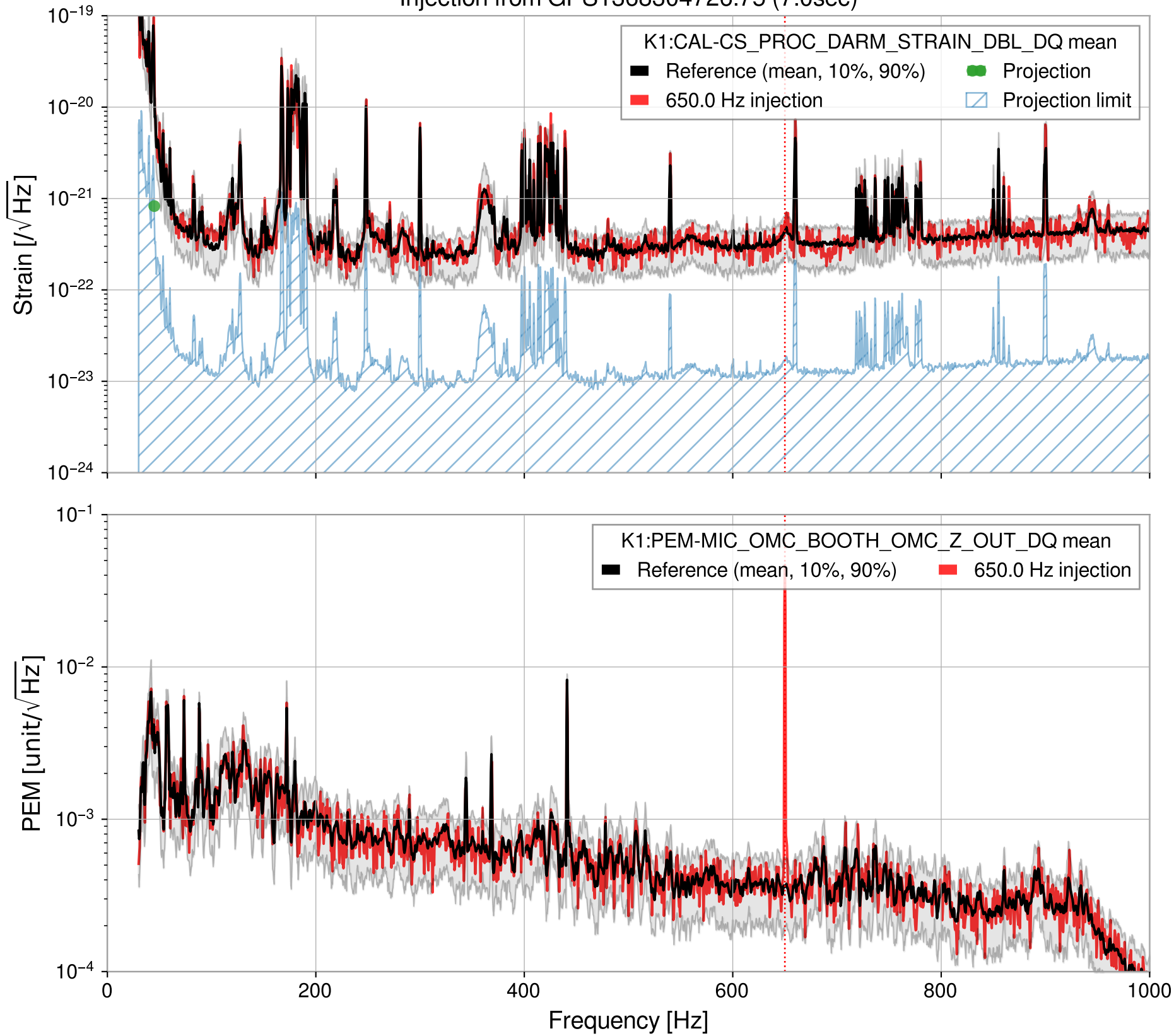
Injection from GPS1368304726.75 (7.0sec)
