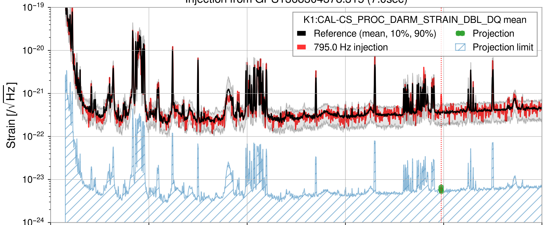
Injection from GPS1368304378.315 (7.0sec)
