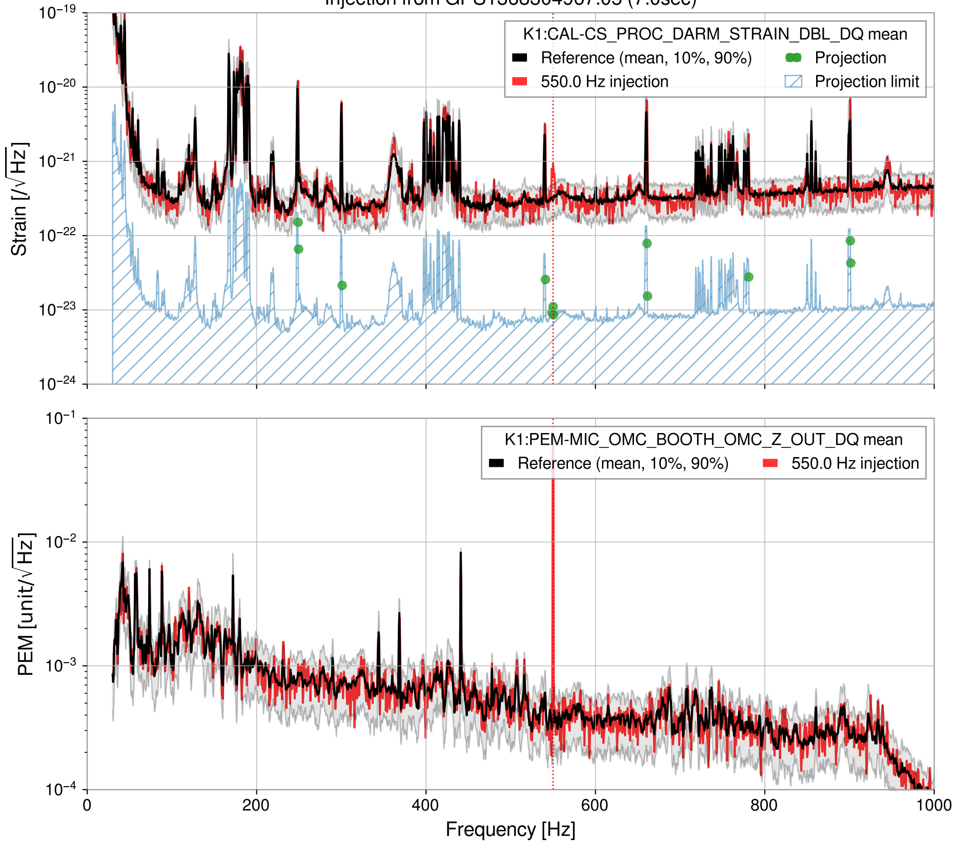
Injection from GPS1368304967.05 (7.0sec)
