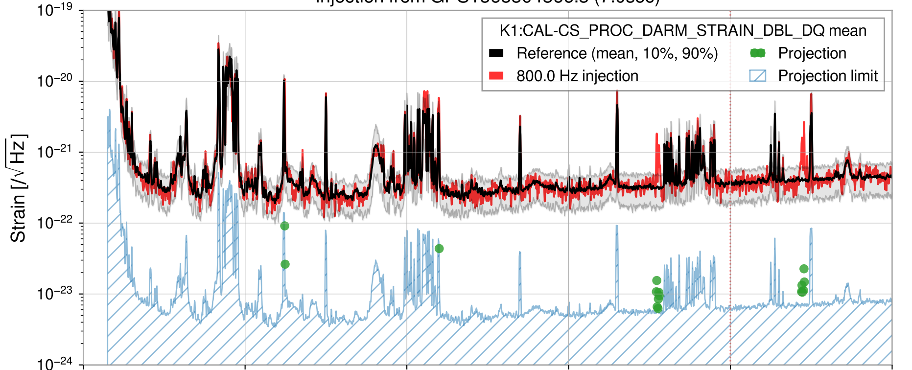
Injection from GPS1368304366.3 (7.0sec)
