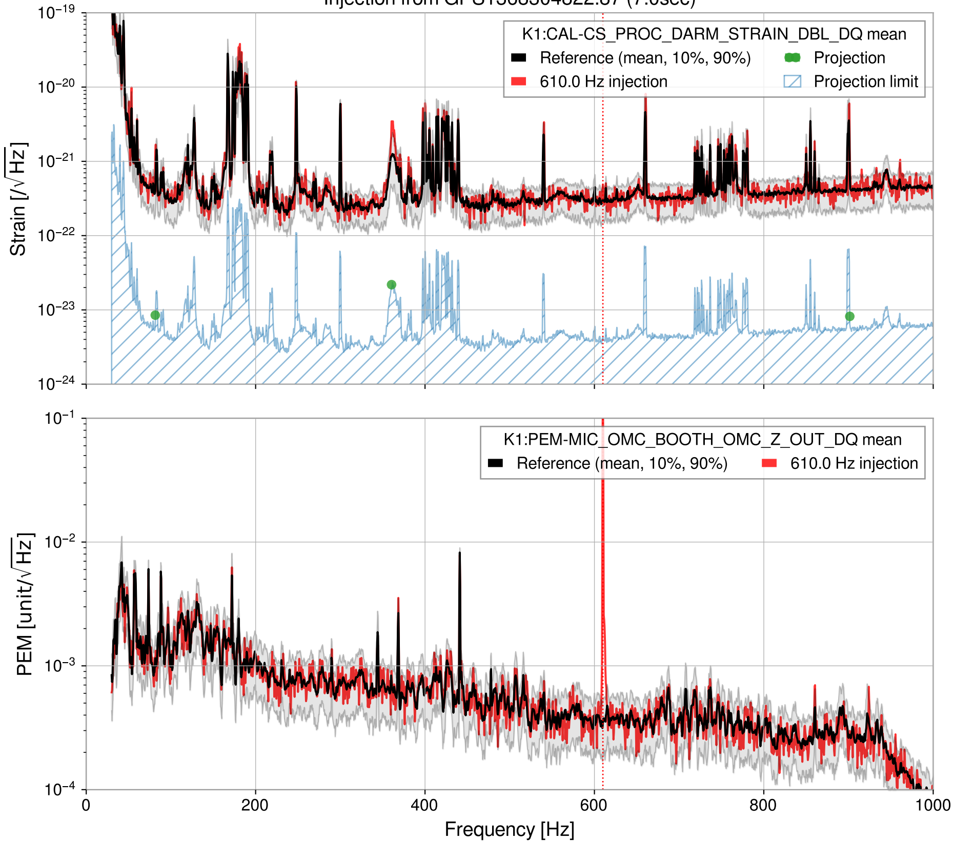
Injection from GPS1368304822.87 (7.0sec)
