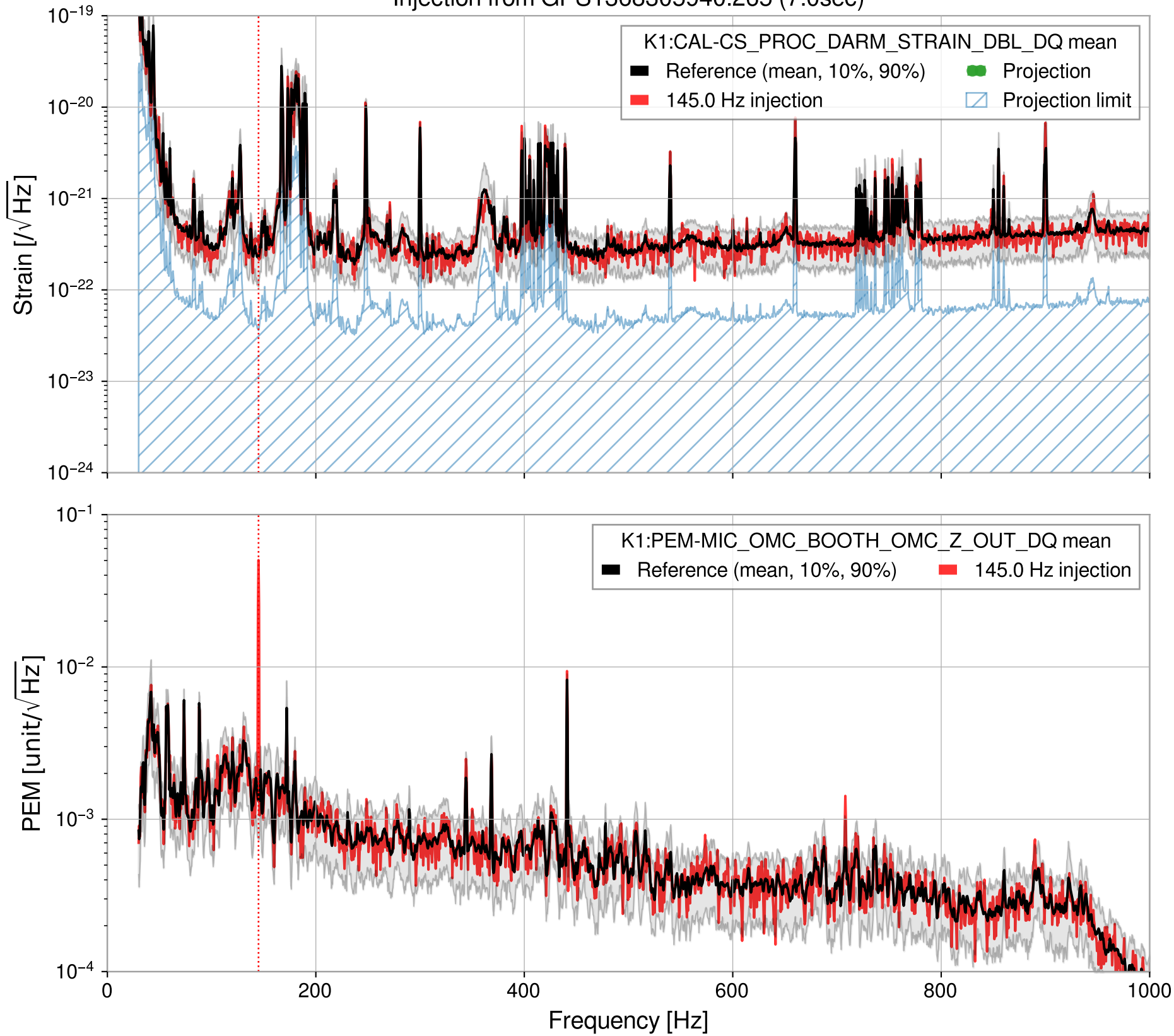
Injection from GPS1368305940.265 (7.0sec)
