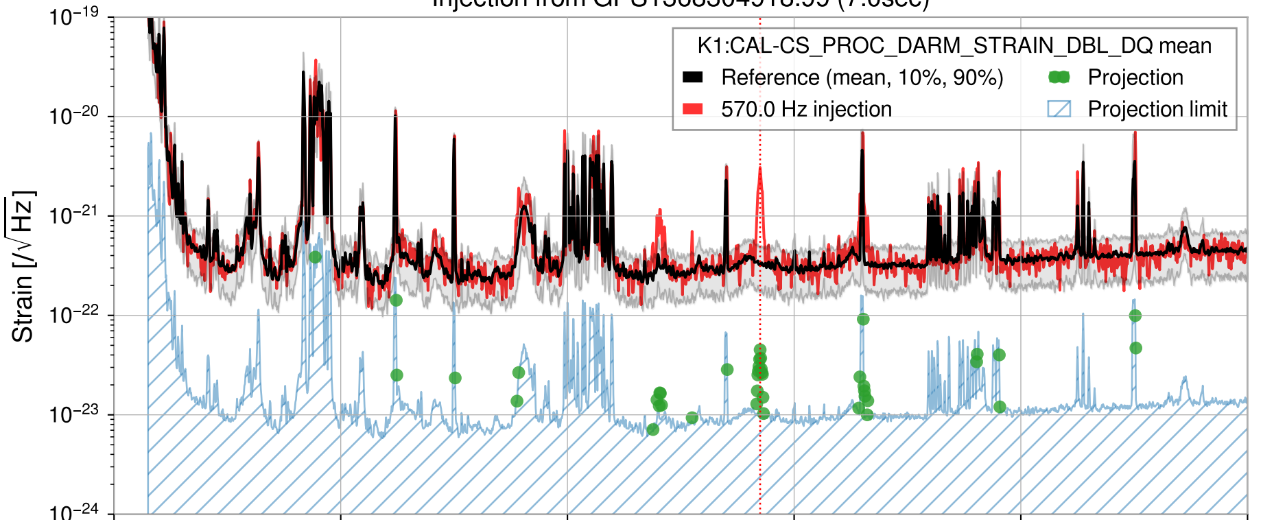
Injection from GPS1368304918.99 (7.0sec)
