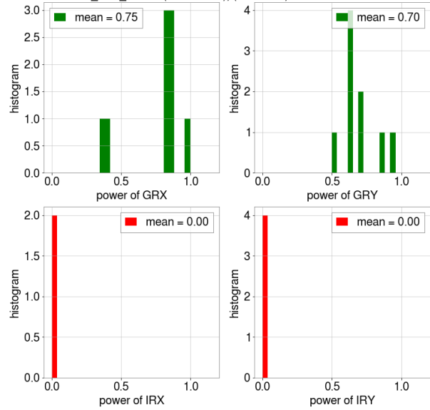
ckloss from ENGAGE_ALS_DARM (state = 210), (n=9/1129)
