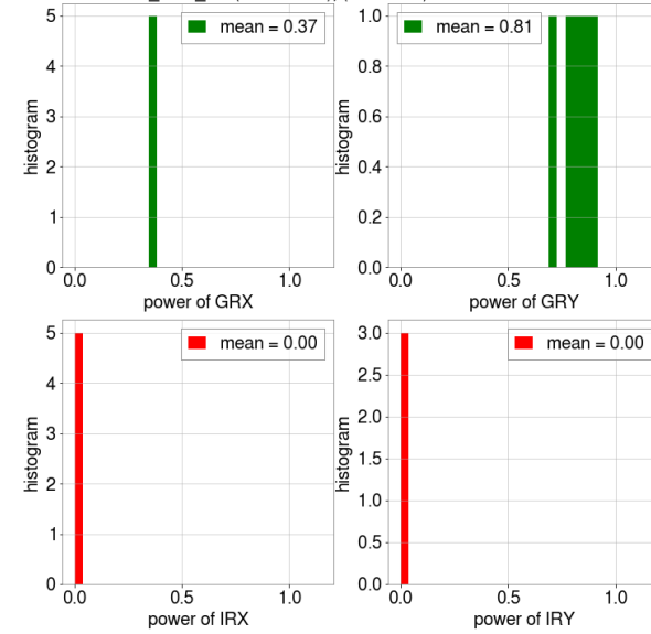
lockloss from ENGAGE_FNC_XY (state = 205), (n=5/1129)
