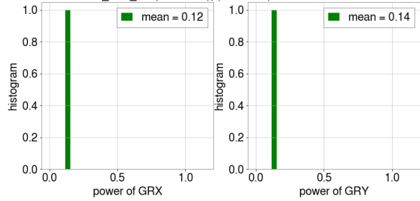
lockloss from LOCKING_ALS_XY (state = 10), (n=1/1129)
