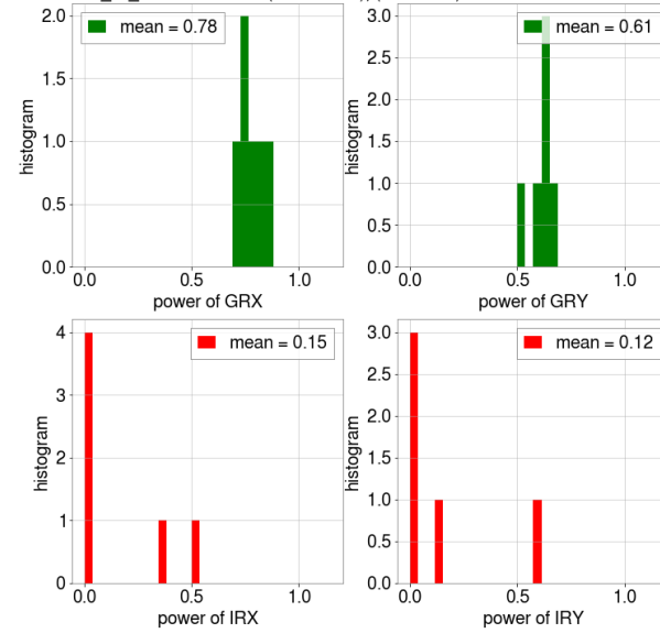
kloss from FIND_IR_RESONANCES (state = 305), (n=6/1129)
