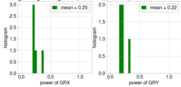
loss from SET_LASER_POWER_NORM (state = 105), (n=5/1129)
