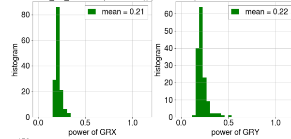
lockloss from ALS_XY_LOCKED (state = 100), (n=145/1129)
