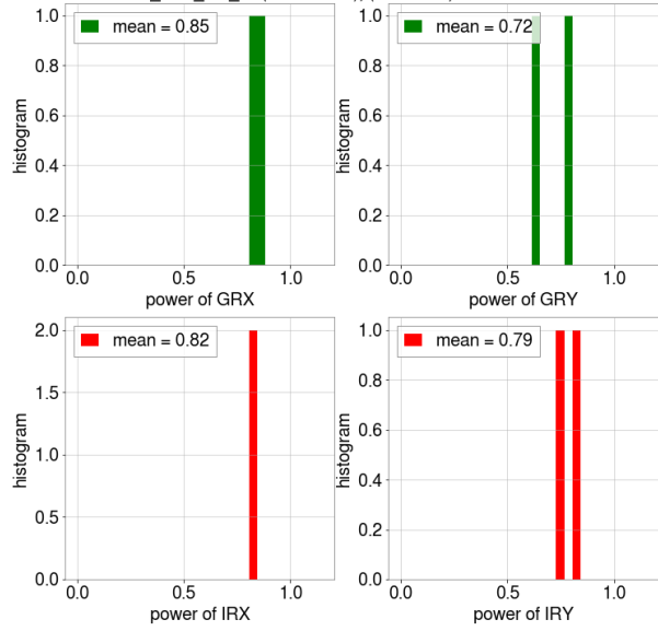
kloss from HANDOVER_ALS_TO_IR (state = 405), (n=2/1129)
