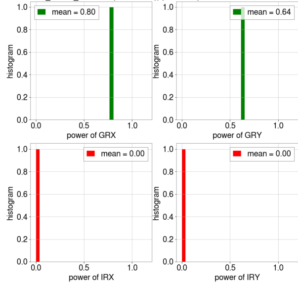
ckloss from ALS_CARM_LOCKED (state = 200), (n=1/1129)
