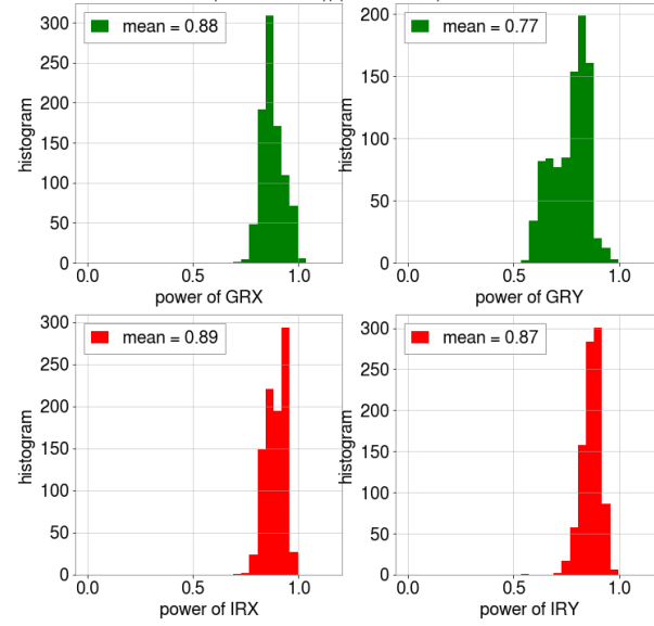
ockloss from OBSERVATION (state = 10000), (n=913/1129)
