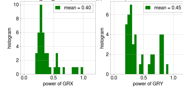
lockloss from ENGAGE_ALS_CARM (state = 110), (n=42/1129)
