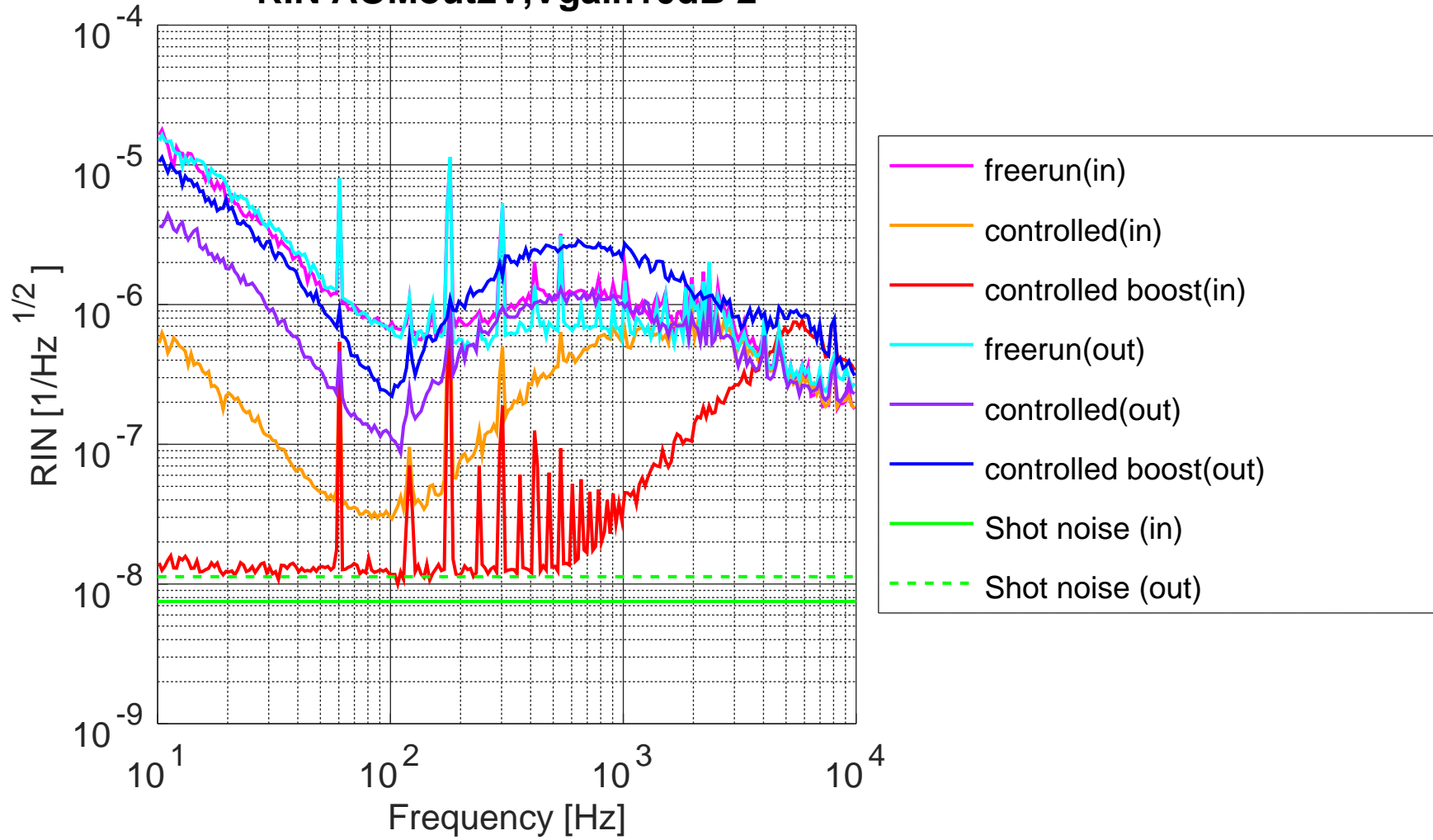
RIN AOMout2V,Vgain10dB 2
