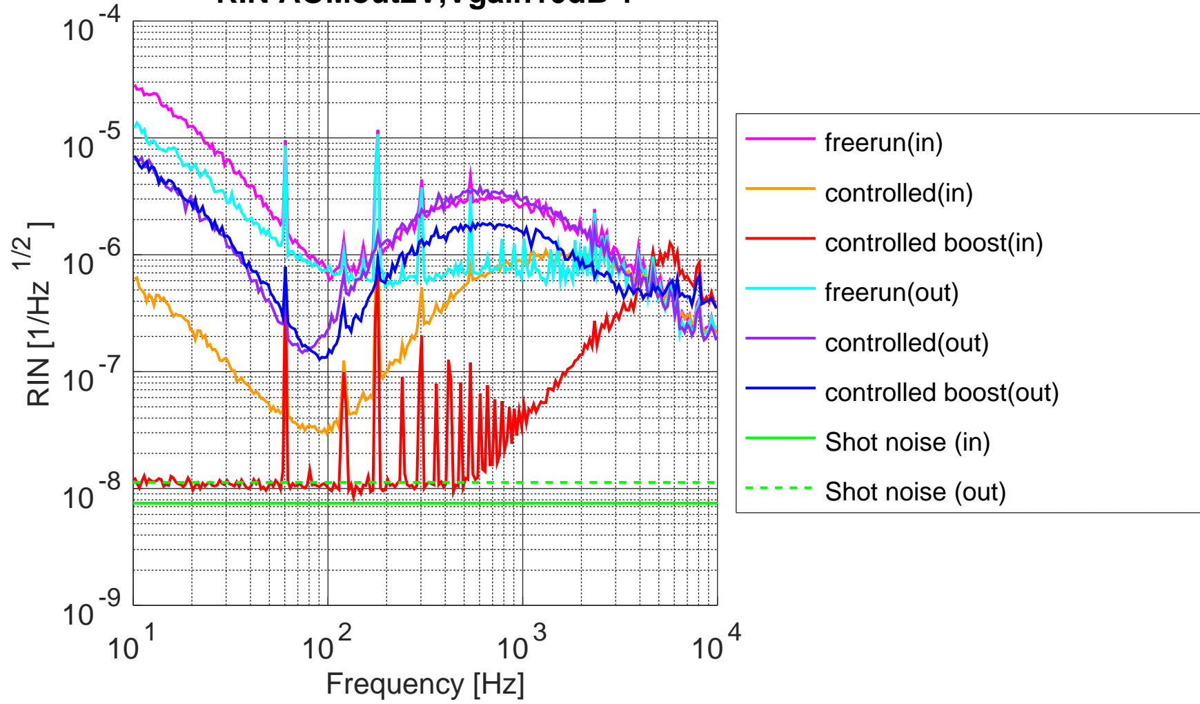
RIN AOMout2V,Vgain10dB 1
