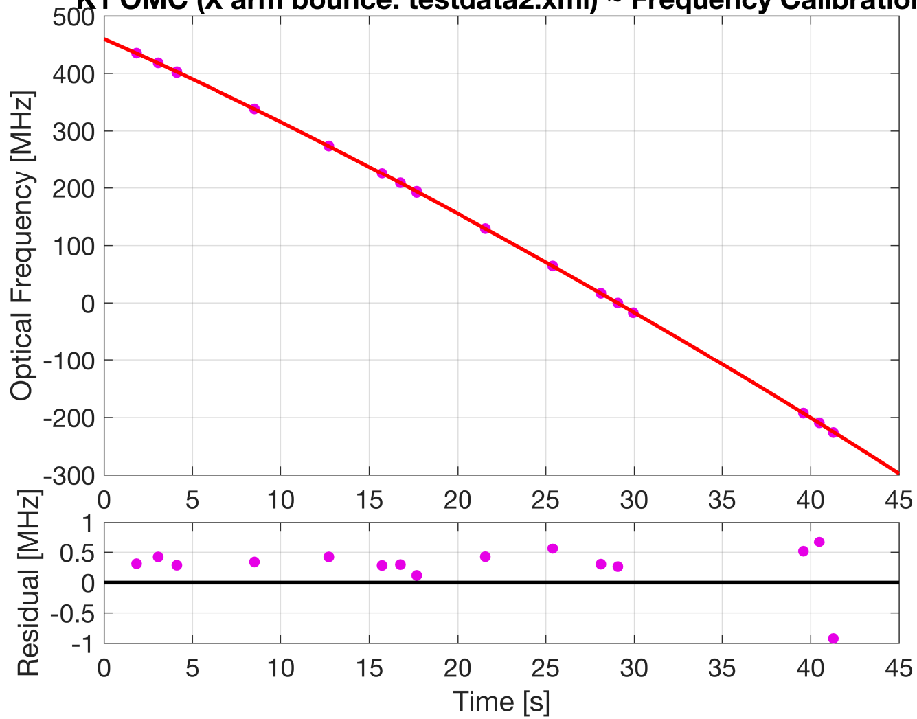
K1 OMC (X arm bounce: testdata2.xml) ~ Frequency Calibration
