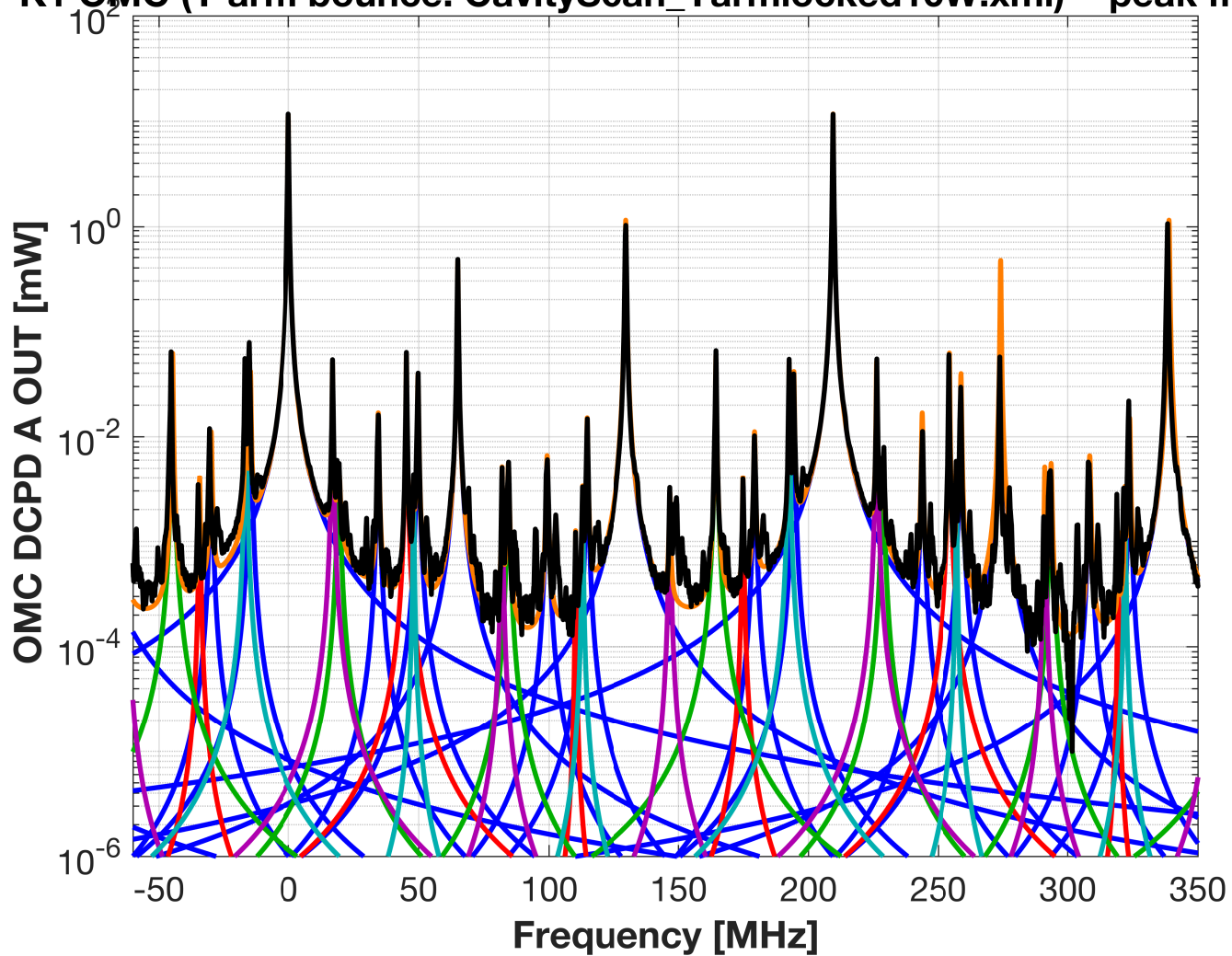
K1 OMC (Y arm bounce: CavityScan_Yarmlocked10W.xml) ~ peak fitting
