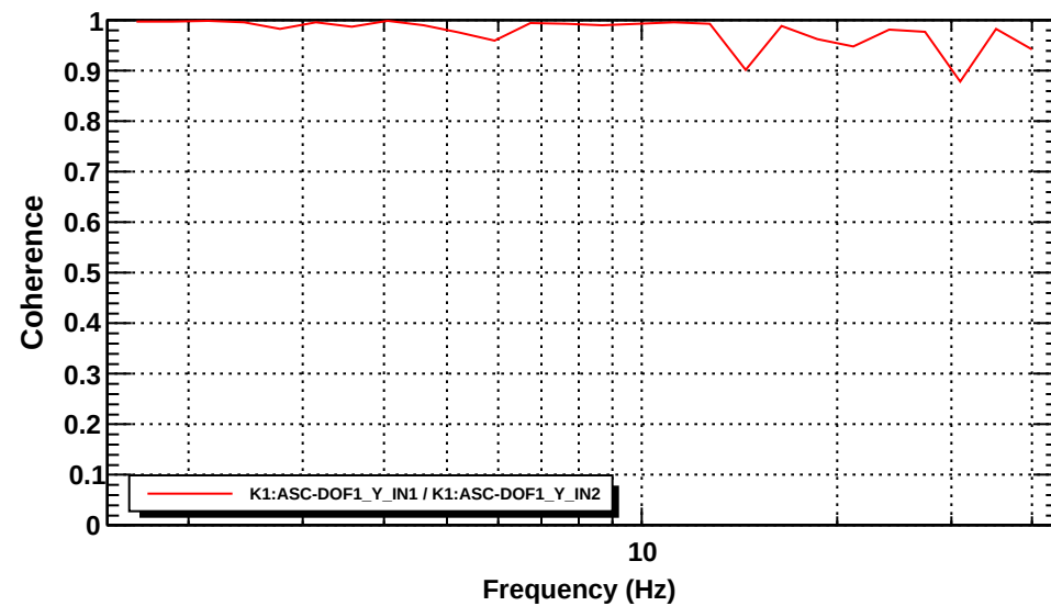
Coherence function
